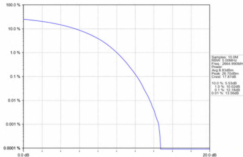
n41_15kHz_SISO_NTNV_50MHz_CP-OFDM 64 QAM_2664.99MHz_Outer_Full
