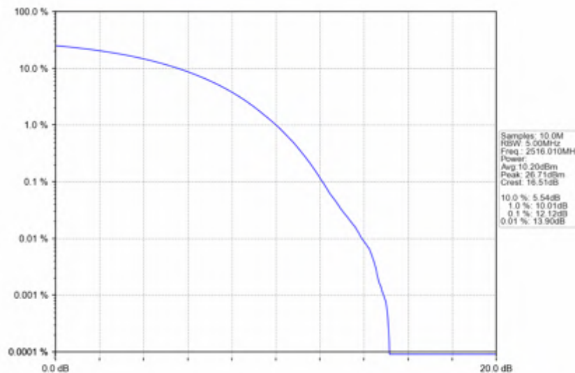
n41_15kHz_SISO_NTNV_40MHz_CP-OFDM QPSK_2516.01MHz_Outer_Full
