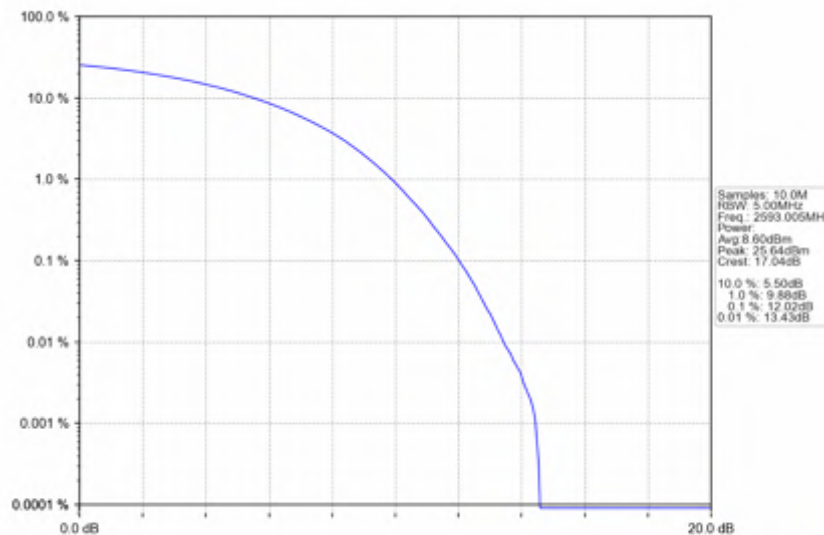
n41_15kHz_SISO_NTNV_50MHz_CP-OFDM 64 QAM_2593.005MHz_Outer_Full
