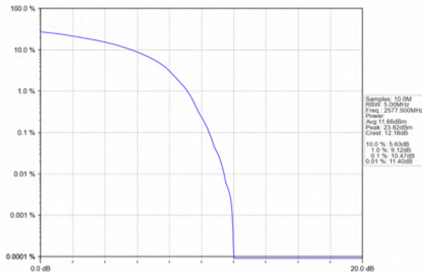
n38_30kHz_SISO_NTNV_15MHz_DFT-s-OFDM_256_QAM_2577.5MHz_Outer_Full
