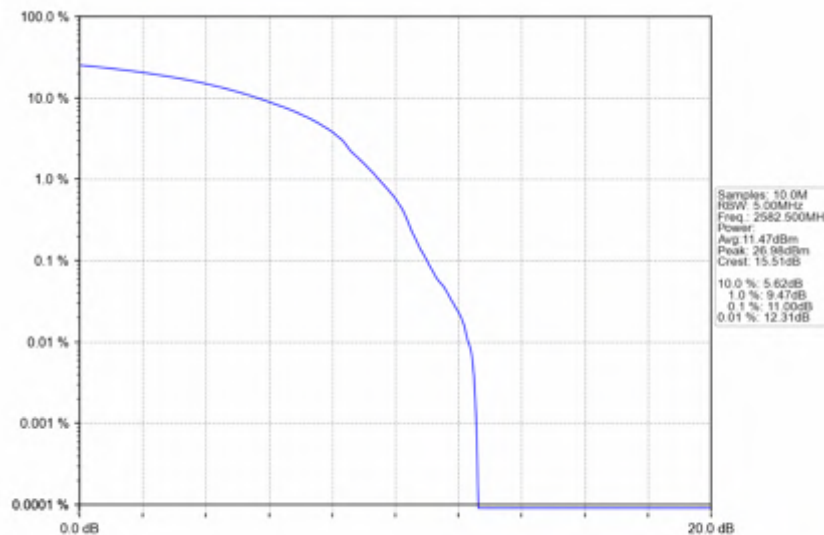
n38_30kHz_SISO_NTNV_25MHz_DFT-s-OFDM_16_QAM_2582.5MHz_Outer_Full
