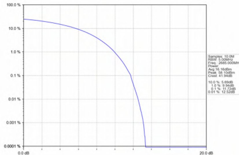
n41_15kHz_SISO_NTNV_10MHz_CP-OFDM QPSK_2685MHz_Outer_Full
