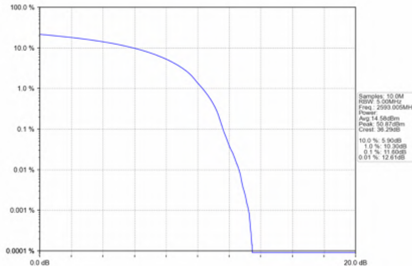
n41_15kHz_SISO_NTNV_20MHz_DFT-s-OFDM QPSK_2593.005MHz_Outer_Full
