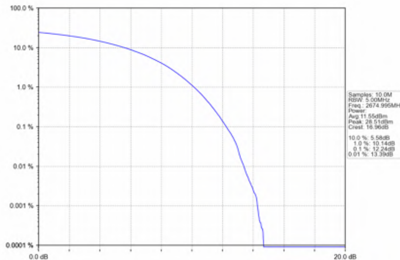
n41_15kHz_SISO_NTNV_30MHz_CP-OFDM 16 QAM_2674.995MHz_Outer_Full
