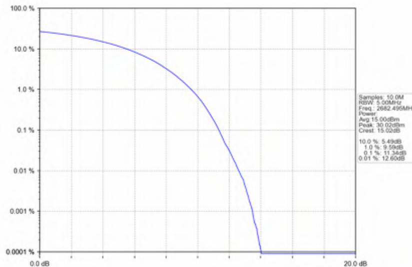
n41_15kHz_SISO_NTNV_15MHz_CP-OFDM_QPSK_2682.495MHz_Outer_Full
