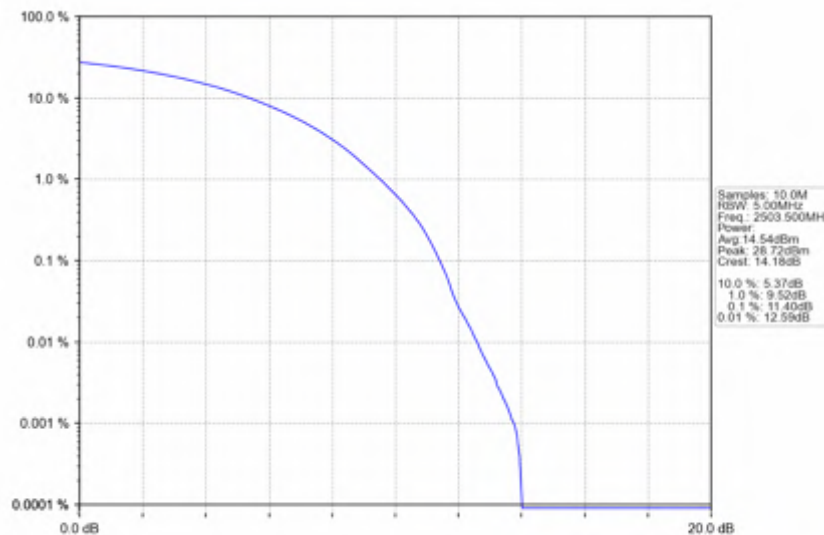
n41_15kHz_SISO_NTNV_15MHz_CP-OFDM 64 QAM_2503.5MHz_Outer_Full
