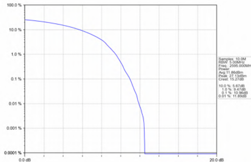
n38_30kHz_SISO_NTNV_30MHz_DFT-s-OFDM QPSK_2595MHz_Outer_Full
