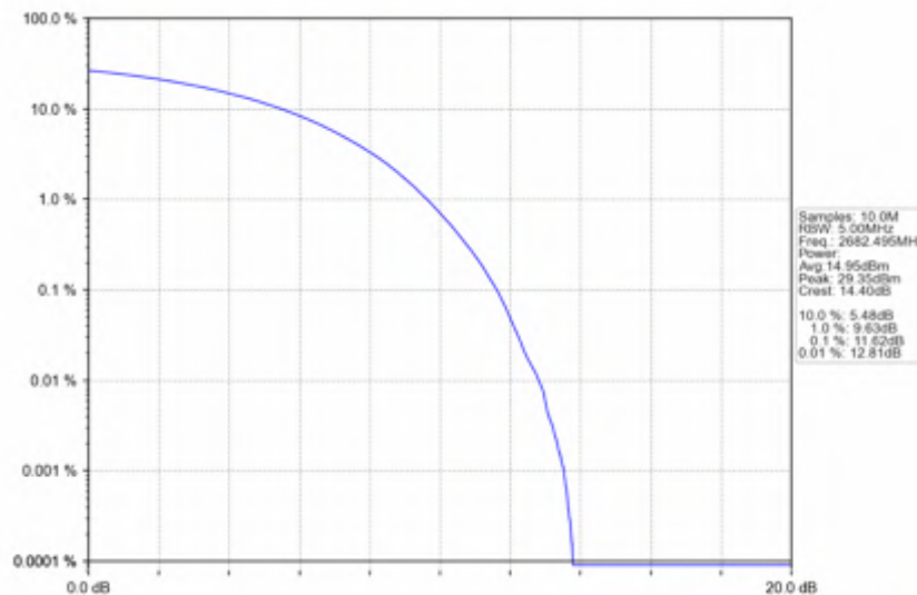
n41_15kHz_SISO_NTNV_15MHz_CP-OFDM 16 QAM_2682.495MHz_Outer_Full
