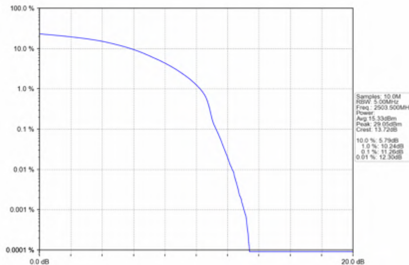
n41_15kHz_SISO_NTNV_15MHz_DFT-s-OFDM_16_QAM_2503.5MHz_Outer_Full
