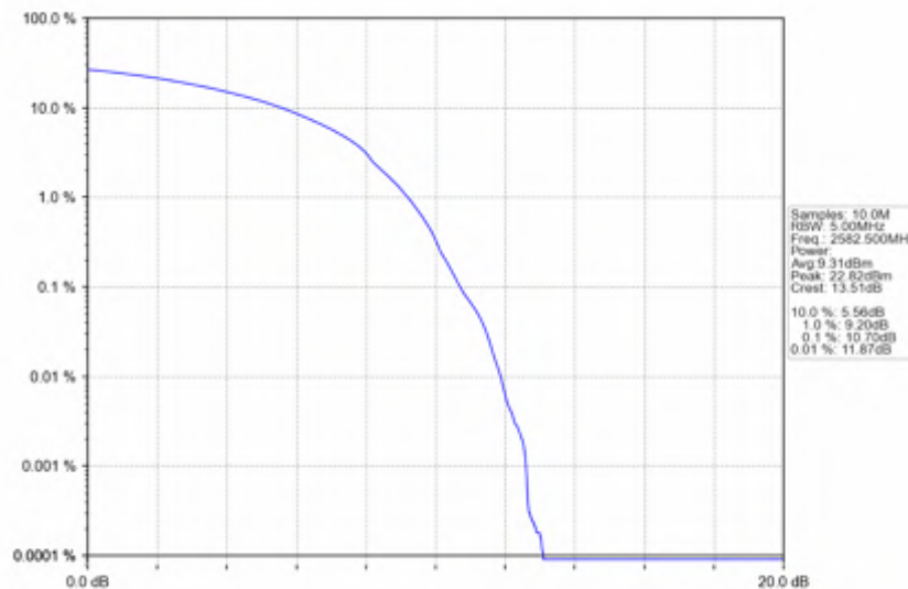
n38_30kHz_SISO_NTNV_25MHz_DFT-s-OFDM_256_QAM_2582.5MHz_Outer_Full
