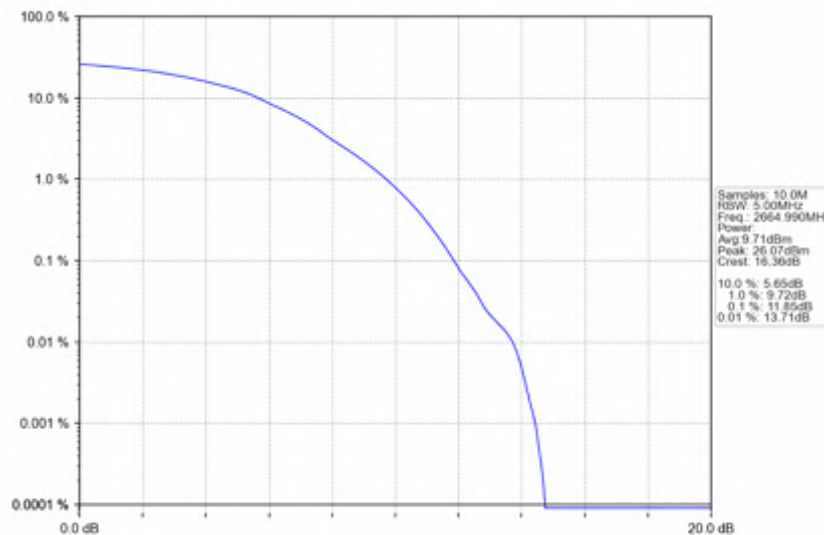
n41_15kHz_SISO_NTNV_50MHz_DFT-s-OFDM 64 QAM_2664.99MHz_Outer_Full
