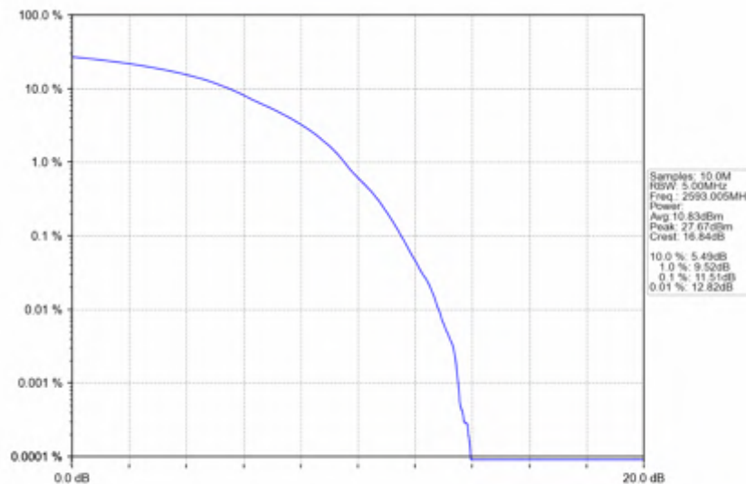
n41_15kHz_SISO_NTNV_40MHz_DFT-s-OFDM 64 QAM_2593.005MHz_Outer_Full
