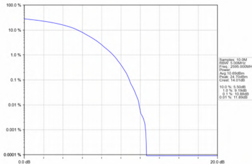
n38_30kHz_SISO_NTNV_40MHz_DFT-s-OFDM QPSK_2595MHz_Outer_Full
