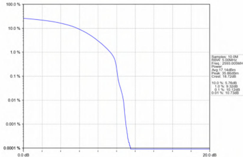
n41_15kHz_SISO_NTNV_15MHz_DFT-s-OFDM QPSK_2593.005MHz_Outer_Full
