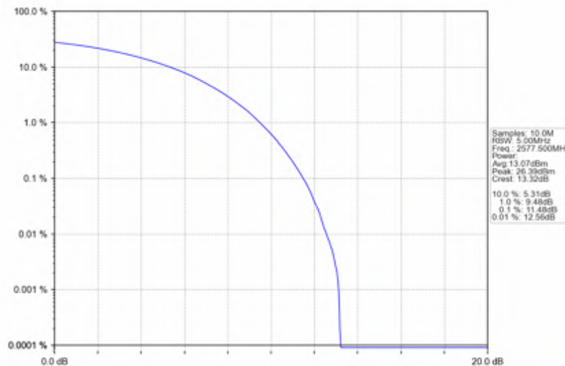
n38_30kHz_SISO_NTNV_15MHz_CP-OFDM_QPSK_2577.5MHz_Outer_Full
