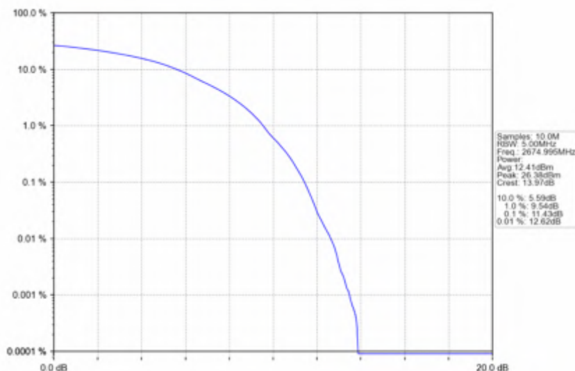
n41_15kHz_SISO_NTNV_30MHz_DFT-s-OFDM 64 QAM_2674.995MHz_Outer_Full
