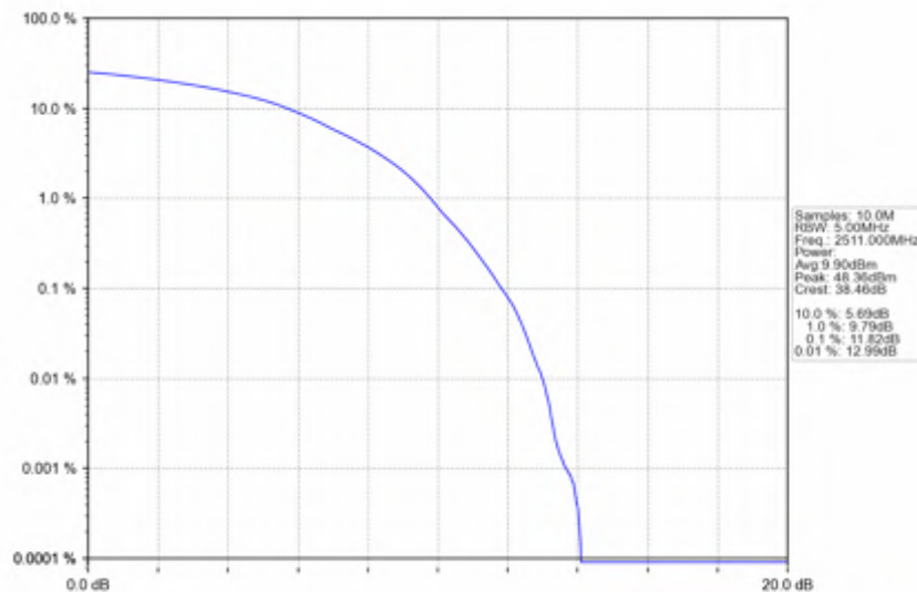
n41_15kHz_SISO_NTNV_30MHz_DFT-s-OFDM_256_QAM_2511MHz_Outer_Full
