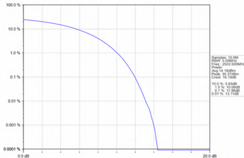
n41 15kHz SISO NTNV 15MHz CP-OFDM QPSK 2503.5MHz Outer Full
