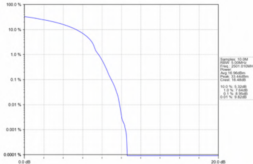
n41_30kHz_SISO_NTNV_10MHz_DFT-s-OFDM_16_QAM_2501.01MHz_Outer_Full
