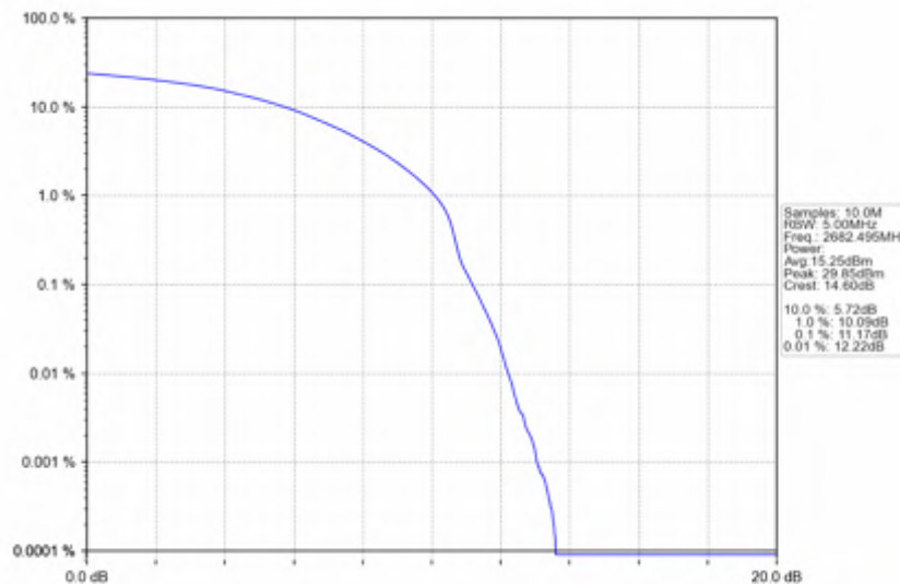
n41_15kHz_SISO_NTNV_15MHz_DFT-s-OFDM 64 QAM_2682.495MHz_Outer_Full
