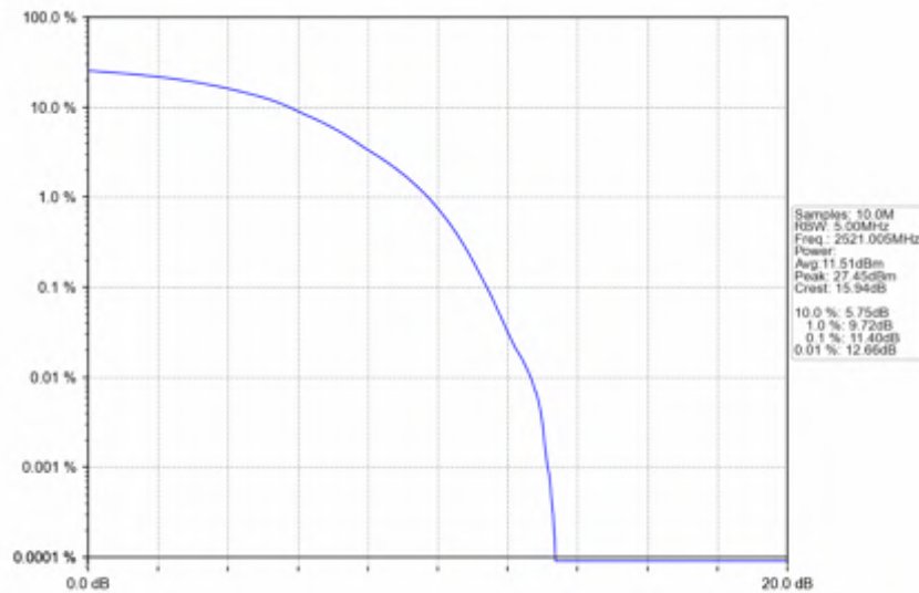
n41_15kHz_SISO_NTNV_50MHz_DFT-s-OFDM_PI/2_BPSK_2521.005MHz_Outer_Full
