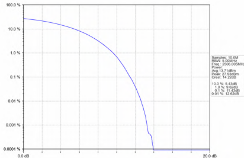
n41_15kHz_SISO_NTNV_20MHz_CP-OFDM_16 QAM_2506.005MHz_Outer_Full
