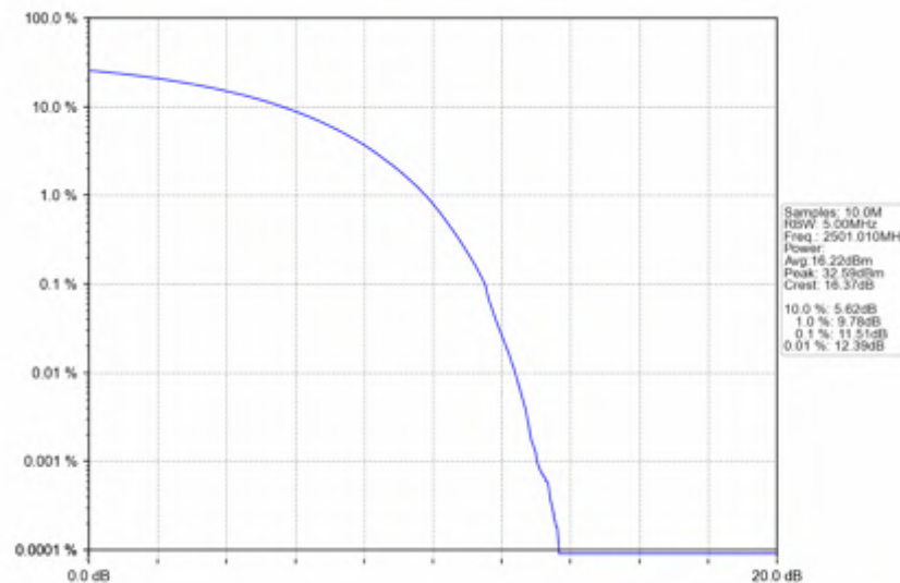
n41_15kHz_SISO_NTNV_10MHz_CP-OFDM_16_QAM_2501.01MHz_Outer_Full
