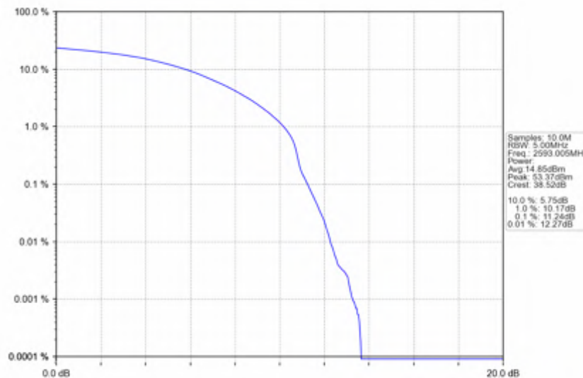
n41_15kHz_SISO_NTNV_15MHz_DFT-s-OFDM 64 QAM_2593.005MHz_Outer_Full
