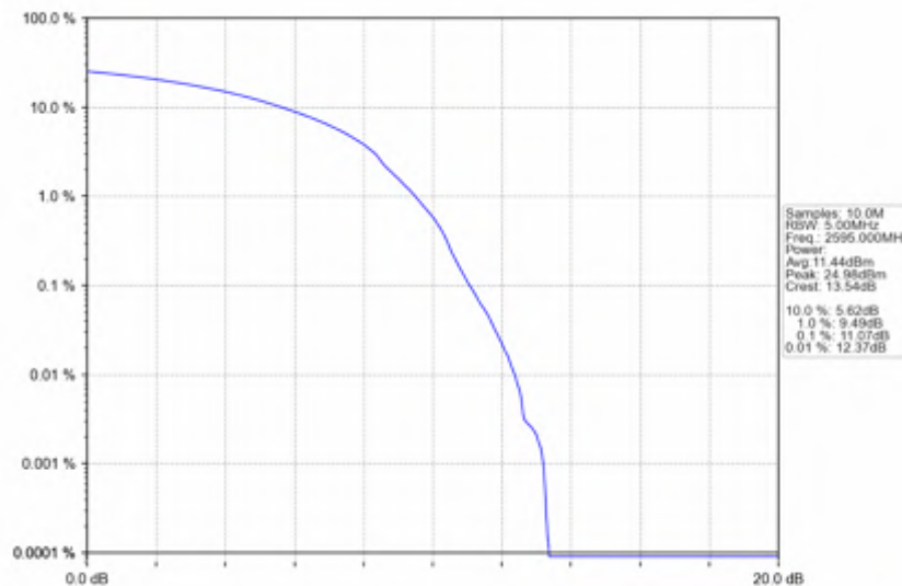
n38_30kHz_SISO_NTNV_25MHz_DFT-s-OFDM_16_QAM_2595MHz_Outer_Full
