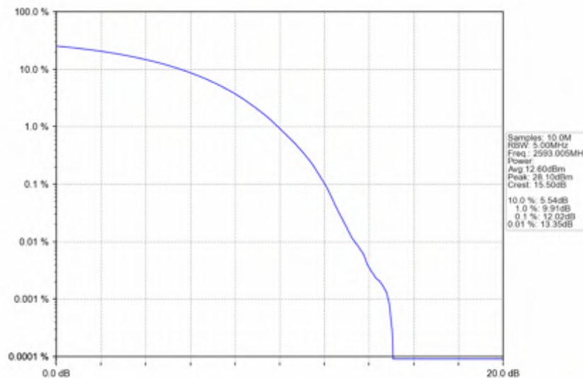
n41_15kHz_SISO_NTNV_20MHz_CP-OFDM 64 QAM_2593.005MHz_Outer_Full
