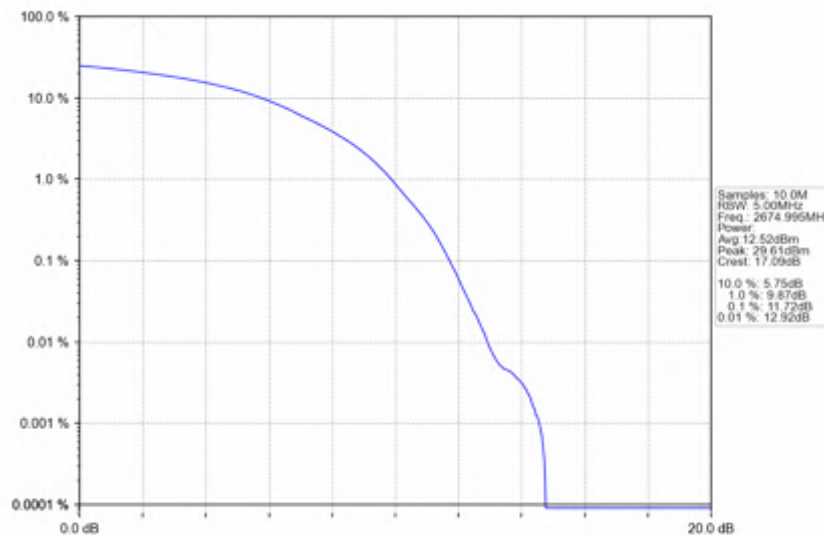
n41_15kHz_SISO_NTNV_30MHz_DFT-s-OFDM 16 QAM_2674.995MHz_Outer_Full
