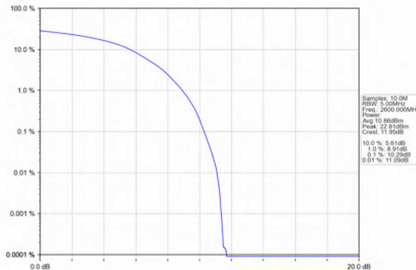
n38_30kHz_SISO_NTNV_40MHz_DFT-s-OFDM_PI/2_BPSK_2600MHz_Outer_Full
