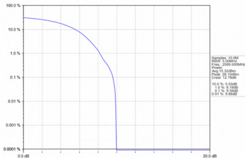
n38_30kHz_SISO_NTNV_15MHz_DFT-s-OFDM PI/2 BPSK_2595MHz_Outer_Full
