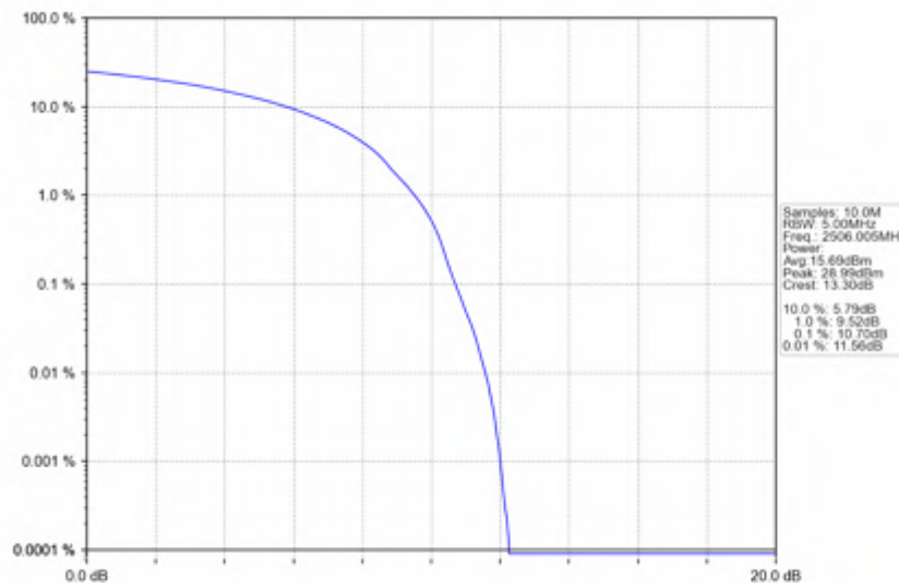
n41_15kHz_SISO_NTNV_20MHz_DFT-s-OFDM QPSK_2506.005MHz_Outer_Full
