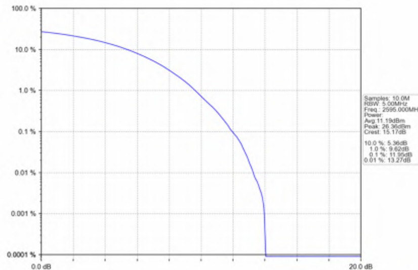
n38_30kHz_SISO_NTNV_10MHz_CP-OFDM_256_QAM_2595MHz_Outer_Full
