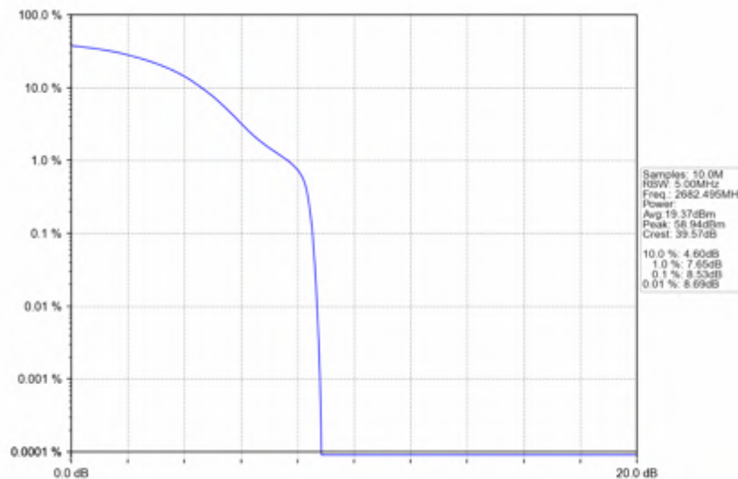
n41_15kHz_SISO_NTNV_15MHz_DFT-s-OFDM PI/2 BPSK_2682.495MHz_Outer_Full
