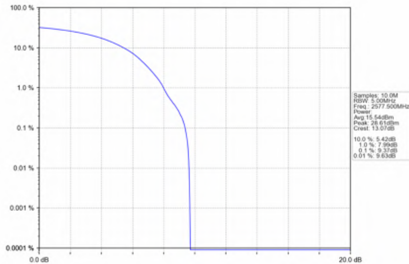
n38_30kHz_SISO_NTNV_15MHz_DFT-s-OFDM PI/2 BPSK_2577.5MHz_Outer_Full
