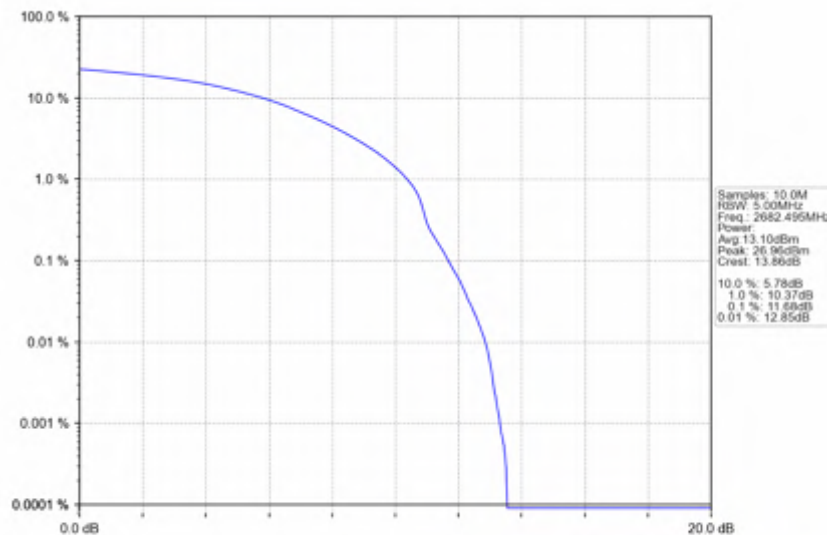
n41_15kHz_SISO_NTNV_15MHz_DFT-s-OFDM_256_QAM_2682.495MHz_Outer_Full
