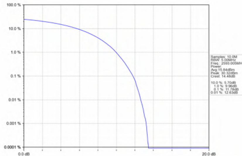
n41_15kHz_SISO_NTNV_10MHz_CP-OFDM QPSK_2593.005MHz_Outer_Full
