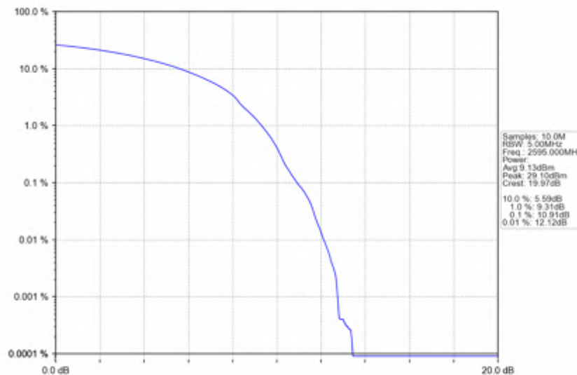
n38_30kHz_SISO_NTNV_25MHz_DFT-s-OFDM_256_QAM_2595MHz_Outer_Full
