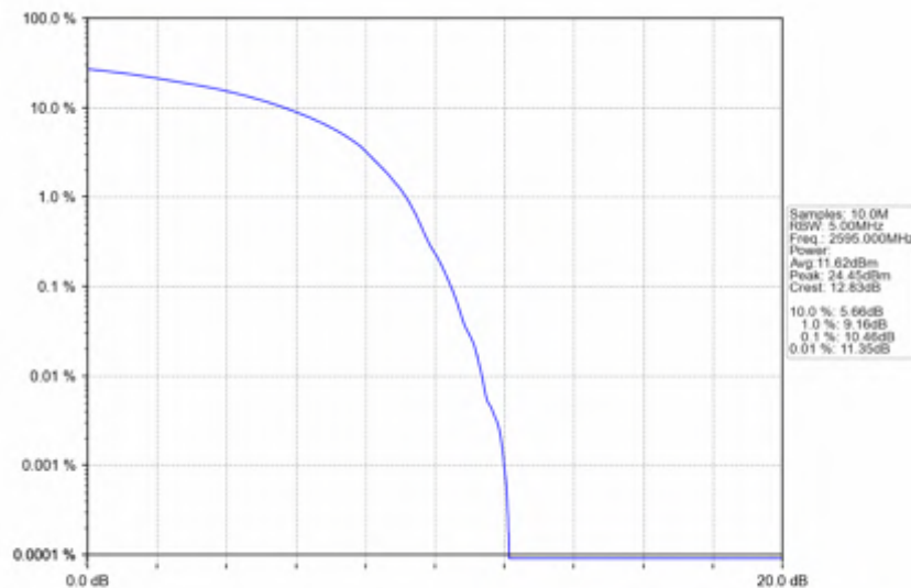
n38_30kHz_SISO_NTNV_15MHz_DFT-s-OFDM_256_QAM_2595MHz_Outer_Full
