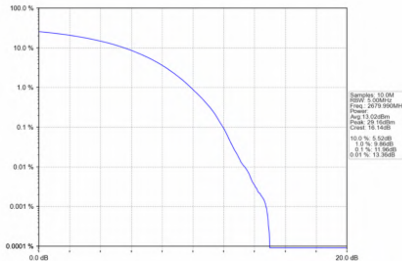
n41_15kHz_SISO_NTNV_20MHz_CP-OFDM 64 QAM_2679.99MHz_Outer_Full
