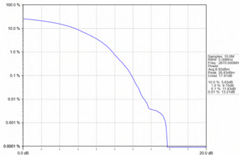
n41_15kHz_SISO_NTNV_40MHz_DFT-s-OFDM 256 QAM_2670MHz_Outer_Full
