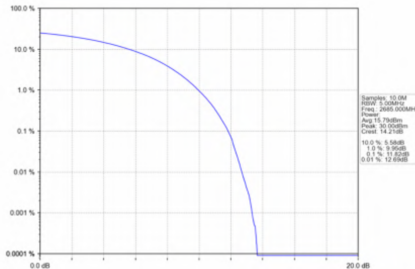
n41_15kHz_SISO_NTNV_10MHz_CP-OFDM 64 QAM_2685MHz_Outer_Full
