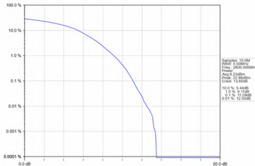
n38_30kHz_SISO_NTNV_40MHz_DFT-s-OFDM_64_QAM_2600MHz_Outer_Full
