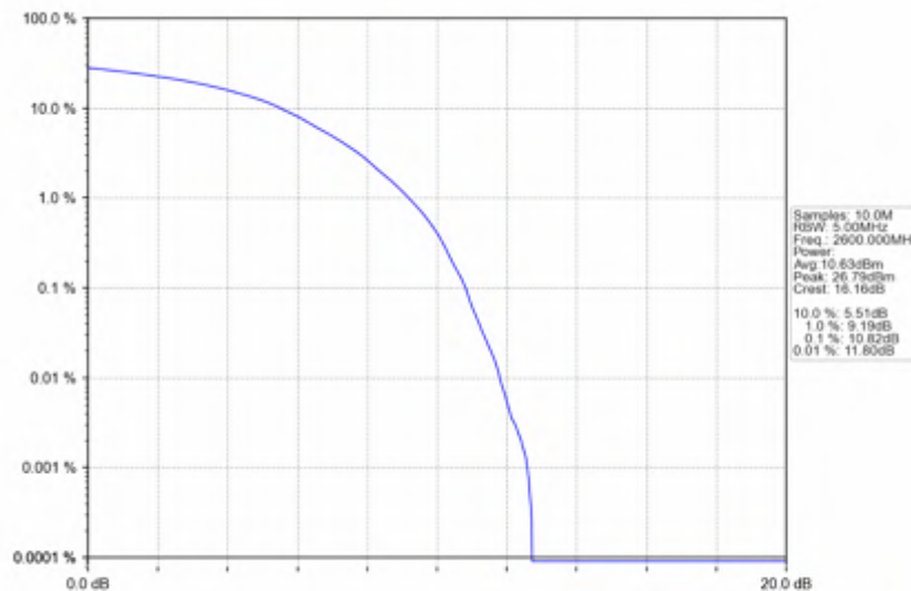
n38_30kHz_SISO_NTNV_40MHz_DFT-s-OFDM QPSK_2600MHz_Outer_Full
