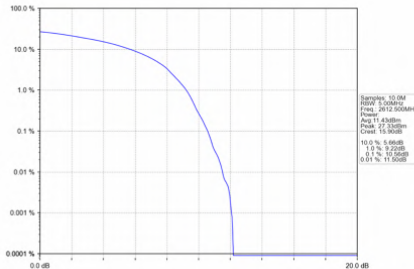
n38_30kHz_SISO_NTNV_15MHz_DFT-s-OFDM_256_QAM_2612.5MHz_Outer_Full
