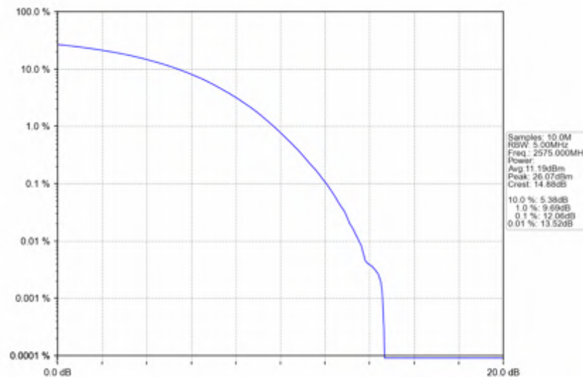
n38_30kHz_SISO_NTNV_10MHz_CP-OFDM_256_QAM_2575MHz_Outer_Full
