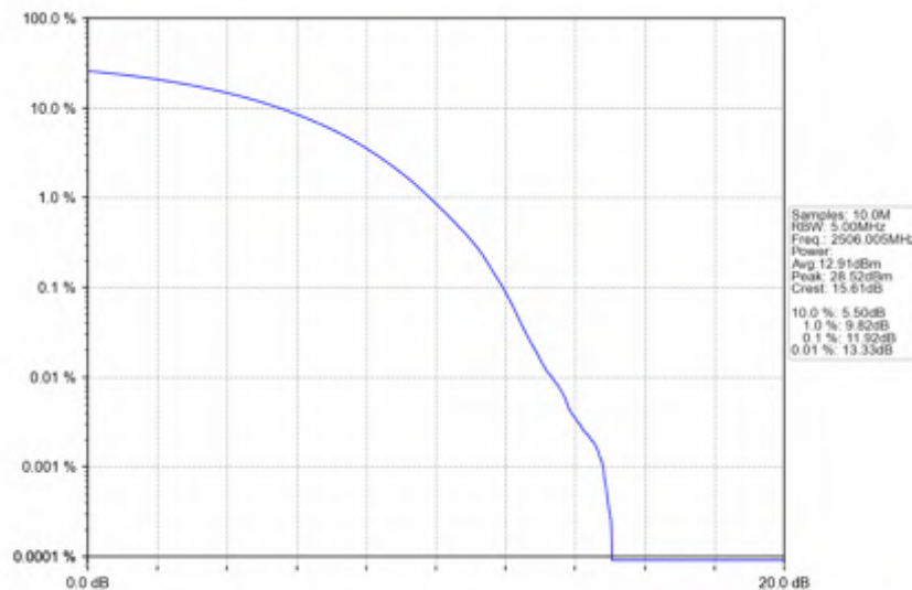
n41_15kHz_SISO_NTNV_20MHz_CP-OFDM 64 QAM_2506.005MHz_Outer_Full
