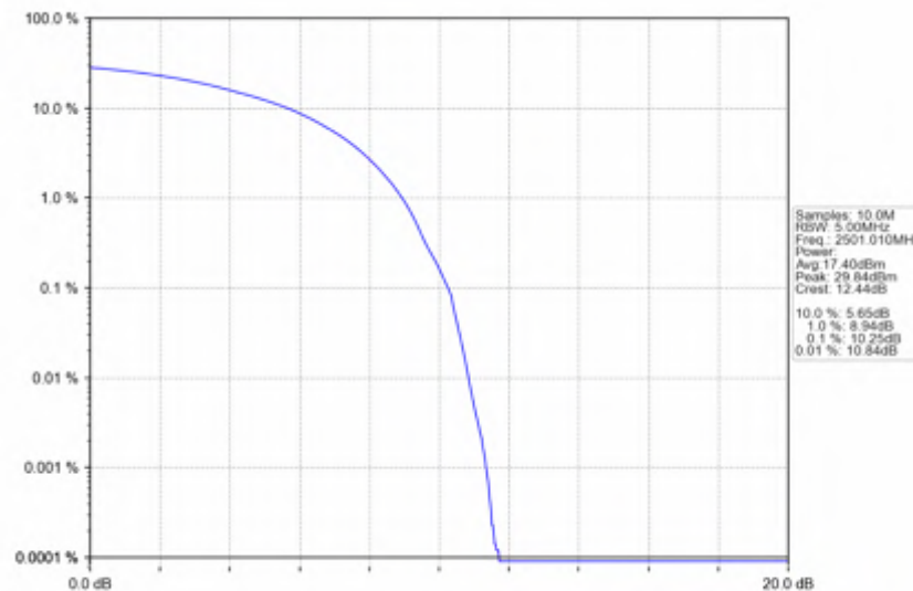
n41_15kHz_SISO_NTNV_10MHz_DFT-s-OFDM_64_QAM_2501.01MHz_Outer_Full
