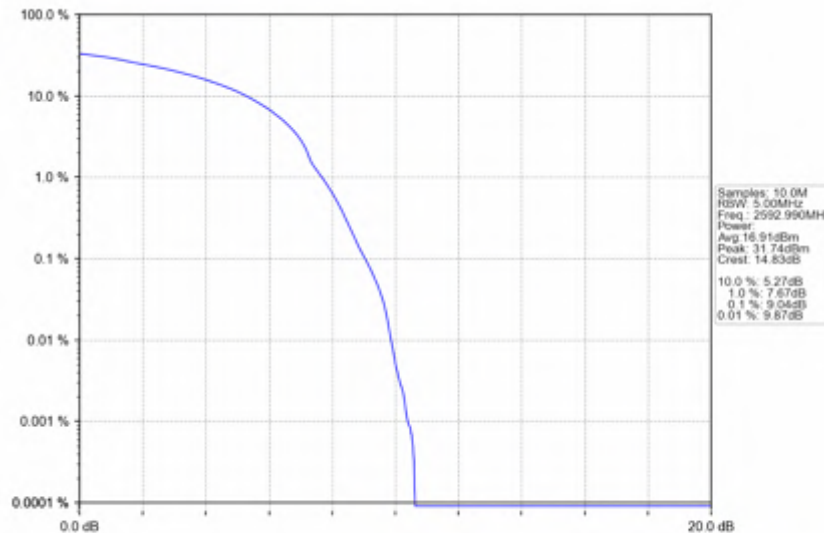
n41_30kHz_SISO_NTNV_10MHz_DFT-s-OFDM_16_QAM_2592.99MHz_Outer_Full
