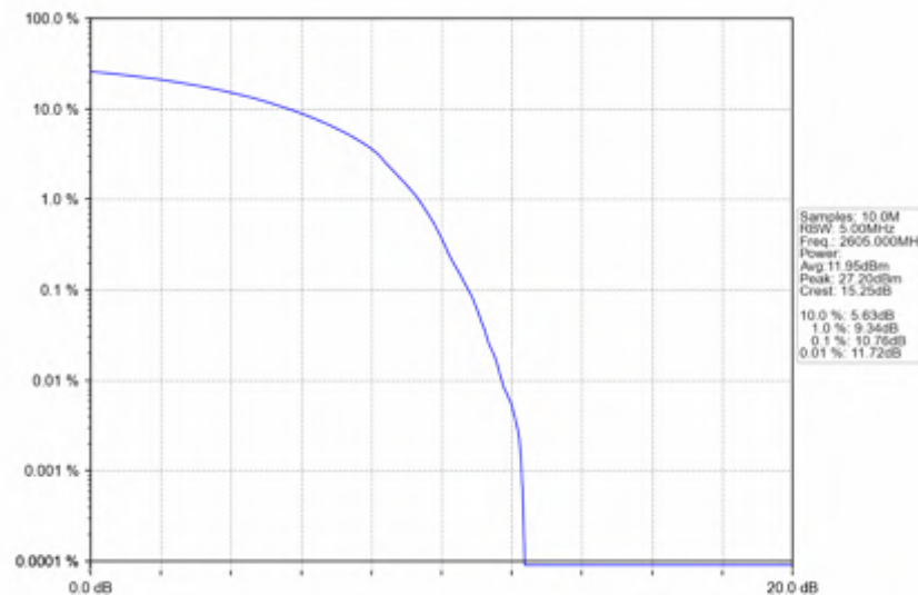
n38_30kHz_SISO_NTNV_30MHz_DFT-s-OFDM QPSK_2605MHz_Outer_Full
