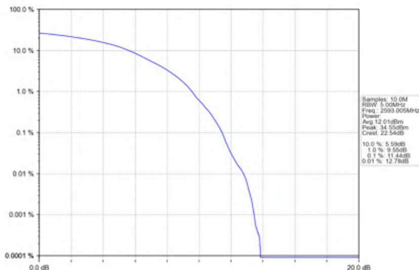
n41_15kHz_SISO_NTNV_30MHz_DFT-s-OFDM 64 QAM_2593.005MHz_Outer_Full
