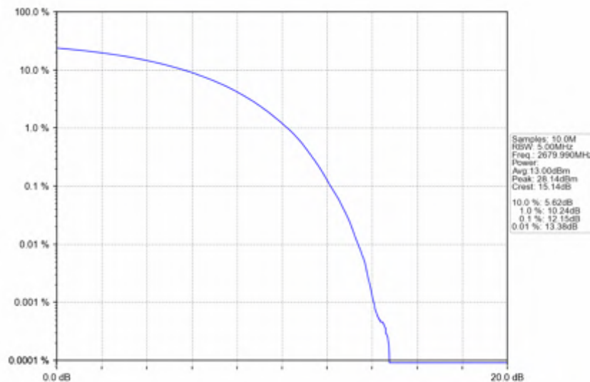
n41_15kHz_SISO_NTNV_20MHz_CP-OFDM 16 QAM_2679.99MHz_Outer_Full
