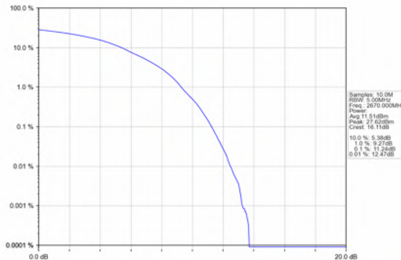
n41_15kHz_SISO_NTNV_40MHz_DFT-s-OFDM 64 QAM_2670MHz_Outer_Full
