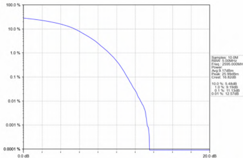
n38_30kHz_SISO_NTNV_40MHz_DFT-s-OFDM_64_QAM_2595MHz_Outer_Full
