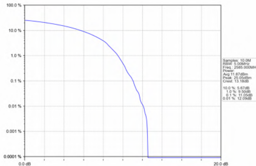
n38_30kHz_SISO_NTNV_30MHz_DFT-s-OFDM QPSK_2585MHz_Outer_Full
