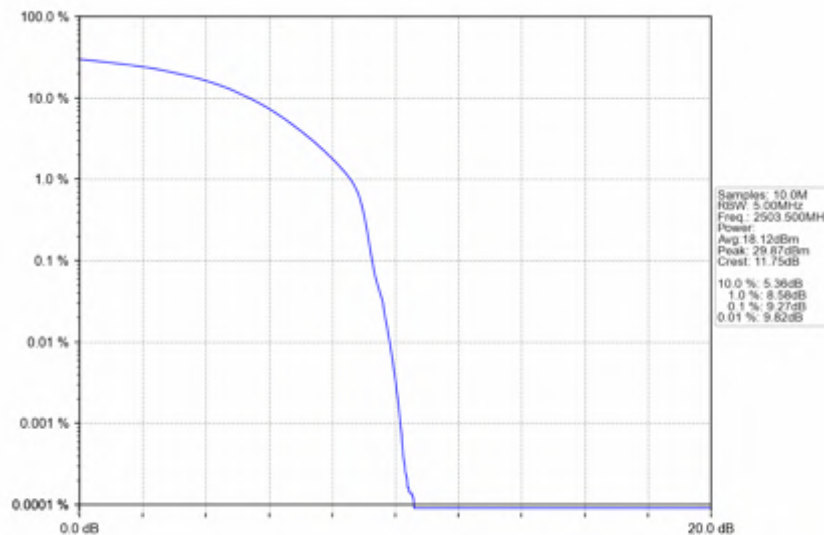
n41_15kHz_SISO_NTNV_15MHz_DFT-s-OFDM QPSK_2503.5MHz_Outer_Full
