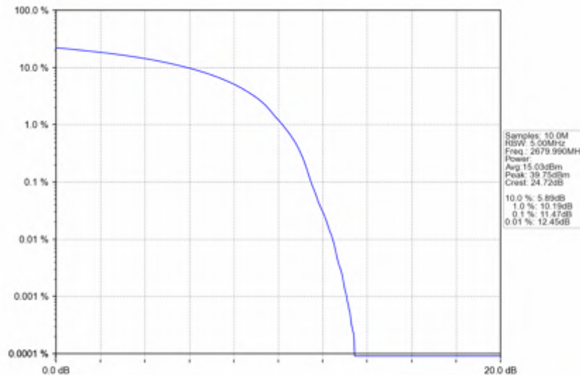
n41_15kHz_SISO_NTNV_20MHz_DFT-s-OFDM QPSK_2679.99MHz_Outer_Full
