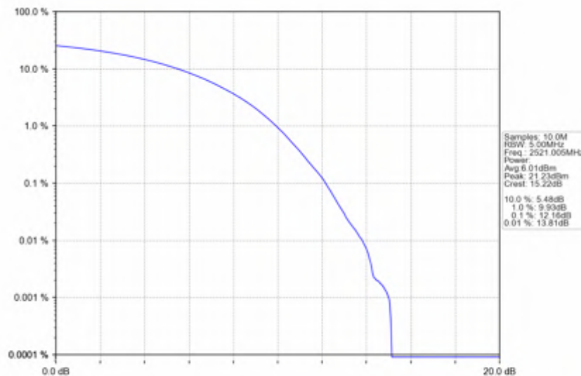
n41_15kHz_SISO_NTNV_50MHz_CP-OFDM_256_QAM_2521.005MHz_Outer_Full
