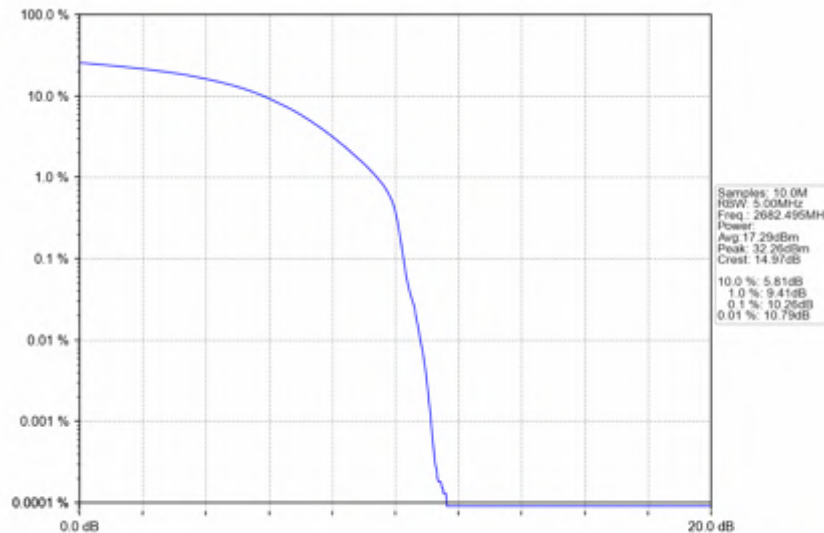
n41_15kHz_SISO_NTNV_15MHz_DFT-s-OFDM QPSK_2682.495MHz_Outer_Full
