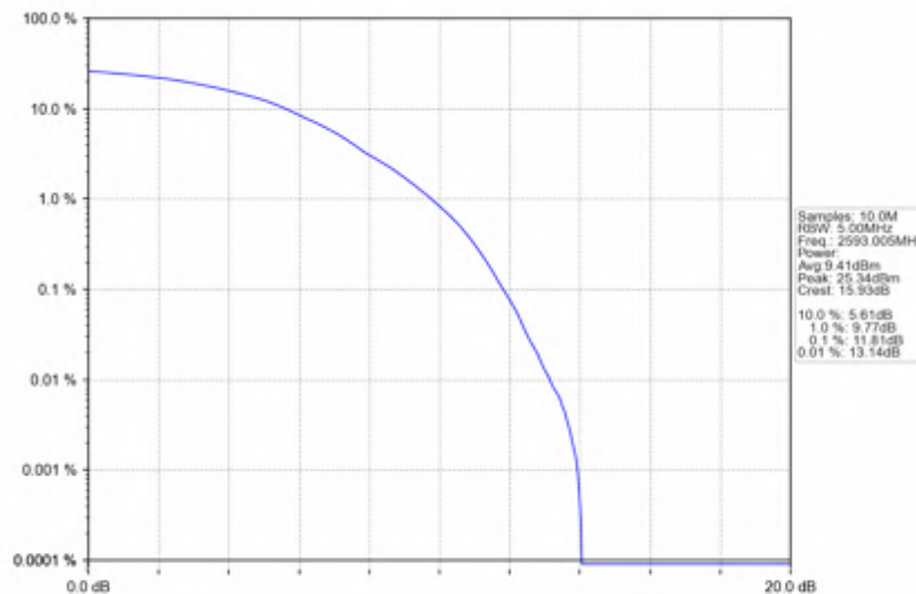
n41_15kHz_SISO_NTNV_50MHz_DFT-s-OFDM 64 QAM_2593.005MHz_Outer_Full
