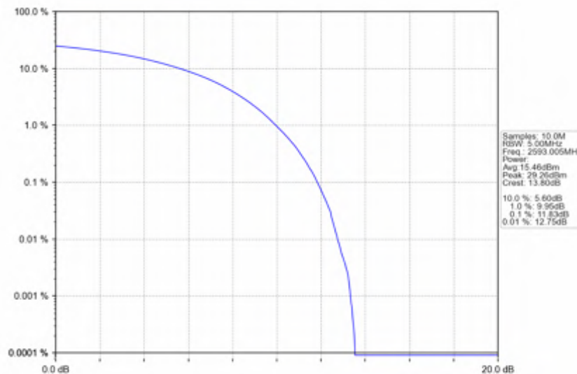
n41_15kHz_SISO_NTNV_10MHz_CP-OFDM 64 QAM_2593.005MHz_Outer_Full
