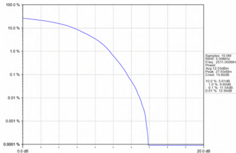
n41_15kHz_SISO_NTNV_30MHz_DFT-s-OFDM 64 QAM_2511MHz_Outer_Full
