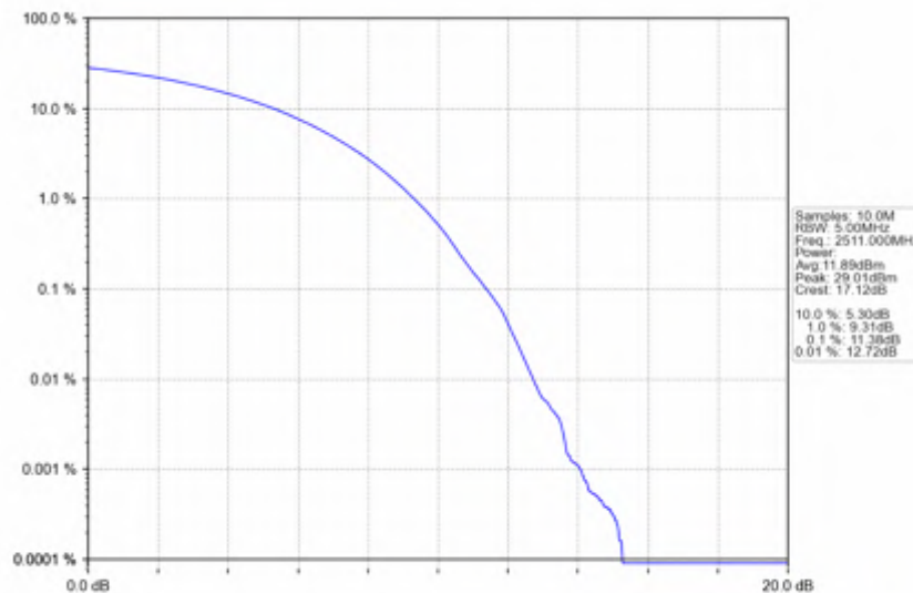
n41_15kHz_SISO_NTNV_30MHz_CP-OFDM 64 QAM_2511MHz_Outer_Full
