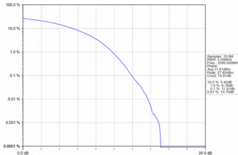
n38_15kHz_SISO_NTNV_15MHz_CP-OFDM_64_QAM_2595MHz_Outer_Full
