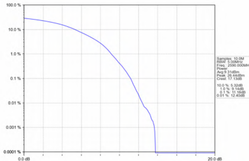
n38_15kHz_SISO_NTNV_40MHz_DFT-s-OFDM_16_QAM_2590MHz_Outer_Full
