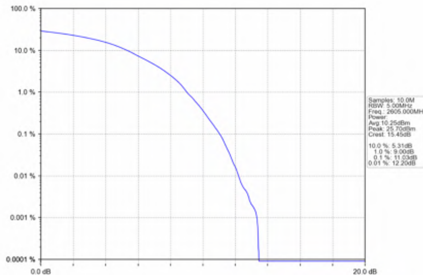
n38_15kHz_SISO_NTNV_30MHz_DFT-s-OFDM_64_QAM_2605MHz_Outer_Full
