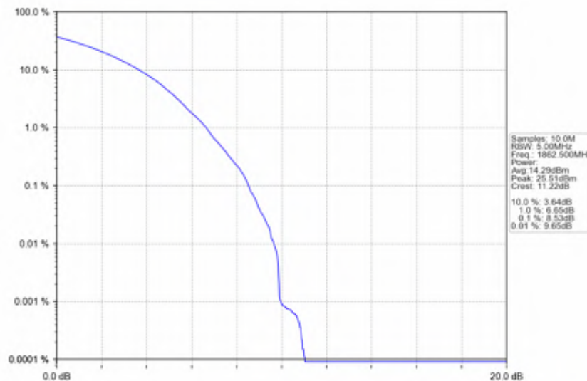
n25_30kHz_SISO_NTNV_25MHz_CP-OFDM_QPSK_1862.5MHz_Outer_Full
