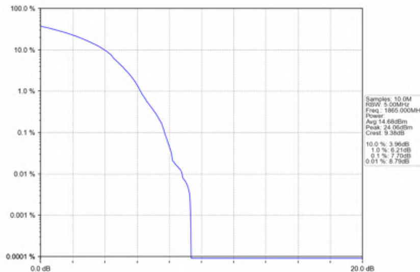
n25_30kHz_SISO_NTNV_30MHz_DFT-s-OFDM_16_QAM_1865MHz_Outer_Full
