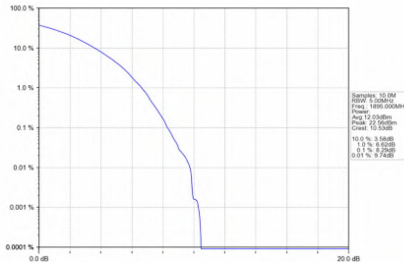
n25_30kHz_SISO_NTNV_40MHz_CP-OFDM QPSK_1895MHz_Outer_Full
