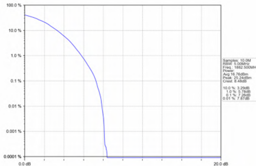
n25_30kHz_SISO_NTNV_20MHz_DFT-s-OFDM_16_QAM_1882.5MHz_Outer_Full
