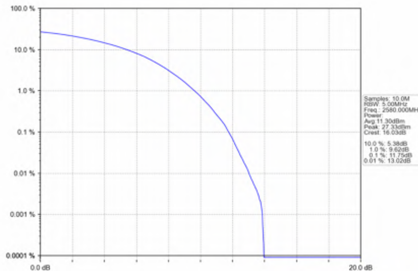
n38_15kHz_SISO_NTNV_20MHz_CP-OFDM_16_QAM_2580MHz_Outer_Full
