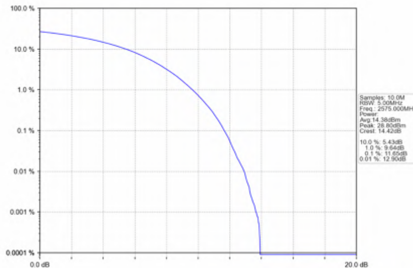
n38_15kHz_SISO_NTNV_10MHz_CP-OFDM_16_QAM_2575MHz_Outer_Full
