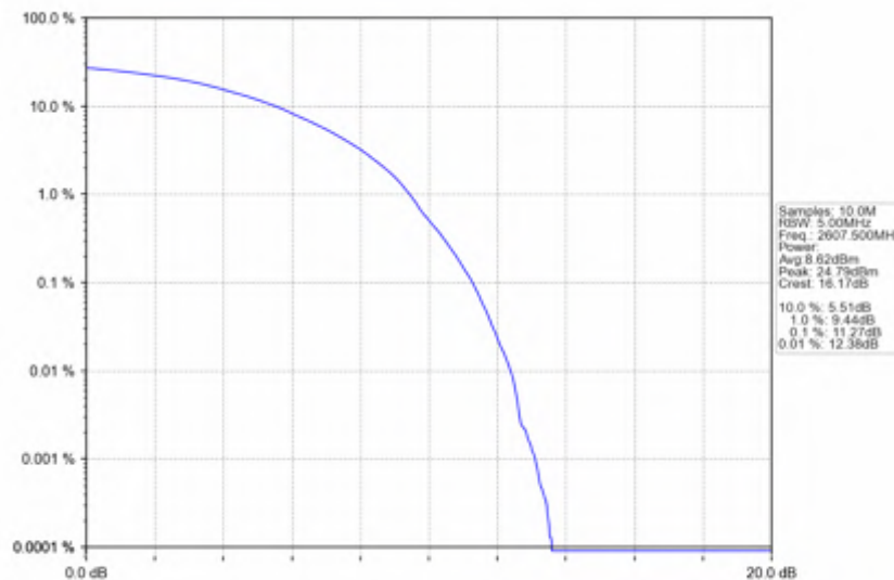
n38_15kHz_SISO_NTNV_25MHz_DFT-s-OFDM_256_QAM_2607.5MHz_Outer_Full
