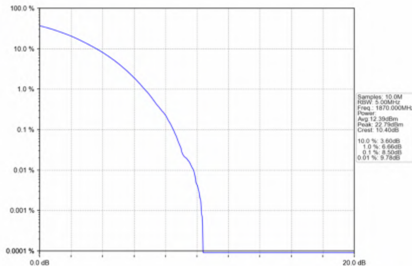
n25_30kHz_SISO_NTNV_40MHz_CP-OFDM QPSK_1870MHz_Outer_Full
