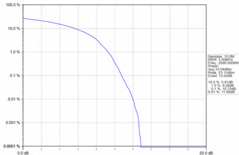
n38_15kHz_SISO_NTNV_20MHz_DFT-s-OFDM_256_QAM_2595MHz_Outer_Full
