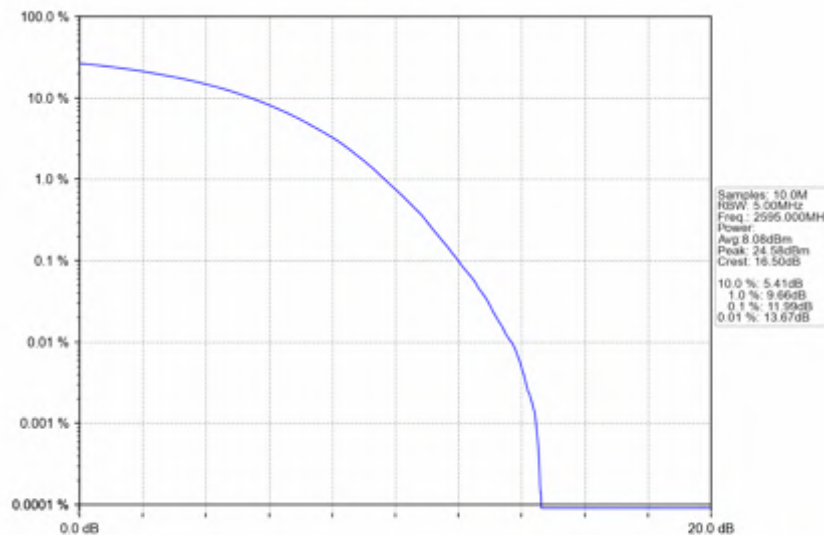
n38_15kHz_SISO_NTNV_40MHz_CP-OFDM QPSK_2595MHz_Outer_Full
