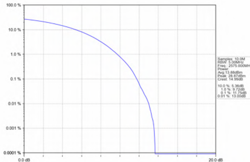
n38_15kHz_SISO_NTNV_10MHz_CP-OFDM 64 QAM_2575MHz_Outer_Full
