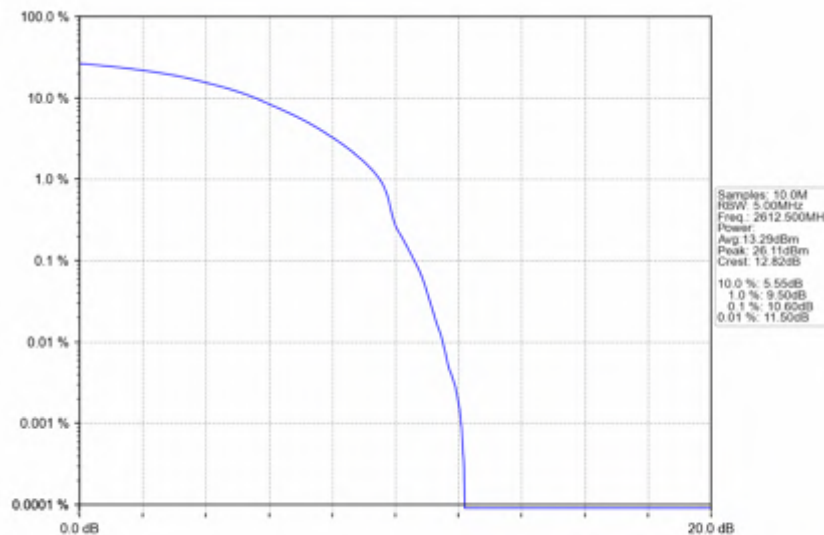
n38_15kHz_SISO_NTNV_15MHz_DFT-s-OFDM 64 QAM_2612.5MHz_Outer_Full
