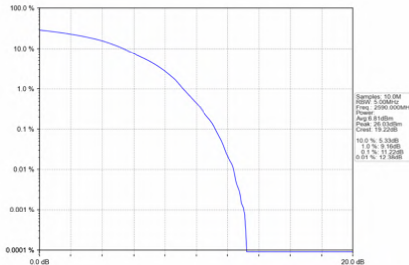
n38_15kHz_SISO_NTNV_40MHz_DFT-s-OFDM_256_QAM_2590MHz_Outer_Full
