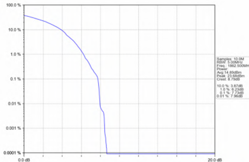
n25_30kHz_SISO_NTV_25MHz_DFT-s-OFDM 64 QAM_1862.5MHz_Outer_Full
