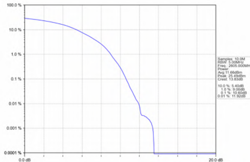
n38_15kHz_SISO_NTNV_30MHz_DFT-s-OFDM QPSK_2605MHz_Outer_Full
