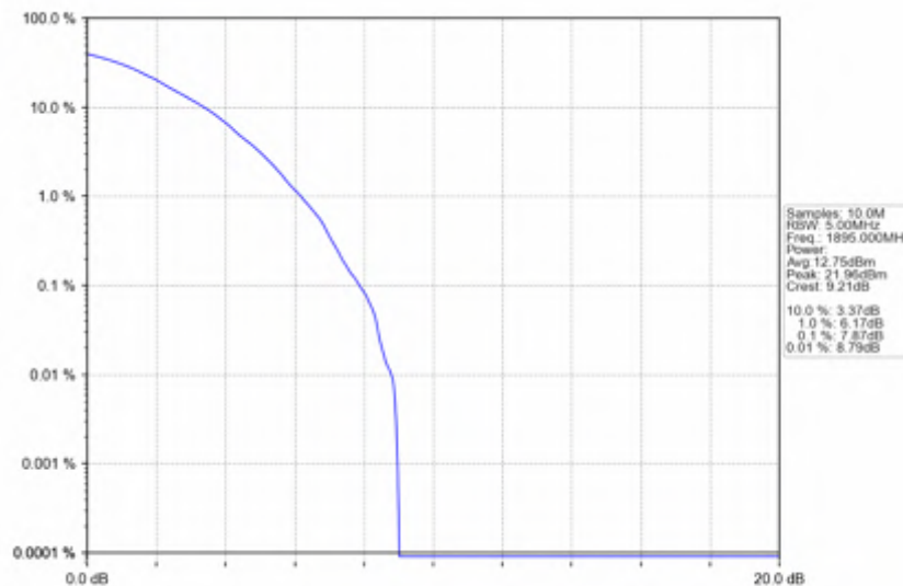
n25_30kHz_SISO_NTNV_40MHz_DFT-s-OFDM 64 QAM_1895MHz_Outer_Full
