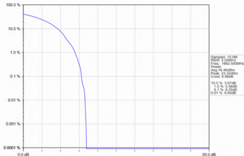
n25_30kHz_SISO_NTNV_30MHz_DFT-s-OFDM_PI/2_BPSK_1882.5MHz_Outer_Full
