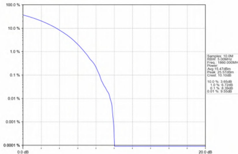
n25_30kHz_SISO_NTNV_20MHz_CP-OFDM_16_QAM_1860MHz_Outer_Full
