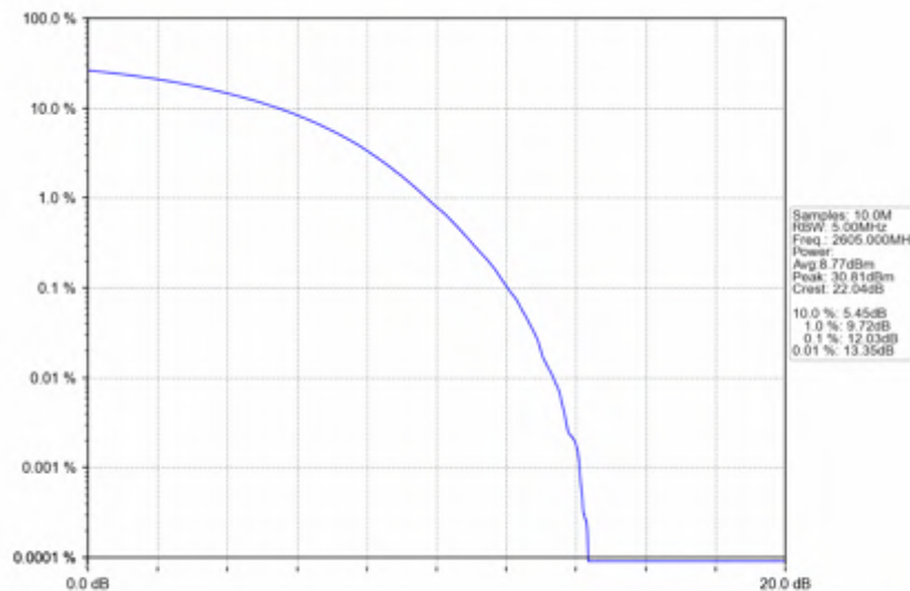
n38_15kHz_SISO_NTNV_30MHz_CP-OFDM 64 QAM_2605MHz_Outer_Full
