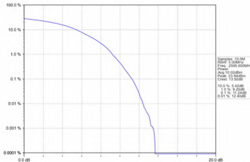
n38_15kHz_SISO_NTNV_30MHz_DFT-s-OFDM_64_QAM_2595MHz_Outer_Full
