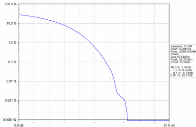
n38_15kHz_SISO_NTNV_20MHz_CP-OFDM 64 QAM_2595MHz_Outer_Full
