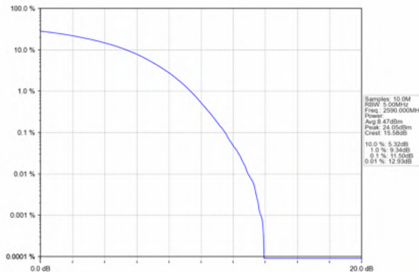
n38_15kHz_SISO_NTNV_40MHz_CP-OFDM_16_QAM_2590MHz_Outer_Full
