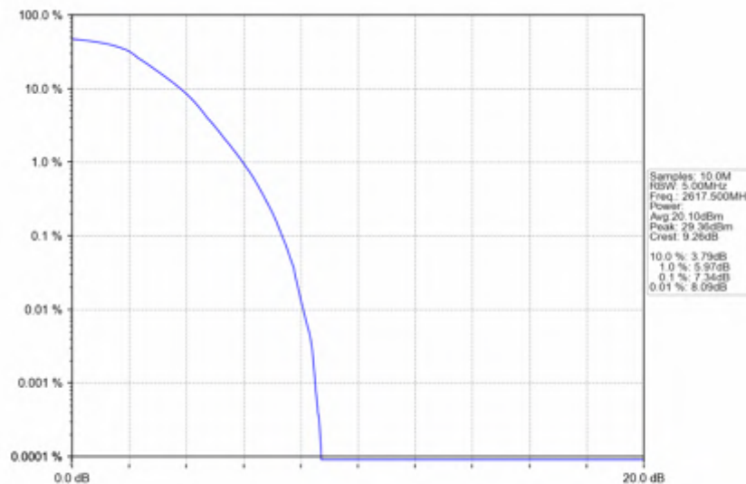
n38_15kHz_SISO_NTNV_5MHz_DFT-s-OFDM_QPSK_2617.5MHz_Outer_Full
