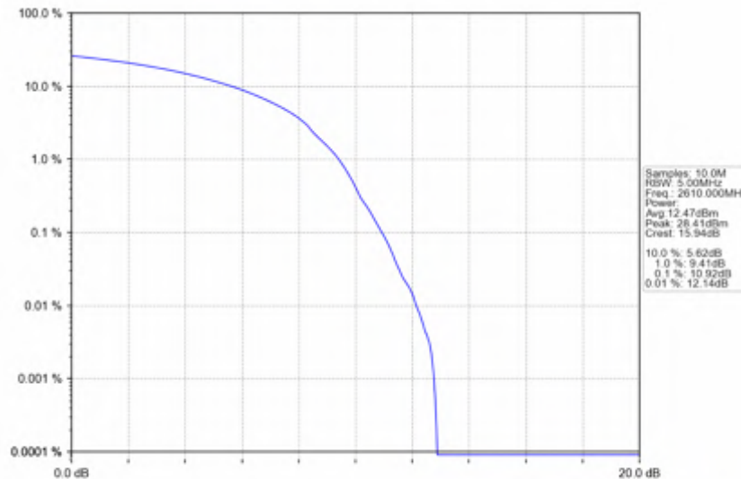
n38_15kHz_SISO_NTNV_20MHz_DFT-s-OFDM_16_QAM_2610MHz_Outer_Full
