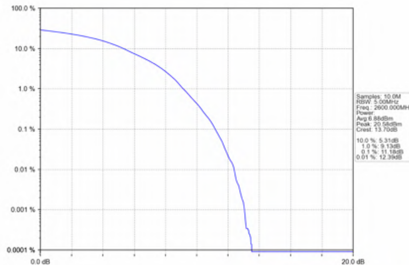
n38_15kHz_SISO_NTNV_40MHz_DFT-s-OFDM 256 QAM_2600MHz_Outer_Full
