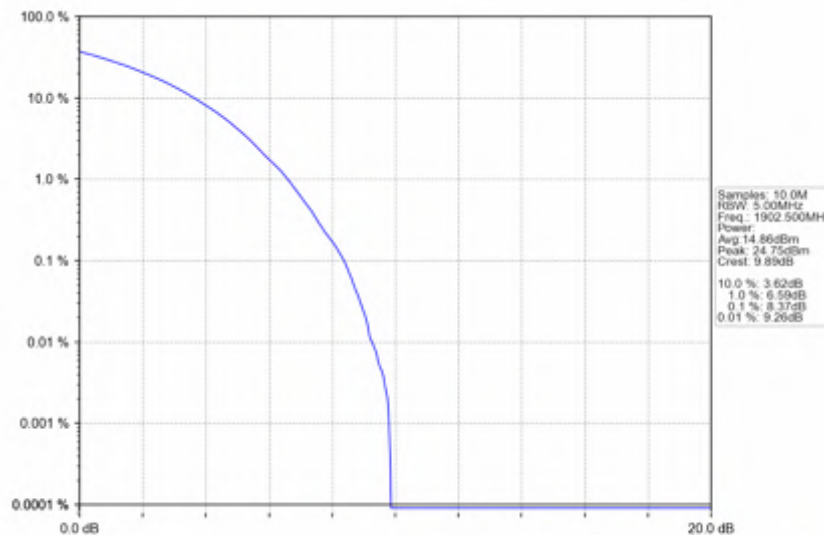
n25_30kHz_SISO_NTNV_25MHz_CP-OFDM QPSK_1902.5MHz_Outer_Full
