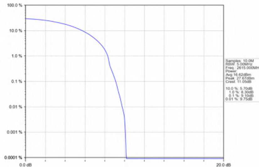
n38_30kHz_SISO_NTNV_10MHz_DFT-s-OFDM QPSK_2615MHz_Outer_Full
