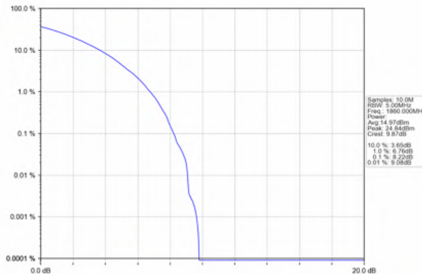
n25_30kHz_SISO_NTNV_20MHz_CP-OFDM 64 QAM_1860MHz_Outer_Full
