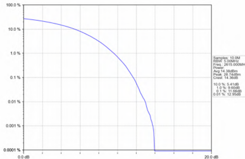
n38_15kHz_SISO_NTNV_10MHz_CP-OFDM 16 QAM_2615MHz_Outer_Full
