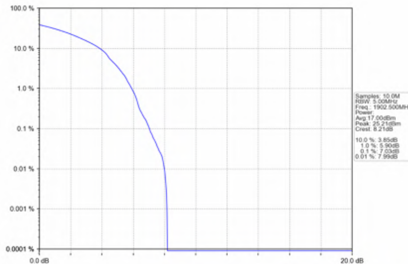
n25_30kHz_SISO_NTNV_25MHz_DFT-s-OFDM QPSK_1902.5MHz_Outer_Full
