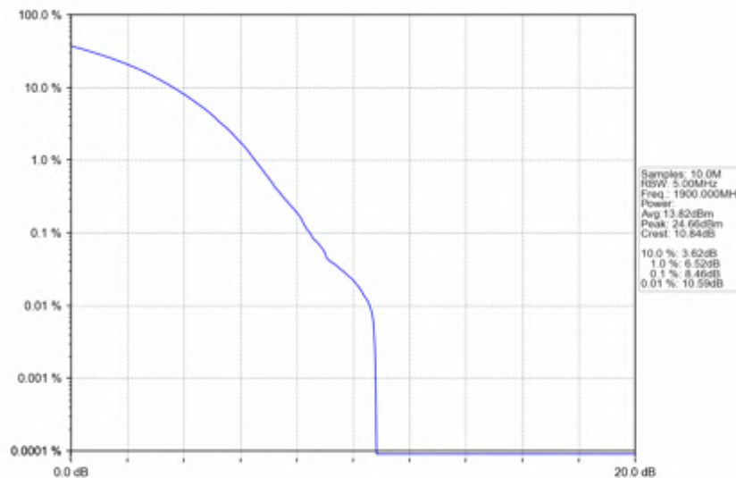
n25_30kHz_SISO_NTNV_30MHz_CP-OFDM QPSK_1900MHz_Outer_Full
