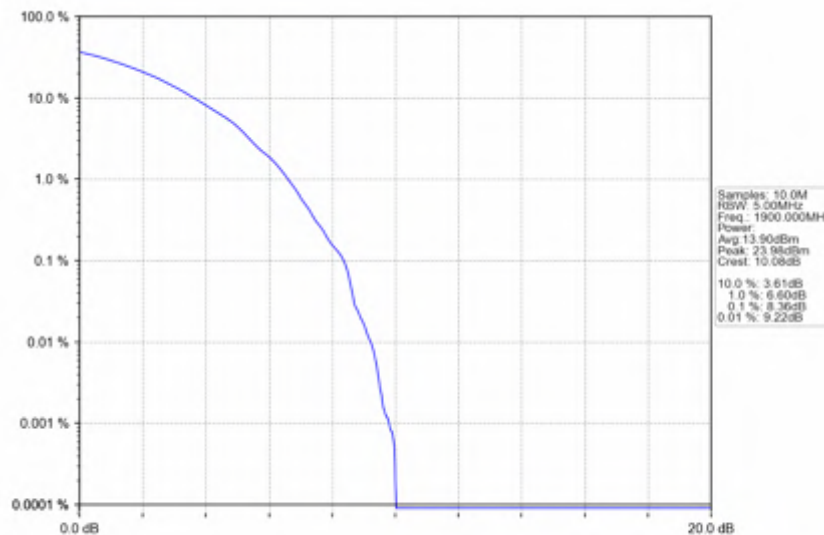
n25_30kHz_SISO_NTNV_30MHz_CP-OFDM 16 QAM_1900MHz_Outer_Full
