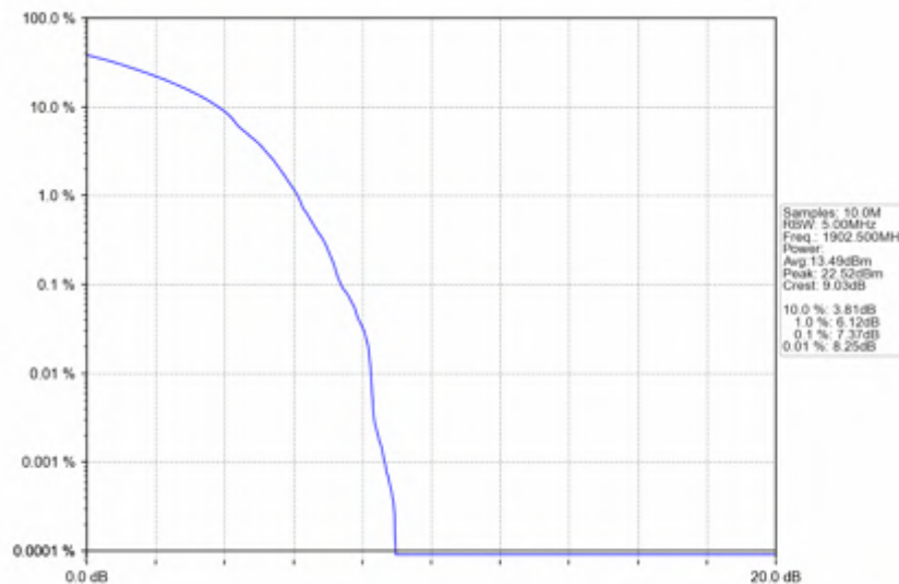
n25_30kHz_SISO_NTNV_25MHz_DFT-s-OFDM_256_QAM_1902.5MHz_Outer_Full
