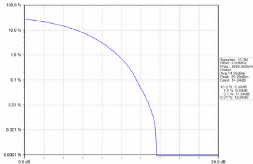
n38_15kHz_SISO_NTNV_10MHz_CP-OFDM 64 QAM_2595MHz_Outer_Full
