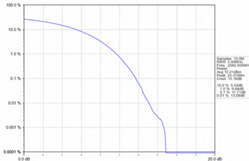
n38_15kHz_SISO_NTNV_25MHz_CP-OFDM_16_QAM_2582.5MHz_Outer_Full
