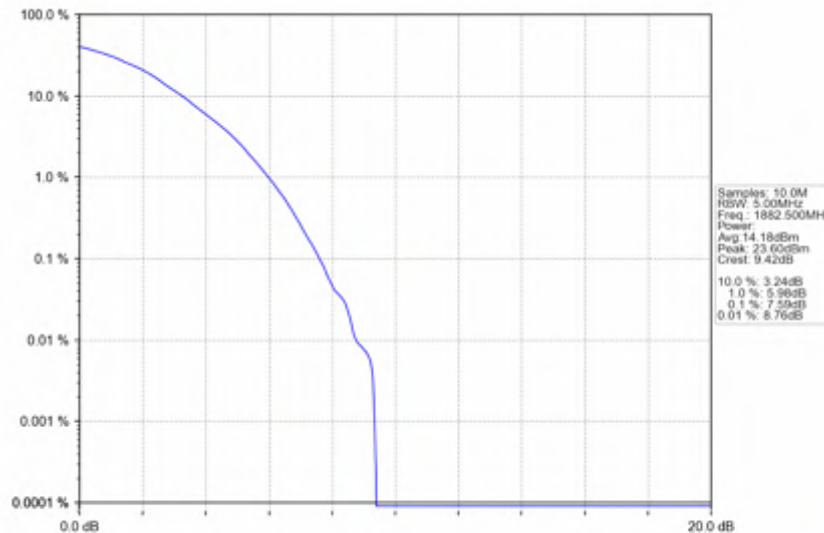
n25_30kHz_SISO_NTNV_20MHz_DFT-s-OFDM_256_QAM_1882.5MHz_Outer_Full
