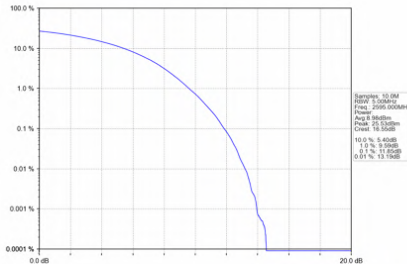
n38_15kHz_SISO_NTNV_30MHz_CP-OFDM 64 QAM_2595MHz_Outer_Full
