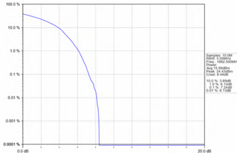
n25_30kHz_SISO_NTNV_30MHz_DFT-s-OFDM QPSK_1882.5MHz_Outer_Full
