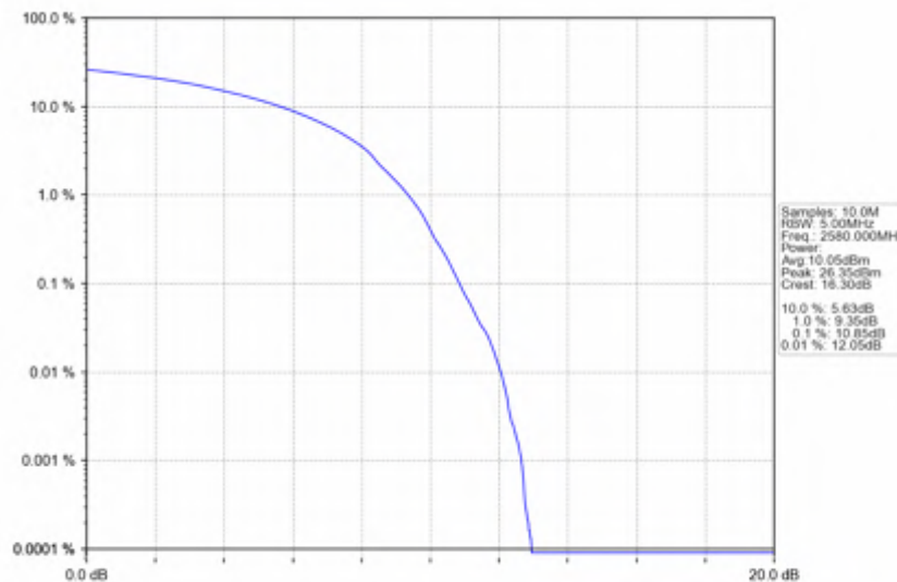
n38_15kHz_SISO_NTNV_20MHz_DFT-s-OFDM_256_QAM_2580MHz_Outer_Full
