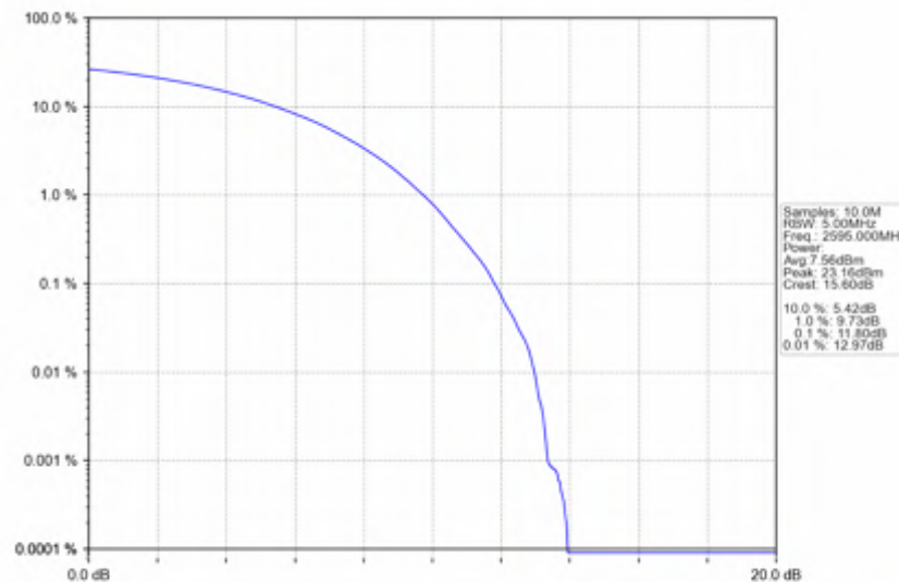
n38_15kHz_SISO_NTNV_20MHz_CP-OFDM 256 QAM_2595MHz_Outer_Full
