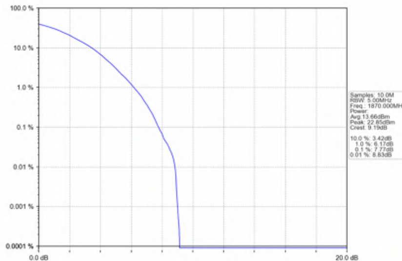
n25_30kHz_SISO_NTNV_40MHz_DFT-s-OFDM_16_QAM_1870MHz_Outer_Full
