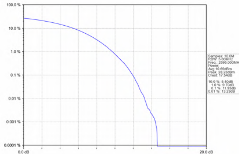
n38_15kHz_SISO_NTNV_10MHz_CP-OFDM 256 QAM_2595MHz_Outer_Full
