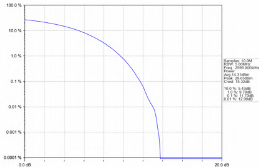
n38_15kHz_SISO_NTNV_10MHz_CP-OFDM QPSK_2595MHz_Outer_Full
