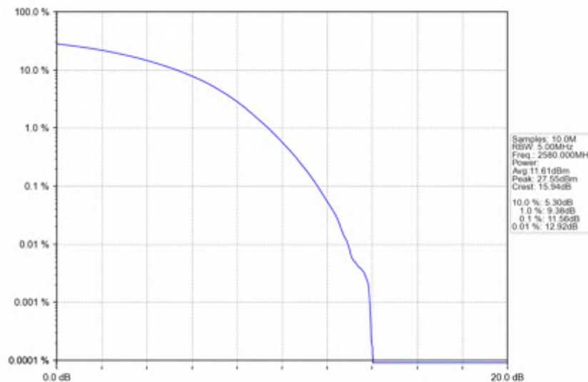
n38_15kHz_SISO_NTNV_20MHz_CP-OFDM QPSK_2580MHz_Outer_Full
