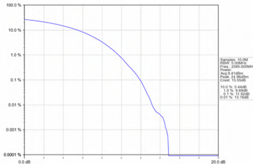
n38_15kHz_SISO_NTNV_30MHz_CP-OFDM QPSK_2585MHz_Outer_Full
