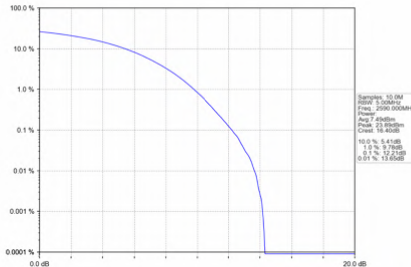
n38_15kHz_SISO_NTNV_40MHz_CP-OFDM 64 QAM_2590MHz_Outer_Full
