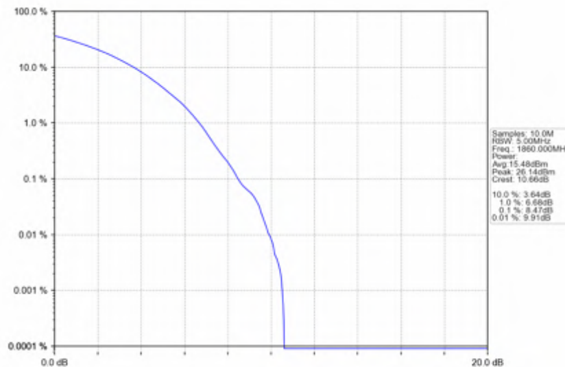
n25_30kHz_SISO_NTNV_20MHz_CP-OFDM QPSK_1860MHz_Outer_Full
