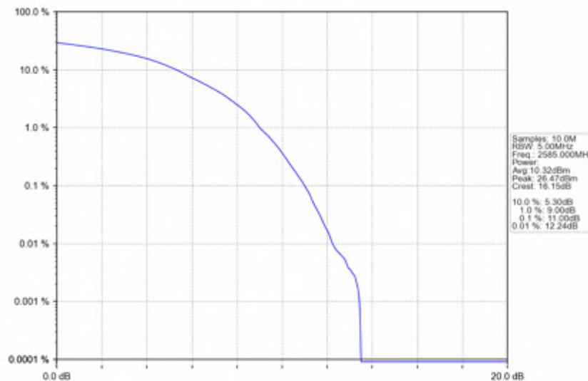
n38_15kHz_SISO_NTNV_30MHz_DFT-s-OFDM_64_QAM_2585MHz_Outer_Full
