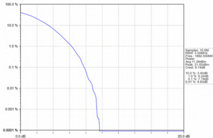
n25_30kHz_SISO_NTNV_40MHz_DFT-s-OFDM_256_QAM_1882.5MHz_Outer_Full
