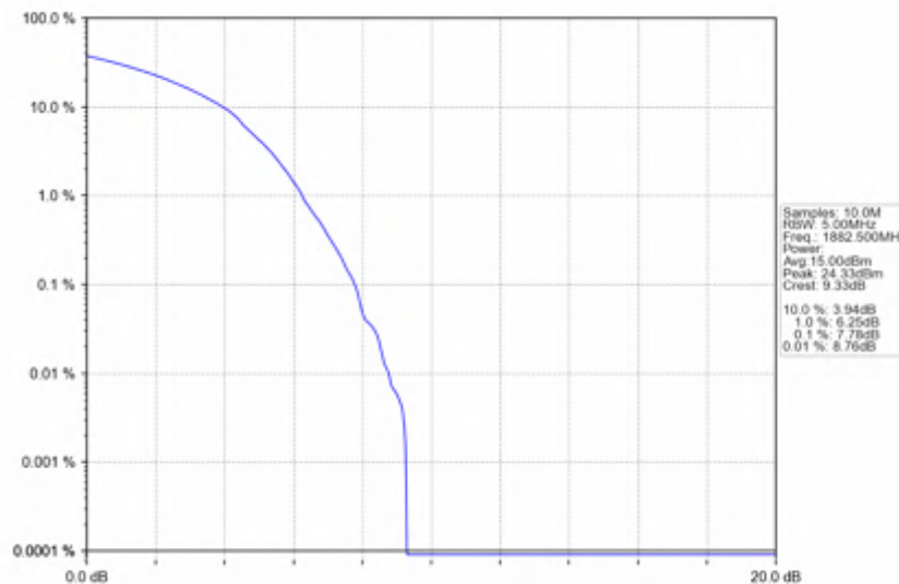
n25_30kHz_SISO_NTNV_30MHz_DFT-s-OFDM_16_QAM_1882.5MHz_Outer_Full
