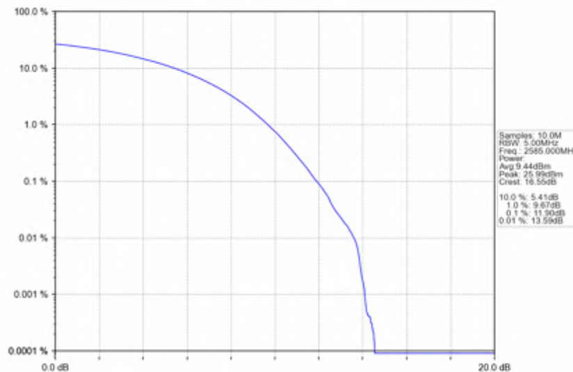
n38_15kHz_SISO_NTNV_30MHz_CP-OFDM_16_QAM_2585MHz_Outer_Full
