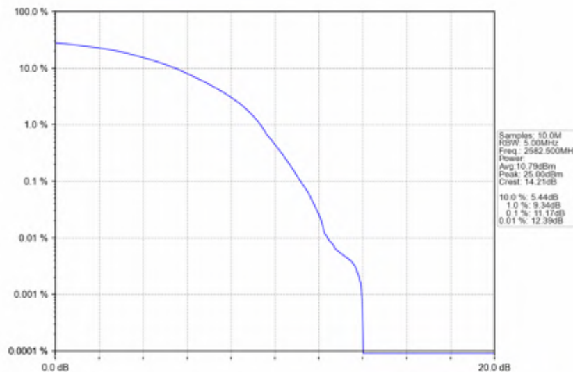
n38_15kHz_SISO_NTV_25MHz_DFT-s-OFDM 64 QAM_2582.5MHz_Outer_Full
