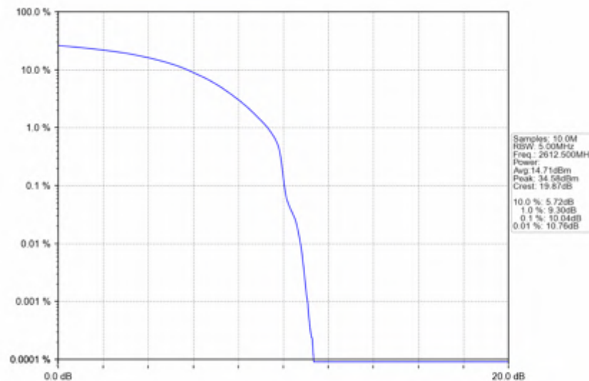
n38_15kHz_SISO_NTNV_15MHz_DFT-s-OFDM QPSK_2612.5MHz_Outer_Full
