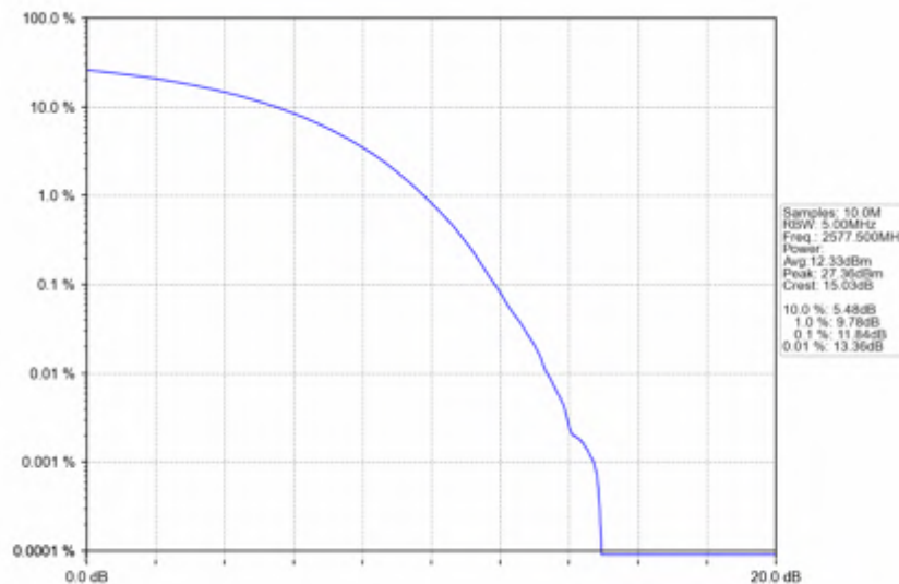
n38_15kHz_SISO_NTNV_15MHz_CP-OFDM_16_QAM_2577.5MHz_Outer_Full
