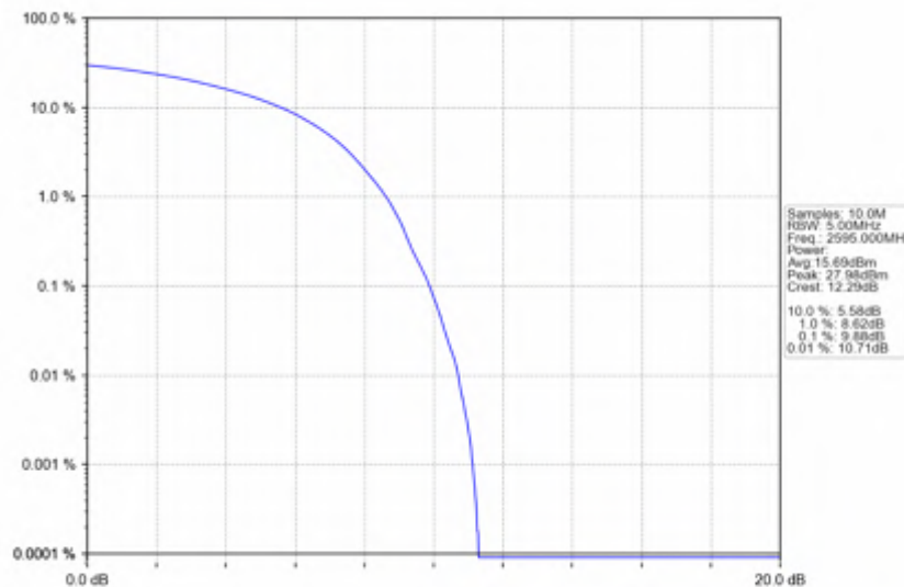
n38_15kHz_SISO_NTNV_10MHz_DFT-s-OFDM_16_QAM_2595MHz_Outer_Full
