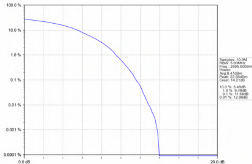
n38_15kHz_SISO_NTNV_40MHz_DFT-s-OFDM_64_QAM_2595MHz_Outer_Full
