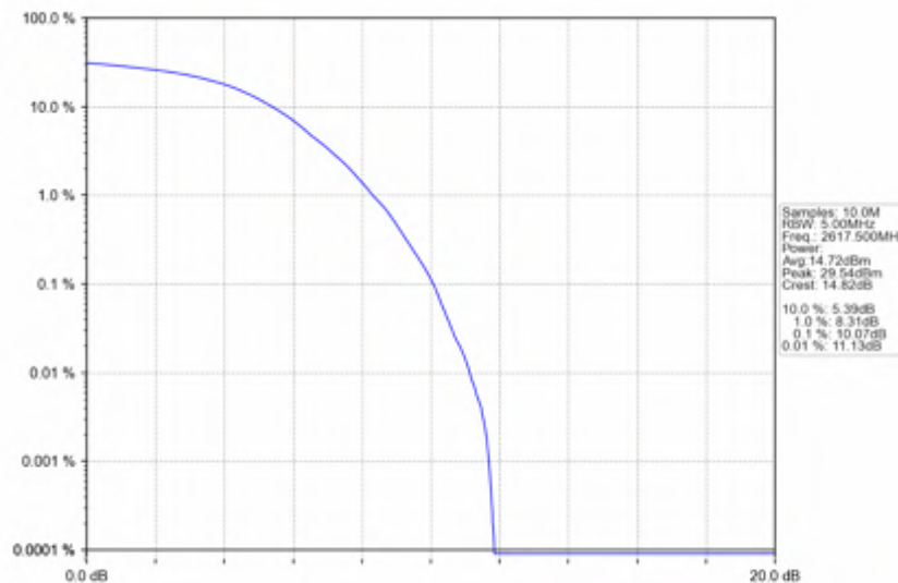
n38_15kHz_SISO_NTNV_5MHz_DFT-s-OFDM 256 QAM_2617.5MHz_Outer_Full
