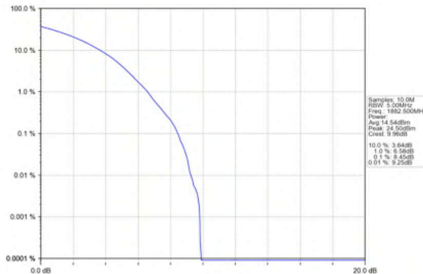
n25_30kHz_SISO_NTNV_25MHz_CP-OFDM QPSK_1882.5MHz_Outer_Full
