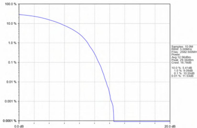
n38_15kHz_SISO_NTNV_25MHz_DFT-s-OFDM QPSK_2582.5MHz_Outer_Full
