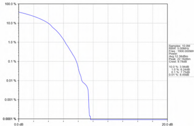
n25_30kHz_SISO_NTNV_30MHz_DFT-s-OFDM 256 QAM_1900MHz_Outer_Full
