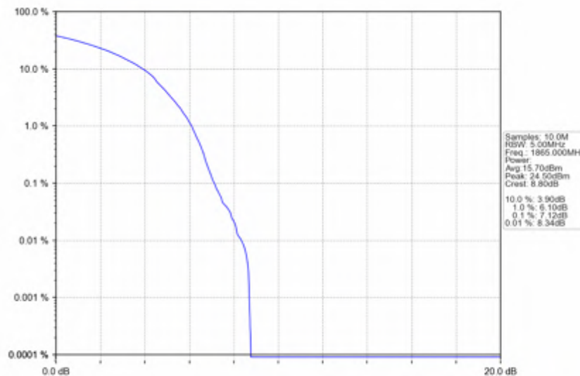
n25_30kHz_SISO_NTNV_30MHz_DFT-s-OFDM QPSK_1865MHz_Outer_Full
