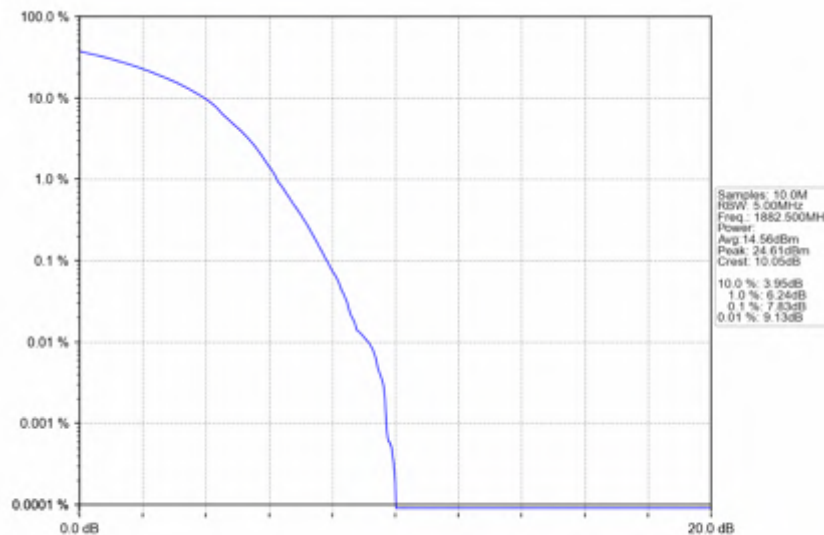
n25_30kHz_SISO_NTNV_30MHz_DFT-s-OFDM 64 QAM_1882.5MHz_Outer_Full
