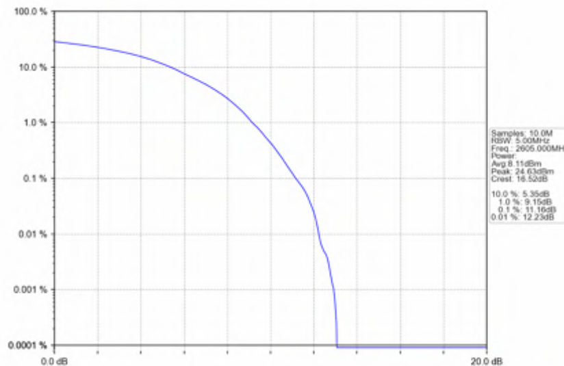
n38_15kHz_SISO_NTNV_30MHz_DFT-s-OFDM 256 QAM_2605MHz_Outer_Full
