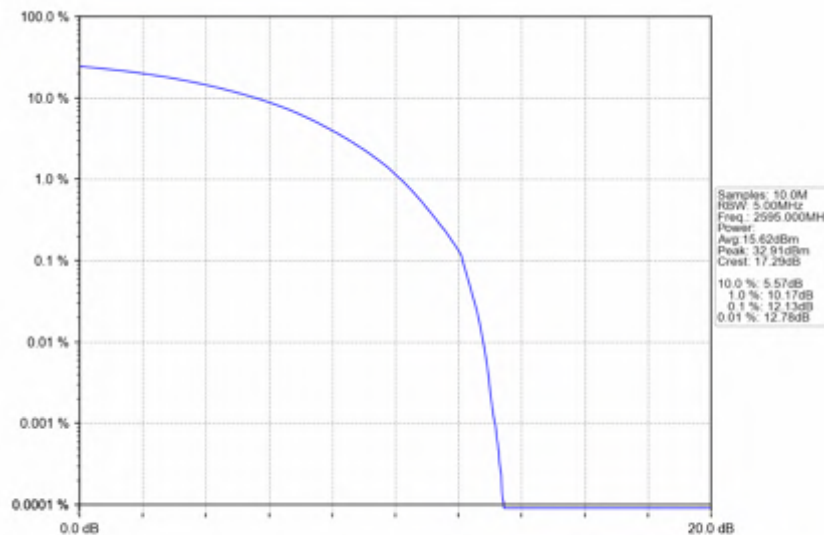
n38_15kHz_SISO_NTNV_5MHz_CP-OFDM QPSK_2595MHz_Outer_Full
