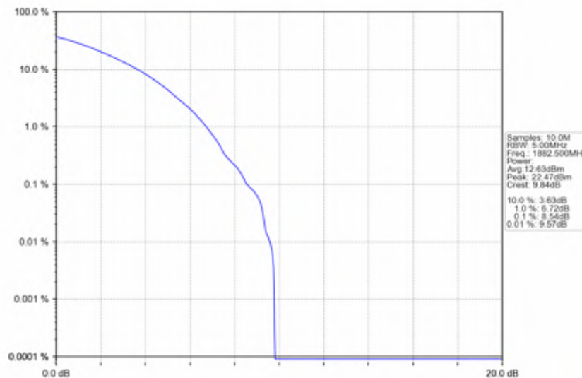
n25_30kHz_SISO_NTNV_40MHz_CP-OFDM QPSK_1882.5MHz_Outer_Full
