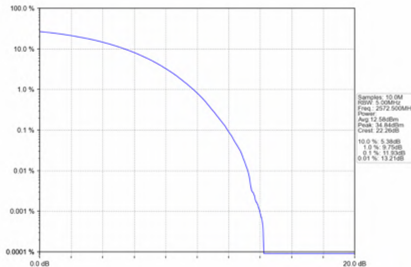
n38_15kHz_SISO_NTNV_5MHz_CP-OFDM 256 QAM_2572.5MHz_Outer_Full
