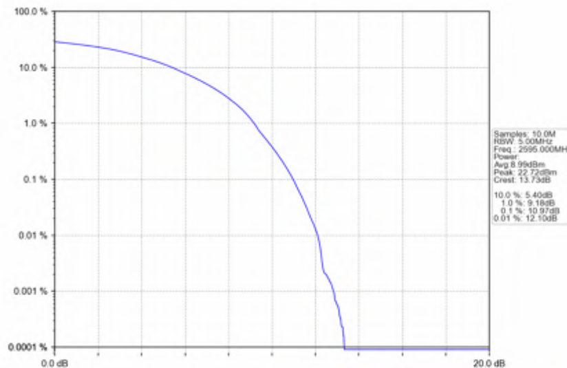
n38_15kHz_SISO_NTNV_25MHz_DFT-s-OFDM_256_QAM_2595MHz_Outer_Full
