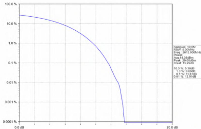
n38_15kHz_SISO_NTNV_10MHz_CP-OFDM QPSK_2615MHz_Outer_Full
