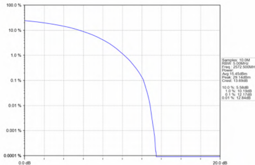
n38_15kHz_SISO_NTNV_5MHz_CP-OFDM QPSK_2572.5MHz_Outer_Full
