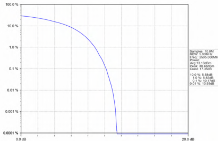
n38_15kHz_SISO_NTNV_10MHz_DFT-s-OFDM_256_QAM_2595MHz_Outer_Full
