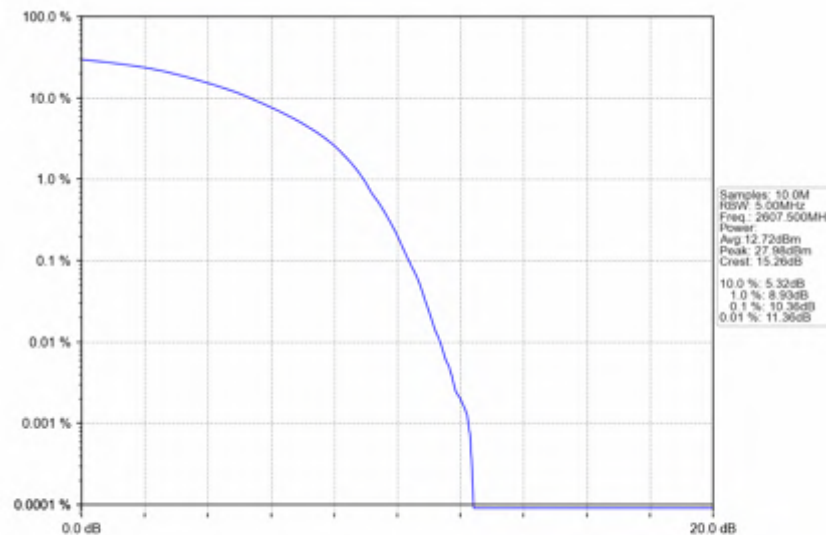
n38_15kHz_SISO_NTNV_25MHz_DFT-s-OFDM QPSK_2607.5MHz_Outer_Full
