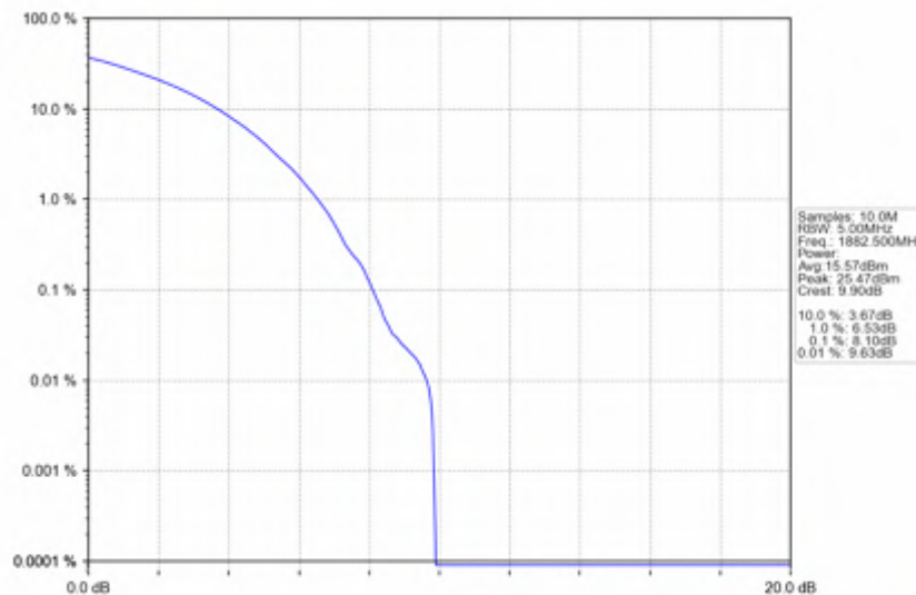
n25_30kHz_SISO_NTNV_20MHz_CP-OFDM QPSK_1882.5MHz_Outer_Full
