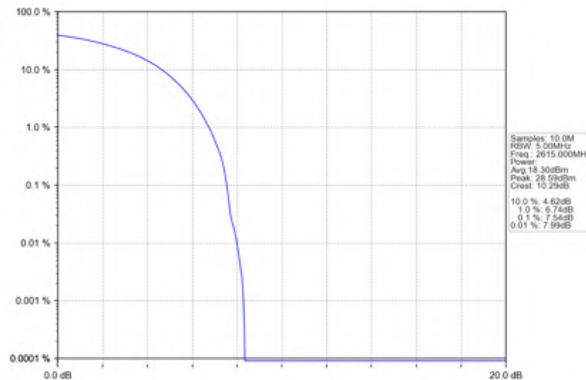
n38_15kHz_SISO_NTNV_10MHz_DFT-s-OFDM QPSK_2615MHz_Outer_Full
