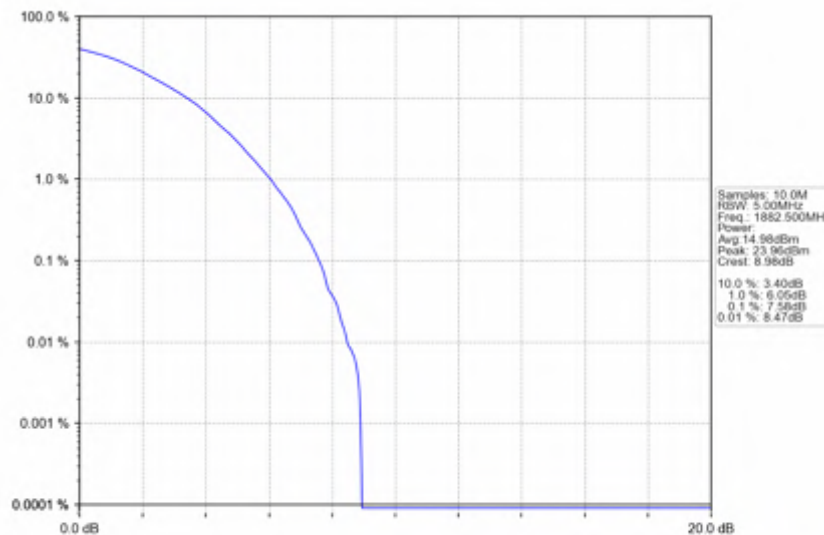
n25_30kHz_SISO_NTNV_40MHz_DFT-s-OFDM QPSK_1882.5MHz_Outer_Full
