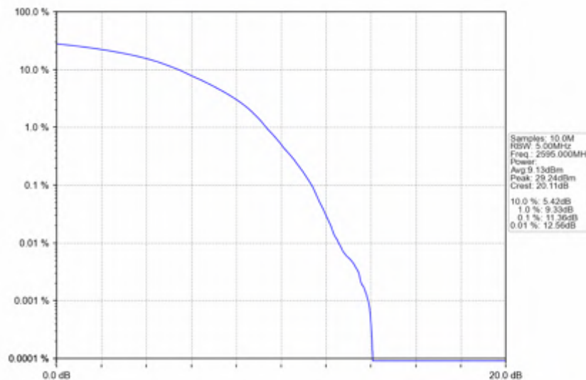
n38_15kHz_SISO_NTNV_40MHz_DFT-s-OFDM_16_QAM_2595MHz_Outer_Full
