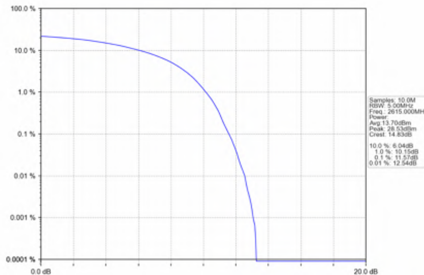
n38_15kHz_SISO_NTNV_10MHz_DFT-s-OFDM_16_QAM_2615MHz_Outer_Full
