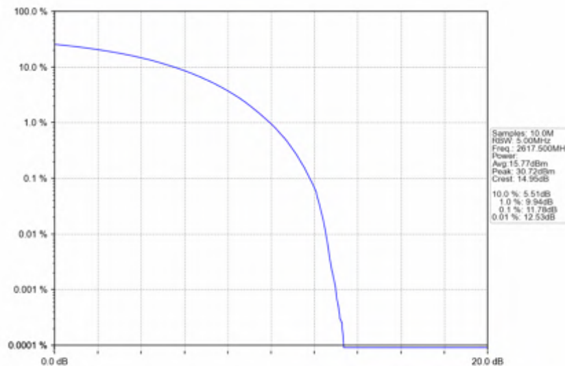
n38_15kHz_SISO_NTNV_5MHz_CP-OFDM_16_QAM_2617.5MHz_Outer_Full
