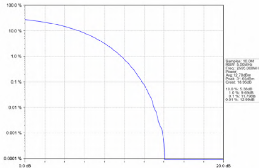
n38_15kHz_SISO_NTNV_5MHz_CP-OFDM 256 QAM_2595MHz_Outer_Full
