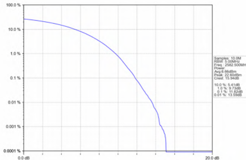
n38_15kHz_SISO_NTNV_25MHz_CP-OFDM_256_QAM_2582.5MHz_Outer_Full
