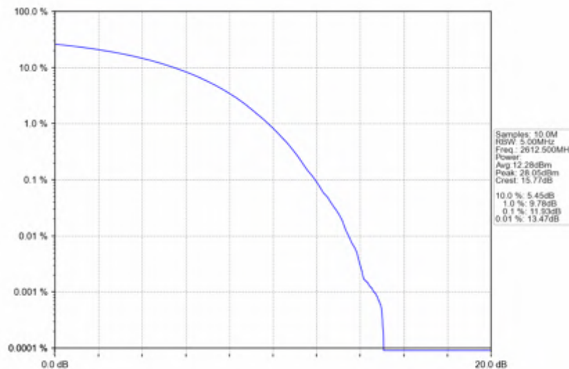
n38_15kHz_SISO_NTNV_15MHz_CP-OFDM 16 QAM_2612.5MHz_Outer_Full
