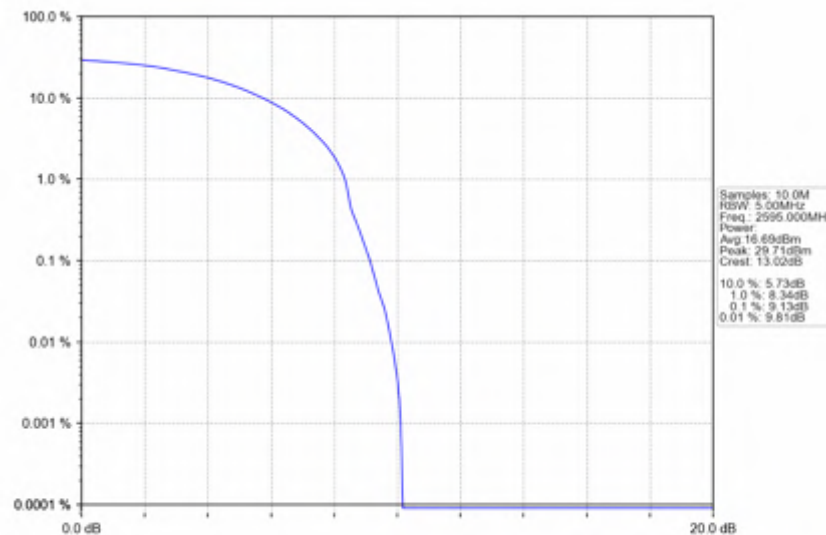
n38_30kHz_SISO_NTNV_10MHz_DFT-s-OFDM QPSK_2595MHz_Outer_Full
