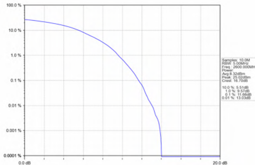
n38_15kHz_SISO_NTNV_40MHz_DFT-s-OFDM_64_QAM_2600MHz_Outer_Full
