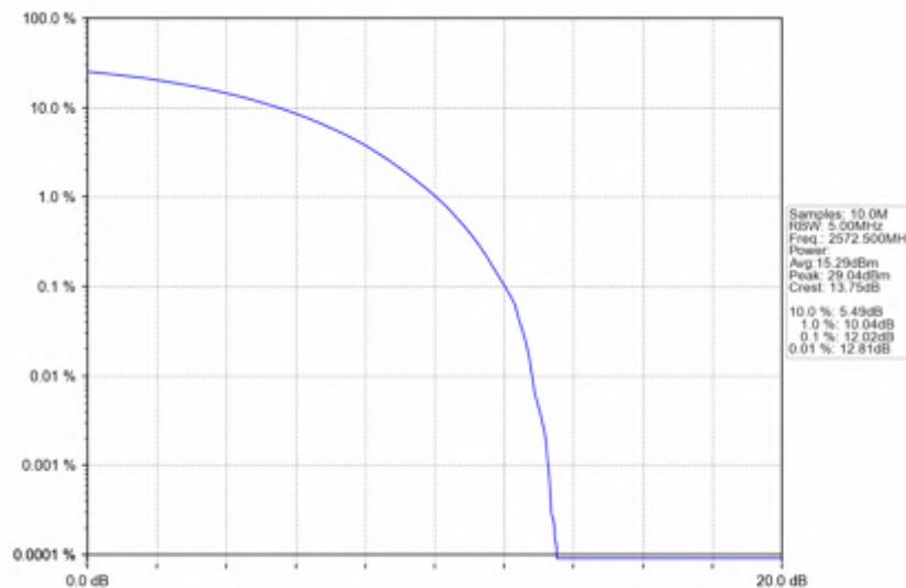
n38_15kHz_SISO_NTNV_5MHz_CP-OFDM_64_QAM_2572.5MHz_Outer_Full
