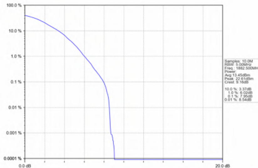
n25_30kHz_SISO_NTNV_40MHz_DFT-s-OFDM 64 QAM_1882.5MHz_Outer_Full
