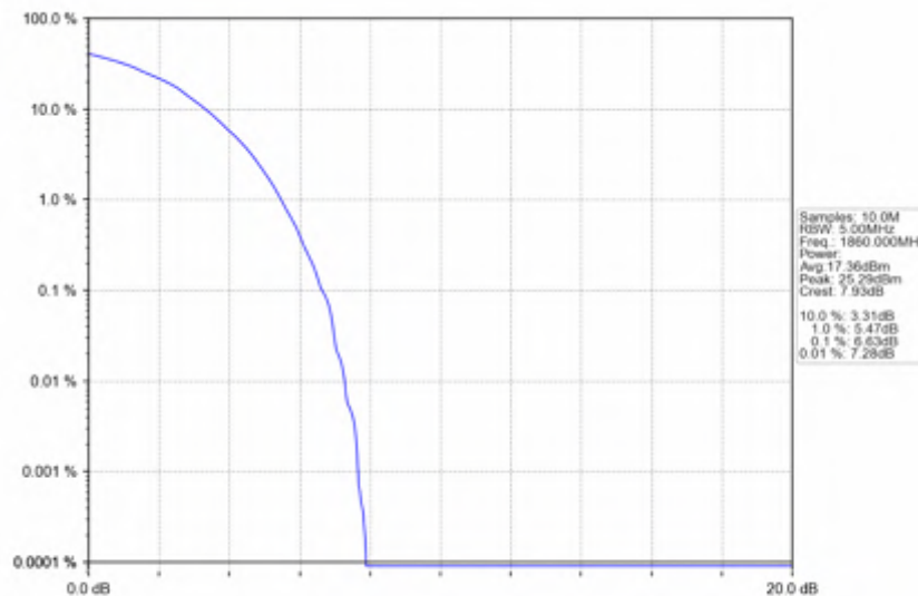
n25_30kHz_SISO_NTNV_20MHz_DFT-s-OFDM QPSK_1860MHz_Outer_Full
