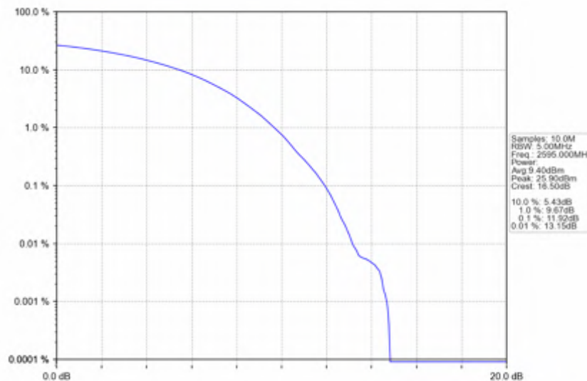
n38_15kHz_SISO_NTNV_30MHz_CP-OFDM QPSK_2595MHz_Outer_Full
