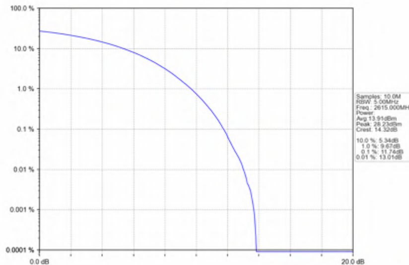
n38_15kHz_SISO_NTNV_10MHz_CP-OFDM 64 QAM_2615MHz_Outer_Full
