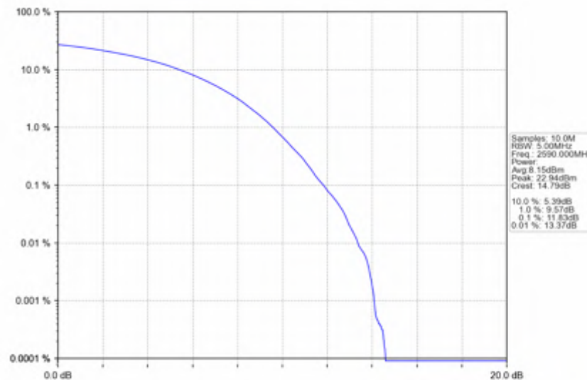
n38_15kHz_SISO_NTNV_40MHz_CP-OFDM QPSK_2590MHz_Outer_Full
