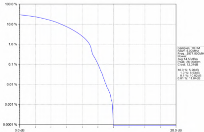
n38_15kHz_SISO_NTV_15MHz_DFT-s-OFDM_16_QAM_2577.5MHz_Outer_Full
