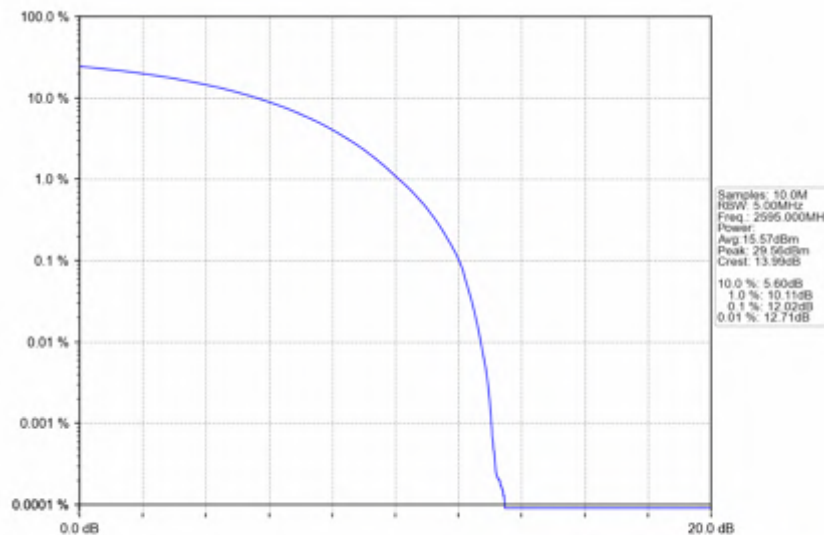
n38_15kHz_SISO_NTNV_5MHz_CP-OFDM_16_QAM_2595MHz_Outer_Full
