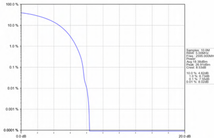
n38_15kHz_SISO_NTNV_10MHz_DFT-s-OFDM QPSK_2595MHz_Outer_Full
