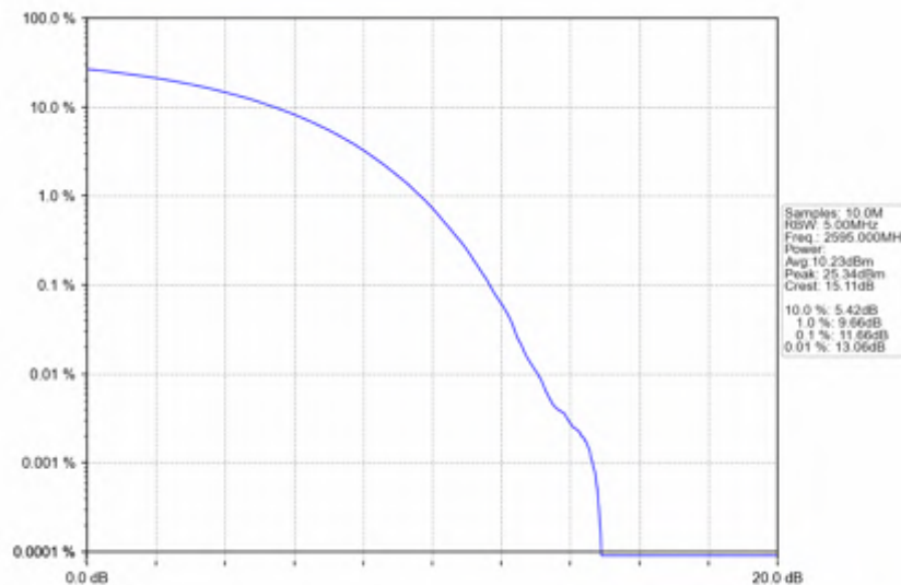
n38_15kHz_SISO_NTNV_25MHz_CP-OFDM_16_QAM_2595MHz_Outer_Full
