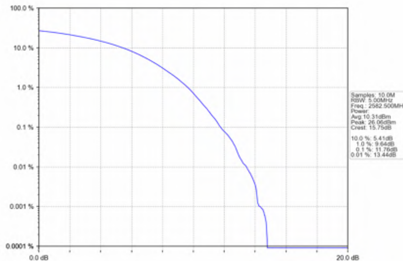
n38_15kHz_SISO_NTNV_25MHz_CP-OFDM_QPSK_2582.5MHz_Outer_Full
