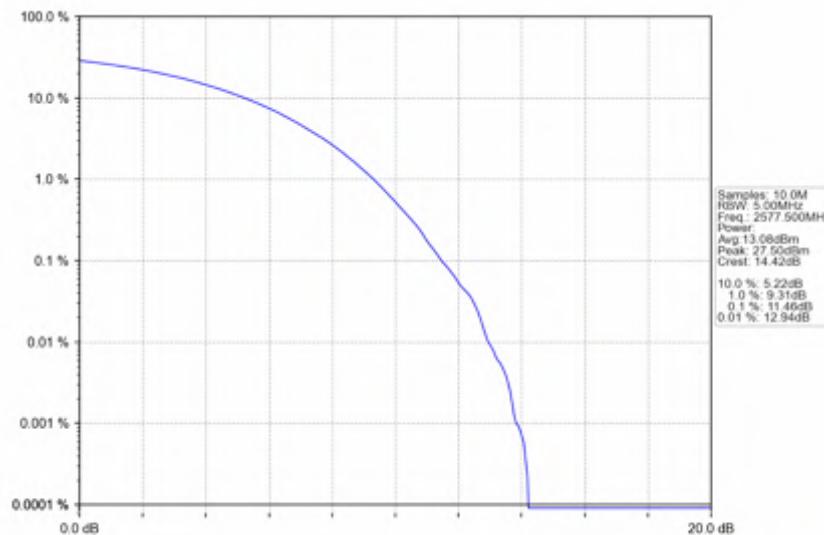
n38_15kHz_SISO_NTNV_15MHz_CP-OFDM_QPSK_2577.5MHz_Outer_Full
