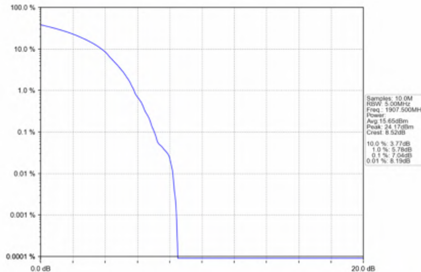
n25_30kHz_SISO_NTNV_15MHz_DFT-s-OFDM_256_QAM_1907.5MHz_Outer_Full
