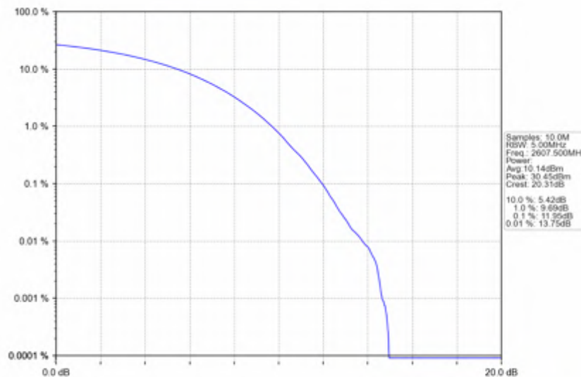
n38_15kHz_SISO_NTNV_25MHz_CP-OFDM QPSK_2607.5MHz_Outer_Full
