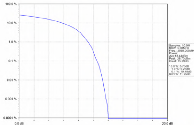
n38_15kHz_SISO_NTNV_20MHz_DFT-s-OFDM QPSK_2595MHz_Outer_Full
