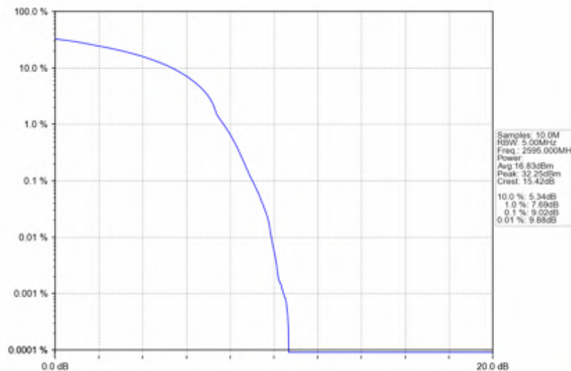
n38_30kHz_SISO_NTNV_10MHz_DFT-s-OFDM_16_QAM_2595MHz_Outer_Full
