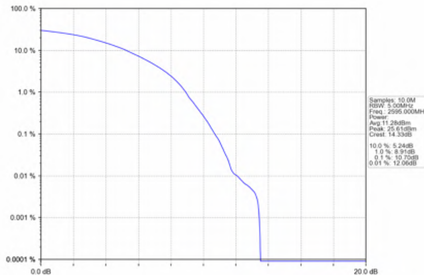
n38_15kHz_SISO_NTNV_25MHz_DFT-s-OFDM_64_QAM_2595MHz_Outer_Full
