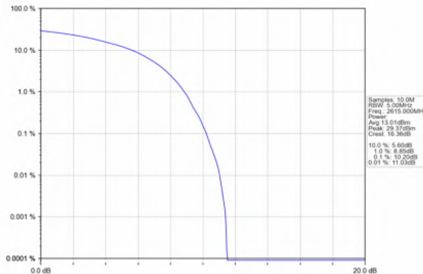
n38_15kHz_SISO_NTNV_10MHz_DFT-s-OFDM 256 QAM_2615MHz_Outer_Full
