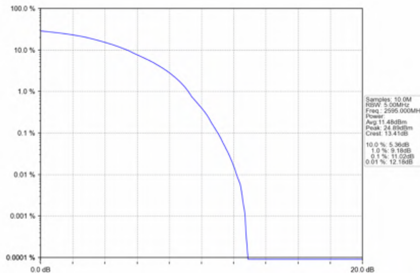
n38_15kHz_SISO_NTNV_25MHz_DFT-s-OFDM_16_QAM_2595MHz_Outer_Full
