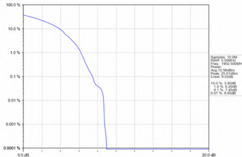
n25_30kHz_SISO_NTV_25MHz_DFT-s-OFDM 16 QAM_1902.5MHz_Outer_Full
