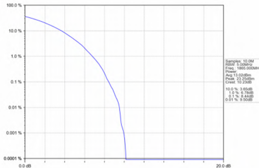
n25_30kHz_SISO_NTNV_30MHz_CP-OFDM 64 QAM_1865MHz_Outer_Full
