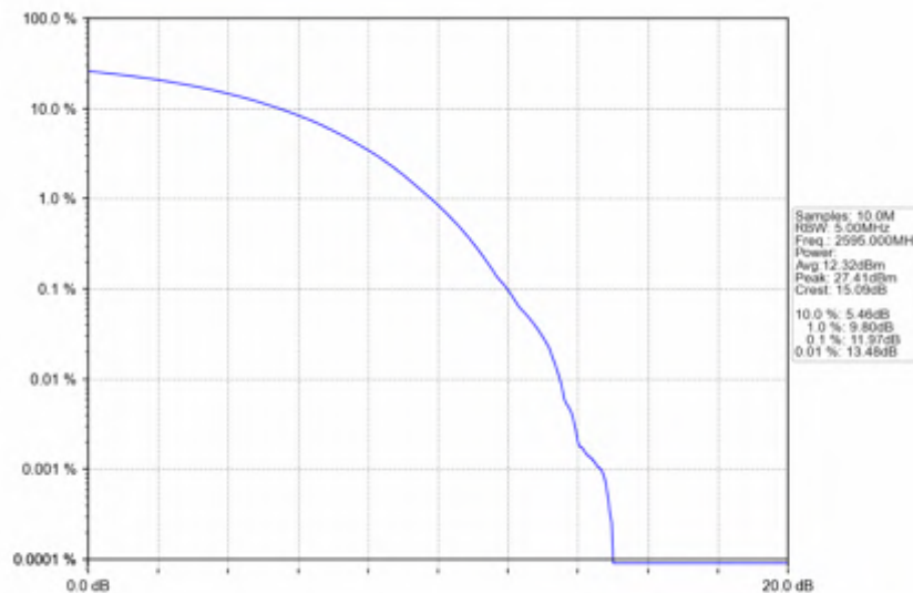
n38_15kHz_SISO_NTNV_15MHz_CP-OFDM_16_QAM_2595MHz_Outer_Full
