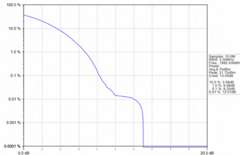
n25_15kHz_SISO_NTNV_40MHz_CP-OFDM 256 QAM_1882.5MHz_Outer_Full
