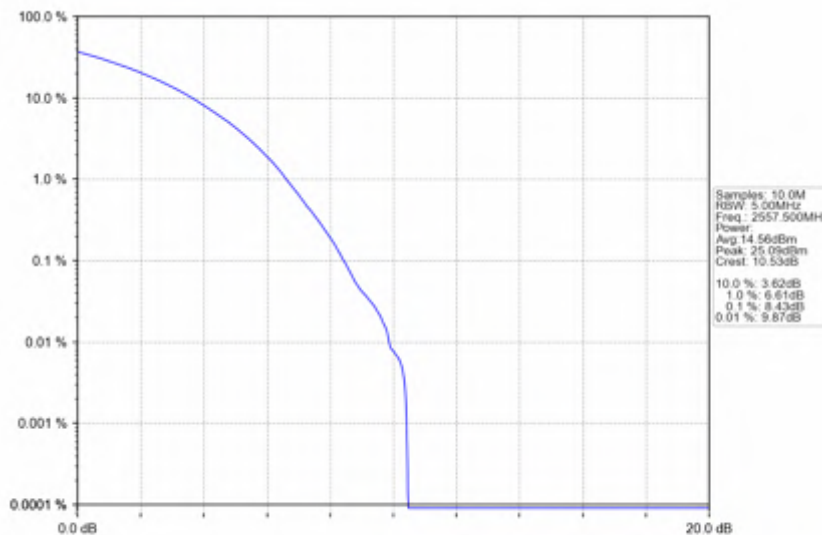
n7_30kHz_SISO_NTNV_25MHz_CP-OFDM_16_QAM_2557.5MHz_Outer_Full
