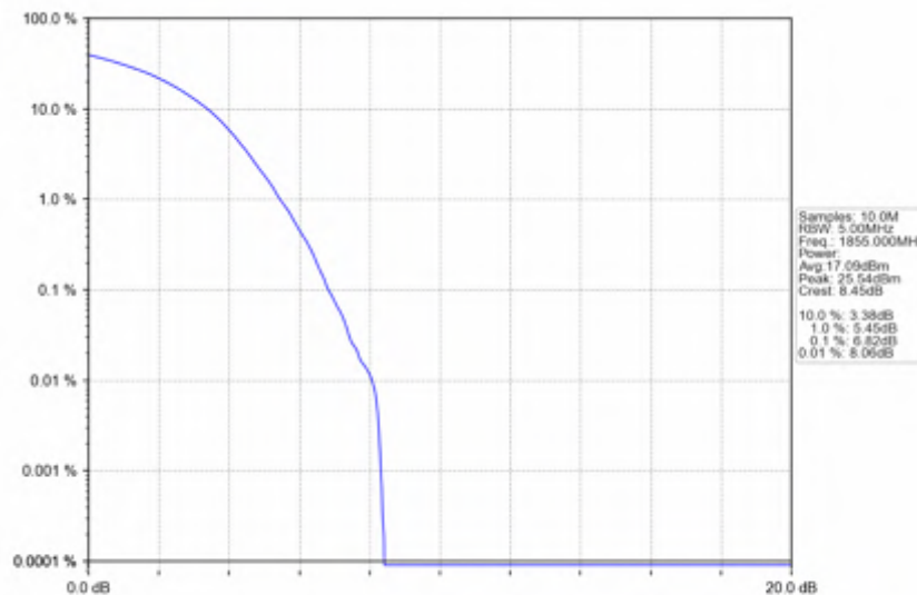
n25_30kHz_SISO_NTNV_10MHz_DFT-s-OFDM_256_QAM_1855MHz_Outer_Full
