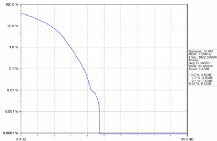
n25_15kHz_SISO_NTV_25MHz_DFT-s-OFDM_16_QAM_1862.5MHz_Outer_Full
