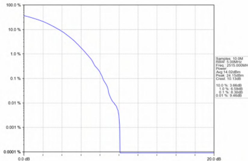
n7_30kHz_SISO_NTNV_30MHz_CP-OFDM_QPSK_2515MHz_Outer_Full
