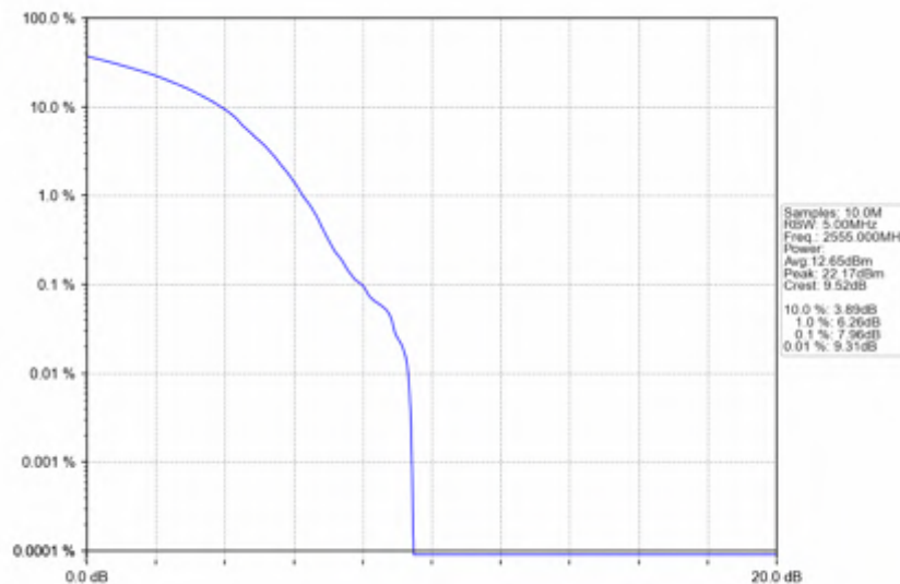
n7_30kHz_SISO_NTNV_30MHz_DFT-s-OFDM_256_QAM_2555MHz_Outer_Full
