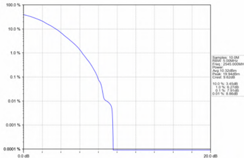
n7_30kHz_SISO_NTNV_50MHz_DFT-s-OFDM_256_QAM_2545MHz_Outer_Full
