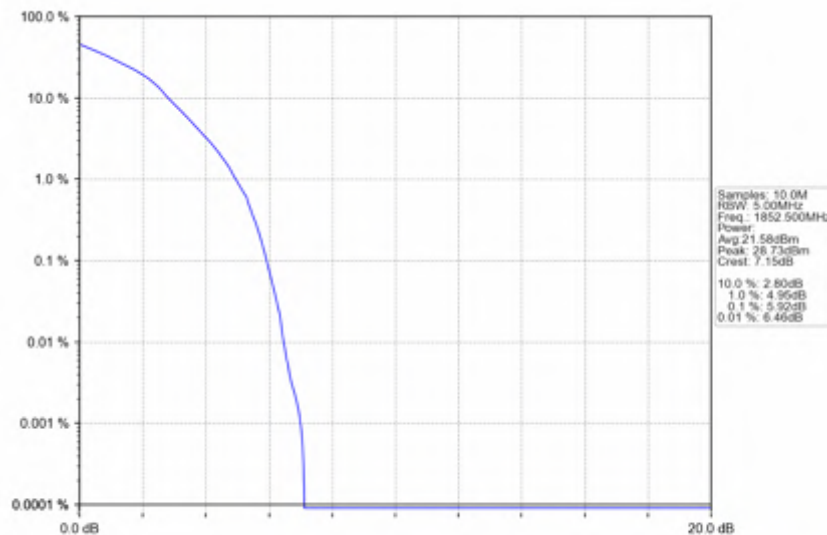
n25_15kHz_SISO_NTNV_5MHz_DFT-s-OFDM_16_QAM_1852.5MHz_Outer_Full
