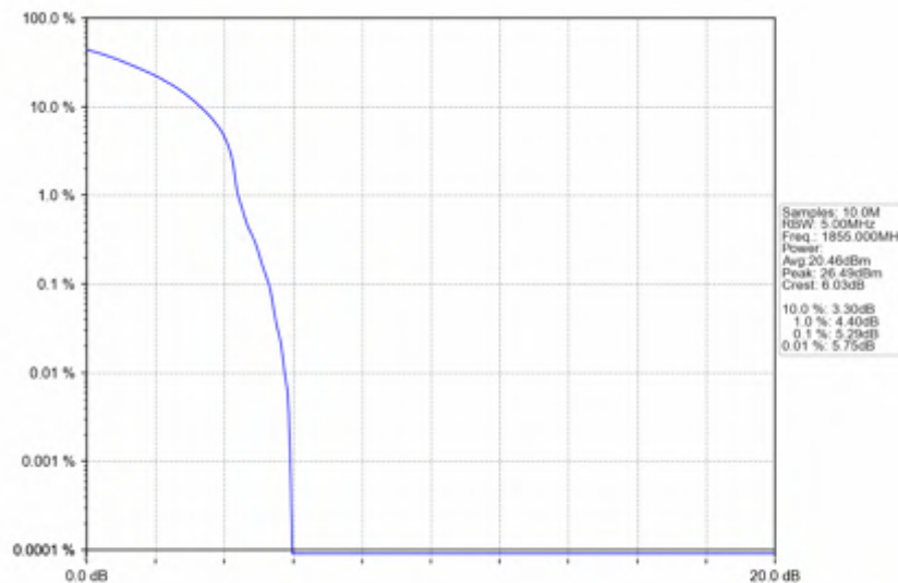
n25_30kHz_SISO_NTNV_10MHz_DFT-s-OFDM QPSK_1855MHz_Outer_Full
