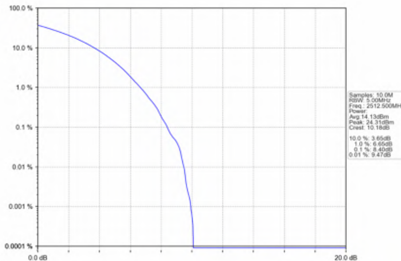
n7_30kHz_SISO_NTNV_25MHz_CP-OFDM_64_QAM_2512.5MHz_Outer_Full
