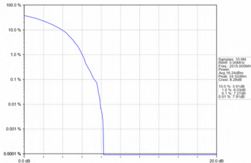
n7_30kHz_SISO_NTNV_30MHz_DFT-s-OFDM QPSK_2515MHz_Outer_Full
