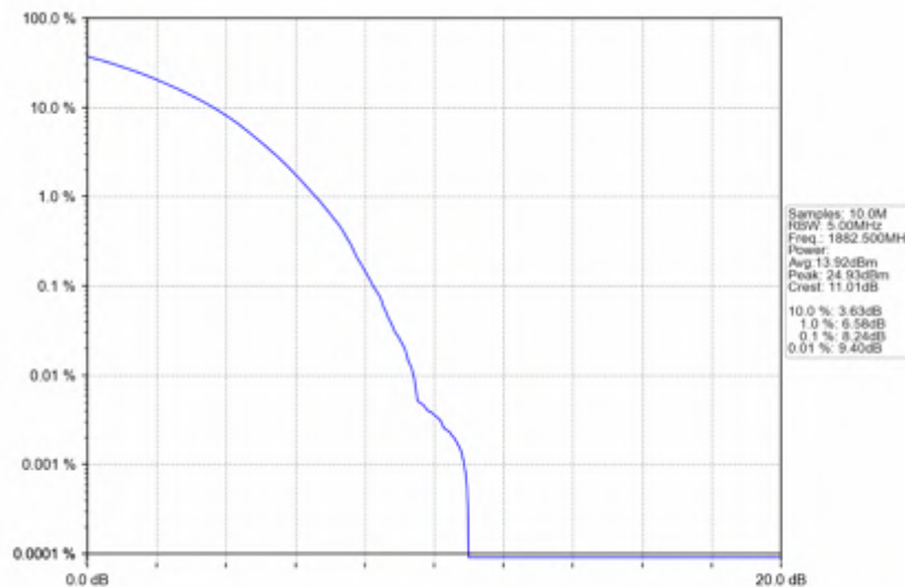
n25_15kHz_SISO_NTNV_25MHz_CP-OFDM 64 QAM_1882.5MHz_Outer_Full
