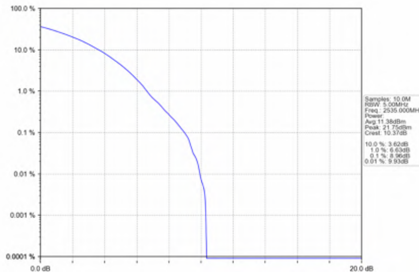
n7_30kHz_SISO_NTNV_50MHz_CP-OFDM_QPSK_2535MHz_Outer_Full
