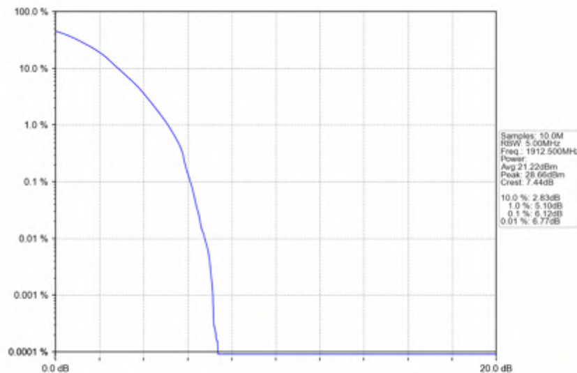
n25_15kHz_SISO_NTNV_5MHz_DFT-s-OFDM 64 QAM_1912.5MHz_Outer_Full
