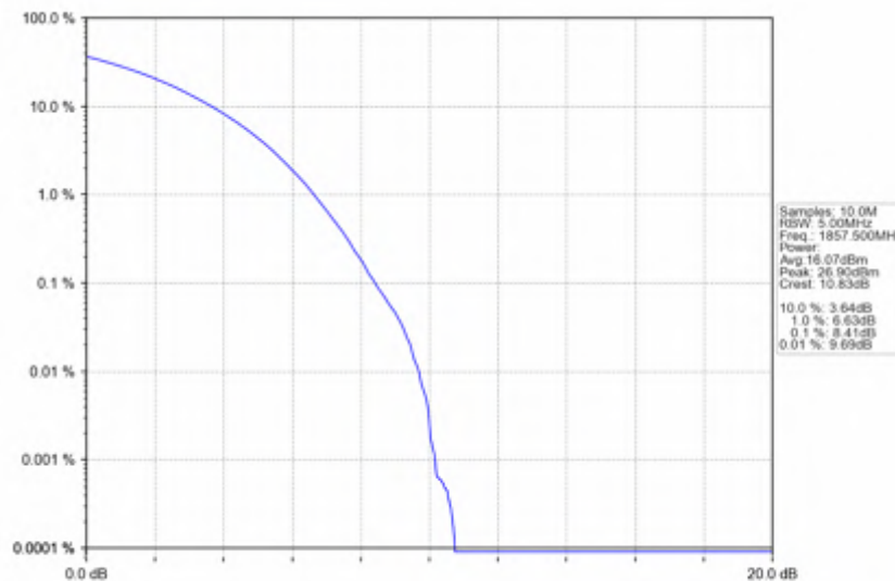
n25_15kHz_SISO_NTNV_15MHz_CP-OFDM 64 QAM_1857.5MHz_Outer_Full
