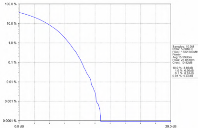
n25_15kHz_SISO_NTNV_15MHz_CP-OFDM 64 QAM_1882.5MHz_Outer_Full
