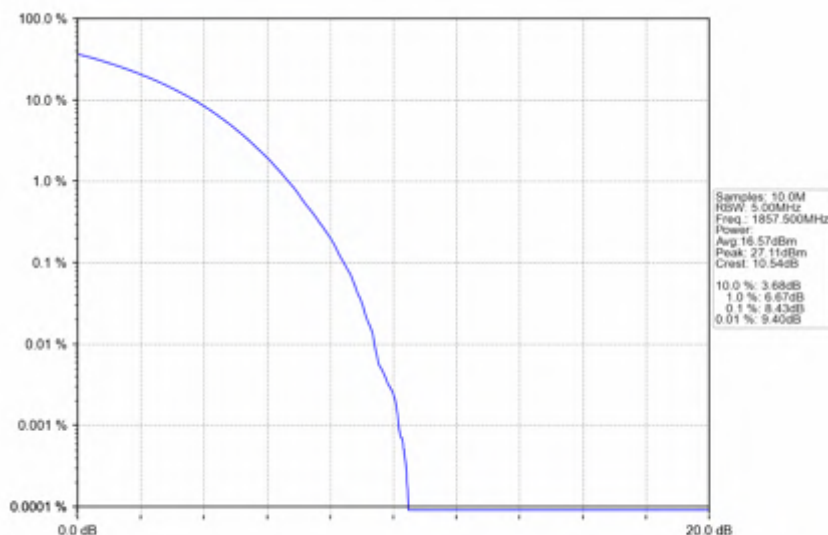
n25_15kHz_SISO_NTNV_15MHz_CP-OFDM_QPSK_1857.5MHz_Outer_Full
