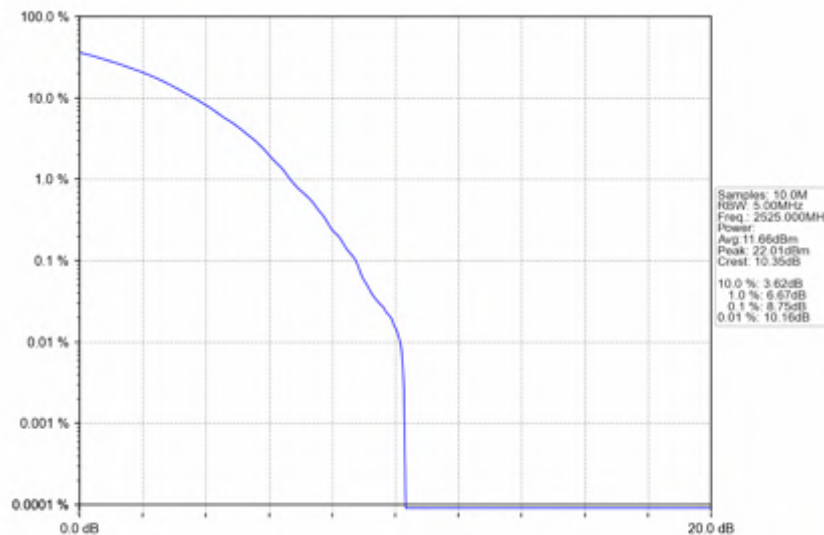
n7_30kHz_SISO_NTNV_50MHz_CP-OFDM_QPSK_2525MHz_Outer_Full
