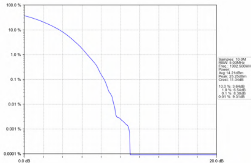
n25_15kHz_SISO_NTNV_25MHz_CP-OFDM 64 QAM_1902.5MHz_Outer_Full
