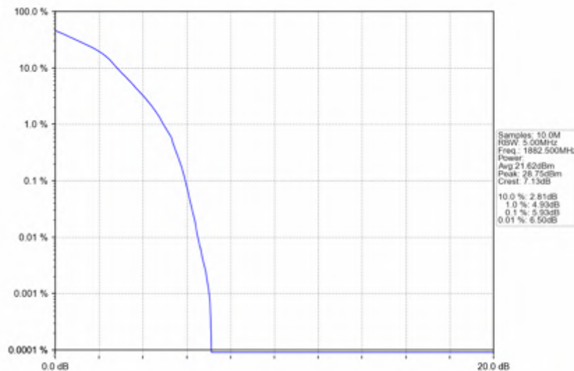
n25_15kHz_SISO_NTNV_5MHz_DFT-s-OFDM_16_QAM_1882.5MHz_Outer_Full
