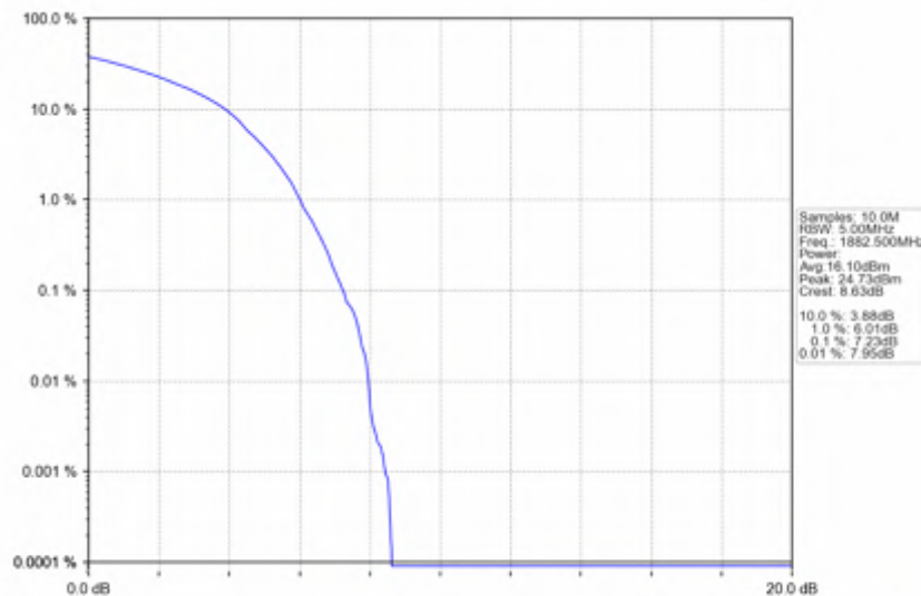
n25_15kHz_SISO_NTNV_20MHz_DFT-s-OFDM 64 QAM_1882.5MHz_Outer_Full
