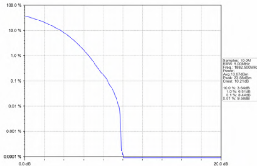
n25_15kHz_SISO_NTNV_30MHz_CP-OFDM QPSK_1882.5MHz_Outer_Full
