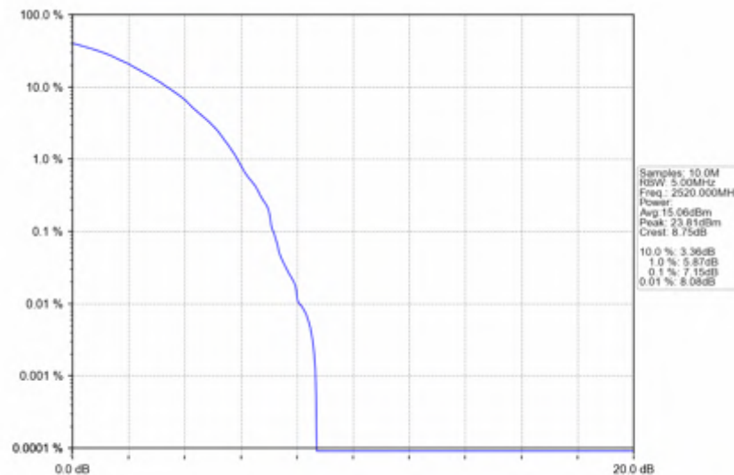
n7_30kHz_SISO_NTNV_40MHz_DFT-s-OFDM QPSK_2520MHz_Outer_Full
