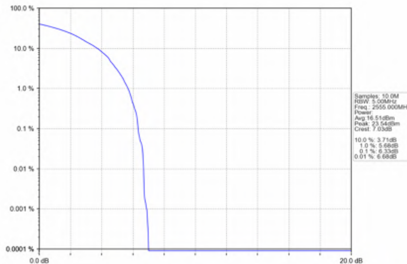
n7_30kHz_SISO_NTNV_30MHz_DFT-s-OFDM PI/2 BPSK_2555MHz_Outer_Full
