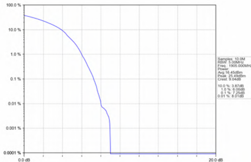
n25_15kHz_SISO_NTNV_20MHz_DFT-s-OFDM 64 QAM_1905MHz_Outer_Full
