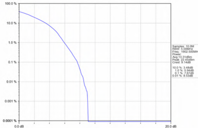
n25_15kHz_SISO_NTNV_25MHz_DFT-s-OFDM_256_QAM_1902.5MHz_Outer_Full
