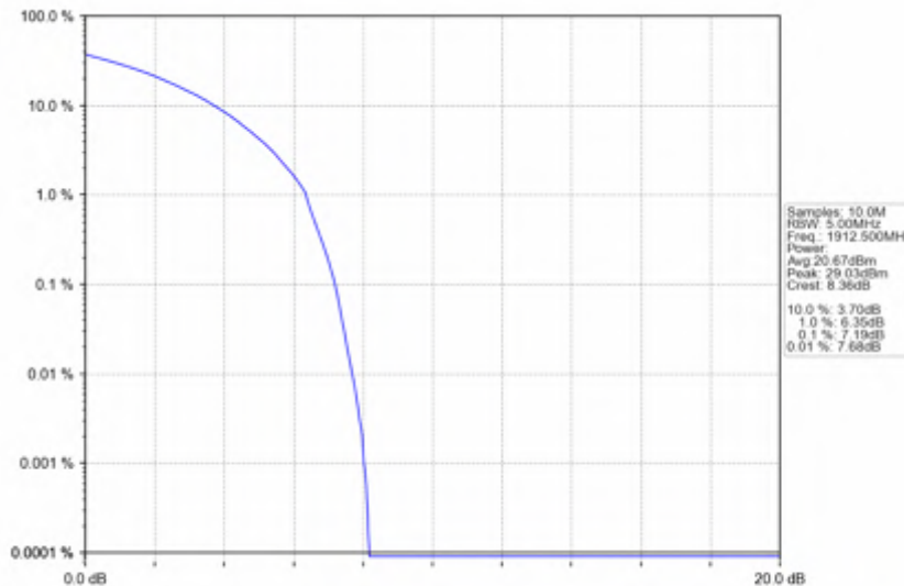
n25_15kHz_SISO_NTNV_5MHz_CP-OFDM_16_QAM_1912.5MHz_Outer_Full
