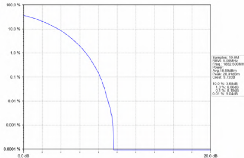
n25_15kHz_SISO_NTNV_10MHz_CP-OFDM QPSK_1882.5MHz_Outer_Full
