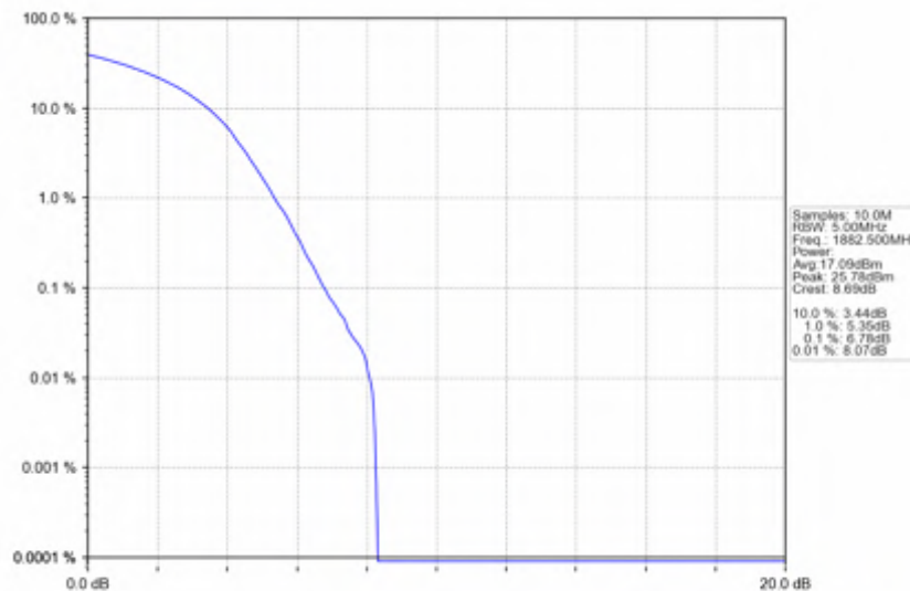
n25_30kHz_SISO_NTNV_10MHz_DFT-s-OFDM_256_QAM_1882.5MHz_Outer_Full
