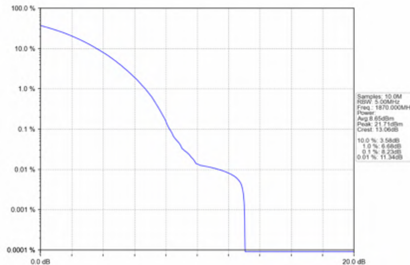
n25_15kHz_SISO_NTNV_40MHz_CP-OFDM 256 QAM_1870MHz_Outer_Full
