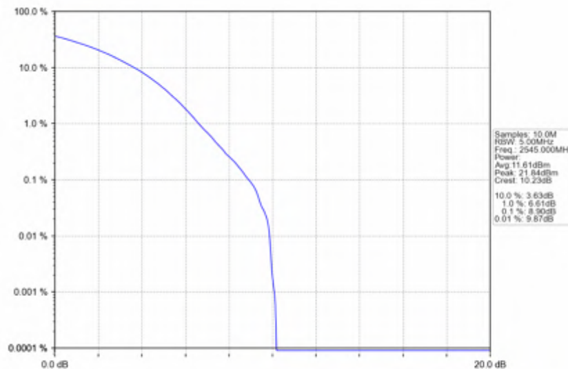
n7_30kHz_SISO_NTNV_50MHz_CP-OFDM_QPSK_2545MHz_Outer_Full
