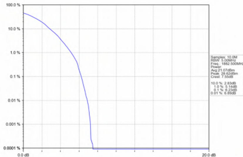
n25_15kHz_SISO_NTNV_5MHz_DFT-s-OFDM 64 QAM_1882.5MHz_Outer_Full
