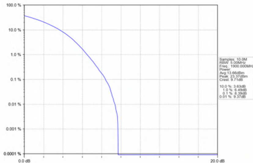
n25_15kHz_SISO_NTNV_30MHz_CP-OFDM QPSK_1900MHz_Outer_Full
