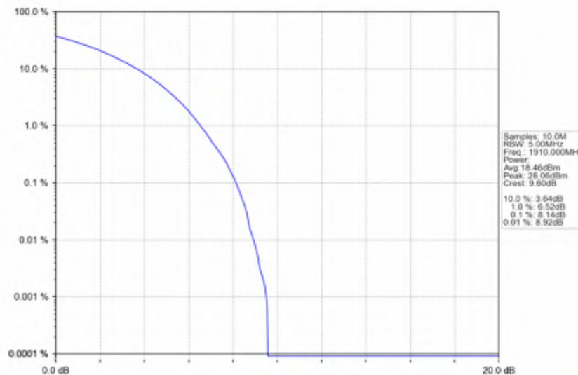
n25_15kHz_SISO_NTNV_10MHz_CP-OFDM QPSK_1910MHz_Outer_Full
