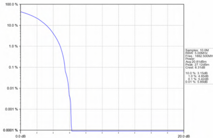
n25_15kHz_SISO_NTNV_10MHz_DFT-s-OFDM QPSK_1882.5MHz_Outer_Full
