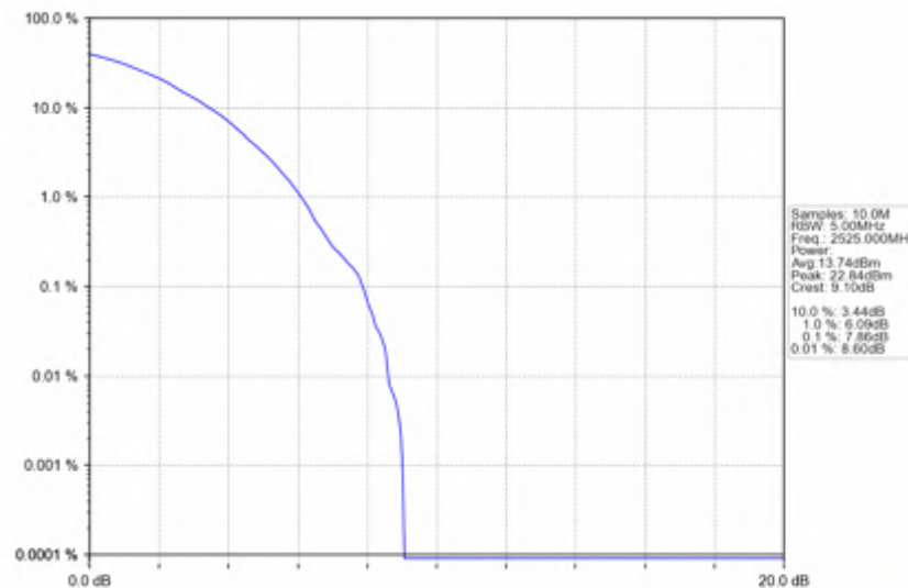
n7_30kHz_SISO_NTNV_50MHz_DFT-s-OFDM QPSK_2525MHz_Outer_Full
