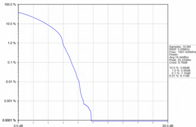
n25_15kHz_SISO_NTNV_15MHz_DFT-s-OFDM_256_QAM_1907.5MHz_Outer_Full
