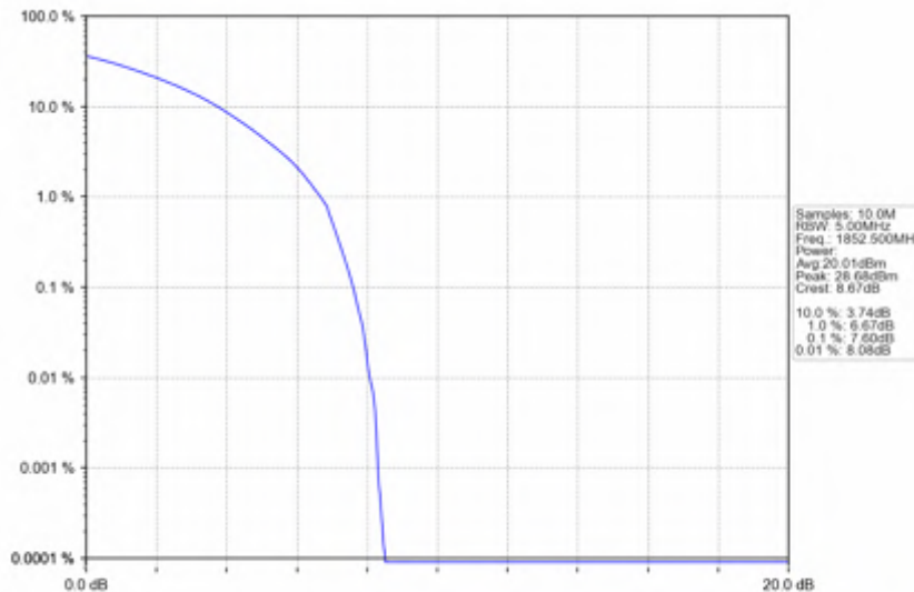
n25_15kHz_SISO_NTNV_5MHz_CP-OFDM_64_QAM_1852.5MHz_Outer_Full
