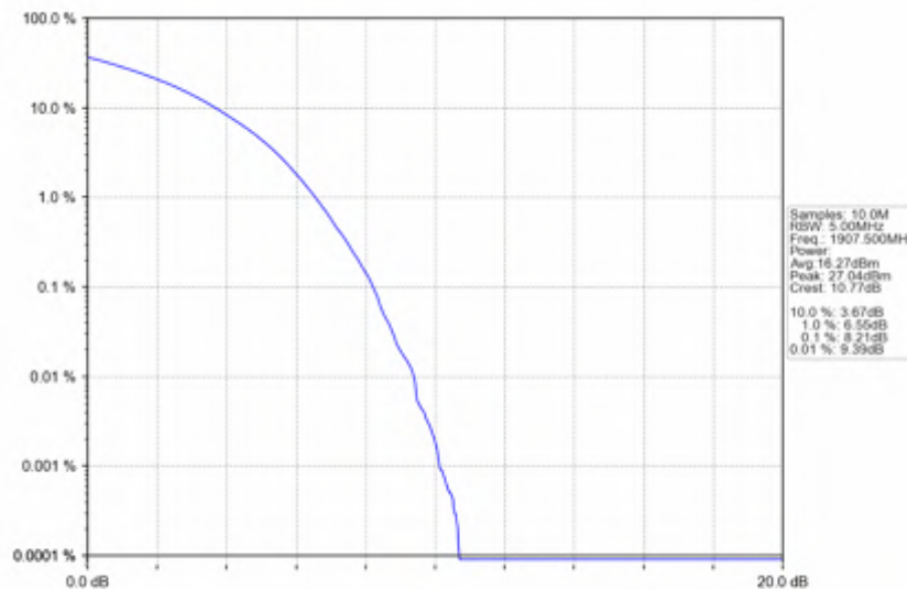
n25_15kHz_SISO_NTNV_15MHz_CP-OFDM 64 QAM_1907.5MHz_Outer_Full
