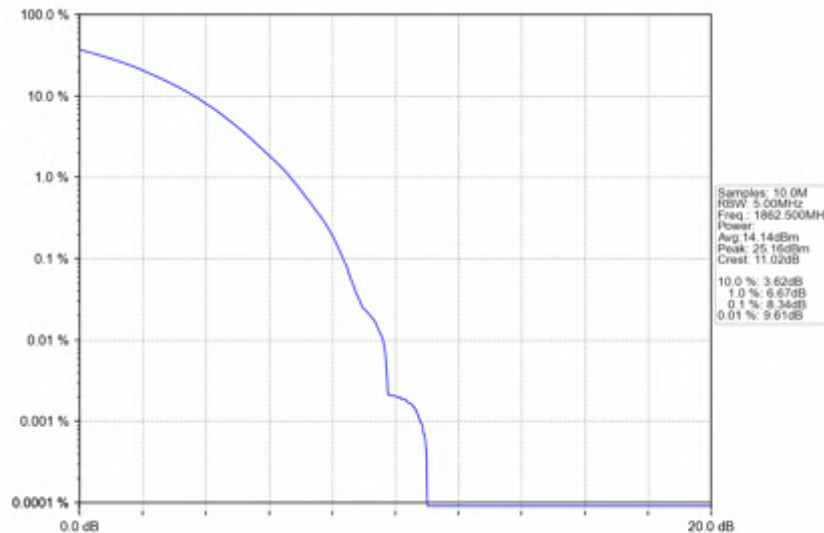
n25_15kHz_SISO_NTNV_25MHz_CP-OFDM_QPSK_1862.5MHz_Outer_Full
