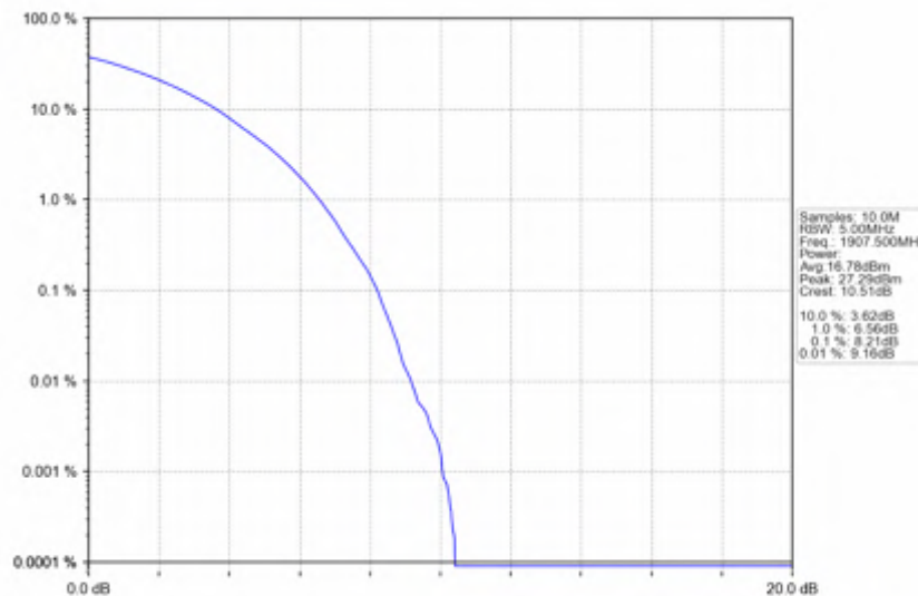
n25_15kHz_SISO_NTNV_15MHz_CP-OFDM 16 QAM_1907.5MHz_Outer_Full
