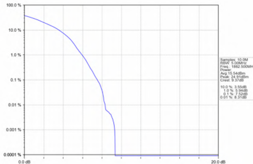
n25_15kHz_SISO_NTV_25MHz_DFT-s-OFDM_16_QAM_1882.5MHz_Outer_Full
