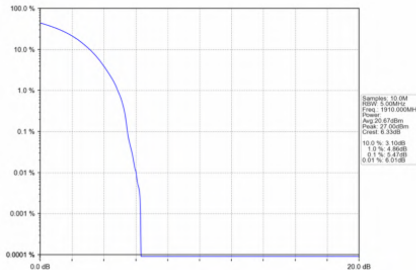
n25_15kHz_SISO_NTNV_10MHz_DFT-s-OFDM QPSK_1910MHz_Outer_Full
