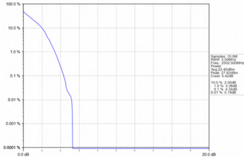
n7_15kHz_SISO_NTNV_5MHz_DFT-s-OFDM PI/2 BPSK_2502.5MHz_Outer_Full
