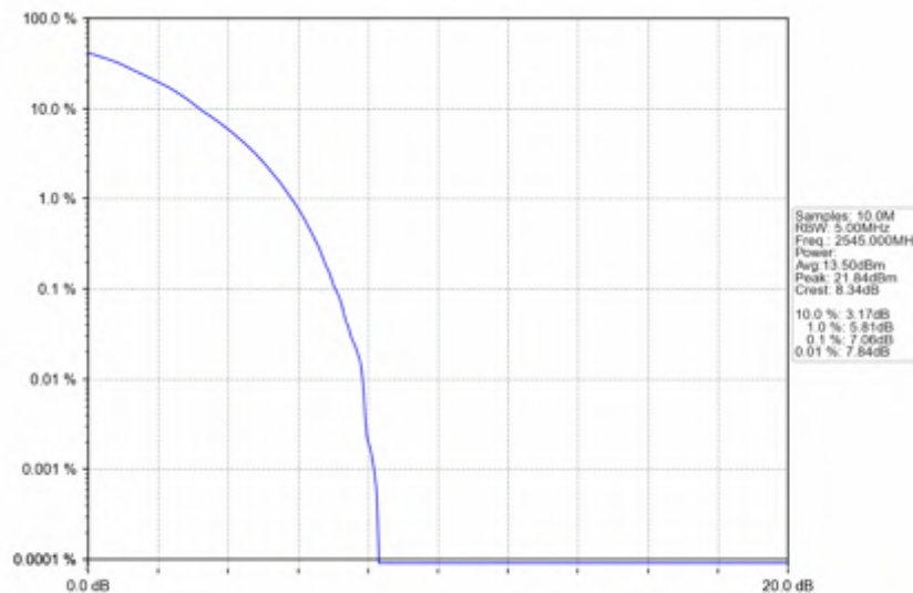
n7_15kHz_SISO_NTNV_50MHz_DFT-s-OFDM PI/2 BPSK_2545MHz_Outer_Full
