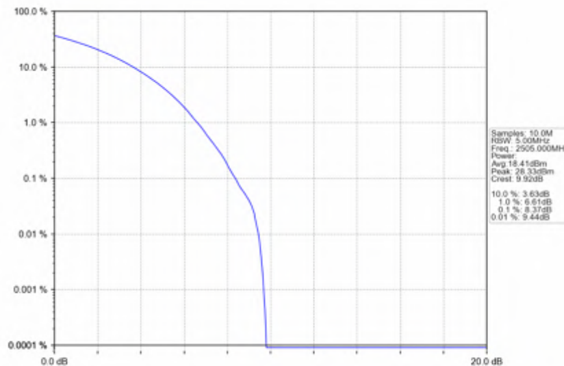
n7_30kHz_SISO_NTNV_10MHz_CP-OFDM 64 QAM_2505MHz_Outer_Full
