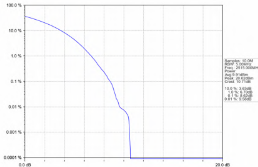
n7 15kHz SISO NTNv 30MHz CP-OFDM 256 QAM 2515MHz Outer Full
