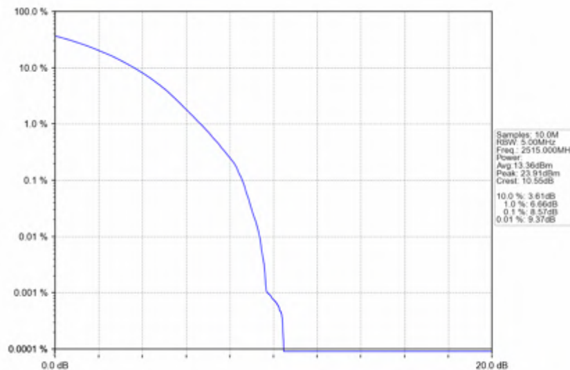
n7_15kHz_SISO_NTNV_30MHz_CP-OFDM_16_QAM_2515MHz_Outer_Full
