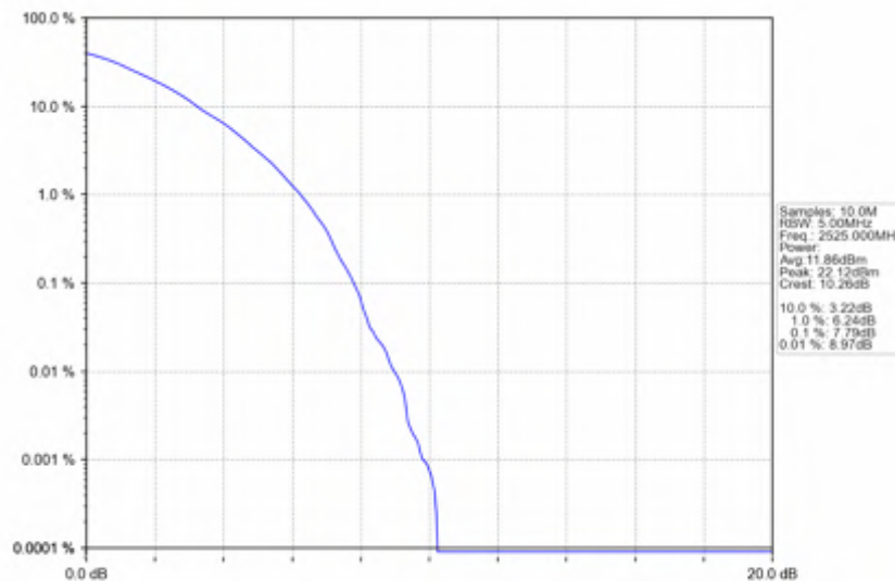
n7_15kHz_SISO_NTNV_50MHz_DFT-s-OFDM_16_QAM_2525MHz_Outer_Full
