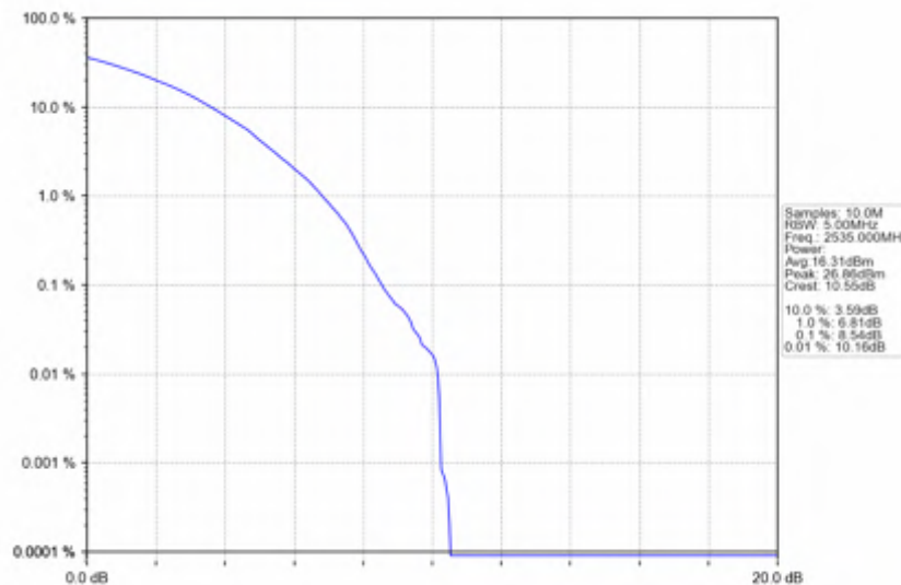
n7_15kHz_SISO_NTNV_5MHz_CP-OFDM 256 QAM 2535MHz_Outer_Full
