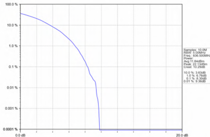
n5_30kHz_SISO_NTNV_20MHz_CP-OFDM 256 QAM_836.5MHz_Outer_Full
