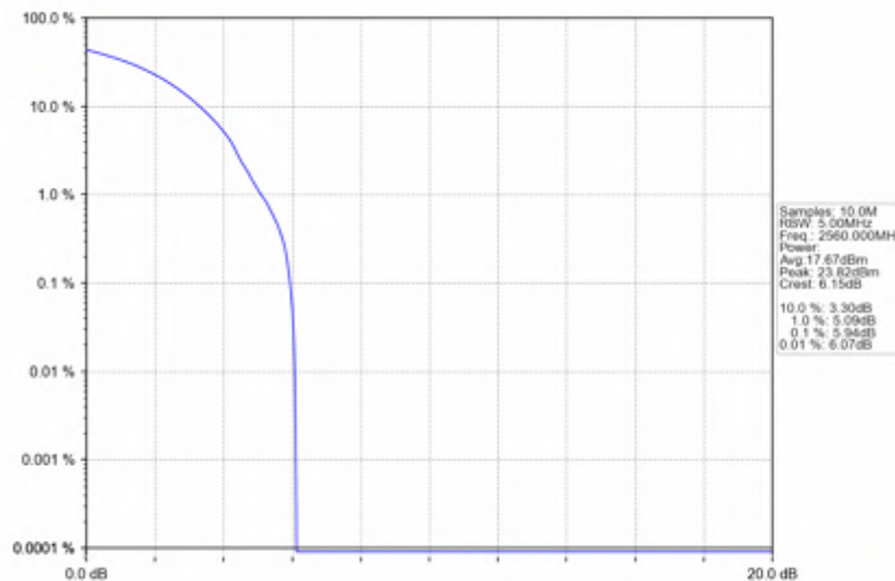
n7_15kHz_SISO_NTNV_20MHz_DFT-s-OFDM PI/2 BPSK_2560MHz_Outer_Full
