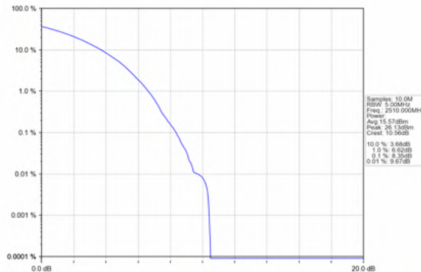
n7_30kHz_SISO_NTNV_20MHz_CP-OFDM_QPSK_2510MHz_Outer_Full
