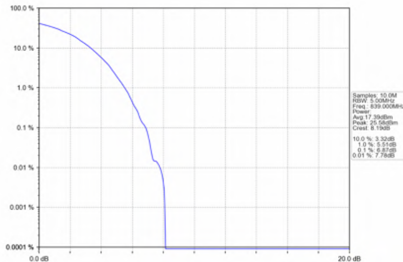
n5_30kHz_SISO_NTNV_20MHz_DFT-s-OFDM QPSK_839MHz_Outer_Full
