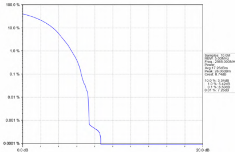
n7_30kHz_SISO_NTNV_10MHz_DFT-s-OFDM_256_QAM_2565MHz_Outer_Full
