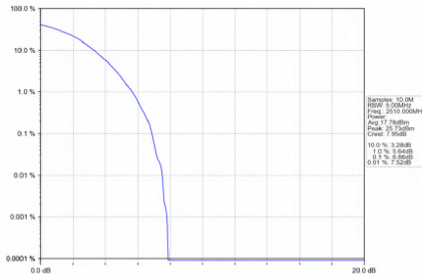
n7_30kHz_SISO_NTNV_20MHz_DFT-s-OFDM QPSK_2510MHz_Outer_Full
