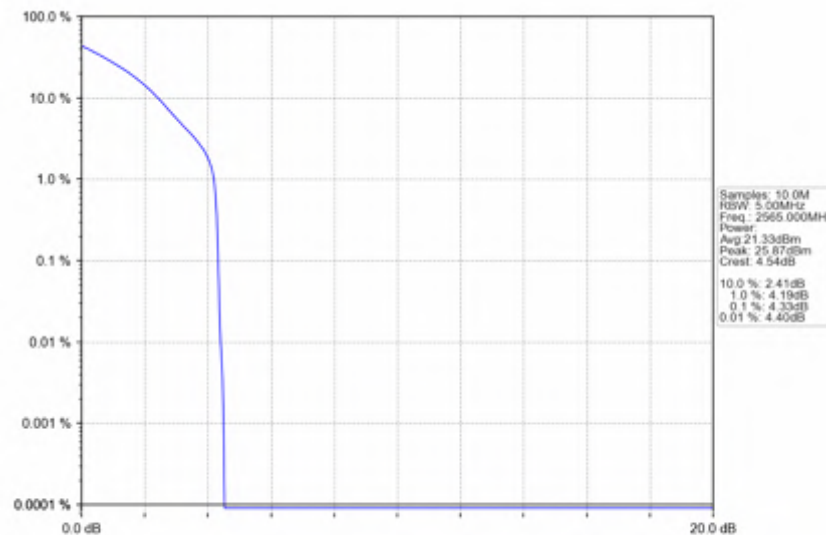
n7_30kHz_SISO_NTNV_10MHz_DFT-s-OFDM PI/2 BPSK_2565MHz_Outer_Full
