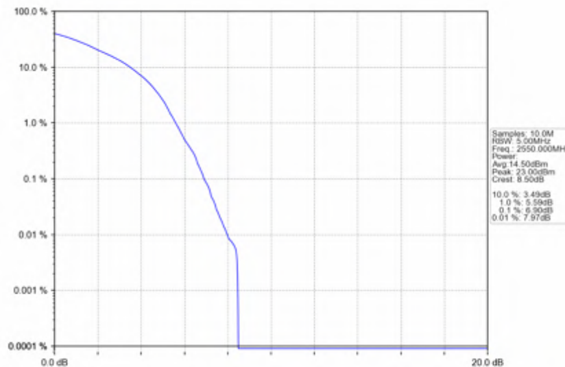
n7_15kHz_SISO_NTNV_40MHz_DFT-s-OFDM PI/2 BPSK_2550MHz_Outer_Full
