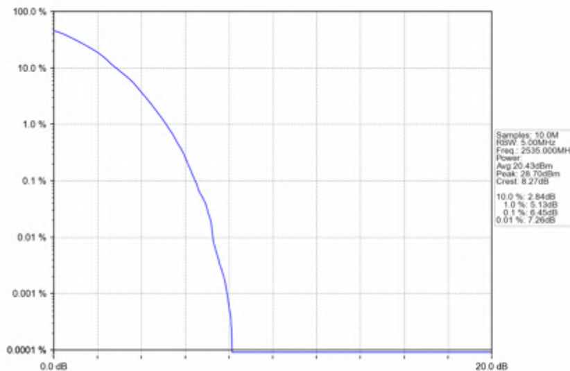
n7_15kHz_SISO_NTNV_5MHz_DFT-s-OFDM 64 QAM_2535MHz_Outer_Full
