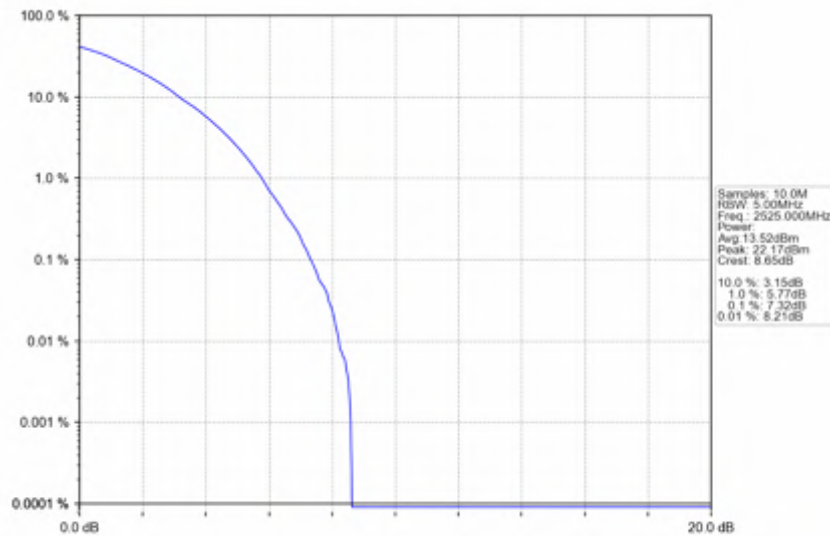
n7_15kHz_SISO_NTNV_50MHz_DFT-s-OFDM PI/2 BPSK_2525MHz_Outer_Full
