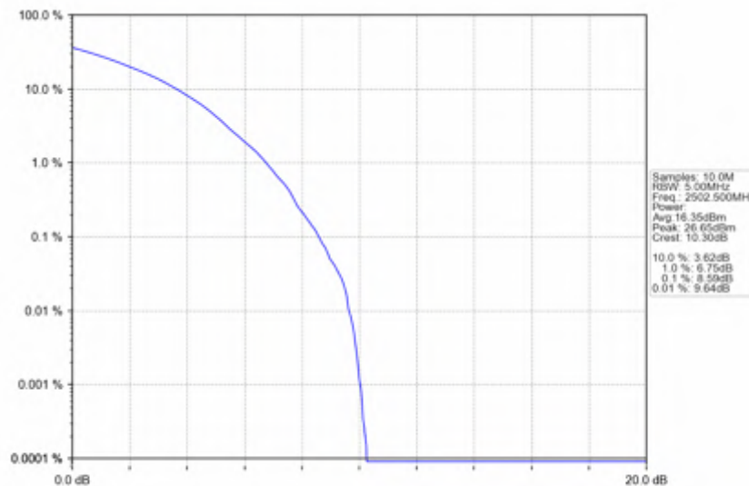
n7_15kHz_SISO_NTNV_5MHz_CP-OFDM 256 QAM 2502.5MHz_Outer_Full
