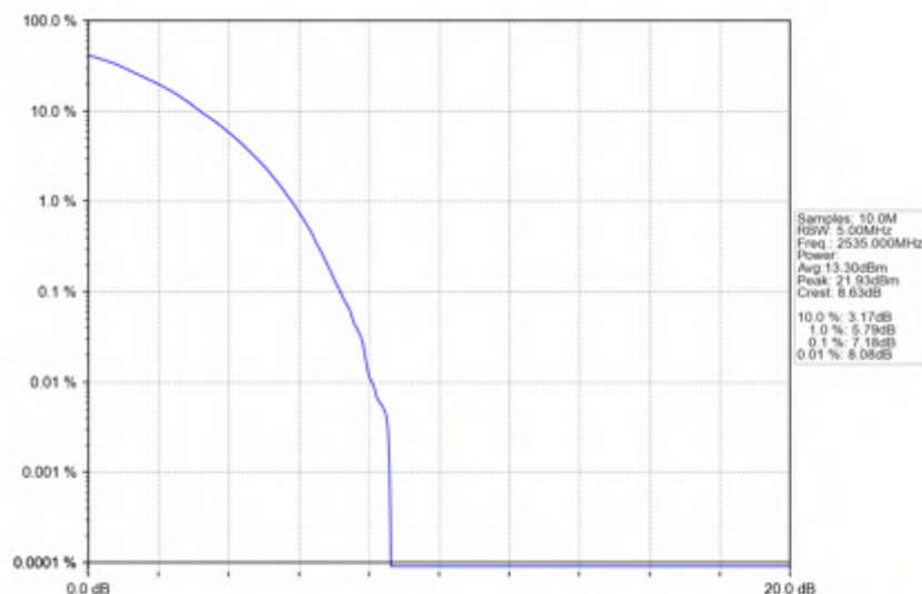
n7_15kHz_SISO_NTNV_50MHz_DFT-s-OFDM PI/2 BPSK_2535MHz_Outer_Full
