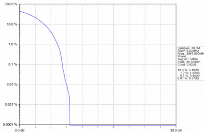
n7 15kHz SISO NTNV 10MHz DFT-s-OFDM QPSK 2565MHz Outer Full
