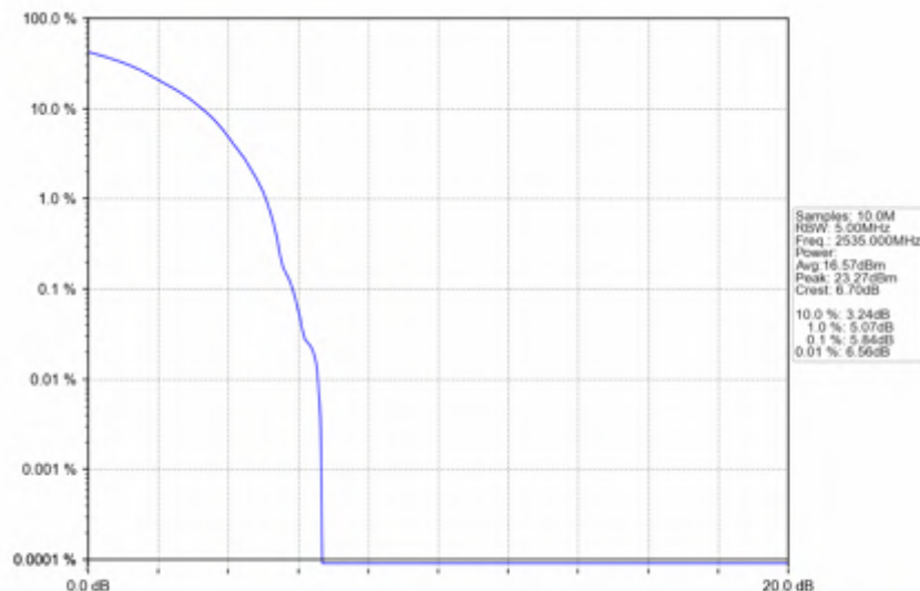
n7_15kHz_SISO_NTNV_25MHz_DFT-s-OFDM_PI/2_BPSK_2535MHz_Outer_Full
