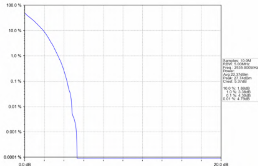
n7_15kHz_SISO_NTNV_5MHz_DFT-s-OFDM PI/2 BPSK_2535MHz_Outer_Full
