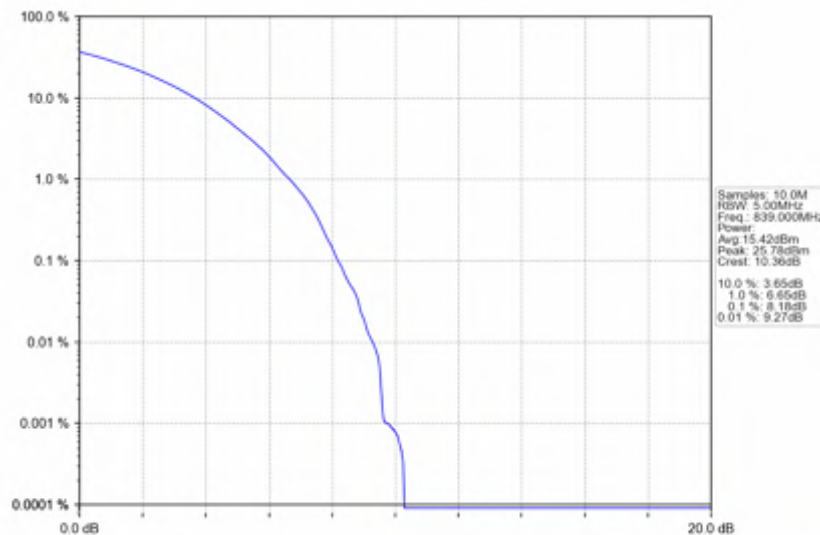
n5_30kHz_SISO_NTNV_20MHz_CP-OFDM QPSK_839MHz_Outer_Full
