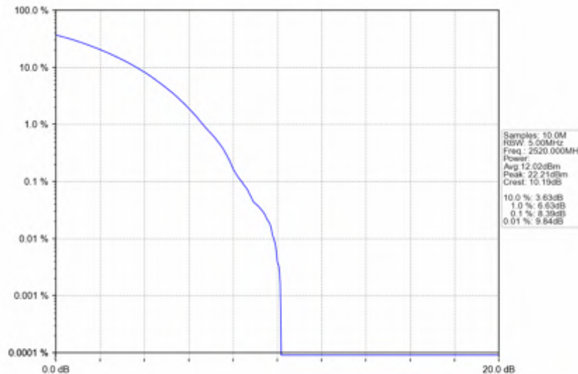
n7_15kHz_SISO_NTNV_40MHz_CP-OFDM_QPSK_2520MHz_Outer_Full
