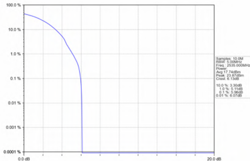
n7_15kHz_SISO_NTNV_20MHz_DFT-s-OFDM PI/2 BPSK_2535MHz_Outer_Full
