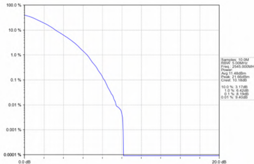
n7_15kHz_SISO_NTNV_50MHz_DFT-s-OFDM_64_QAM_2545MHz_Outer_Full
