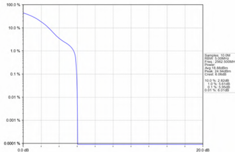
n7_15kHz_SISO_NTNV_15MHz_DFT-s-OFDM PI/2 BPSK_2562.5MHz_Outer_Full
