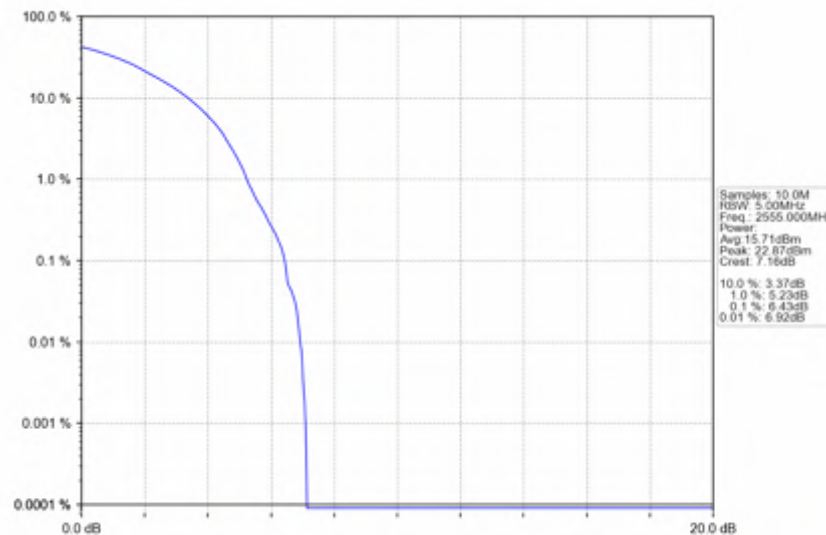
n7_15kHz_SISO_NTNV_30MHz_DFT-s-OFDM PI/2 BPSK_2555MHz_Outer_Full
