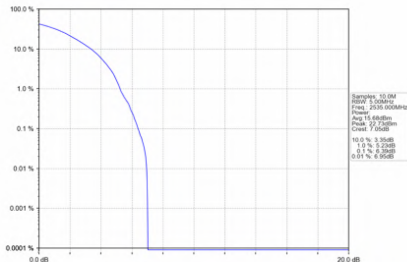
n7_15kHz_SISO_NTNV_30MHz_DFT-s-OFDM PI/2 BPSK_2535MHz_Outer_Full
