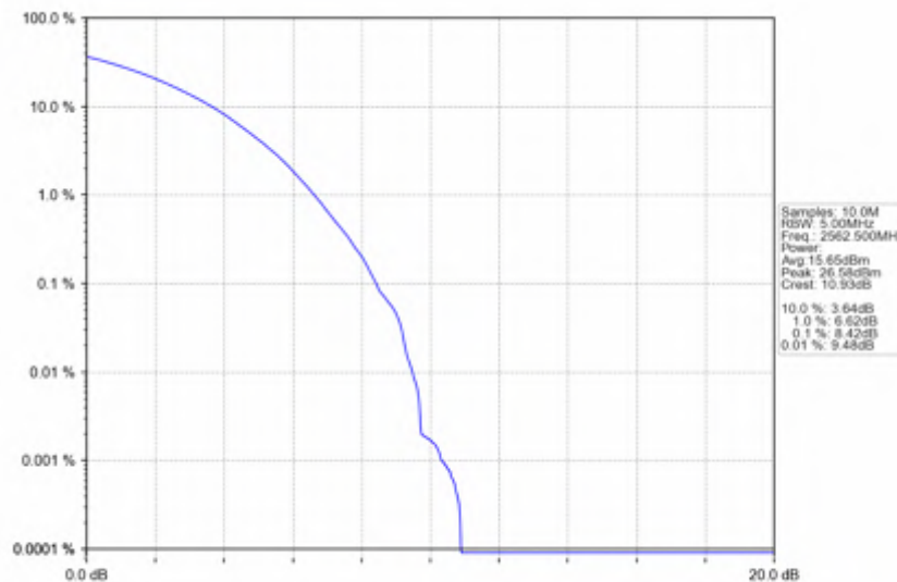
n7_15kHz_SISO_NTNV_15MHz_CP-OFDM 64 QAM_2562.5MHz_Outer_Full
