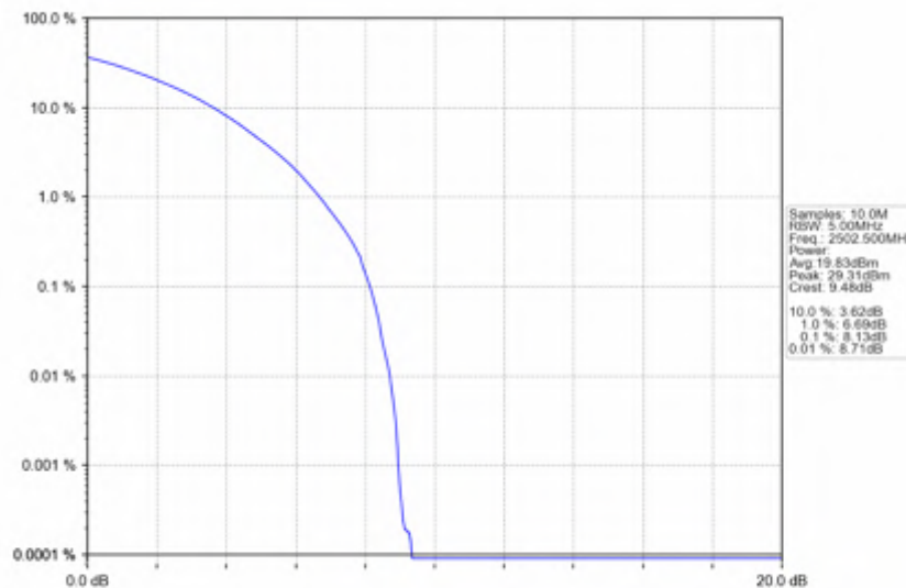
n7_15kHz_SISO_NTNV_5MHz_CP-OFDM_16_QAM_2502.5MHz_Outer_Full
