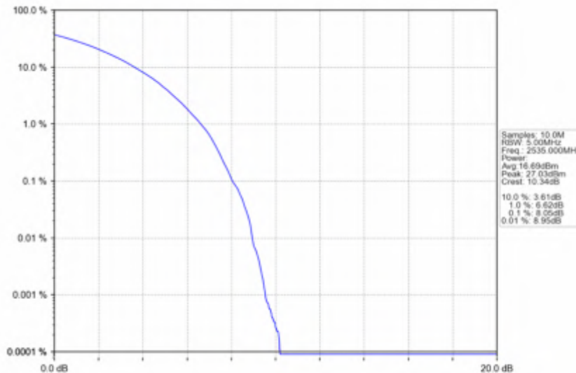
n7_30kHz_SISO_NTNV_15MHz_CP-OFDM_16_QAM_2535MHz_Outer_Full
