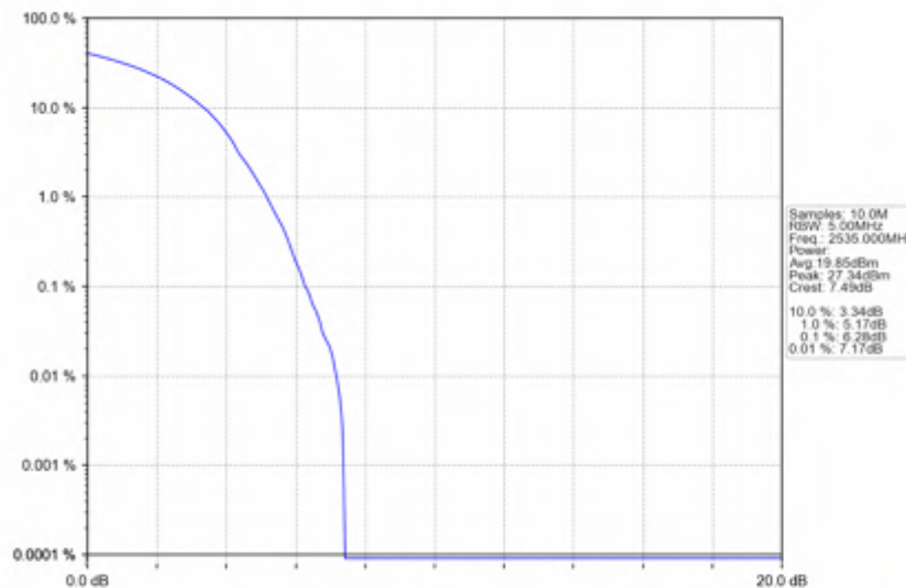
n7_30kHz_SISO_NTNV_10MHz_DFT-s-OFDM_16_QAM_2535MHz_Outer_Full
