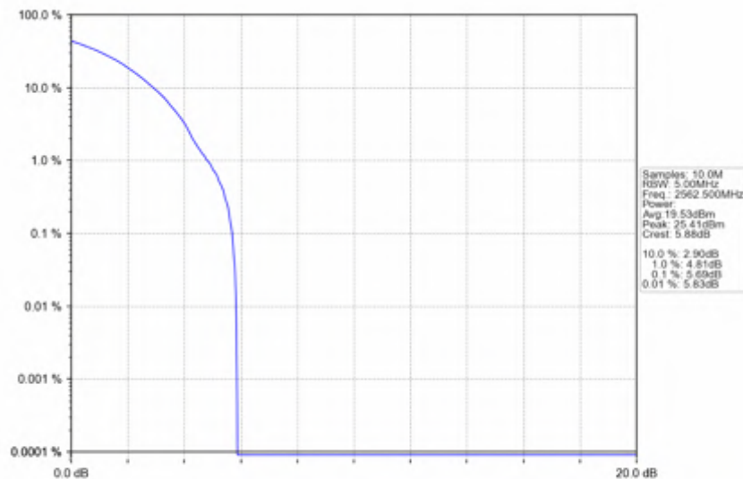
n7_30kHz_SISO_NTNV_15MHz_DFT-s-OFDM PI/2 BPSK_2562.5MHz_Outer_Full
