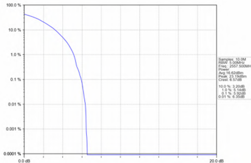
n7_15kHz_SISO_NTNV_25MHz_DFT-s-OFDM PI/2 BPSK_2557.5MHz_Outer_Full
