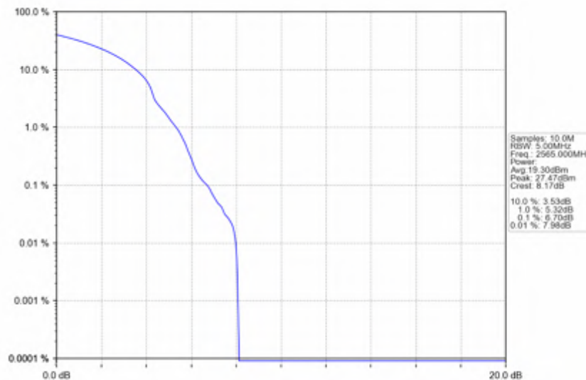
n7_30kHz_SISO_NTNV_10MHz_DFT-s-OFDM_64_QAM_2565MHz_Outer_Full
