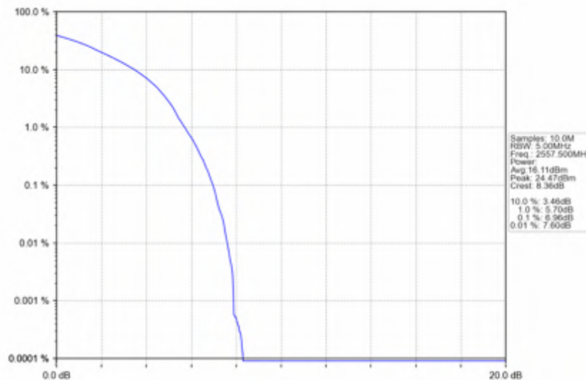
n7_15kHz_SISO_NTNV_25MHz_DFT-s-OFDM QPSK_2557.5MHz_Outer_Full
