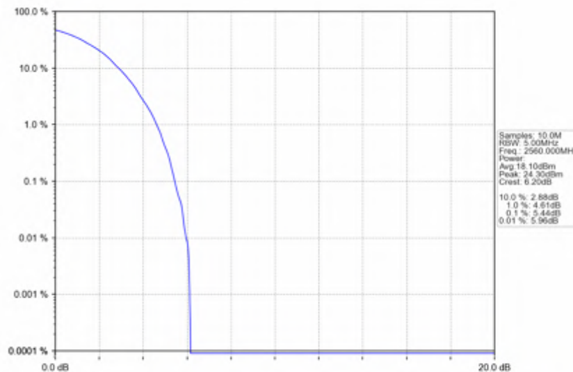
n7_30kHz_SISO_NTNV_20MHz_DFT-s-OFDM PI/2 BPSK_2560MHz_Outer_Full
