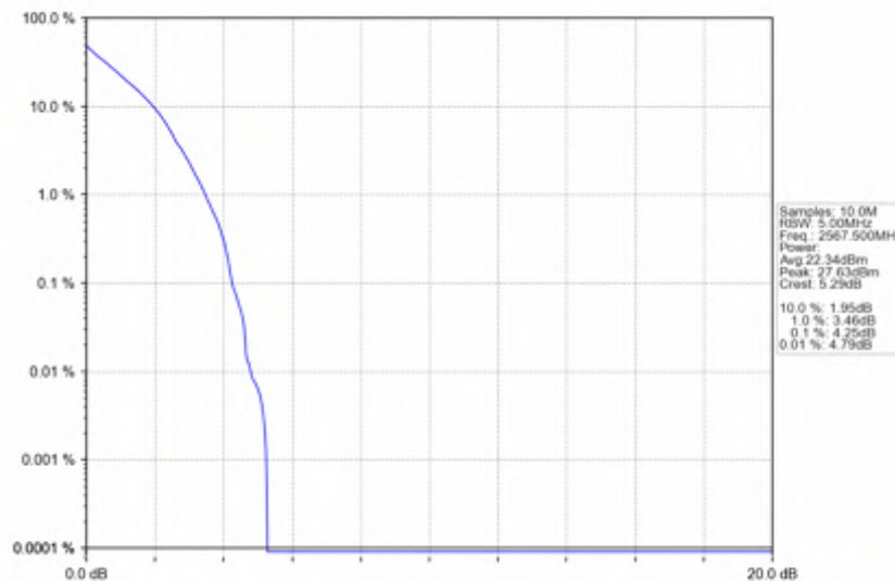
n7_15kHz_SISO_NTNV_5MHz_DFT-s-OFDM PI/2 BPSK_2567.5MHz_Outer_Full
