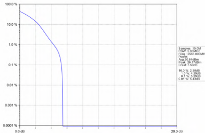
n7_15kHz_SISO_NTNV_10MHz_DFT-s-OFDM PI/2 BPSK_2565MHz_Outer_Full
