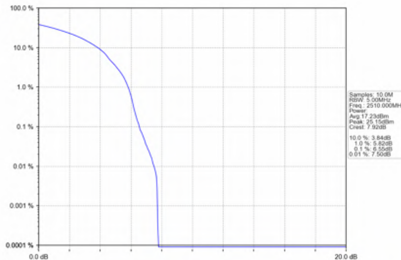
n7_15kHz_SISO_NTNV_20MHz_DFT-s-OFDM QPSK_2510MHz_Outer_Full
