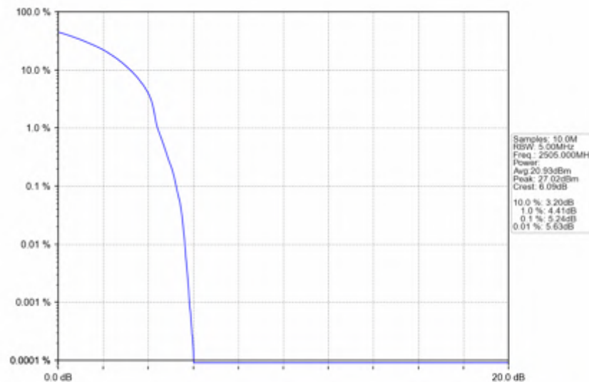
n7_30kHz_SISO_NTNV_10MHz_DFT-s-OFDM QPSK_2505MHz_Outer_Full
