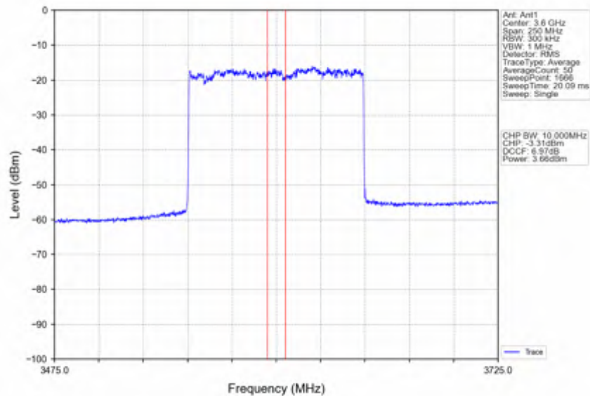
n78d_30kHz_SISO_NTNV_100MHz_CP-OFDM 64 QAM_3600MHz_Inner_Full
