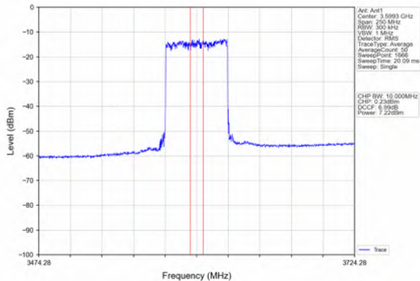
n78d_30kHz_SISO_NTNV_100MHz_DFT-s-OFDM 256 QAM_3600MHz_Inner_Full
