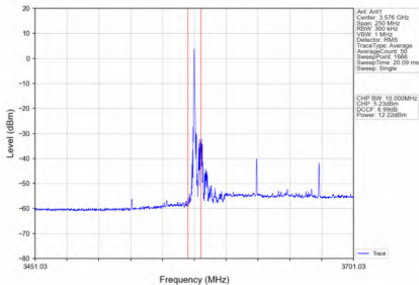
n78d_30kHz_SISO_NTNV_100MHz_CP-OFDM 256 QAM_3624.99MHz_Edge_1RB_Right
