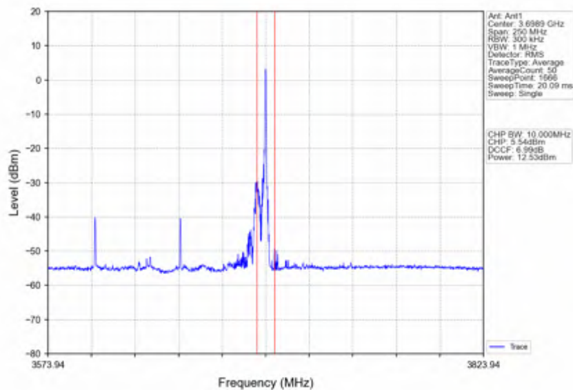
n78d_30kHz_SISO_NTNV_100MHz_CP-OFDM QPSK_3649.98MHz_Edge_1RB_Right
