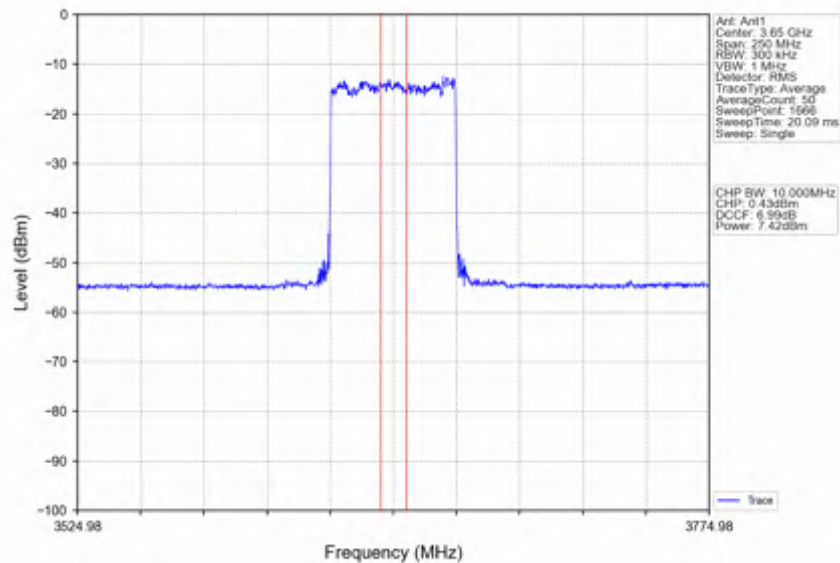
n78d_30kHz_SISO_NTNV_100MHz_CP-OFDM 64 QAM_3649.98MHz_Inner_Full
