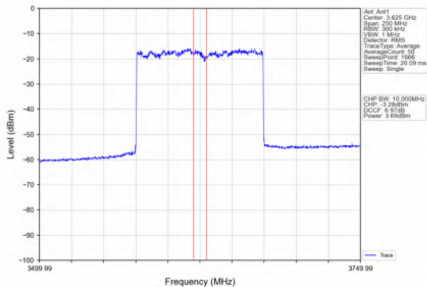
n78d 30kHz SISO NTNV 100MHz CP-OFDM 16 QAM 3624.99MHz Inner Full
