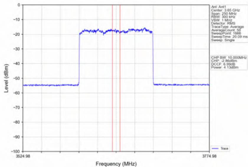
n78d 30kHz SISO NTNV 100MHz CP-OFDM 16 QAM 3649.98MHz Inner Full
