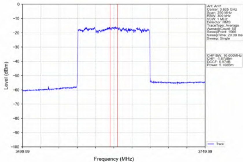
n78d_30kHz_SISO_NTNV_100MHz_CP-OFDM 256 QAM_3624.99MHz_Inner_Full
