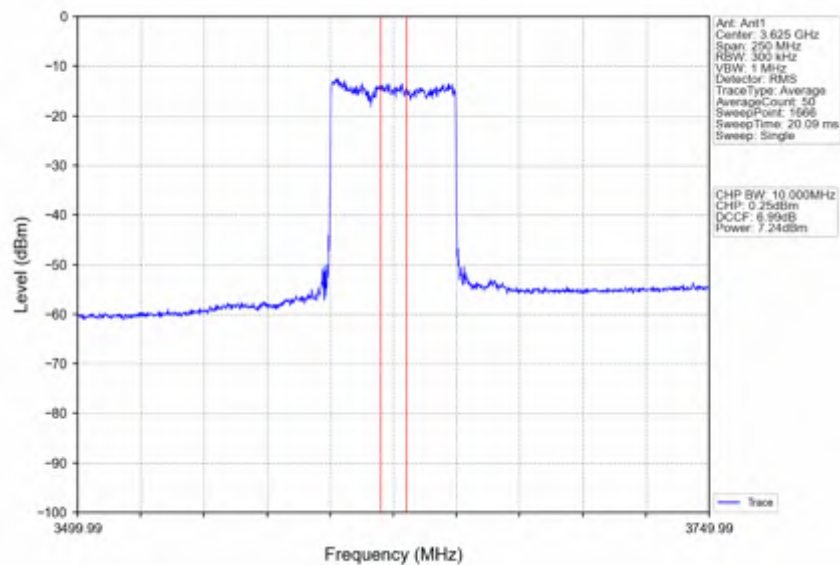
n78d_30kHz_SISO_NTNV_100MHz_CP-OFDM 64 QAM_3624.99MHz_Inner_Full
