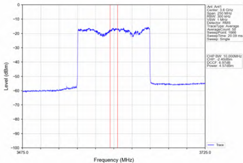
n78d 30kHz SISO NTNv 100MHz CP-OFDM QPSK 3600MHz Inner Full
