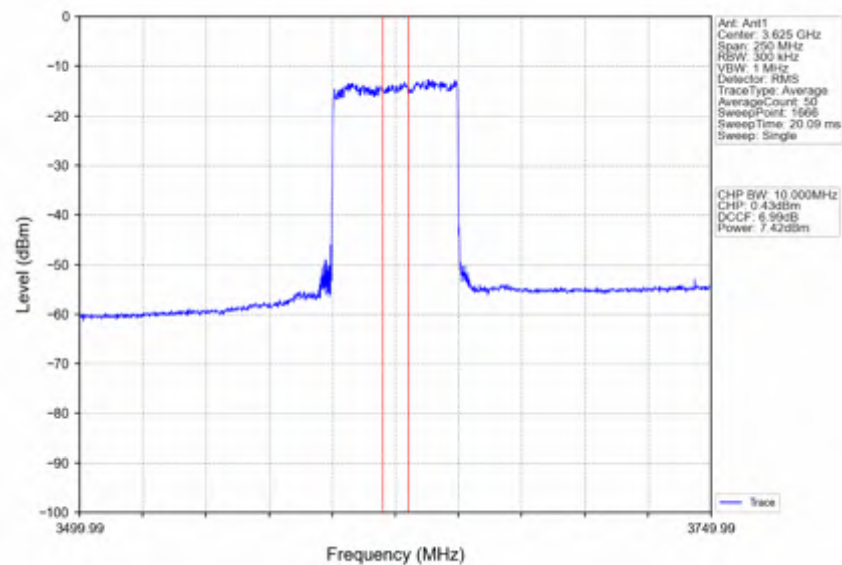
n78d_30kHz_SISO_NTNV_100MHz_CP-OFDM QPSK_3624.99MHz_Inner_Full
