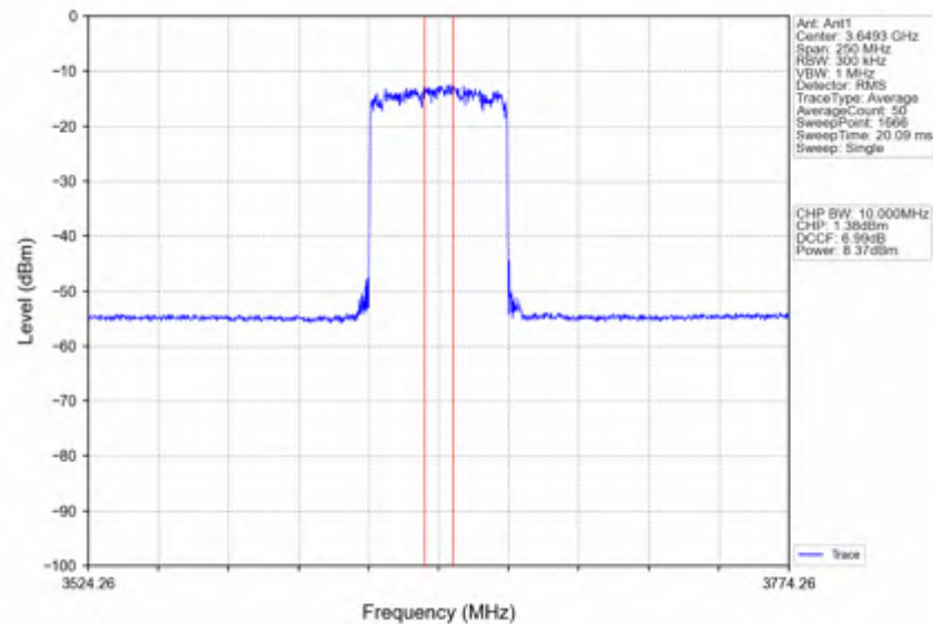
n78d_30kHz_SISO_NTNV_100MHz_DFT-s-OFDM 64 QAM_3649.98MHz_Inner_Full
