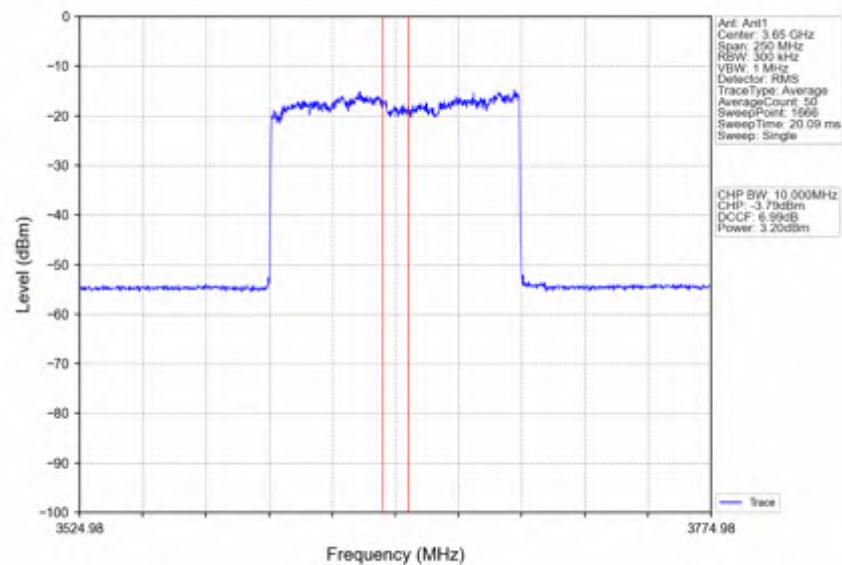
n78d_30kHz_SISO_NTNV_100MHz_CP-OFDM QPSK_3649.98MHz_Inner_Full
