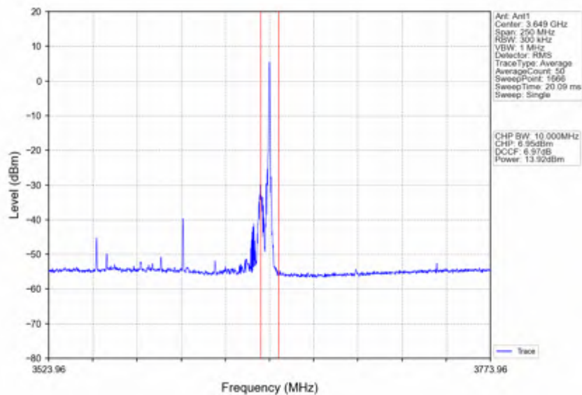
n78d_30kHz_SISO_NTNV_100MHz_DFT-s-OFDM_256_QAM_3600MHz_Edge_1RB_Right
