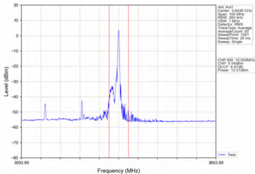
n78d_30kHz_SISO_NTNV_40MHz_DFT-s-OFDM 64 QAM_3624.99MHz_Edge_1RB_Right
