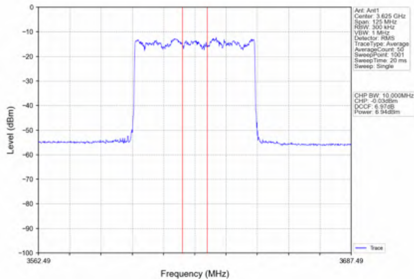
n78d_30kHz_SISO_NTNV_50MHz_CP-OFDM 16 QAM 3624.99MHz_Inner_Full
