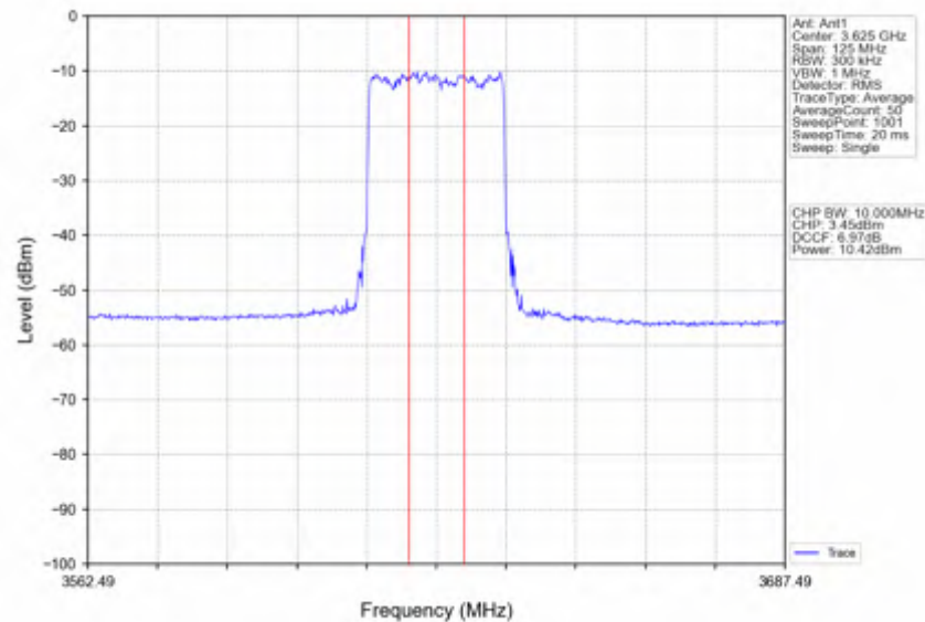
n78d_30kHz_SISO_NTNV_50MHz_CP-OFDM QPSK_3624.99MHz_Inner_Full
