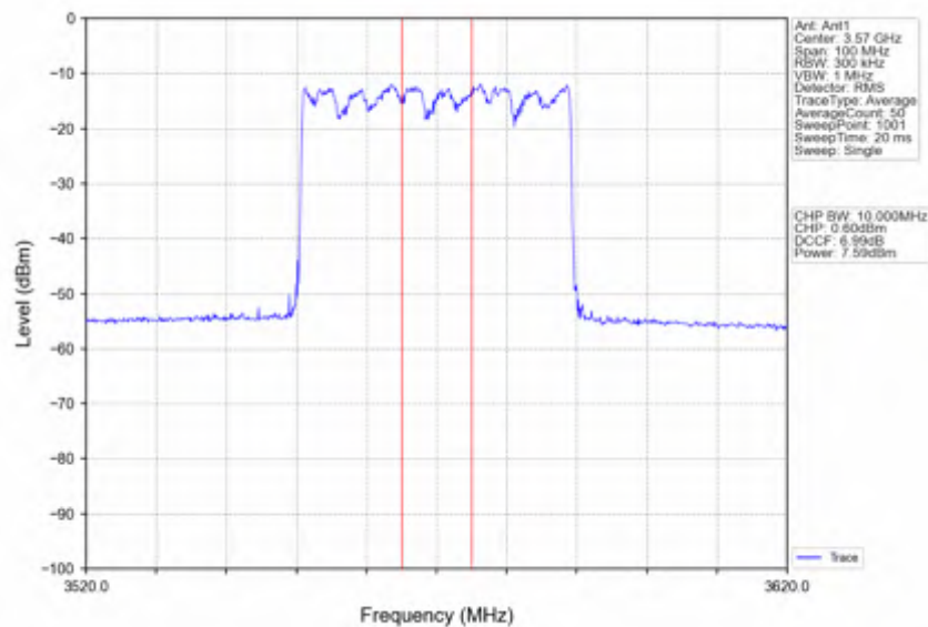
n78d_30kHz_SISO_NTV_40MHz_CP-OFDM_64_QAM_3570MHz_Inner_Full
