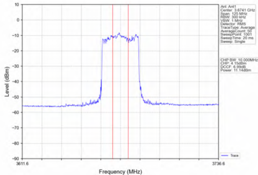
n78d_30kHz_SISO_NTNV_50MHz_DFT-s-OFDM QPSK_3675MHz_Inner_Full
