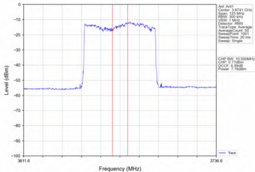
n78d_30kHz_SISO_NTNV_50MHz_DFT-s-OFDM PI/2 BPSK_3675MHz_Inner_Full
