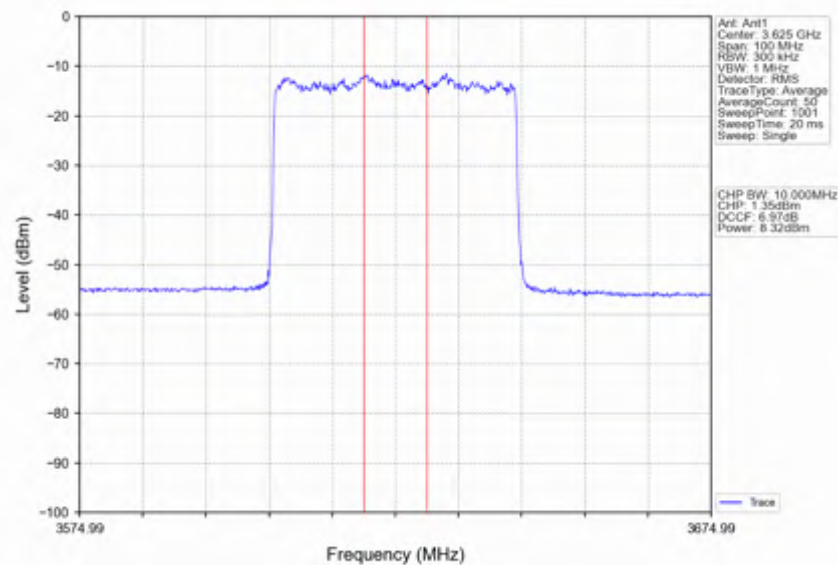
n78d 30kHz SISO NTV 40MHz CP-OFDM QPSK 3624.99MHz Inner Full
