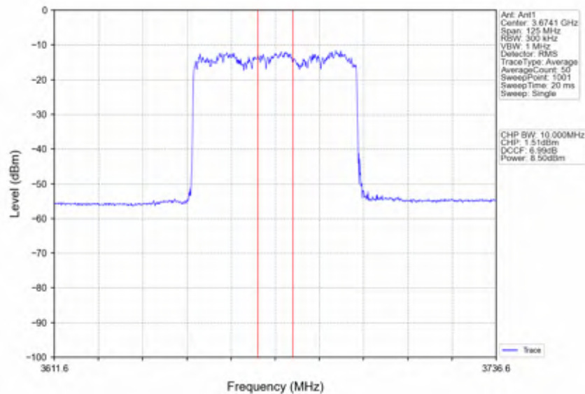
n78d_30kHz_SISO_NTNV_50MHz_DFT-s-OFDM 64 QAM_3675MHz_Inner_Full
