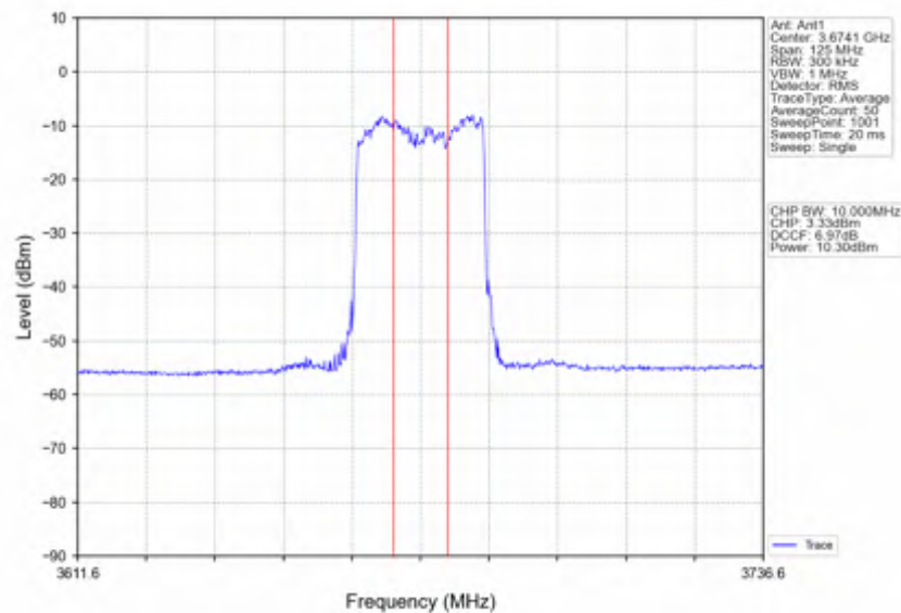
n78d_30kHz_SISO_NTNV_50MHz_DFT-s-OFDM_256_QAM_3675MHz_Inner_Full
