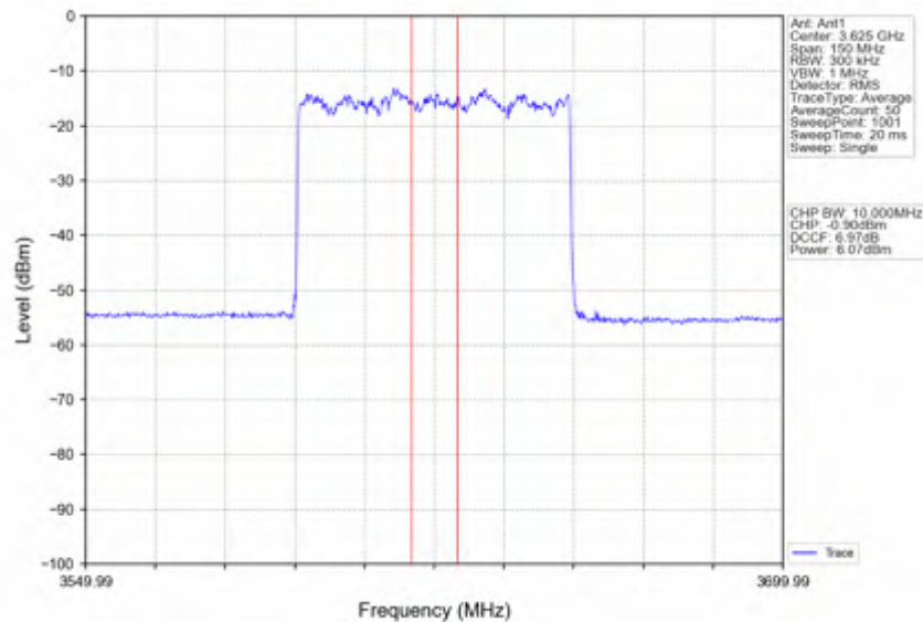
n78d_30kHz_SISO_NTNV_60MHz_DFT-s-OFDM_QPSK_3624.99MHz_Inner_Full
