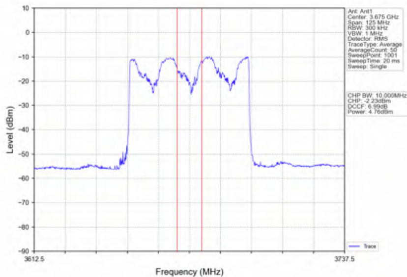
n78d_30kHz_SISO_NTNV_50MHz_CP-OFDM 64 QAM_3675MHz_Inner_Full
