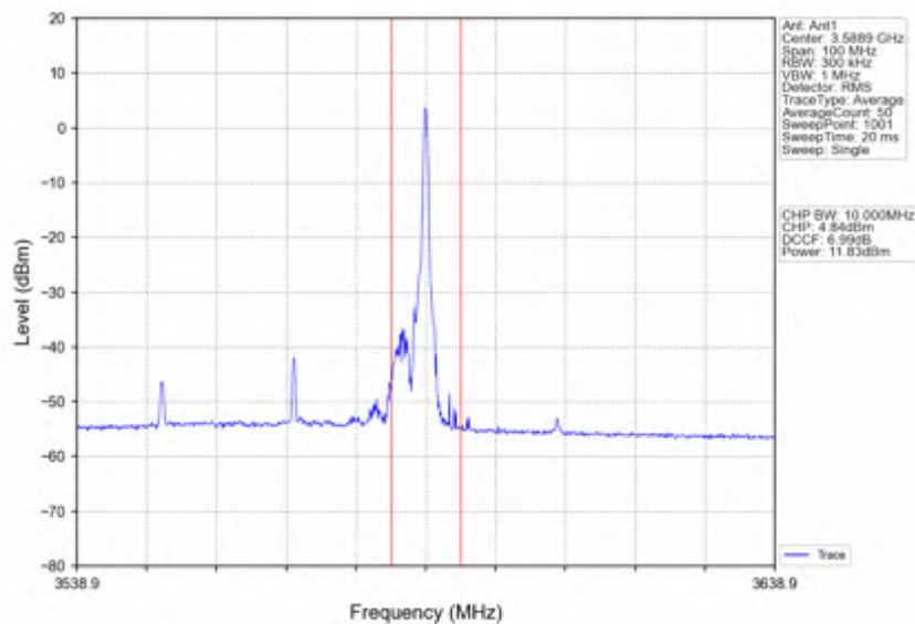
n78d_30kHz_SISO_NTNV_40MHz_CP-OFDM QPSK_3570MHz_Edge_1RB_Right
