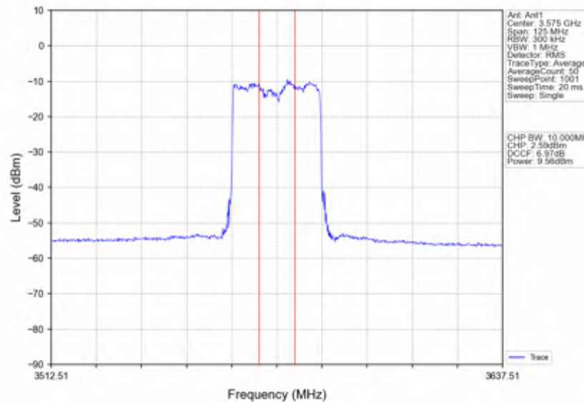
n78d_30kHz_SISO_NTNV_50MHz_CP-OFDM 64 QAM_3575.01MHz_Inner_Full
