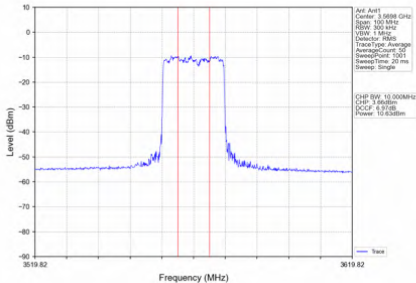
n78d_30kHz_SISO_NTNV_40MHz_CP-OFDM_QPSK_3570MHz_Inner_Full
