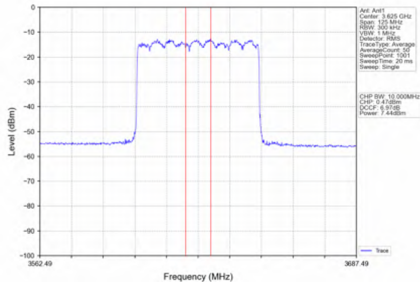
n78d_30kHz_SISO_NTNV_50MHz_CP-OFDM_256_QAM_3624.99MHz_Inner_Full
