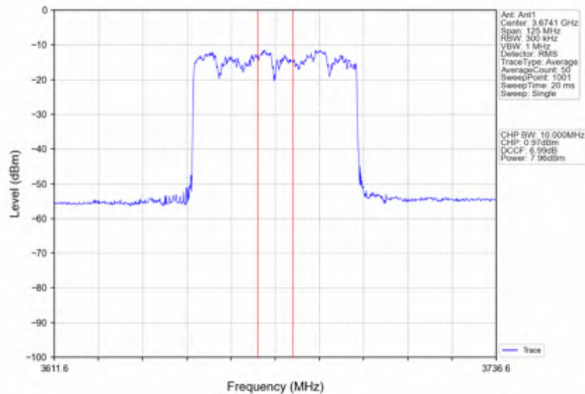
n78d_30kHz_SISO_NTNV_50MHz_DFT-s-OFDM QPSK_3675MHz_Inner_Full
