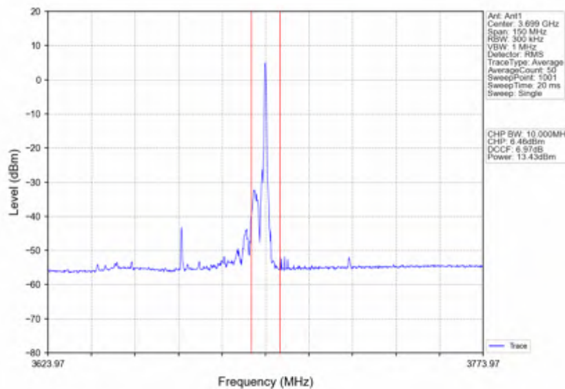
n78d_30kHz_SISO_NTNV_60MHz_DFT-s-OFDM PI/2 BPSK_3669.99MHz_Edge_1RB_Right
