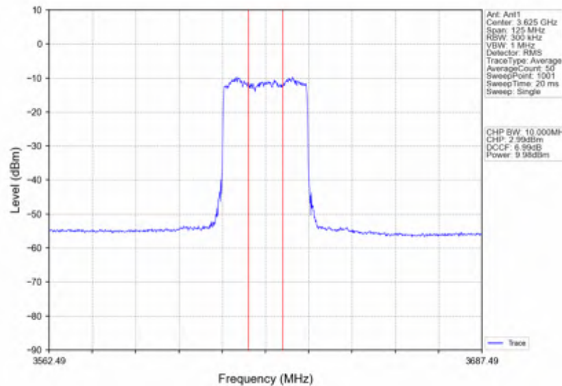
n78d_30kHz_SISO_NTNV_50MHz_CP-OFDM_256_QAM_3624.99MHz_Inner_Full
