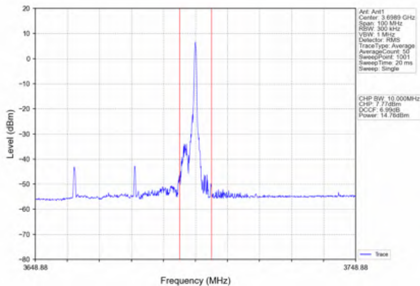
n78d_30kHz_SISO_NTNV_40MHz_DFT-s-OFDM 64 QAM_3679.98MHz_Edge_1RB_Right
