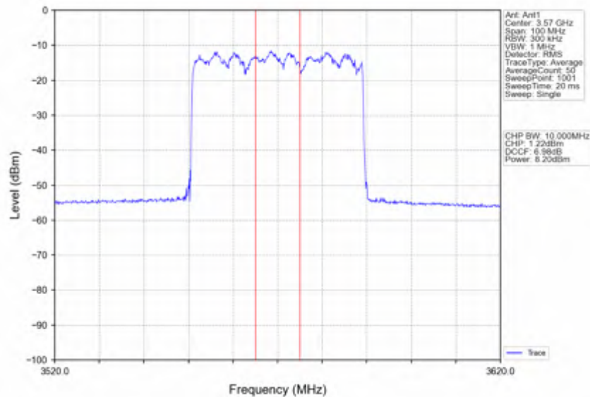
n78d_30kHz_SISO_NTNV_40MHz_CP-OFDM_256_QAM_3570MHz_Inner_Full
