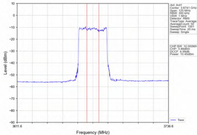
n78d_30kHz_SISO_NTNV_50MHz_DFT-s-OFDM PI/2 BPSK_3675MHz_Inner_Full
