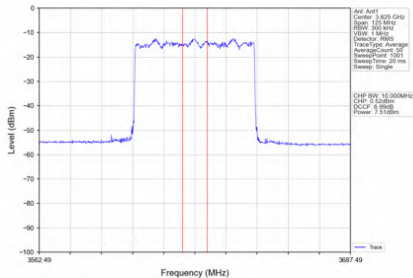
n78d_30kHz_SISO_NTNV_50MHz_CP-OFDM 64 QAM_3624.99MHz_Inner_Full
