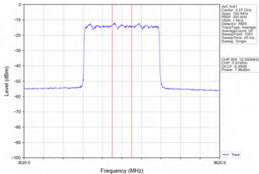
n78d_30kHz_SISO_NTNV_40MHz_CP-OFDM_QPSK_3570MHz_Inner_Full
