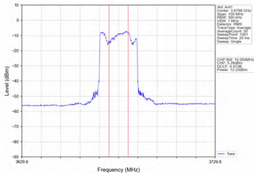
n78d_30kHz_SISO_NTNV_40MHz_CP-OFDM 256 QAM_3679.98MHz_Inner_Full
