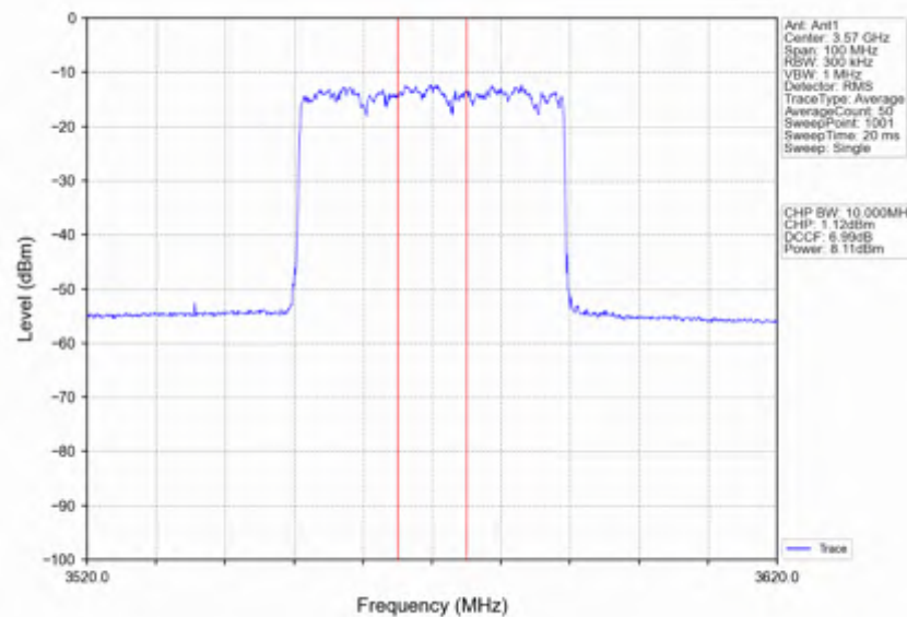
n78d_30kHz_SISO_NTV_40MHz_CP-OFDM_16_QAM_3570MHz_Inner_Full
