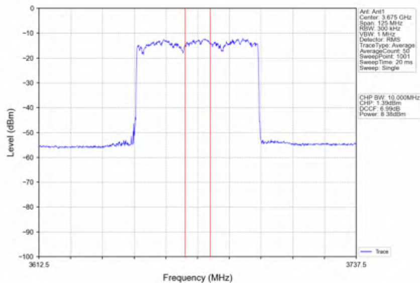
n78d_30kHz_SISO_NTNV_50MHz_CP-OFDM 16 QAM_3675MHz_Inner_Full
