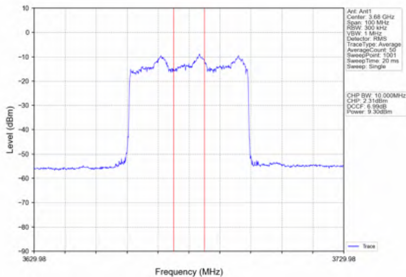
n78d_30kHz_SISO_NTNV_40MHz_CP-OFDM 16 QAM_3679.98MHz_Inner_Full
