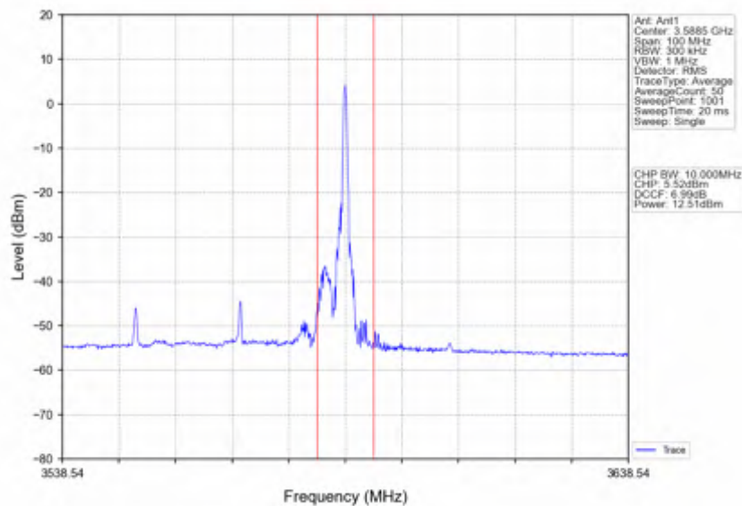
n78d_30kHz_SISO_NTNV_40MHz_CP-OFDM_16 QAM_3570MHz_Inner_1RB_Right
