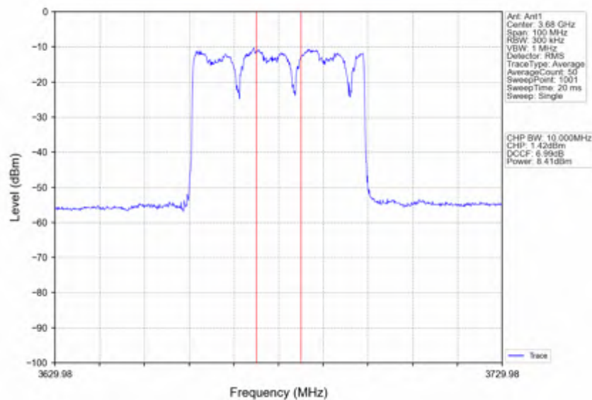
n78d_30kHz_SISO_NTNV_40MHz_CP-OFDM 256 QAM_3679.98MHz_Inner_Full
