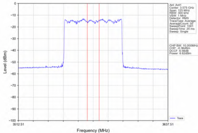
n78d_30kHz_SISO_NTNV_50MHz_CP-OFDM_256_QAM_3575.01MHz_Inner_Full
