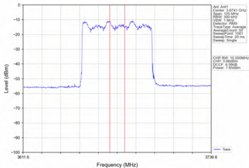
n78d_30kHz_SISO_NTNV_50MHz_DFT-s-OFDM_256_QAM_3675MHz_Inner_Full
