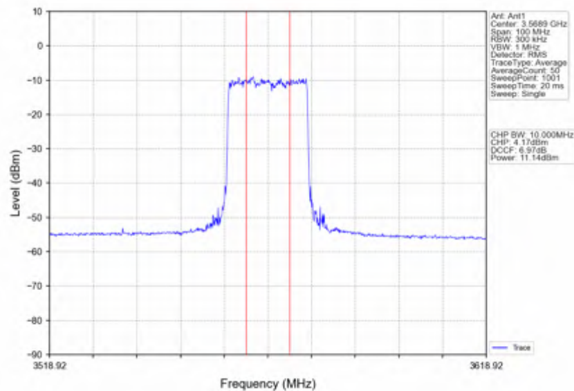
n78d_30kHz_SISO_NTNV_40MHz_DFT-s-OFDM_256_QAM_3570MHz_Inner_Full
