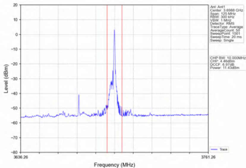
n78d_30kHz_SISO_NTNV_50MHz_DFT-s-OFDM 16 QAM_3675MHz_Edge_1RB_Right
