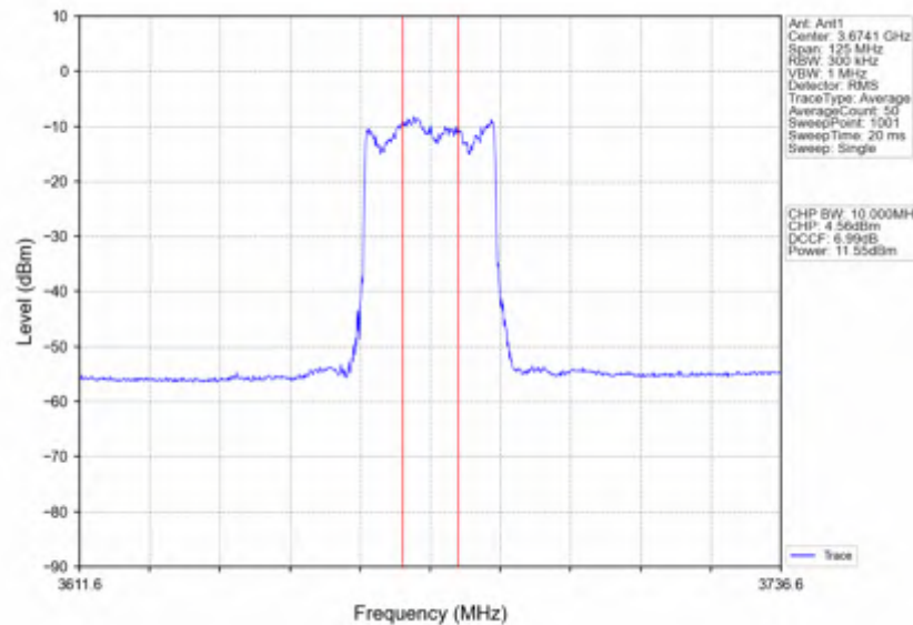
n78d_30kHz_SISO_NTNV_50MHz_DFT-s-OFDM 64 QAM_3675MHz_Inner_Full
