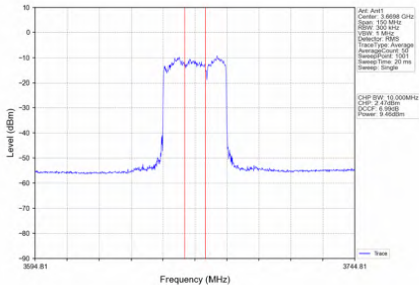
n78d_30kHz_SISO_NTNV_60MHz_DFT-s-OFDM_QPSK_3669.99MHz_Inner_Full
