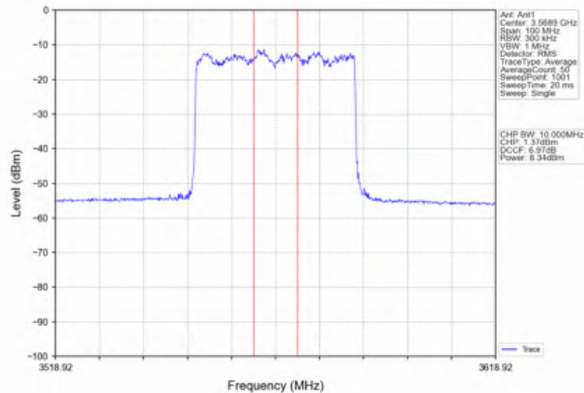
n78d_30kHz_SISO_NTNV_40MHz_DFT-s-OFDM 16 QAM_3570MHz_Inner_Full
