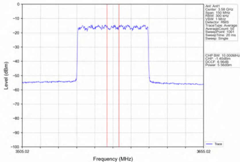
n78d_30kHz_SISO_NTNV_60MHz_DFT-s-OFDM_QPSK_3580.02MHz_Inner_Full
