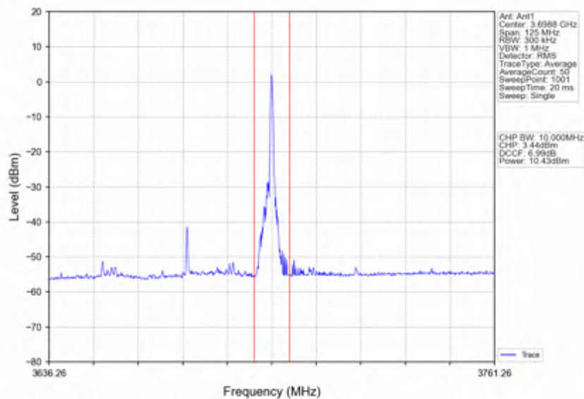
n78d_30kHz_SISO_NTNV_50MHz_DFT-s-OFDM PI/2 BPSK_3675MHz_Edge_1RB_Right
