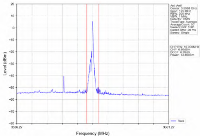
n78d_30kHz_SISO_NTNV_50MHz_DFT-s-OFDM 64 QAM_3575.01MHz_Edge_1RB_Right
