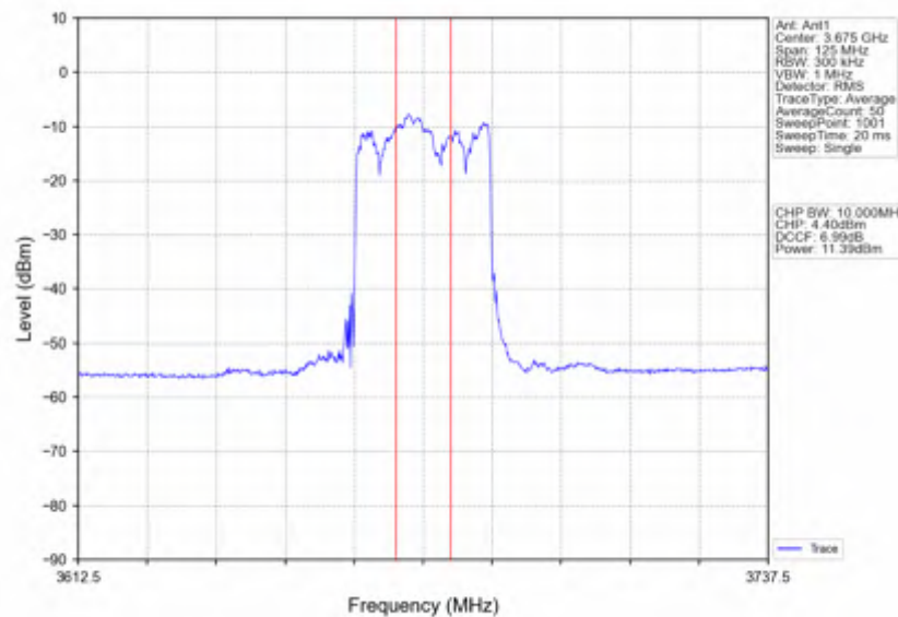
n78d_30kHz_SISO_NTNV_50MHz_CP-OFDM_256_QAM_3675MHz_Inner_Full
