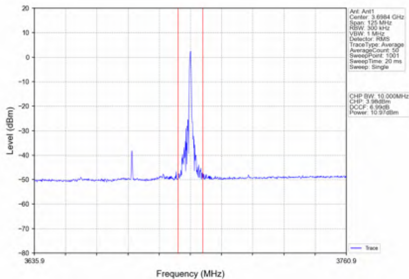
n78d_30kHz_SISO_NTNV_50MHz_CP-OFDM 64 QAM_3675MHz_Inner_1RB_Right
