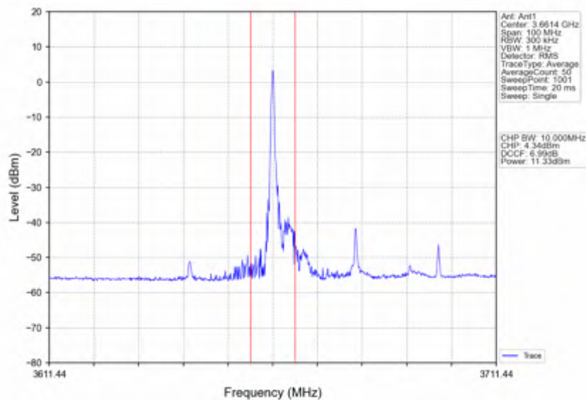
n78d_30kHz_SISO_NTNV_40MHz_DFT-s-OFDM_QPSK_3679.98MHz_Inner_1RB_Right
