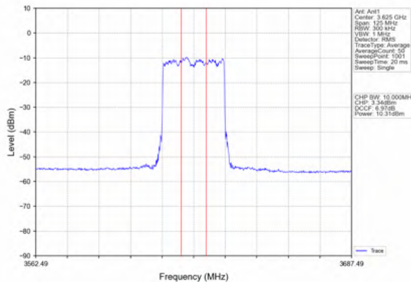
n78d_30kHz_SISO_NTNV_50MHz_CP-OFDM 64 QAM_3624.99MHz_Inner_Full
