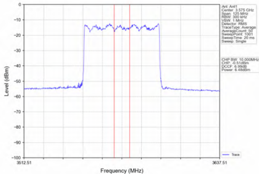
n78d_30kHz_SISO_NTNV_50MHz_CP-OFDM 64 QAM_3575.01MHz_Inner_Full
