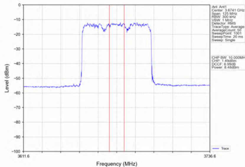
n78d_30kHz_SISO_NTNV_50MHz_DFT-s-OFDM 16 QAM_3675MHz_Inner_Full
