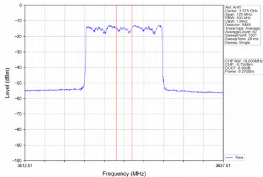
n78d_30kHz_SISO_NTNV_50MHz_CP-OFDM QPSK_3575.01MHz_Inner_Full
