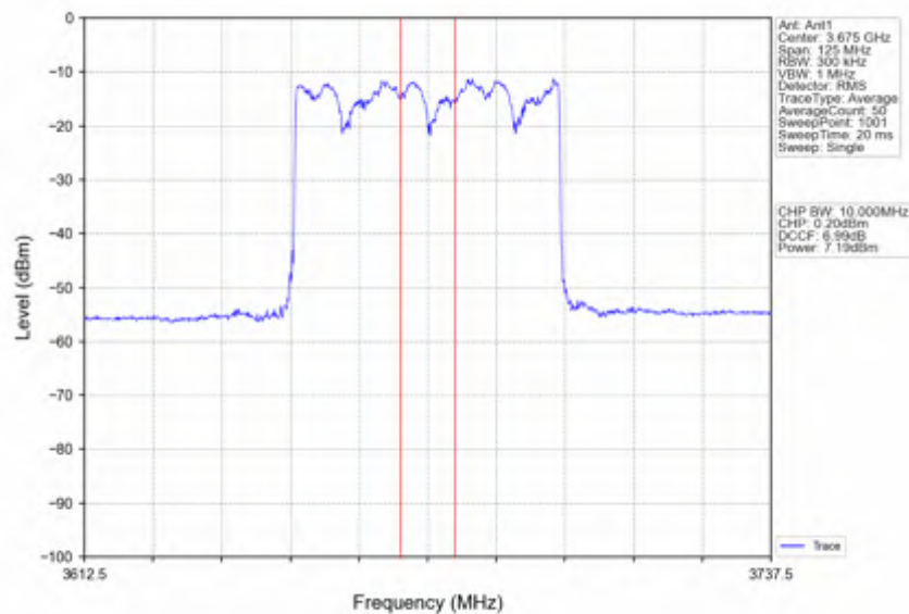
n78d_30kHz_SISO_NTNV_50MHz_CP-OFDM_QPSK_3675MHz_Inner_Full
