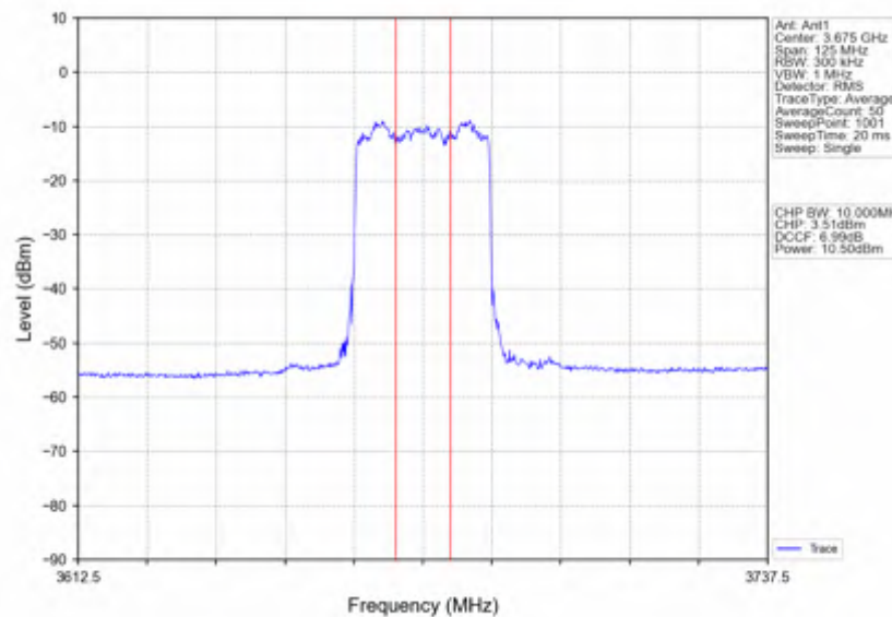
n78d_30kHz_SISO_NTNV_50MHz_CP-OFDM 16 QAM_3675MHz_Inner_Full
