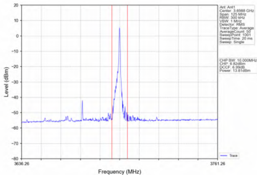
n78d_30kHz_SISO_NTNV_50MHz_DFT-s-OFDM QPSK_3675MHz_Edge_1RB_Right
