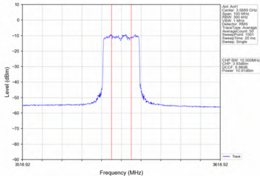
n78d_30kHz_SISO_NTNV_40MHz_DFT-s-OFDM 16 QAM_3570MHz_Inner_Full
