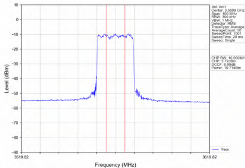
n78d_30kHz_SISO_NTV_40MHz_CP-OFDM_16_QAM_3570MHz_Inner_Full
