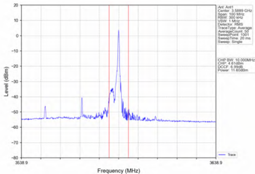
n78d_30kHz_SISO_NTNV_40MHz_CP-OFDM 64 QAM_3570MHz_Edge_1RB_Right
