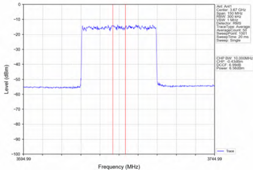
n78d_30kHz_SISO_NTNV_60MHz_DFT-s-OFDM_QPSK_3669.99MHz_Inner_Full
