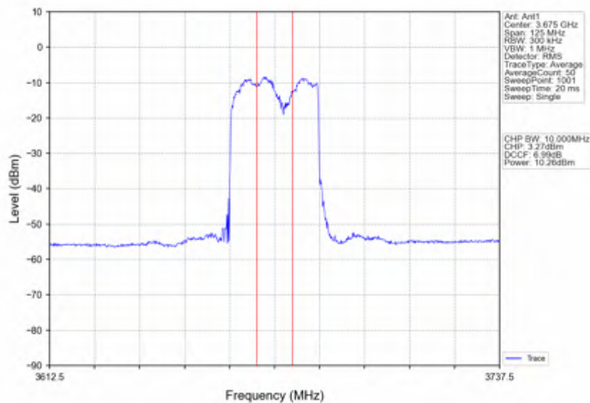
n78d_30kHz_SISO_NTNV_50MHz_CP-OFDM_QPSK_3675MHz_Inner_Full
