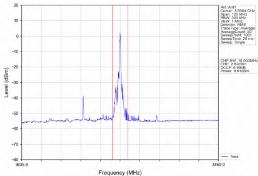
n78d_30kHz_SISO_NTNV_50MHz_CP-OFDM QPSK_3675MHz_Inner_1RB_Right
