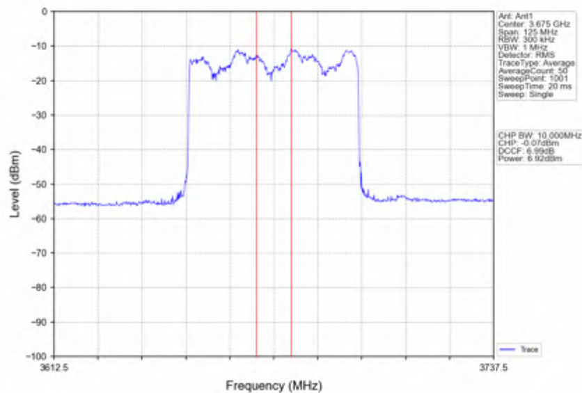
n78d_30kHz_SISO_NTNV_50MHz_CP-OFDM_256_QAM_3675MHz_Inner_Full
