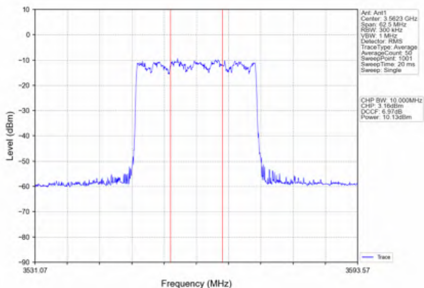
n78d 30kHz SISO NTNV 25MHz DFT-s-OFDM QPSK 3562.5MHz Inner Full
