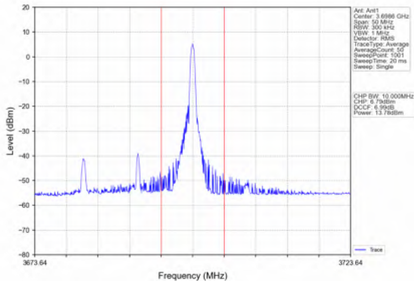
n78d_30kHz_SISO_NTNV_20MHz_DFT-s-OFDM QPSK_3690MHz_Inner_1RB_Right
