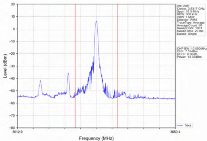
n78d_30kHz_SISO_NTNV_15MHz_CP-OFDM 64 QAM_3624.99MHz_Edge_1RB_Right
