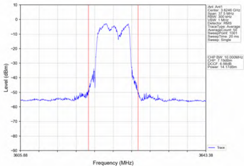
n78d_30kHz_SISO_NTNV_15MHz_DFT-s-OFDM_16_QAM_3624.99MHz_Inner_Full
