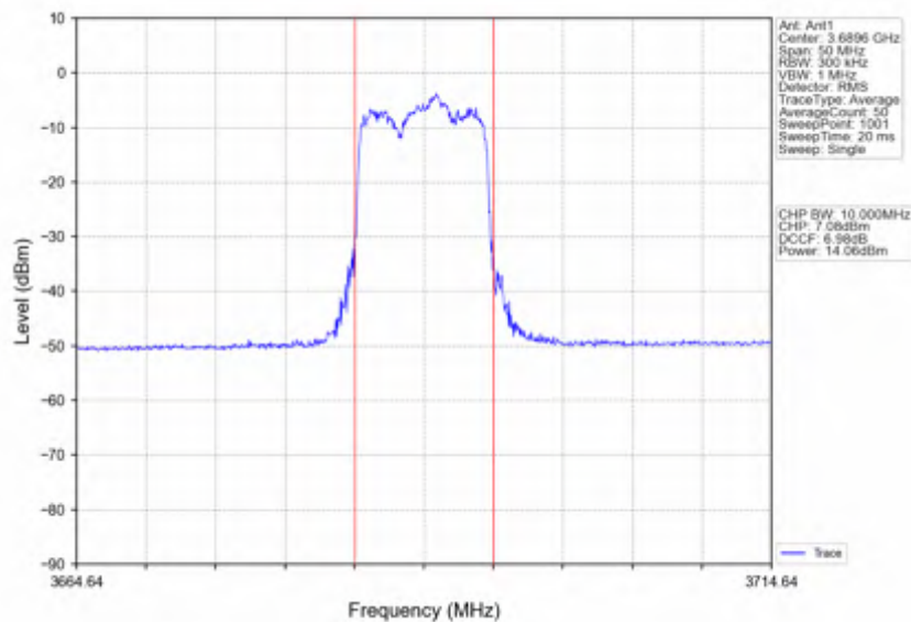
n78d_30kHz_SISO_NTNV_20MHz_DFT-s-OFDM 16 QAM_3690MHz_Inner_Full
