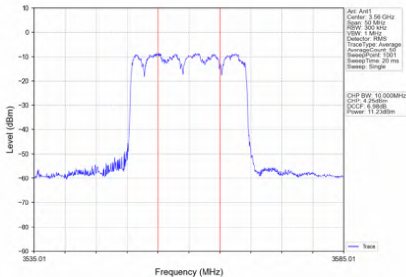
n78d_30kHz_SISO_NTNV_20MHz_CP-OFDM QPSK_3560.01MHz_Inner_Full
