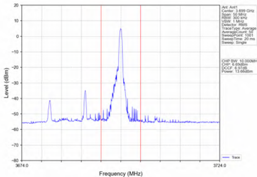
n78d_30kHz_SISO_NTNV_20MHz_DFT-s-OFDM_256_QAM_3690MHz_Edge_1RB_Right
