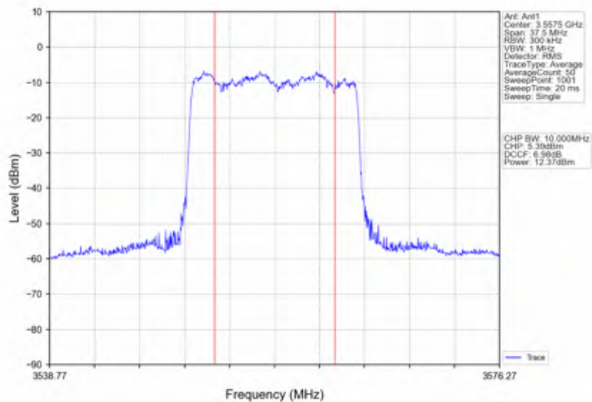
n78d_30kHz_SISO_NTNV_15MHz_CP-OFDM_256_QAM_3557.52MHz_Inner_Full
