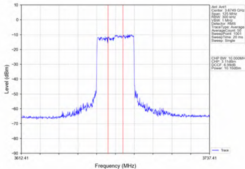
n78d_15kHz_SISO_NTNV_50MHz_DFT-s-OFDM_QPSK_3675MHz_Inner_Full
