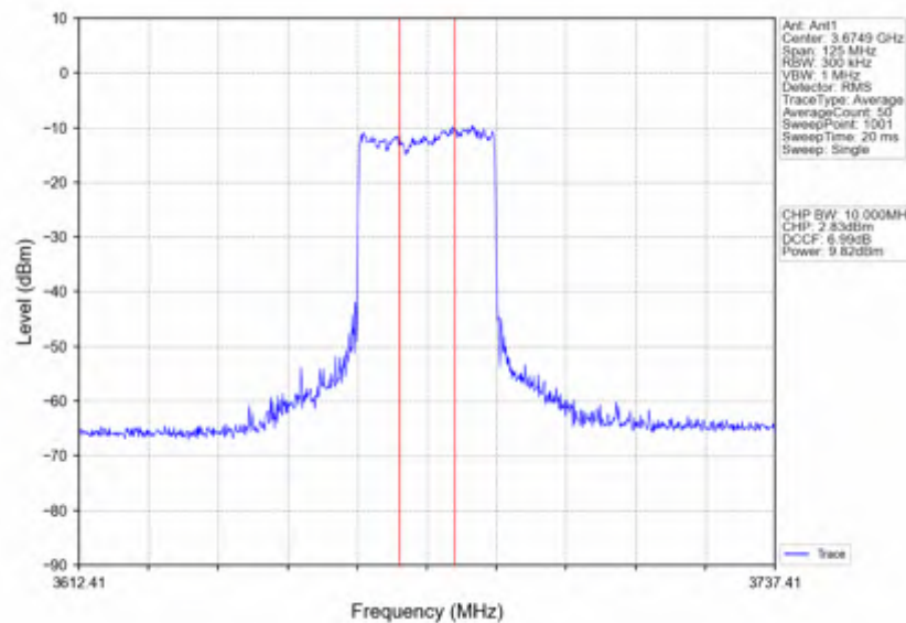
n78d_15kHz_SISO_NTNV_50MHz_CP-OFDM 16 QAM_3675MHz_Inner_Full
