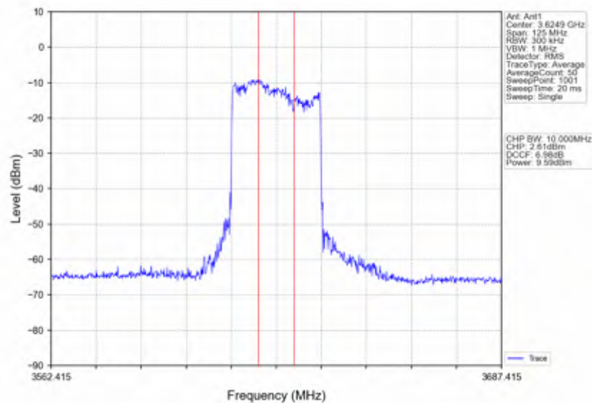
n78d_15kHz_SISO_NTNV_50MHz_DFT-s-OFDM 256 QAM_3625.005MHz_Inner_Full
