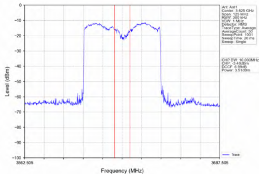
n78d_15kHz_SISO_NTNV_50MHz_CP-OFDM QPSK_3625.005MHz_Inner_Full
