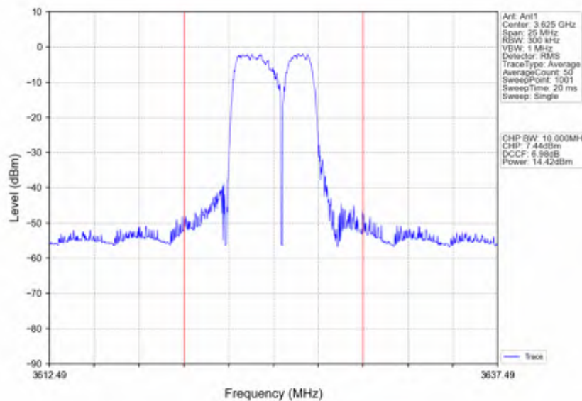
n78d_30kHz_SISO_NTNV_10MHz_CP-OFDM QPSK_3624.99MHz_Inner_Full
