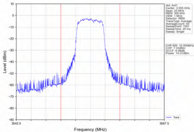
n78d_30kHz_SISO_NTNV_10MHz_DFT-s-OFDM 16 QAM_3555MHz_Inner_Full
