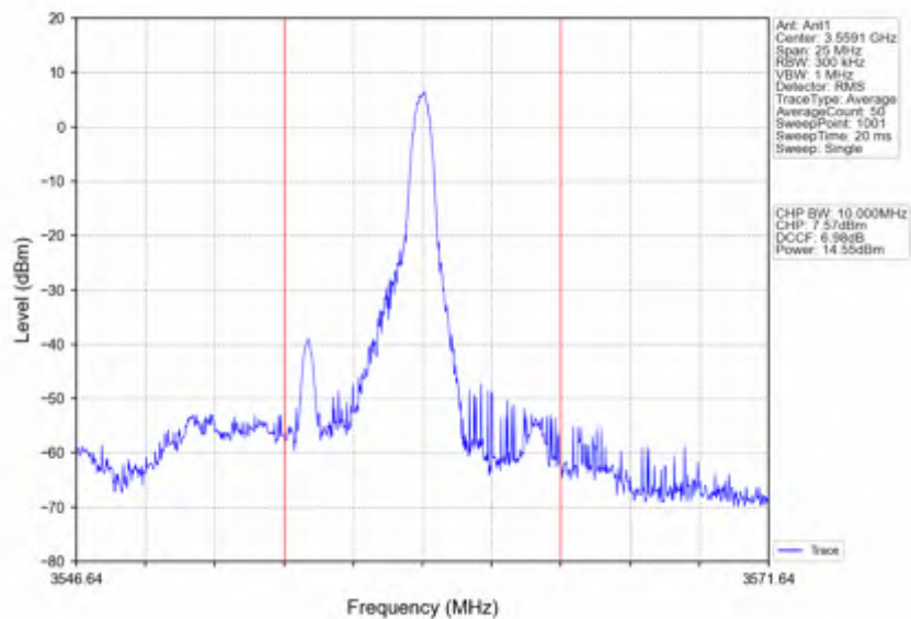
n78d_30kHz_SISO_NTNV_10MHz_DFT-s-OFDM_16_QAM_3555MHz_Edge_1RB_Right
