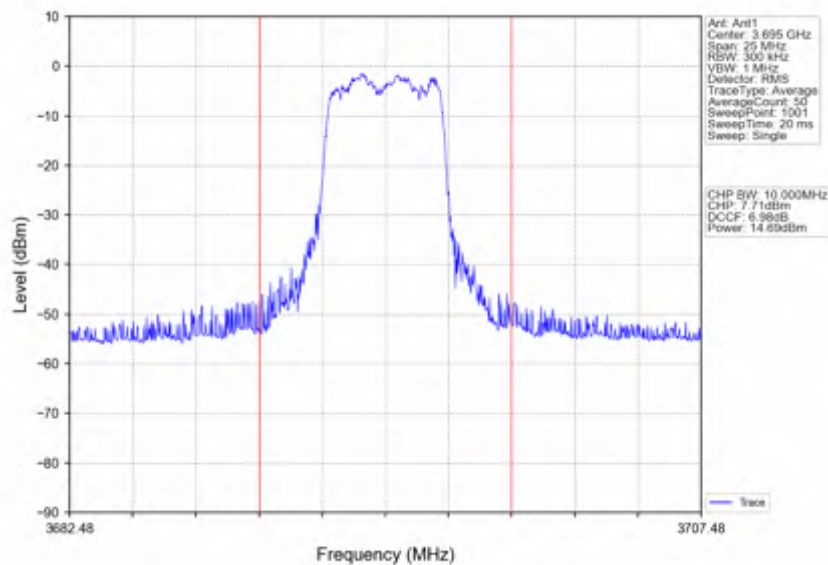
n78d_30kHz_SISO_NTNV_10MHz_CP-OFDM 64 QAM_3694.98MHz_Inner_Full
