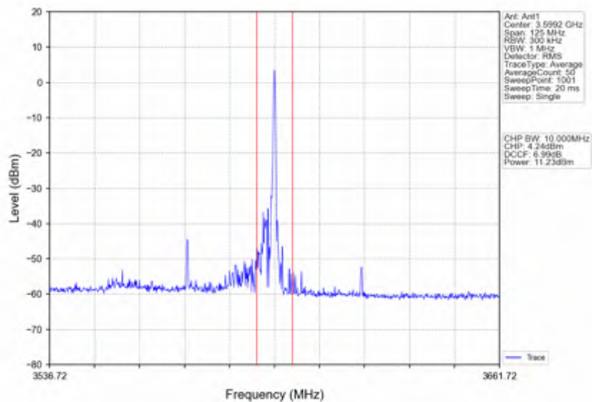
n78d_15kHz_SISO_NTNV_50MHz_DFT-s-OFDM_16_QAM_3575.01MHz_Edge_1RB_Right
