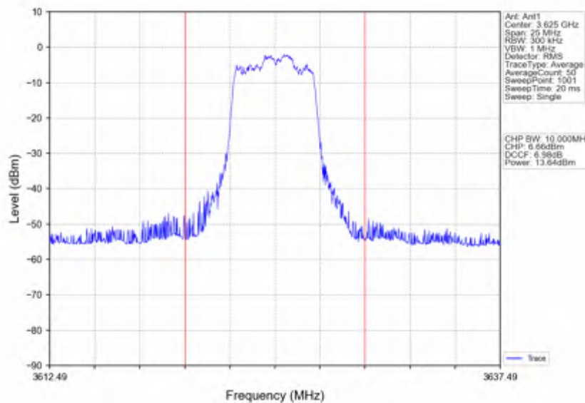
n78d_30kHz_SISO_NTNV_10MHz_CP-OFDM 64 QAM_3624.99MHz_Inner_Full
