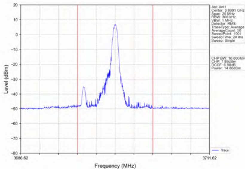
n78d_30kHz_SISO_NTNV_10MHz_DFT-s-OFDM 64 QAM_3694.98MHz_Edge_1RB_Right
