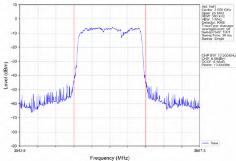
n78d_30kHz_SISO_NTNV_10MHz_CP-OFDM 16 QAM_3555MHz_Inner_Full
