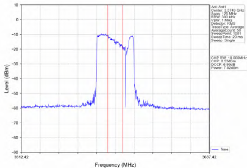
n78d_15kHz_SISO_NTNV_50MHz_CP-OFDM QPSK_3575.01MHz_Inner_Full
