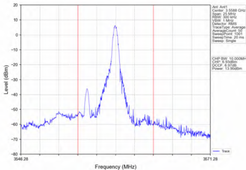
n78d_30kHz_SISO_NTNV_10MHz_CP-OFDM_16 QAM_3555MHz_Inner_1RB_Right
