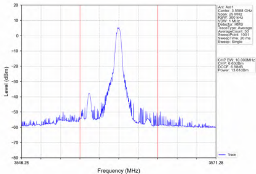
n78d_30kHz_SISO_NTNV_10MHz_DFT-s-OFDM_PI/2_BPSK_3555MHz_Inner_1RB_Right
