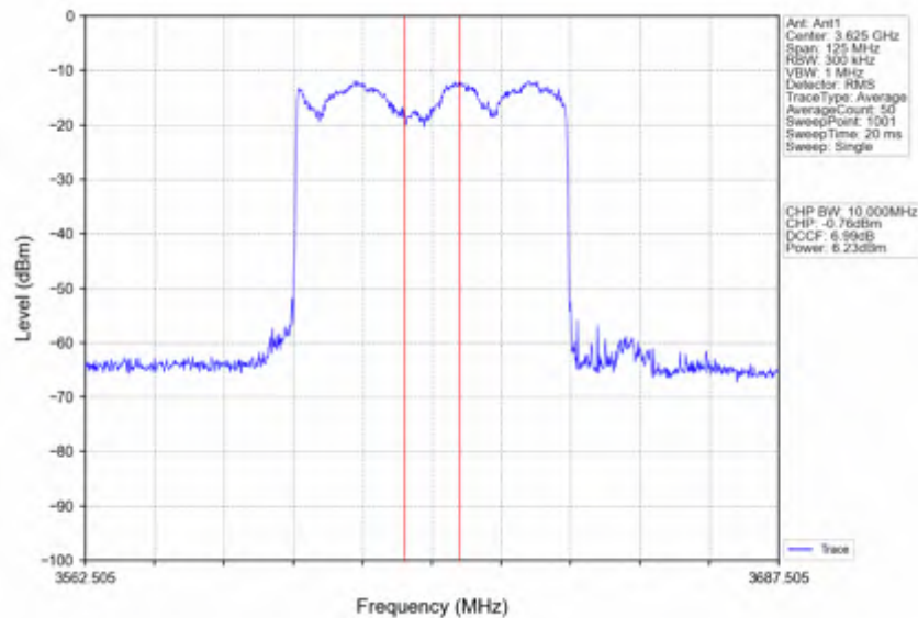
n78d_15kHz_SISO_NTNV_50MHz_CP-OFDM_16_QAM_3625.005MHz_Inner_Full
