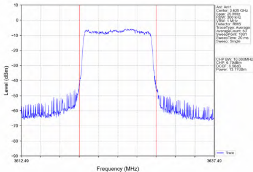
n78d_30kHz_SISO_NTNV_10MHz_DFT-s-OFDM_16 QAM_3624.99MHz_Inner_Full
