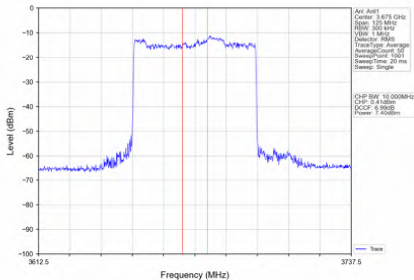
n78d_15kHz_SISO_NTNV_50MHz_CP-OFDM 64 QAM_3675MHz_Inner_Full
