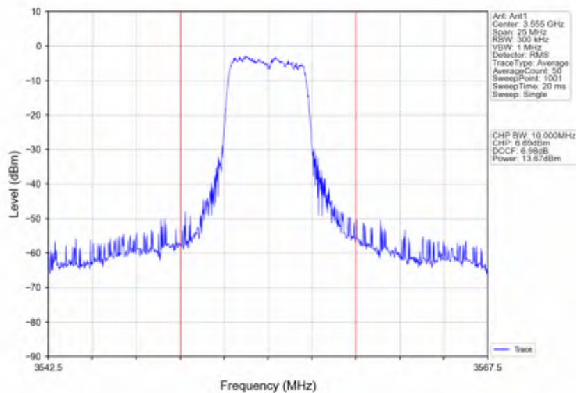
n78d_30kHz_SISO_NTNV_10MHz_CP-OFDM 64 QAM_3555MHz_Inner_Full
