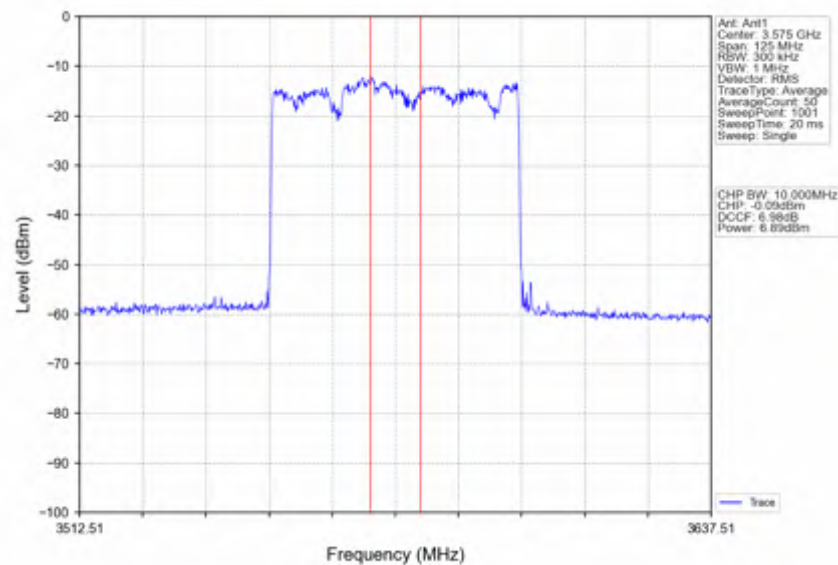
n78d_15kHz_SISO_NTNV_50MHz_DFT-s-OFDM_256_QAM_3575.01MHz_Inner_Full
