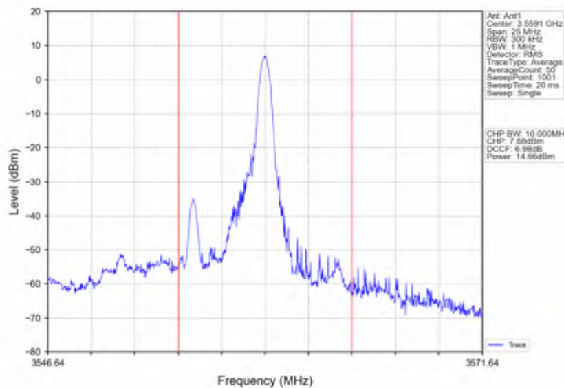
n78d_30kHz_SISO_NTNV_10MHz_CP-OFDM 16 QAM_3555MHz_Edge_1RB_Right
