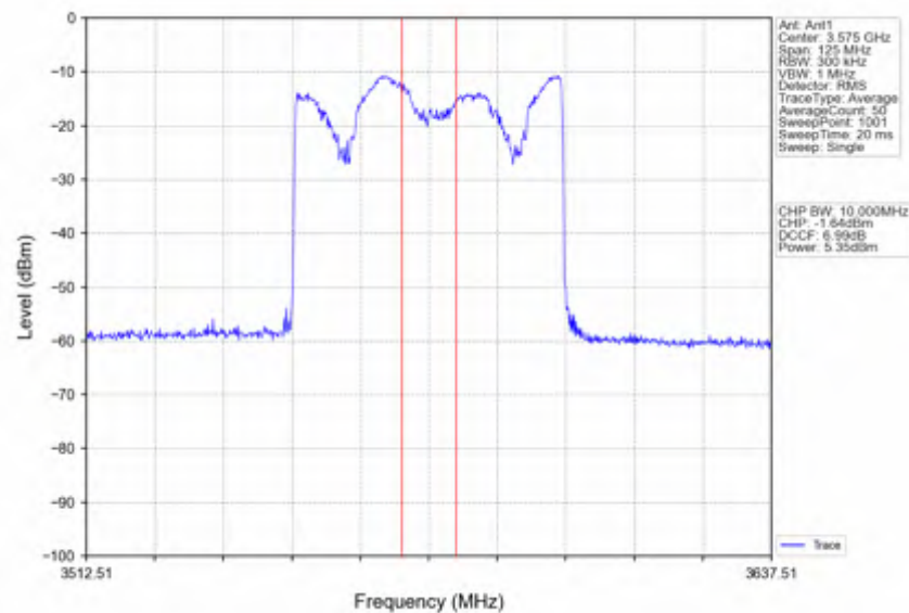
n78d_15kHz_SISO_NTNV_50MHz_CP-OFDM QPSK_3575.01MHz_Inner_Full
