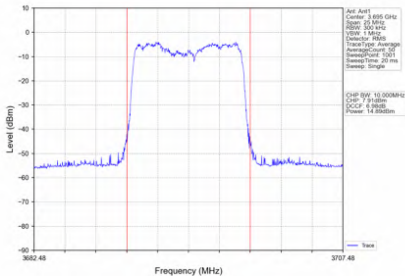
n78d_30kHz_SISO_NTNV_10MHz_DFT-s-OFDM PI/2 BPSK_3694.98MHz_Inner_Full
