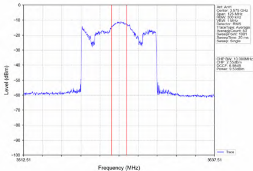
n78d_15kHz_SISO_NTNV_50MHz_CP-OFDM 256 QAM_3575.01MHz_Inner_Full
