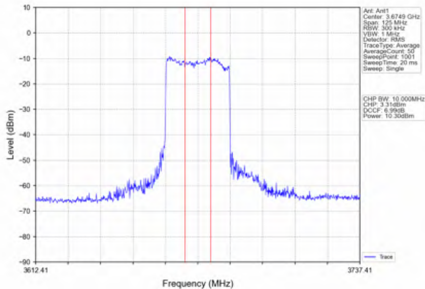
n78d_15kHz_SISO_NTNV_50MHz_CP-OFDM_QPSK_3675MHz_Inner_Full
