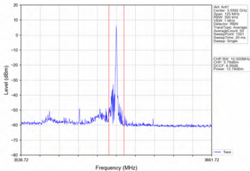
n78d_15kHz_SISO_NTNV_50MHz_CP-OFDM 16 QAM_3575.01MHz_Edge_1RB_Right
