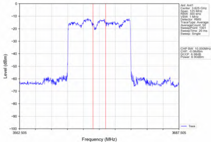
n78d_15kHz_SISO_NTNV_50MHz_DFT-s-OFDM QPSK_3625.005MHz_Inner_Full
