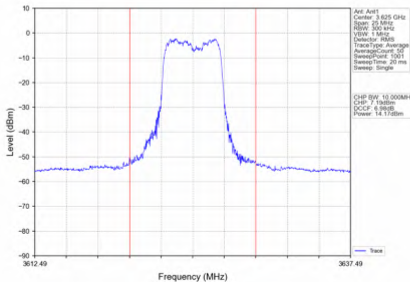
n78d_30kHz_SISO_NTNV_10MHz_CP-OFDM_256_QAM_3624.99MHz_Inner_Full
