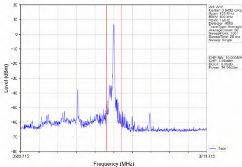
n78d_15kHz_SISO_NTNV_50MHz_CP-OFDM QPSK_3625.005MHz_Edge_1RB_Right
