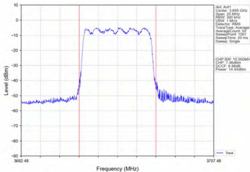
n78d_30kHz_SISO_NTNV_10MHz_DFT-s-OFDM_QPSK_3694.98MHz_Inner_Full
