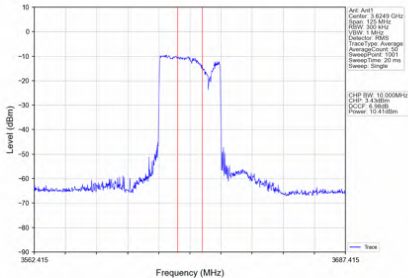
n78d_15kHz_SISO_NTNV_50MHz_CP-OFDM_16_QAM_3625.005MHz_Inner_Full
