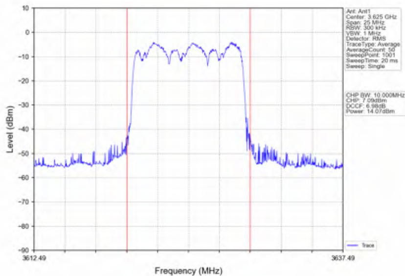
n78d_30kHz_SISO_NTNV_10MHz_CP-OFDM QPSK_3624.99MHz_Inner_Full
