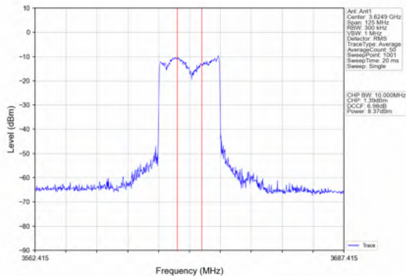
n78d_15kHz_SISO_NTNV_50MHz_CP-OFDM QPSK_3625.005MHz_Inner_Full
