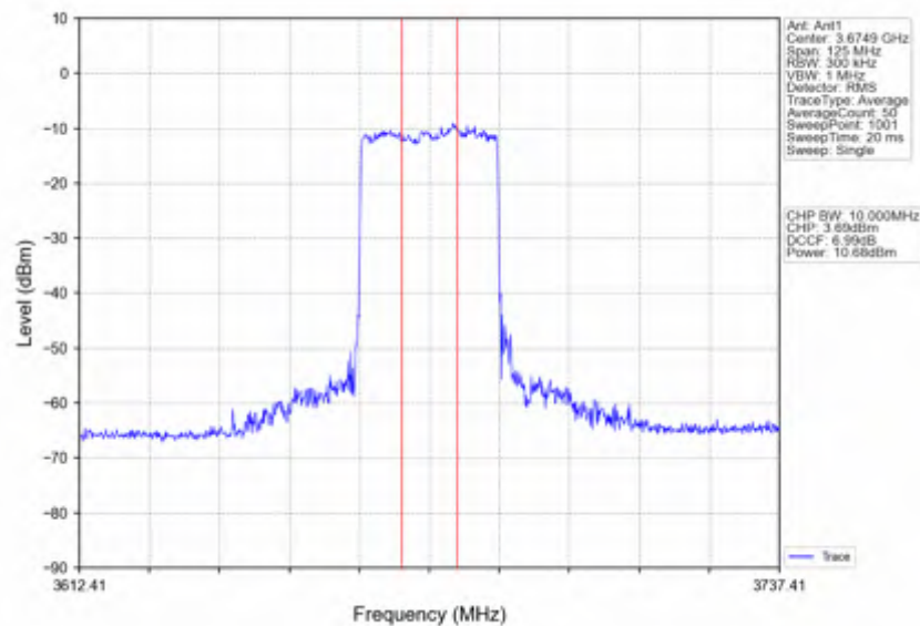
n78d_15kHz_SISO_NTNV_50MHz_CP-OFDM_256_QAM_3675MHz_Inner_Full
