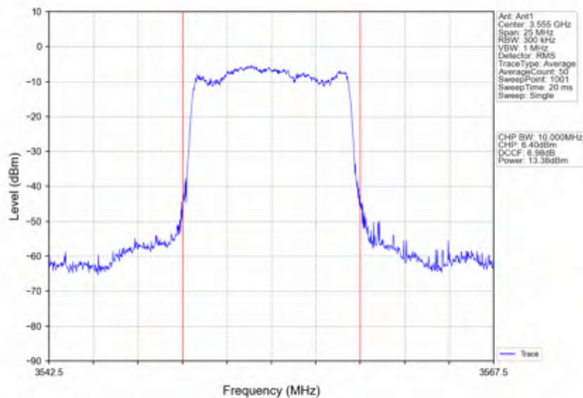
n78d_30kHz_SISO_NTNV_10MHz_CP-OFDM QPSK_3555MHz_Inner_Full
