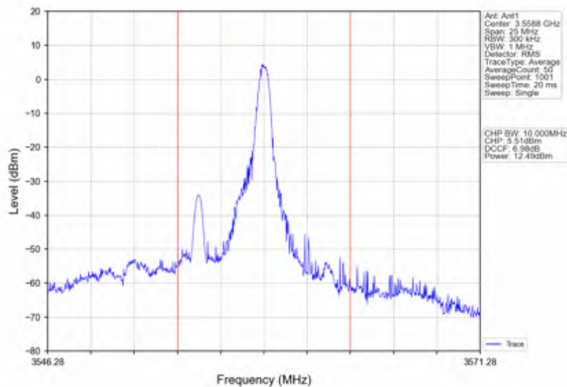
n78d_30kHz_SISO_NTV_10MHz_CP-OFDM 256 QAM 3555MHz_Inner_1RB_Right
