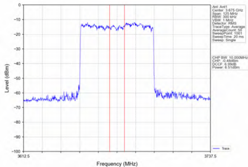
n78d_15kHz_SISO_NTNV_50MHz_DFT-s-OFDM_QPSK_3675MHz_Inner_Full
