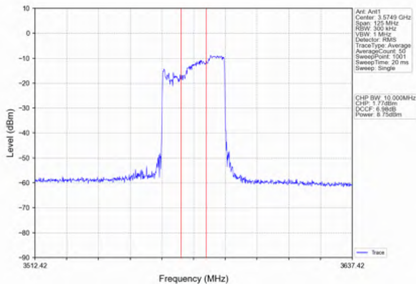
n78d_15kHz_SISO_NTNV_50MHz_CP-OFDM 256 QAM_3575.01MHz_Inner_Full
