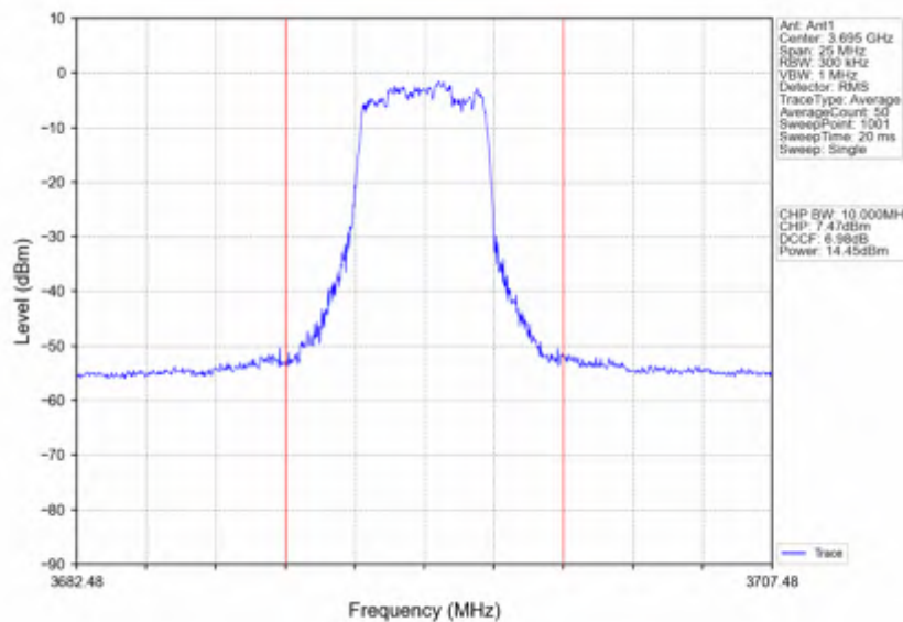
n78d_30kHz_SISO_NTNV_10MHz_CP-OFDM_256_QAM_3694.98MHz_Inner_Full
