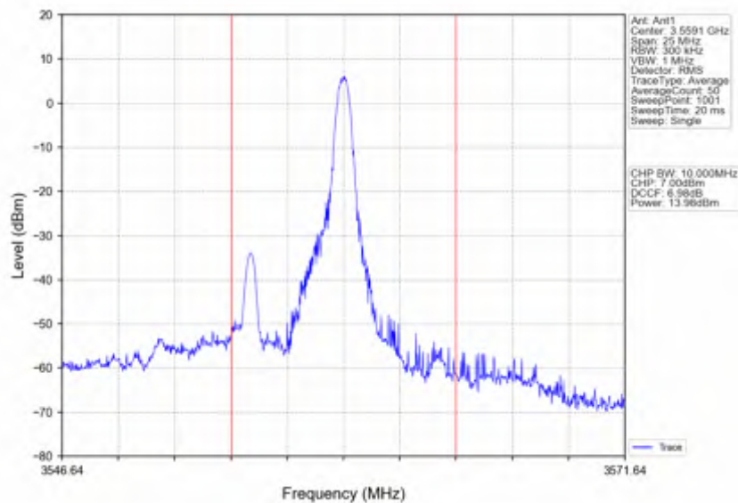
n78d_30kHz_SISO_NTNV_10MHz_CP-OFDM_64_QAM_3555MHz_Edge_1RB_Right
