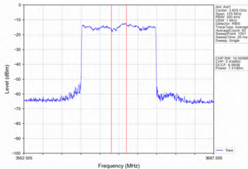
n78d_15kHz_SISO_NTNV_50MHz_CP-OFDM 64 QAM_3625.005MHz_Inner_Full
