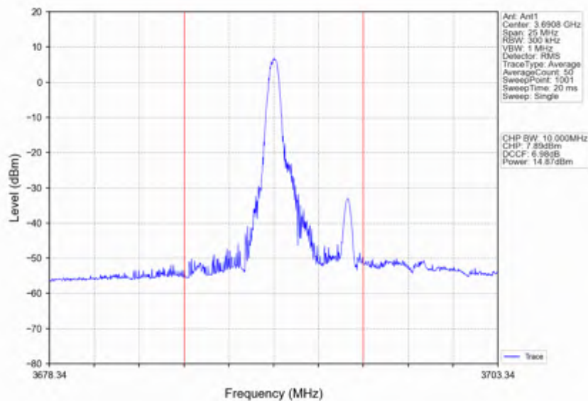
n78d_30kHz_SISO_NTNV_10MHz_CP-OFDM 16 QAM_3694.98MHz_Edge_1RB_Right
