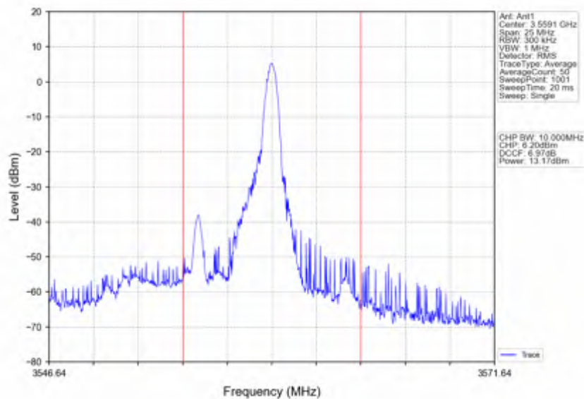
n78d_30kHz_SISO_NTV_10MHz_DFT-s-OFDM QPSK_3555MHz_Edge_1RB_Right
