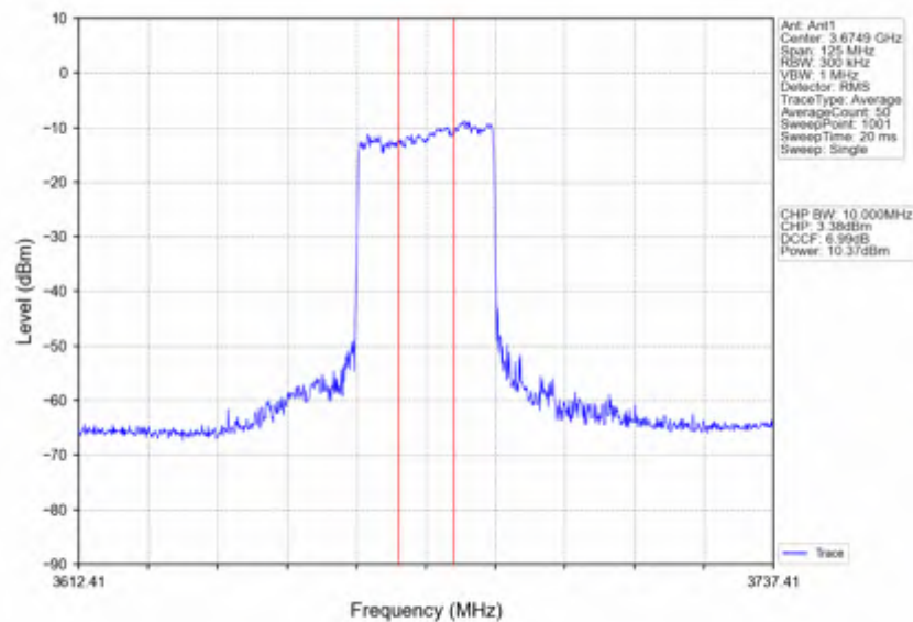
n78d_15kHz_SISO_NTNV_50MHz_CP-OFDM 64 QAM_3675MHz_Inner_Full
