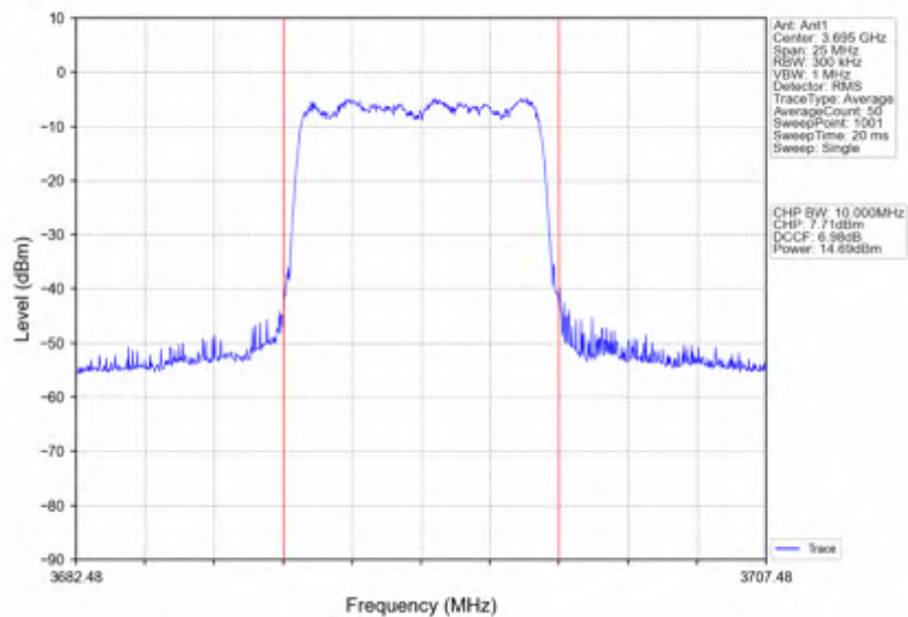
n78d_30kHz_SISO_NTNV_10MHz_CP-OFDM QPSK_3694.98MHz_Inner_Full
