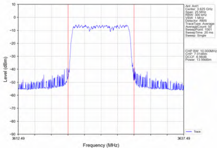
n78d_30kHz_SISO_NTNV_10MHz_CP-OFDM_256_QAM_3624.99MHz_Inner_Full
