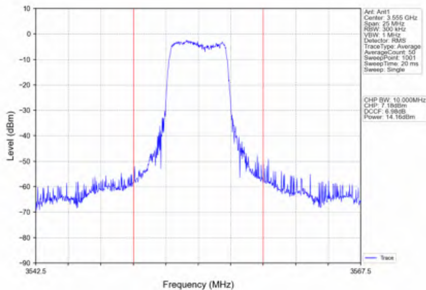
n78d 30kHz SISO NTNV 10MHz DFT-s-OFDM 256 QAM 3555MHz Inner Full
