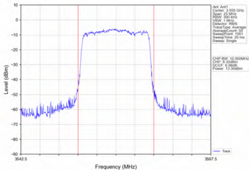
n78d_30kHz_SISO_NTNV_10MHz_DFT-s-OFDM_QPSK_3555MHz_Inner_Full
