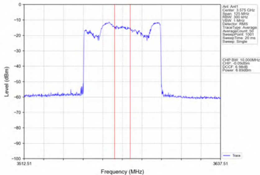
n78d_15kHz_SISO_NTNV_50MHz_CP-OFDM 64 QAM_3575.01MHz_Inner_Full
