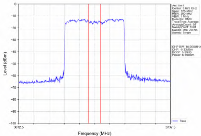
n78d_15kHz_SISO_NTNV_50MHz_CP-OFDM_256_QAM_3675MHz_Inner_Full
