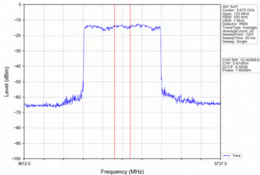
n78d_15kHz_SISO_NTNV_50MHz_CP-OFDM_QPSK_3675MHz_Inner_Full
