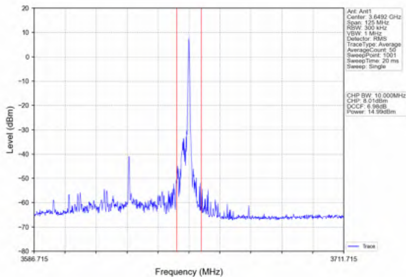
n78d_15kHz_SISO_NTNV_50MHz_CP-OFDM 256 QAM_3625.005MHz_Edge_1RB_Right
