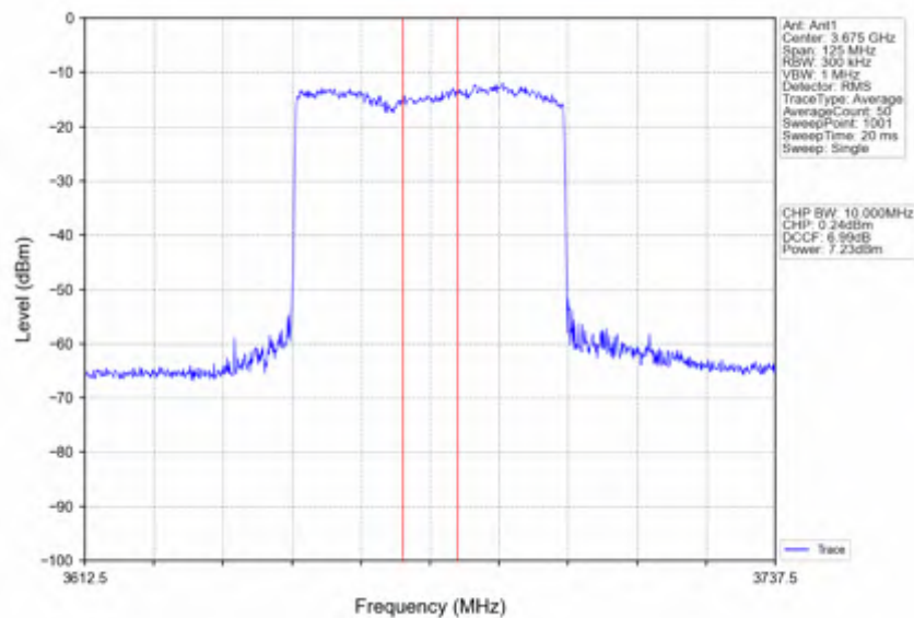
n78d_15kHz_SISO_NTNV_50MHz_CP-OFDM 16 QAM_3675MHz_Inner_Full
