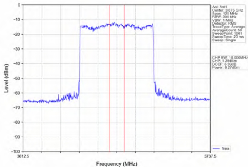
n78d 15kHz SISO NTNV 50MHz DFT-s-OFDM 256 QAM 3675MHz Inner Full
