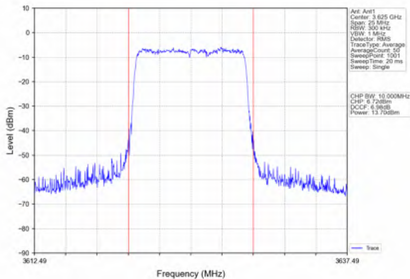
n78d_30kHz_SISO_NTNV_10MHz_DFT-s-OFDM_QPSK_3624.99MHz_Inner_Full
