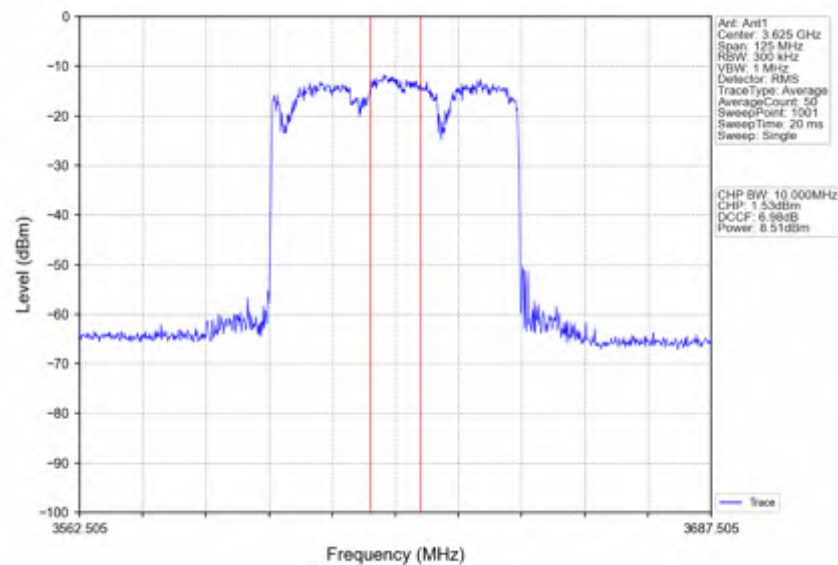
n78d_15kHz_SISO_NTNV_50MHz_DFT-s-OFDM 256 QAM_3625.005MHz_Inner_Full
