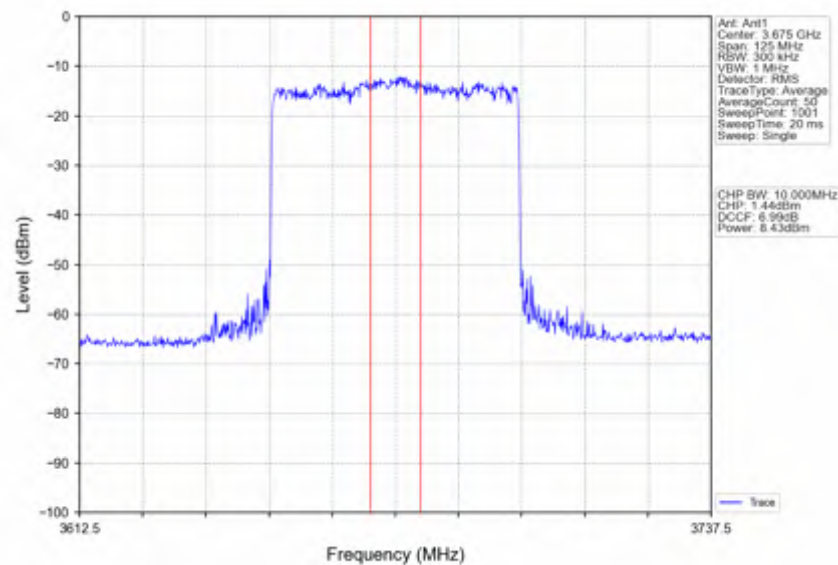
n78d_15kHz_SISO_NTNV_50MHz_DFT-s-OFDM 16 QAM_3675MHz_Inner_Full
