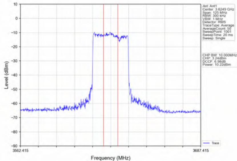
n78d_15kHz_SISO_NTNV_50MHz_DFT-s-OFDM QPSK_3625.005MHz_Inner_Full
