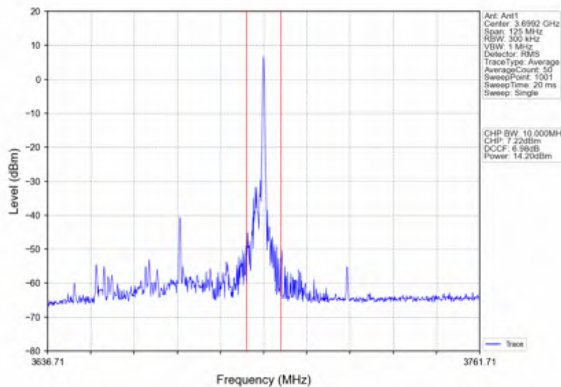
n78d_15kHz_SISO_NTNV_50MHz_DFT-s-OFDM QPSK_3675MHz_Edge_1RB_Right
