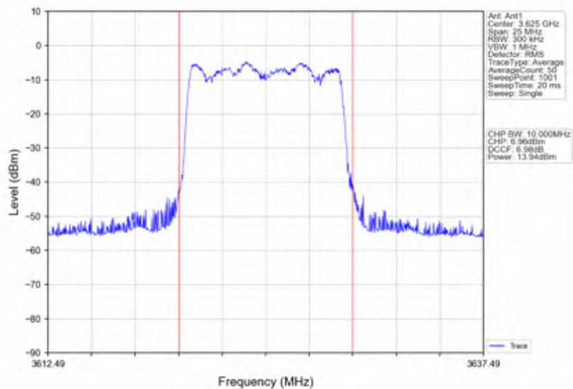
n78d_30kHz_SISO_NTNV_10MHz_CP-OFDM 64 QAM_3624.99MHz_Inner_Full
