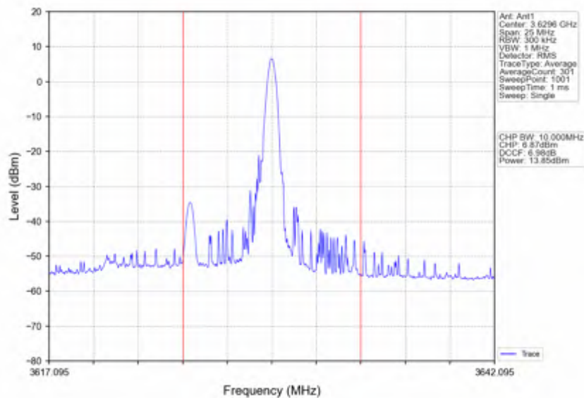
n78d_15kHz_SISO_NTNV_10MHz_CP-OFDM QPSK_3625.005MHz_Edge_1RB_Right
