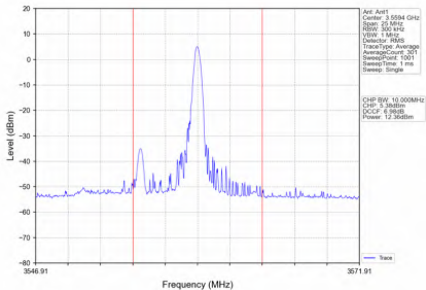
n78d 15kHz SISO NTV 10MHz CP-OFDM 64 QAM 3555MHz Inner 1RB Right
