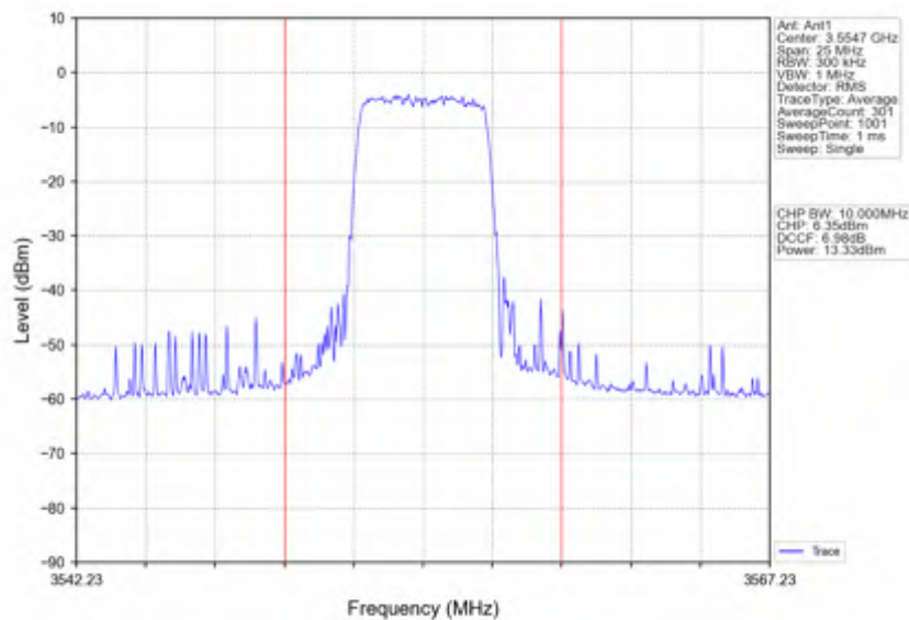
n78d_15kHz_SISO_NTNV_10MHz_DFT-s-OFDM 64 QAM_3555MHz_Inner_Full
