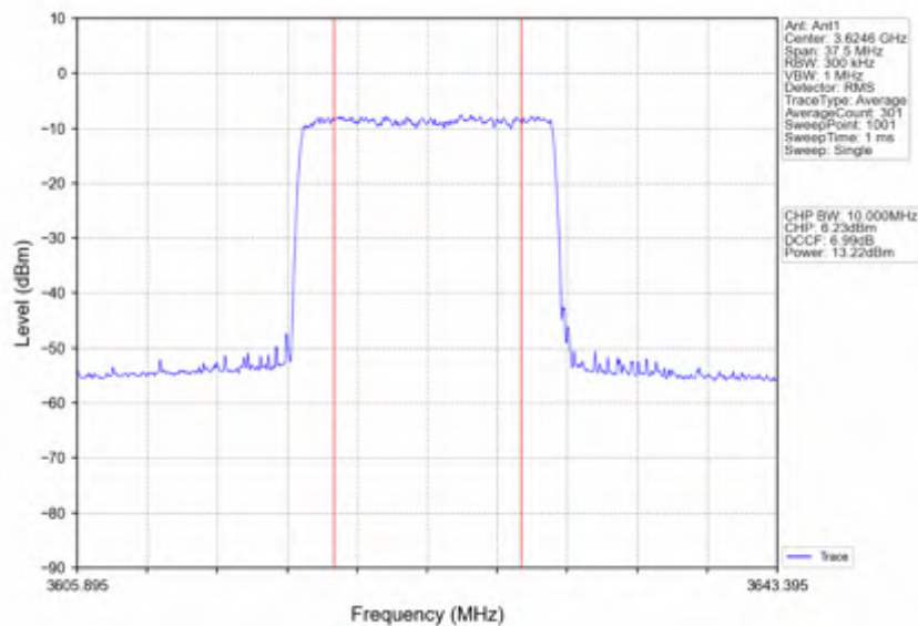
n78d_15kHz_SISO_NTNV_15MHz_DFT-s-OFDM_QPSK_3625.005MHz_Inner_Full
