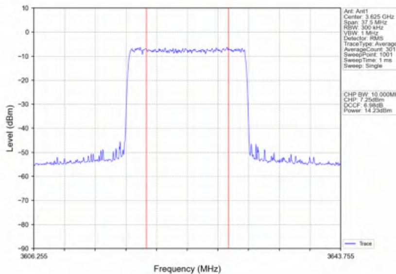
n78d_15kHz_SISO_NTNV_15MHz_CP-OFDM QPSK_3625.005MHz_Inner_Full
