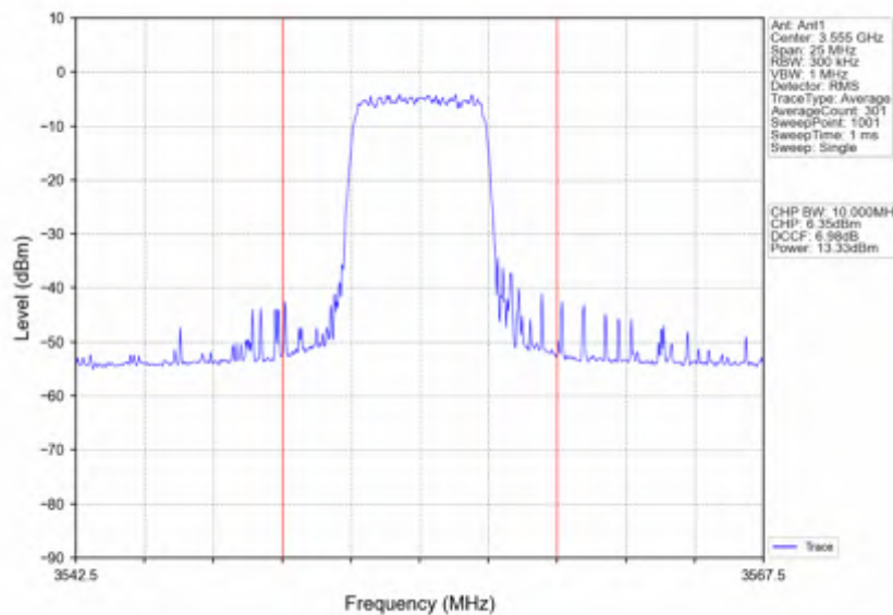
n78d_15kHz_SISO_NTV_10MHz_CP-OFDM_256_QAM_3555MHz_Inner_Full
