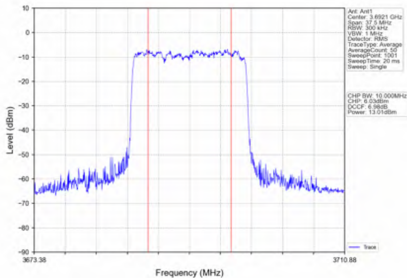
n78d_15kHz_SISO_NTNV_15MHz_DFT-s-OFDM 64 QAM_3692.49MHz_Inner_Full
