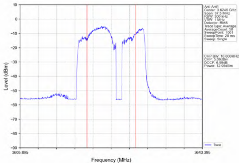
n78d_15kHz_SISO_NTNV_15MHz_DFT-s-OFDM_PI/2_BPSK_3625.005MHz_Inner_Full
