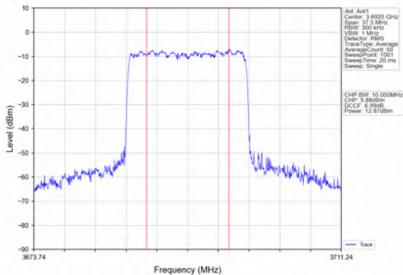
n78d_15kHz_SISO_NTNV_15MHz_CP-OFDM 16 QAM 3692.49MHz_Inner_Full
