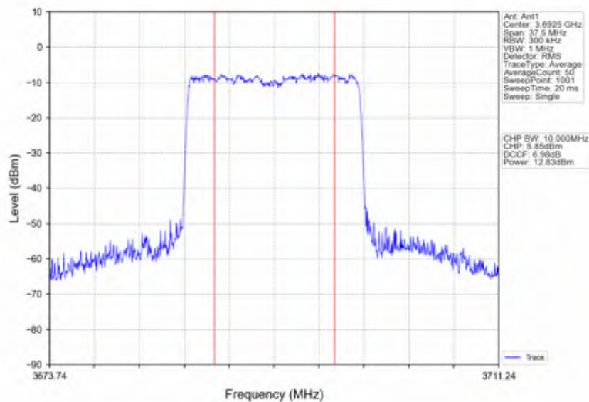
n78d 15kHz SISO NTN 15MHz CP-OFDM QPSK 3692.49MHz Inner Full
