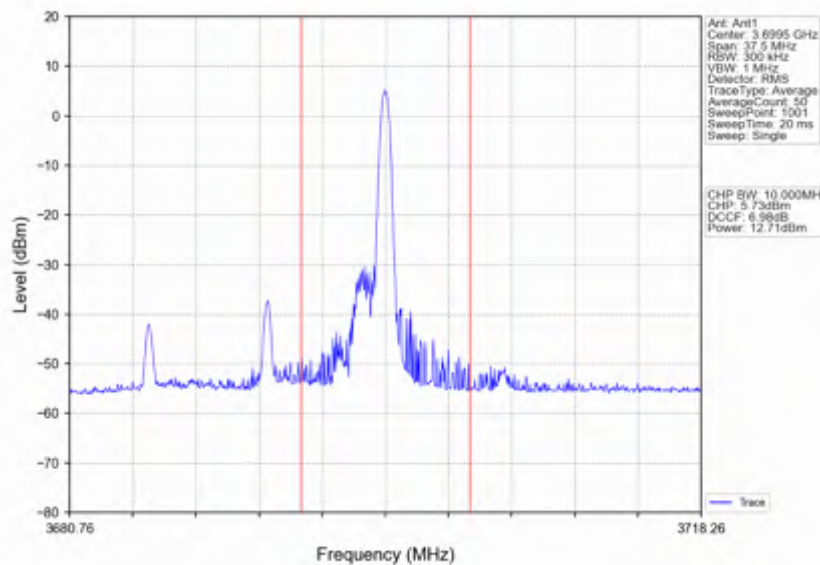
n78d_15kHz_SISO_NTNV_15MHz_DFT-s-OFDM PI/2 BPSK_3692.49MHz_Edge_1RB_Right
