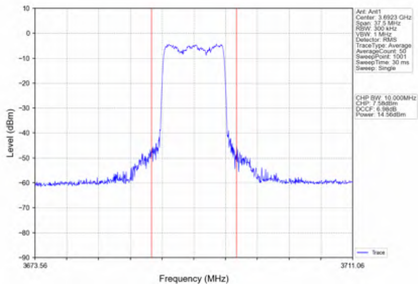
n78d_15kHz_SISO_NTNV_15MHz_CP-OFDM 256 QAM_3692.49MHz_Inner_Full
