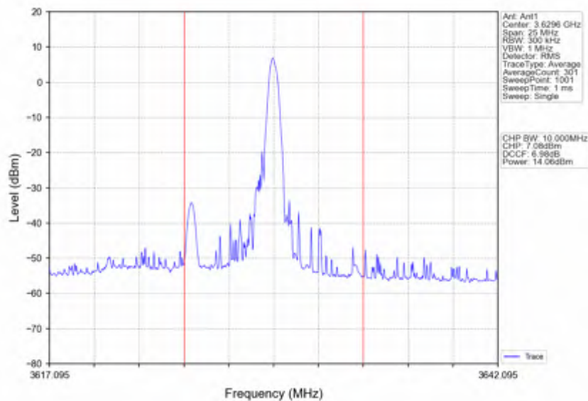
n78d_15kHz_SISO_NTNV_10MHz_CP-OFDM_16_QAM_3625.005MHz_Edge_1RB_Right
