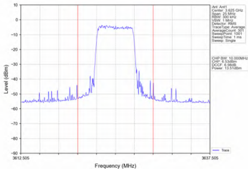
n78d_15kHz_SISO_NTNV_10MHz_CP-OFDM QPSK_3625.005MHz_Inner_Full
