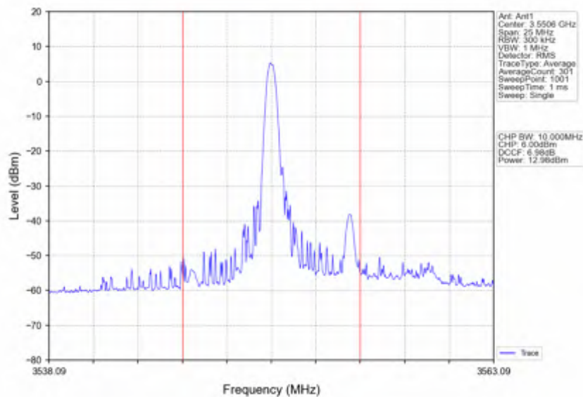
n78d_15kHz_SISO_NTNV_10MHz_DFT-s-OFDM_256_QAM_3555MHz_Inner_1RB_Right
