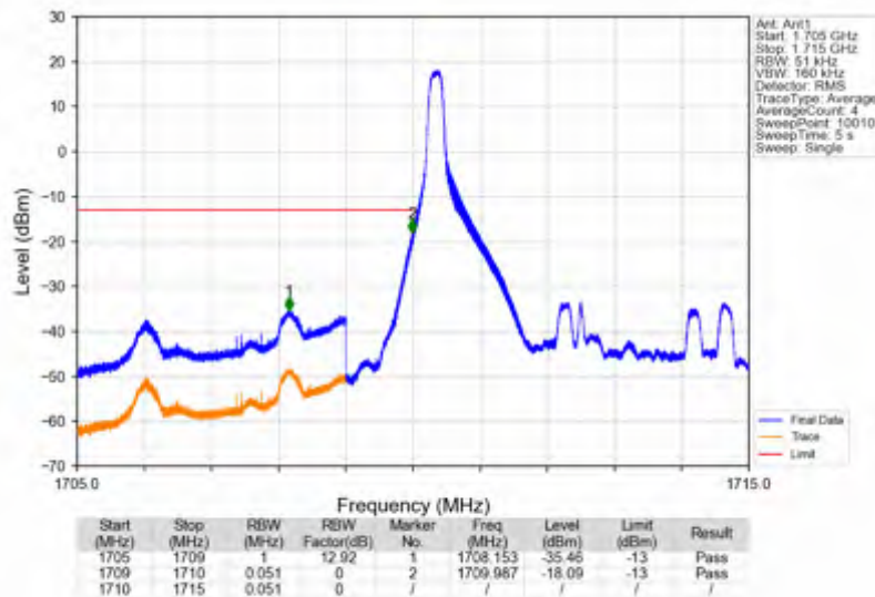
Band66_5MHz_QPSK_LCH_1712.5MHz_RB_1_0_NTNV
