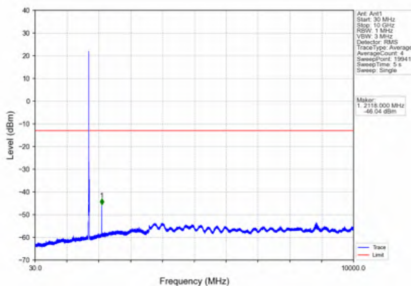
Band66_10MHz_QPSK_LCH_1715MHz_RB_1_0_NTNV
