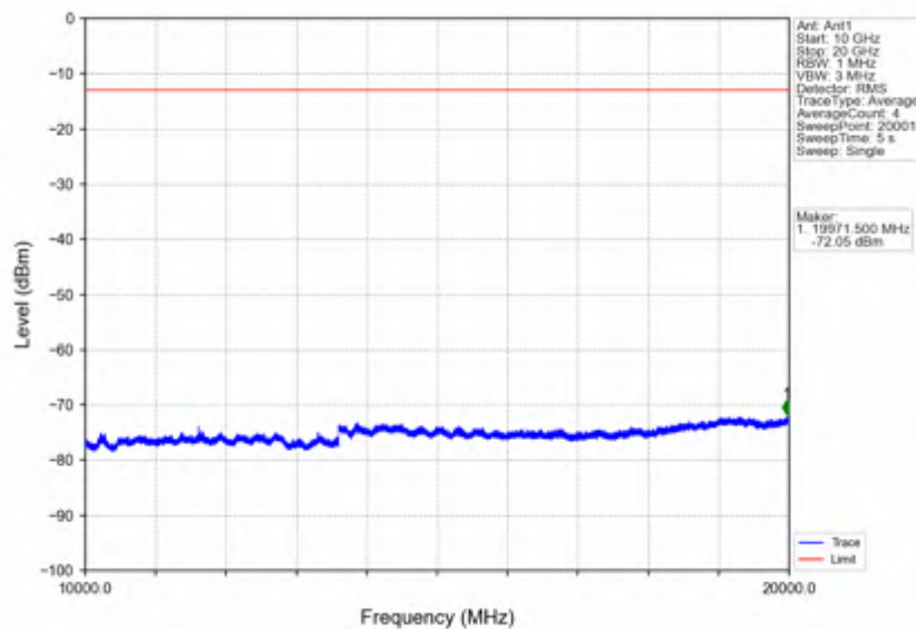
Band66 15MHz 64QAM HCH 1772.5MHz RB 1 0 NTNV
