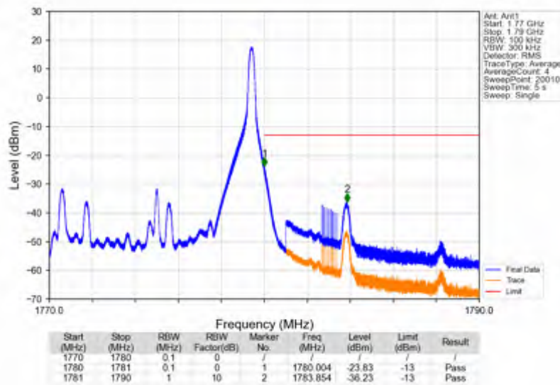
Band66_10MHz_256QAM_HCH_1775MHz_RB_1_49_NTNV
