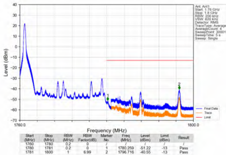
Band66_20MHz_16QAM_HCH_1770MHz_RB_100_0_NTNV
