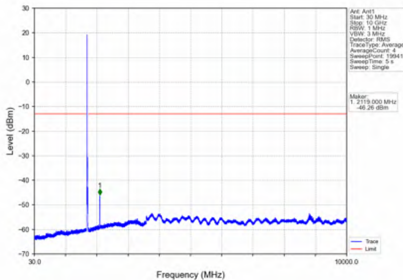
Band66 15MHz 256QAM LCH 1717.5MHz RB 1 0 NTNV
