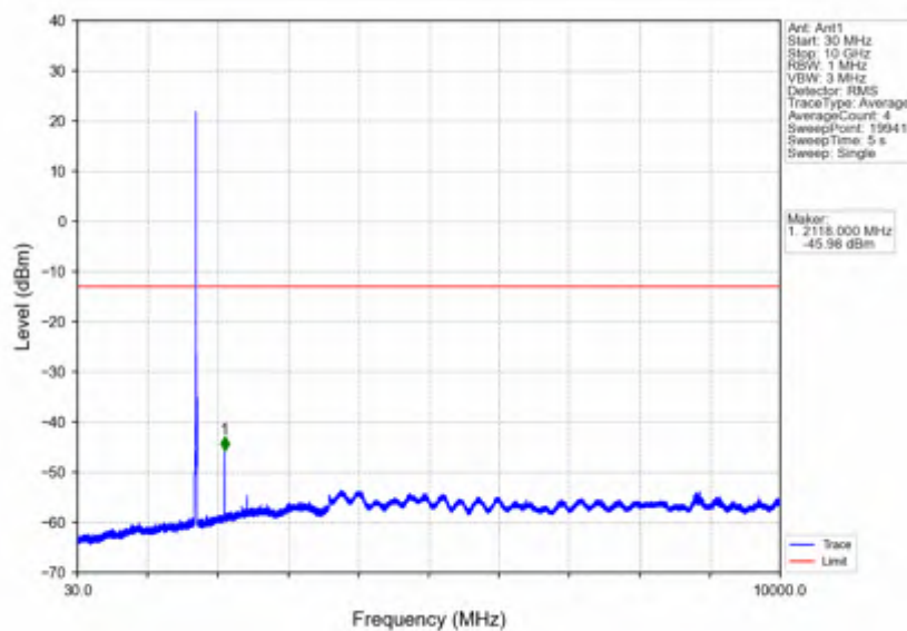
Band66_10MHz_16QAM_LCH_1715MHz_RB_1_0_NTNV
