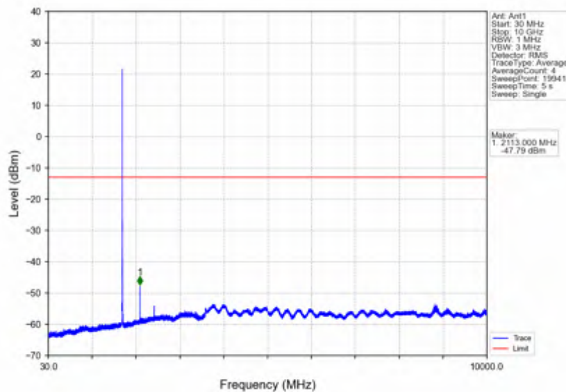
Band66 5MHz 16QAM LCH 1712.5MHz RB 1 0 NTNV
