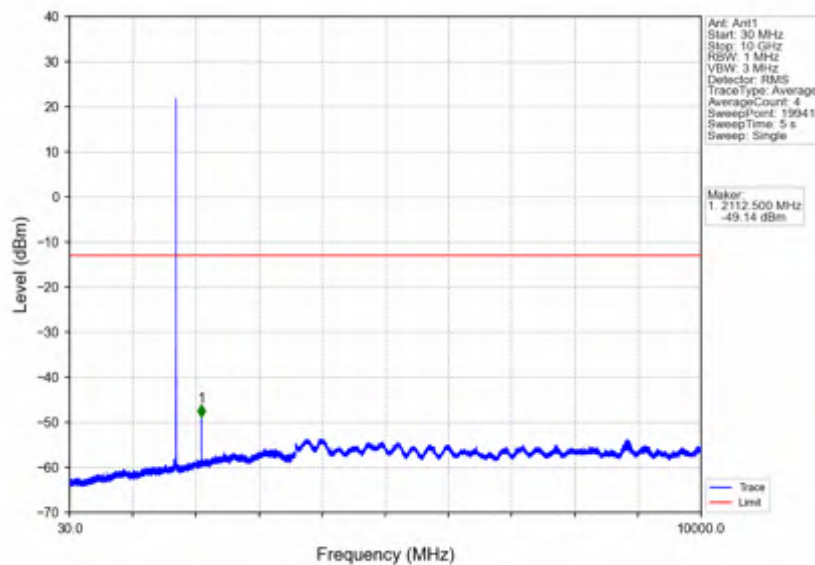
Band66 3MHz 64QAM LCH 1711.5MHz RB 1 0 NTNV
