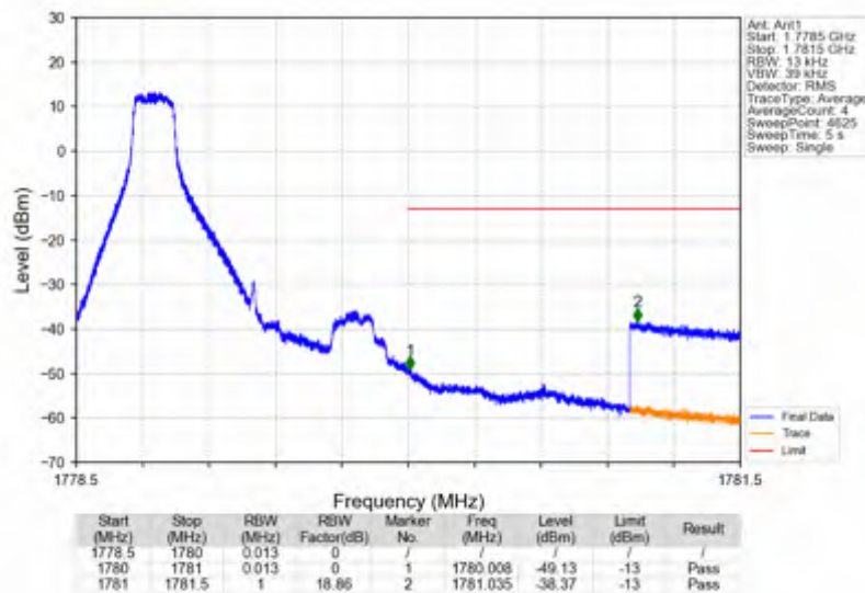
Band66_1.4MHz_16QAM_HCH_1779.3MHz_RB_6_0_NTNV
