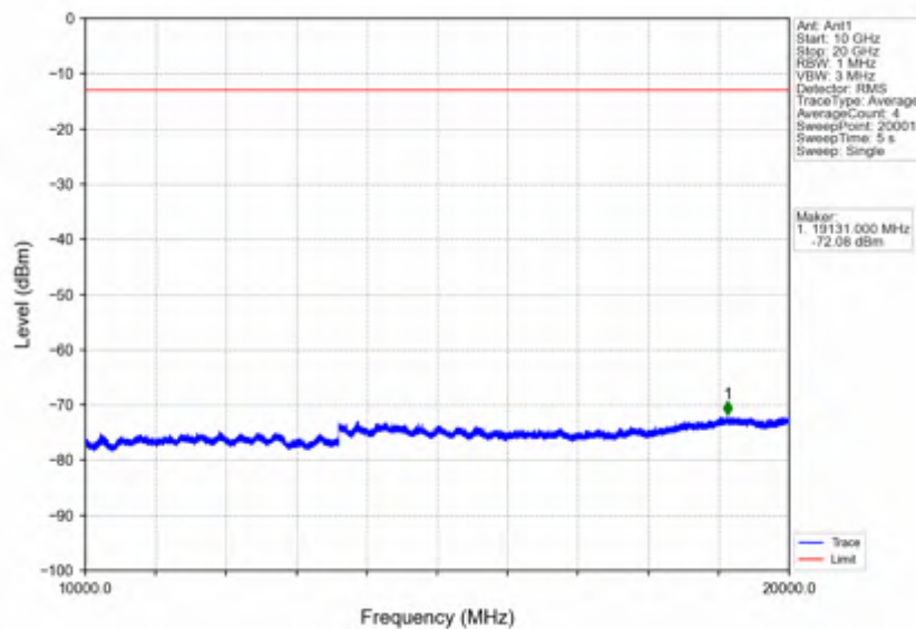
Band66_1.4MHz_256QAM_HCH_1779.3MHz_RB_1_0_NTNV
