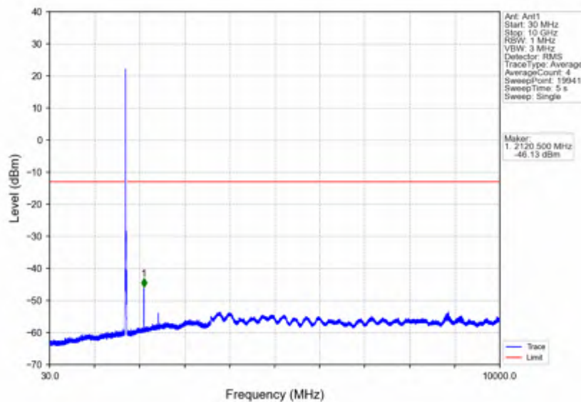
Band66 15MHz 16QAM LCH 1717.5MHz RB 1 0 NTNV
