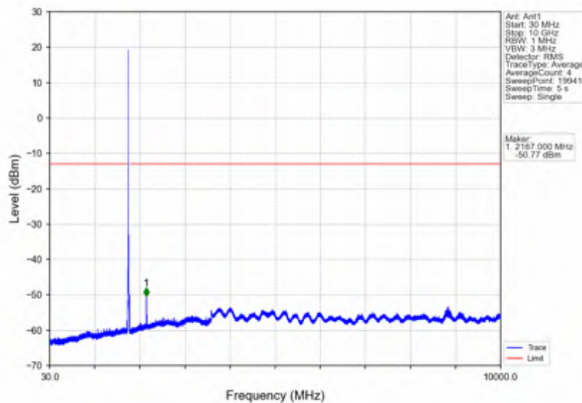
Band66 15MHz 256QAM HCH 1772.5MHz RB 1 0 NTNV
