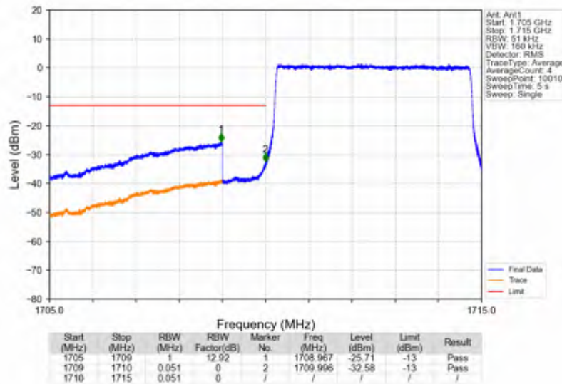
Band66_5MHz_256QAM_LCH_1712.5MHz_RB_25_0_NTNV
