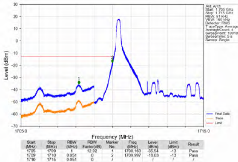
Band66_5MHz_16QAM_LCH_1712.5MHz_RB_25_0_NTNV
