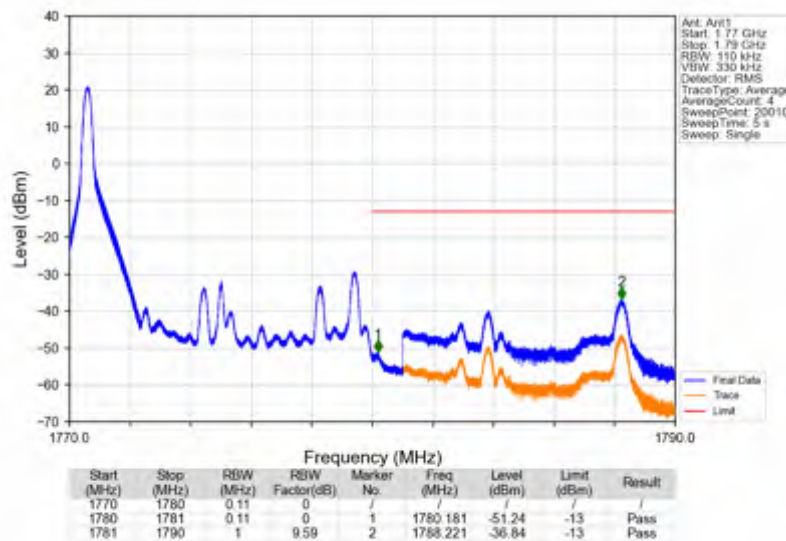
Band66_10MHz_QPSK_HCH_1775MHz_RB_50_0_NTV
