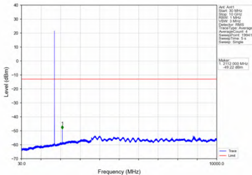
Band66 3MHz 16QAM LCH 1711.5MHz RB 1 0 NTNV
