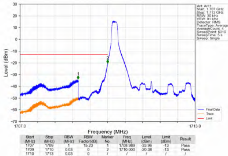
Band66_3MHz_64QAM_LCH_1711.5MHz_RB_15_0_NTNV
