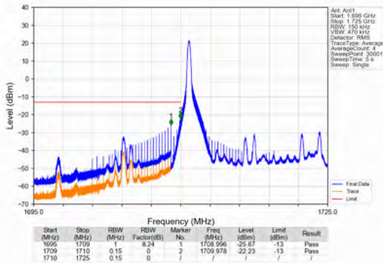
Band66_15MHz_QPSK_LCH_1717.5MHz_RB_1_0_NTNV
