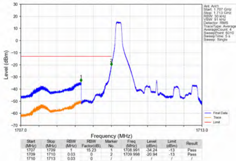
Band66 3MHz 16QAM LCH 1711.5MHz RB 1 0 NTNV
