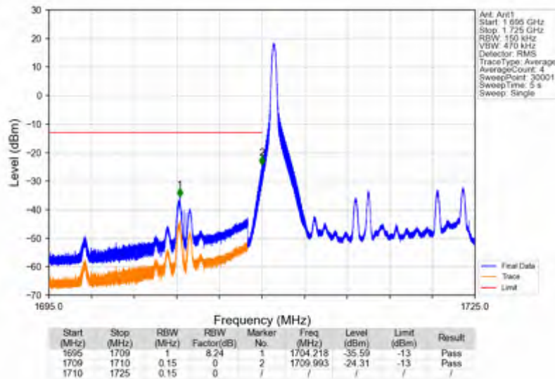
Band66 15MHz 256QAM LCH 1717.5MHz RB 1 0 NTNV
