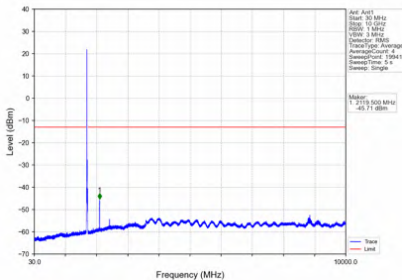
Band66_15MHz_64QAM_LCH_1717.5MHz_RB_1_0_NTNV
