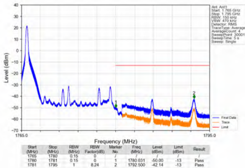
Band66_15MHz_64QAM_HCH_1772.5MHz_RB_75_0_NTNV
