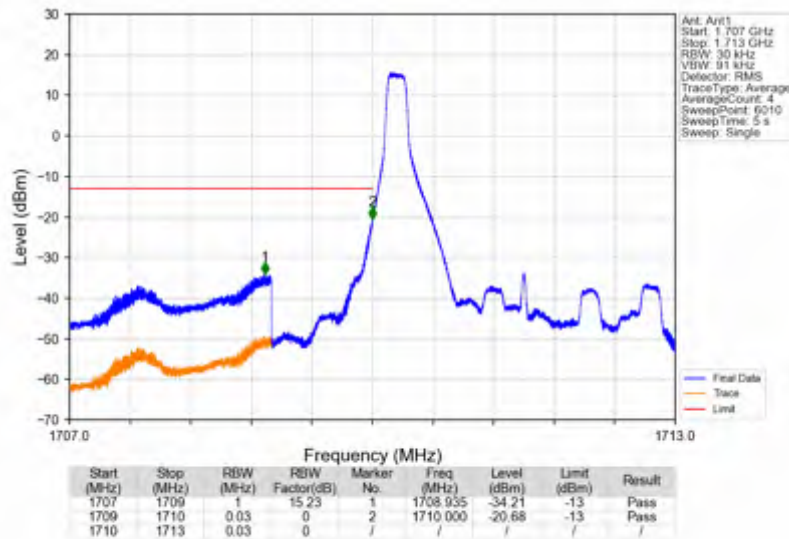
Band66 3MHz 64QAM LCH 1711.5MHz RB 1 0 NTNV
