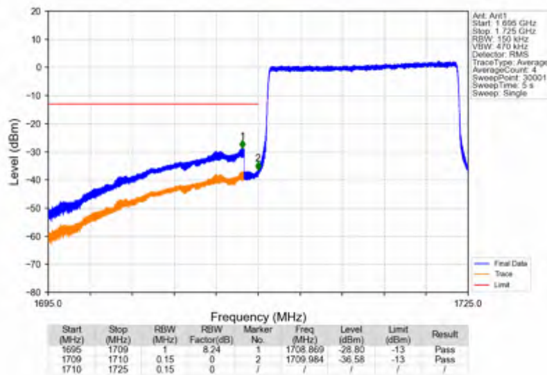
Band66_15MHz_256QAM_LCH_1717.5MHz_RB_75_0_NTNV
