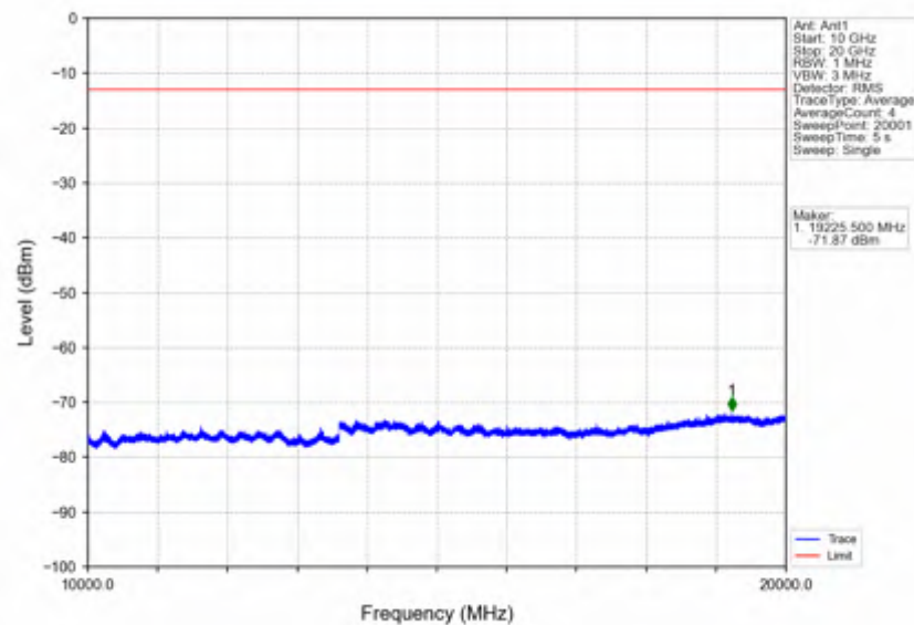
Band66_15MHz_16QAM_LCH_1717.5MHz_RB_75_0_NTNV
