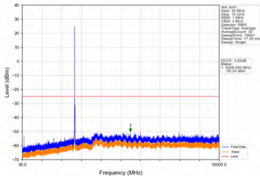
Band41_15MHz_16QAM_HCH_2682.5MHz_RB_1_0_NTNV
