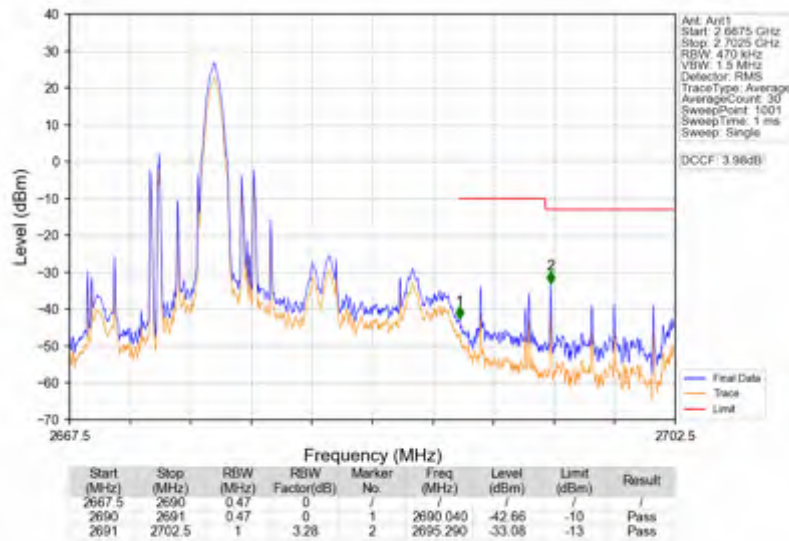
Band41_15MHz_16QAM_HCH_2682.5MHz_RB_1_74_NTNV
