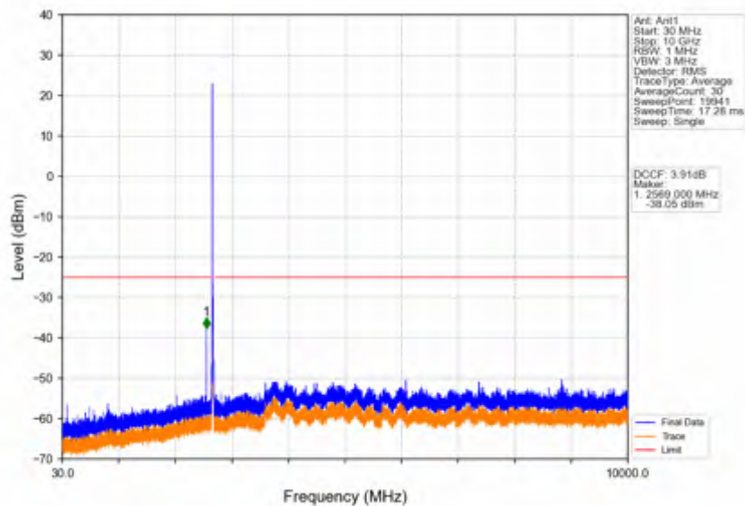
Band41_15MHz_64QAM_HCH_2682.5MHz_RB_1_0_NTNV
