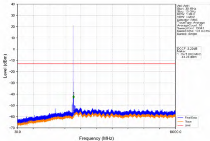
Band42a_10MHz_QPSK_HCH_3545MHz_RB_1_0_NTNV
