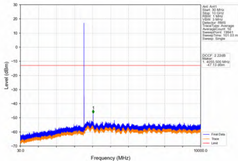
Band42a_5MHz_256QAM_HCH_3547.5MHz_RB_1_0_NTNV
