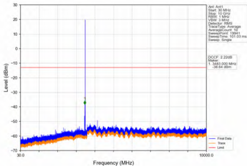
Band42a_5MHz_16QAM_MCH_3500MHz_RB_1_0_NTNV
