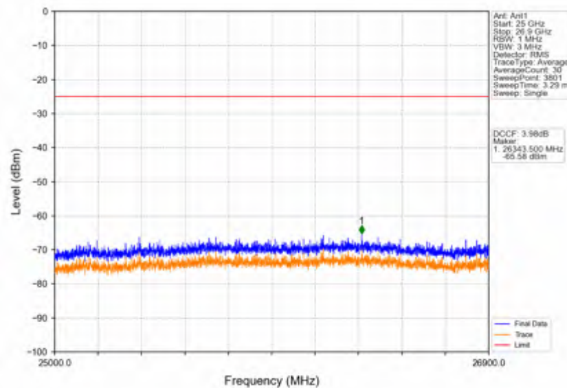
Band41_5MHz_64QAM_LCH_2498.5MHz_RB_1_0_NTNV
