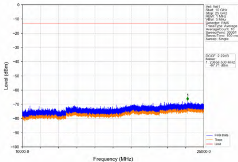
Band42a_5MHz_256QAM_HCH_3547.5MHz_RB_1_0_NTNV
