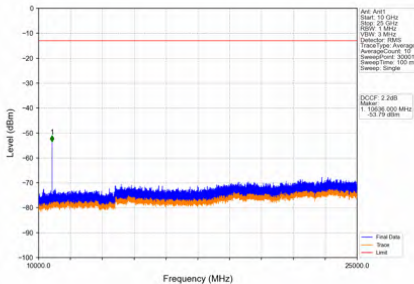
Band42a_5MHz_64QAM_HCH_3547.5MHz_RB_1_0_NTNV
