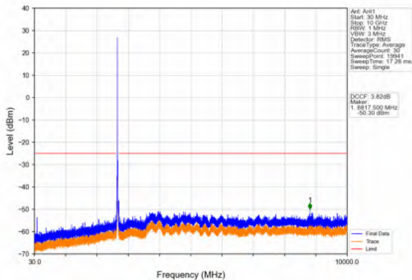
Band41_20MHz_64QAM_HCH_2680MHz_RB_1_0_NTNV
