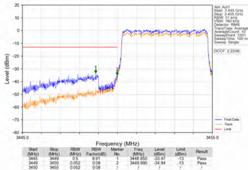
Band42a_5MHz_256QAM_LCH_3452.5MHz_RB_25_0_NTNV
