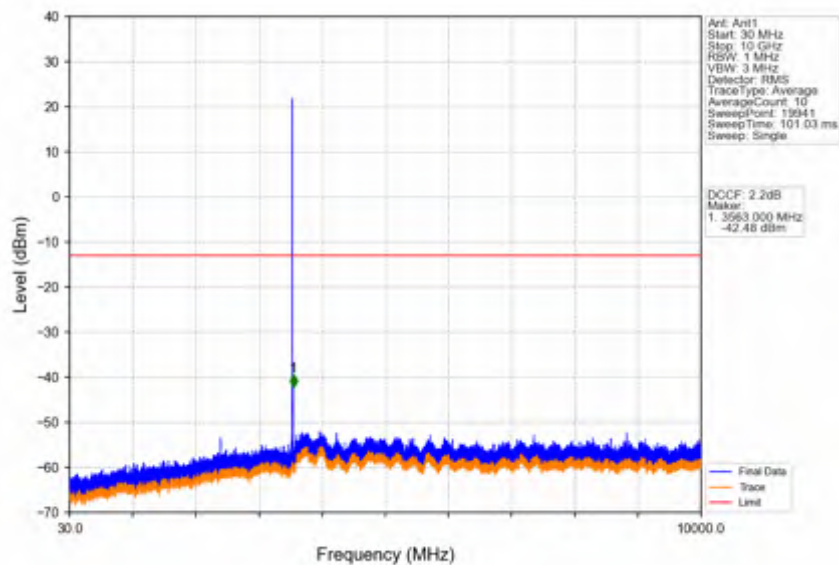
Band42a_5MHz_64QAM_HCH_3547.5MHz_RB_1_0_NTNV
