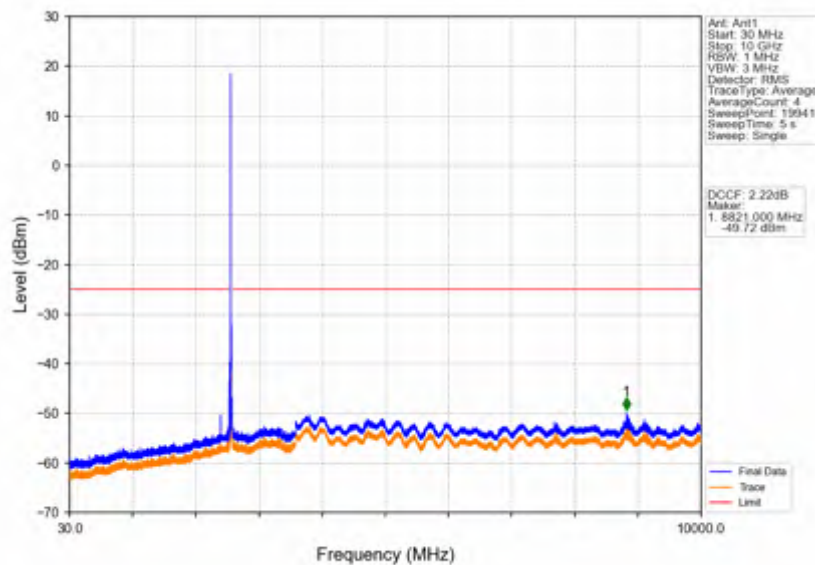
Band38_15MHz_256QAM_LCH_2577.5MHz_RB_1_0_NTNV
