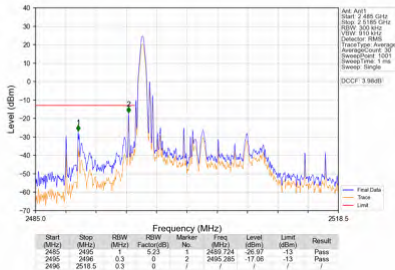
Band41_15MHz_16QAM_LCH_2503.5MHz_RB_75_0_NTNV
