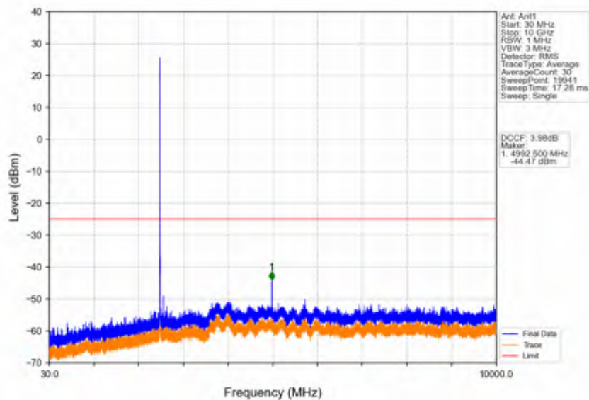
Band41_5MHz_16QAM_LCH_2498.5MHz_RB_1_0_NTNV
