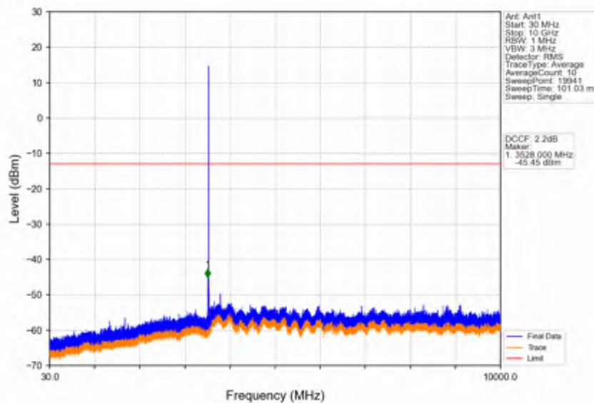
Band42a_5MHz_16QAM_HCH_3547.5MHz_RB_1_0_NTNV
