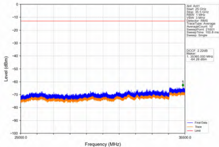
Band42a_5MHz_QPSK_LCH_3452.5MHz_RB_1_0_NTNV
