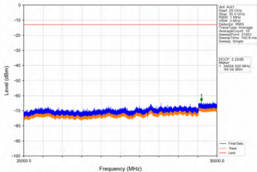
Band42a_5MHz_16QAM_HCH_3547.5MHz_RB_1_0_NTNV
