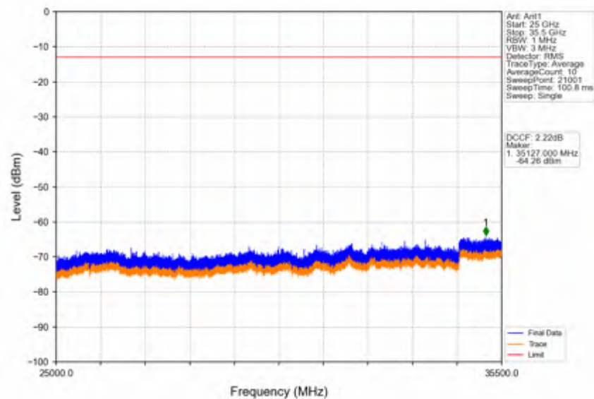
Band42a_5MHz_QPSK_MCH_3500MHz_RB_1_0_NTNV
