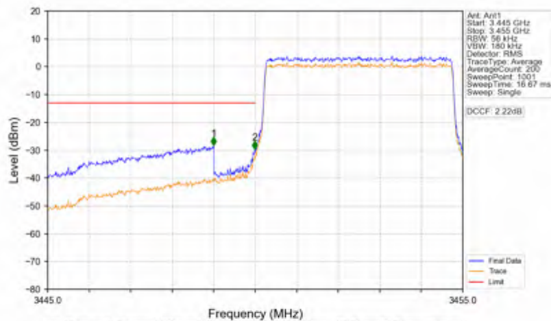
Band42a_5MHz_16QAM_LCH_3452.5MHz_RB_25_0_NTNV
