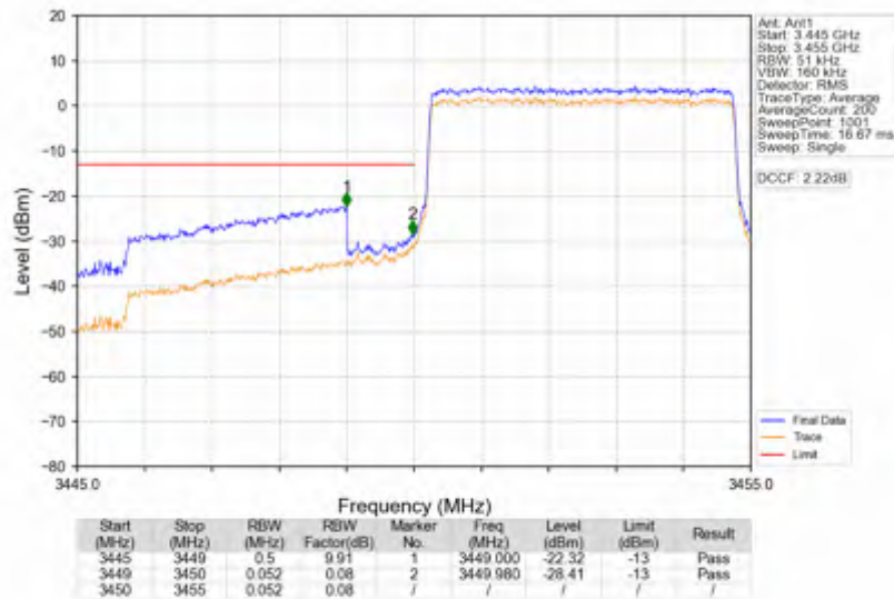
Band42a_5MHz_QPSK_LCH_3452.5MHz_RB_25_0_NTNV
