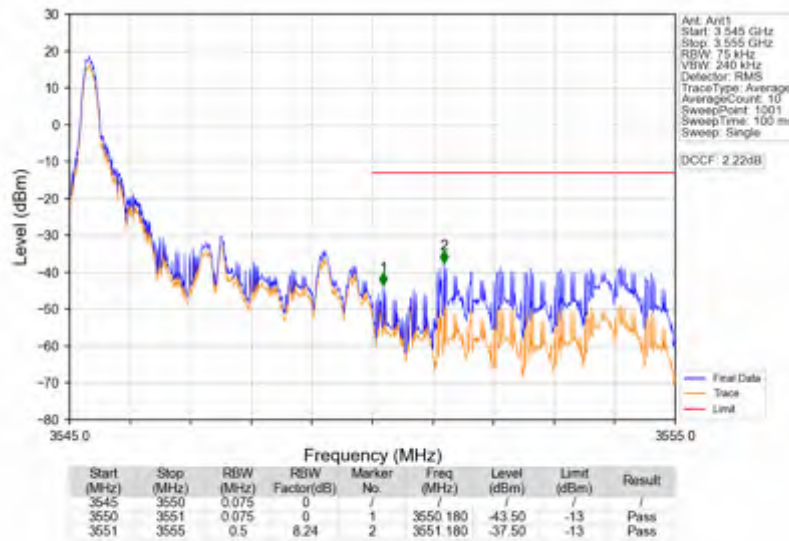
Band42a_5MHz_16QAM_HCH_3547.5MHz_RB_1_24_NTNV
