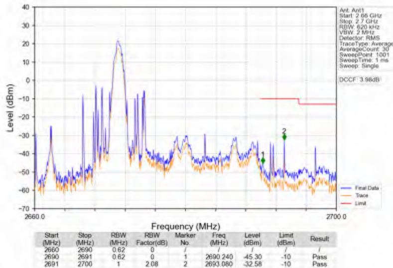
Band41_20MHz_64QAM_HCH_2680MHz_RB_1_99_NTNV
