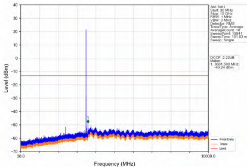
Band42a_5MHz_64QAM_MCH_3500MHz_RB_1_0_NTNV
