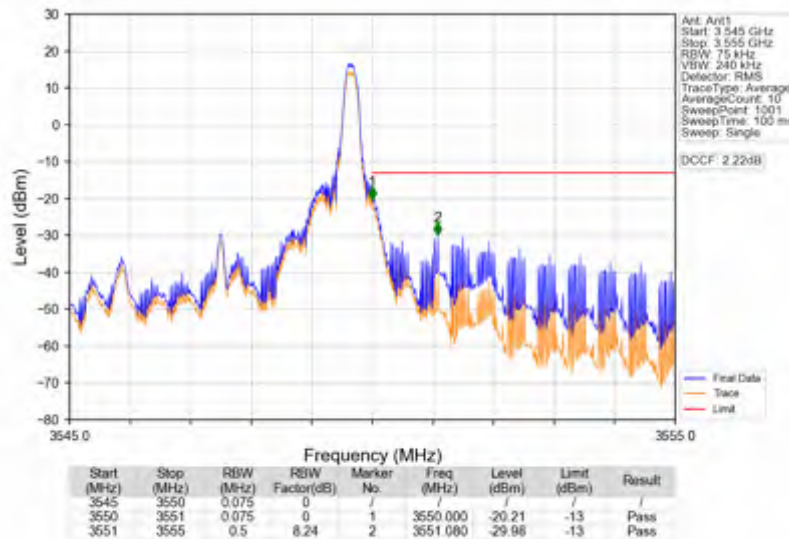
Band42a_5MHz_256QAM_HCH_3547.5MHz_RB_1_24_NTNV
