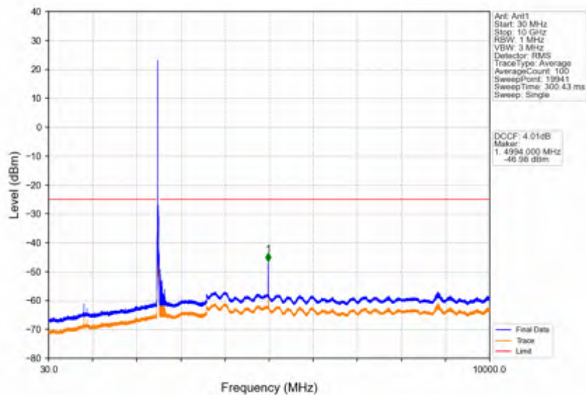
Band41_20MHz_16QAM_LCH_2506MHz_RB_1_0_NTNV
