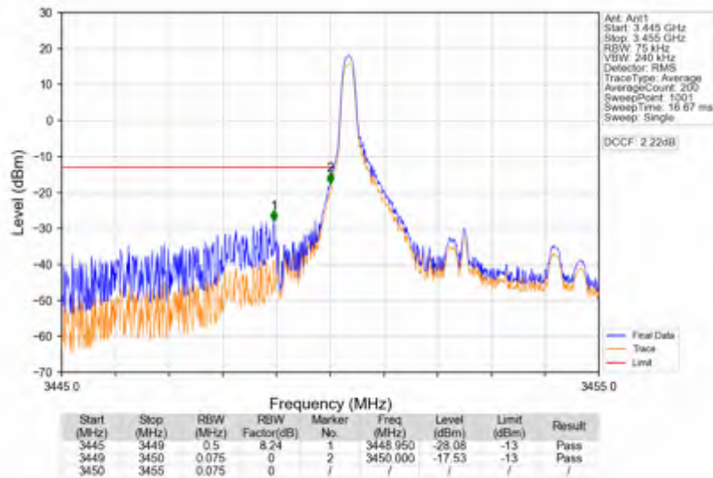
Band42a_5MHz_64QAM_LCH_3452.5MHz_RB_1_0_NTNV
