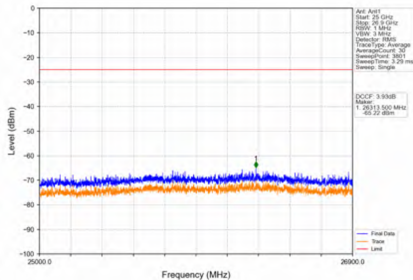
Band41_15MHz_16QAM_HCH_2682.5MHz_RB_1_0_NTNV
