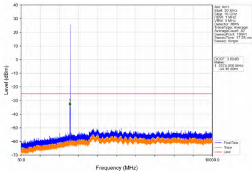
Band41_5MHz_16QAM_MCH_2593MHz_RB_1_0_NTNV
