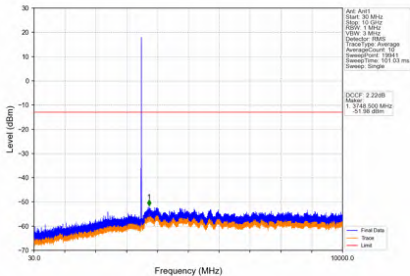
Band42a_5MHz_256QAM_MCH_3500MHz_RB_1_0_NTNV
