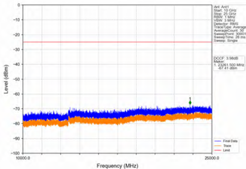
Band41_15MHz_256QAM_MCH_2593MHz_RB_1_0_NTNV
