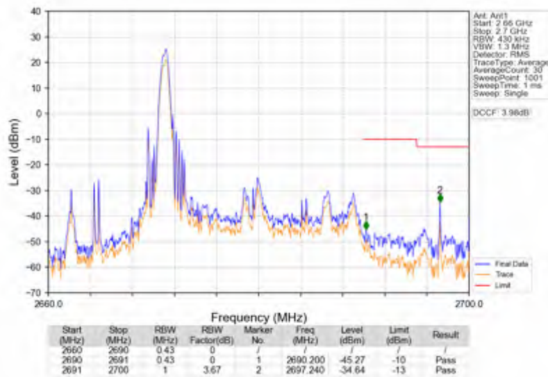
Band41_20MHz_16QAM_HCH_2680MHz_RB_100_0_NTNV
