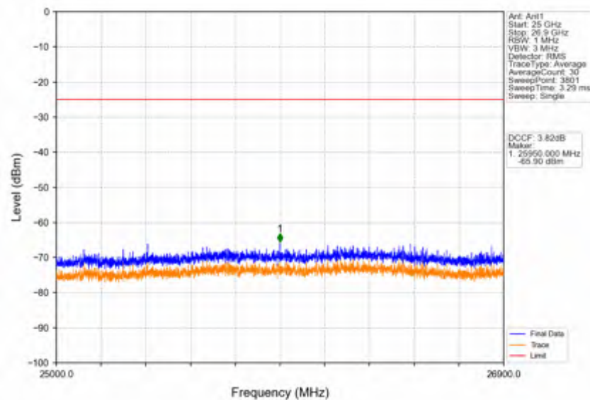
Band41_5MHz_16QAM_HCH_2687.5MHz_RB_1_0_NTNV
