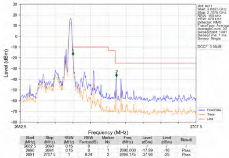
Band41_5MHz_256QAM_HCH_2687.5MHz_RB_1_24_NTNV
