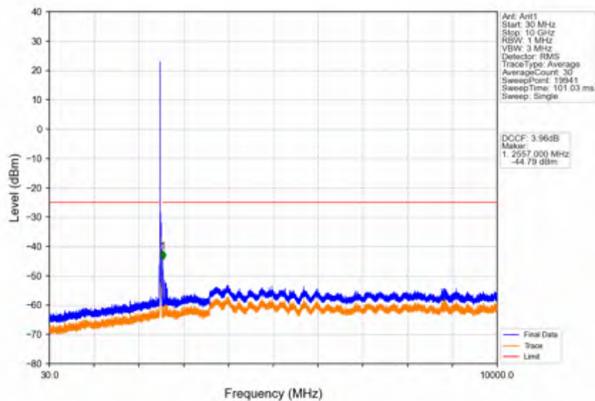
Band41_20MHz_256QAM_LCH_2506MHz_RB_1_0_NTNV
