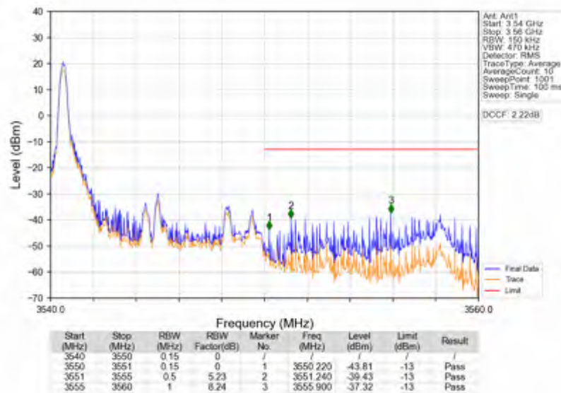
Band42a_10MHz_QPSK_HCH_3545MHz_RB_1_49_NTNV
