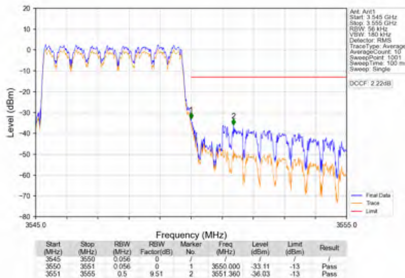
Band42a_5MHz_256QAM_HCH_3547.5MHz_RB_25_0_NTNV
