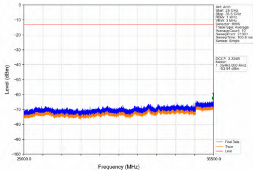
Band42a_10MHz_16QAM_HCH_3545MHz_RB_1_0_NTNV
