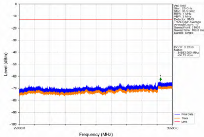
Band42a_5MHz_16QAM_LCH_3452.5MHz_RB_25_0_NTNV
