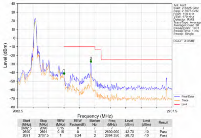
Band41_5MHz_16QAM_HCH_2687.5MHz_RB_1_24_NTNV
