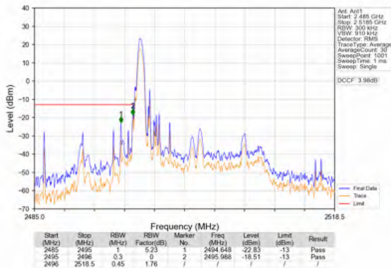
Band41_15MHz_256QAM_LCH_2503.5MHz_RB_1_0_NTNV
