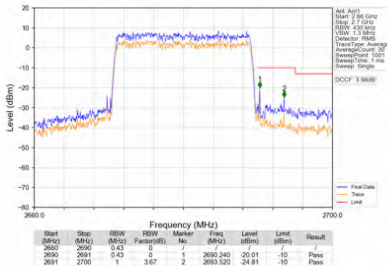
Band41_20MHz_256QAM_HCH_2680MHz_RB_100_0_NTNV
