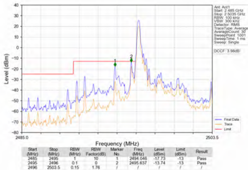
Band41_5MHz_16QAM_LCH_2498.5MHz_RB_1_0_NTNV
