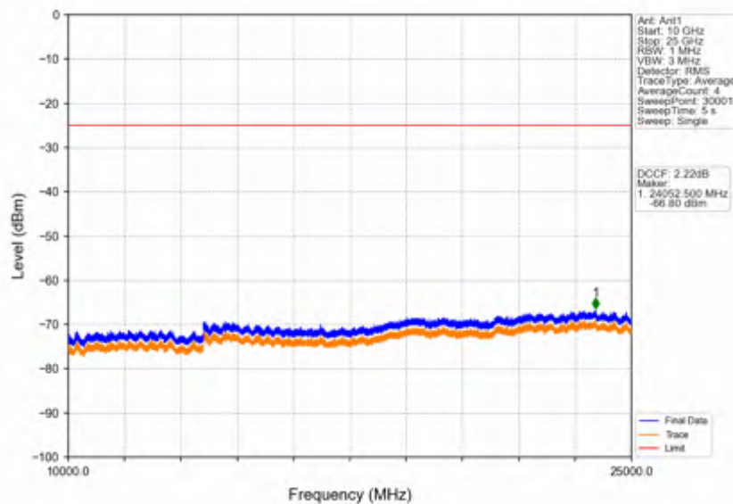
Band38_15MHz_256QAM_MCH_2595MHz_RB_1_0_NTNV
