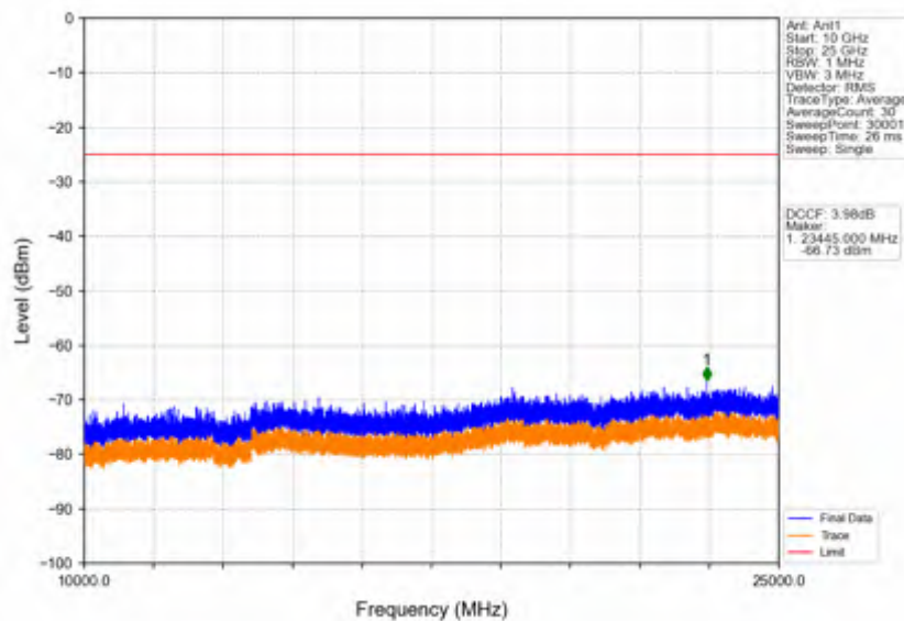
Band41_15MHz_256QAM_LCH_2503.5MHz_RB_1_0_NTNV
