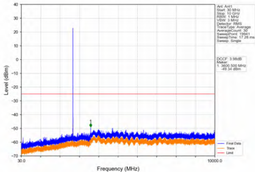
Band41_5MHz_256QAM_HCH_2687.5MHz_RB_1_0_NTNV
