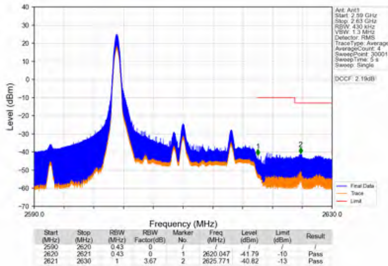
Band38_20MHz_64QAM_HCH_2610MHz_RB_100_0_NTNV
