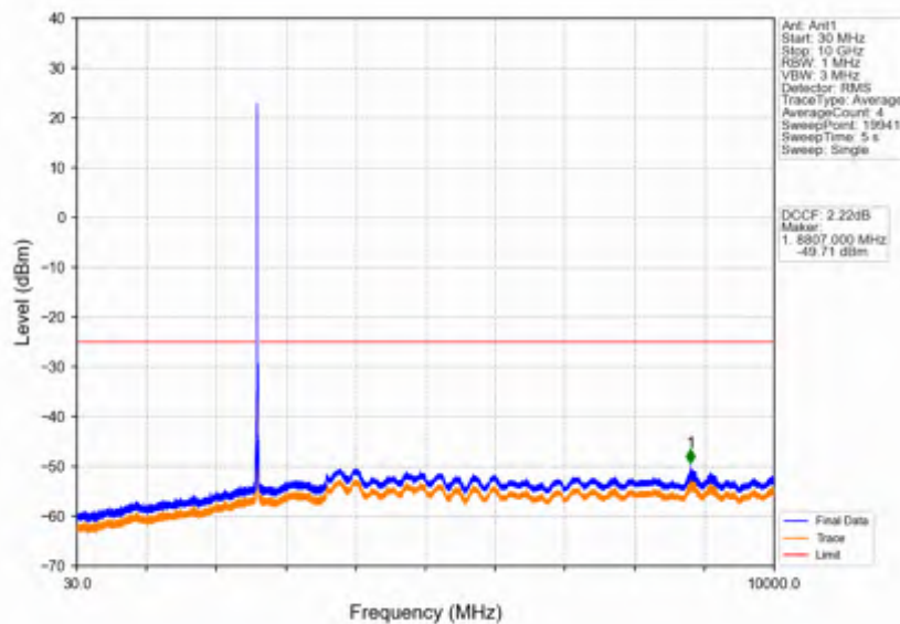
Band38_15MHz_64QAM_HCH_2612.5MHz_RB_1_0_NTNV
