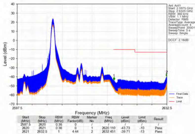
Band38_15MHz_64QAM_HCH_2612.5MHz_RB_1_74_NTNV
