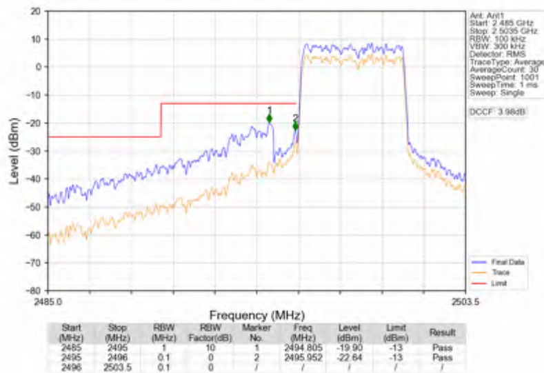
Band41_5MHz_256QAM_LCH_2498.5MHz_RB_25_0_NTNV
