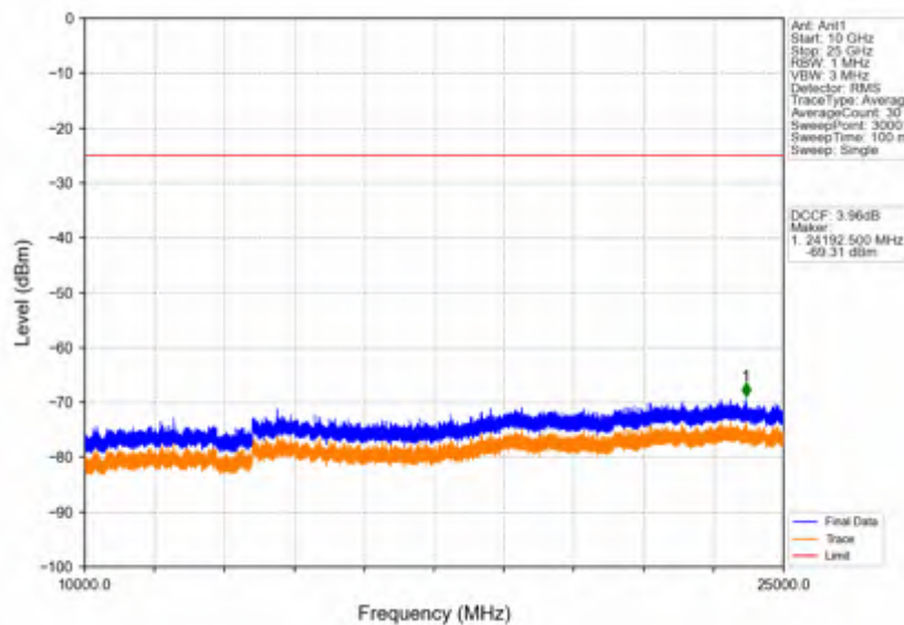
Band41_20MHz_256QAM_LCH_2506MHz_RB_1_0_NTNV
