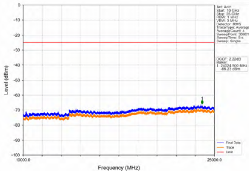
Band38_15MHz_256QAM_LCH_2577.5MHz_RB_1_0_NTNV
