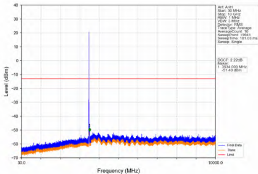
Band42a_10MHz_16QAM_MCH_3500MHz_RB_1_0_NTNV
