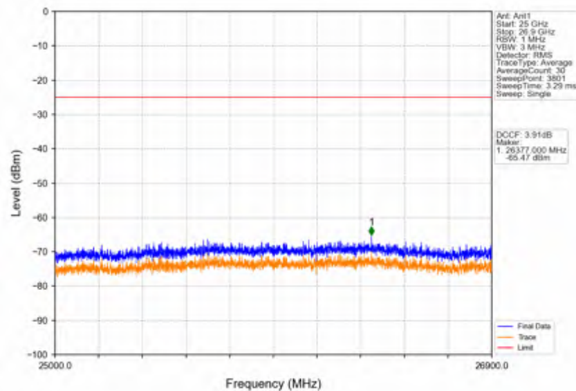
Band41_20MHz_16QAM_HCH_2680MHz_RB_1_0_NTNV
