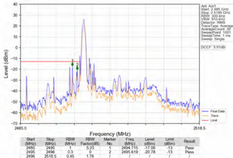
Band41_15MHz_64QAM_LCH_2503.5MHz_RB_1_0_NTNV
