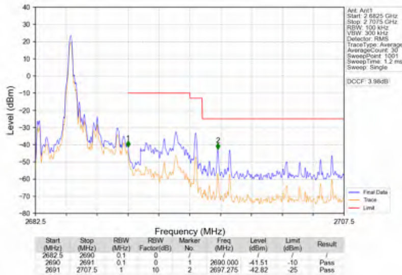
Band41_5MHz_16QAM_HCH_2687.5MHz_RB_25_0_NTNV
