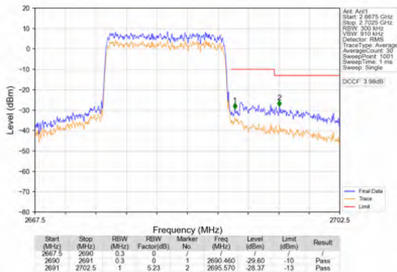
Band41_15MHz_256QAM_HCH_2682.5MHz_RB_75_0_NTNV
