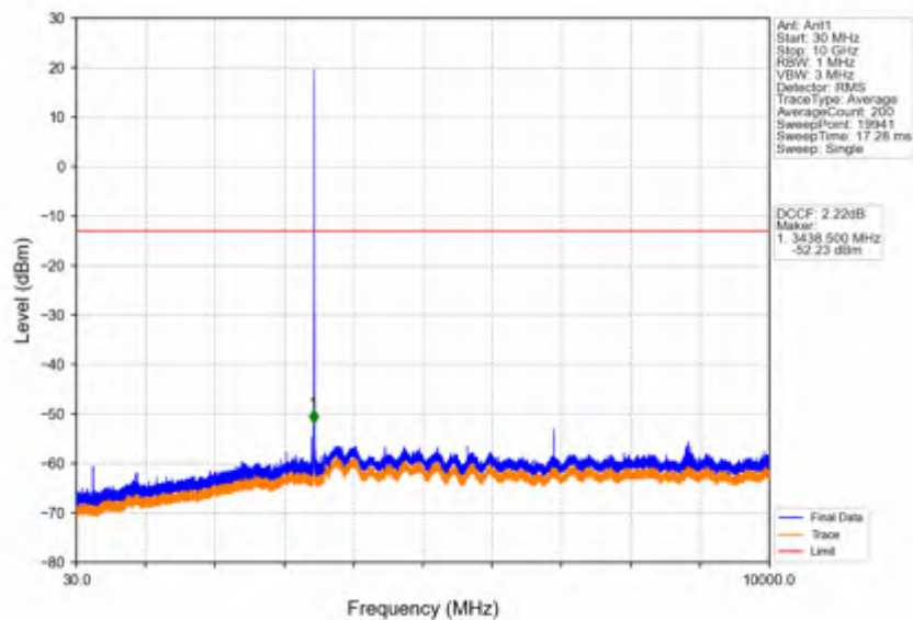
Band42a_5MHz_64QAM_LCH_3452.5MHz_RB_1_0_NTNV
