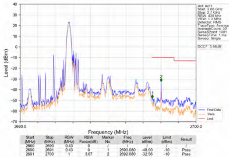
Band41_20MHz_64QAM_HCH_2680MHz_RB_100_0_NTNV
