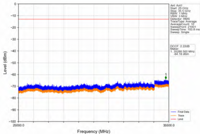
Band42a_5MHz_256QAM_HCH_3547.5MHz_RB_1_0_NTNV
