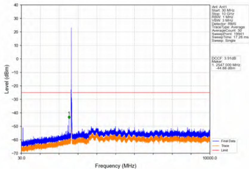
Band41_20MHz_16QAM_HCH_2680MHz_RB_1_0_NTNV
