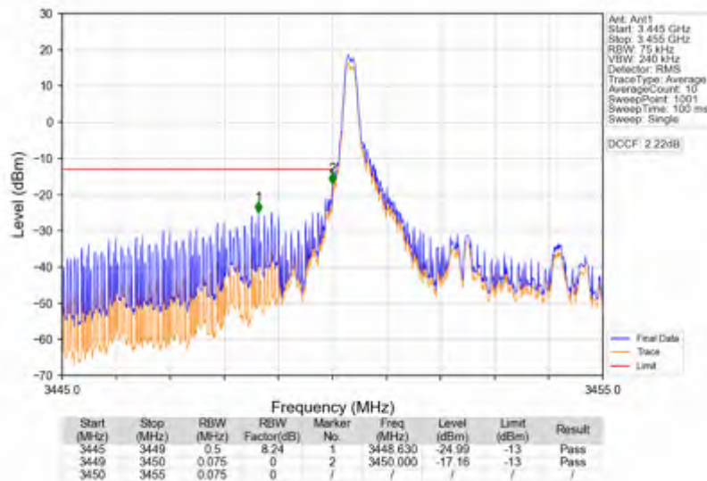
Band42a_5MHz_QPSK_LCH_3452.5MHz_RB_1_0_NTNV
