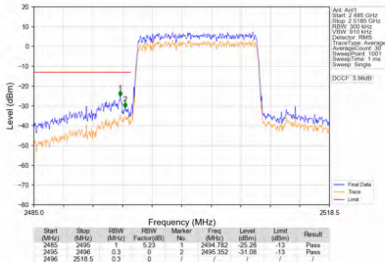
Band41_15MHz_256QAM_LCH_2503.5MHz_RB_75_0_NTNV
