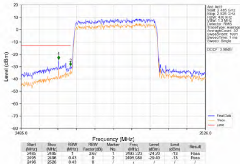
Band41_20MHz_256QAM_LCH_2506MHz_RB_100_0_NTNV
