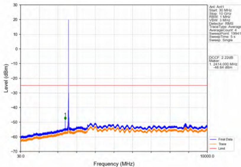
Band38_15MHz_256QAM_MCH_2595MHz_RB_1_0_NTNV
