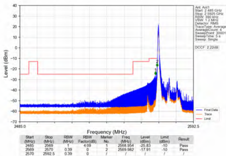
Band38_15MHz_256QAM_LCH_2577.5MHz_RB_1_0_NTNV
