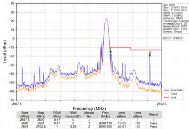
Band41_15MHz_256QAM_HCH_2682.5MHz_RB_1_74_NTNV
