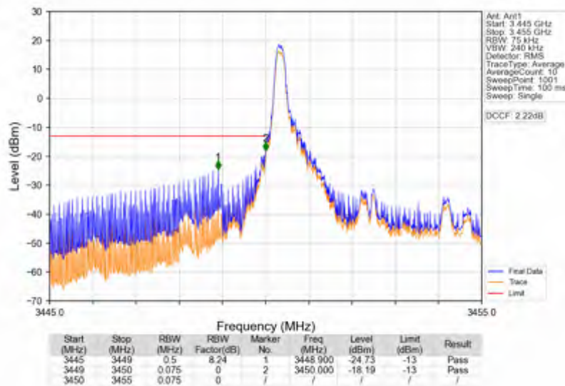
Band42a_5MHz_16QAM_LCH_3452.5MHz_RB_1_0_NTNV
