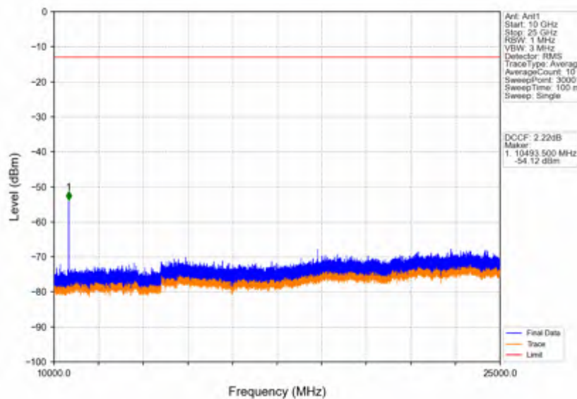
Band42a_5MHz_16QAM_MCH_3500MHz_RB_1_0_NTNV
