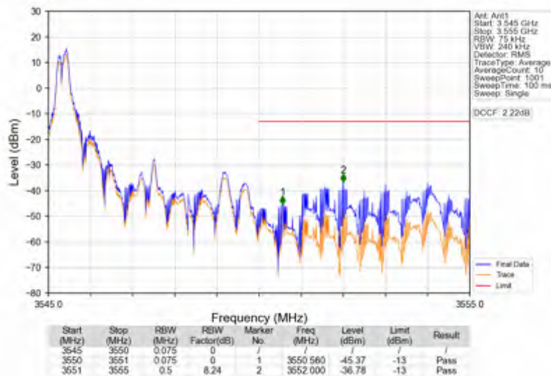
Band42a_5MHz_QPSK_HCH_3547.5MHz_RB_1_24_NTNV
