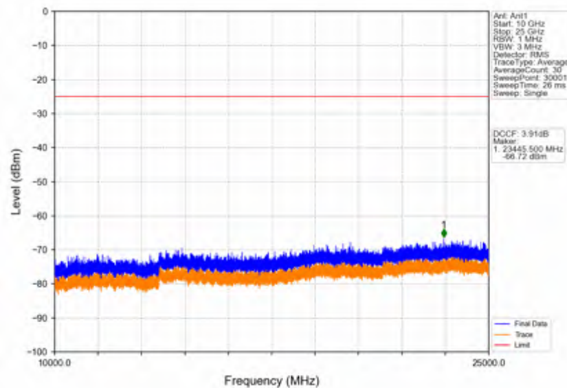
Band41_20MHz_16QAM_HCH_2680MHz_RB_1_0_NTV
