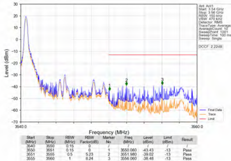
Band42a_10MHz_QPSK_HCH_3545MHz_RB_50_0_NTNV
