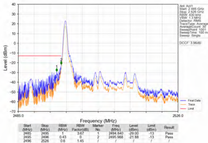
Band41_20MHz_256QAM_LCH_2506MHz_RB_1_0_NTNV
