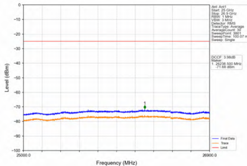
Band41_10MHz_64QAM_LCH_2501MHz_RB_1_0_NTNV
