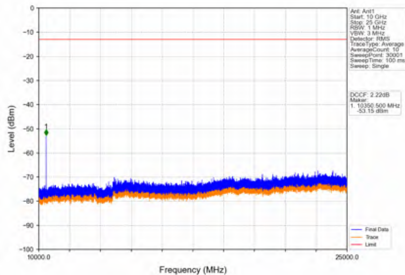
Band42a_5MHz_QPSK_LCH_3452.5MHz_RB_1_0_NTNV
