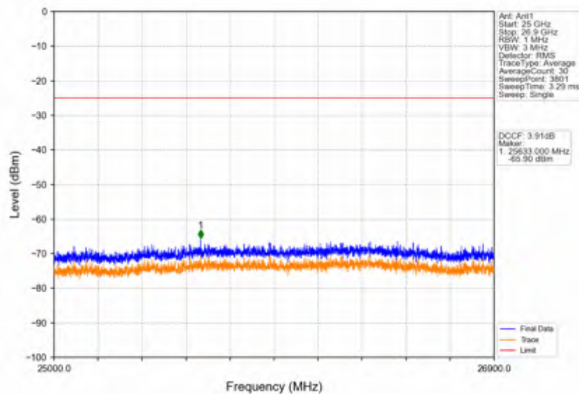
Band41_15MHz_64QAM_HCH_2682.5MHz_RB_1_74_NTNV
