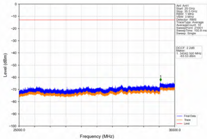
Band42a_5MHz_64QAM_HCH_3547.5MHz_RB_1_24_NTNV
