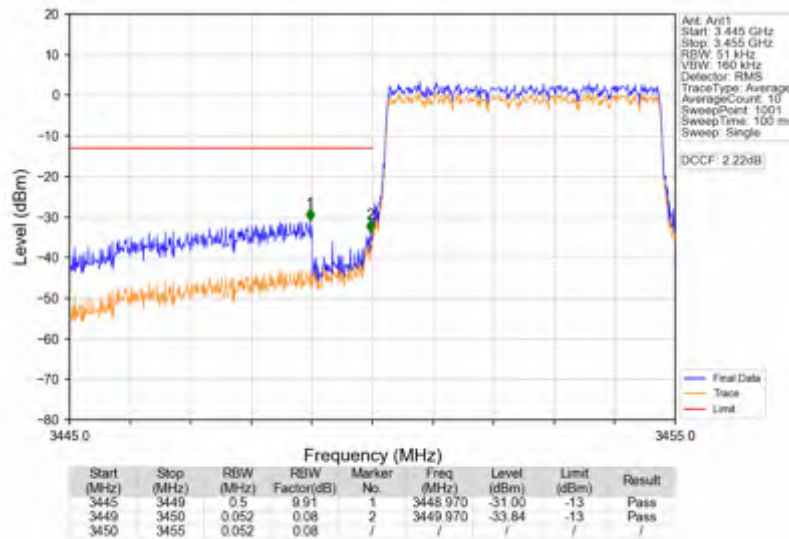
Band42a_5MHz_64QAM_LCH_3452.5MHz_RB_25_0_NTNV
