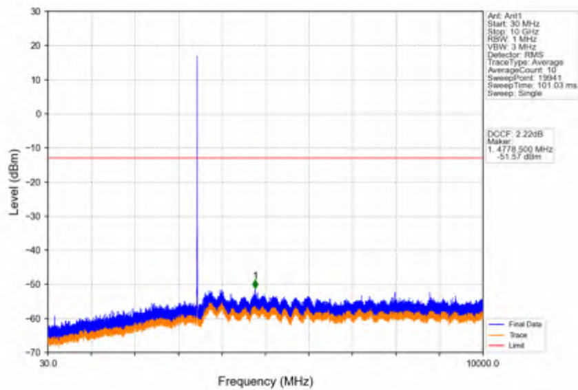
Band42a_5MHz_256QAM_LCH_3452.5MHz_RB_1_0_NTNV
