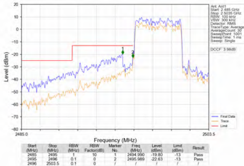
Band41_5MHz_64QAM_LCH_2498.5MHz_RB_25_0_NTNV
