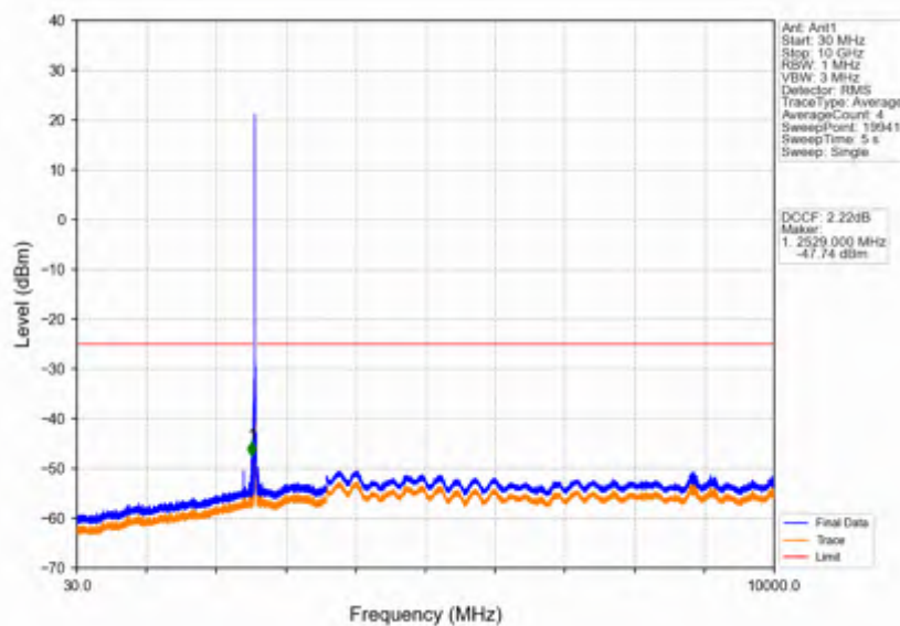
Band38_15MHz_64QAM_LCH_2577.5MHz_RB_1_0_NTNV
