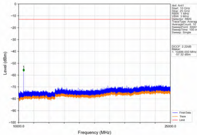
Band42a_10MHz_16QAM_MCH_3500MHz_RB_1_0_NTNV
