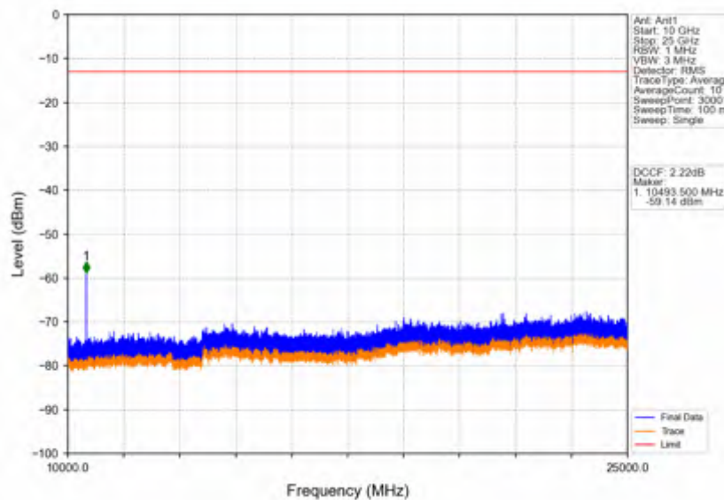
Band42a_5MHz_256QAM_MCH_3500MHz_RB_1_0_NTNV
