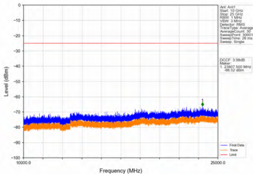
Band41_5MHz_256QAM_LCH_2498.5MHz_RB_1_0_NTNV
