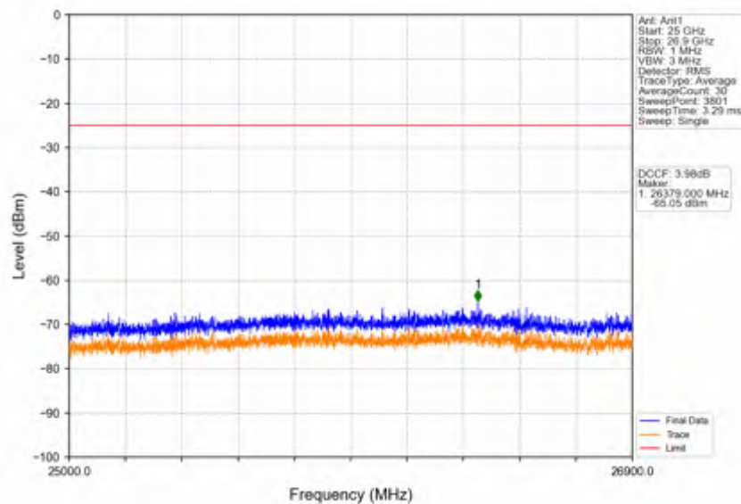
Band41_15MHz_256QAM_HCH_2682.5MHz_RB_1_0_NTNV
