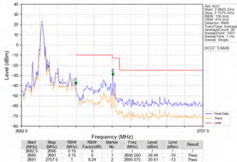
Band41_5MHz_64QAM_HCH_2687.5MHz_RB_1_24_NTNV
