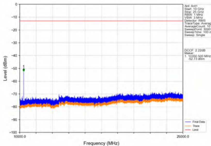
Band42a_5MHz_16QAM_LCH_3452.5MHz_RB_1_0_NTNV
