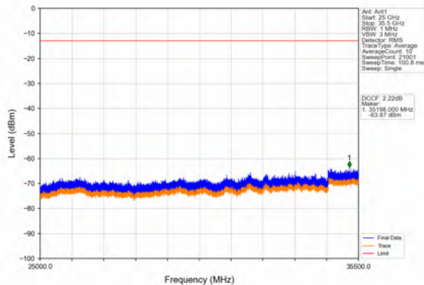
Band42a_5MHz_64QAM_MCH_3500MHz_RB_1_0_NTNV
