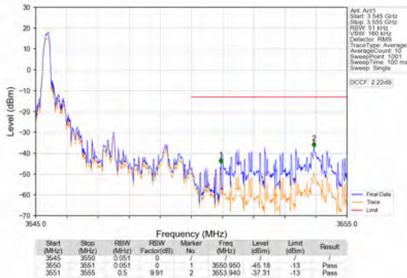
Band42a_5MHz_QPSK_HCH_3547.5MHz_RB_25_0_NTNV
