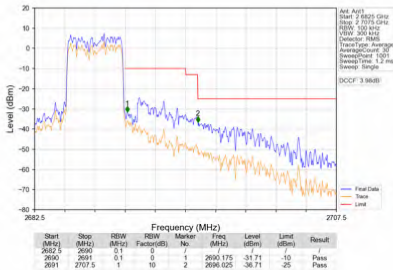
Band41_5MHz_256QAM_HCH_2687.5MHz_RB_25_0_NTNV
