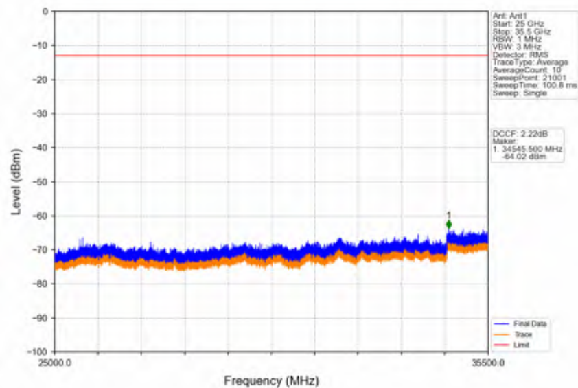
Band42a_5MHz_256QAM_LCH_3452.5MHz_RB_25_0_NTNV
