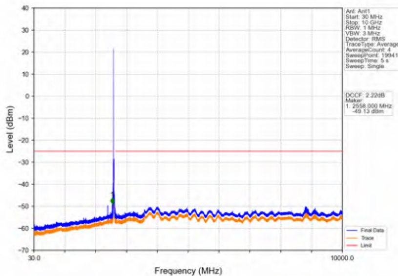
Band38_20MHz_64QAM_HCH_2610MHz_RB_1_0_NTNV
