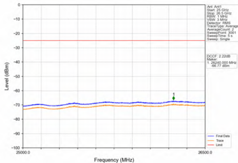
Band38_15MHz_256QAM_HCH_2612.5MHz_RB_1_0_NTNV
