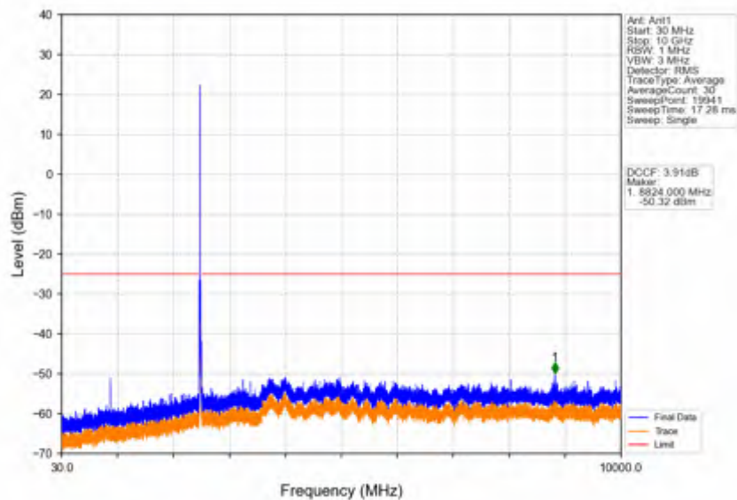
Band41_15MHz_16QAM_LCH_2503.5MHz_RB_1_0_NTNV
