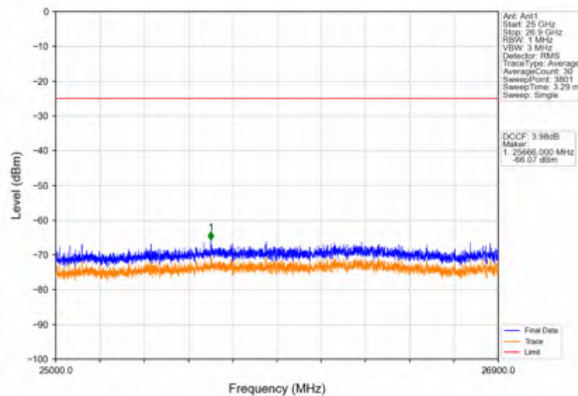
Band41_15MHz_256QAM_HCH_2682.5MHz_RB_1_0_NTNV
