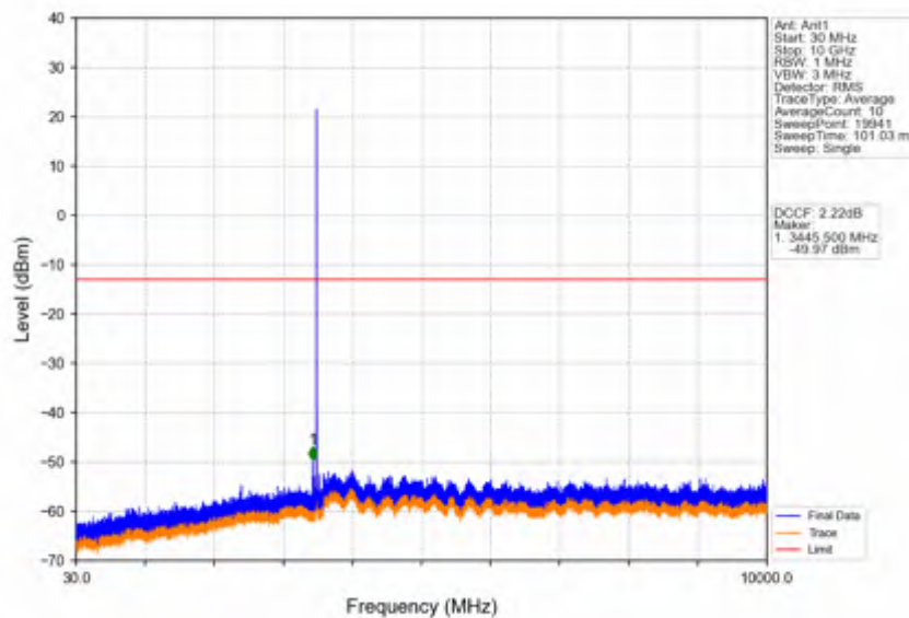
Band42a_5MHz_QPSK_MCH_3500MHz_RB_1_0_NTNV
