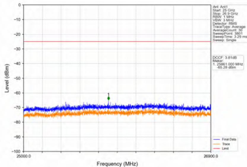
Band41_5MHz_64QAM_HCH_2687.5MHz_RB_1_24_NTNV
