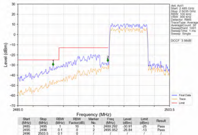
Band41_5MHz_16QAM_LCH_2498.5MHz_RB_25_0_NTNV
