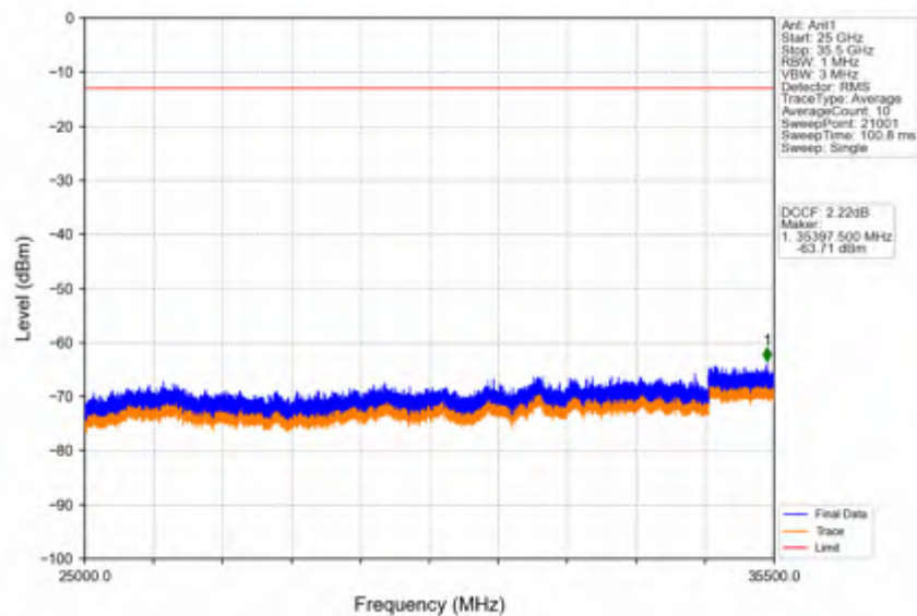
Band42a_5MHz_QPSK_HCH_3547.5MHz_RB_1_24_NTNV
