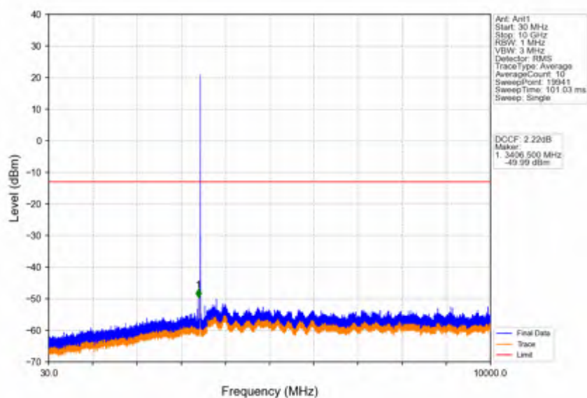
Band42a_5MHz_QPSK_LCH_3452.5MHz_RB_1_0_NTNV
