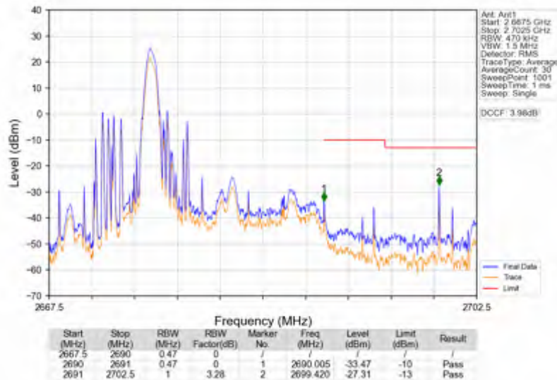
Band41_15MHz_64QAM_HCH_2682.5MHz_RB_1_74_NTNV
