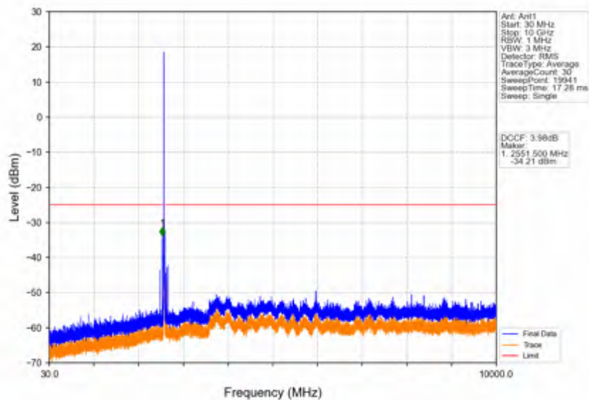
Band41_15MHz_256QAM_MCH_2593MHz_RB_1_0_NTNV
