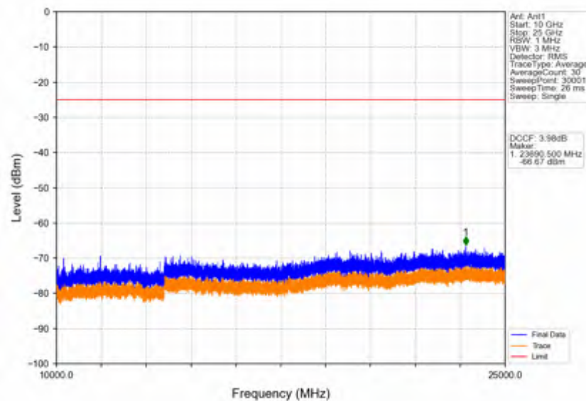
Band41_5MHz_256QAM_HCH_2687.5MHz_RB_1_0_NTNV
