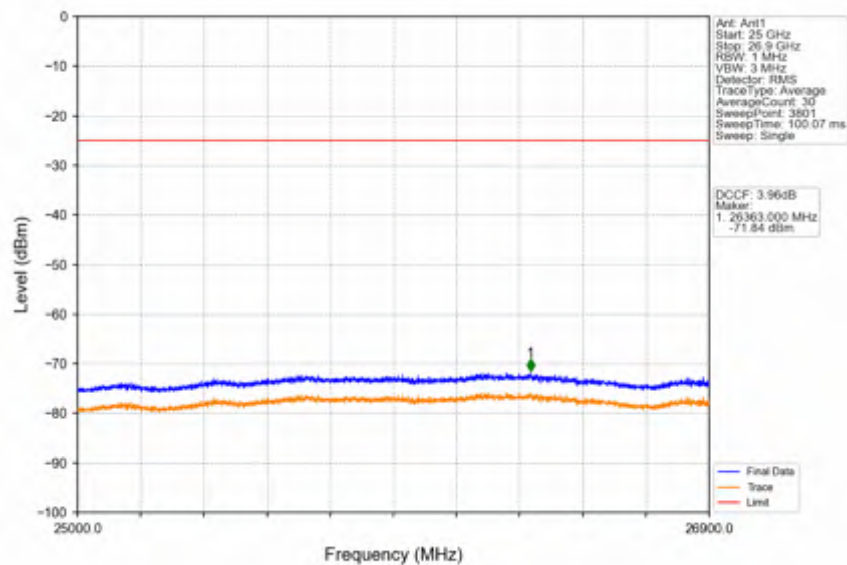
Band41_20MHz_256QAM_LCH_2506MHz_RB_100_0_NTNV
