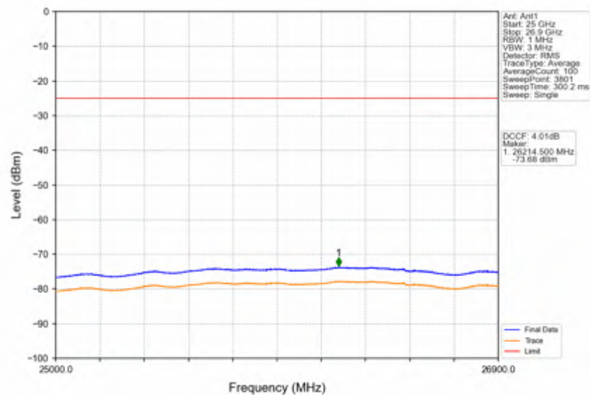
Band41_20MHz_64QAM_LCH_2506MHz_RB_1_0_NTNV
