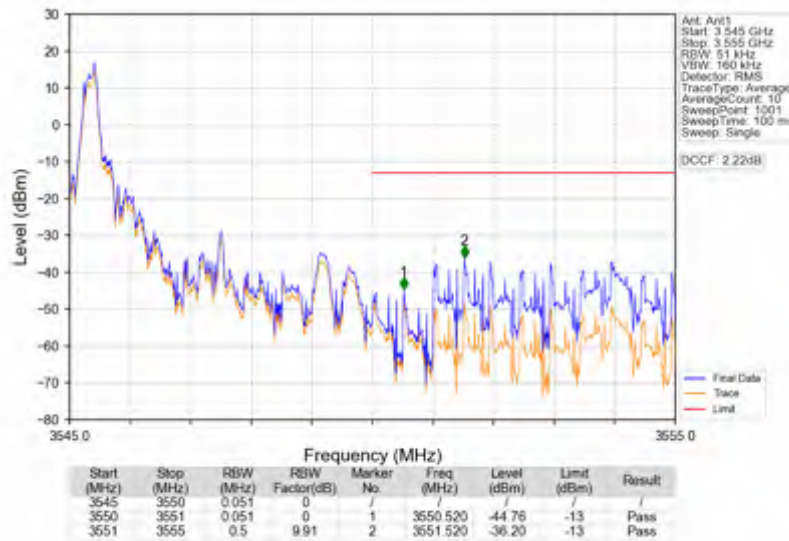
Band42a_5MHz_16QAM_HCH_3547.5MHz_RB_25_0_NTNV
