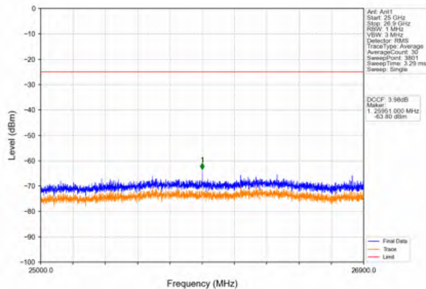
Band41_20MHz_256QAM_HCH_2680MHz_RB_1_0_NTNV
