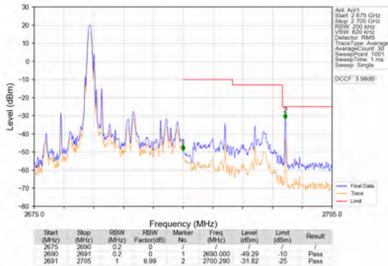
Band41_10MHz_64QAM_HCH_2685MHz_RB_50_0_NTNV
