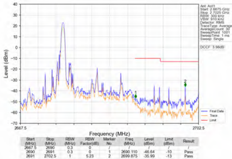
Band41_15MHz_64QAM_HCH_2682.5MHz_RB_75_0_NTNV
