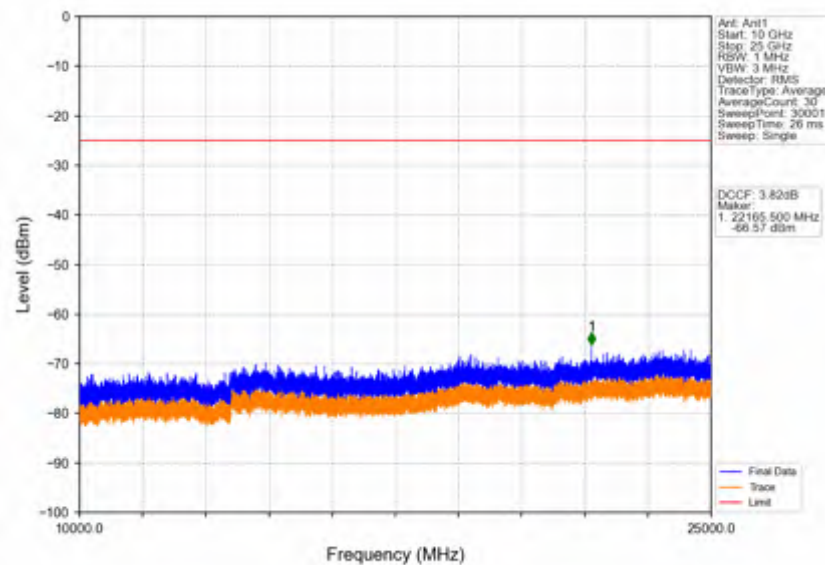
Band41_20MHz_64QAM_MCH_2593MHz_RB_1_0_NTNV
