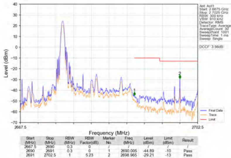
Band41_15MHz_16QAM_HCH_2682.5MHz_RB_75_0_NTNV
