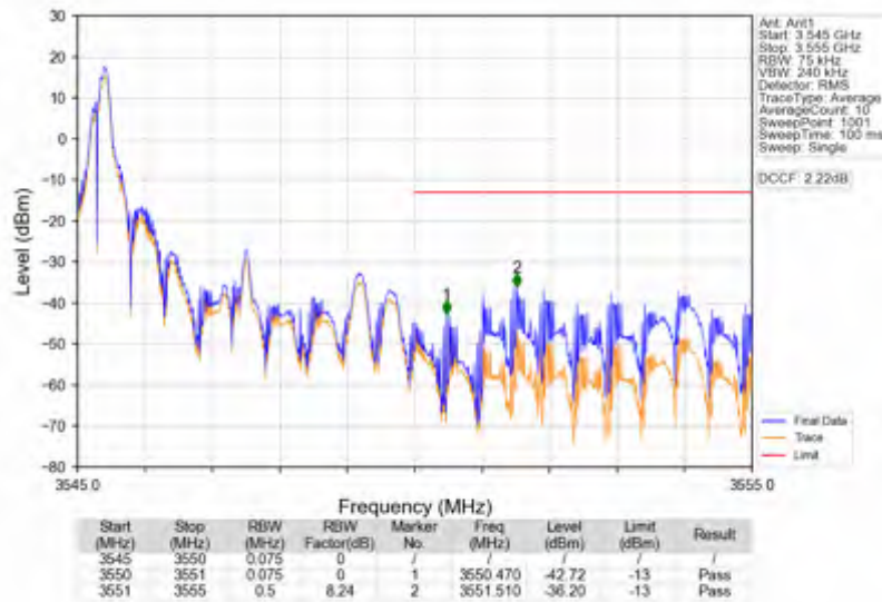
Band42a_5MHz_64QAM_HCH_3547.5MHz_RB_1_24_NTNV
