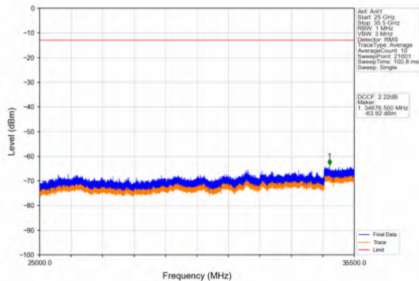
Band42a_10MHz_QPSK_HCH_3545MHz_RB_1_49_NTNV
