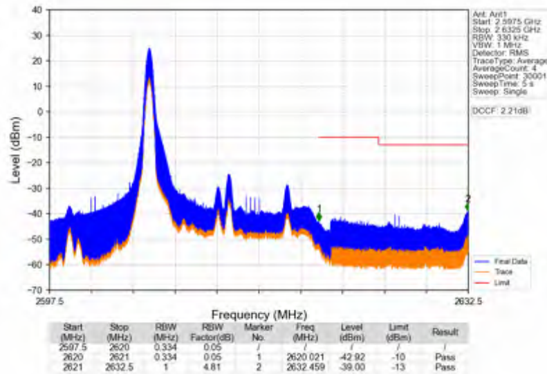
Band38_15MHz_16QAM_HCH_2612.5MHz_RB_1_74_NTNV
