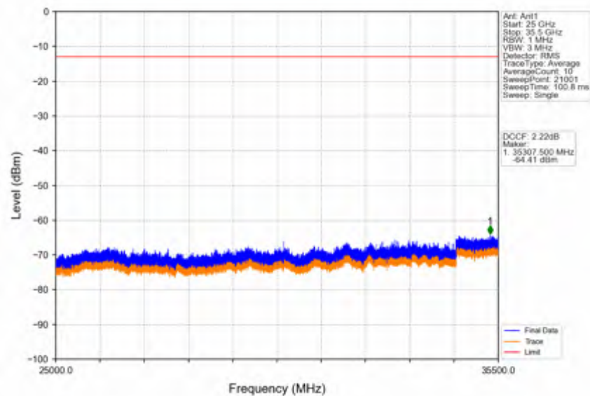
Band42a_5MHz_64QAM_LCH_3452.5MHz_RB_1_0_NTNV
