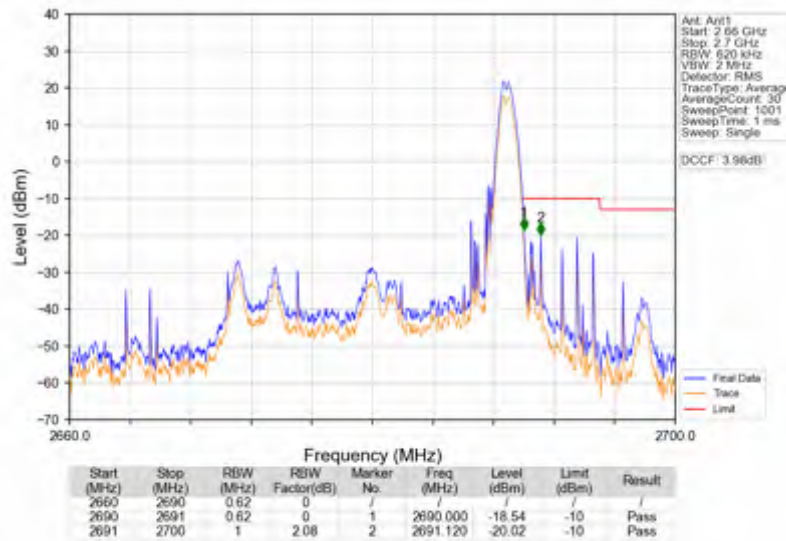
Band41_20MHz_256QAM_HCH_2680MHz_RB_1_99_NTNV
