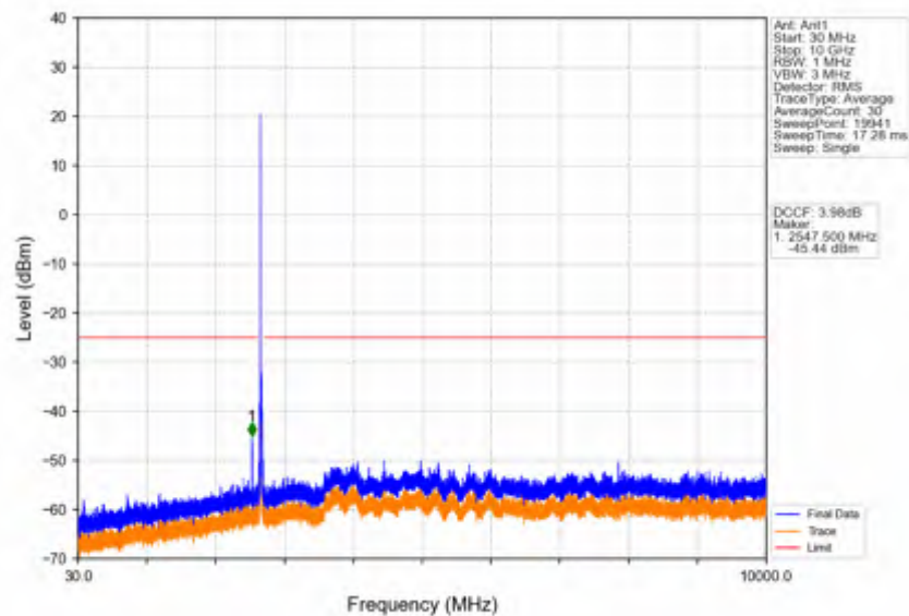
Band41_20MHz_256QAM_HCH_2680MHz_RB_1_0_NTNV
