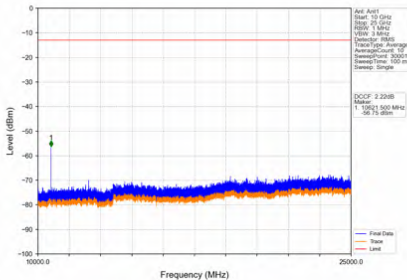
Band42a_10MHz_QPSK_HCH_3545MHz_RB_1_0_NTNV
