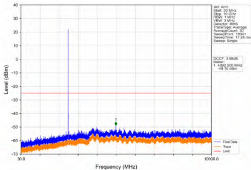
Band41_5MHz_256QAM_LCH_2498.5MHz_RB_1_0_NTNV
