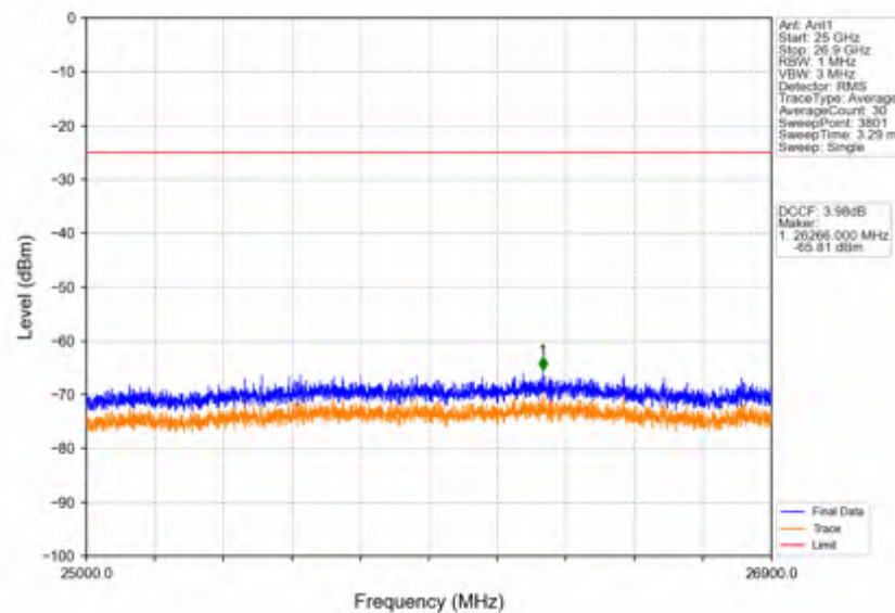
Band41_20MHz_256QAM_HCH_2680MHz_RB_1_0_NTNV
