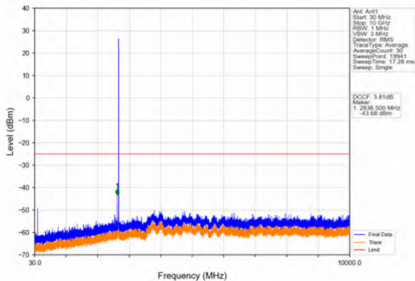
Band41_5MHz_64QAM_HCH_2687.5MHz_RB_1_0_NTNV
