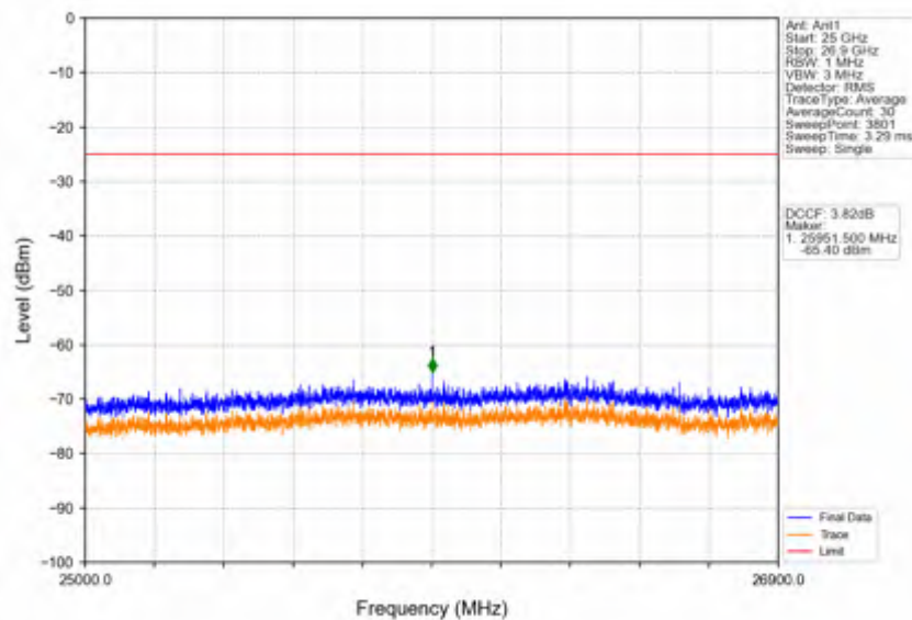
Band41_20MHz_64QAM_HCH_2680MHz_RB_1_99_NTNV
