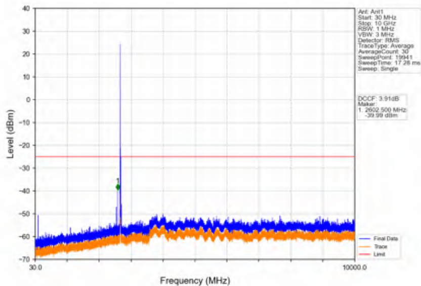
Band41_10MHz_64QAM_HCH_2685MHz_RB_1_0_NTNV
