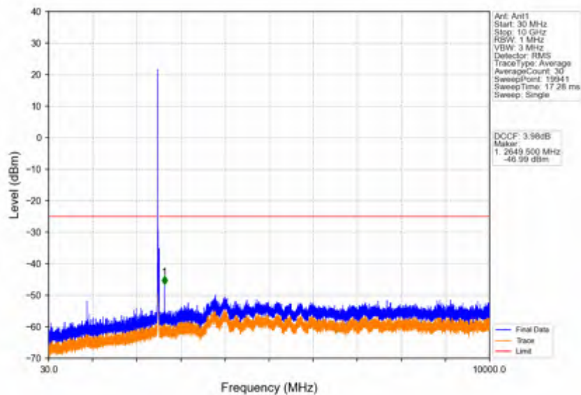
Band41_15MHz_256QAM_LCH_2503.5MHz_RB_1_0_NTNV
