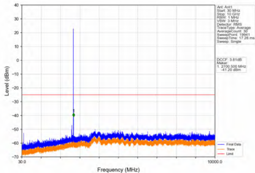
Band41_5MHz_16QAM_HCH_2687.5MHz_RB_1_0_NTNV
