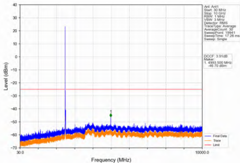
Band41_15MHz_64QAM_LCH_2503.5MHz_RB_1_0_NTNV
