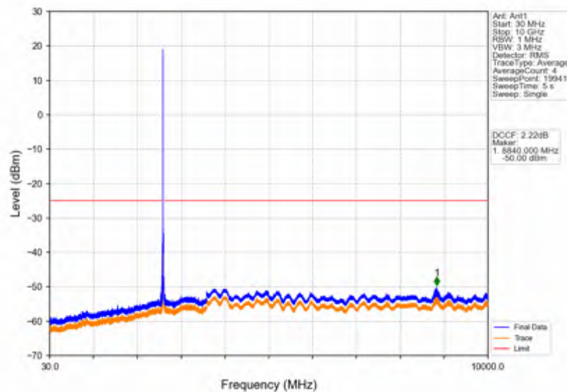
Band38_15MHz_256QAM_HCH_2612.5MHz_RB_1_0_NTNV
