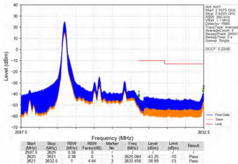
Band38_15MHz_64QAM_HCH_2612.5MHz_RB_75_0_NTNV
