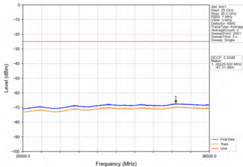
Band38_15MHz_64QAM_HCH_2612.5MHz_RB_1_74_NTNV
