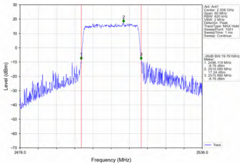
Band41_20MHz_256QAM_LCH_2506MHz_RB_100_0_NTNV
