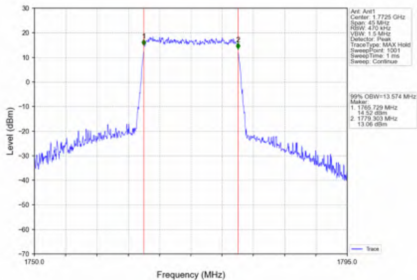
Band66_15MHz_16QAM_HCH_1772.5MHz_RB_75_0_NTNV
