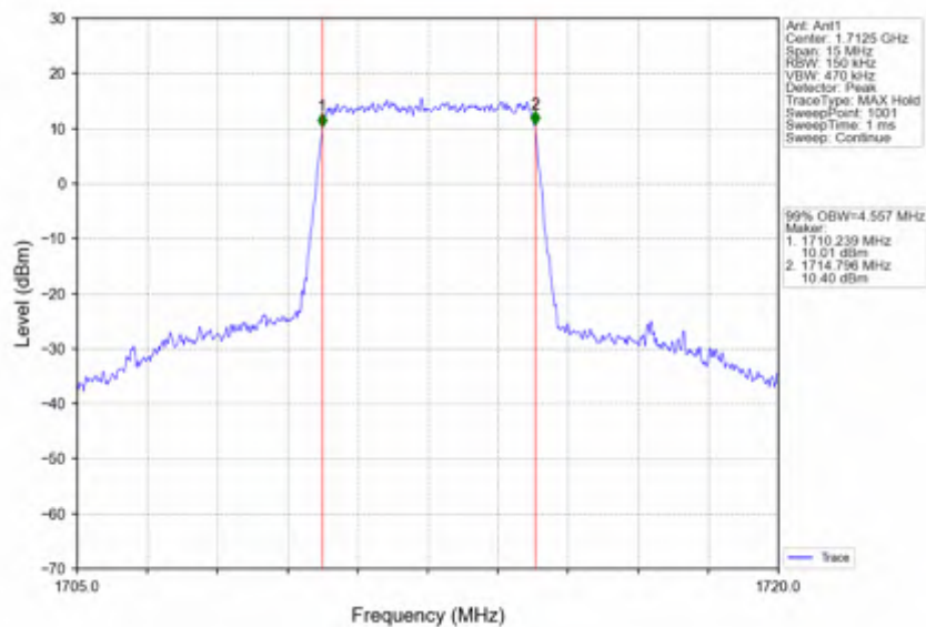
Band66 5MHz 256QAM LCH 1712.5MHz RB 25 0 NTNV
