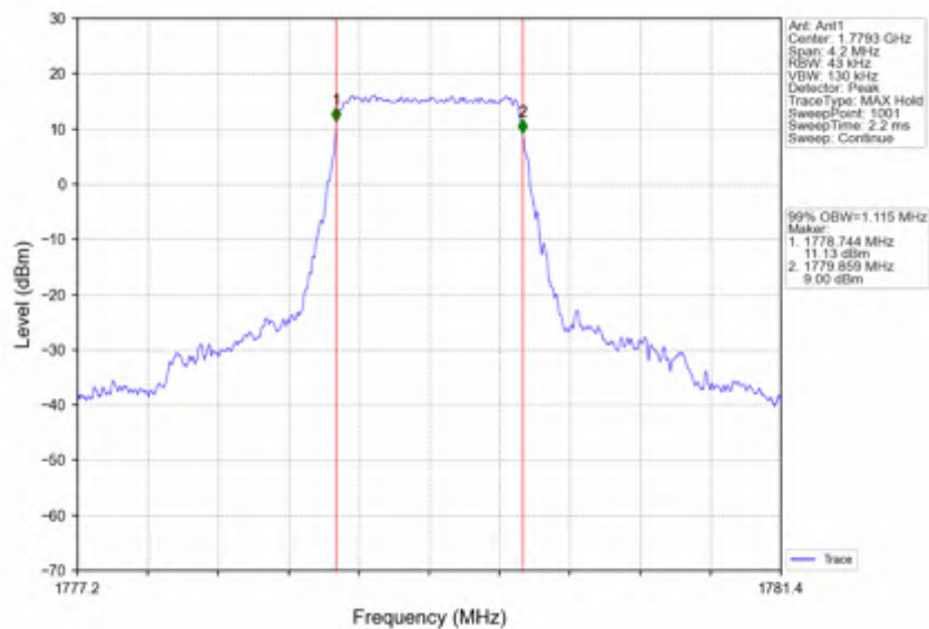
Band66 1.4MHz 256QAM HCH 1779.3MHz RB 6 0 NTNV
