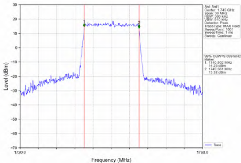
Band66_10MHz_QPSK_MCH_1745MHz_RB_50_0_NTNV
