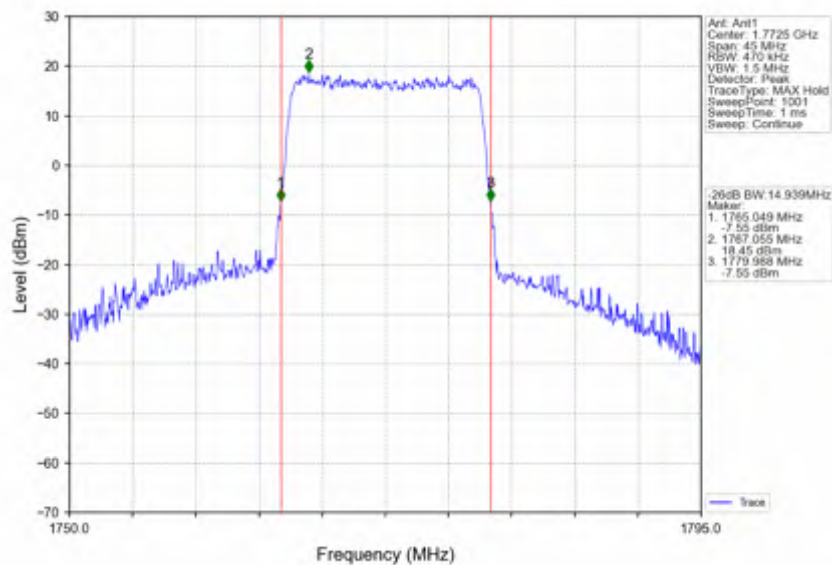
Band66_15MHz_16QAM_HCH_1772.5MHz_RB_75_0_NTNV
