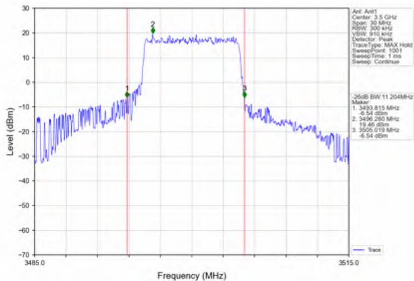
Band42a_10MHz_64QAM_MCH_3500MHz_RB_50_0_NTNV
