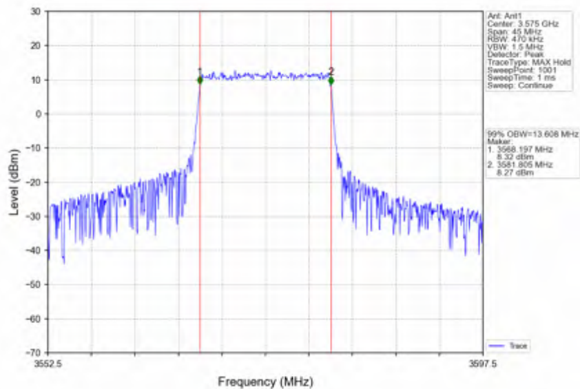
Band42c_15MHz_64QAM_MCH_3575MHz_RB_75_0_NTNV
