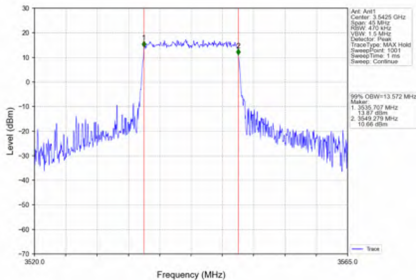
Band42a_15MHz_256QAM_HCH_3542.5MHz_RB_75_0_NTNV
