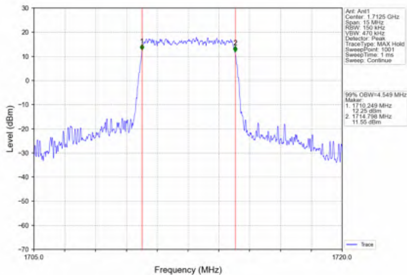
Band66_5MHz_16QAM_LCH_1712.5MHz_RB_25_0_NTNV
