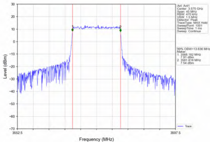
Band42c_15MHz_QPSK_MCH_3575MHz_RB_75_0_NTNV
