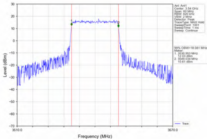
Band42a_20MHz_256QAM_HCH_3540MHz_RB_100_0_NTNV
