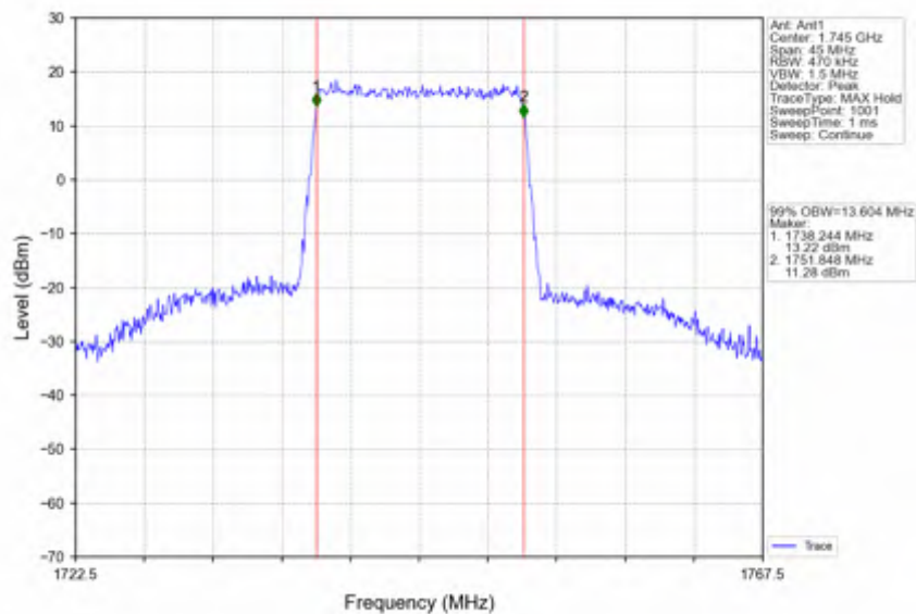
Band66_15MHz_QPSK_MCH_1745MHz_RB_75_0_NTNV
