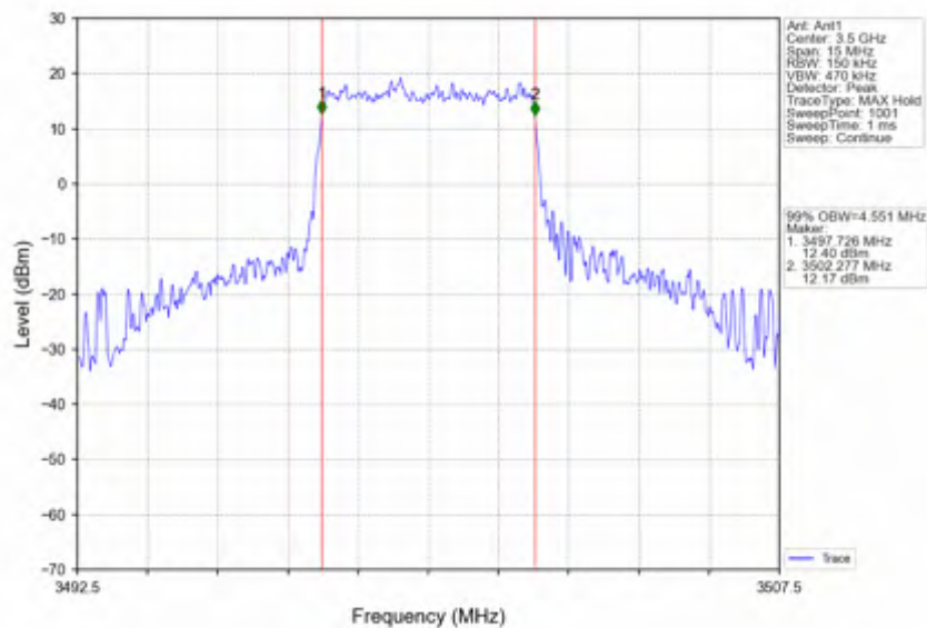
Band42a_5MHz_64QAM_MCH_3500MHz_RB_25_0_NTNV
