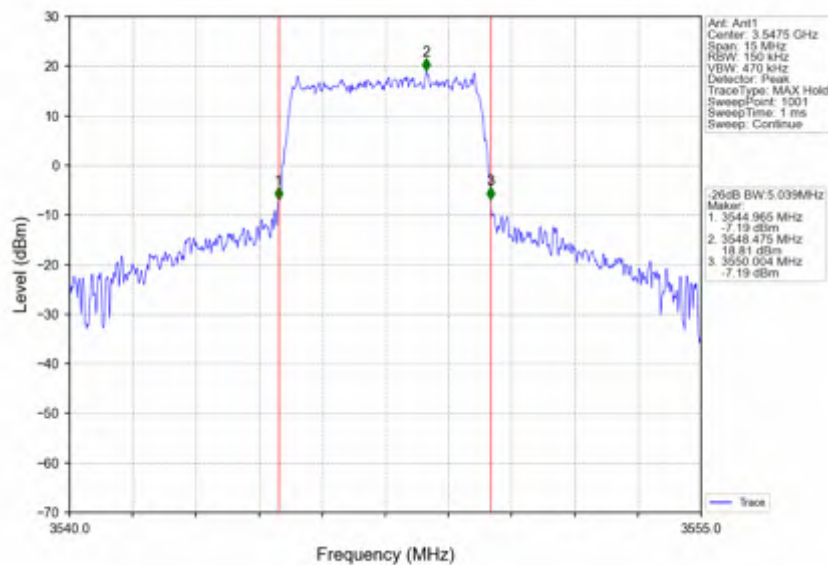
Band42a_5MHz_16QAM_HCH_3547.5MHz_RB_25_0_NTNV
