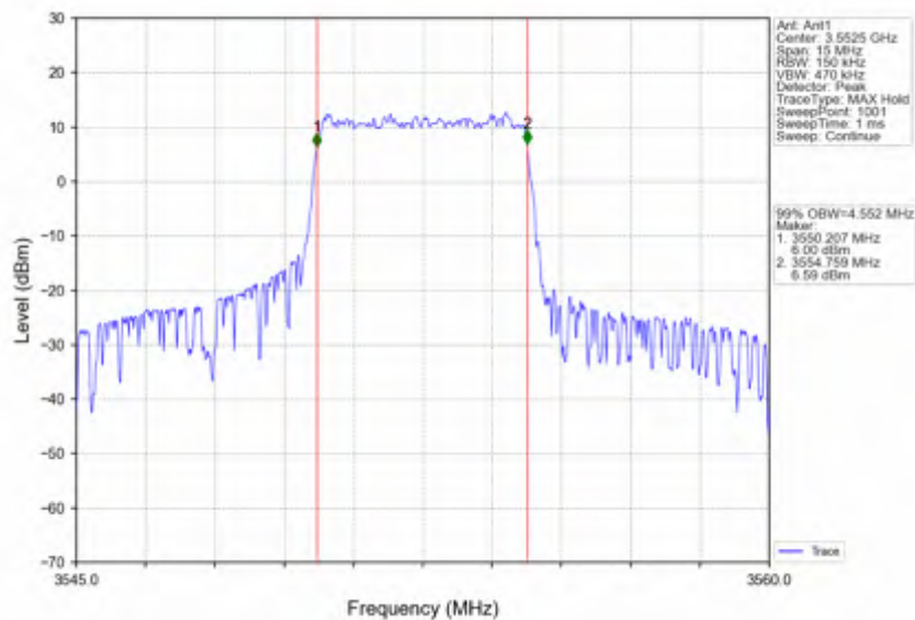
Band42c_5MHz_16QAM_LCH_3552.5MHz_RB_25_0_NTNV
