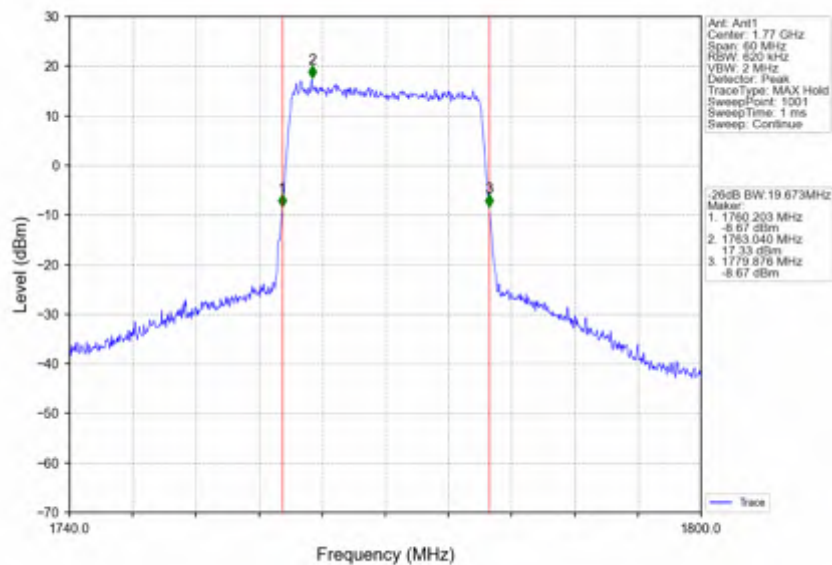
Band66_20MHz_256QAM_HCH_1770MHz_RB_100_0_NTNV
