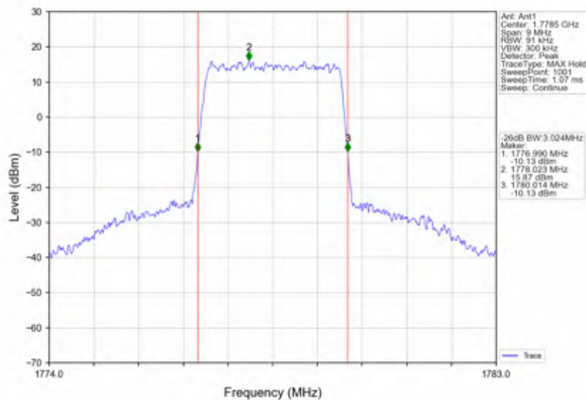
Band66_3MHz_256QAM_HCH_1778.5MHz_RB_15_0_NTNV
