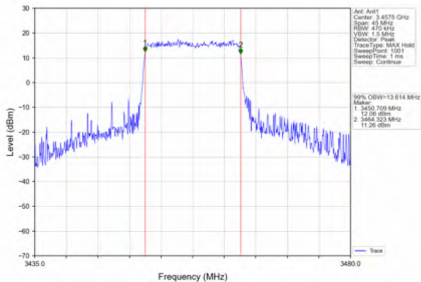
Band42a_15MHz_256QAM_LCH_3457.5MHz_RB_75_0_NTNV
