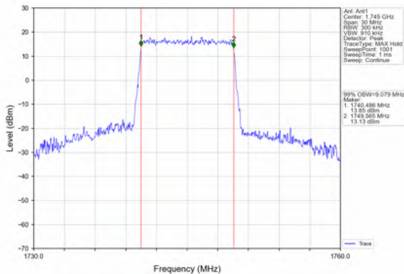
Band66_10MHz_64QAM_MCH_1745MHz_RB_50_0_NTNV
