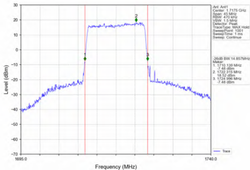
Band66_15MHz_16QAM_LCH_1717.5MHz_RB_75_0_NTNV
