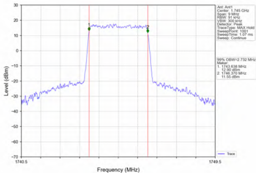
Band66 3MHz 64QAM MCH 1745MHz RB 15 0 NTN
