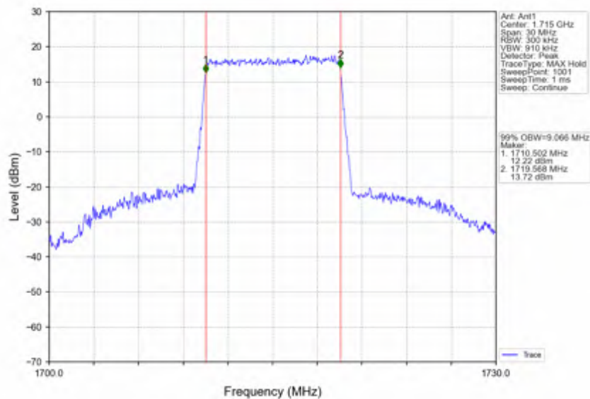
Band66_10MHz_16QAM_LCH_1715MHz_RB_50_0_NTNV
