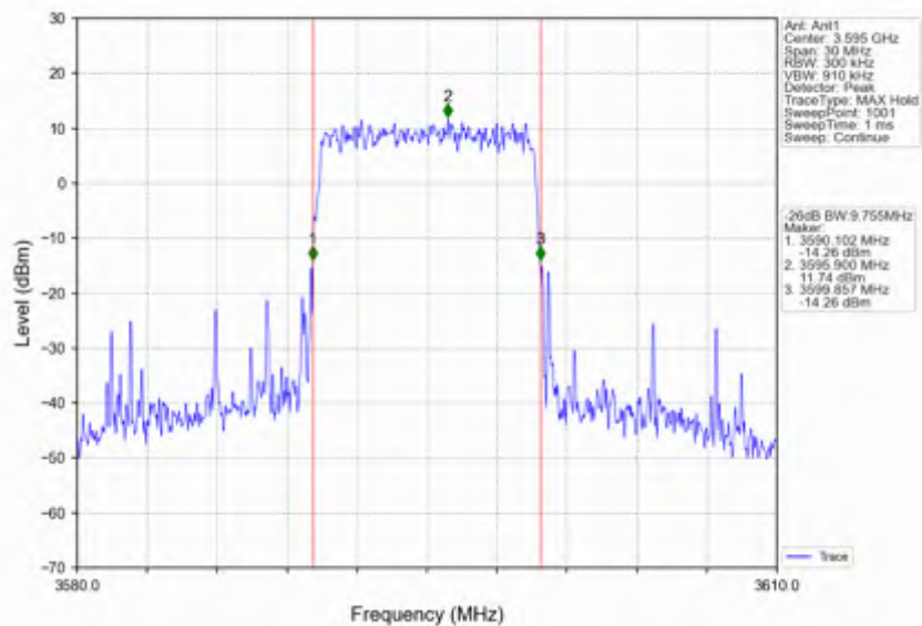
Band42c 10MHz 256QAM HCH 3595MHz RB 50 0 NTNV
