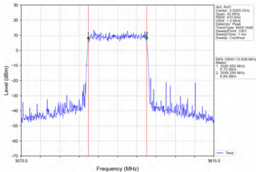
Band42c_15MHz_16QAM_HCH_3592.5MHz_RB_75_0_NTNV
