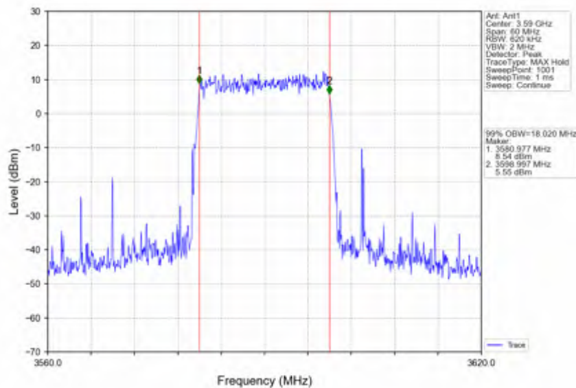
Band42c_20MHz_256QAM_HCH_3590MHz_RB_100_0_NTNV
