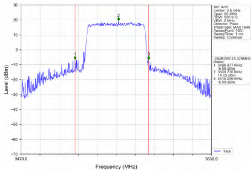
Band42a_20MHz_64QAM_MCH_3500MHz_RB_100_0_NTNV
