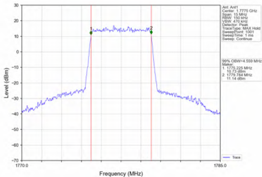
Band66_5MHz_256QAM_HCH_1777.5MHz_RB_25_0_NTNV
