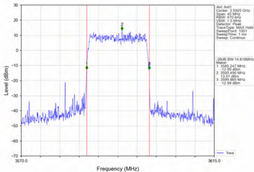
Band42c_15MHz_256QAM_HCH_3592.5MHz_RB_75_0_NTNV
