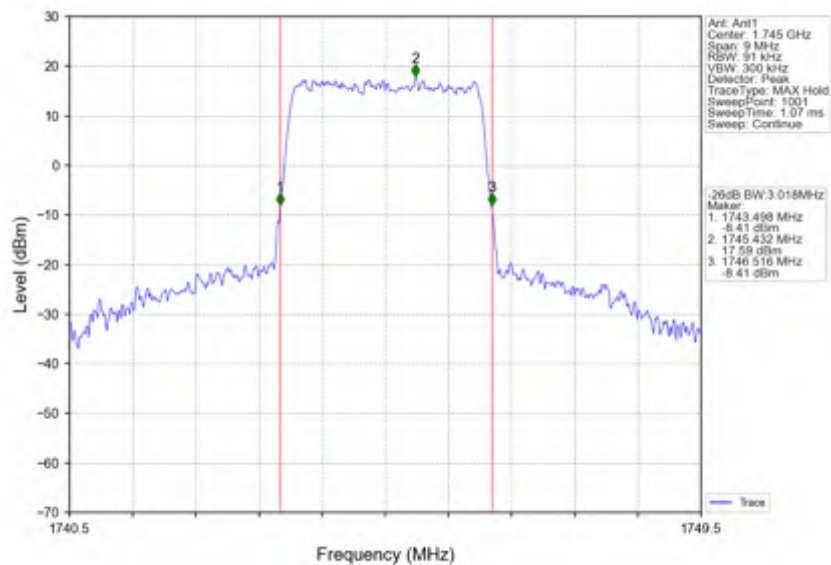
Band66_3MHz_QPSK_MCH_1745MHz_RB_15_0_NTNV
