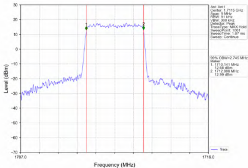
Band66_3MHz_16QAM_LCH_1711.5MHz_RB_15_0_NTNV
