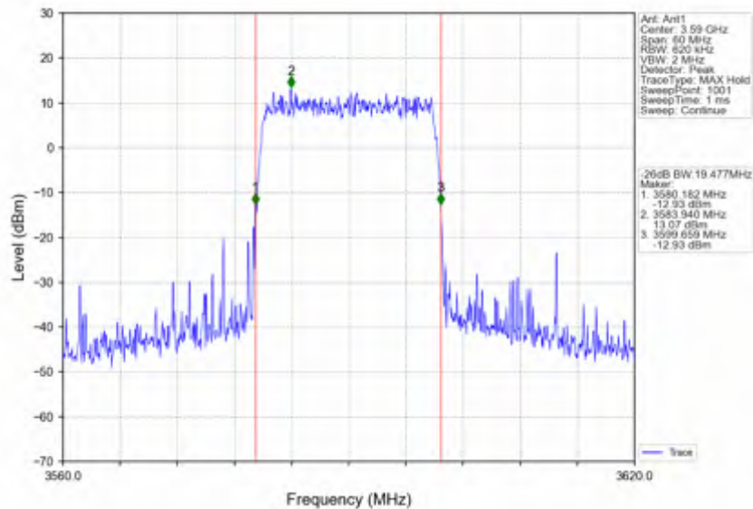
Band42c_20MHz_16QAM_HCH_3590MHz_RB_100_0_NTNV
