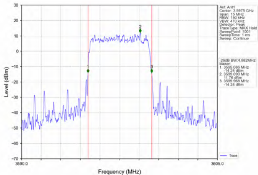
Band42c 5MHz 256QAM HCH 3597.5MHz RB 25 0 NTNV
