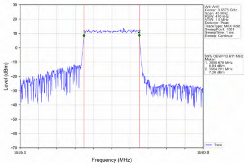
Band42c_15MHz_16QAM_LCH_3557.5MHz_RB_75_0_NTNV
