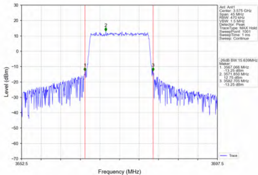
Band42c_15MHz_64QAM_MCH_3575MHz_RB_75_0_NTNV
