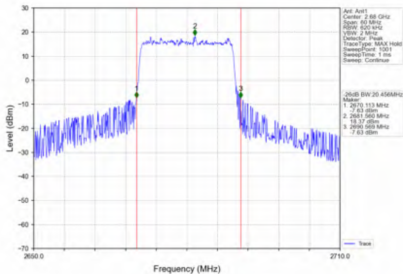
Band41_20MHz_256QAM_HCH_2680MHz_RB_100_0_NTNV
