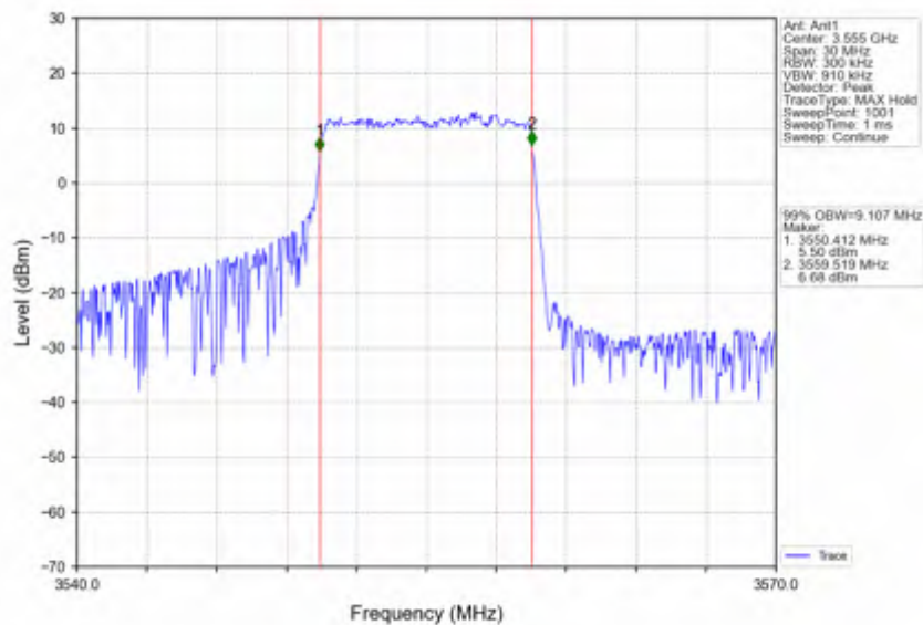
Band42c_10MHz_16QAM_LCH_3555MHz_RB_50_0_NTNV
