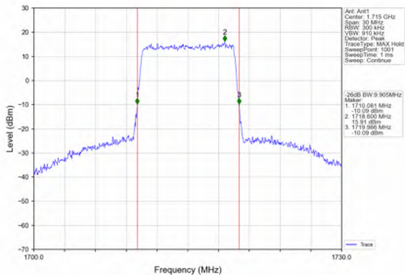
Band66_10MHz_256QAM_LCH_1715MHz_RB_50_0_NTNV
