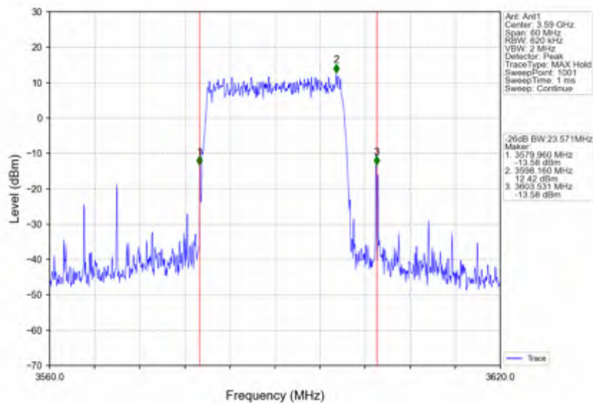
Band42c_20MHz_256QAM_HCH_3590MHz_RB_100_0_NTNV
