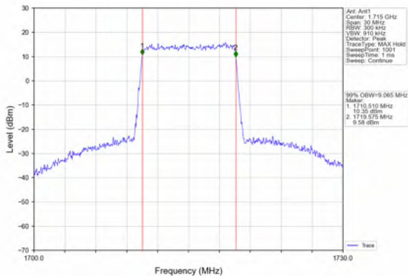
Band66_10MHz_256QAM_LCH_1715MHz_RB_50_0_NTNV
