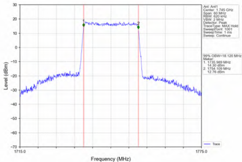
Band66_20MHz_64QAM_MCH_1745MHz_RB_100_0_NTNV
