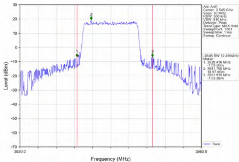
Band42a_10MHz_16QAM_HCH_3545MHz_RB_50_0_NTNV
