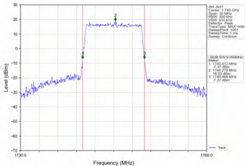
Band66_10MHz_QPSK_MCH_1745MHz_RB_50_0_NTNV
