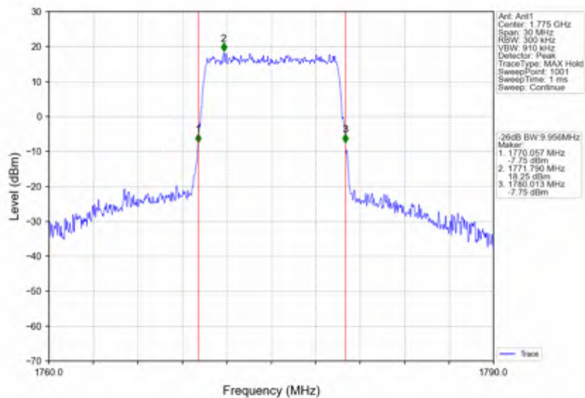
Band66_10MHz_16QAM_HCH_1775MHz_RB_50_0_NTNV
