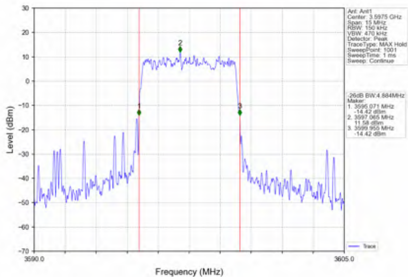
Band42c_5MHz_16QAM_HCH_3597.5MHz_RB_25_0_NTNV
