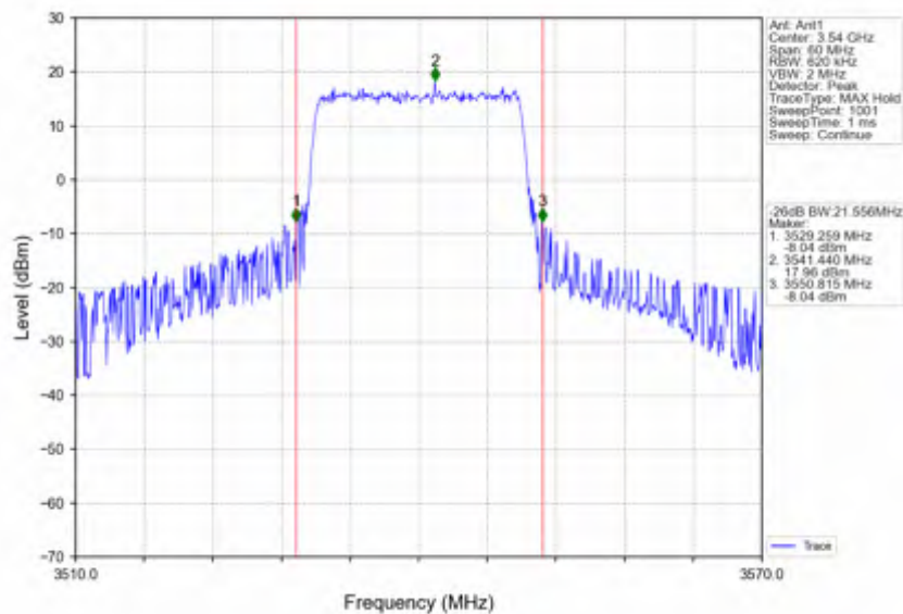
Band42a_20MHz_256QAM_HCH_3540MHz_RB_100_0_NTNV
