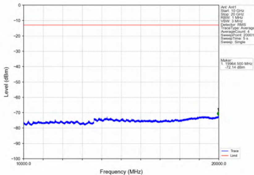
Band4_15MHz_256QAM_MCH_1732.5MHz_RB_1_0_NTNV
