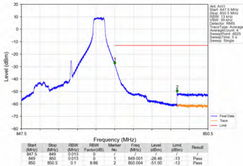
Band5_1.4MHz_256QAM_HCH_848.3MHz_RB_1_5_NTNV
