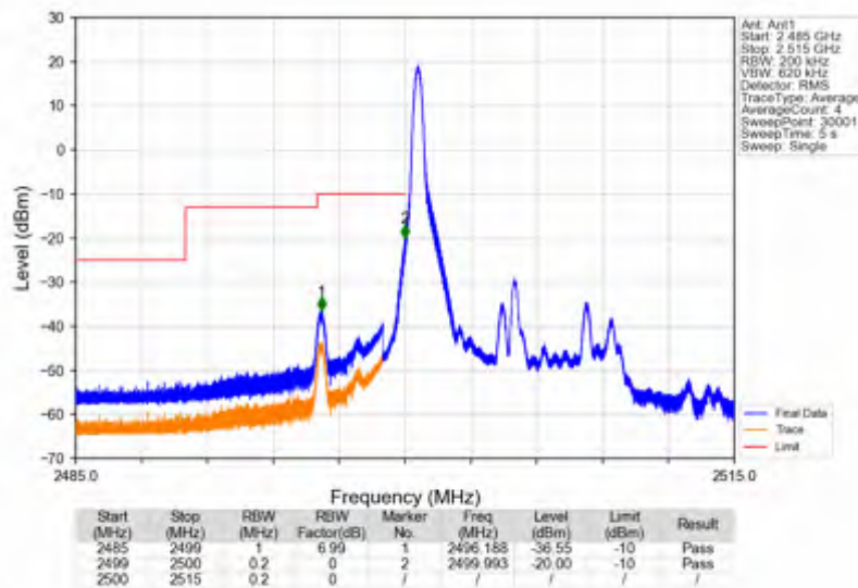
Band7_10MHz_256QAM_LCH_2505MHz_RB_50_0_NTNV
