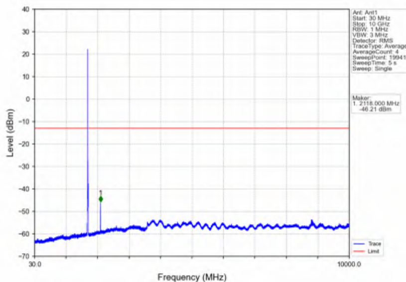
Band4_10MHz_QPSK_LCH_1715MHz_RB_1_0_NTNV
