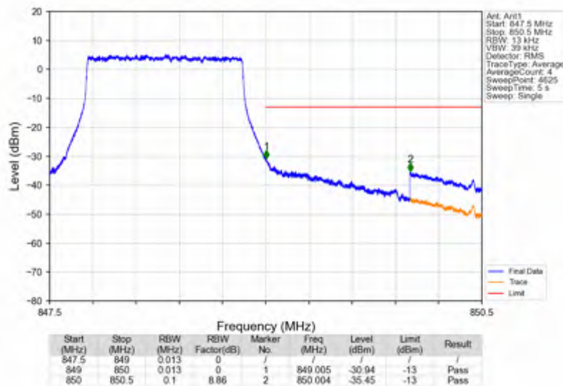
Band5_1.4MHz_16QAM_HCH_848.3MHz_RB_6_0_NTNV
