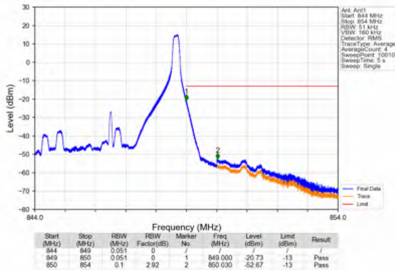
Band5_5MHz_256QAM_HCH_846.5MHz_RB_25_0_NTNV
