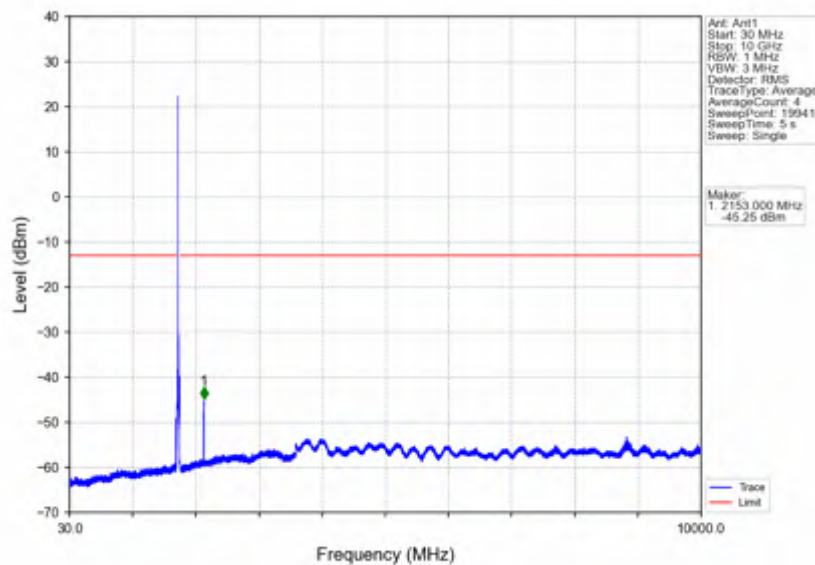
Band4_15MHz_64QAM_HCH_1747.5MHz_RB_1_0_NTNV
