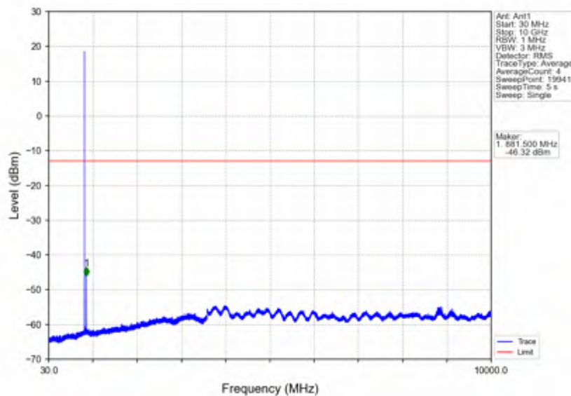
Band5_3MHz_256QAM_HCH_847.5MHz_RB_1_0_NTNV
