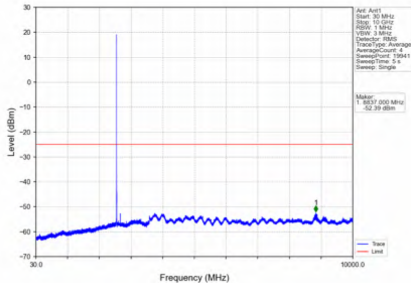
Band7_5MHz_256QAM_HCH_2567.5MHz_RB_1_0_NTNV
