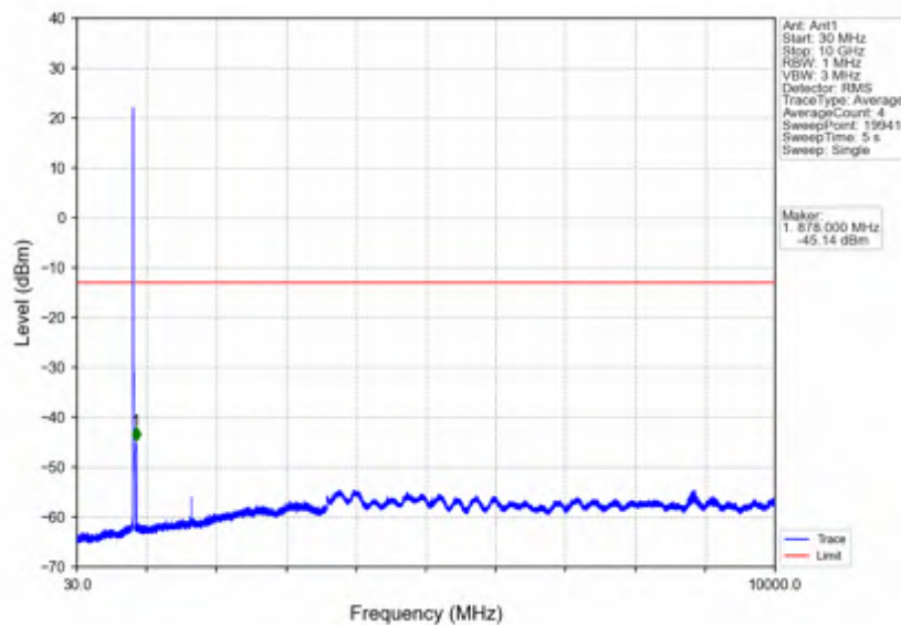
Band5_10MHz_QPSK_MCH_836.5MHz_RB_1_0_NTNV
