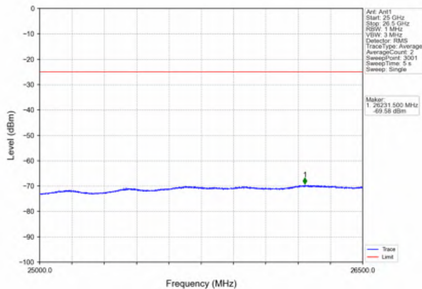
Band7_10MHz_256QAM_LCH_2505MHz_RB_50_0_NTNV
