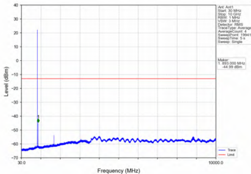
Band5_1.4MHz_64QAM_HCH_848.3MHz_RB_1_5_NTNV
