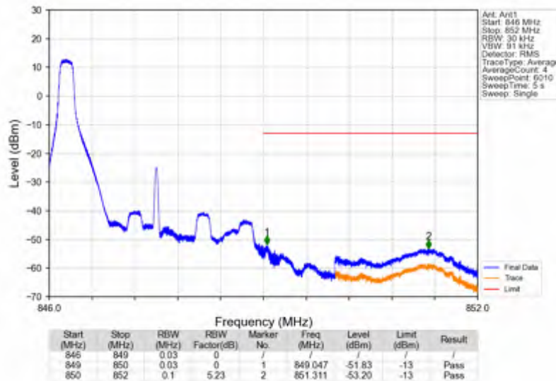
Band5_3MHz_256QAM_HCH_847.5MHz_RB_1_14_NTNV
