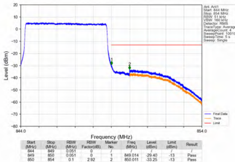
Band5_5MHz_16QAM_HCH_846.5MHz_RB_25_0_NTNV
