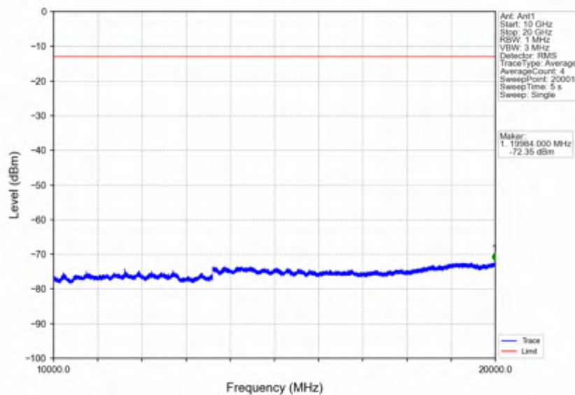
Band4_10MHz_16QAM_MCH_1732.5MHz_RB_1_0_NTNV
