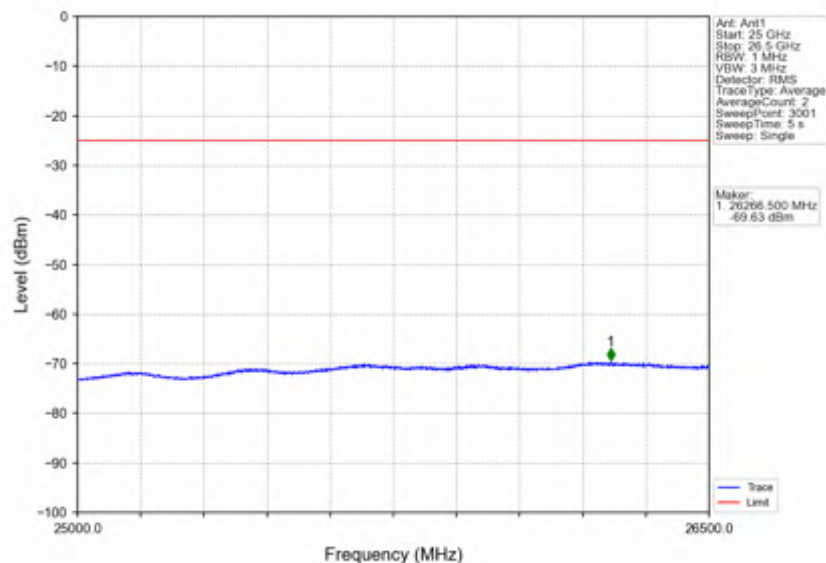
Band7_5MHz_256QAM_LCH_2502.5MHz_RB_25_0_NTNV
