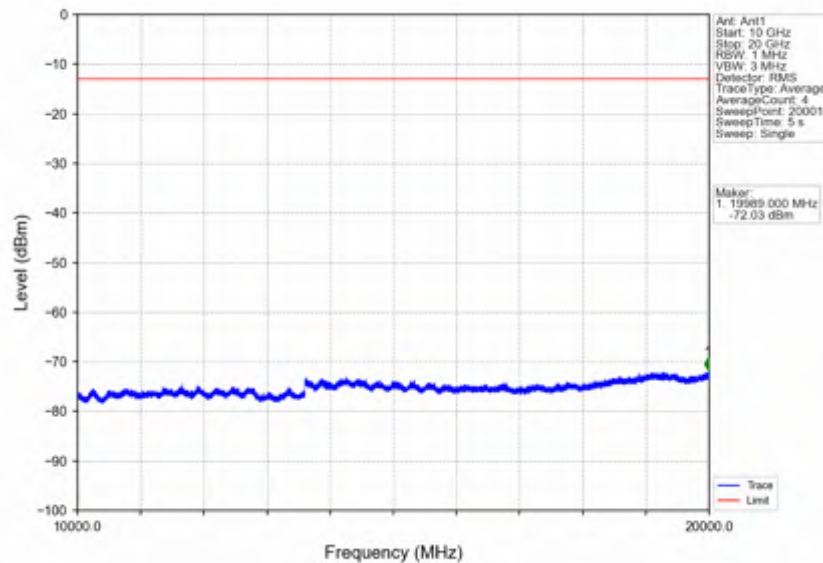
Band4_20MHz_64QAM_LCH_1720MHz_RB_100_0_NTNV
