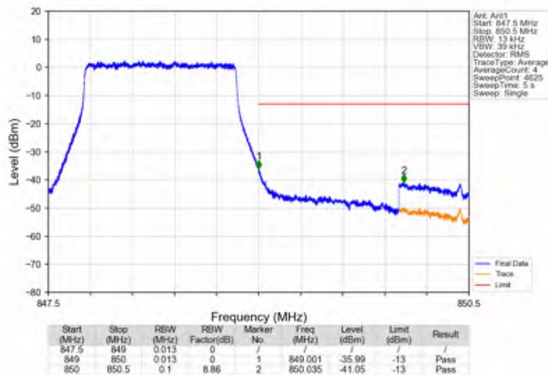
Band5_1.4MHz_256QAM_HCH_848.3MHz_RB_6_0_NTNV
