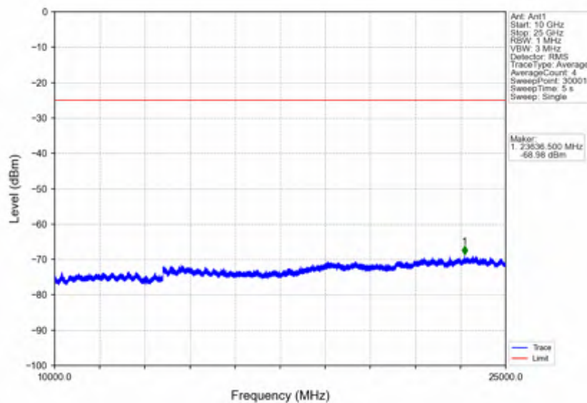
Band7_10MHz_64QAM_HCH_2565MHz_RB_1_0_NTNV
