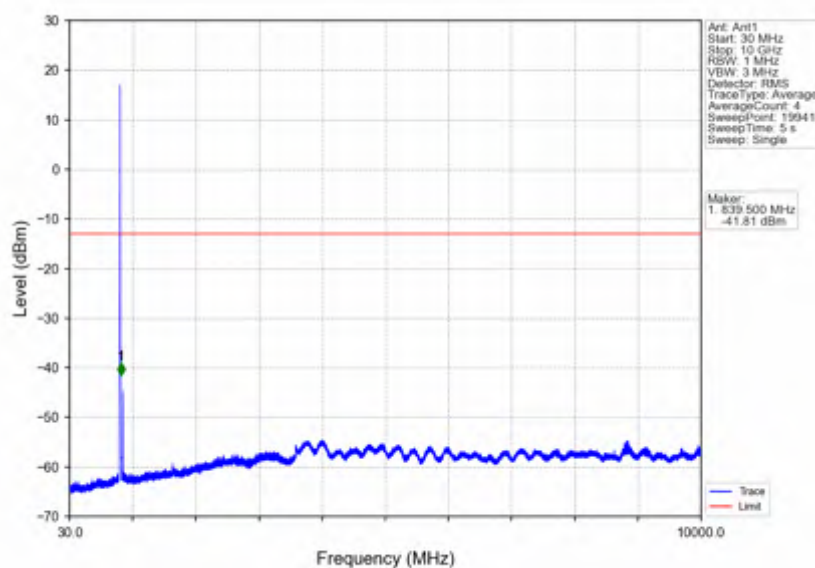
Band5_5MHz_QPSK_LCH_826.5MHz_RB_1_0_NTNV
