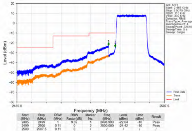
Band7_5MHz_64QAM_LCH_2502.5MHz_RB_1_0_NTNV
