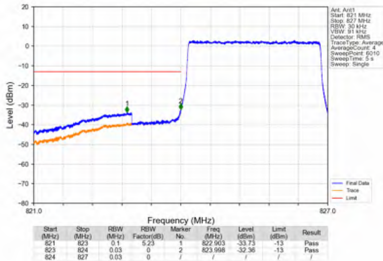
Band5_3MHz_64QAM_LCH_825.5MHz_RB_15_0_NTNV
