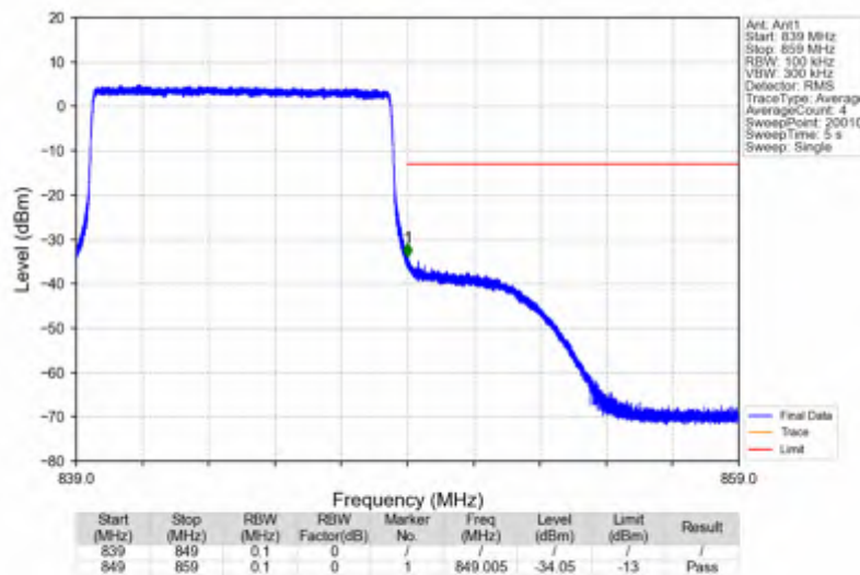
Band5_10MHz_16QAM_HCH_844MHz_RB_50_0_NTNV
