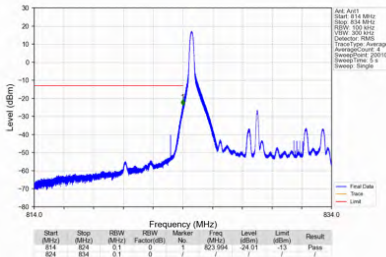
Band5_10MHz_256QAM_LCH_829MHz_RB_1_0_NTNV
