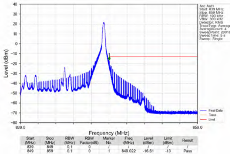
Band5_10MHz_16QAM_HCH_844MHz_RB_1_49_NTNV
