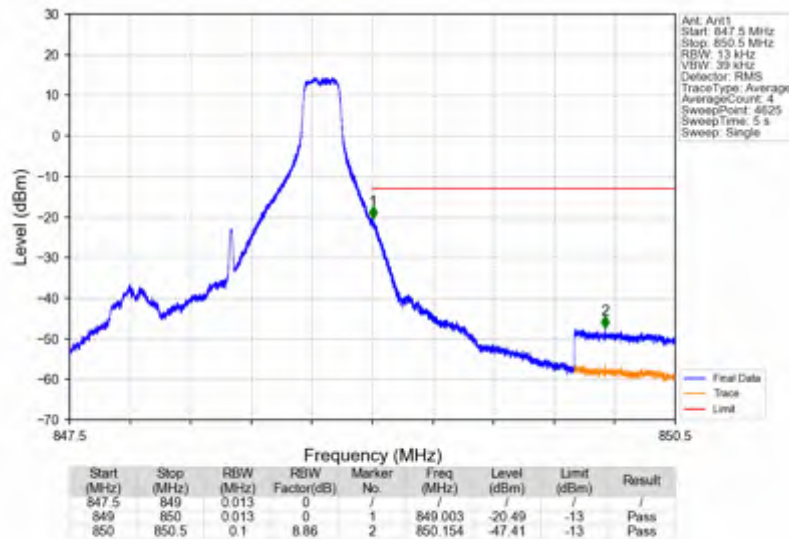
Band5_1.4MHz_QPSK_HCH_848.3MHz_RB_1_5_NTNV
