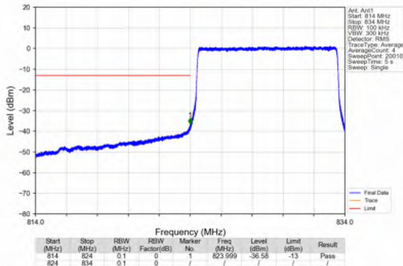
Band5_10MHz_256QAM_LCH_829MHz_RB_50_0_NTNV
