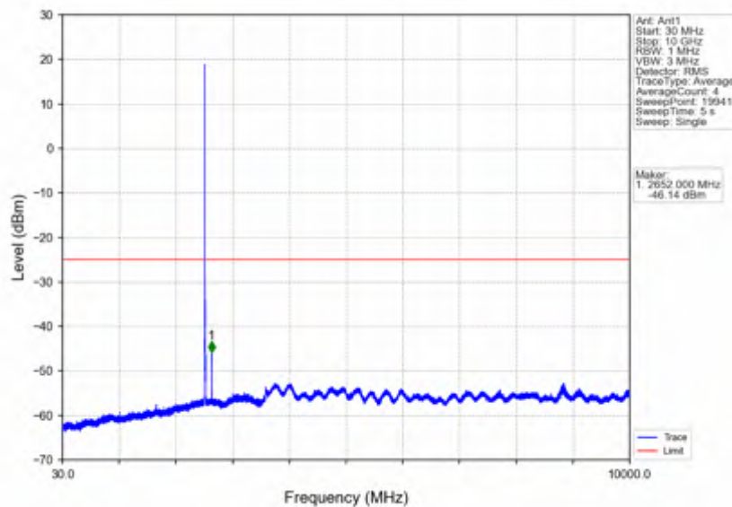
Band7_10MHz_256QAM_MCH_2535MHz_RB_1_0_NTNV
