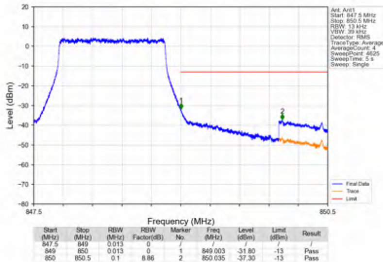
Band5_1.4MHz_64QAM_HCH_848.3MHz_RB_6_0_NTNV
