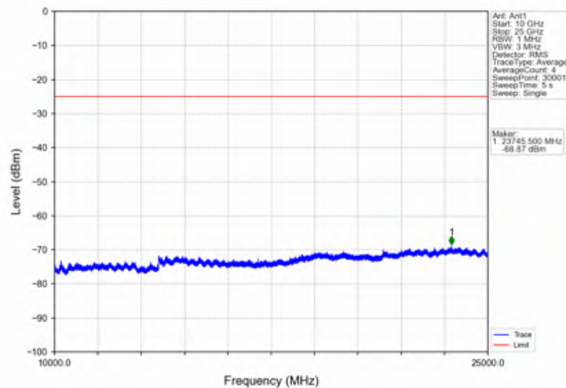
Band7_10MHz_16QAM_HCH_2565MHz_RB_1_0_NTNV
