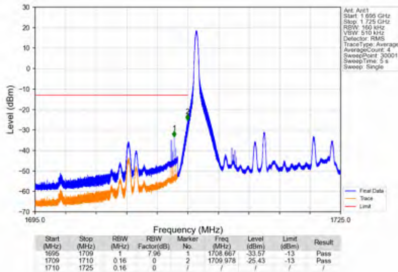
Band4_15MHz_256QAM_LCH_1717.5MHz_RB_1_0_NTNV
