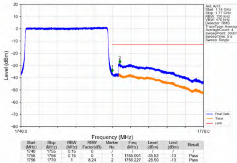
Band4_15MHz_256QAM_HCH_1747.5MHz_RB_75_0_NTNV
