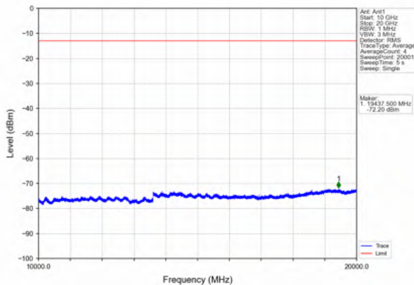
Band4_20MHz_16QAM_HCH_1745MHz_RB_1_0_NTNV
