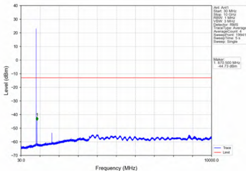
Band5_3MHz_QPSK_LCH_825.5MHz_RB_1_0_NTNV
