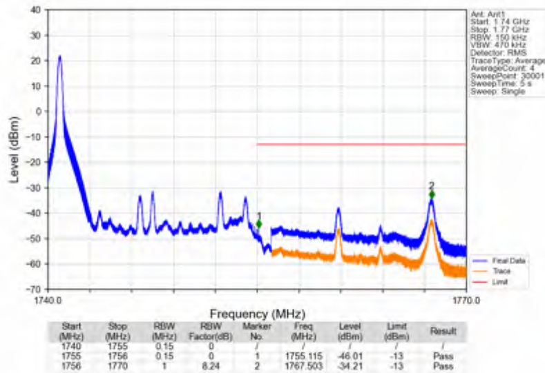
Band4_15MHz_16QAM_HCH_1747.5MHz_RB_75_0_NTNV
