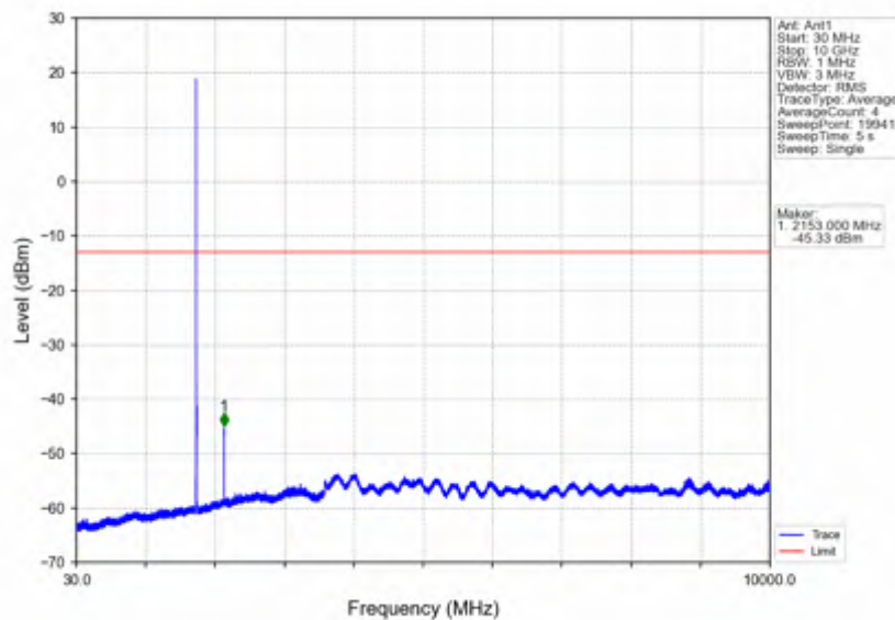
Band4_5MHz_256QAM_HCH_1752.5MHz_RB_1_0_NTNV
