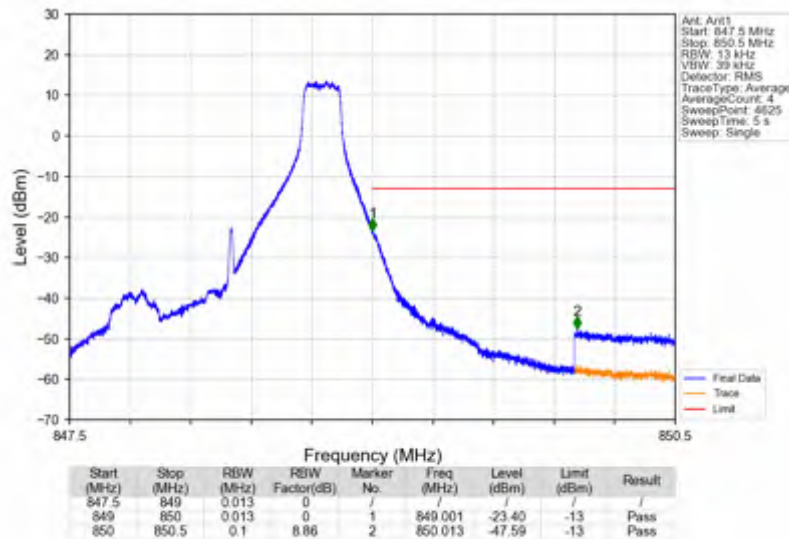
Band5_1.4MHz_16QAM_HCH_848.3MHz_RB_1_5_NTNV
