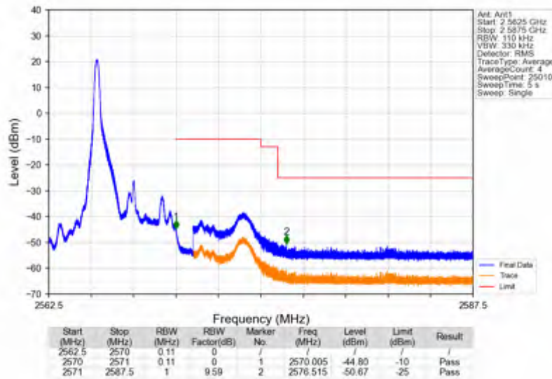
Band7_5MHz_16QAM_HCH_2567.5MHz_RB_1_24_NTNV
