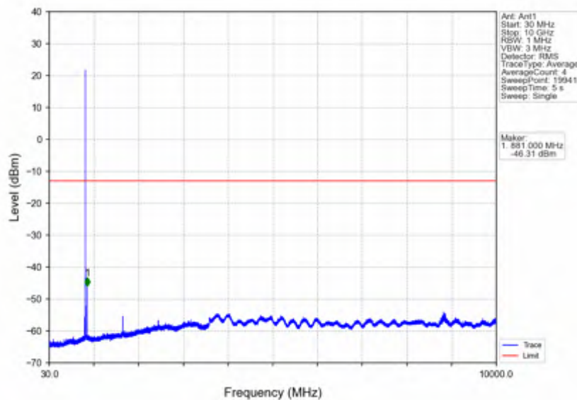
Band5_3MHz_64QAM_MCH_836.5MHz_RB_1_0_NTNV
