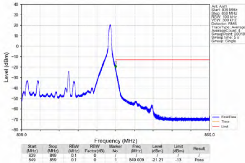
Band5_10MHz_64QAM_HCH_844MHz_RB_1_49_NTNV
