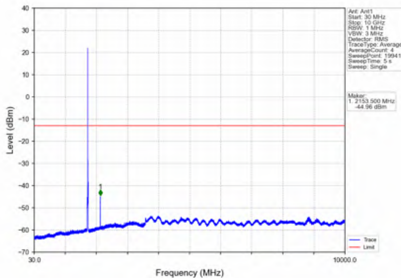
Band4_10MHz_16QAM_HCH_1750MHz_RB_1_0_NTNV
