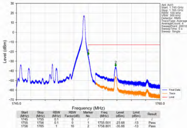
Band4_10MHz_256QAM_HCH_1750MHz_RB_1_49_NTNV
