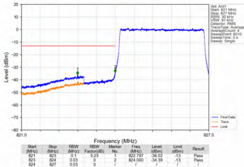
Band5_3MHz_256QAM_LCH_825.5MHz_RB_15_0_NTNV
