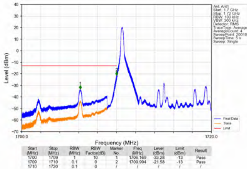
Band4_10MHz_QPSK_LCH_1715MHz_RB_50_0_NTNV
