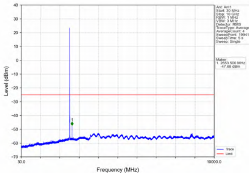
Band7_5MHz_16QAM_MCH_2535MHz_RB_1_0_NTNV
