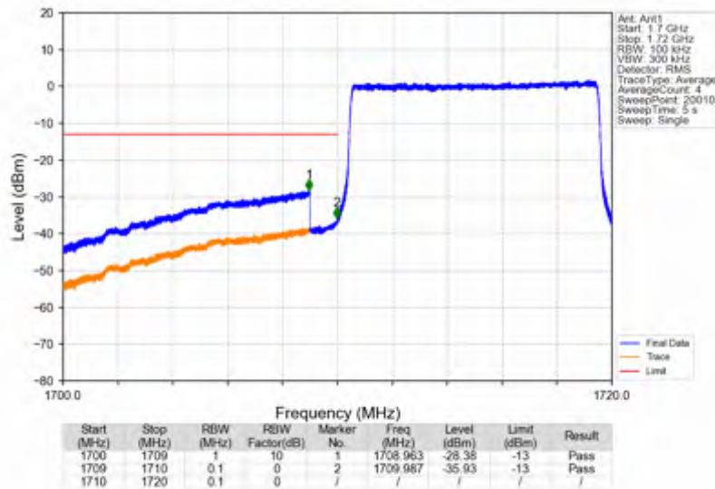
Band4_10MHz_256QAM_LCH_1715MHz_RB_50_0_NTNV
