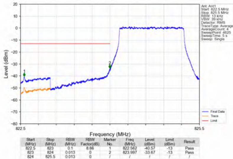
Band5_1.4MHz_256QAM_LCH_824.7MHz_RB_6_0_NTNV
