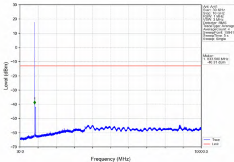
Band5_5MHz_64QAM_HCH_846.5MHz_RB_1_24_NTNV
