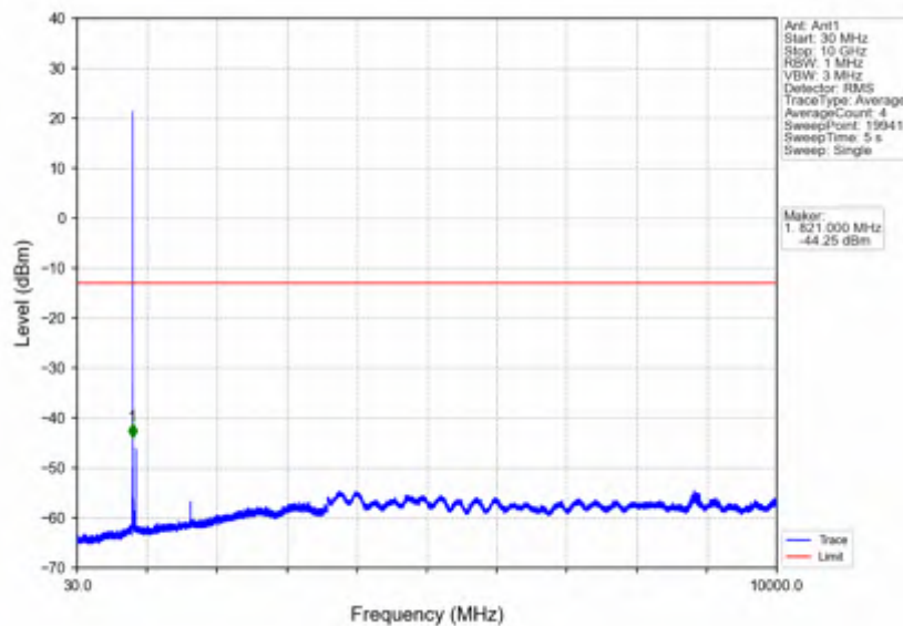
Band5 1.4MHz 64QAM LCH 824.7MHz RB 1 0 NTNV
