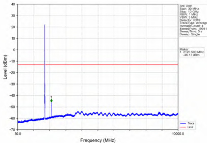
Band4_15MHz_64QAM_LCH_1717.5MHz_RB_1_0_NTNV
