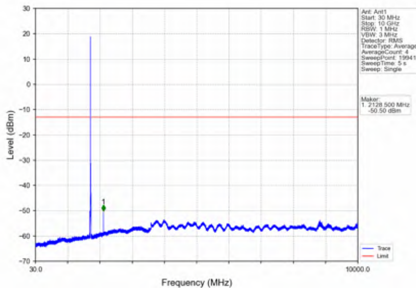
Band4_10MHz_256QAM_MCH_1732.5MHz_RB_1_0_NTNV
