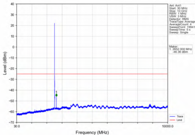
Band7_10MHz_64QAM_MCH_2535MHz_RB_1_0_NTNV
