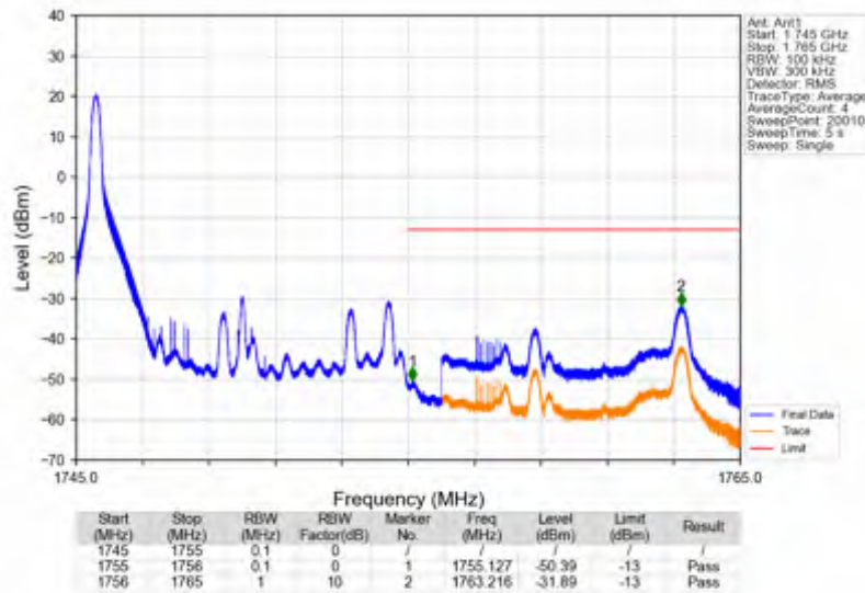
Band4_10MHz_64QAM_HCH_1750MHz_RB_50_0_NTNV
