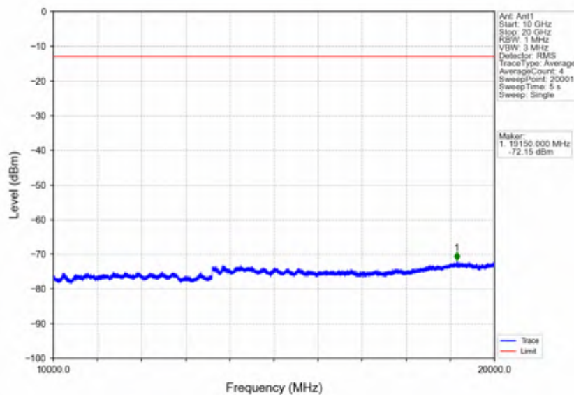
Band4_10MHz_256QAM_HCH_1750MHz_RB_1_0_NTNV
