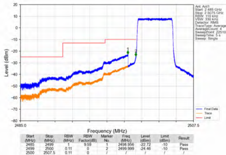
Band7_5MHz_16QAM_LCH_2502.5MHz_RB_25_0_NTNV
