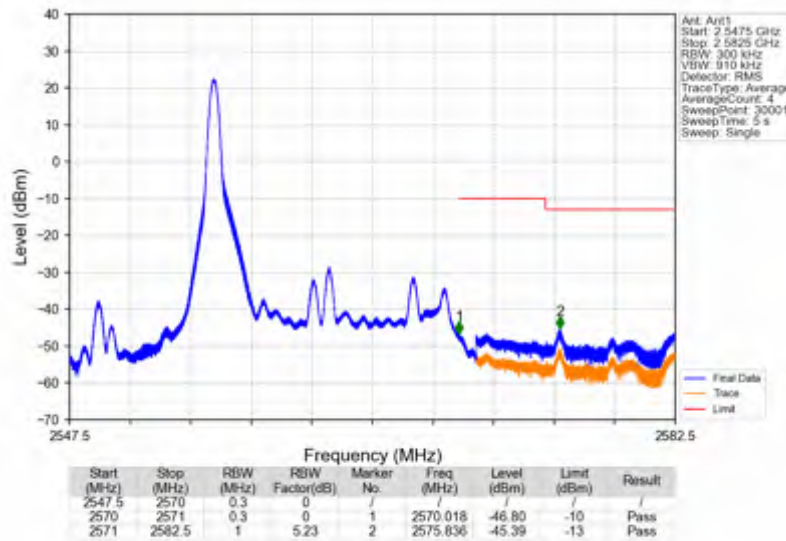
Band7_15MHz_QPSK_HCH_2562.5MHz_RB_75_0_NTNV
