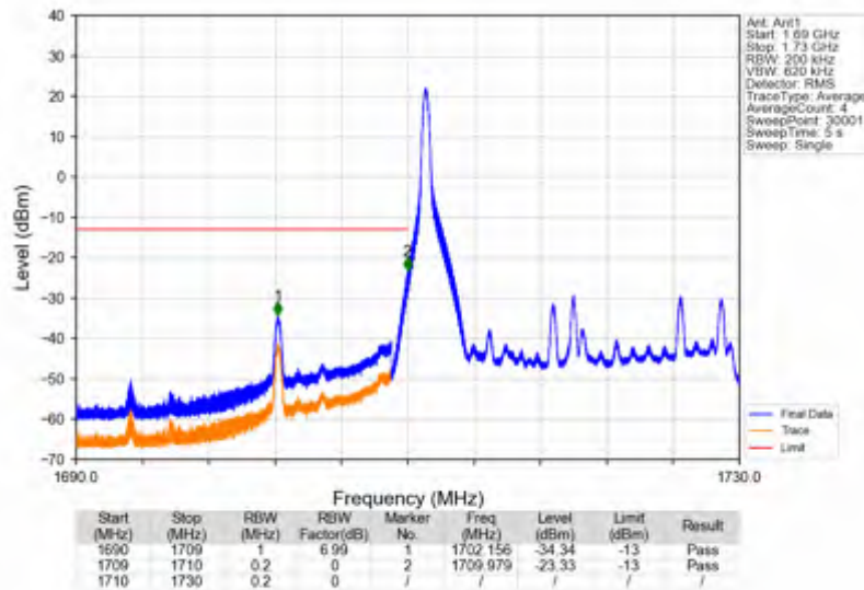
Band4_20MHz_64QAM_LCH_1720MHz_RB_1_0_NTNV
