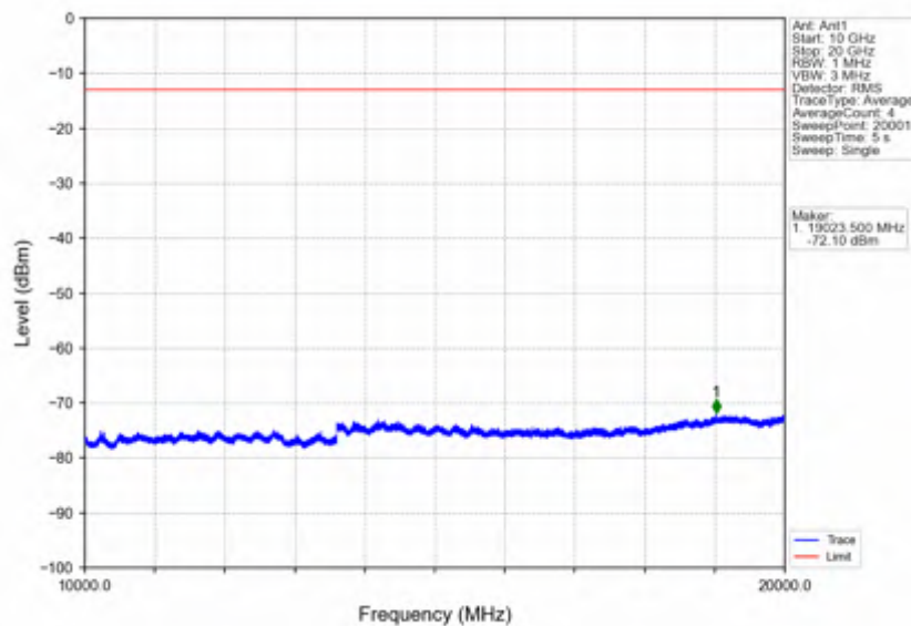
Band4_15MHz_64QAM_HCH_1747.5MHz_RB_1_0_NTNV
