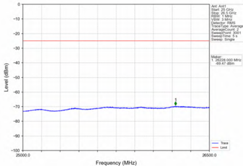
Band7_15MHz_QPSK_LCH_2507.5MHz_RB_1_0_NTNV
