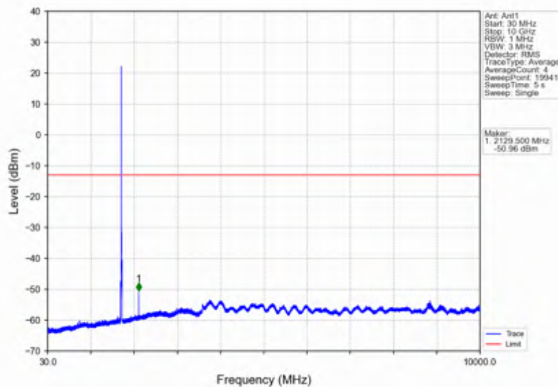
Band4_10MHz_QPSK_MCH_1732.5MHz_RB_1_0_NTNV
