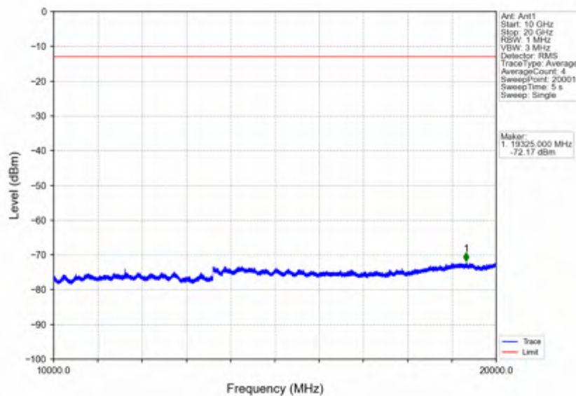
Band4_10MHz_256QAM_MCH_1732.5MHz_RB_1_0_NTNV
