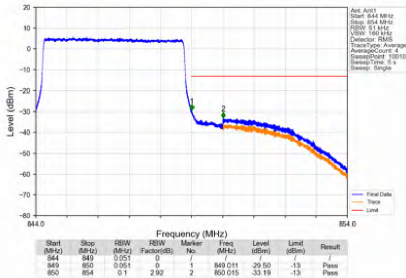
Band5_5MHz_64QAM_HCH_846.5MHz_RB_25_0_NTNV
