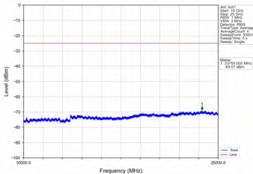
Band7_10MHz_256QAM_LCH_2505MHz_RB_1_0_NTNV
