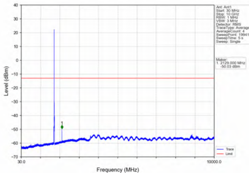
Band4_10MHz_64QAM_MCH_1732.5MHz_RB_1_0_NTNV
