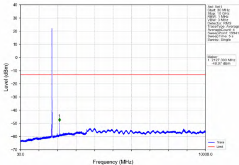
Band4_15MHz_QPSK_MCH_1732.5MHz_RB_1_0_NTNV
