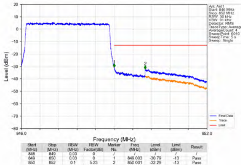
Band5_3MHz_16QAM_HCH_847.5MHz_RB_1_14_NTNV
