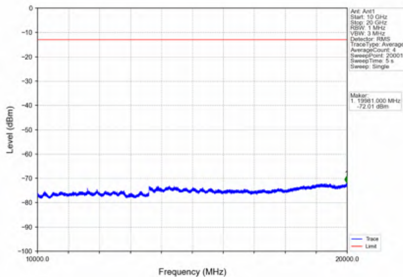
Band4_20MHz_256QAM_HCH_1745MHz_RB_1_0_NTNV
