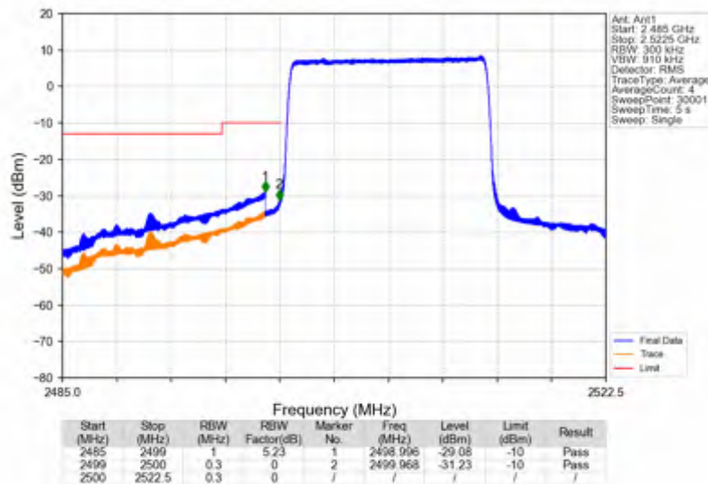
Band7_15MHz_QPSK_LCH_2507.5MHz_RB_1_0_NTNV
