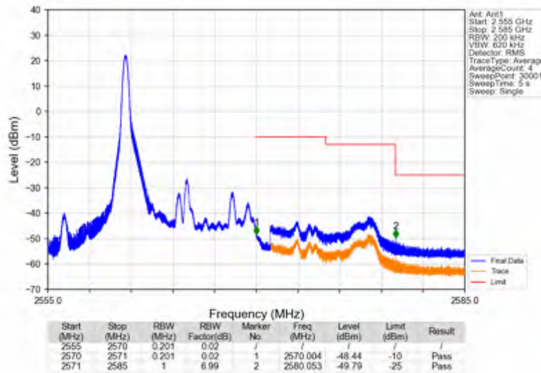
Band7_10MHz_64QAM_HCH_2565MHz_RB_1_49_NTNV
