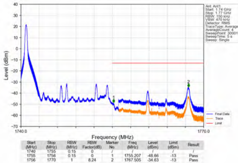
Band4_15MHz_QPSK_HCH_1747.5MHz_RB_75_0_NTNV
