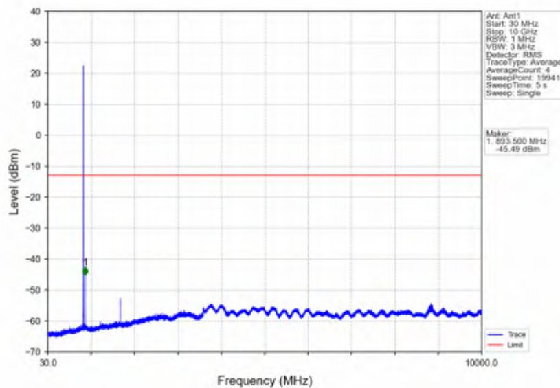
Band5_1.4MHz_16QAM_HCH_848.3MHz_RB_1_0_NTNV
