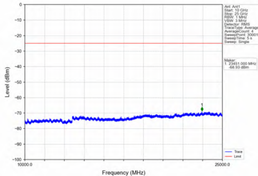
Band7_15MHz_QPSK_MCH_2535MHz_RB_1_0_NTNV
