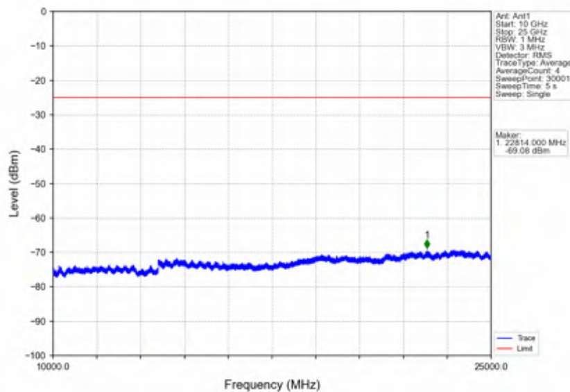
Band7_10MHz_16QAM_MCH_2535MHz_RB_1_0_NTNV
