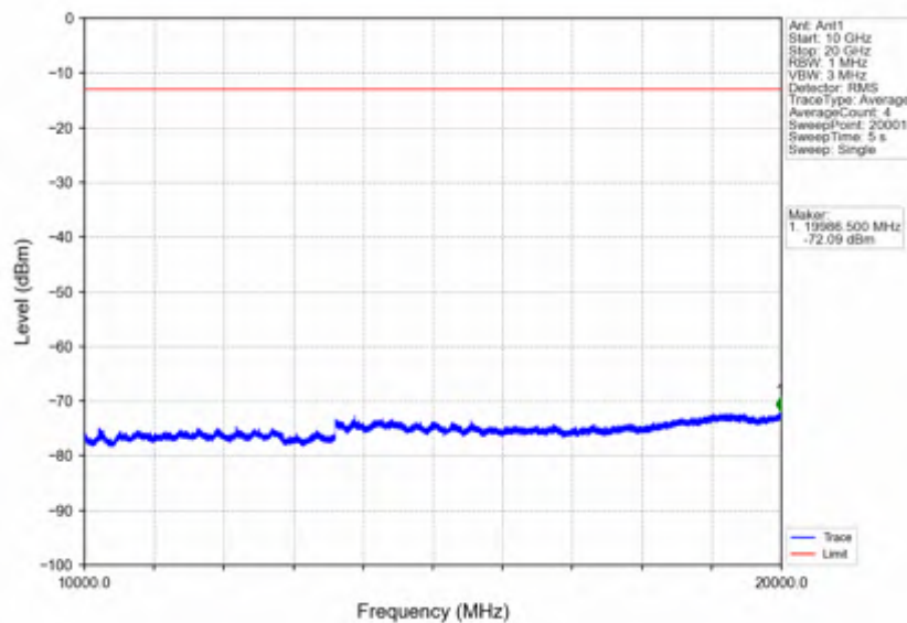
Band4_20MHz_16QAM_MCH_1732.5MHz_RB_1_0_NTNV
