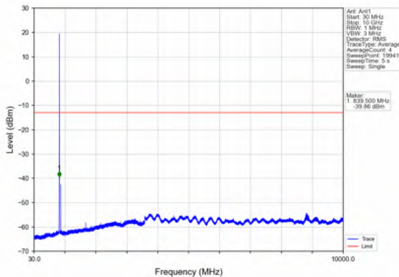
Band5_3MHz_64QAM_HCH_847.5MHz_RB_1_14_NTNV
