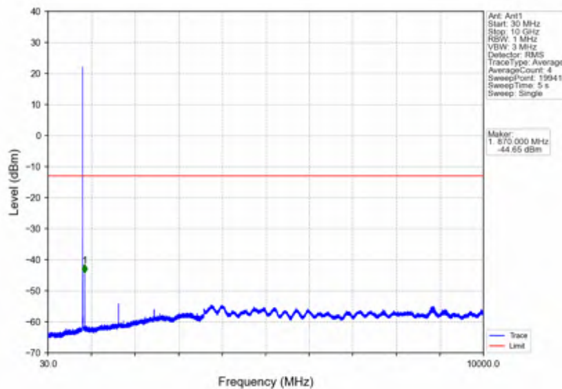
Band5_3MHz_16QAM_LCH_825.5MHz_RB_15_0_NTNV
