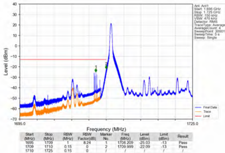
Band4_15MHz_16QAM_LCH_1717.5MHz_RB_75_0_NTNV
