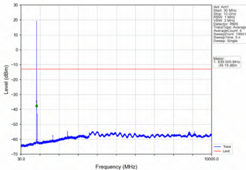
Band5_3MHz_16QAM_HCH_847.5MHz_RB_1_0_NTNV
