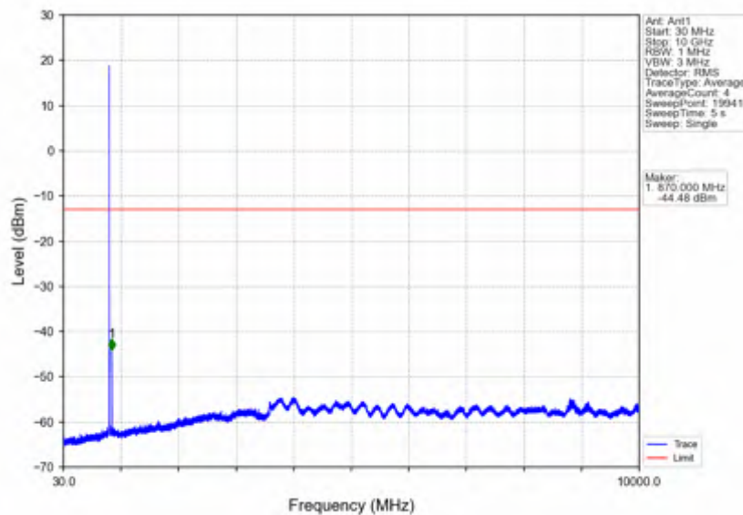
Band5_5MHz_256QAM_LCH_826.5MHz_RB_25_0_NTNV
