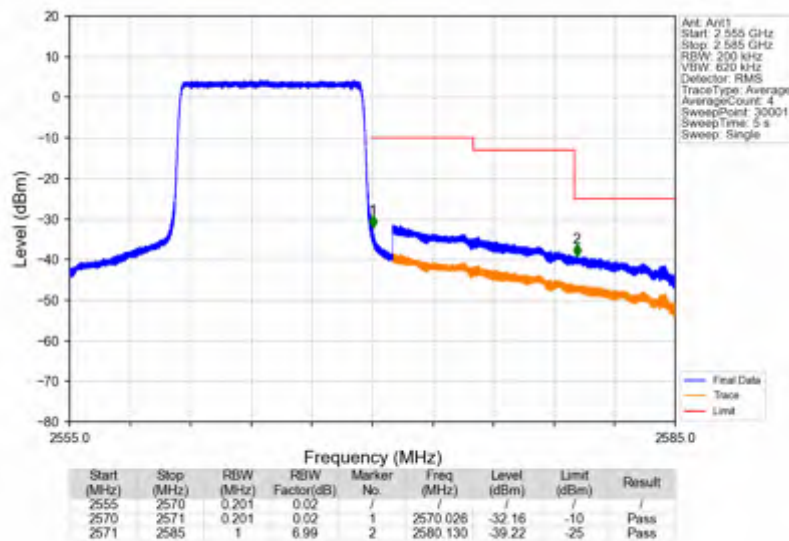
Band7_10MHz_256QAM_HCH_2565MHz_RB_50_0_NTNV
