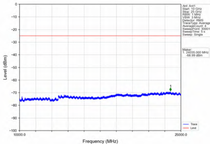
Band7_10MHz_256QAM_MCH_2535MHz_RB_1_0_NTNV
