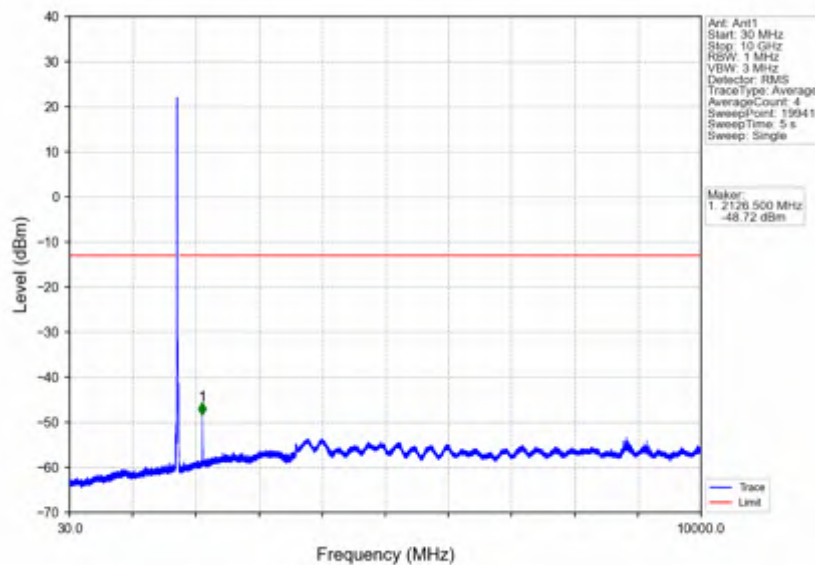
Band4_15MHz_64QAM_MCH_1732.5MHz_RB_1_0_NTNV
