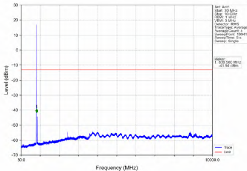
Band5_5MHz_16QAM_LCH_826.5MHz_RB_25_0_NTNV
