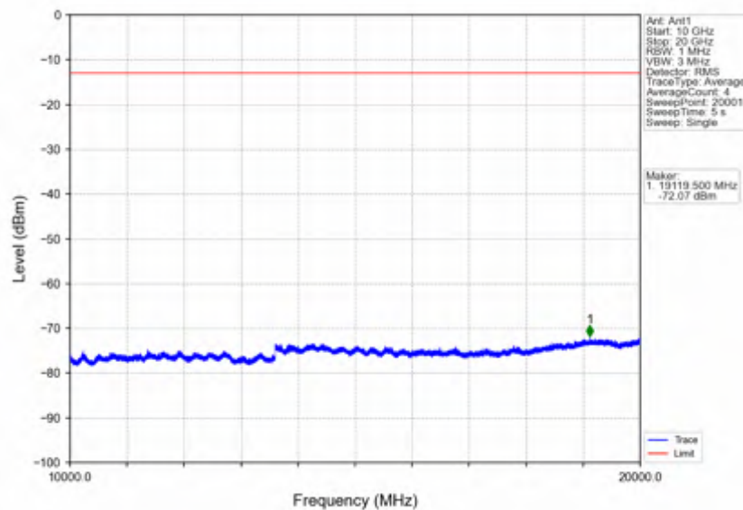
Band4_10MHz_256QAM_LCH_1715MHz_RB_50_0_NTNV
