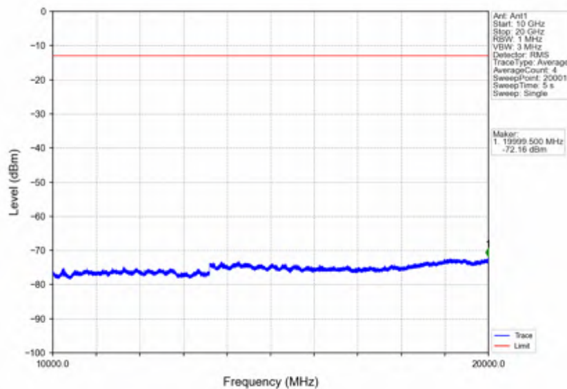
Band4_10MHz_64QAM_MCH_1732.5MHz_RB_1_0_NTNV
