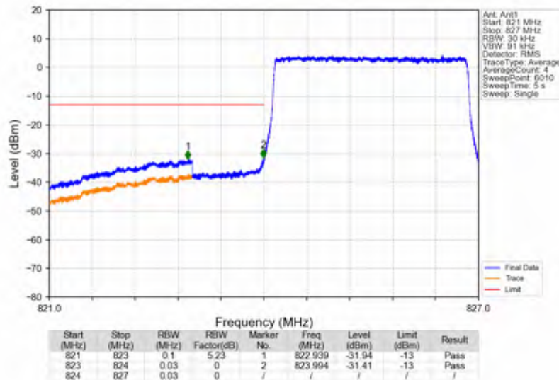
Band5_3MHz_16QAM_LCH_825.5MHz_RB_15_0_NTNV
