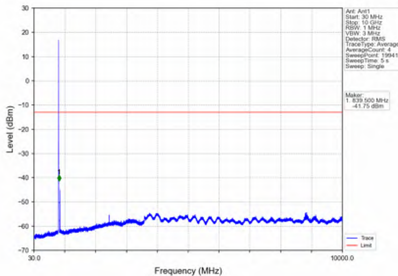
Band5_5MHz_64QAM_LCH_826.5MHz_RB_1_0_NTNV
