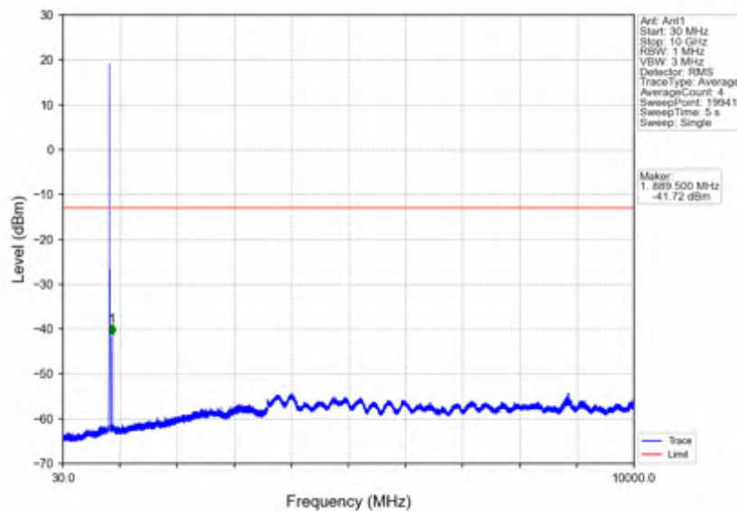
Band5_10MHz_256QAM_HCH_844MHz_RB_1_0_NTNV
