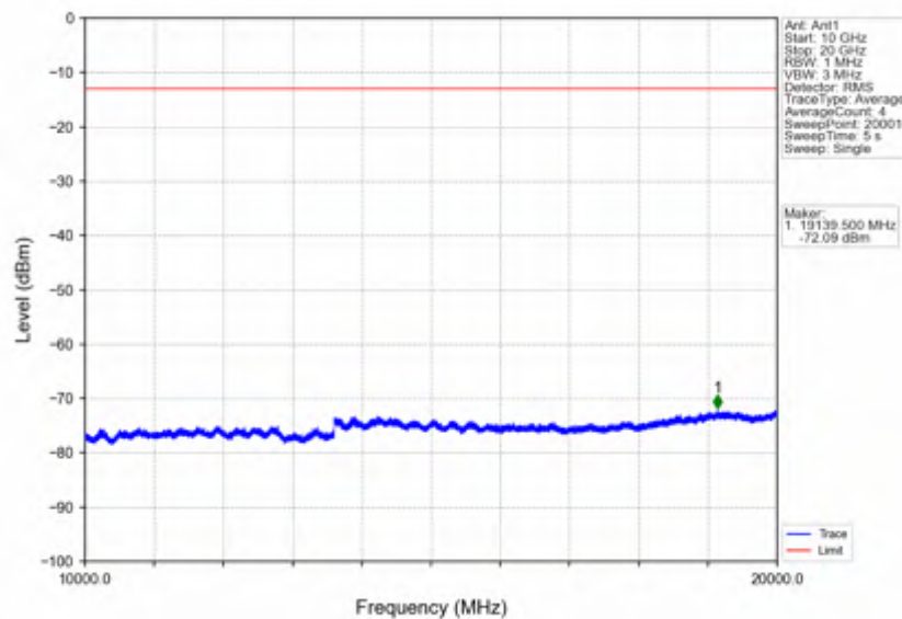
Band4_10MHz_QPSK_LCH_1715MHz_RB_50_0_NTNV
