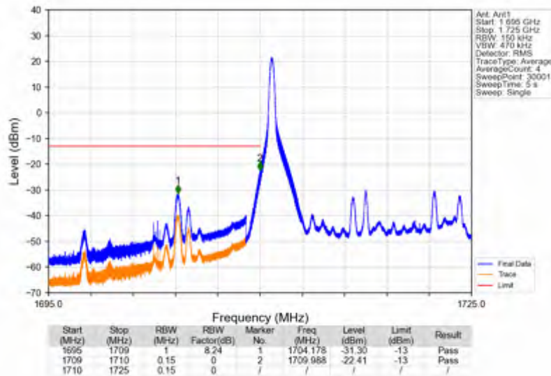
Band4_15MHz_16QAM_LCH_1717.5MHz_RB_1_0_NTNV
