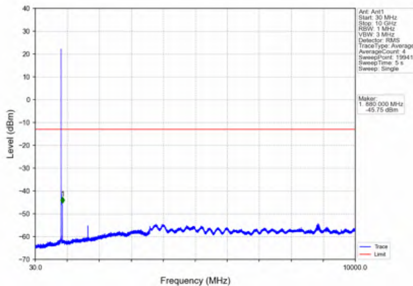
Band5_5MHz_QPSK_MCH_836.5MHz_RB_1_0_NTNV
