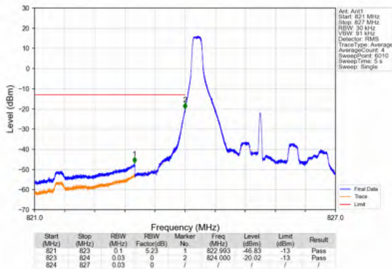
Band5_3MHz_16QAM_LCH_825.5MHz_RB_1_0_NTNV
