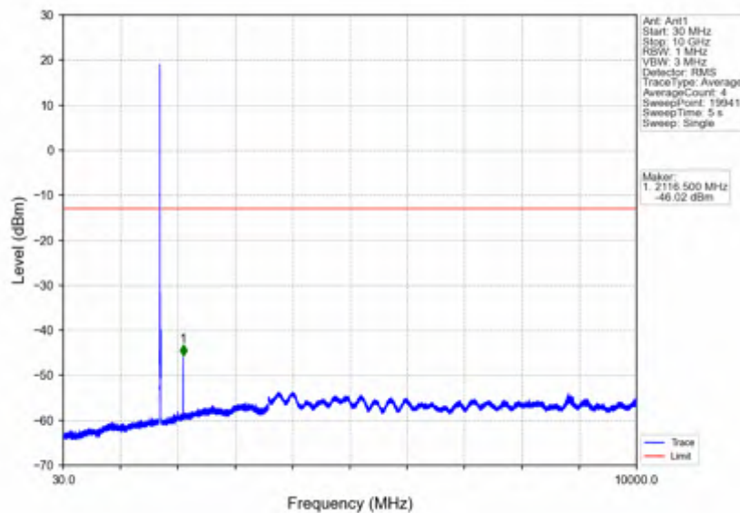
Band4 10MHz 256QAM LCH 1715MHz RB 1 0 NTNV
