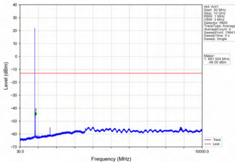
Band5_5MHz_64QAM_MCH_836.5MHz_RB_1_0_NTNV
