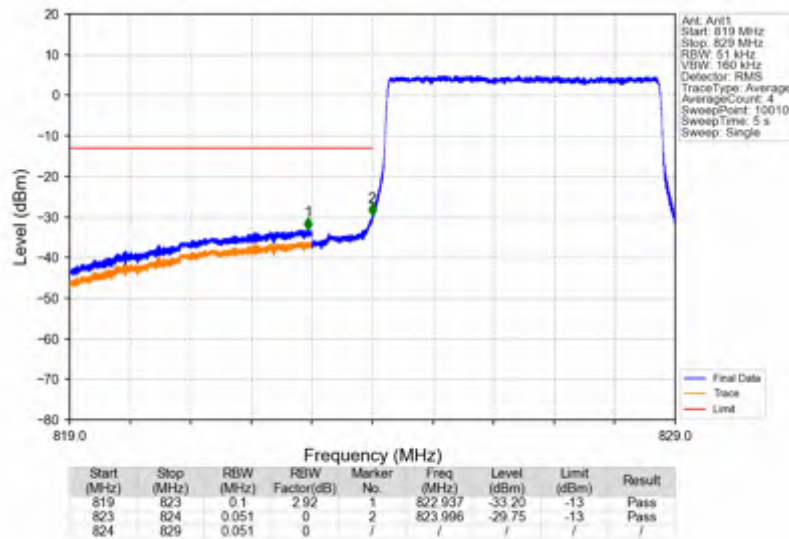
Band5_5MHz_QPSK_LCH_826.5MHz_RB_25_0_NTNV
