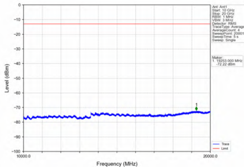
Band4_15MHz_256QAM_LCH_1717.5MHz_RB_75_0_NTNV
