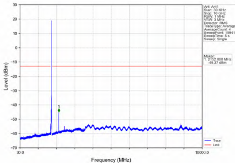
Band4_20MHz_256QAM_HCH_1745MHz_RB_1_0_NTNV
