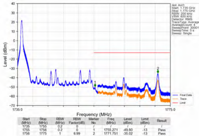
Band4_20MHz_16QAM_HCH_1745MHz_RB_100_0_NTNV
