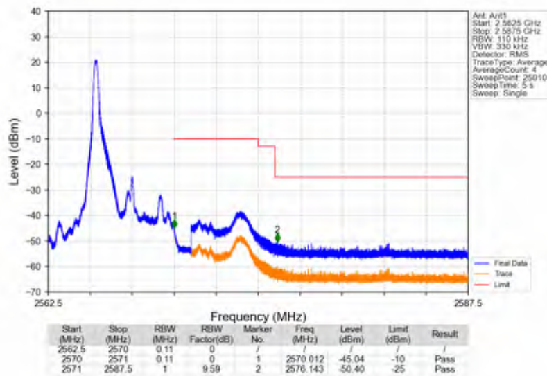
Band7 5MHz 64QAM HCH 2567.5MHz RB 1 24 NTN
