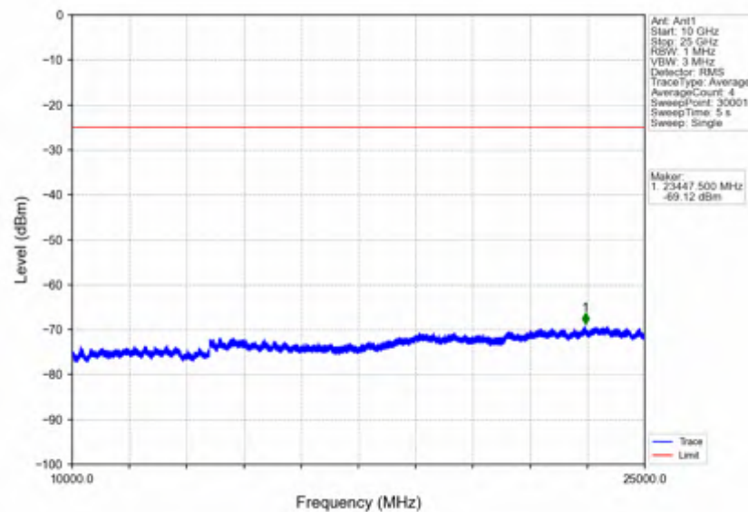
Band7_5MHz_64QAM_LCH_2502.5MHz_RB_1_0_NTNV
