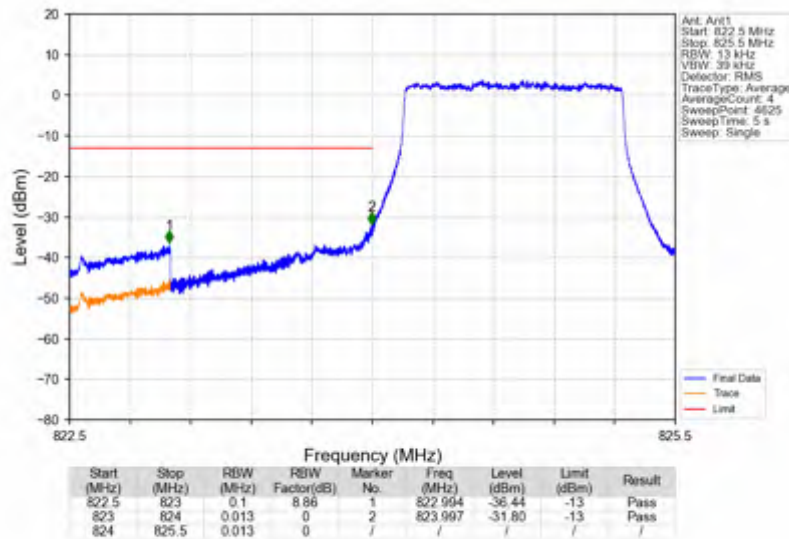
Band5_1.4MHz_64QAM_LCH_824.7MHz_RB_6_0_NTNV
