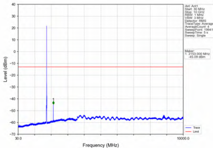
Band4_10MHz_64QAM_HCH_1750MHz_RB_1_0_NTNV
