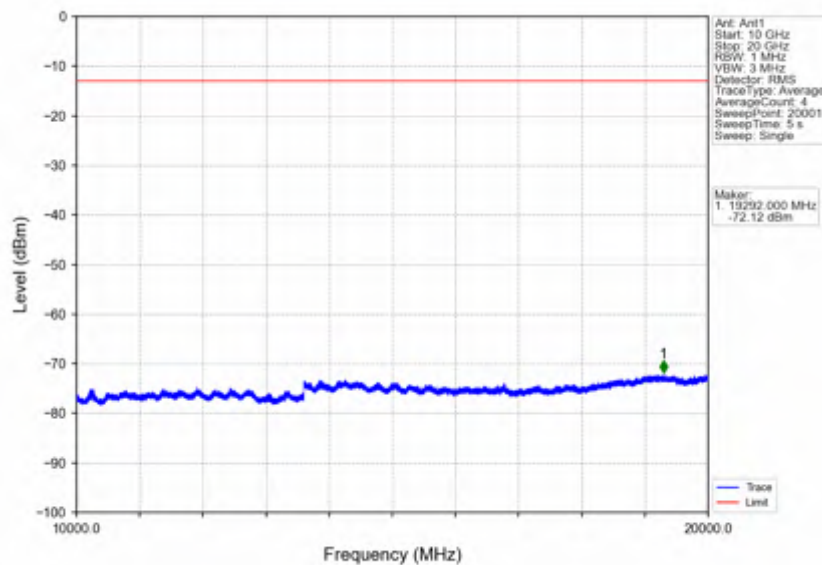
Band4_15MHz_16QAM_HCH_1747.5MHz_RB_1_0_NTNV
