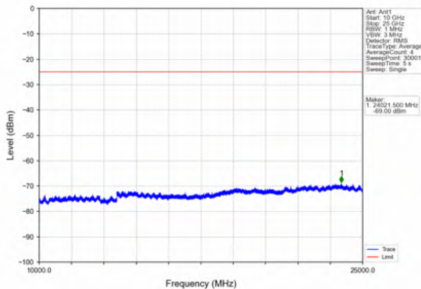
Band7_5MHz_16QAM_LCH_2502.5MHz_RB_1_0_NTNV
