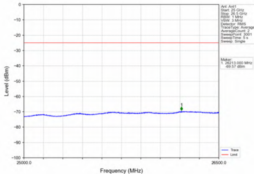
Band7_10MHz_64QAM_HCH_2565MHz_RB_1_49_NTNV
