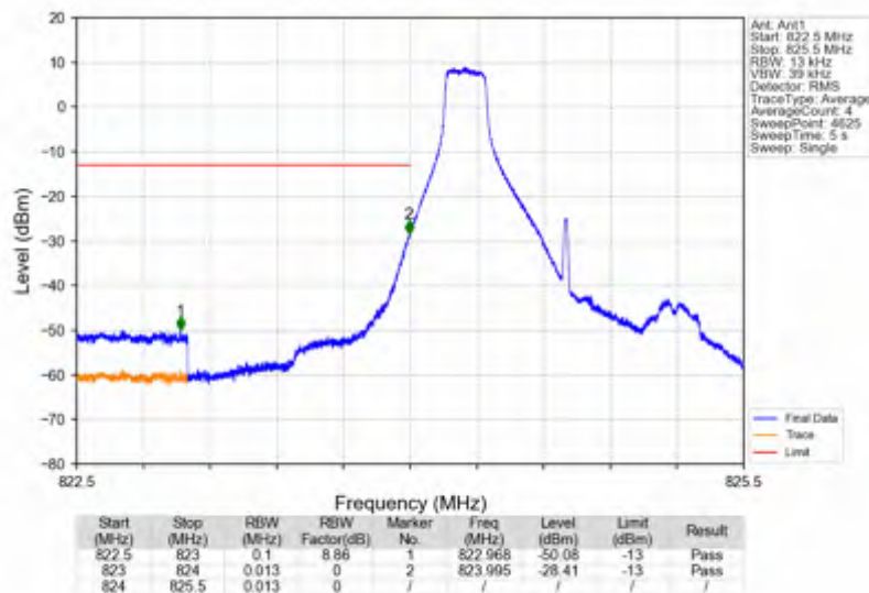
Band5_1.4MHz_256QAM_LCH_824.7MHz_RB_1_0_NTNV
