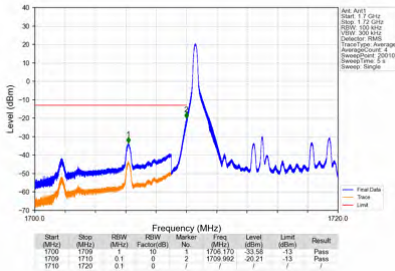
Band4_10MHz_QPSK_LCH_1715MHz_RB_1_0_NTNV
