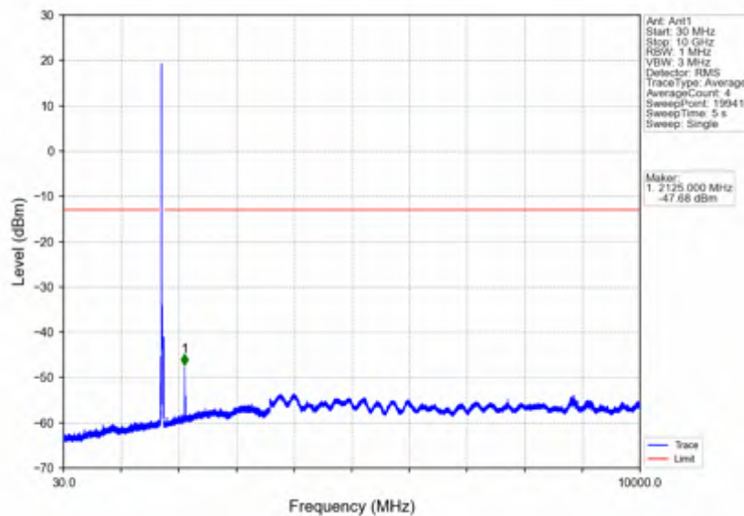
Band4_20MHz_256QAM_MCH_1732.5MHz_RB_1_0_NTNV
