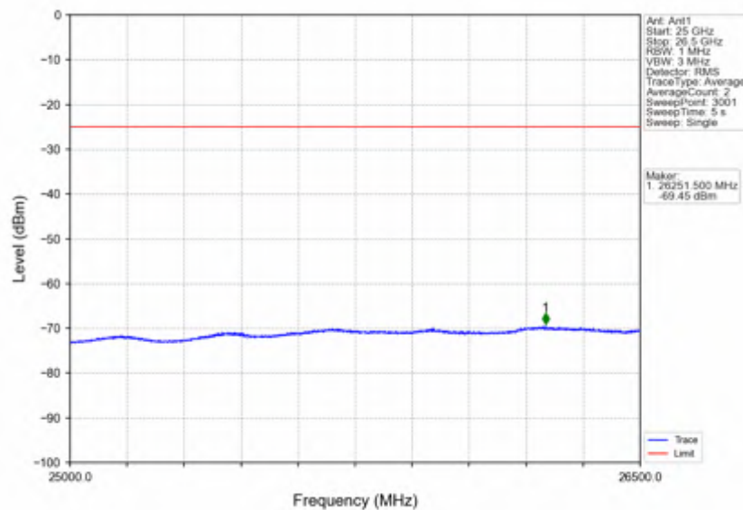
Band7_10MHz_16QAM_LCH_2505MHz_RB_50_0_NTNV
