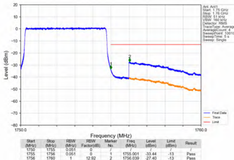
Band4_5MHz_256QAM_HCH_1752.5MHz_RB_25_0_NTNV
