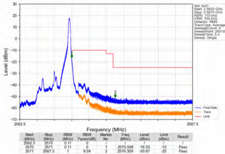
Band7_5MHz_256QAM_HCH_2567.5MHz_RB_1_24_NTNV
