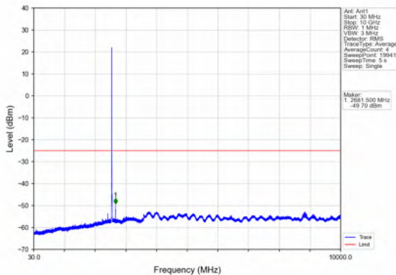
Band7_10MHz_64QAM_HCH_2565MHz_RB_1_0_NTNV
