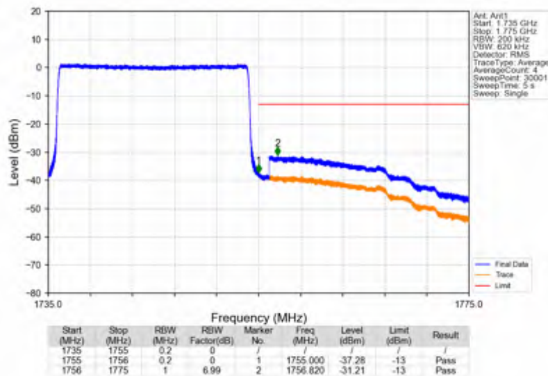
Band4_20MHz_256QAM_HCH_1745MHz_RB_100_0_NTNV
