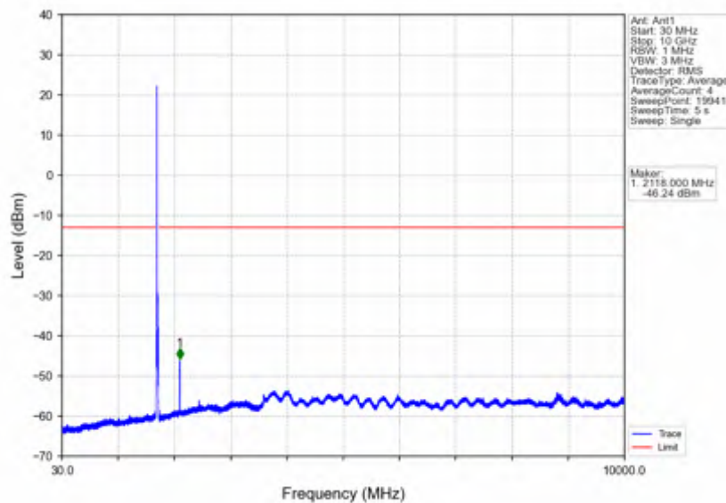
Band4_15MHz_16QAM_LCH_1717.5MHz_RB_1_0_NTNV
