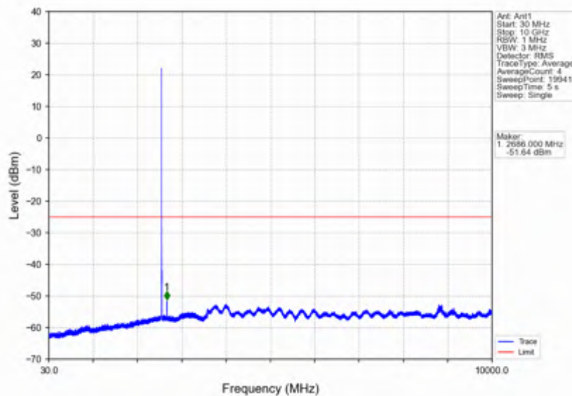
Band7_5MHz_64QAM_HCH_2567.5MHz_RB_1_0_NTNV
