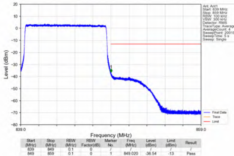
Band5_10MHz_64QAM_HCH_844MHz_RB_50_0_NTNV
