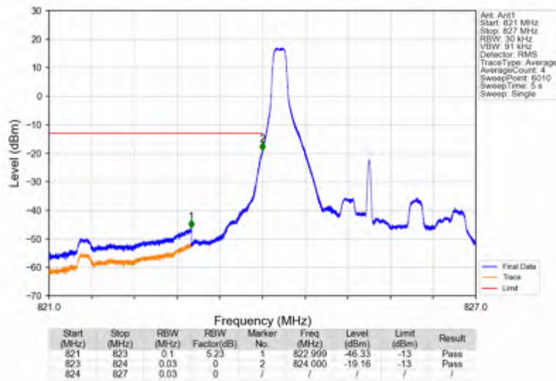
Band5_3MHz_QPSK_LCH_825.5MHz_RB_1_0_NTNV
