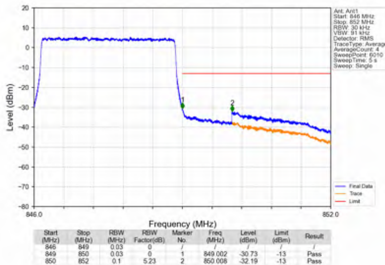
Band5_3MHz_16QAM_HCH_847.5MHz_RB_15_0_NTNV
