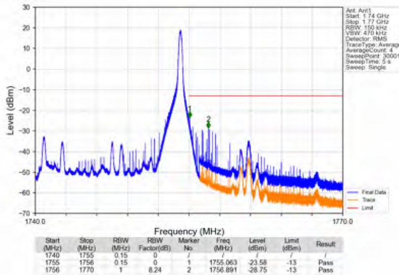
Band4_15MHz_256QAM_HCH_1747.5MHz_RB_1_74_NTNV
