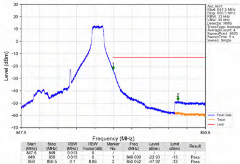
Band5_1.4MHz_64QAM_HCH_848.3MHz_RB_1_5_NTNV
