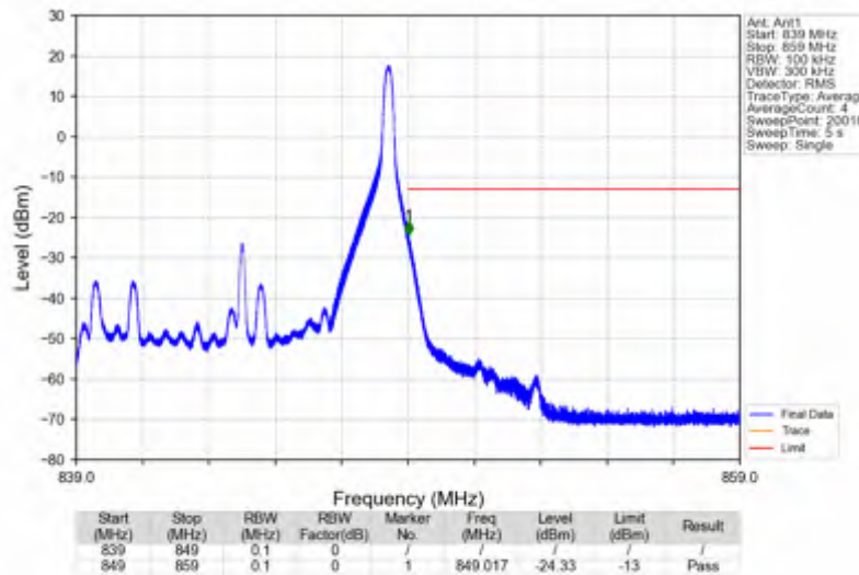
Band5_10MHz_256QAM_HCH_844MHz_RB_1_49_NTNV
