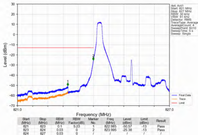
Band5_3MHz_256QAM_LCH_825.5MHz_RB_1_0_NTNV
