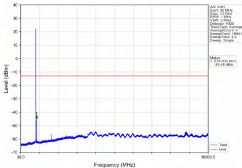
Band5_10MHz_64QAM_MCH_836.5MHz_RB_1_0_NTNV
