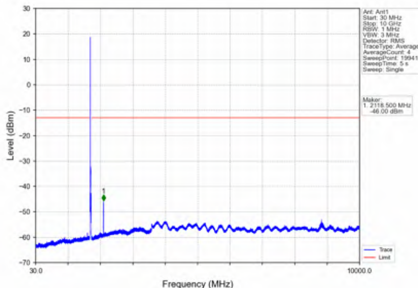
Band4_15MHz_256QAM_LCH_1717.5MHz_RB_1_0_NTNV
