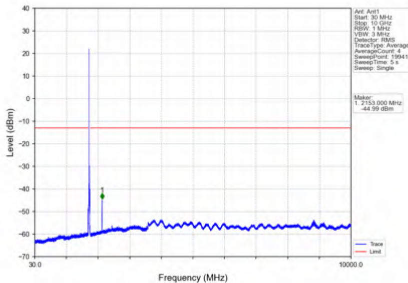
Band4_15MHz_QPSK_HCH_1747.5MHz_RB_1_0_NTNV
