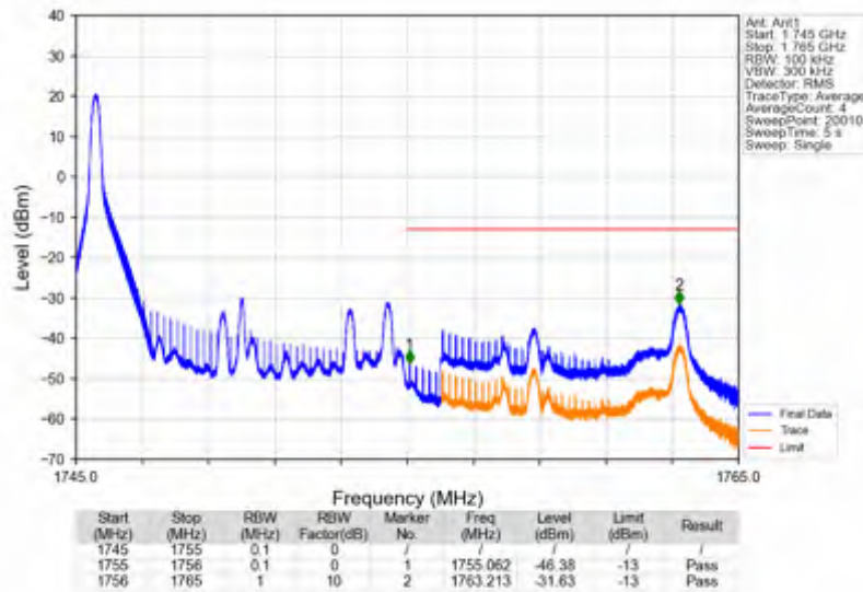
Band4_10MHz_16QAM_HCH_1750MHz_RB_50_0_NTNV
