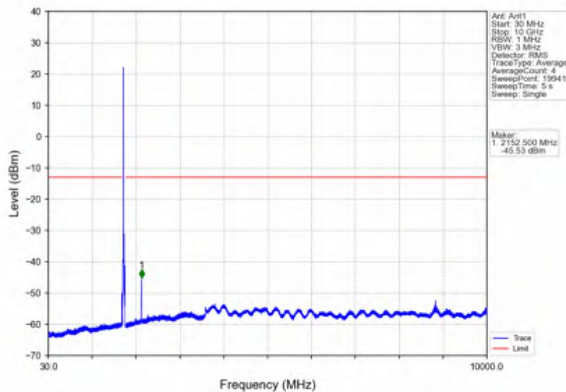
Band4_20MHz_16QAM_HCH_1745MHz_RB_1_0_NTNV
