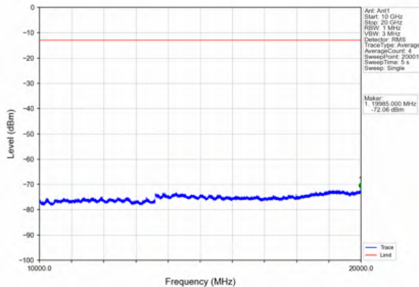
Band4_15MHz_16QAM_LCH_1717.5MHz_RB_75_0_NTNV
