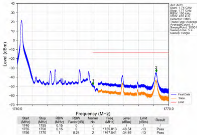
Band4_15MHz_16QAM_HCH_1747.5MHz_RB_1_74_NTNV
