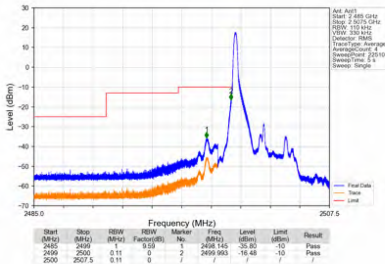
Band7_5MHz_256QAM_LCH_2502.5MHz_RB_25_0_NTNV
