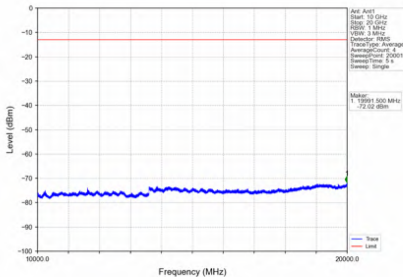
Band4_10MHz_16QAM_HCH_1750MHz_RB_1_0_NTNV
