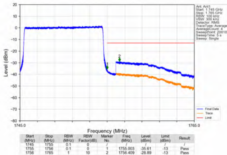
Band4_10MHz_256QAM_HCH_1750MHz_RB_50_0_NTNV
