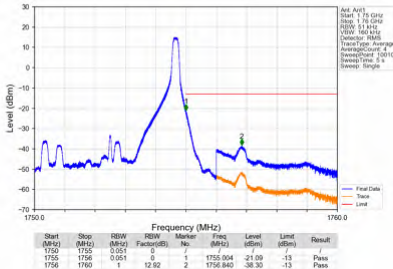
Band4_5MHz_256QAM_HCH_1752.5MHz_RB_1_24_NTNV
