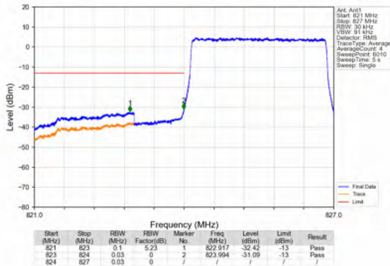
Band5_3MHz_QPSK_LCH_825.5MHz_RB_15_0_NTNV
