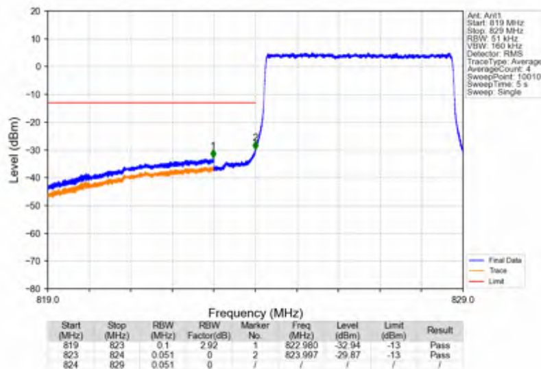
Band5_5MHz_16QAM_LCH_826.5MHz_RB_1_0_NTNV
