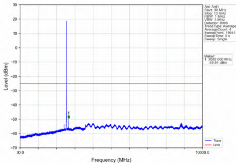
Band7_10MHz_256QAM_HCH_2565MHz_RB_1_0_NTNV
