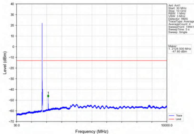
Band4_20MHz_16QAM_MCH_1732.5MHz_RB_1_0_NTNV
