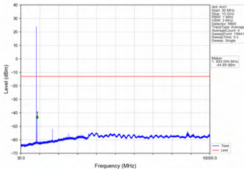
Band5_1.4MHz_QPSK_HCH_848.3MHz_RB_1_5_NTNV
