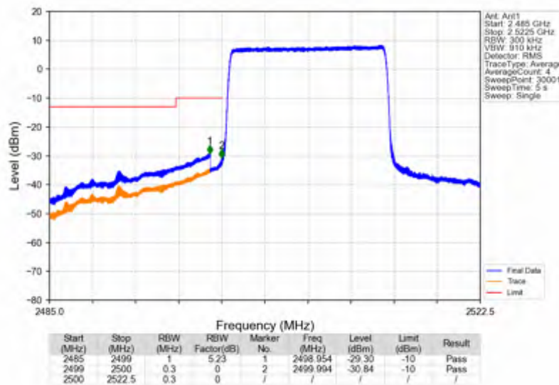
Band7_15MHz_16QAM_LCH_2507.5MHz_RB_1_0_NTNV
