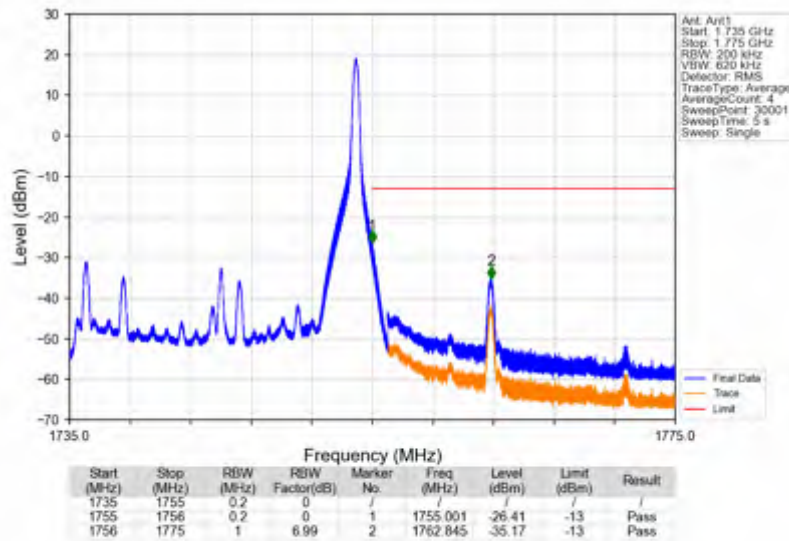
Band4_20MHz_256QAM_HCH_1745MHz_RB_1_99_NTNV
