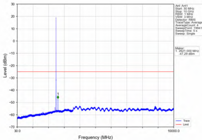
Band7_5MHz_256QAM_LCH_2502.5MHz_RB_1_0_NTNV
