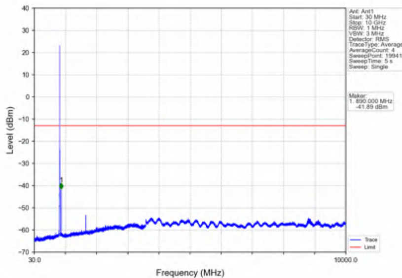
Band5_10MHz_16QAM_HCH_844MHz_RB_1_0_NTNV
