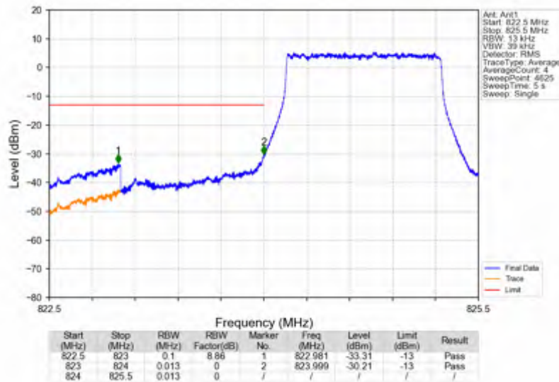
Band5_1.4MHz_QPSK_LCH_824.7MHz_RB_6_0_NTNV
