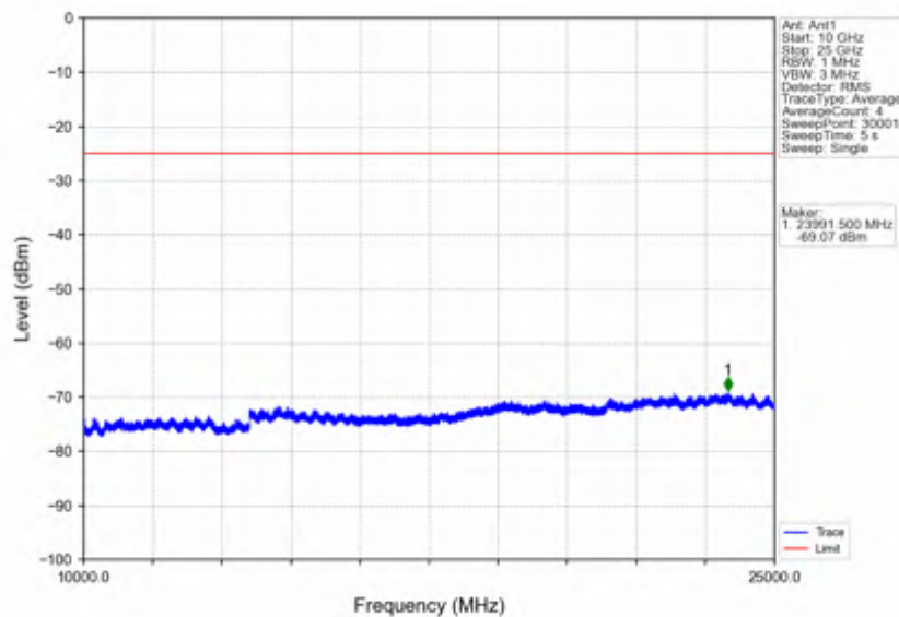
Band7_10MHz_16QAM_LCH_2505MHz_RB_1_0_NTNV
