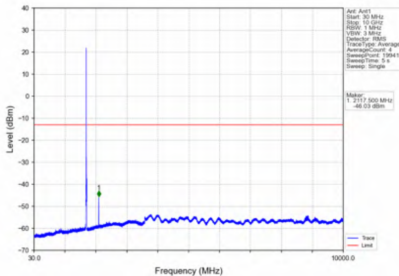
Band4_10MHz_16QAM_LCH_1715MHz_RB_1_0_NTNV
