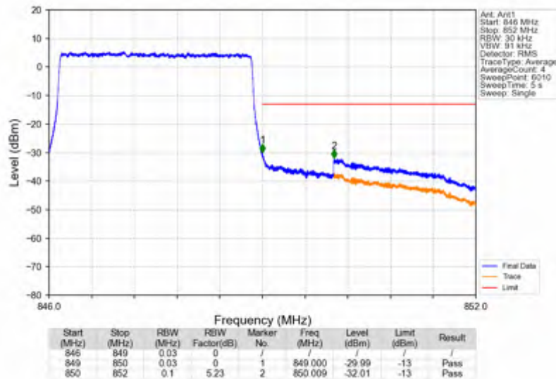
Band5_3MHz_64QAM_HCH_847.5MHz_RB_1_14_NTNV
