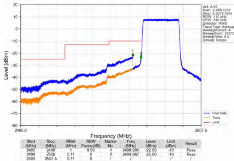
Band7_5MHz_16QAM_LCH_2502.5MHz_RB_1_0_NTNV
