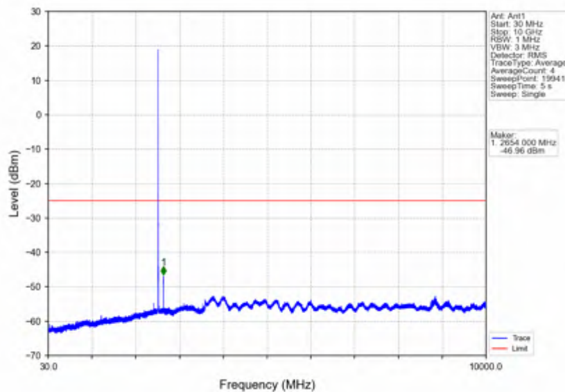
Band7_5MHz_256QAM_MCH_2535MHz_RB_1_0_NTNV
