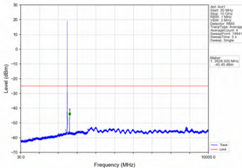
Band7_10MHz_256QAM_LCH_2505MHz_RB_1_0_NTNV
