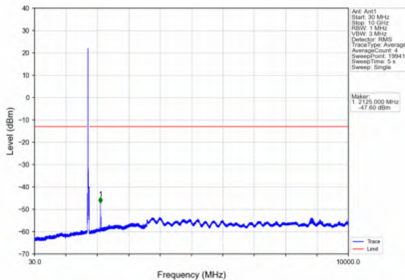
Band4_20MHz_64QAM_MCH_1732.5MHz_RB_1_0_NTNV
