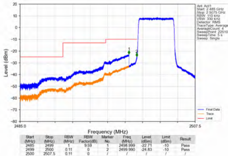
Band7_5MHz_64QAM_LCH_2502.5MHz_RB_25_0_NTNV
