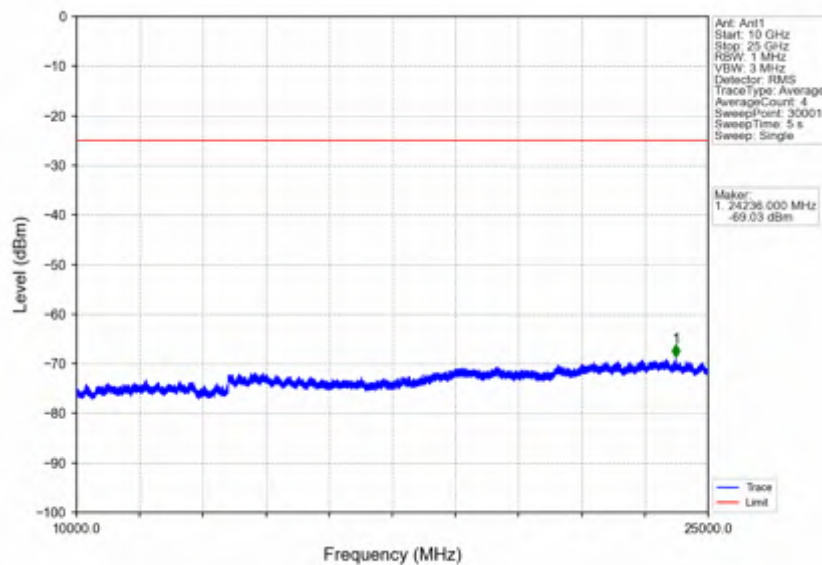
Band7_5MHz_16QAM_MCH_2535MHz_RB_1_0_NTNV
