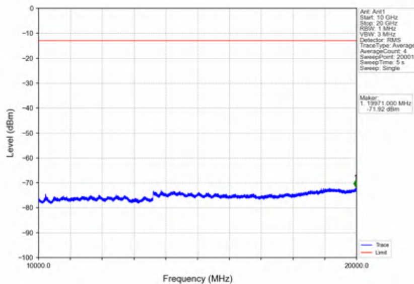
Band4_20MHz_64QAM_HCH_1745MHz_RB_1_0_NTNV
