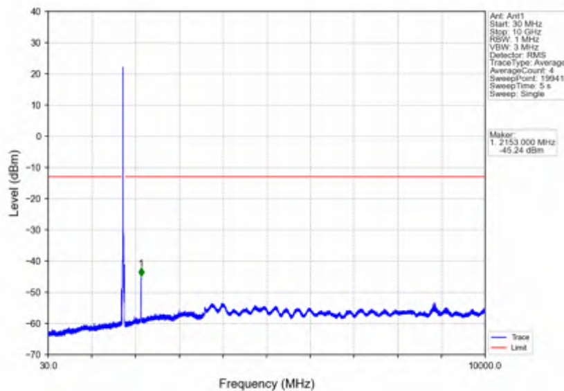
Band4_20MHz_64QAM_HCH_1745MHz_RB_1_0_NTNV
