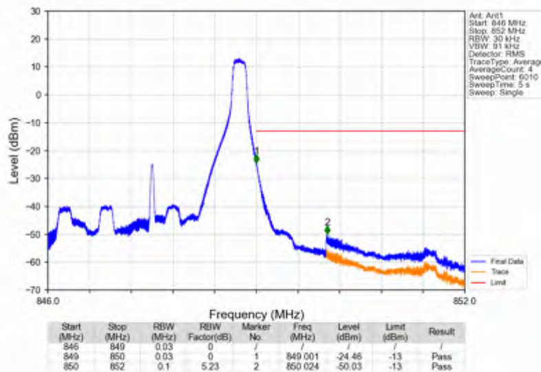
Band5_3MHz_256QAM_HCH_847.5MHz_RB_15_0_NTNV
