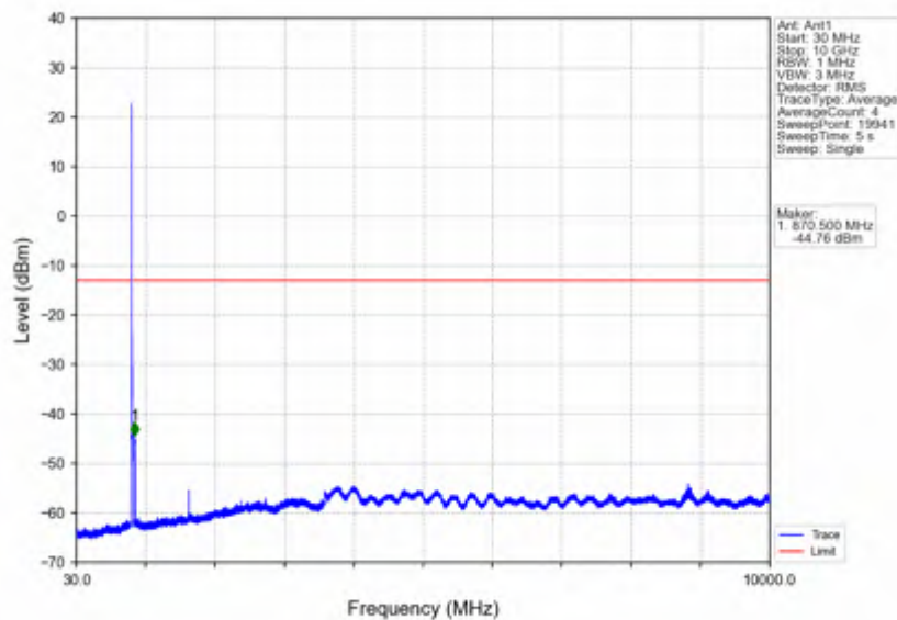
Band5_10MHz_16QAM_LCH_829MHz_RB_50_0_NTNV
