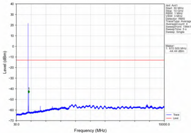
Band5_3MHz_64QAM_LCH_825.5MHz_RB_1_0_NTNV
