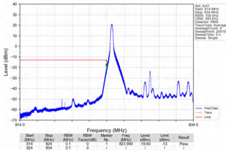
Band5_10MHz_16QAM_LCH_829MHz_RB_1_0_NTNV
