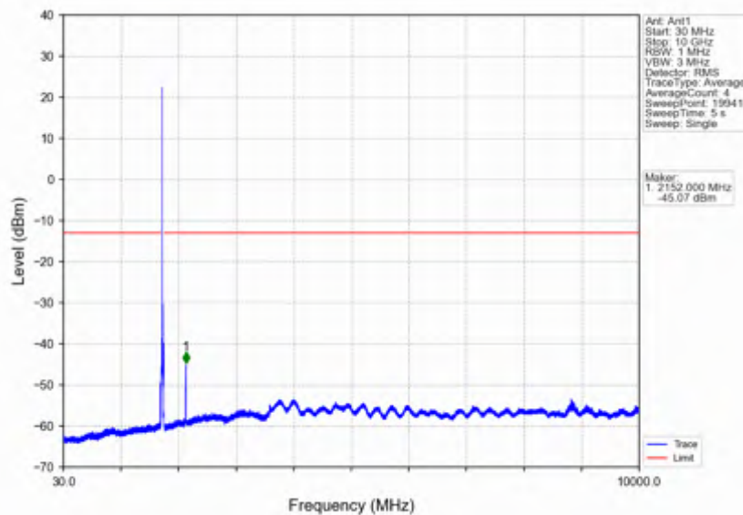
Band4_15MHz_16QAM_HCH_1747.5MHz_RB_1_0_NTNV
