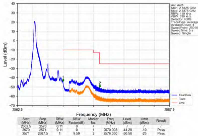
Band7_5MHz_64QAM_HCH_2567.5MHz_RB_25_0_NTNV
