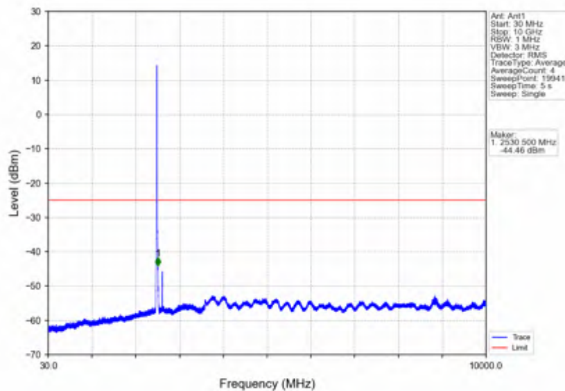
Band7_10MHz_64QAM_LCH_2505MHz_RB_1_0_NTNV
