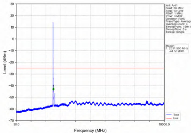
Band7_10MHz_16QAM_LCH_2505MHz_RB_1_0_NTNV
