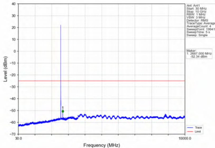
Band7_5MHz_16QAM_HCH_2567.5MHz_RB_1_0_NTNV
