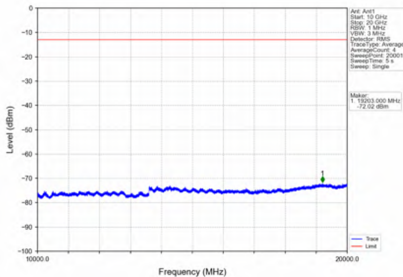
Band4_15MHz_QPSK_MCH_1732.5MHz_RB_1_0_NTNV
