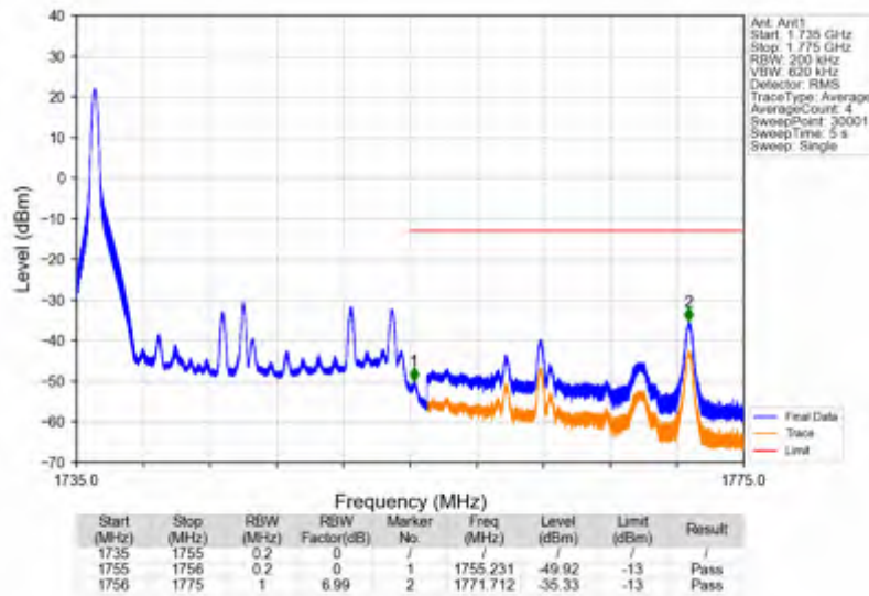
Band4_20MHz_64QAM_HCH_1745MHz_RB_1_99_NTNV
