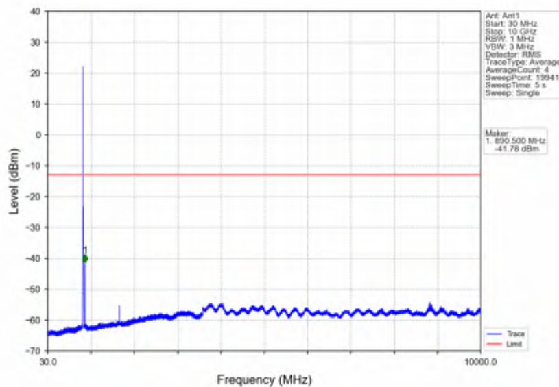
Band5_10MHz_64QAM_HCH_844MHz_RB_1_49_NTNV
