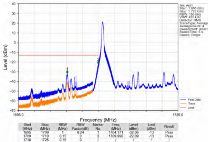
Band4 15MHz 64QAM LCH 1717.5MHz RB 1 0 NTNv
