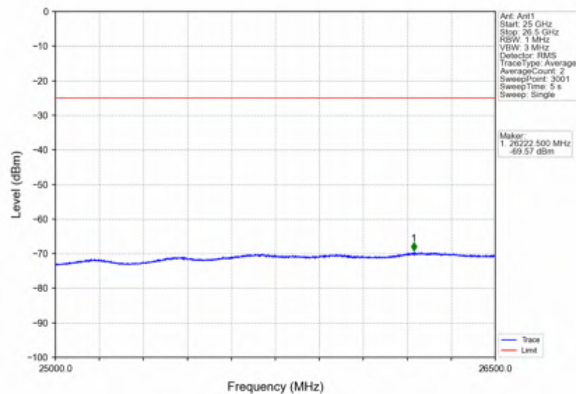
Band7_5MHz_16QAM_LCH_2502.5MHz_RB_25_0_NTNV
