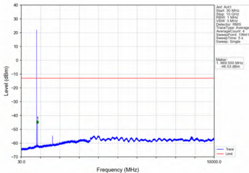
Band5_1.4MHz_16QAM_LCH_824.7MHz_RB_6_0_NTV
