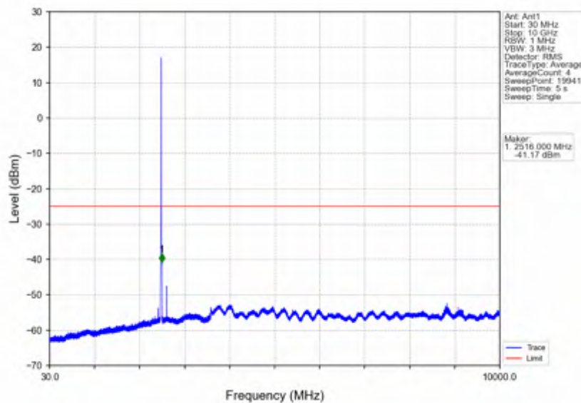
Band7_5MHz_64QAM_LCH_2502.5MHz_RB_1_0_NTNV
