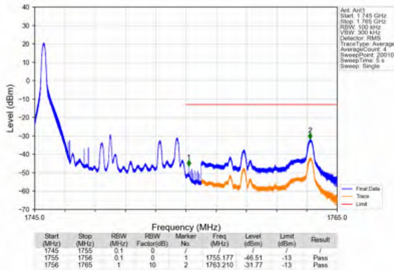
Band4_10MHz_16QAM_HCH_1750MHz_RB_1_49_NTNV
