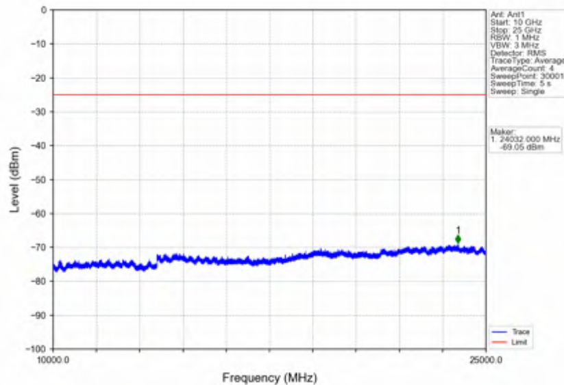
Band7_5MHz_16QAM_HCH_2567.5MHz_RB_1_0_NTNV
