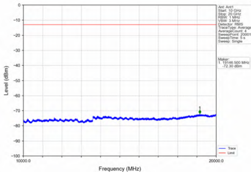
Band4_15MHz_16QAM_MCH_1732.5MHz_RB_1_0_NTNV
