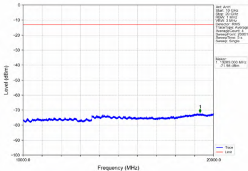
Band4_15MHz_256QAM_HCH_1747.5MHz_RB_1_0_NTNV
