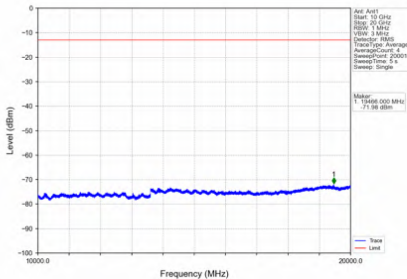
Band4_10MHz_64QAM_HCH_1750MHz_RB_1_0_NTNV
