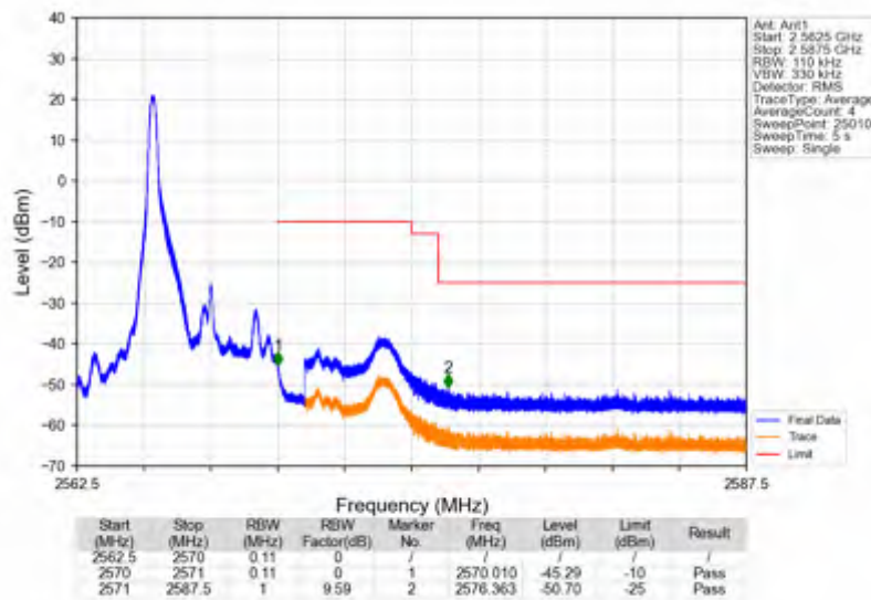
Band7_5MHz_16QAM_HCH_2567.5MHz_RB_25_0_NTNV
