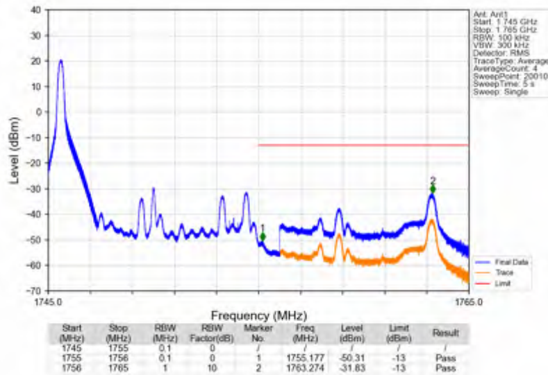
Band4_10MHz_64QAM_HCH_1750MHz_RB_1_49_NTNV
