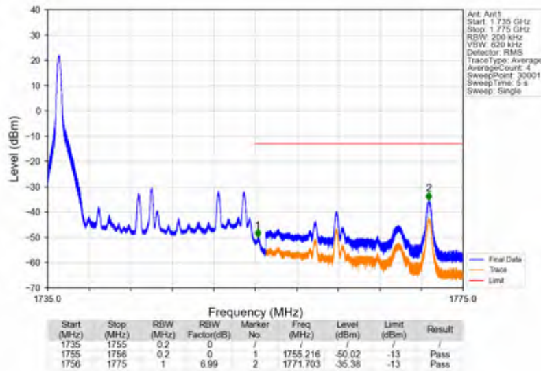
Band4_20MHz_16QAM_HCH_1745MHz_RB_1_99_NTNV
