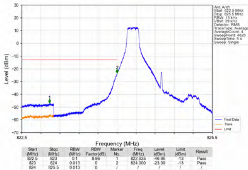
Band5_1.4MHz_16QAM_LCH_824.7MHz_RB_1_0_NTNV
