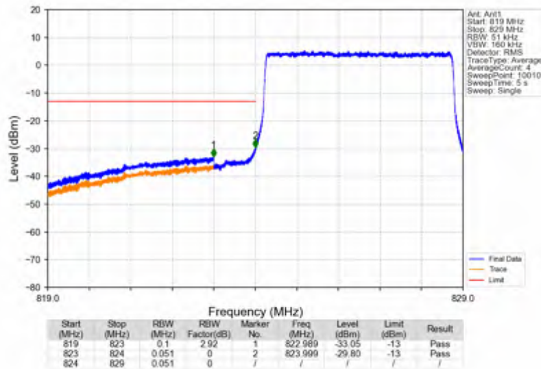
Band5_5MHz_16QAM_LCH_826.5MHz_RB_25_0_NTNV
