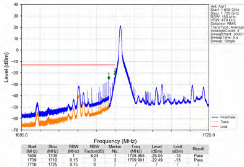
Band4_15MHz_64QAM_LCH_1717.5MHz_RB_75_0_NTNV
