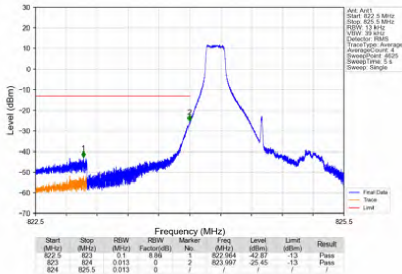
Band5 1.4MHz 64QAM LCH 824.7MHz RB 1 0 NTN
