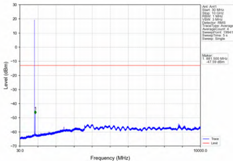
Band5_1.4MHz_256QAM_HCH_848.3MHz_RB_1_0_NTNV
