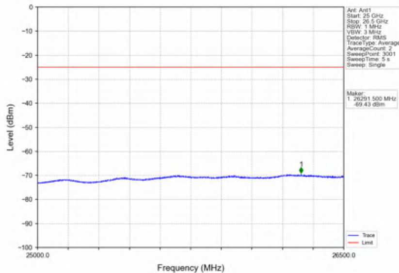
Band7_10MHz_64QAM_MCH_2535MHz_RB_1_0_NTNV
