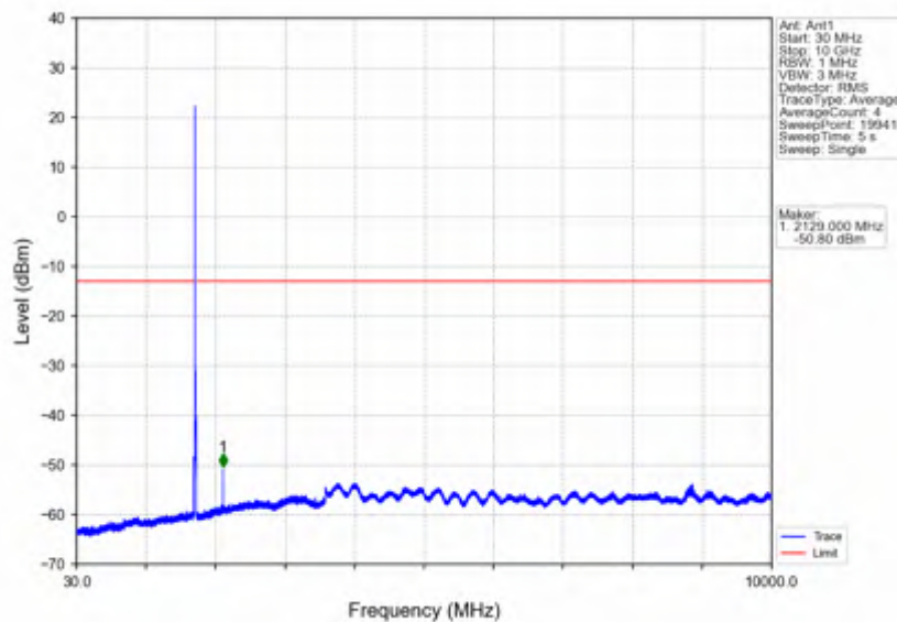
Band4_10MHz_16QAM_MCH_1732.5MHz_RB_1_0_NTNV
