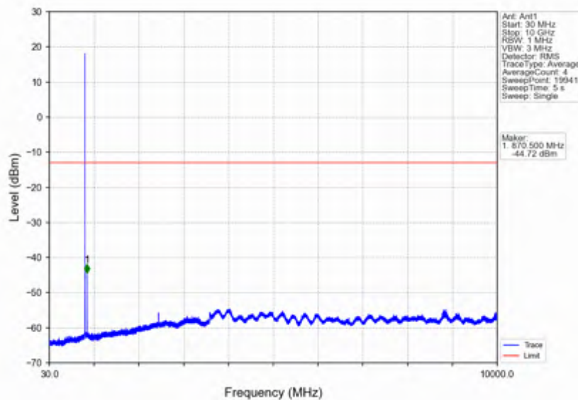
Band5_3MHz_256QAM_LCH_825.5MHz_RB_15_0_NTNV
