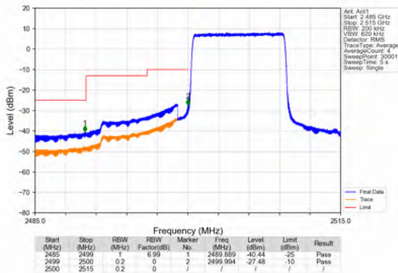
Band7_10MHz_16QAM_LCH_2505MHz_RB_50_0_NTNV
