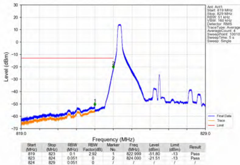
Band5_5MHz_256QAM_LCH_826.5MHz_RB_1_0_NTNV
