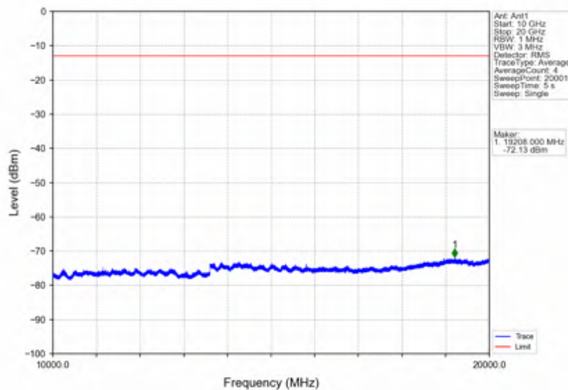
Band4_15MHz_QPSK_HCH_1747.5MHz_RB_1_0_NTNV
