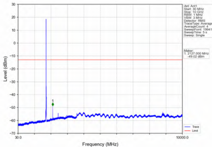
Band4_15MHz_256QAM_MCH_1732.5MHz_RB_1_0_NTNV
