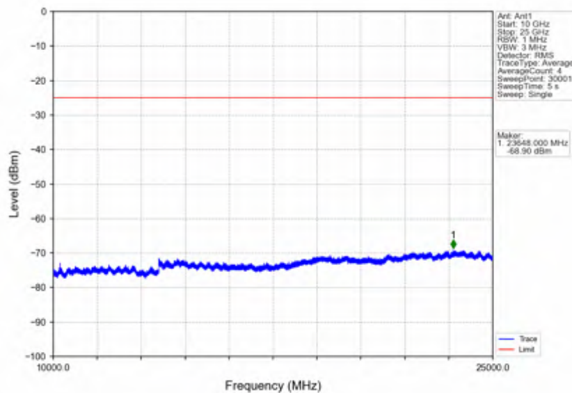
Band7_5MHz_64QAM_HCH_2567.5MHz_RB_1_0_NTNV
