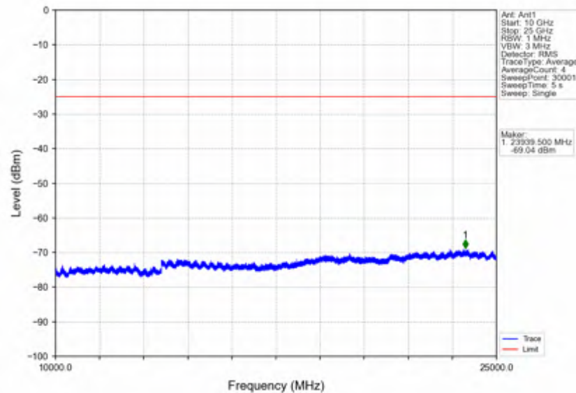
Band7_5MHz_64QAM_MCH_2535MHz_RB_1_0_NTNV
