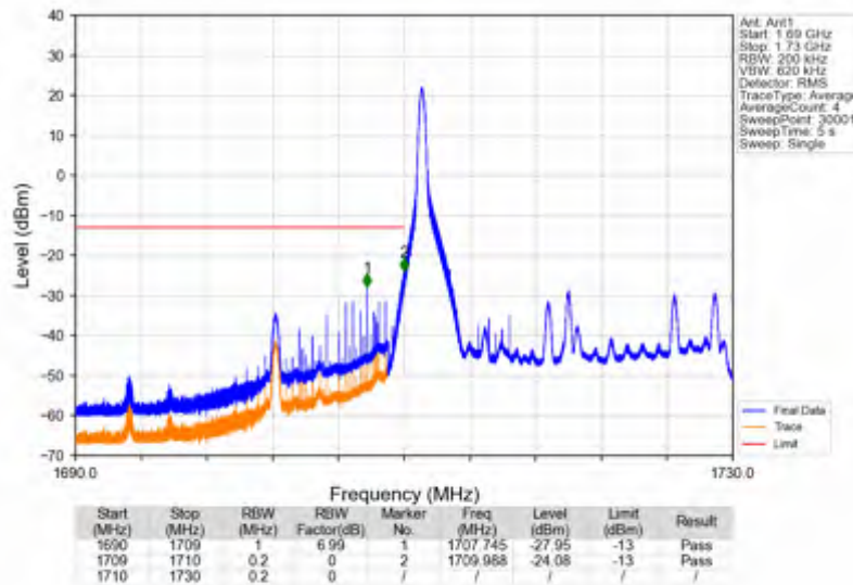
Band4_20MHz_64QAM_LCH_1720MHz_RB_100_0_NTNV
