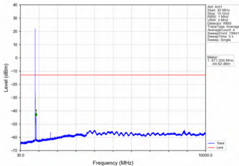
Band5 10MHz 64QAM LCH 829MHz RB 1 0 NTV
