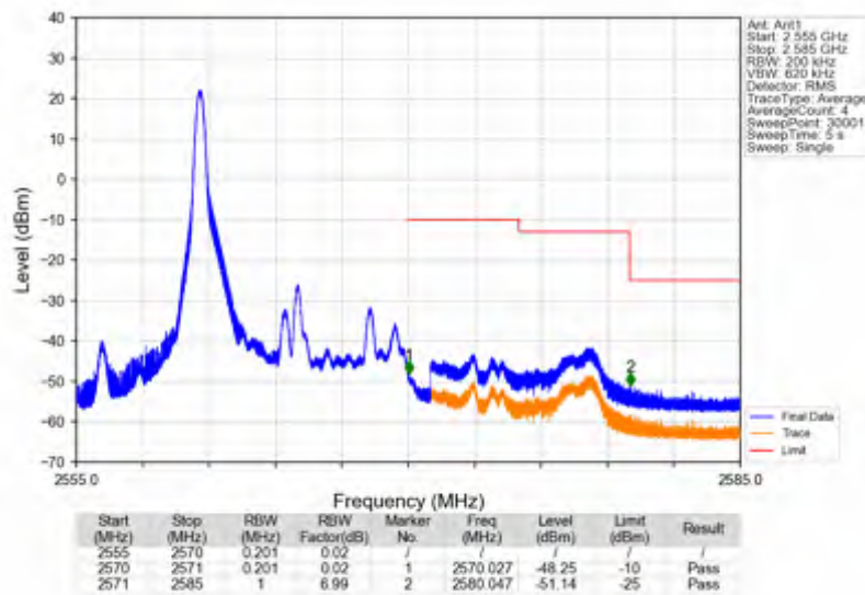
Band7_10MHz_16QAM_HCH_2565MHz_RB_50_0_NTV
