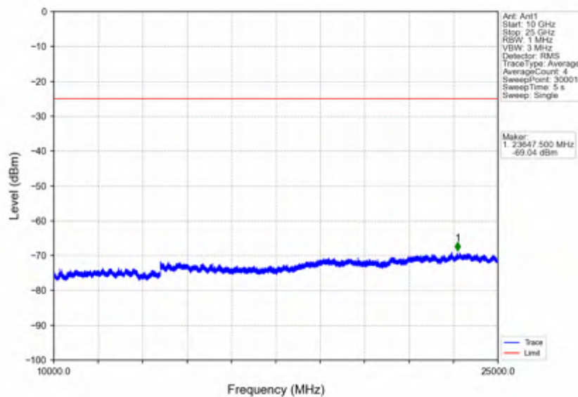
Band7_5MHz_256QAM_MCH_2535MHz_RB_1_0_NTNV
