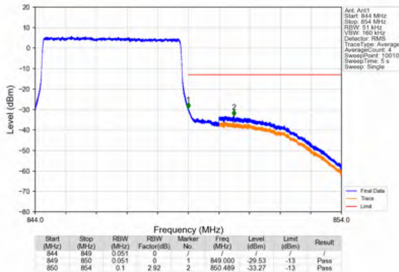
Band5_5MHz_64QAM_HCH_846.5MHz_RB_1_24_NTNV
