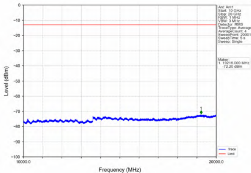
Band4_20MHz_64QAM_MCH_1732.5MHz_RB_1_0_NTNV
