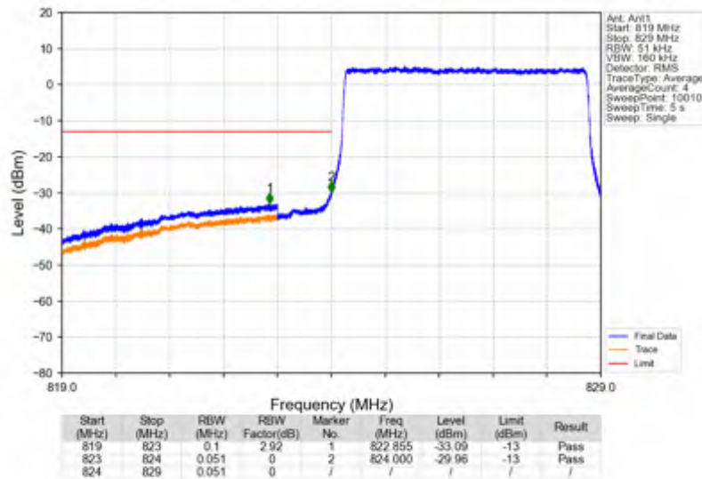
Band5_5MHz_64QAM_LCH_826.5MHz_RB_25_0_NTNV
