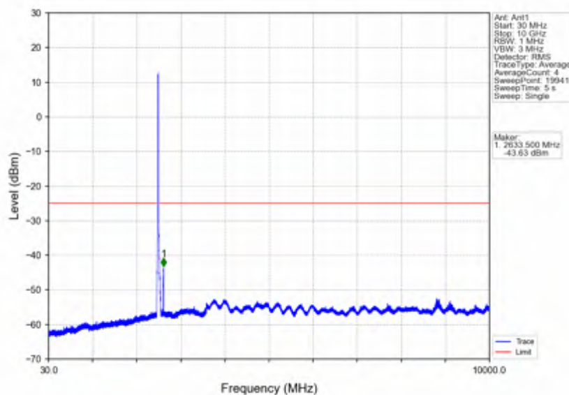
Band7_15MHz_QPSK_LCH_2507.5MHz_RB_1_0_NTNV
