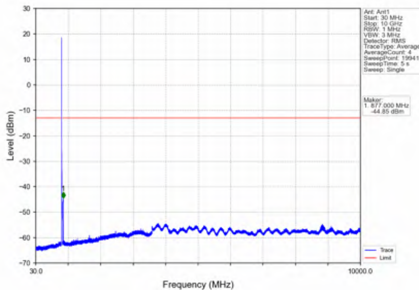
Band5_10MHz_256QAM_LCH_829MHz_RB_50_0_NTNV
