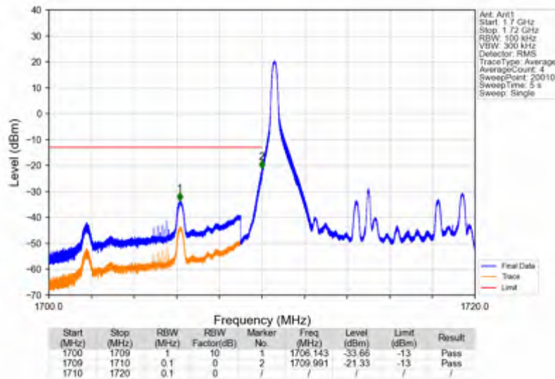
Band4_10MHz_16QAM_LCH_1715MHz_RB_1_0_NTNV
