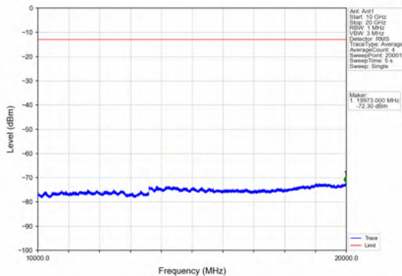
Band4_10MHz_64QAM_LCH_1715MHz_RB_50_0_NTNV
