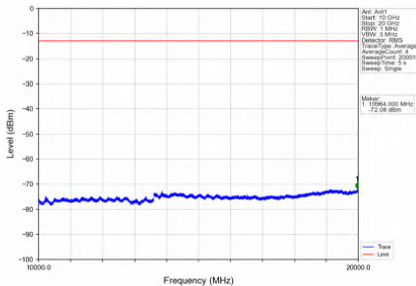
Band4_20MHz_256QAM_MCH_1732.5MHz_RB_1_0_NTNV
