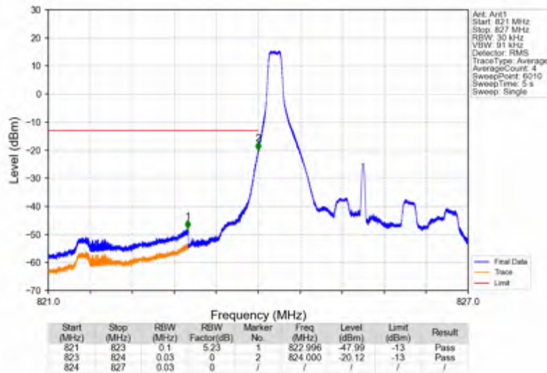
Band5 3MHz 64QAM LCH 825.5MHz RB 1 0 NTVV
