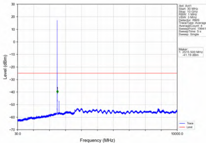
Band7_5MHz_16QAM_LCH_2502.5MHz_RB_1_0_NTNV
