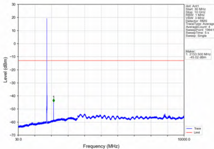
Band4_10MHz_256QAM_HCH_1750MHz_RB_1_0_NTNV
