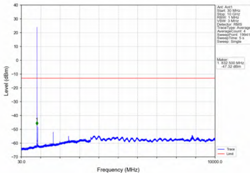
Band5_1.4MHz_QPSK_MCH_836.5MHz_RB_1_0_NTNV
