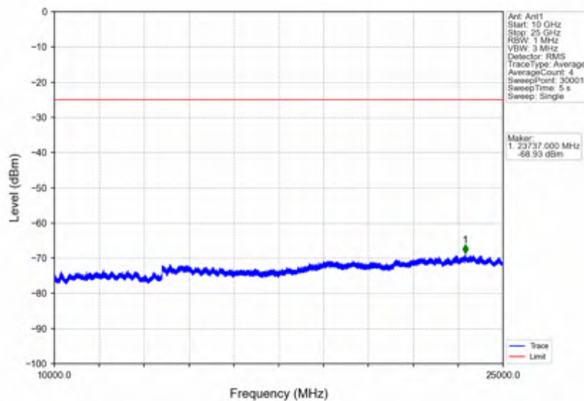
Band7_5MHz_256QAM_LCH_2502.5MHz_RB_1_0_NTNV
