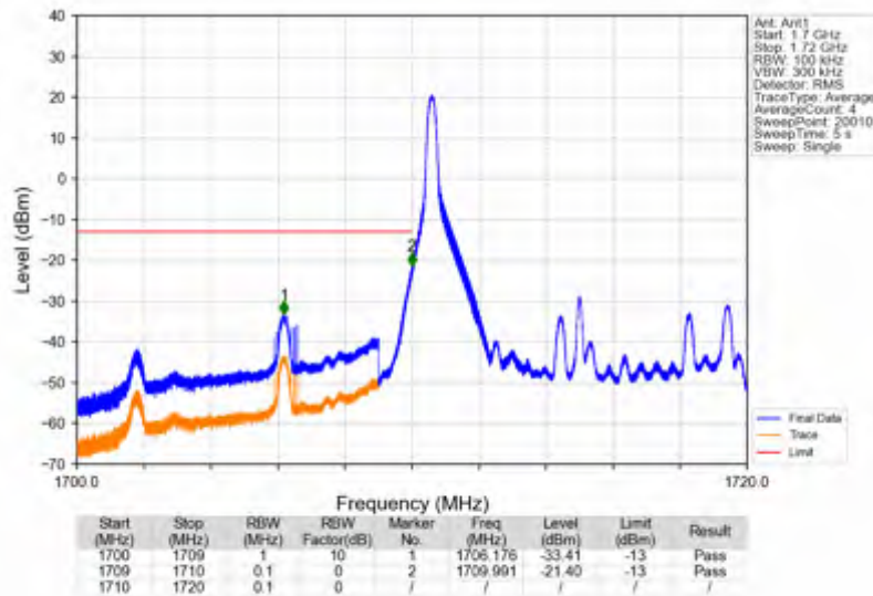
Band4_10MHz_64QAM_LCH_1715MHz_RB_1_0_NTNV
