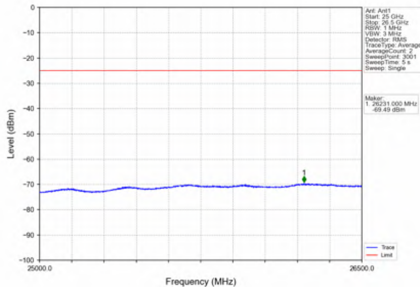
Band7_10MHz_64QAM_LCH_2505MHz_RB_1_0_NTNV
