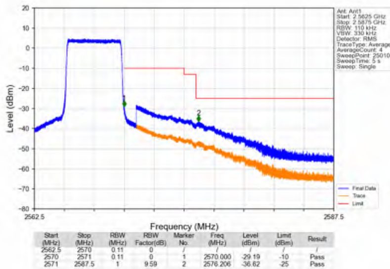
Band7_5MHz_256QAM_HCH_2567.5MHz_RB_25_0_NTNV
