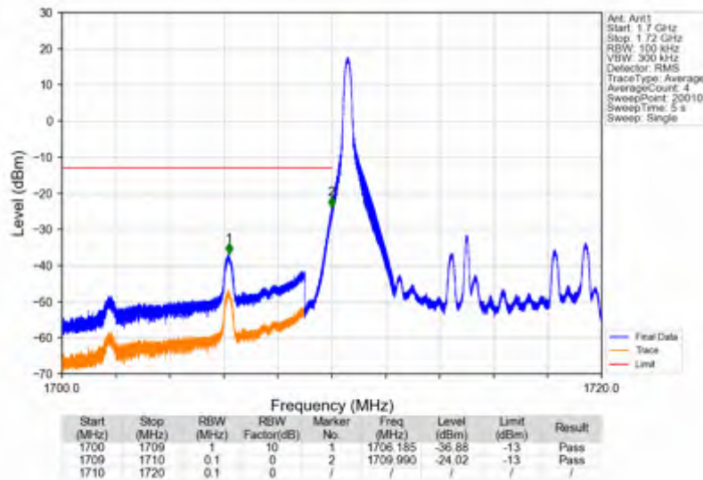
Band4 10MHz 256QAM LCH 1715MHz RB 1 0 NTNV
