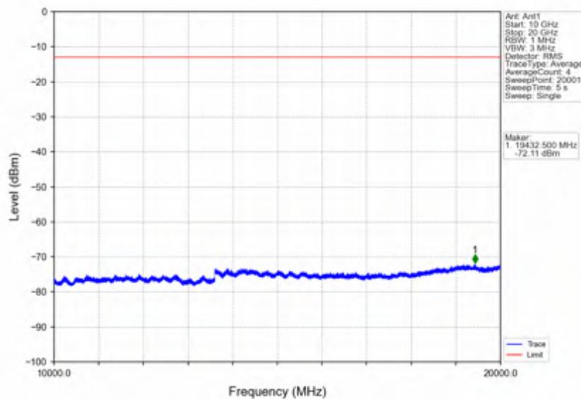
Band4_10MHz_QPSK_MCH_1732.5MHz_RB_1_0_NTNV
