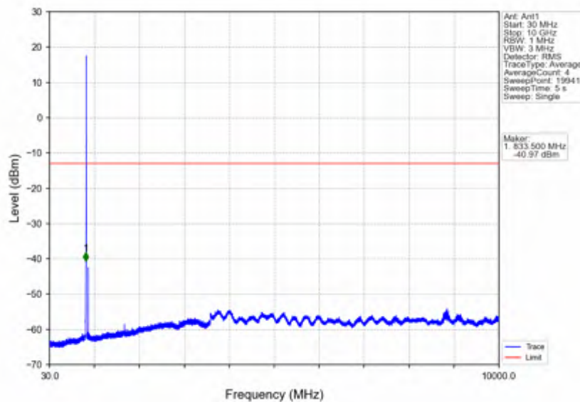
Band5_5MHz_16QAM_HCH_846.5MHz_RB_1_0_NTNV
