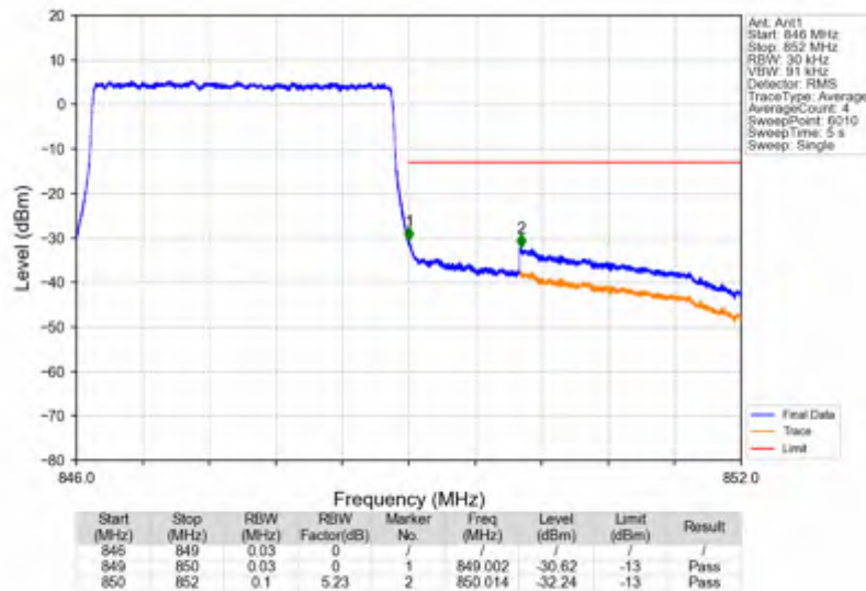
Band5_3MHz_64QAM_HCH_847.5MHz_RB_15_0_NTNV
