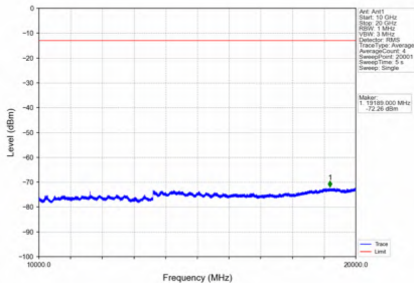
Band4_15MHz_64QAM_LCH_1717.5MHz_RB_75_0_NTNV
