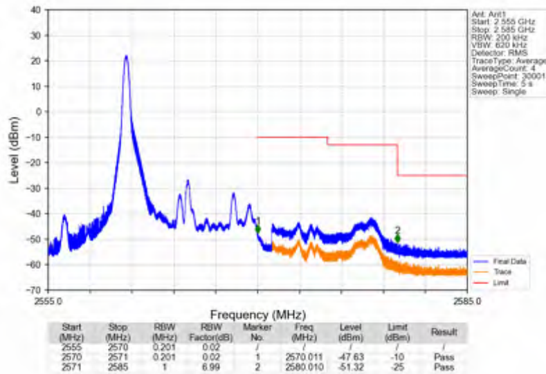
Band7_10MHz_64QAM_HCH_2565MHz_RB_50_0_NTNV
