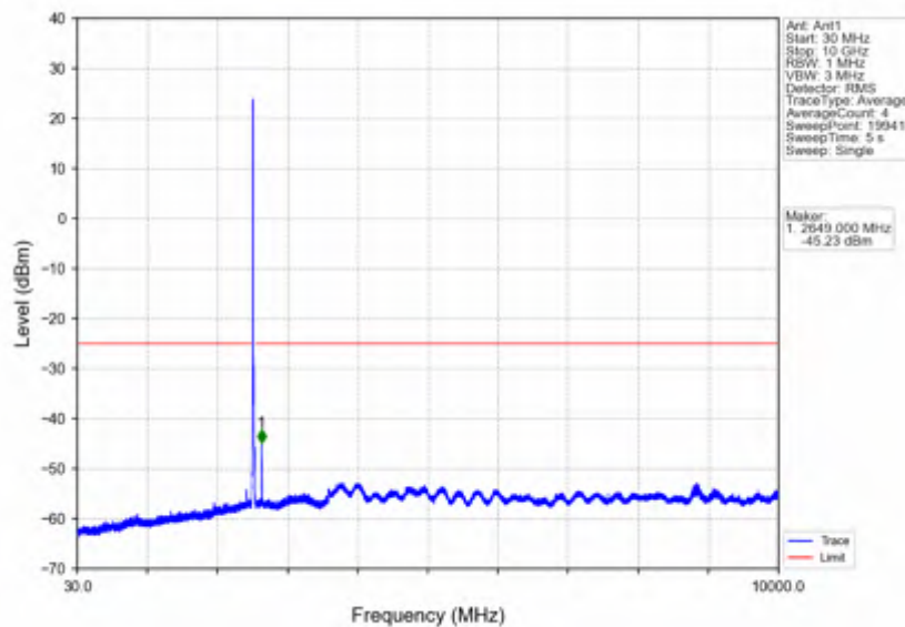
Band7_15MHz_QPSK_MCH_2535MHz_RB_1_0_NTNV
