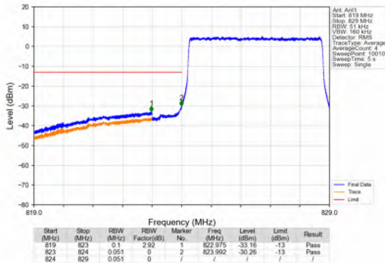
Band5_5MHz_64QAM_LCH_826.5MHz_RB_1_0_NTNV
