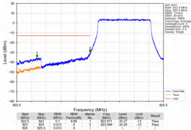
Band5_1.4MHz_16QAM_LCH_824.7MHz_RB_6_0_NTV
