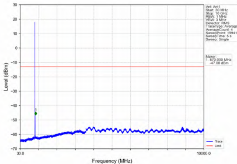
Band5_1.4MHz_256QAM_LCH_824.7MHz_RB_6_0_NTNV
