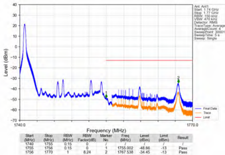
Band4_15MHz_64QAM_HCH_1747.5MHz_RB_75_0_NTNV
