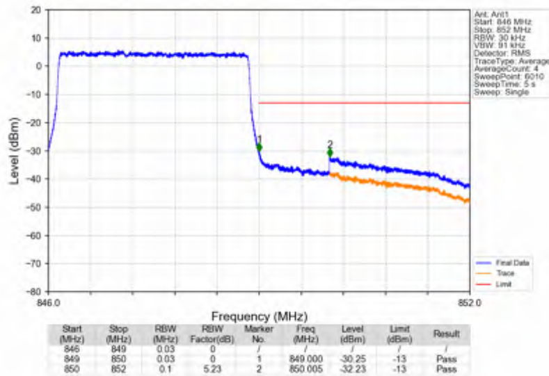
Band5_3MHz_QPSK_HCH_847.5MHz_RB_15_0_NTNV
