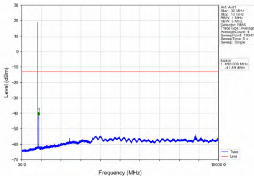
Band5_5MHz_256QAM_HCH_846.5MHz_RB_1_0_NTNV
