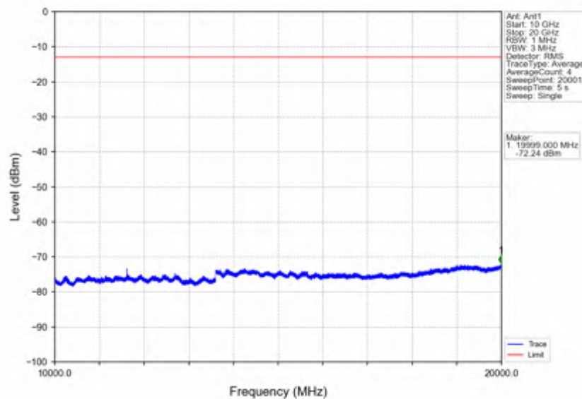
Band4_15MHz_QPSK_LCH_1717.5MHz_RB_75_0_NTNV
