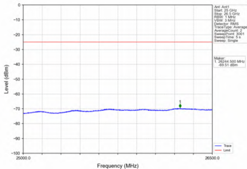
Band7_10MHz_256QAM_HCH_2565MHz_RB_1_0_NTNV
