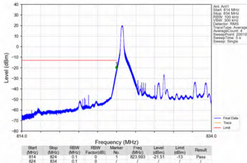
Band5 10MHz 64QAM LCH 829MHz RB 1 0 NTV
