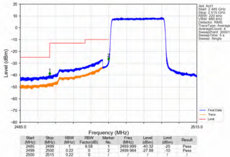
Band7_10MHz_64QAM_LCH_2505MHz_RB_1_0_NTNV
