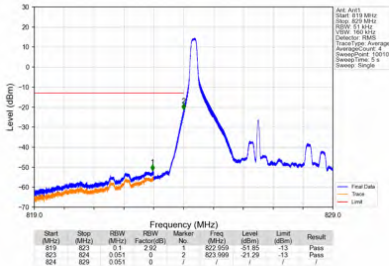
Band5_5MHz_256QAM_LCH_826.5MHz_RB_25_0_NTNV
