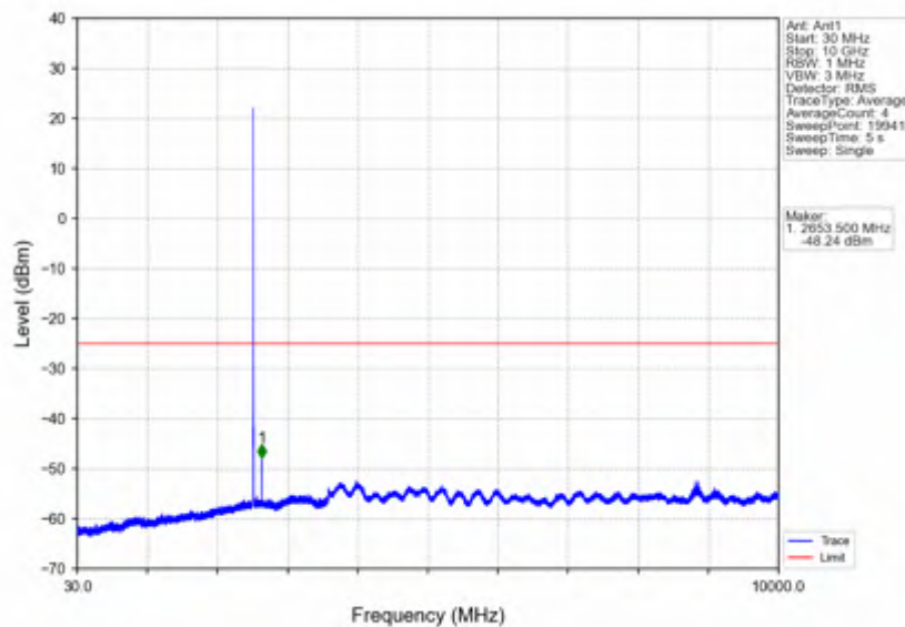
Band7_5MHz_64QAM_MCH_2535MHz_RB_1_0_NTNV
