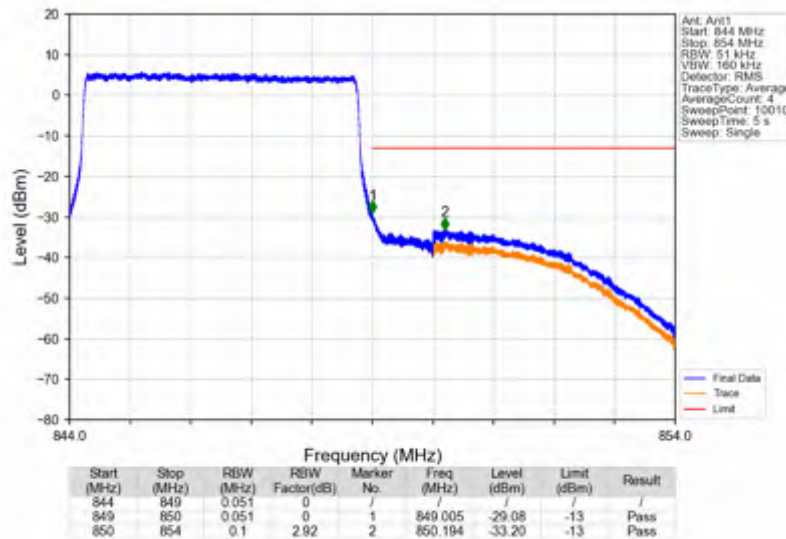
Band5_5MHz_16QAM_HCH_846.5MHz_RB_1_24_NTNV
