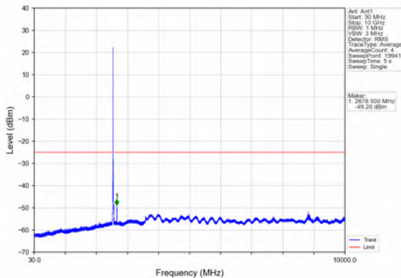
Band7_15MHz_QPSK_HCH_2562.5MHz_RB_1_0_NTNV
