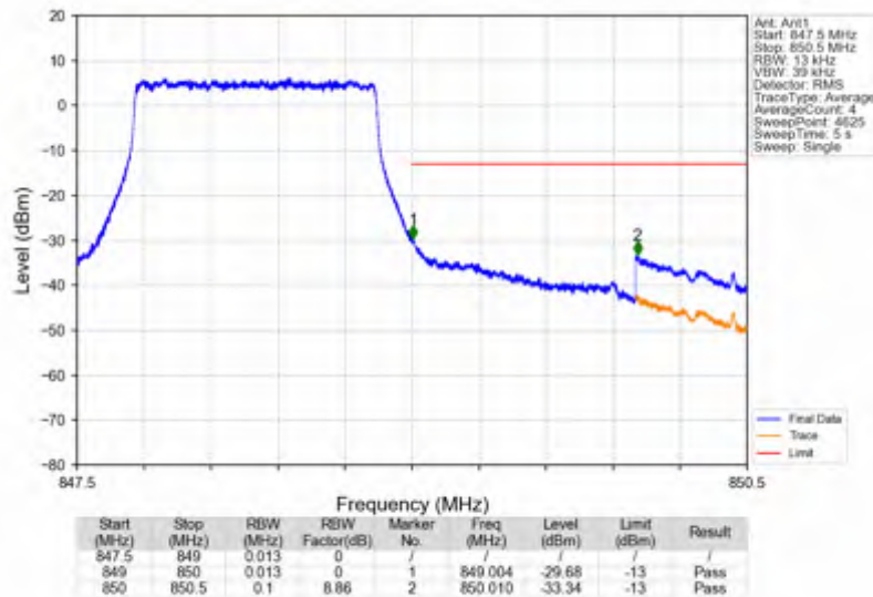
Band5_1.4MHz_QPSK_HCH_848.3MHz_RB_6_0_NTNV
