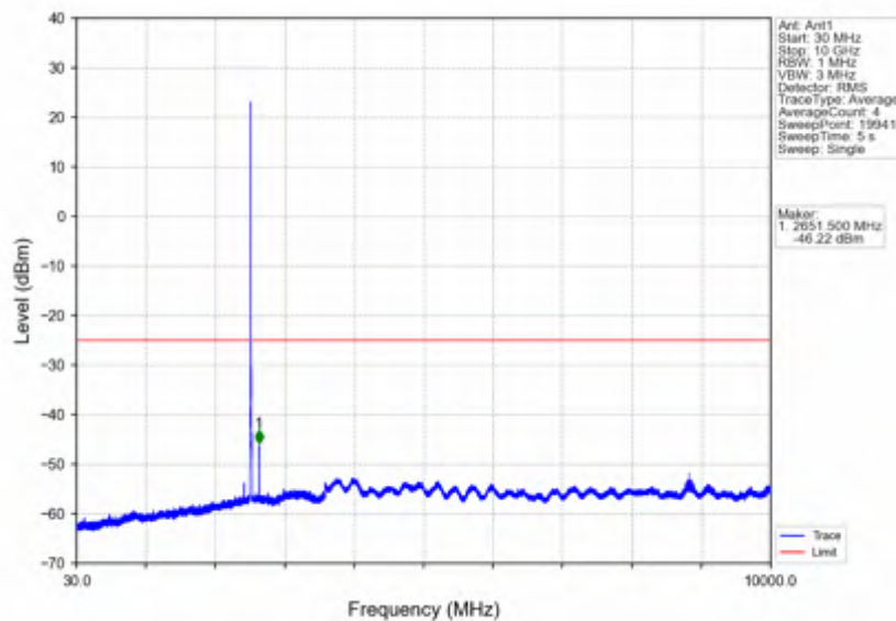
Band7_10MHz_16QAM_MCH_2535MHz_RB_1_0_NTNV
