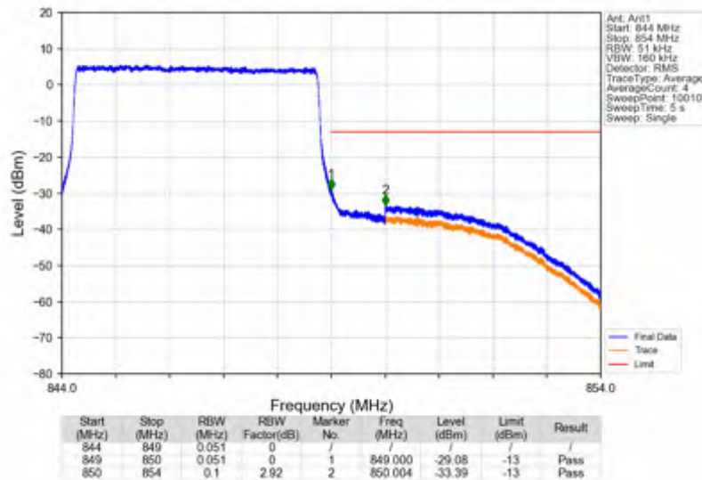
Band5_5MHz_QPSK_HCH_846.5MHz_RB_25_0_NTNV
