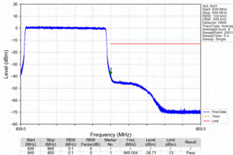
Band5_10MHz_256QAM_HCH_844MHz_RB_50_0_NTNV
