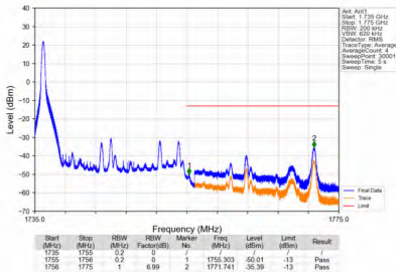
Band4_20MHz_64QAM_HCH_1745MHz_RB_100_0_NTNV
