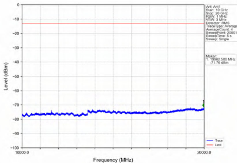
Band4_15MHz_64QAM_MCH_1732.5MHz_RB_1_0_NTNV
