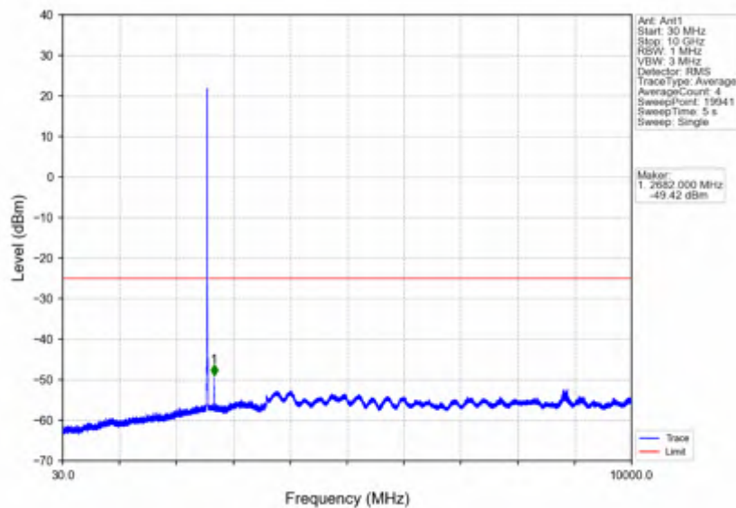
Band7_10MHz_16QAM_HCH_2565MHz_RB_1_0_NTNV
