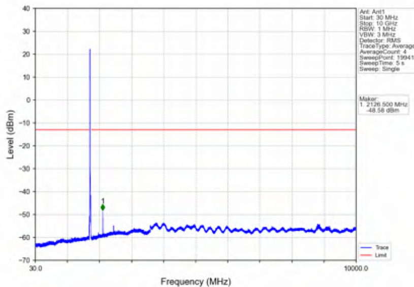
Band4_15MHz_16QAM_MCH_1732.5MHz_RB_1_0_NTNV
