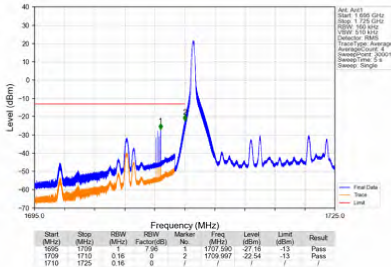
Band4_15MHz_QPSK_LCH_1717.5MHz_RB_75_0_NTNV
