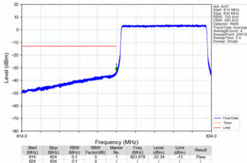
Band5_10MHz_16QAM_LCH_829MHz_RB_50_0_NTNV
