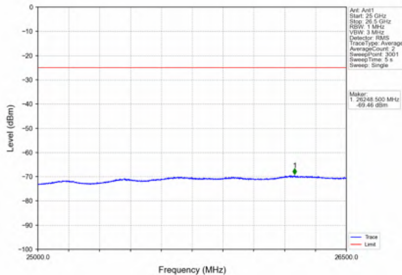
Band7_10MHz_256QAM_HCH_2565MHz_RB_1_0_NTV
