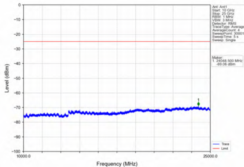
Band7_5MHz_256QAM_HCH_2567.5MHz_RB_1_0_NTNV
