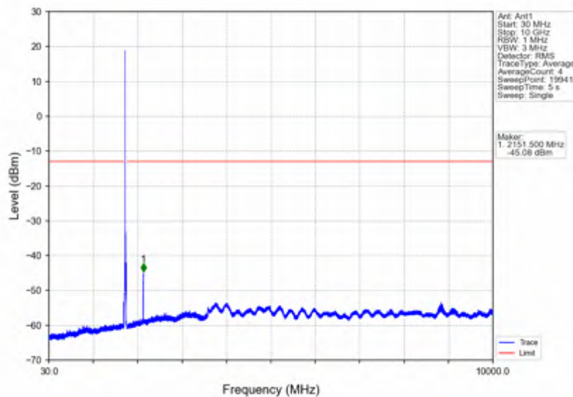
Band4_15MHz_256QAM_HCH_1747.5MHz_RB_1_0_NTNV
