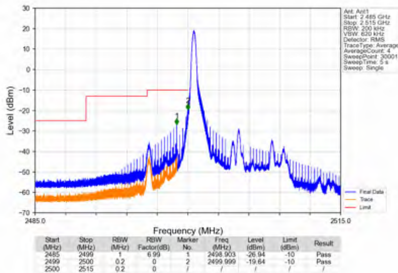
Band7_10MHz_256QAM_LCH_2505MHz_RB_1_0_NTNV
