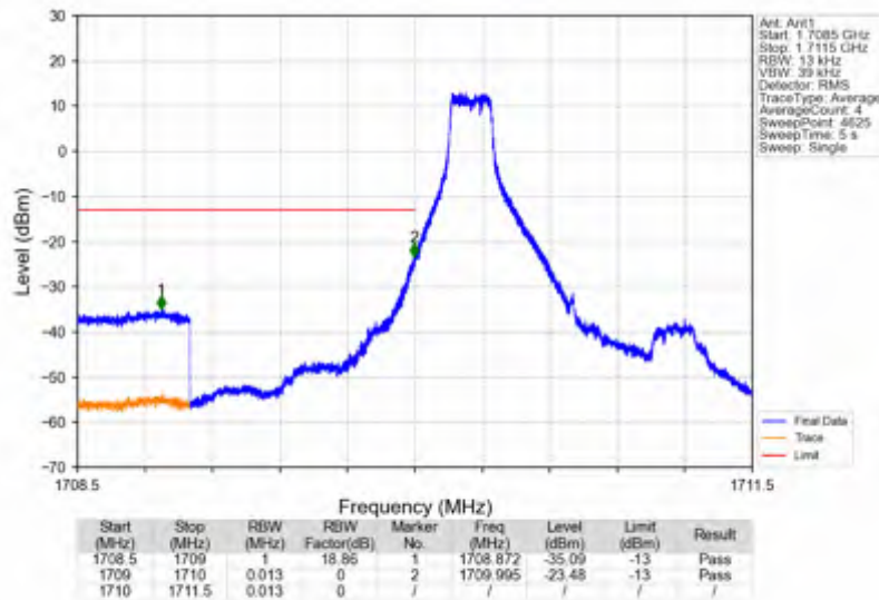
Band4_1.4MHz_16QAM_LCH_1710.7MHz_RB_1_0_NTNV
