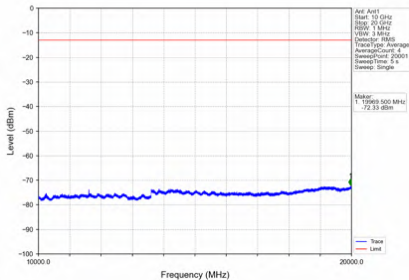
Band2_15MHz_16QAM_LCH_1857.5MHz_RB_75_0_NTNV
