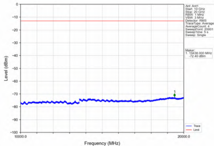
Band4_3MHz_QPSK_LCH_1711.5MHz_RB_15_0_NTNV
