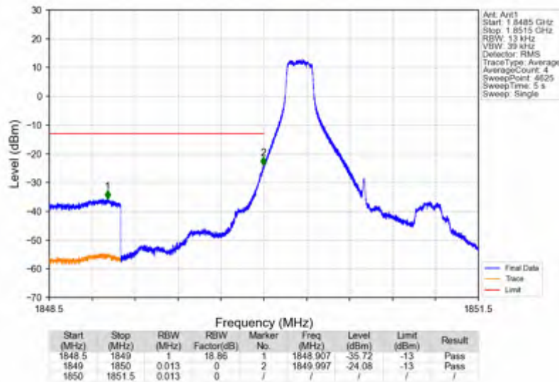
Band2_1.4MHz_16QAM_LCH_1850.7MHz_RB_6_0_NTNV
