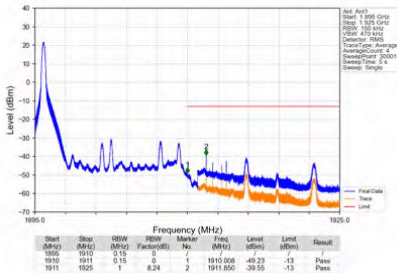
Band2_15MHz_16QAM_HCH_1902.5MHz_RB_75_0_NTNV
