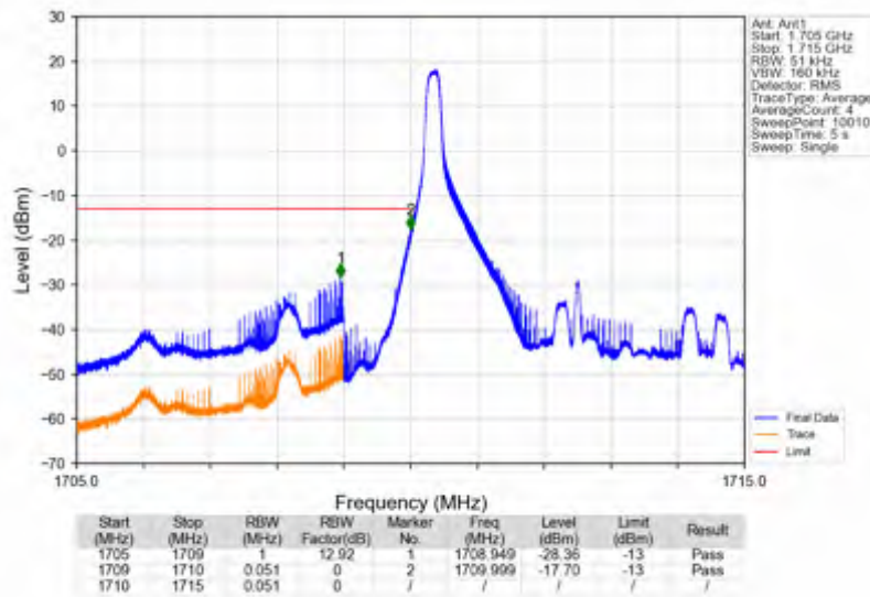
Band4_5MHz_QPSK_LCH_1712.5MHz_RB_1_0_NTNV
