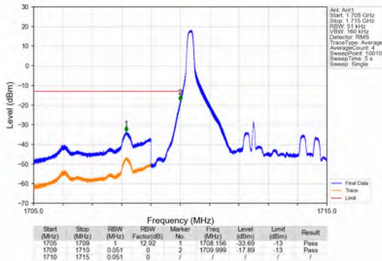
Band4_5MHz_64QAM_LCH_1712.5MHz_RB_1_0_NTNV
