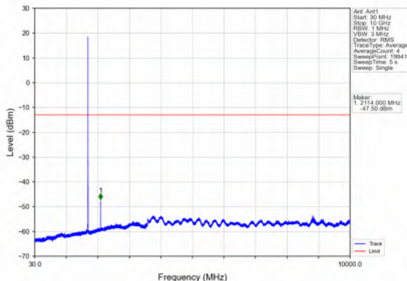
Band4_5MHz_256QAM_LCH_1712.5MHz_RB_1_0_NTNV
