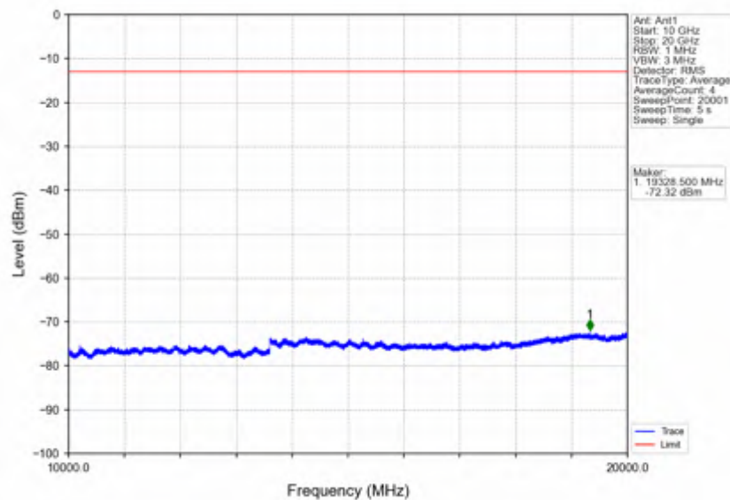
Band2_15MHz_QPSK_LCH_1857.5MHz_RB_75_0_NTNV
