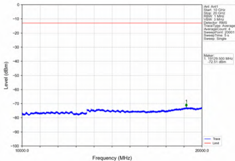
Band2_5MHz_64QAM_LCH_1852.5MHz_RB_25_0_NTNV
