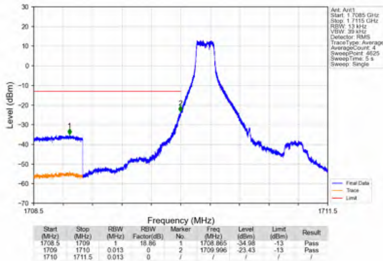
Band4_1.4MHz_16QAM_LCH_1710.7MHz_RB_6_0_NTNV
