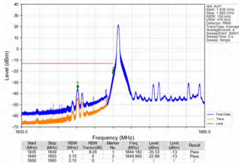
Band2_15MHz_64QAM_LCH_1857.5MHz_RB_75_0_NTNV
