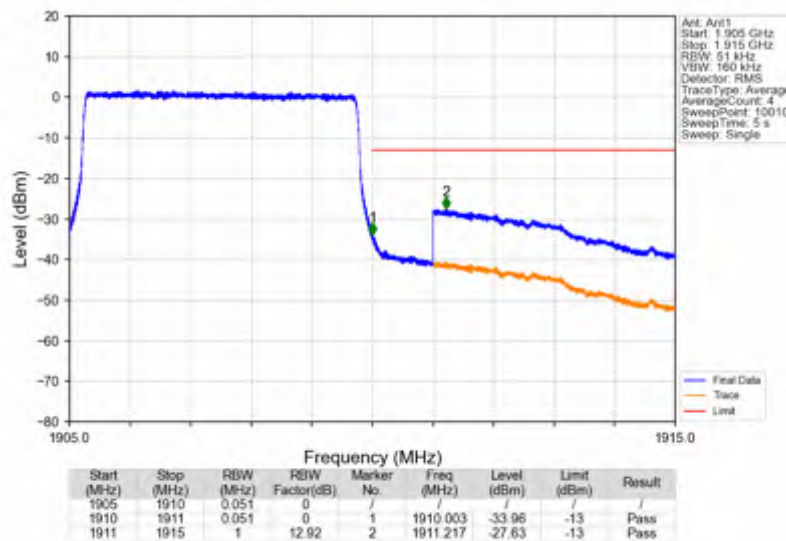
Band2_5MHz_256QAM_HCH_1907.5MHz_RB_25_0_NTNV
