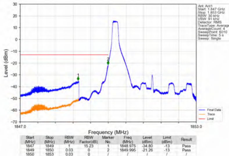
Band2_3MHz_64QAM_LCH_1851.5MHz_RB_15_0_NTNV
