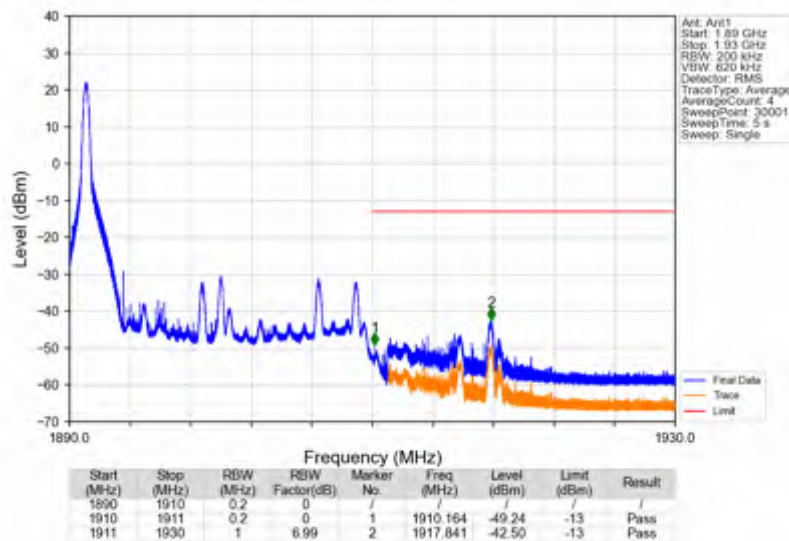
Band2_20MHz_64QAM_HCH_1900MHz_RB_100_0_NTNV
