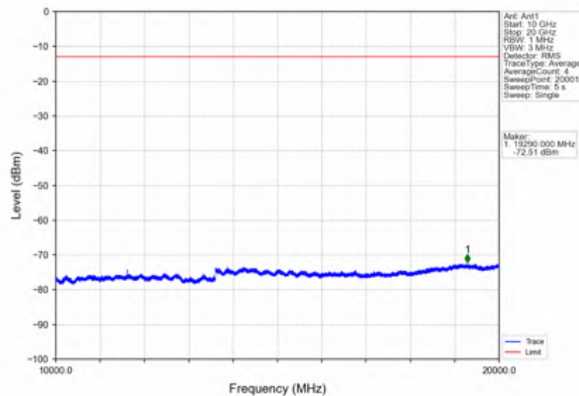
Band2_3MHz_QPSK_LCH_1851.5MHz_RB_15_0_NTNV
