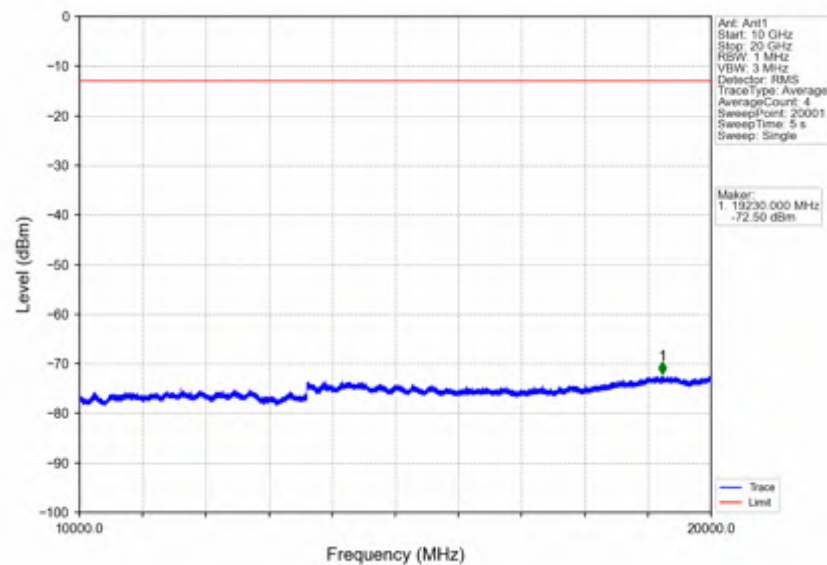
Band2_1.4MHz_QPSK_LCH_1850.7MHz_RB_6_0_NTNV
