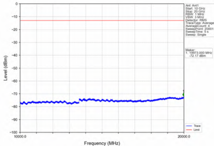
Band4_1.4MHz_16QAM_LCH_1710.7MHz_RB_6_0_NTNV
