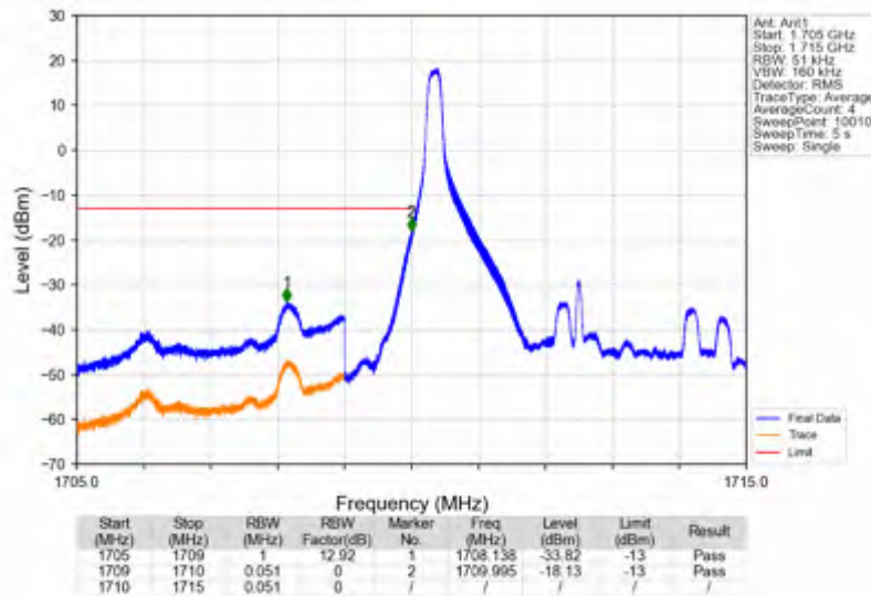
Band4_5MHz_64QAM_LCH_1712.5MHz_RB_25_0_NTNV
