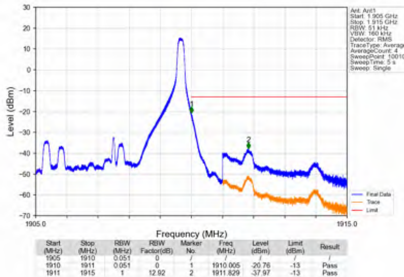
Band2_5MHz_256QAM_HCH_1907.5MHz_RB_1_24_NTNV
