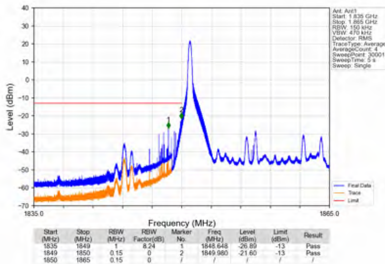
Band2_15MHz_16QAM_LCH_1857.5MHz_RB_75_0_NTNV
