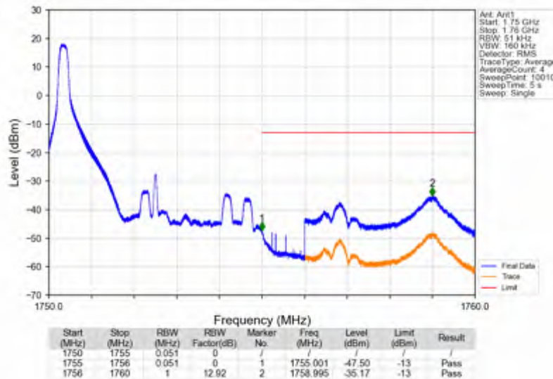
Band4_5MHz_QPSK_HCH_1752.5MHz_RB_1_24_NTNV
