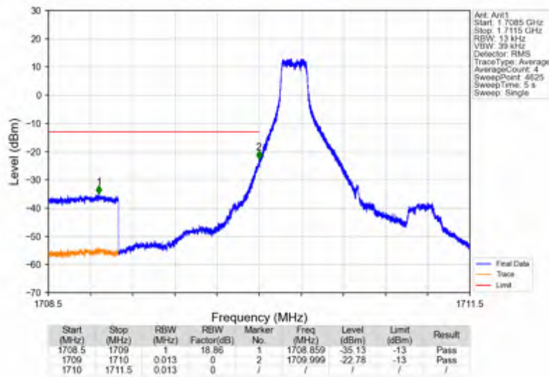
Band4_1.4MHz_QPSK_LCH_1710.7MHz_RB_1_0_NTNV
