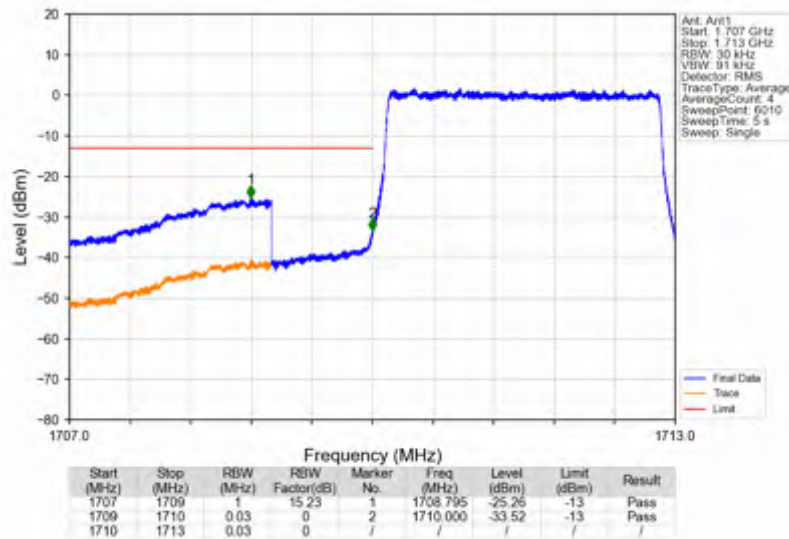
Band4_3MHz_256QAM_LCH_1711.5MHz_RB_15_0_NTNV
