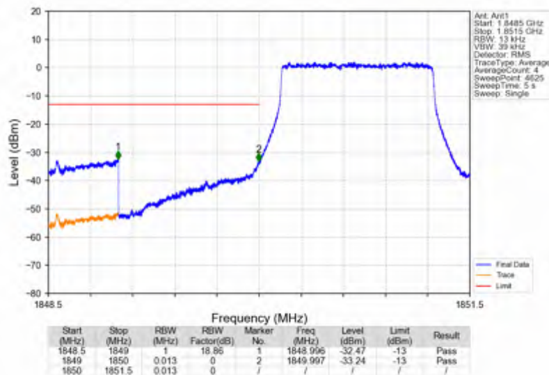
Band2_1.4MHz_256QAM_LCH_1850.7MHz_RB_6_0_NTNV
