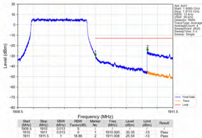
Band2_1.4MHz_QPSK_HCH_1909.3MHz_RB_6_0_NTV
