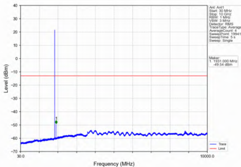
Band2_3MHz_64QAM_LCH_1851.5MHz_RB_1_0_NTNV
