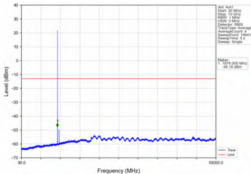
Band2_1.4MHz_64QAM_MCH_1880MHz_RB_1_0_NTV
