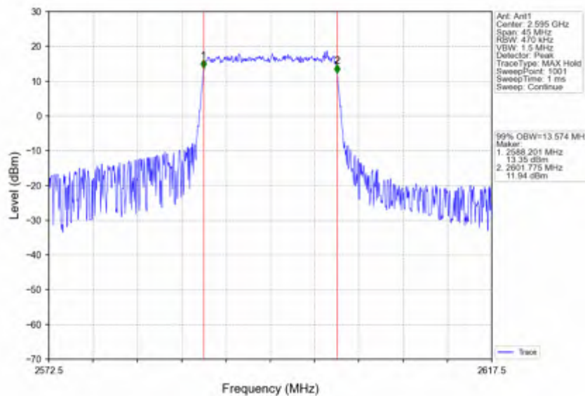
Band38_15MHz_64QAM_MCH_2595MHz_RB_75_0_NTNV
