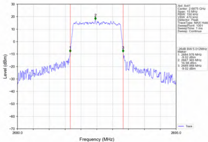
Band41_5MHz_256QAM_HCH_2687.5MHz_RB_25_0_NTNV
