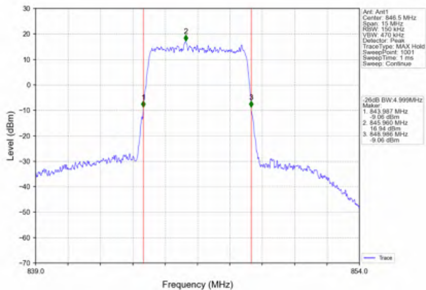
Band26b_5MHz_256QAM_HCH_846.5MHz_RB_25_0_NTNV
