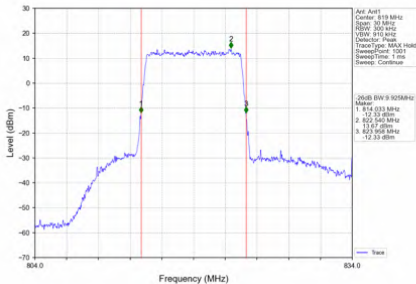
Band26a_10MHz_256QAM_HCH_819MHz_RB_50_0_NTNV
