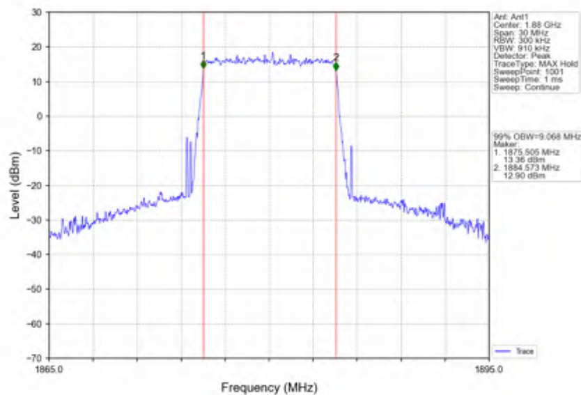
Band2_10MHz_64QAM_MCH_1880MHz_RB_50_0_NTNV
