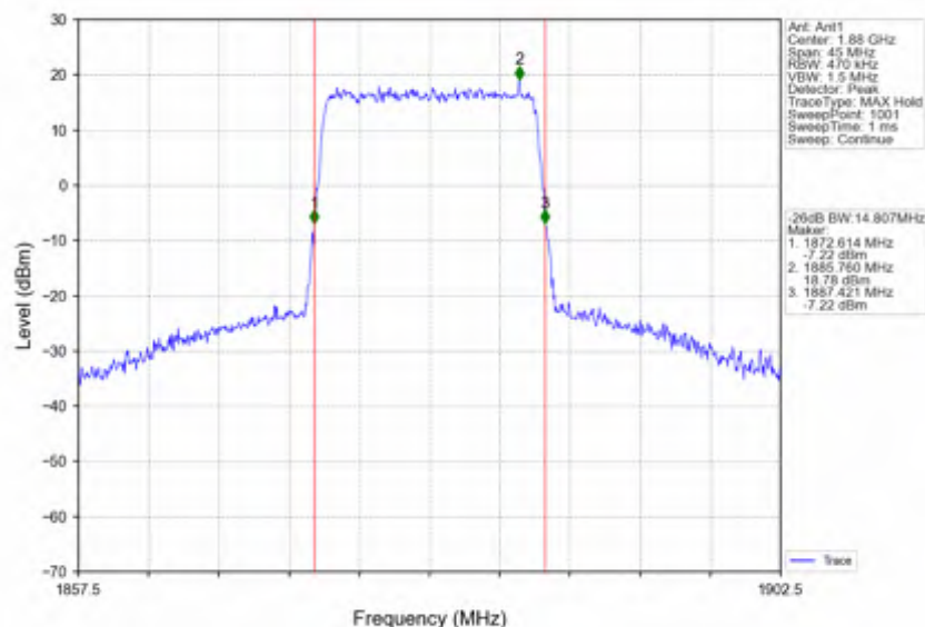
Band2_15MHz_64QAM_MCH_1880MHz_RB_75_0_NTNV
