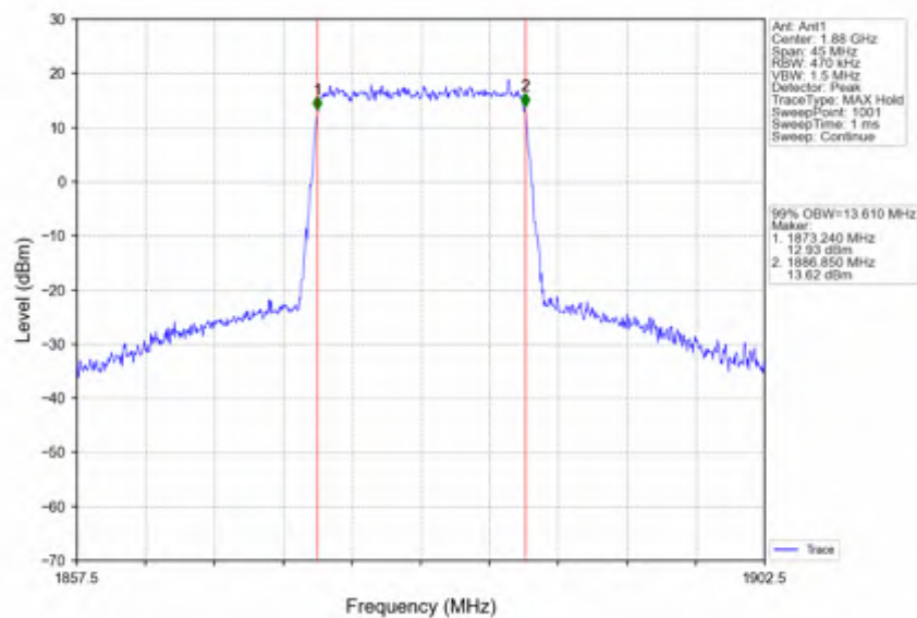
Band2_15MHz_64QAM_MCH_1880MHz_RB_75_0_NTNV
