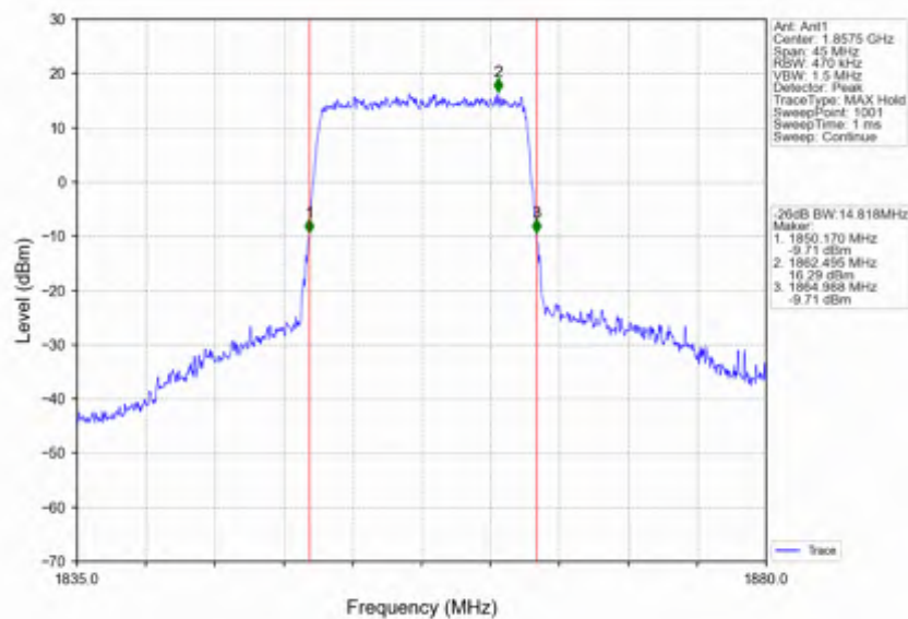
Band2_15MHz_256QAM_LCH_1857.5MHz_RB_75_0_NTNV
