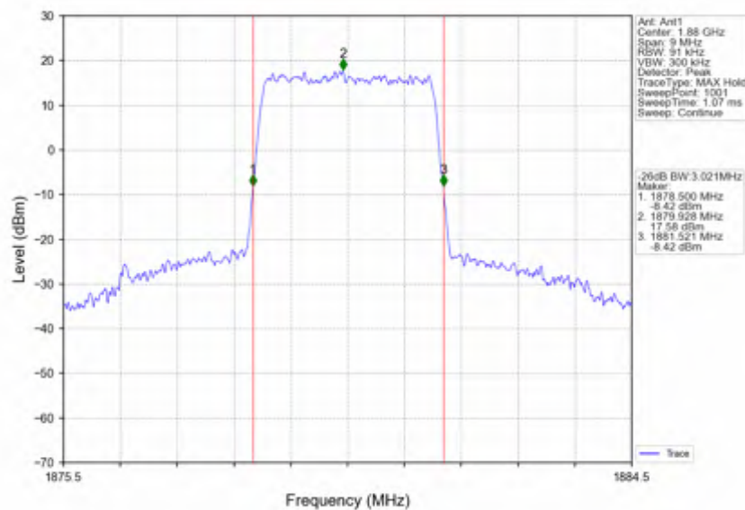
Band2_3MHz_64QAM_MCH_1880MHz_RB_15_0_NTNV
