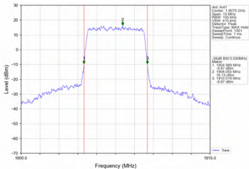
Band2_5MHz_256QAM_HCH_1907.5MHz_RB_25_0_NTNV
