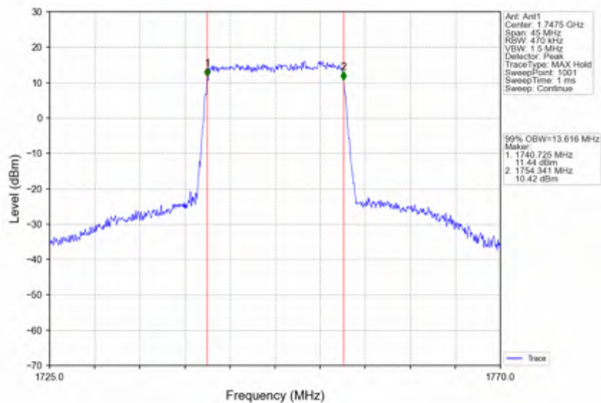
Band4 15MHz 256QAM HCH 1747.5MHz RB 75 0 NTNV
