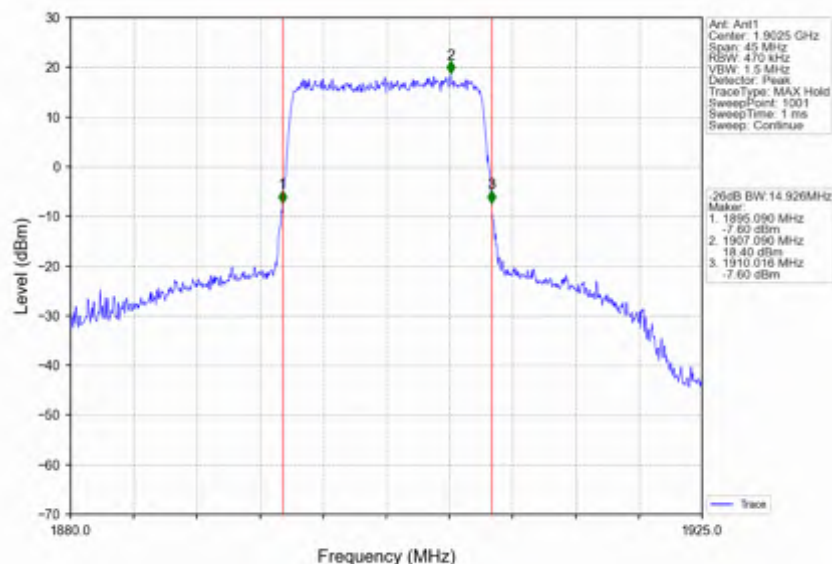
Band2_15MHz_16QAM_HCH_1902.5MHz_RB_75_0_NTNV
