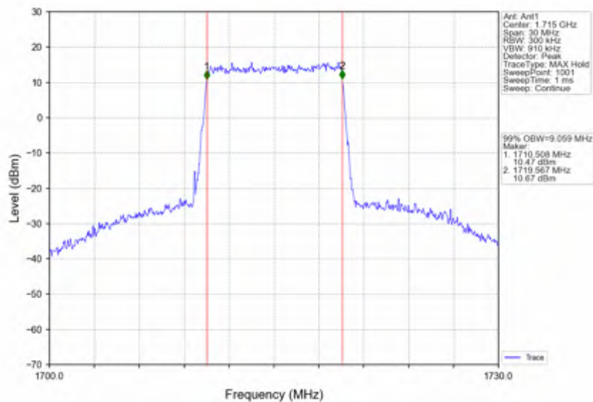
Band4_10MHz_256QAM_LCH_1715MHz_RB_50_0_NTNV
