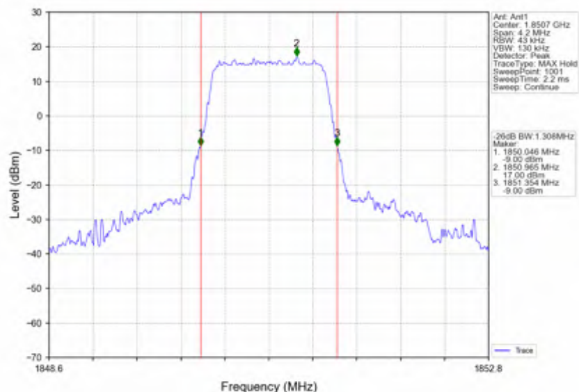
Band2_1.4MHz_256QAM_LCH_1850.7MHz_RB_6_0_NTNV
