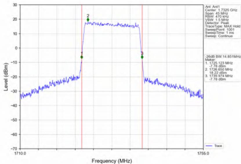
Band4_15MHz_QPSK_MCH_1732.5MHz_RB_75_0_NTNV
