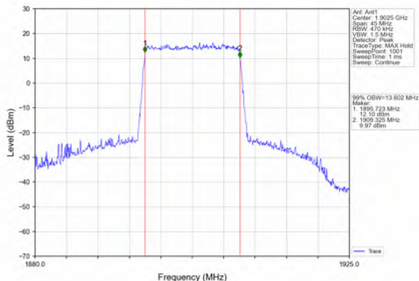
Band2_15MHz_256QAM_HCH_1902.5MHz_RB_75_0_NTNV
