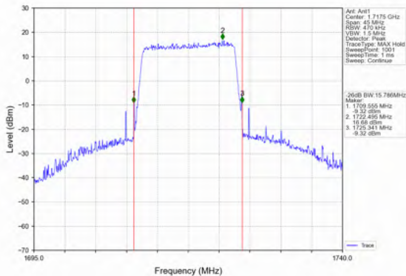
Band4_15MHz_256QAM_LCH_1717.5MHz_RB_75_0_NTNV
