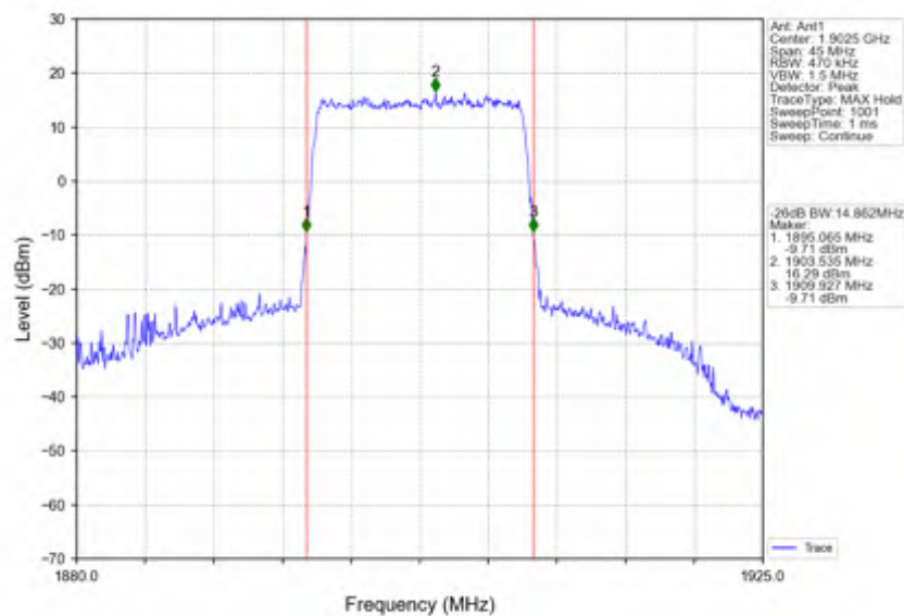
Band2_15MHz_256QAM_HCH_1902.5MHz_RB_75_0_NTNV
