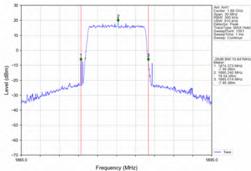
Band2_10MHz_64QAM_MCH_1880MHz_RB_50_0_NTNV
