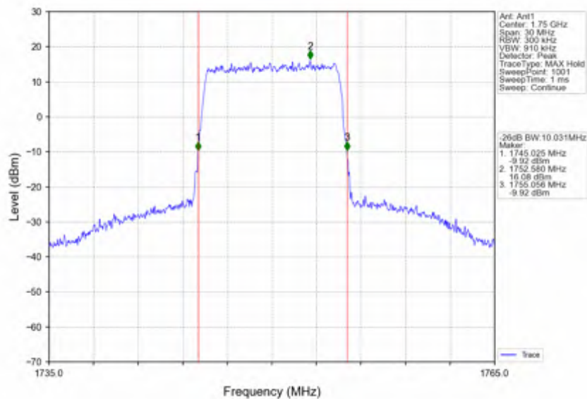
Band4 10MHz 256QAM HCH 1750MHz RB 50 0 NTNV
