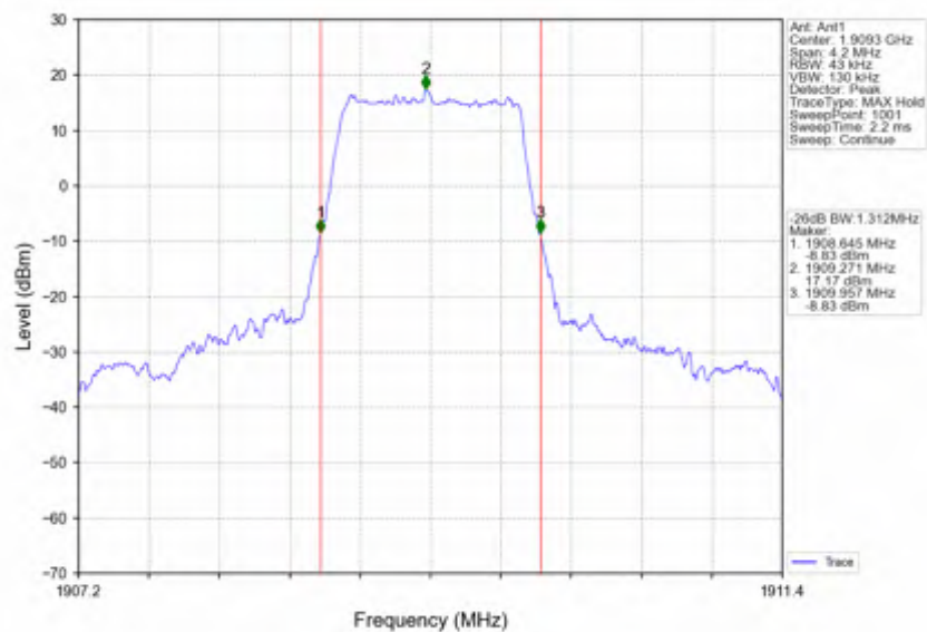
Band2_1.4MHz_256QAM_HCH_1909.3MHz_RB_6_0_NTNV
