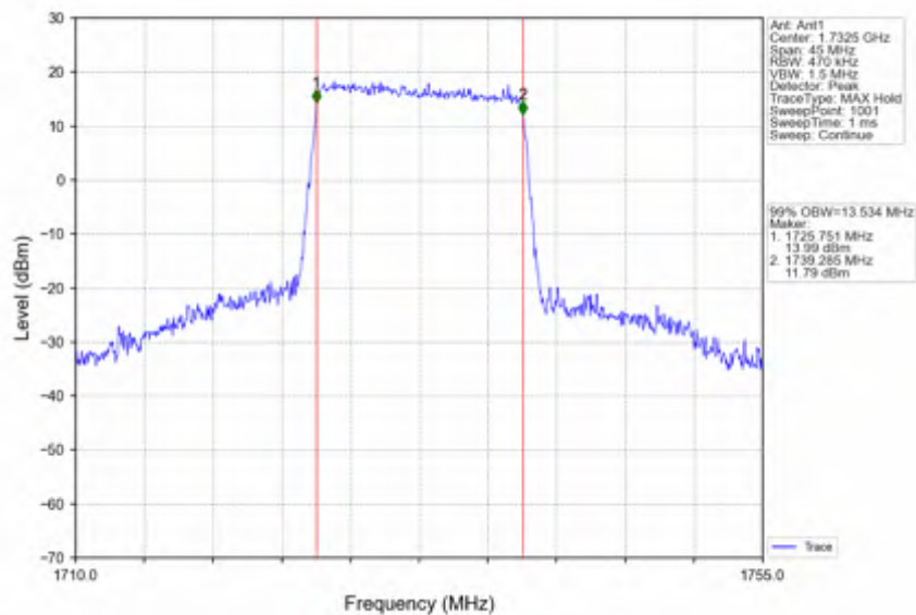
Band4_15MHz_64QAM_MCH_1732.5MHz_RB_75_0_NTNV
