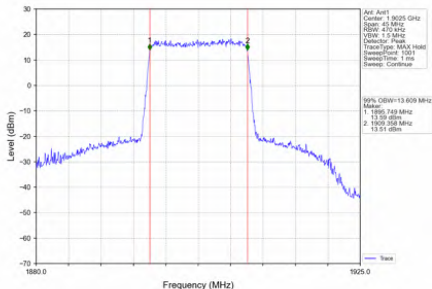
Band2_15MHz_16QAM_HCH_1902.5MHz_RB_75_0_NTNV
