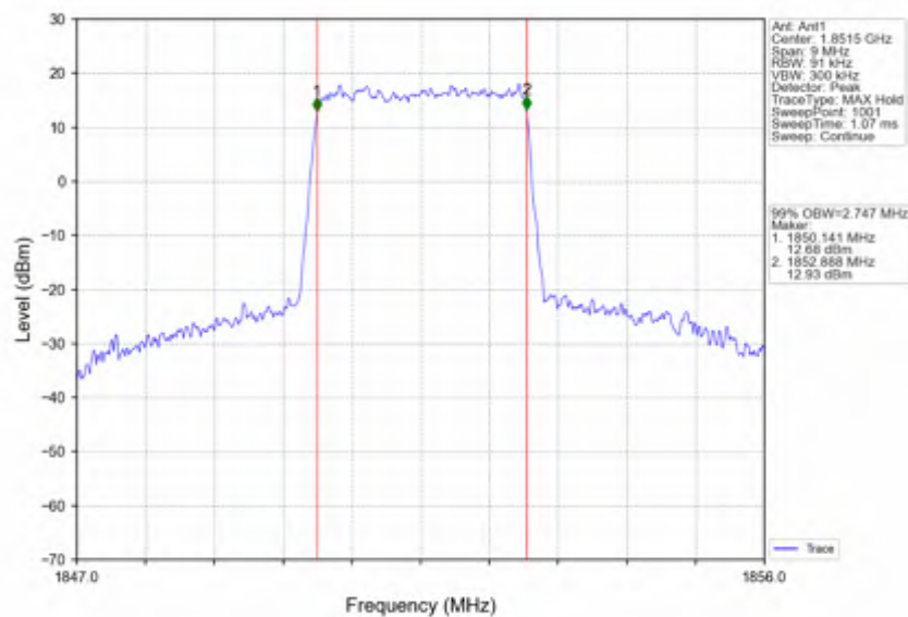
Band2_3MHz_16QAM_LCH_1851.5MHz_RB_15_0_NTNV
