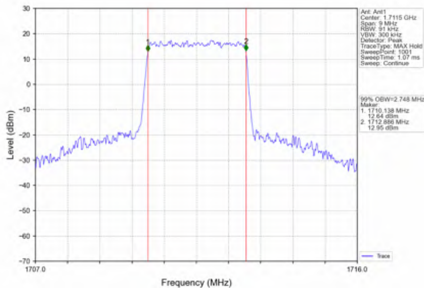
Band4_3MHz_16QAM_LCH_1711.5MHz_RB_15_0_NTNV
