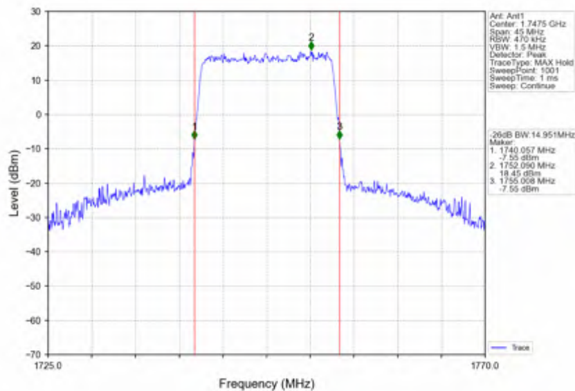
Band4_15MHz_16QAM_HCH_1747.5MHz_RB_75_0_NTNV
