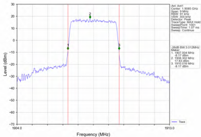
Band2_3MHz_16QAM_HCH_1908.5MHz_RB_15_0_NTNV
