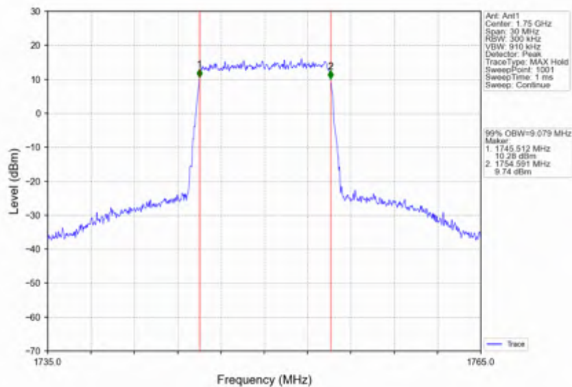
Band4_10MHz_256QAM_HCH_1750MHz_RB_50_0_NTNV
