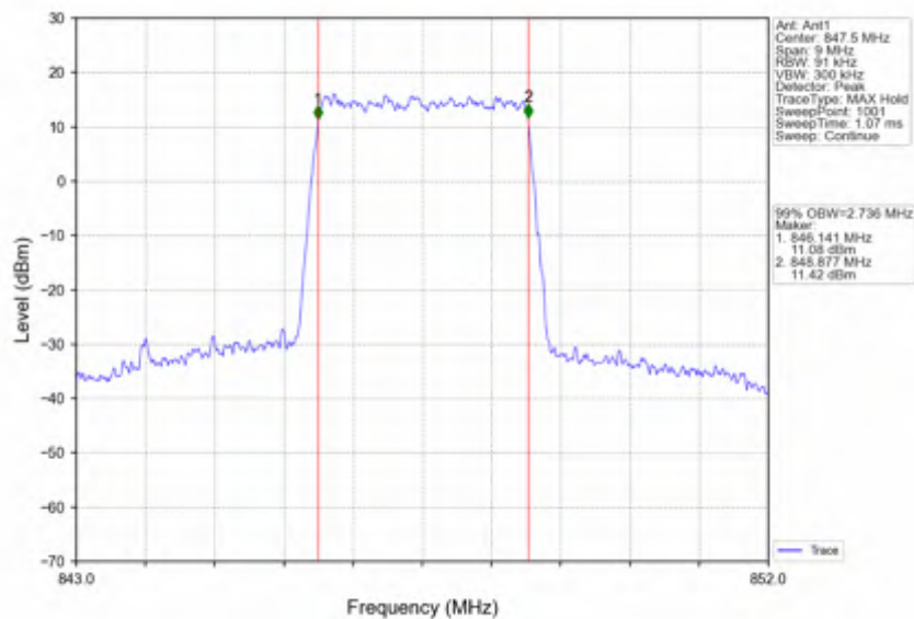
Band5_3MHz_256QAM_HCH_847.5MHz_RB_15_0_NTNV
