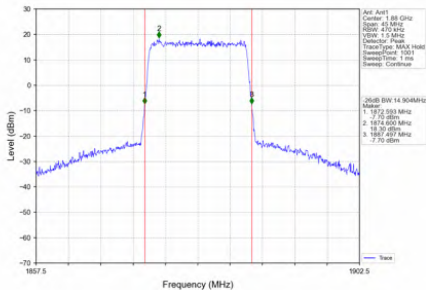
Band2_15MHz_QPSK_MCH_1880MHz_RB_75_0_NTNV
