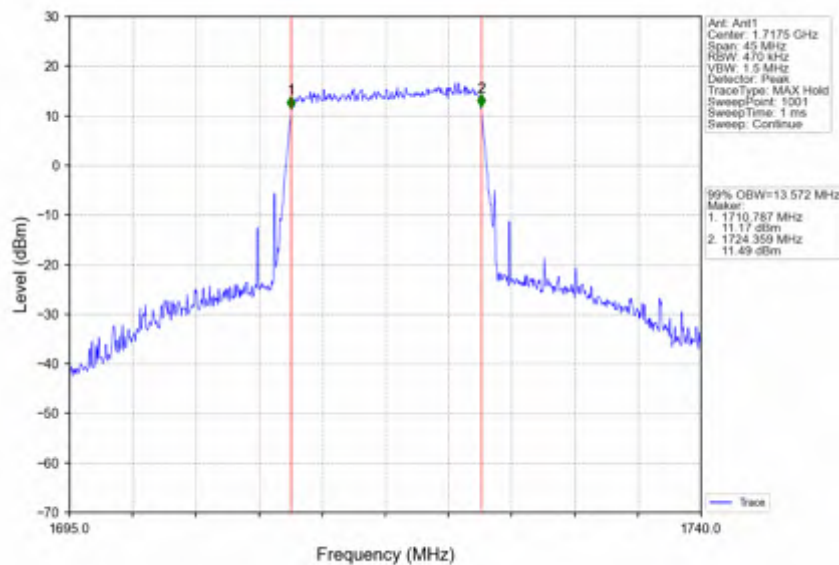
Band4_15MHz_256QAM_LCH_1717.5MHz_RB_75_0_NTNV
