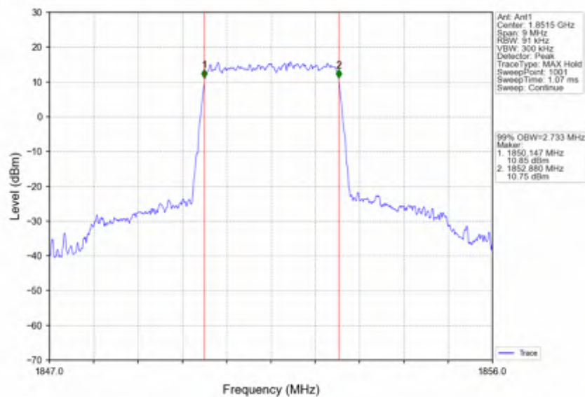
Band2_3MHz_256QAM_LCH_1851.5MHz_RB_15_0_NTNV
