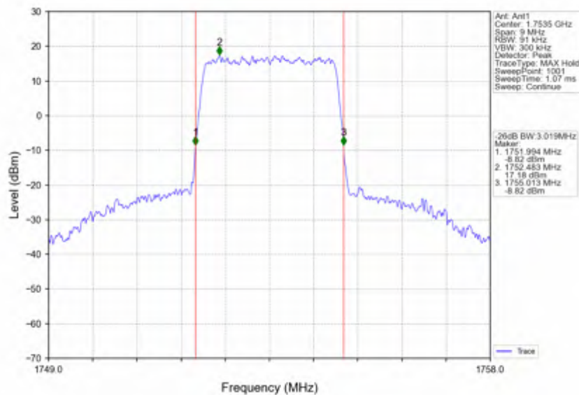
Band4_3MHz_16QAM_HCH_1753.5MHz_RB_15_0_NTNV
