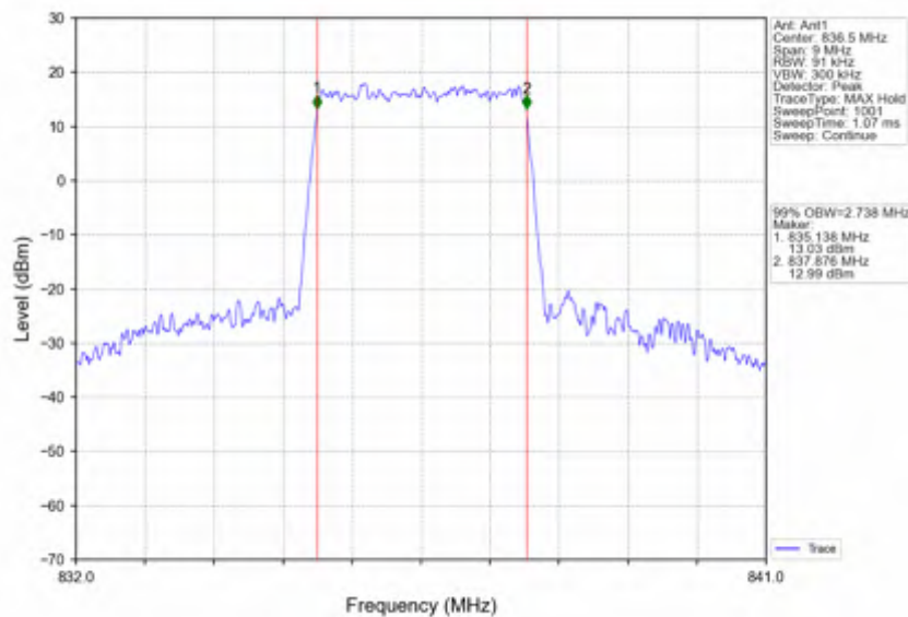
Band5_3MHz_QPSK_MCH_836.5MHz_RB_15_0_NTNV
