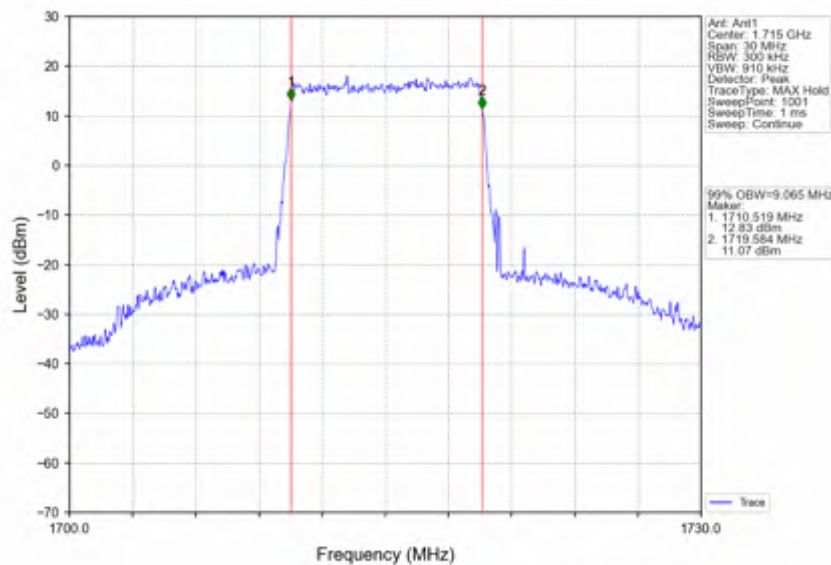
Band4_10MHz_16QAM_LCH_1715MHz_RB_50_0_NTNV
