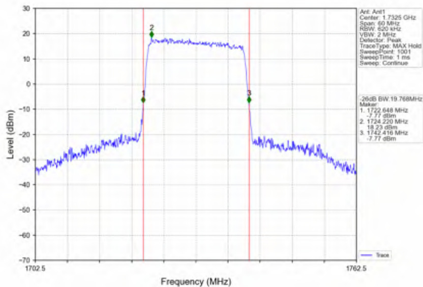
Band4_20MHz_64QAM_MCH_1732.5MHz_RB_100_0_NTNV
