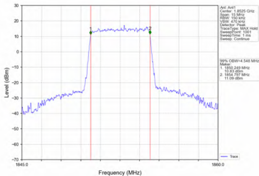
Band2_5MHz_256QAM_LCH_1852.5MHz_RB_25_0_NTNV
