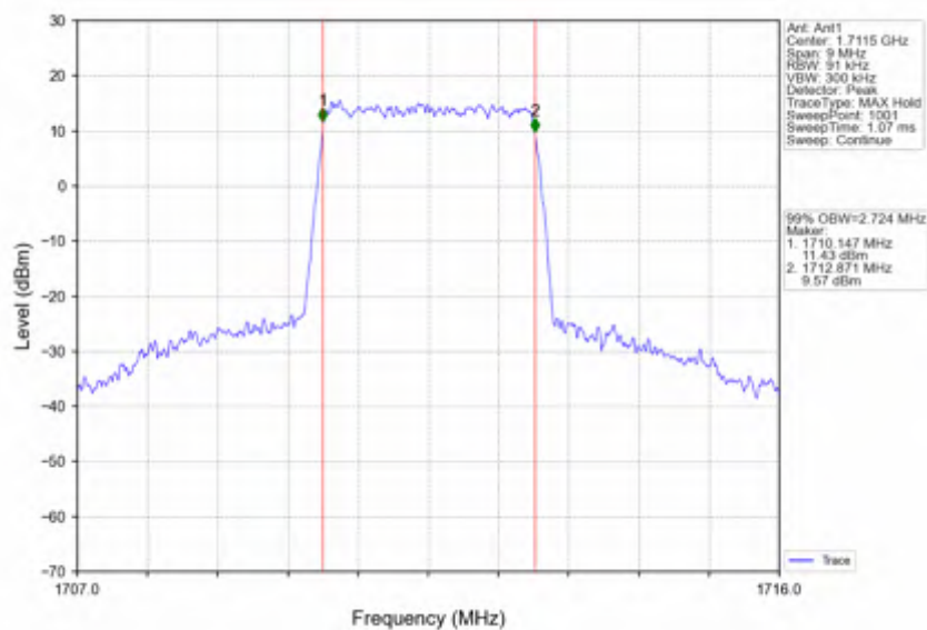
Band4 3MHz 256QAM LCH 1711.5MHz RB 15 0 NTNV
