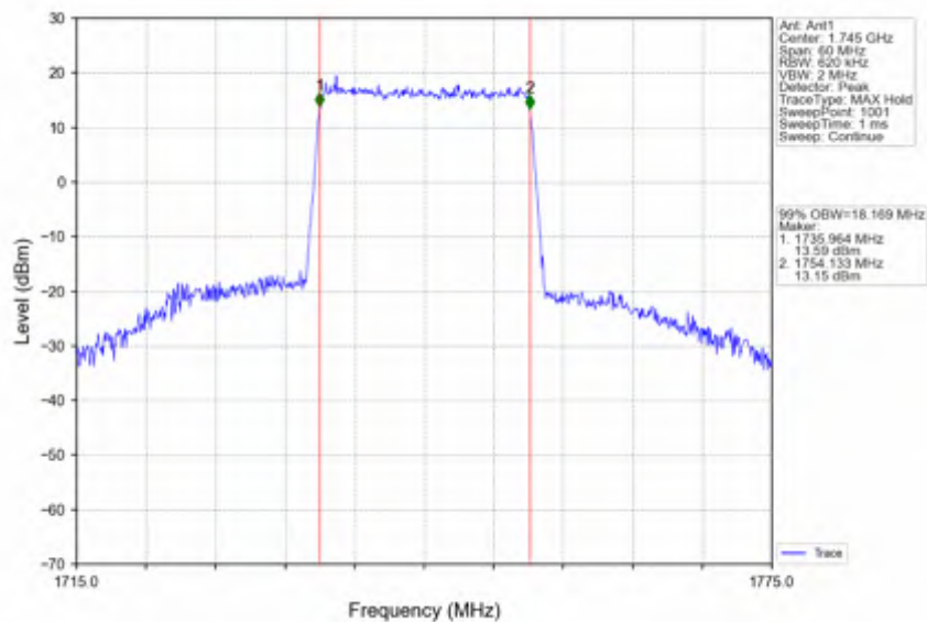
Band4_20MHz_16QAM_HCH_1745MHz_RB_100_0_NTNV
