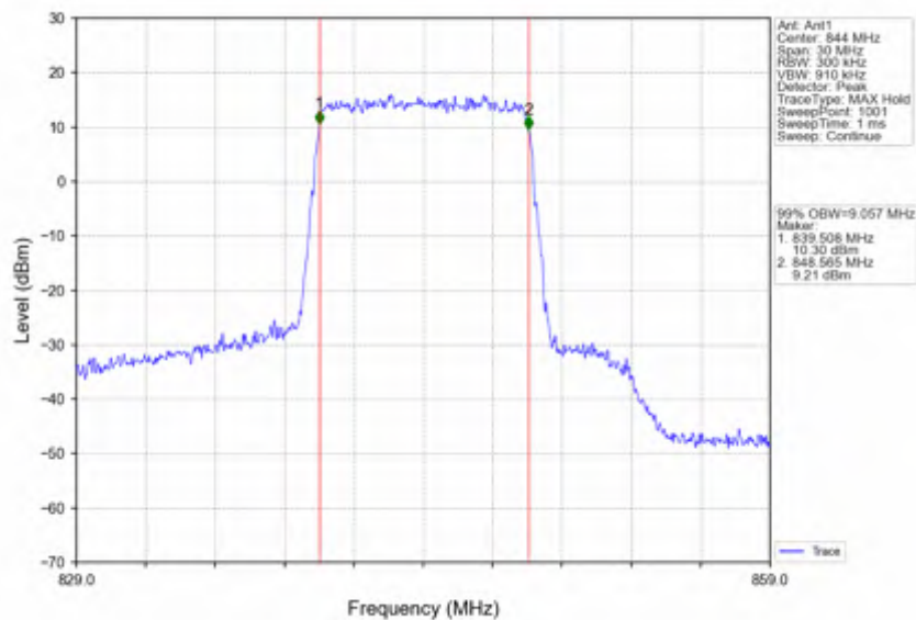
Band5_10MHz_256QAM_HCH_844MHz_RB_50_0_NTNV
