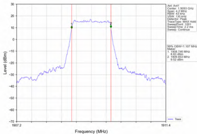
Band2_1.4MHz_256QAM_HCH_1909.3MHz_RB_6_0_NTNV
