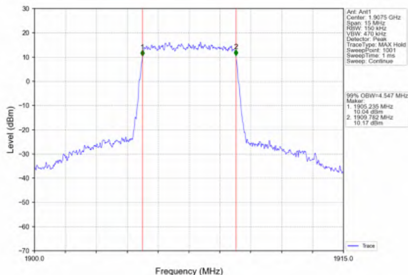
Band2_5MHz_256QAM_HCH_1907.5MHz_RB_25_0_NTNV
