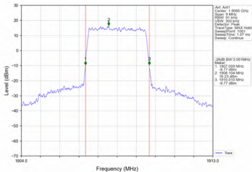
Band2_3MHz_256QAM_HCH_1908.5MHz_RB_15_0_NTNV
