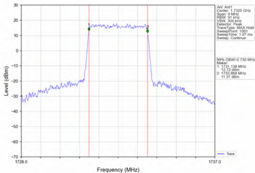
Band4_3MHz_QPSK_MCH_1732.5MHz_RB_15_0_NTNV
