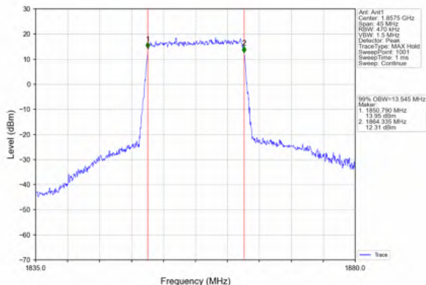
Band2_15MHz_16QAM_LCH_1857.5MHz_RB_75_0_NTNV
