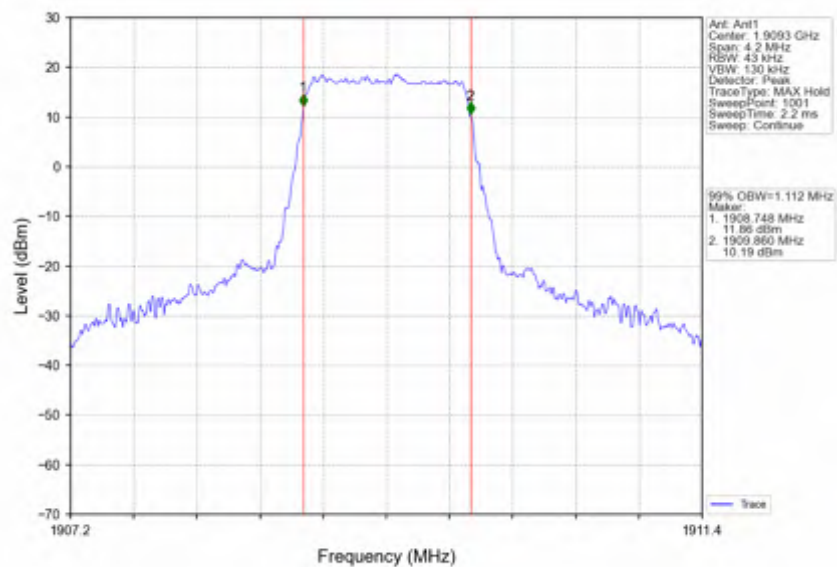
Band2_1.4MHz_16QAM_HCH_1909.3MHz_RB_6_0_NTNV
