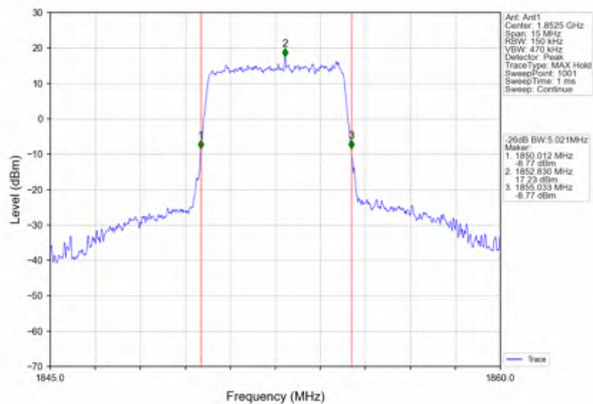
Band2_5MHz_256QAM_LCH_1852.5MHz_RB_25_0_NTNV
