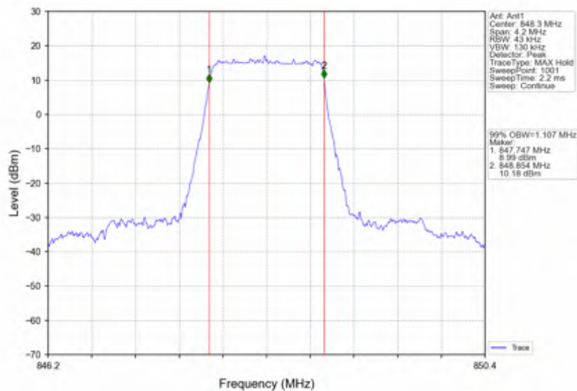
Band5_1.4MHz_256QAM_HCH_848.3MHz_RB_6_0_NTNV
