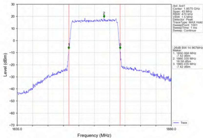
Band2_15MHz_16QAM_LCH_1857.5MHz_RB_75_0_NTNV
