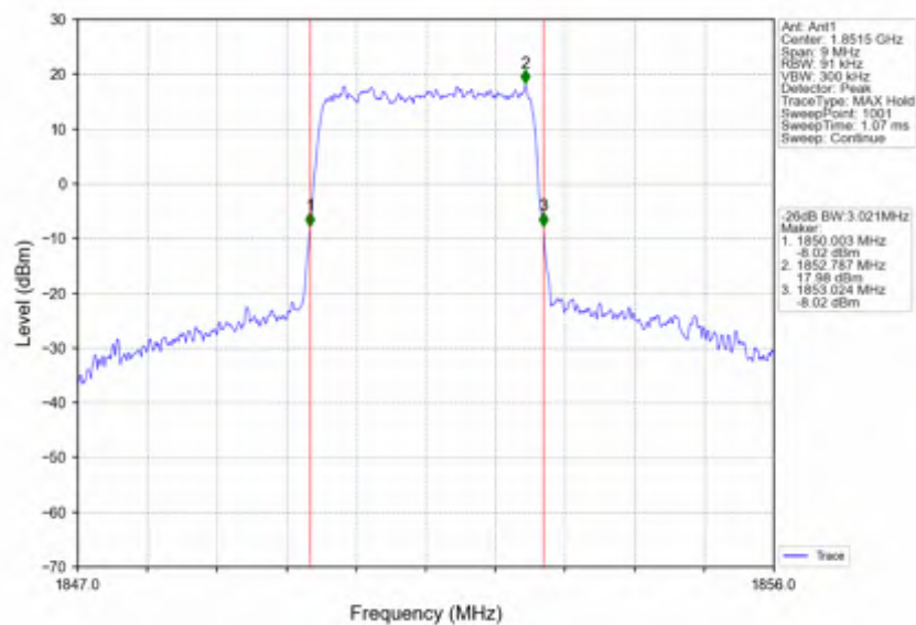
Band2_3MHz_16QAM_LCH_1851.5MHz_RB_15_0_NTNV
