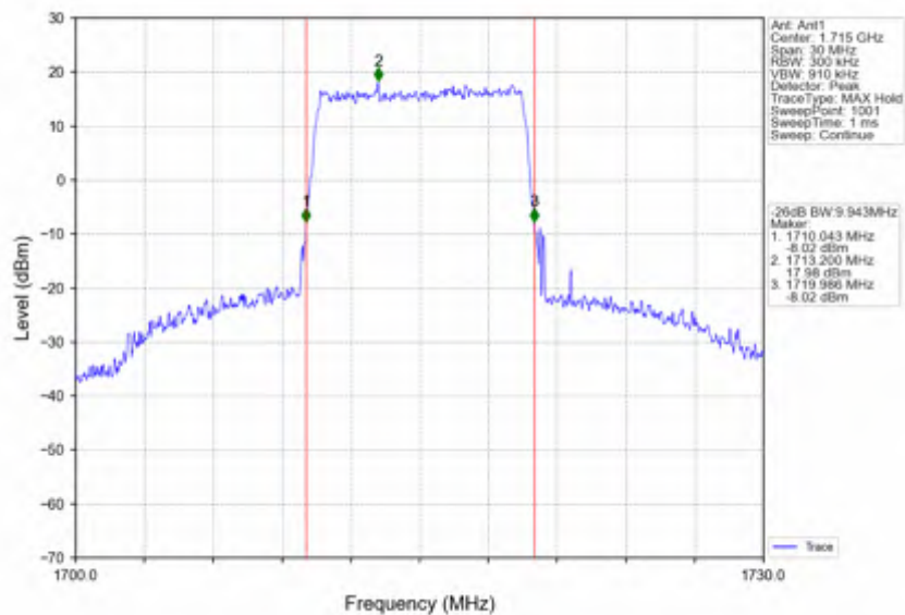
Band4 10MHz 16QAM LCH 1715MHz RB 50 0 NTNV
