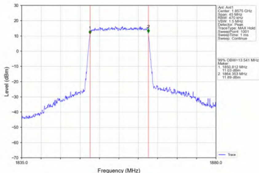
Band2_15MHz_256QAM_LCH_1857.5MHz_RB_75_0_NTNV
