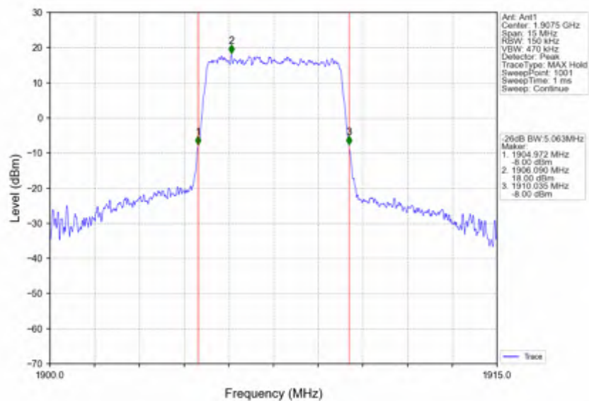
Band2_5MHz_16QAM_HCH_1907.5MHz_RB_25_0_NTNV
