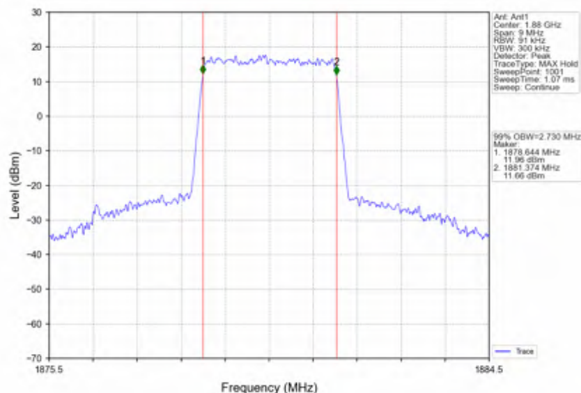
Band2_3MHz_64QAM_MCH_1880MHz_RB_15_0_NTNV
