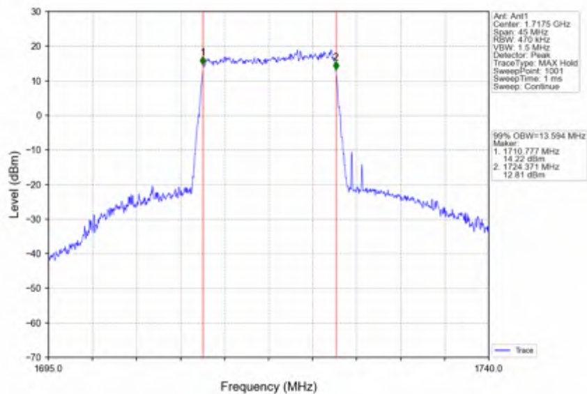
Band4_15MHz_16QAM_LCH_1717.5MHz_RB_75_0_NTNV
