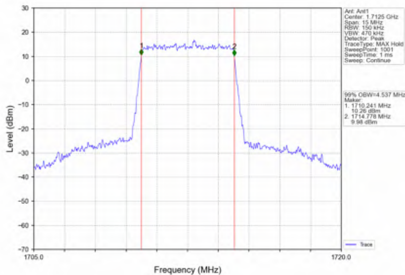
Band4_5MHz_256QAM_LCH_1712.5MHz_RB_25_0_NTNV
