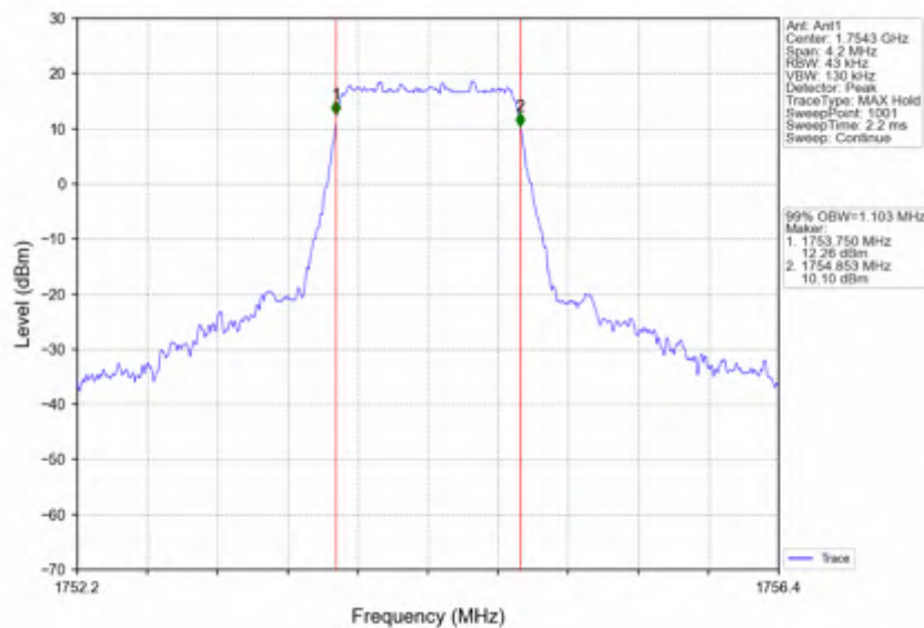
Band4 1.4MHz 16QAM HCH 1754.3MHz RB 6 0 NTN
