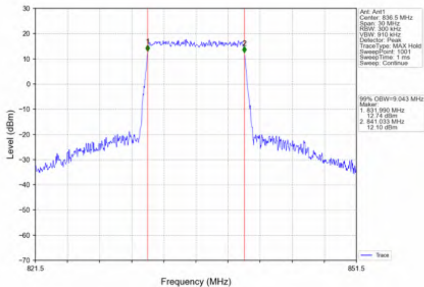
Band5_10MHz_64QAM_MCH_836.5MHz_RB_50_0_NTNV
