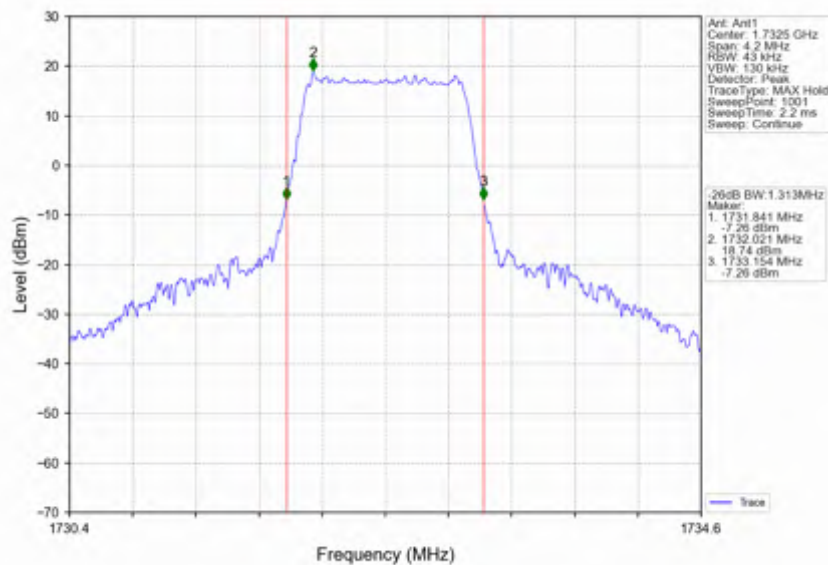
Band4_1.4MHz_64QAM_MCH_1732.5MHz_RB_6_0_NTNV
