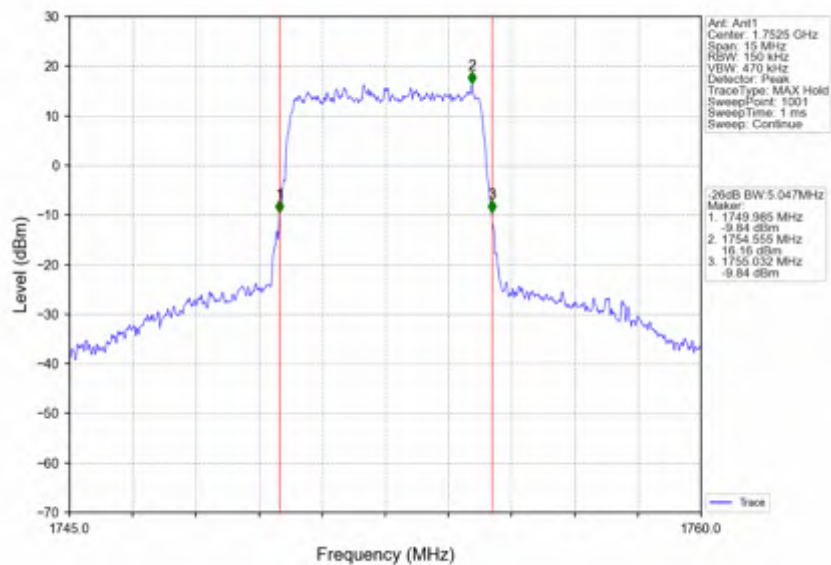
Band4_5MHz_256QAM_HCH_1752.5MHz_RB_25_0_NTNV
