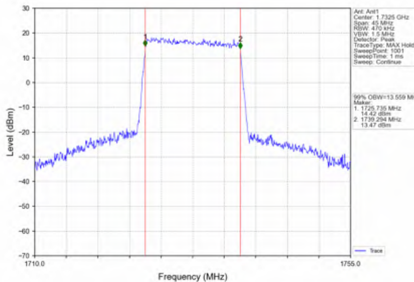
Band4_15MHz_QPSK_MCH_1732.5MHz_RB_75_0_NTNV
