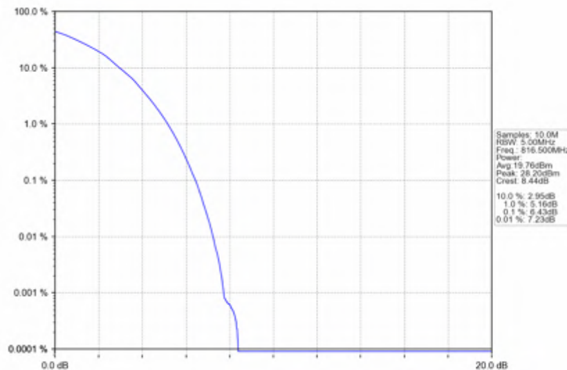
Band26a_5MHz_16QAM_LCH_816.5MHz_RB_25_0_NTNV
