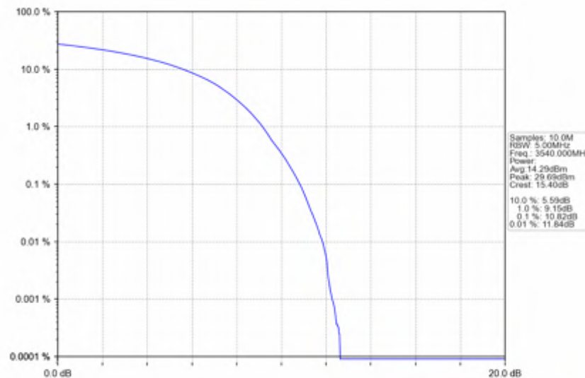
Band42a_20MHz_16QAM_HCH_3540MHz_RB_100_0_NTNV
