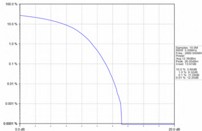
Band41_20MHz_256QAM_HCH_2680MHz_RB_100_0_NTNV
