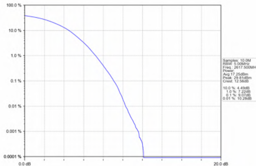
Band38_5MHz_256QAM_HCH_2617.5MHz_RB_25_0_NTNV
