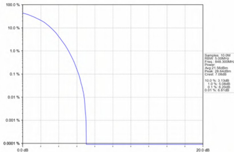
Band26b_1.4MHz_QPSK_HCH_848.3MHz_RB_6_0_NTNV
