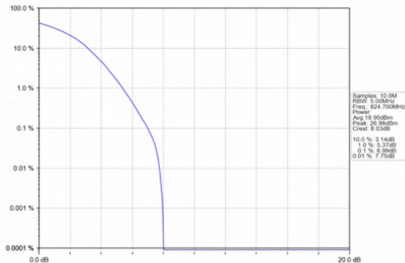
Band26b_1.4MHz_256QAM_LCH_824.7MHz_RB_6_0_NTNV
