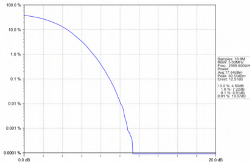
Band38_5MHz_256QAM_MCH_2595MHz_RB_25_0_NTNV
