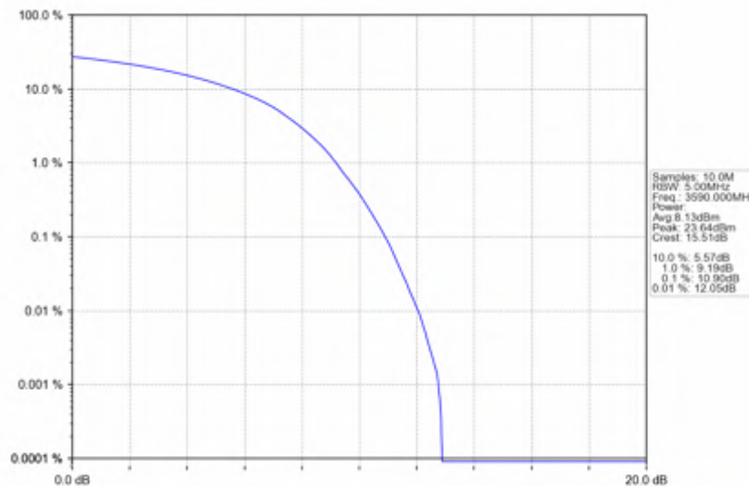
Band42c_20MHz_256QAM_HCH_3590MHz_RB_100_0_NTNV
