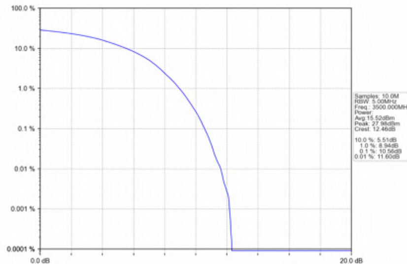
Band42a_15MHz_64QAM_MCH_3500MHz_RB_75_0_NTNV
