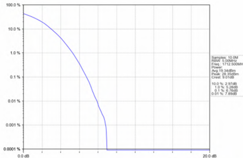
Band66_5MHz_256QAM_LCH_1712.5MHz_RB_25_0_NTNV
