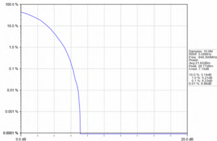
Band26b_1.4MHz_64QAM_HCH_848.3MHz_RB_6_0_NTNV
