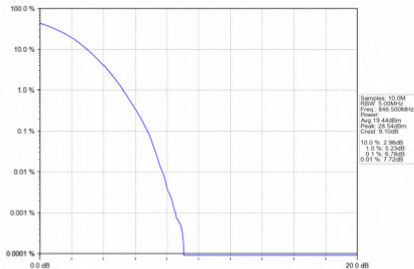
Band26b_5MHz_256QAM_HCH_846.5MHz_RB_25_0_NTNV
