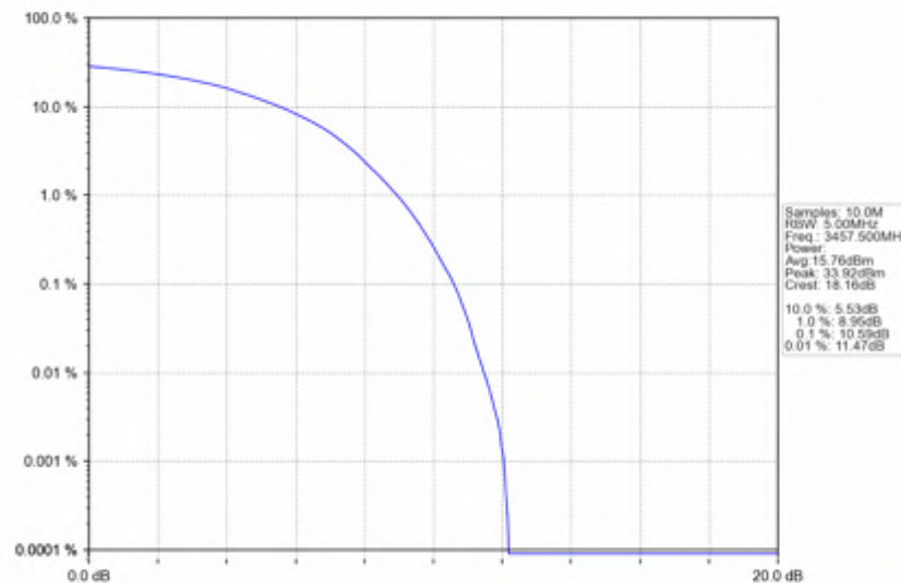
Band42a_15MHz_64QAM_LCH_3457.5MHz_RB_75_0_NTNV
