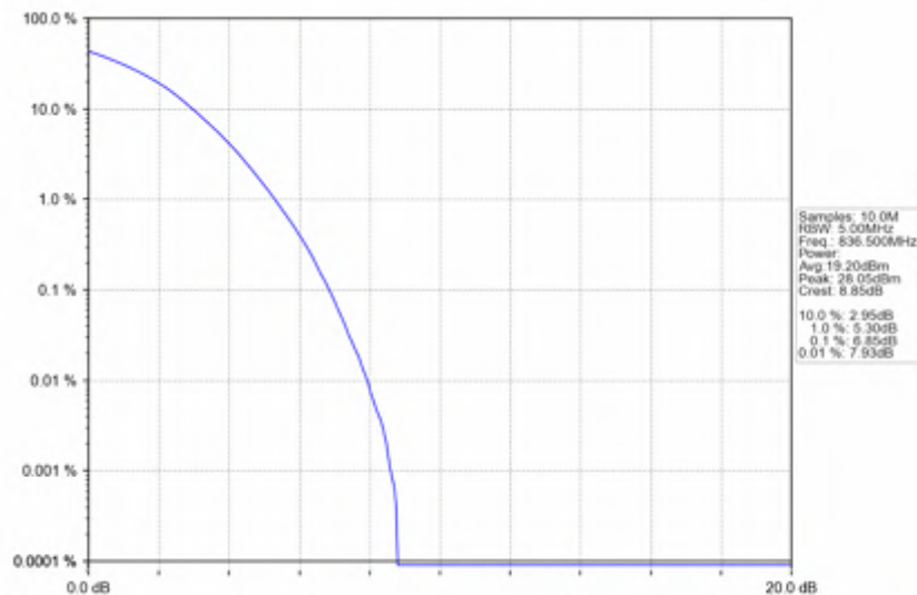
Band26b_5MHz_256QAM_MCH_836.5MHz_RB_25_0_NTNV
