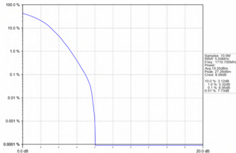
Band66_1.4MHz_256QAM_LCH_1710.7MHz_RB_6_0_NTNV
