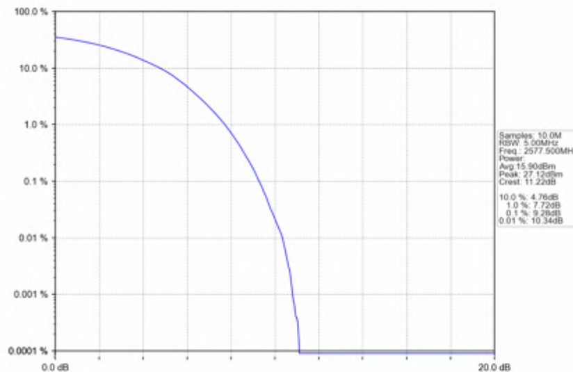
Band38_15MHz_64QAM_LCH_2577.5MHz_RB_75_0_NTNV
