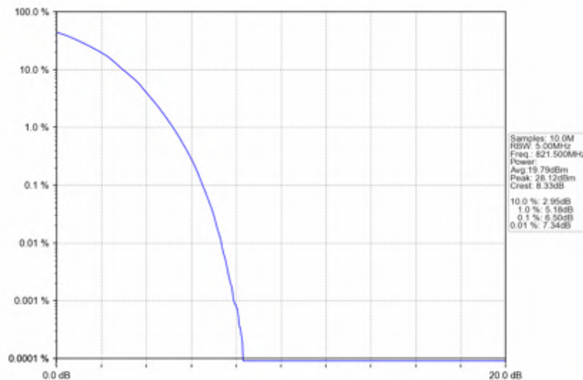
Band26a_5MHz_QPSK_HCH_821.5MHz_RB_25_0_NTNV
