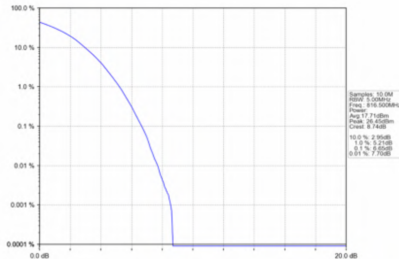
Band26a_5MHz_256QAM_LCH_816.5MHz_RB_25_0_NTNV
