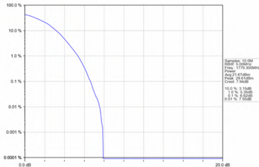
Band66_1.4MHz_64QAM_HCH_1779.3MHz_RB_6_0_NTNV
