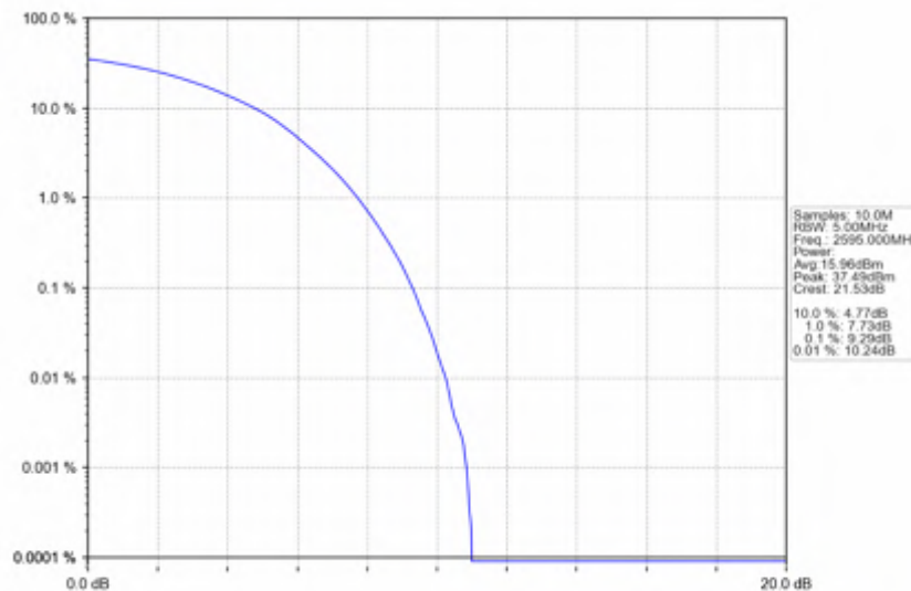
Band38_15MHz_64QAM_MCH_2595MHz_RB_75_0_NTNV
