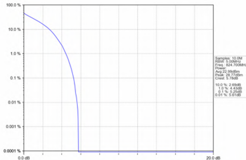
Band26b_1.4MHz_16QAM_LCH_824.7MHz_RB_6_0_NTNV
