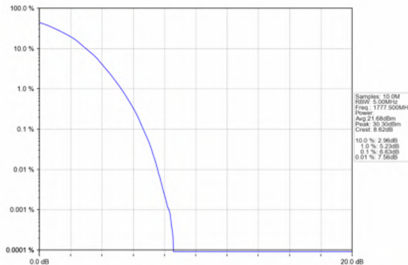
Band66_5MHz_64QAM_HCH_1777.5MHz_RB_25_0_NTNV
