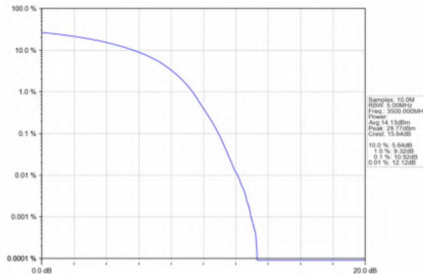
Band42a_20MHz_16QAM_MCH_3500MHz_RB_100_0_NTNV
