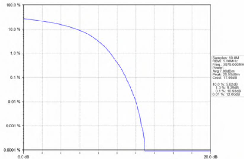
Band42c_20MHz_256QAM_MCH_3575MHz_RB_100_0_NTNV
