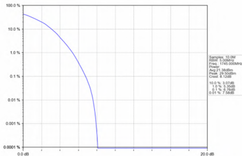
Band66_3MHz_QPSK_MCH_1745MHz_RB_15_0_NTNV
