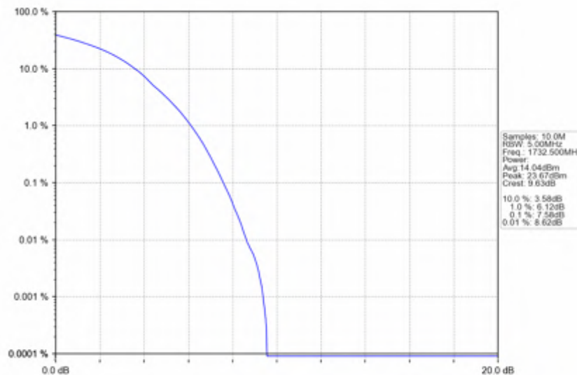
Band4_20MHz_256QAM_MCH_1732.5MHz_RB_100_0_NTNV
