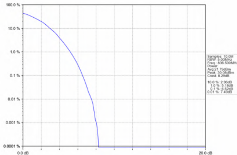
Band5_5MHz_16QAM_MCH_836.5MHz_RB_25_0_NTNV
