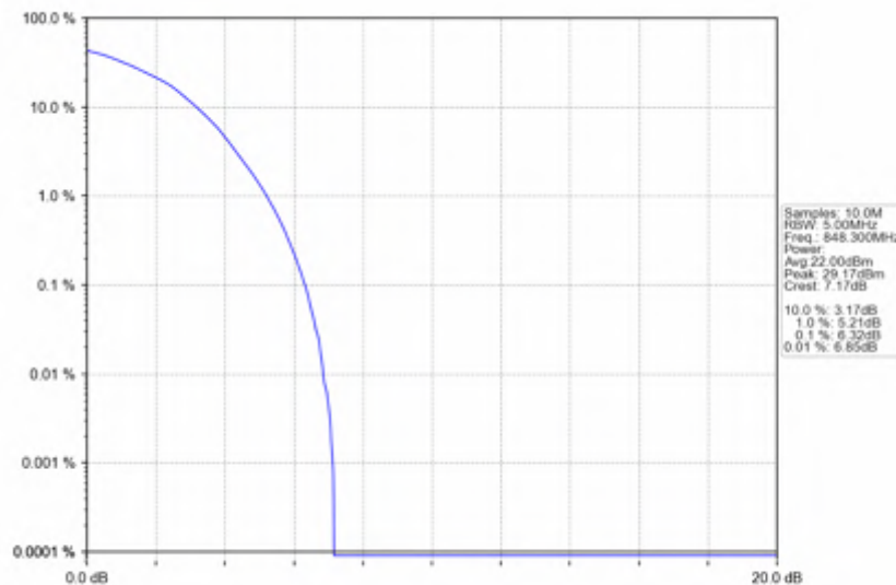
Band5_1.4MHz_16QAM_HCH_848.3MHz_RB_6_0_NTNV
