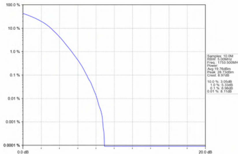
Band4_3MHz_256QAM_HCH_1753.5MHz_RB_15_0_NTNV
