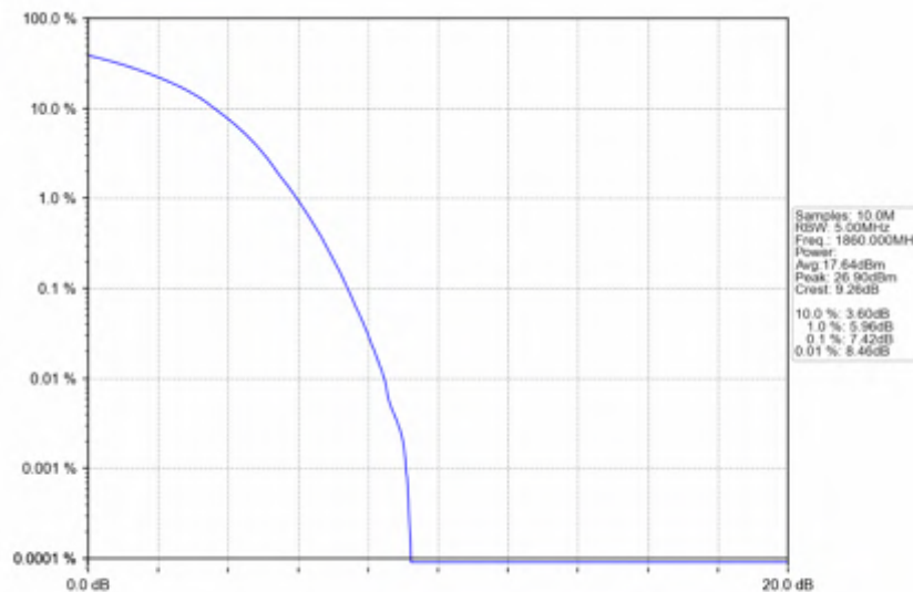
Band25_20MHz_16QAM_LCH_1860MHz_RB_100_0_NTNV
