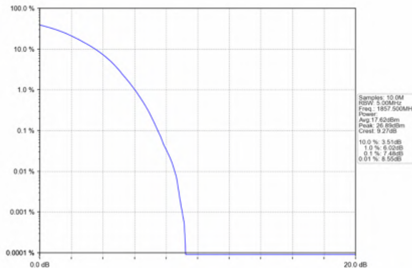
Band2_15MHz_64QAM_LCH_1857.5MHz_RB_75_0_NTNV
