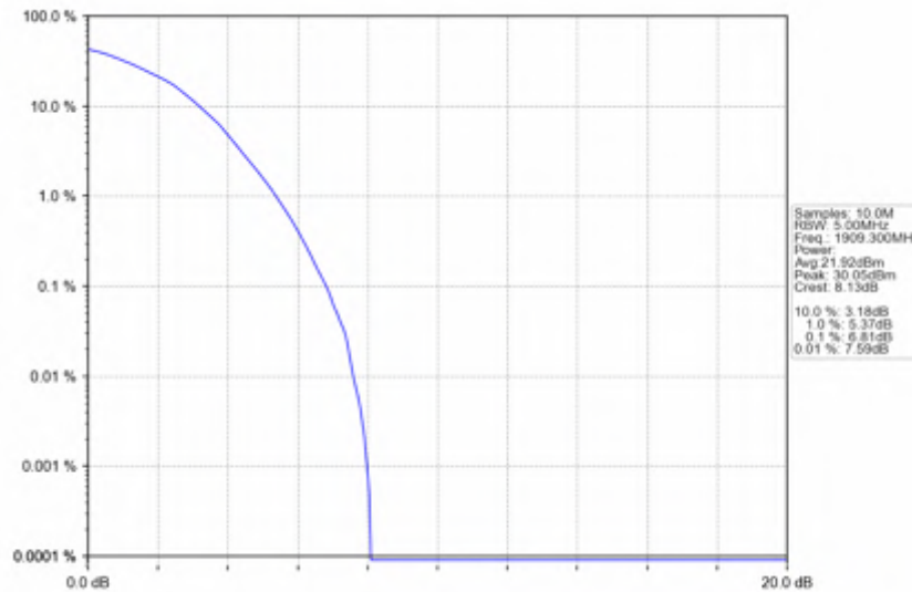
Band2_1.4MHz_QPSK_HCH_1909.3MHz_RB_6_0_NTNV
