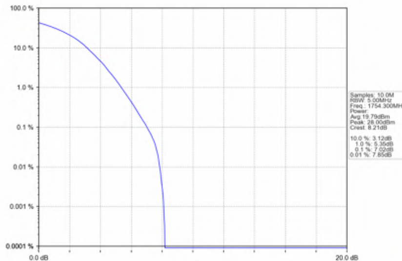
Band4_1.4MHz_256QAM_HCH_1754.3MHz_RB_6_0_NTNV
