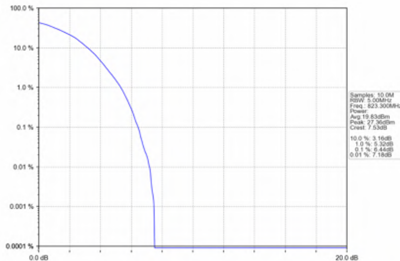
Band26a_1.4MHz_64QAM_HCH_823.3MHz_RB_6_0_NTNV
