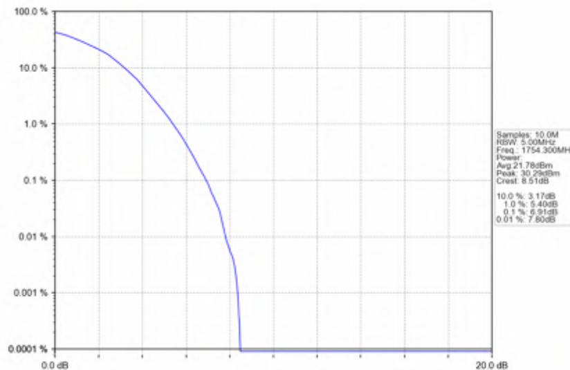
Band4_1.4MHz_QPSK_HCH_1754.3MHz_RB_6_0_NTNV
