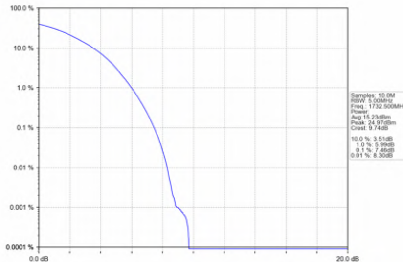
Band4_15MHz_256QAM_MCH_1732.5MHz_RB_75_0_NTNV
