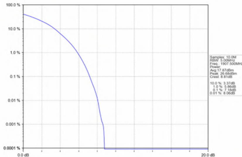
Band25_15MHz_16QAM_HCH_1907.5MHz_RB_75_0_NTNV
