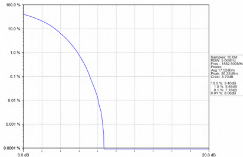
Band25_15MHz_16QAM_MCH_1882.5MHz_RB_75_0_NTNV
