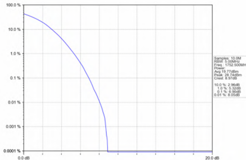
Band4_5MHz_256QAM_HCH_1752.5MHz_RB_25_0_NTNV
