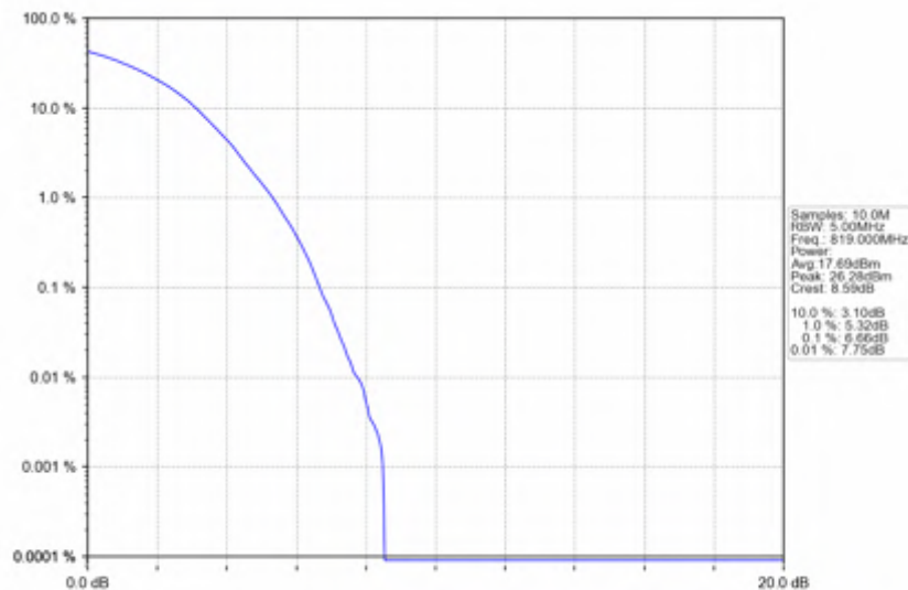
Band26a_1.4MHz_256QAM_MCH_819MHz_RB_6_0_NTNV
