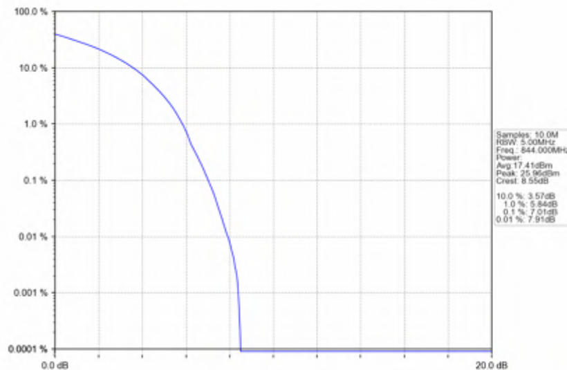
Band5_10MHz_256QAM_HCH_844MHz_RB_50_0_NTNV
