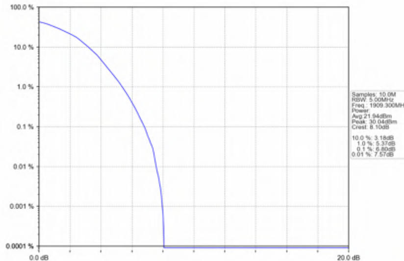
Band2_1.4MHz_16QAM_HCH_1909.3MHz_RB_6_0_NTNV
