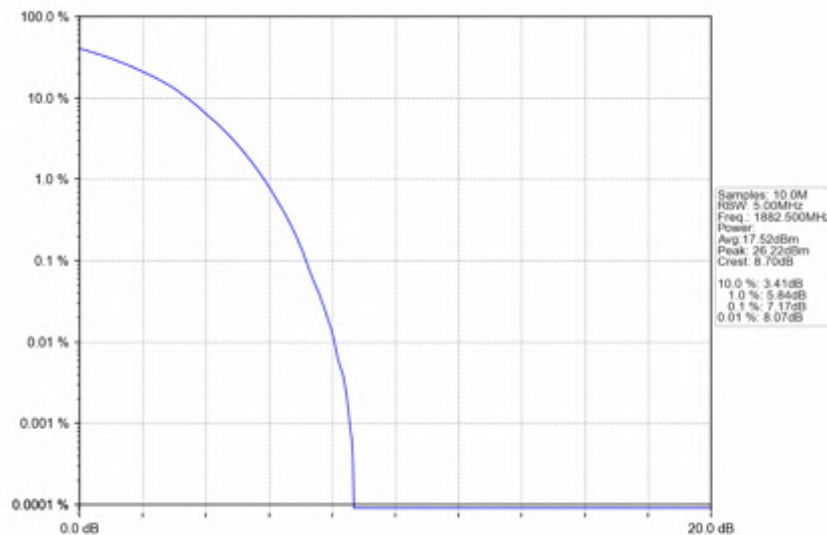
Band25_15MHz_64QAM_MCH_1882.5MHz_RB_75_0_NTNV
