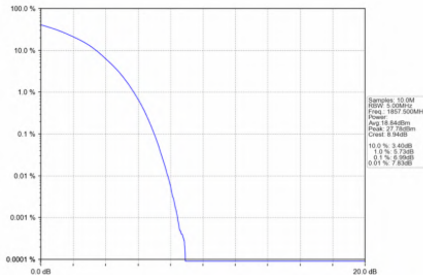
Band25_15MHz_16QAM_LCH_1857.5MHz_RB_75_0_NTNV
