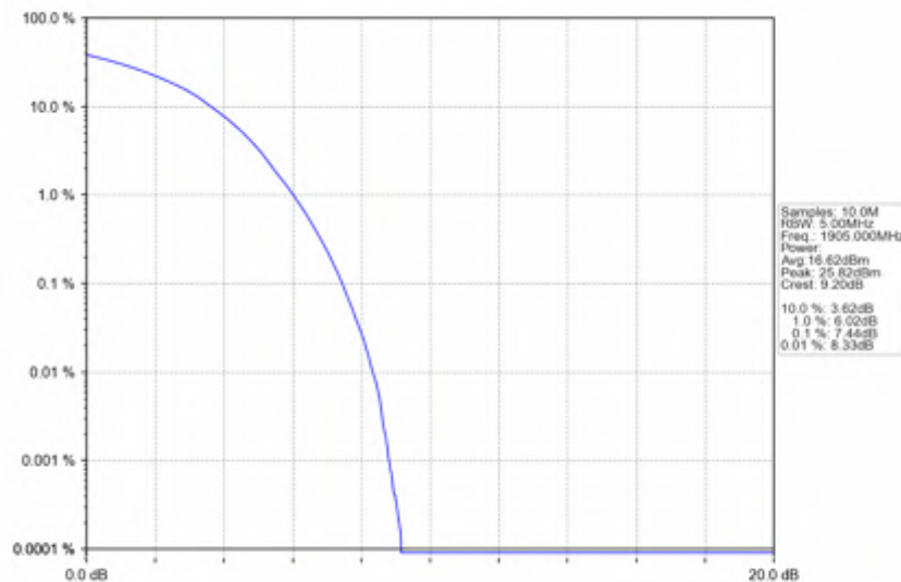
Band25_20MHz_16QAM_HCH_1905MHz_RB_100_0_NTNV
