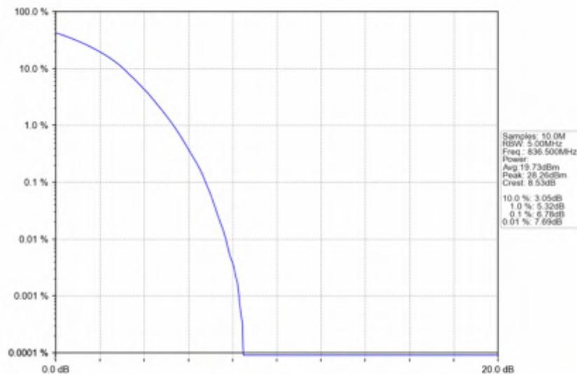
Band5_3MHz_256QAM_MCH_836.5MHz_RB_15_0_NTNV
