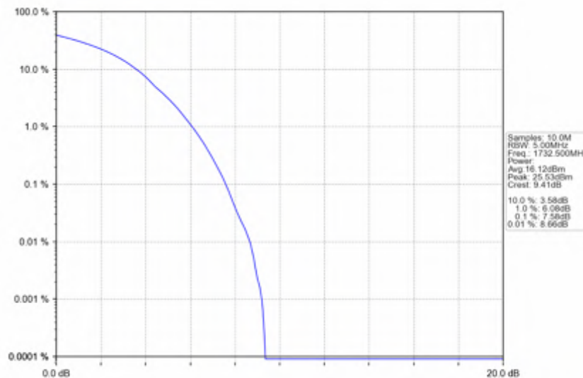
Band4_20MHz_16QAM_MCH_1732.5MHz_RB_100_0_NTNV
