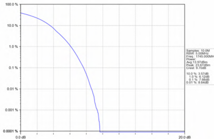
Band4_20MHz_256QAM_HCH_1745MHz_RB_100_0_NTNV
