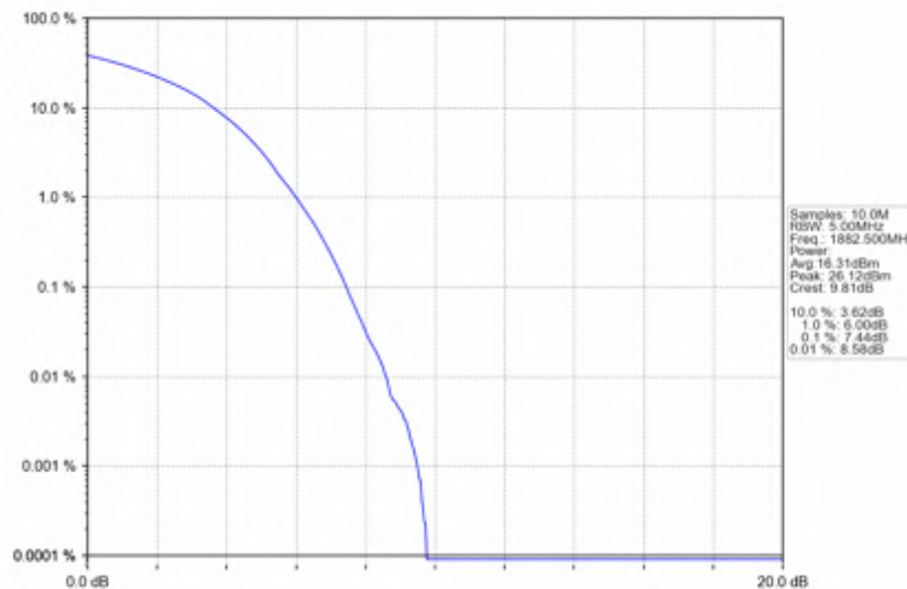
Band25_20MHz_64QAM_MCH_1882.5MHz_RB_100_0_NTNV
