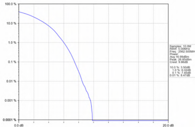
Band7_15MHz_16QAM_HCH_2562.5MHz_RB_75_0_NTNV
