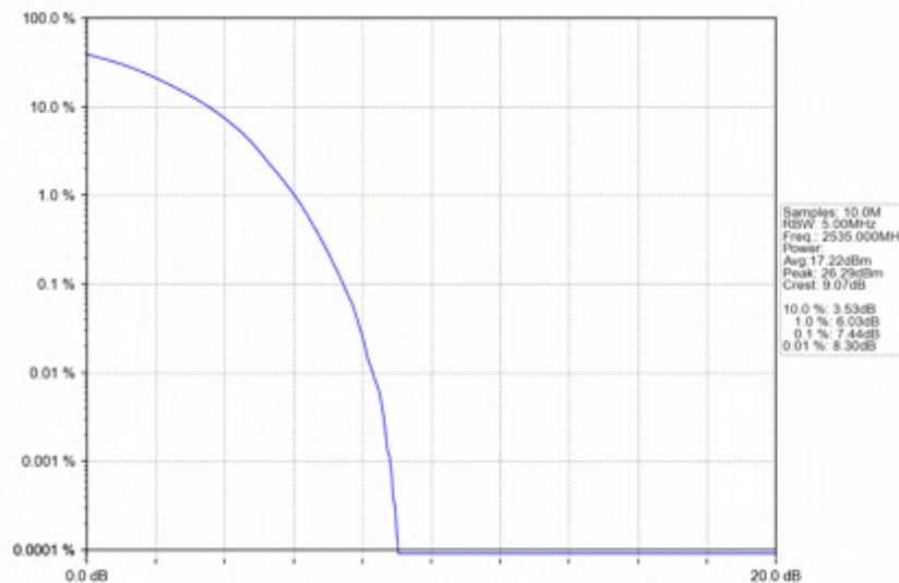
Band7_15MHz_16QAM_MCH_2535MHz_RB_75_0_NTNV
