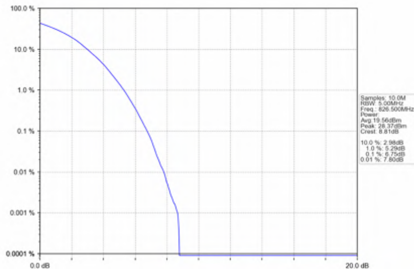
Band5_5MHz_256QAM_LCH_826.5MHz_RB_25_0_NTNV
