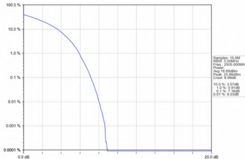
Band7_10MHz_256QAM_LCH_2505MHz_RB_50_0_NTNV
