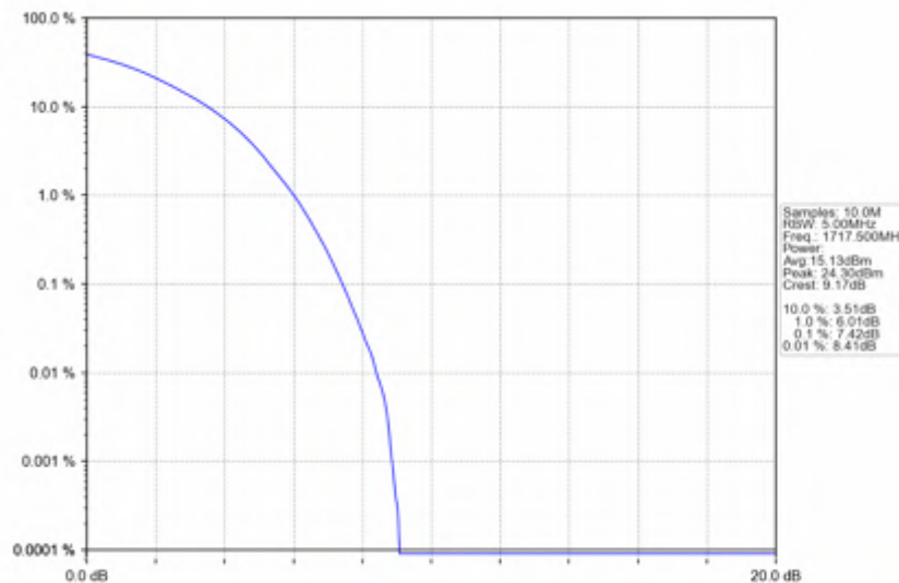
Band4_15MHz_256QAM_LCH_1717.5MHz_RB_75_0_NTNV
