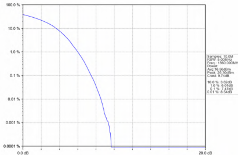
Band25_20MHz_64QAM_LCH_1860MHz_RB_100_0_NTNV
