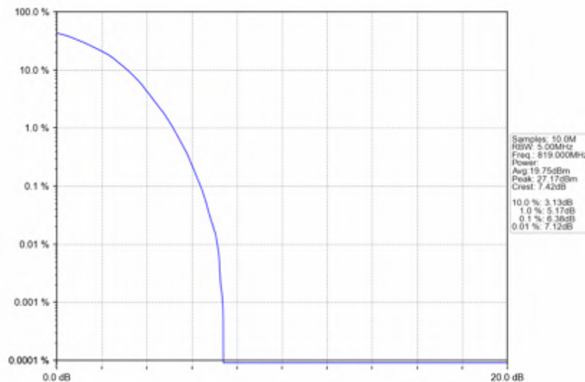
Band26a_1.4MHz_64QAM_MCH_819MHz_RB_6_0_NTNV
