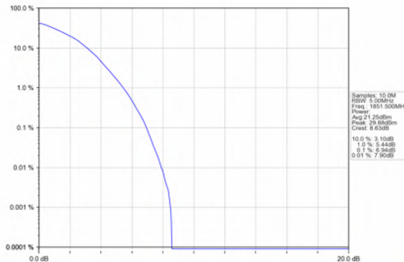
Band25_3MHz_64QAM_LCH_1851.5MHz_RB_15_0_NTNV
