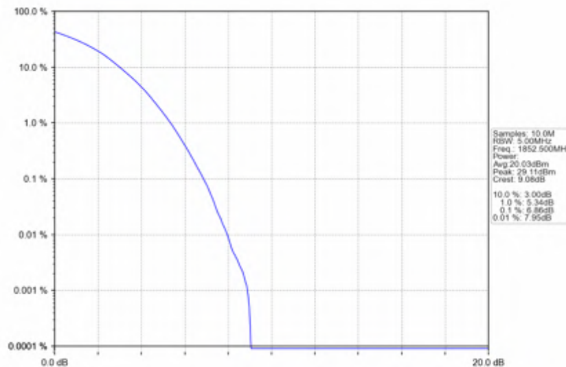
Band2_5MHz_256QAM_LCH_1852.5MHz_RB_25_0_NTNV
