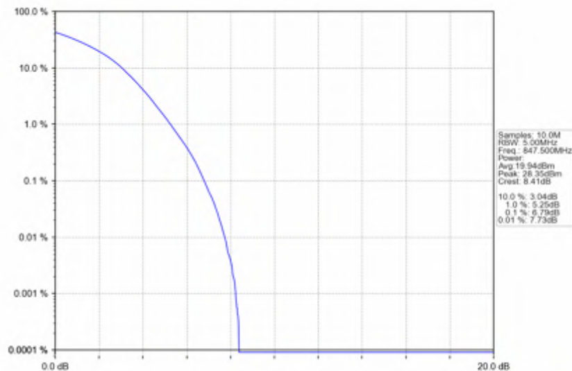
Band5_3MHz_256QAM_HCH_847.5MHz_RB_15_0_NTNV
