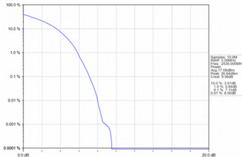
Band7_10MHz_256QAM_MCH_2535MHz_RB_50_0_NTNV
