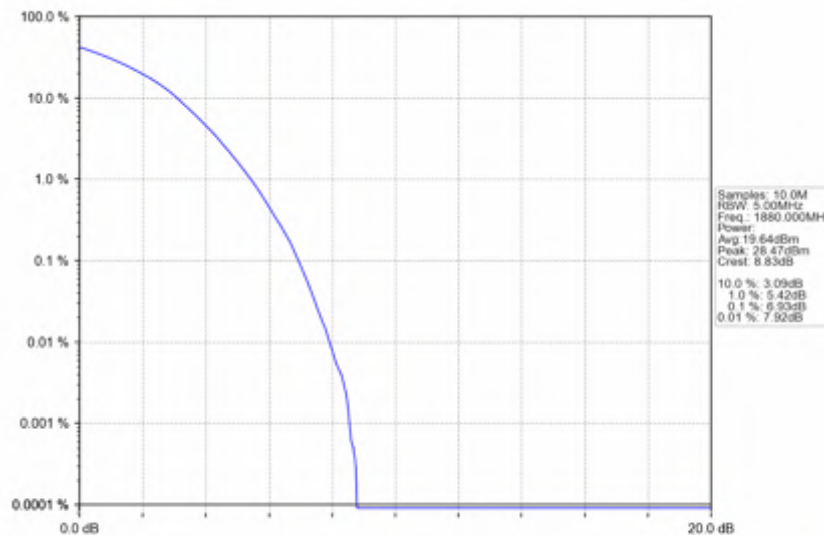
Band2_3MHz_256QAM_MCH_1880MHz_RB_15_0_NTNV
