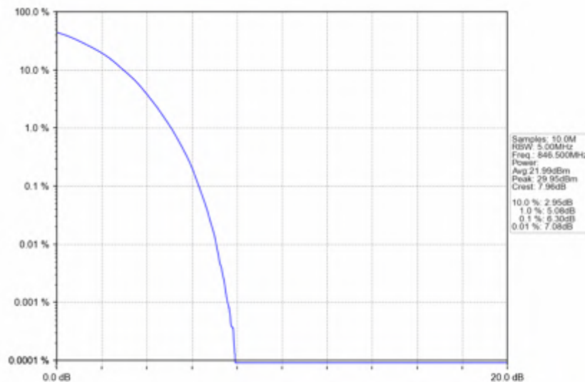
Band5_5MHz_16QAM_HCH_846.5MHz_RB_25_0_NTNV
