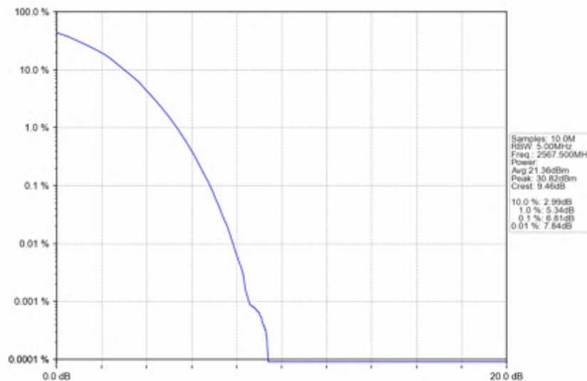
Band7_5MHz_64QAM_HCH_2567.5MHz_RB_25_0_NTNV
