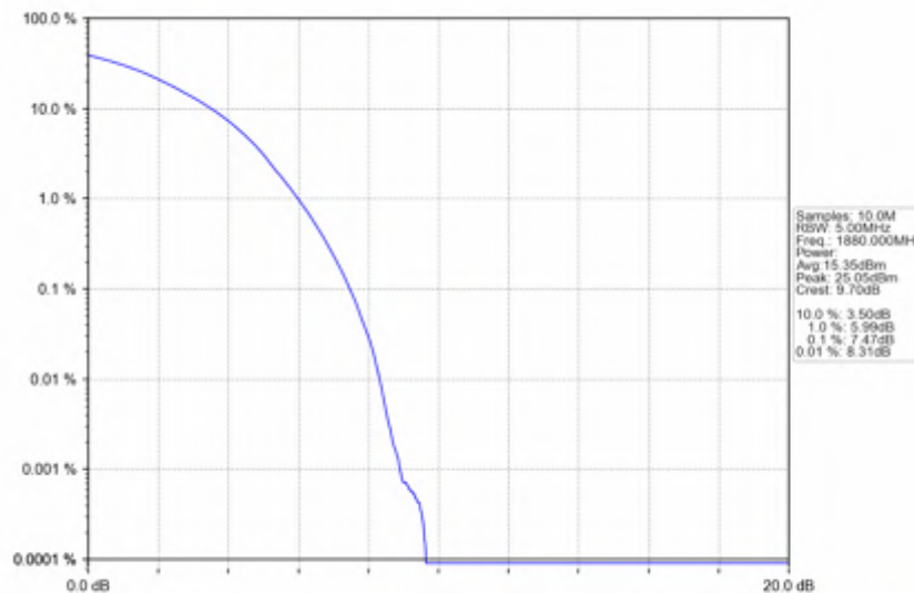
Band2_15MHz_256QAM_MCH_1880MHz_RB_75_0_NTNV
