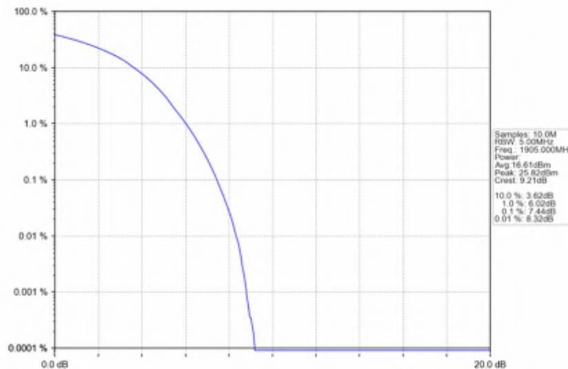
Band25_20MHz_64QAM_HCH_1905MHz_RB_100_0_NTNV
