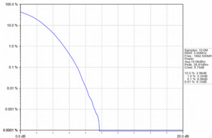
Band25_5MHz_256QAM_MCH_1882.5MHz_RB_25_0_NTNV
