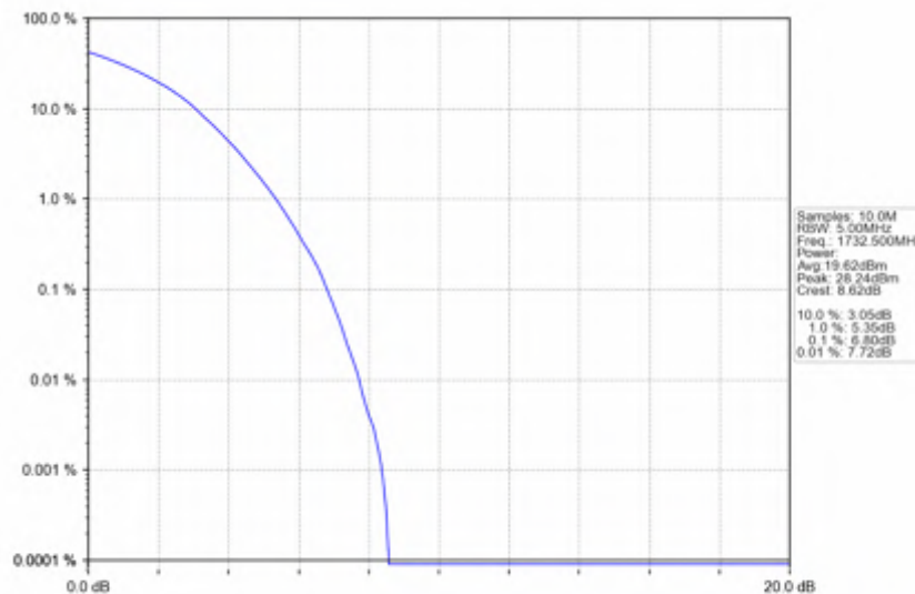
Band4_3MHz_256QAM_MCH_1732.5MHz_RB_15_0_NTNV
