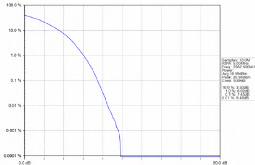
Band7_15MHz_QPSK_HCH_2562.5MHz_RB_75_0_NTNV
