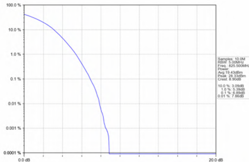
Band5_3MHz_256QAM_LCH_825.5MHz_RB_15_0_NTNV
