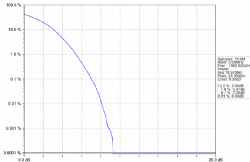
Band25_3MHz_256QAM_MCH_1882.5MHz_RB_15_0_NTNV
