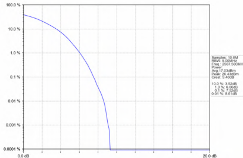
Band7_15MHz_16QAM_LCH_2507.5MHz_RB_75_0_NTNV
