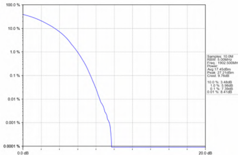
Band2_15MHz_QPSK_HCH_1902.5MHz_RB_75_0_NTNV
