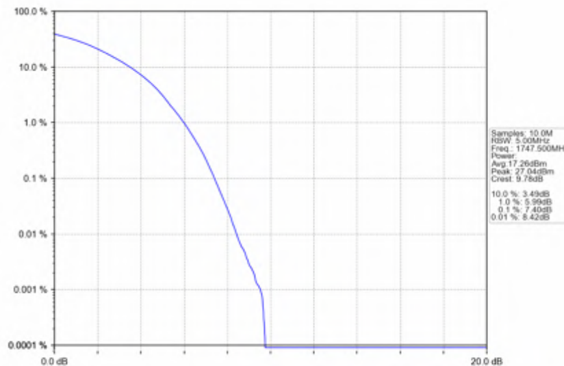
Band4_15MHz_QPSK_HCH_1747.5MHz_RB_75_0_NTNV
