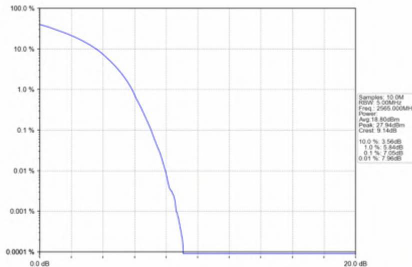
Band7_10MHz_16QAM_HCH_2565MHz_RB_50_0_NTNV
