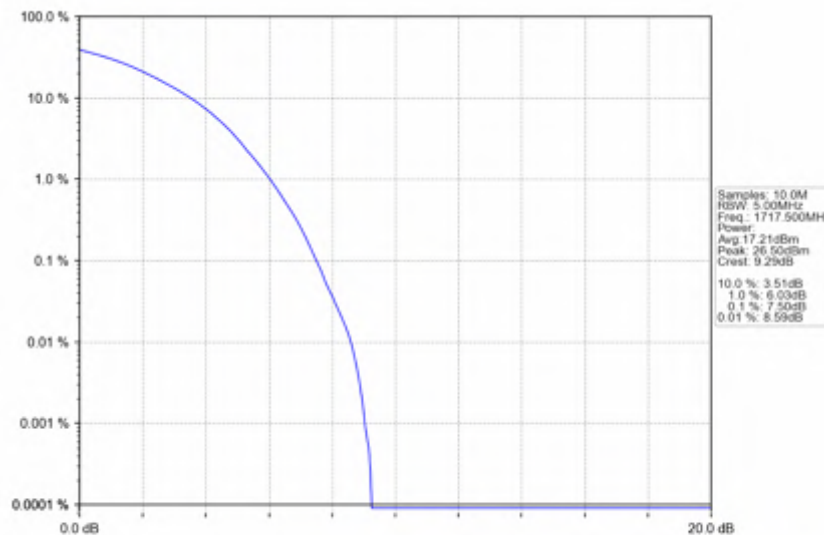
Band4_15MHz_64QAM_LCH_1717.5MHz_RB_75_0_NTNV
