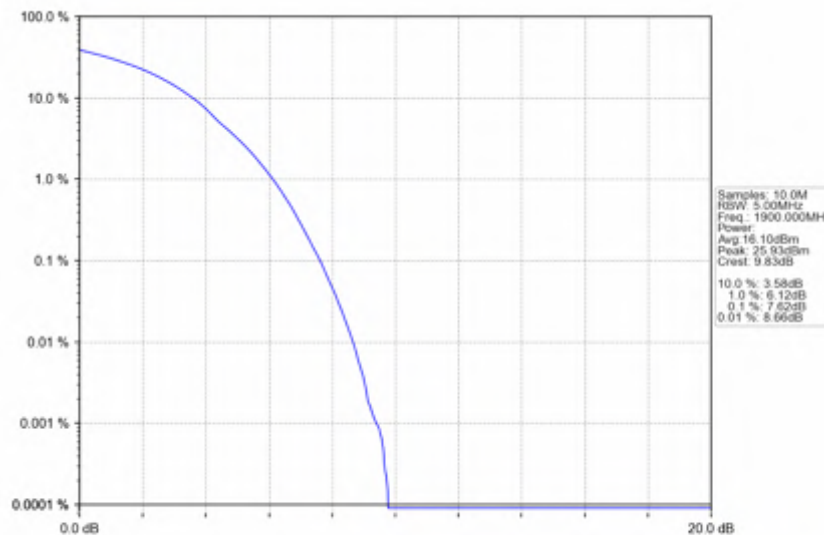
Band2_20MHz_64QAM_HCH_1900MHz_RB_100_0_NTNV
