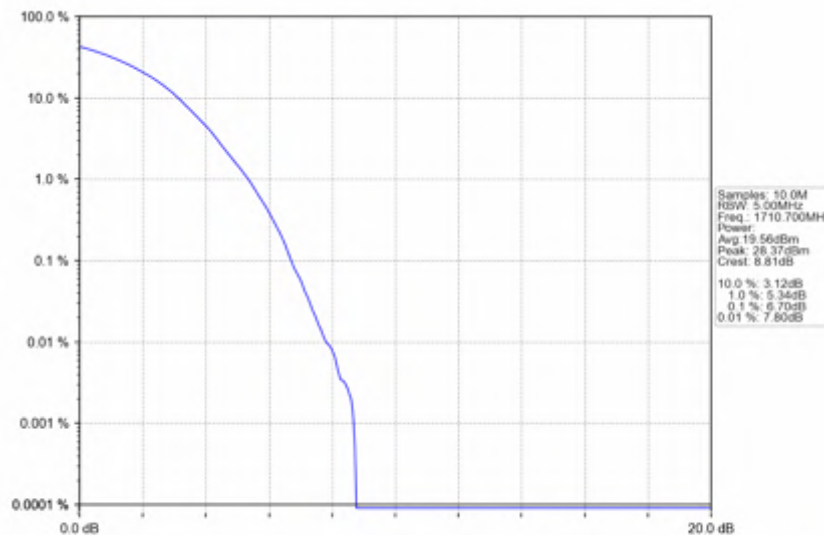
Band4_1.4MHz_256QAM_LCH_1710.7MHz_RB_6_0_NTNV
