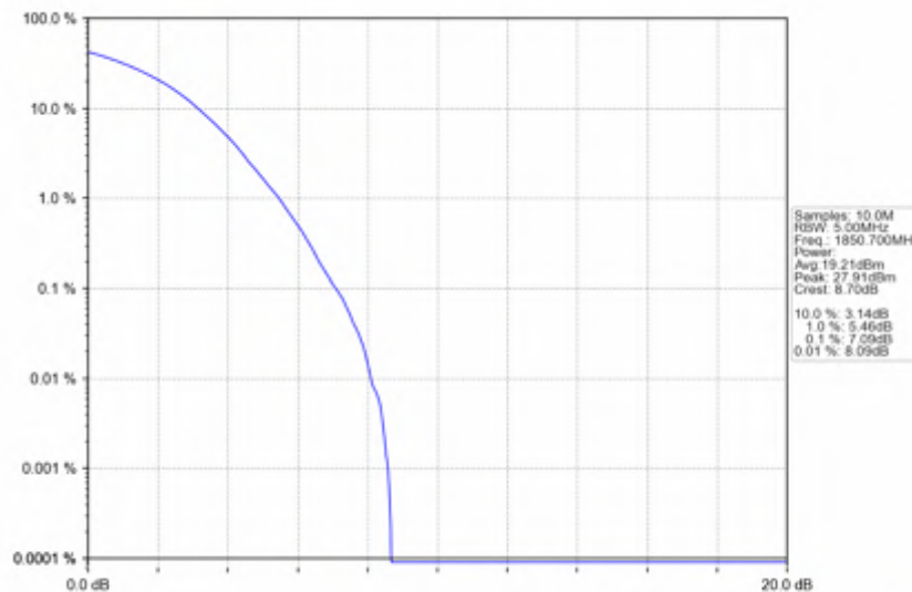
Band25_1.4MHz_256QAM_LCH_1850.7MHz_RB_6_0_NTNV
