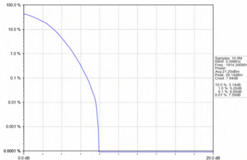
Band25_1.4MHz_64QAM_HCH_1914.3MHz_RB_6_0_NTNV
