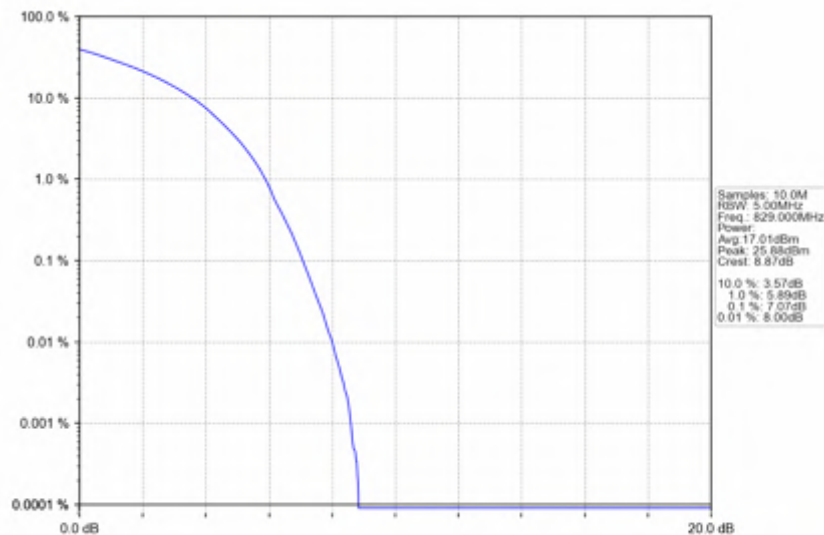
Band5_10MHz_256QAM_LCH_829MHz_RB_50_0_NTNV
