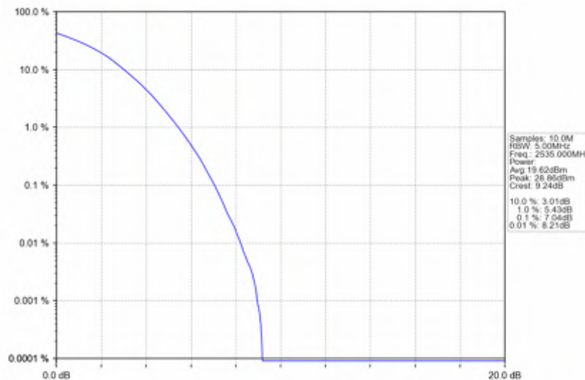
Band7_5MHz_256QAM_MCH_2535MHz_RB_25_0_NTNV
