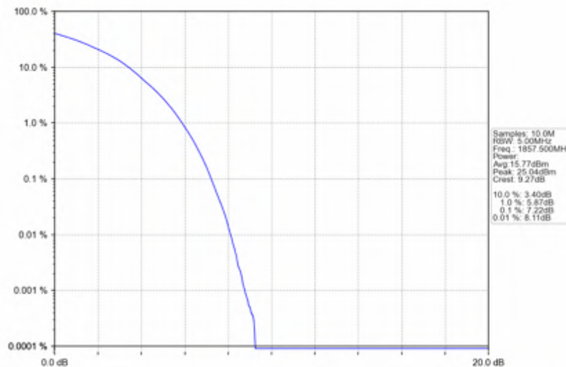
Band25_15MHz_256QAM_LCH_1857.5MHz_RB_75_0_NTNV
