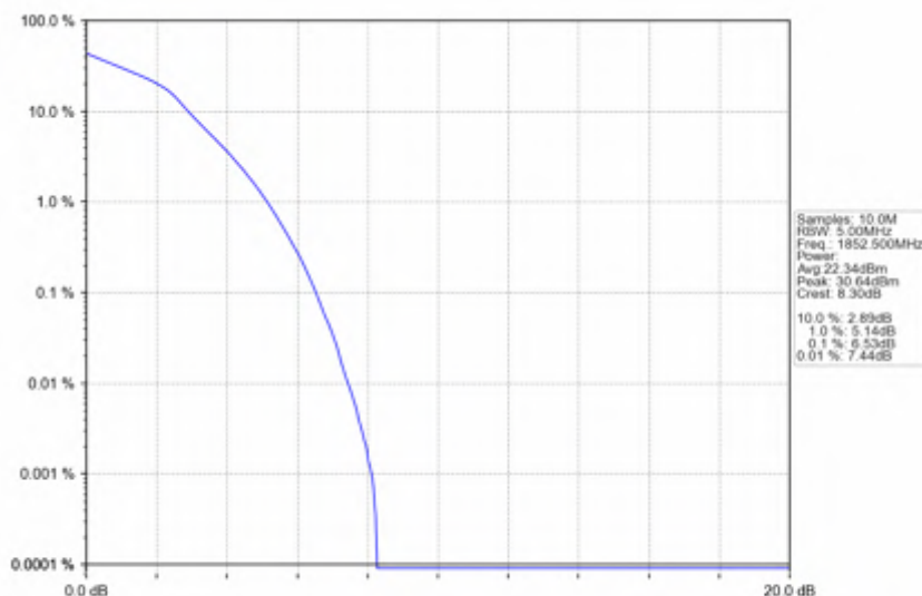
Band25_5MHz_16QAM_LCH_1852.5MHz_RB_25_0_NTNV
