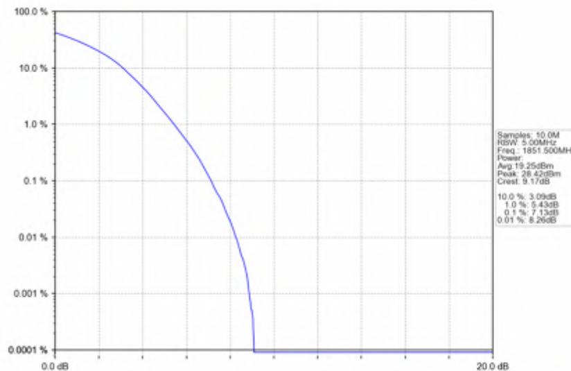
Band25_3MHz_256QAM_LCH_1851.5MHz_RB_15_0_NTNV
