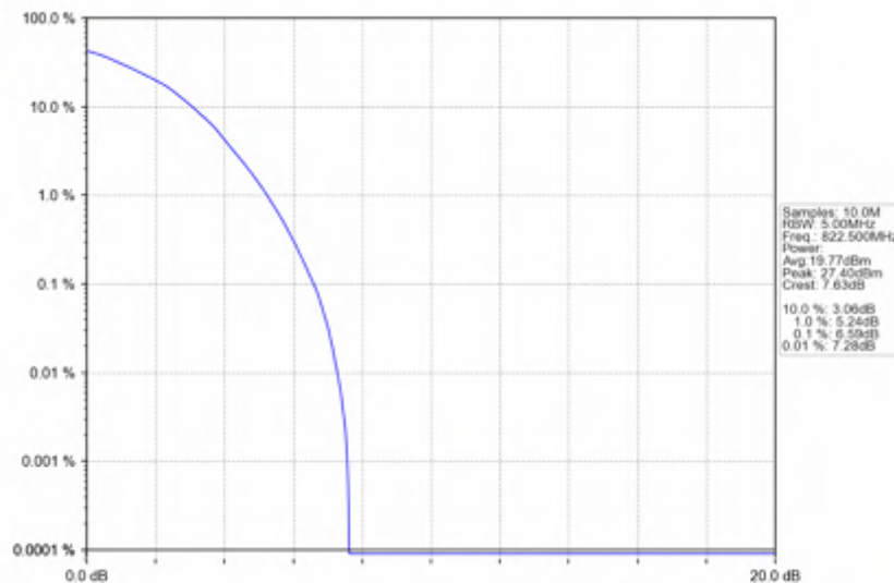
Band26a_3MHz_QPSK_HCH_822.5MHz_RB_15_0_NTNV
