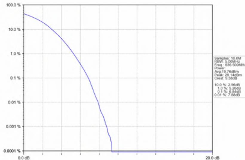
Band5_5MHz_256QAM_MCH_836.5MHz_RB_25_0_NTNV
