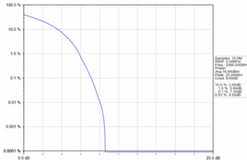
Band7_10MHz_256QAM_HCH_2565MHz_RB_50_0_NTNV
