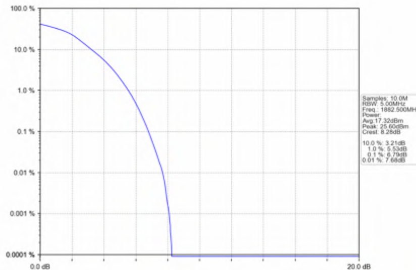
Band25_10MHz_256QAM_MCH_1882.5MHz_RB_50_0_NTNV
