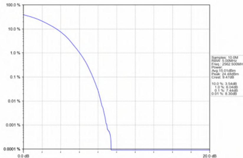
Band7_15MHz_256QAM_HCH_2562.5MHz_RB_75_0_NTNV
