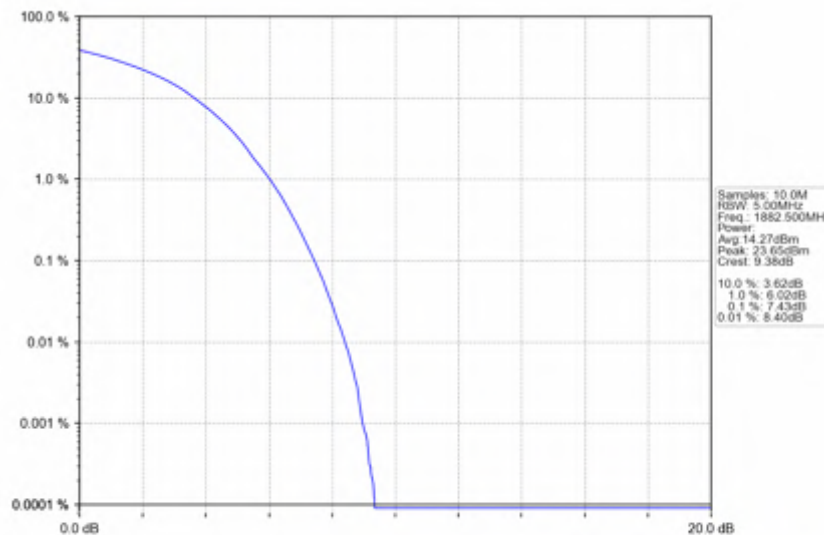
Band25_20MHz_256QAM_MCH_1882.5MHz_RB_100_0_NTNV
