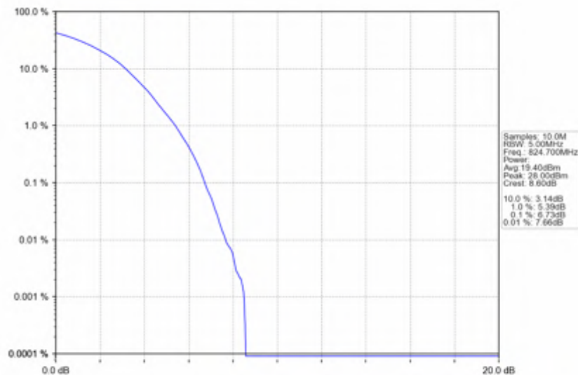
Band5_1.4MHz_256QAM_LCH_824.7MHz_RB_6_0_NTNV
