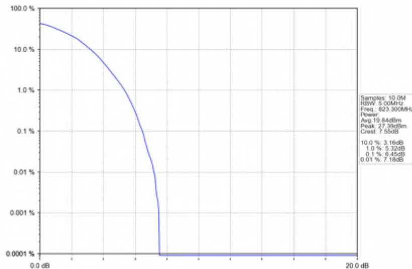
Band26a_1.4MHz_QPSK_HCH_823.3MHz_RB_6_0_NTNV
