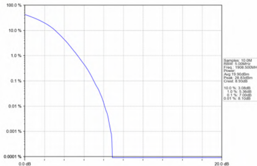
Band2_3MHz_256QAM_HCH_1908.5MHz_RB_15_0_NTNV
