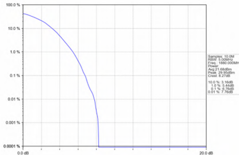
Band2_1.4MHz_64QAM_MCH_1880MHz_RB_6_0_NTNV
