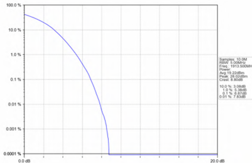
Band25_3MHz_256QAM_HCH_1913.5MHz_RB_15_0_NTNV
