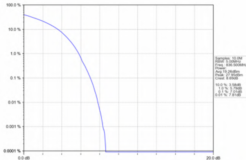
Band5_10MHz_16QAM_MCH_836.5MHz_RB_50_0_NTNV
