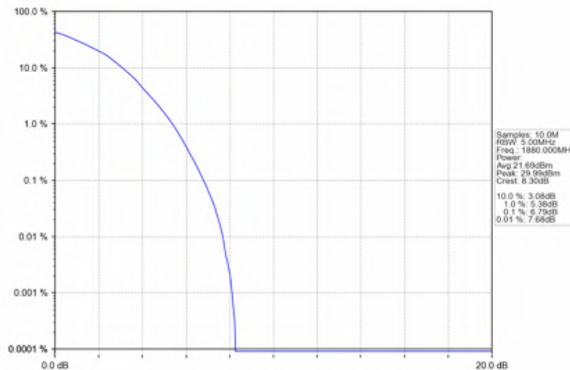
Band2_3MHz_16QAM_MCH_1880MHz_RB_15_0_NTNV
