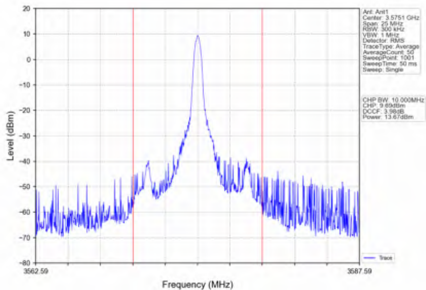
Band42c 10MHz 256QAM MCH 3575MHz RB 1 25 NTNV
