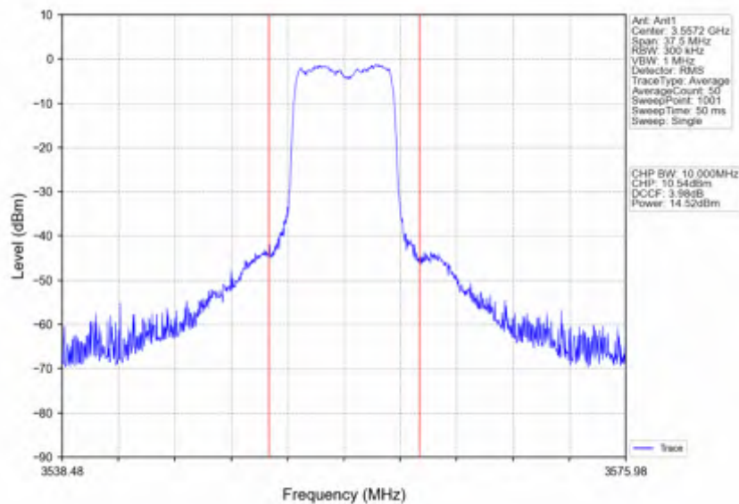
Band42c_15MHz_64QAM_LCH_3557.5MHz_RB_36_39_NTNV
