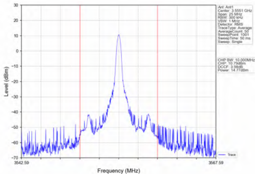
Band42c_10MHz_64QAM_LCH_3555MHz_RB_1_25_NTNV
