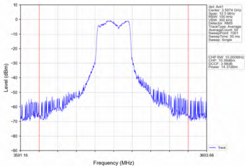
Band42c_5MHz_256QAM_HCH_3597.5MHz_RB_12_6_NTNV
