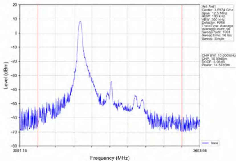
Band42c_5MHz_QPSK_HCH_3597.5MHz_RB_12_13_NTNV
