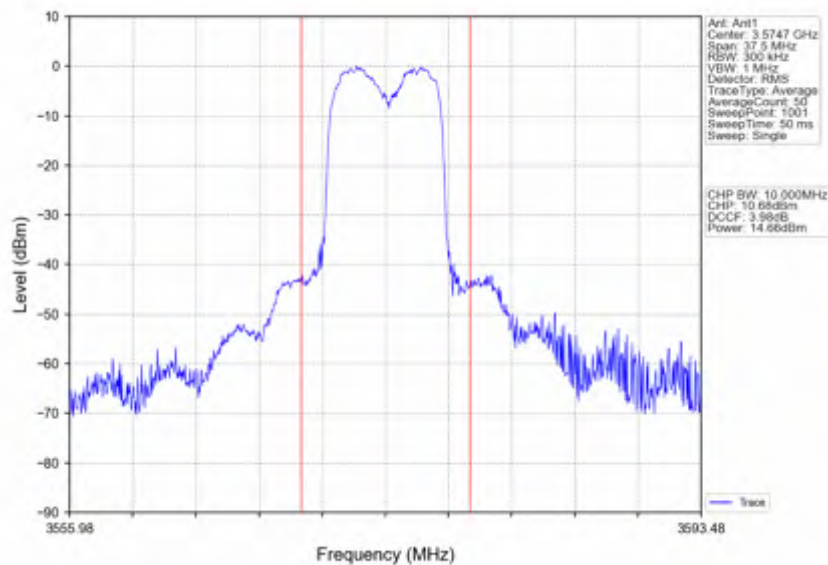
Band42c_15MHz_16QAM_MCH_3575MHz_RB_36_39_NTNV
