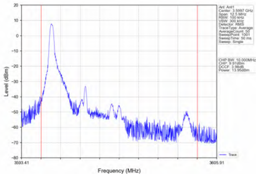
Band42c_5MHz_64QAM_HCH_3597.5MHz_RB_12_0_NTNV
