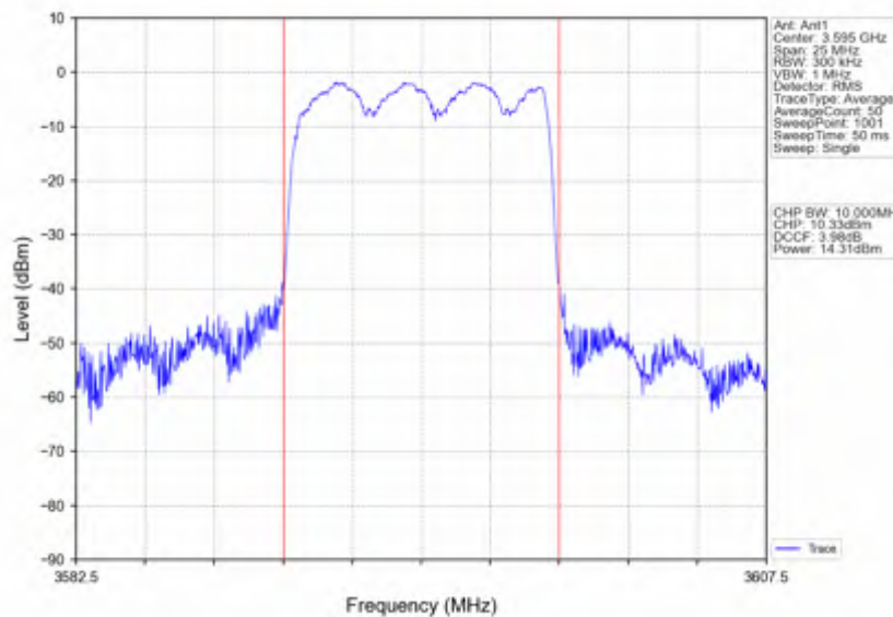
Band42c_10MHz_256QAM_HCH_3595MHz_RB_50_0_NTNV
