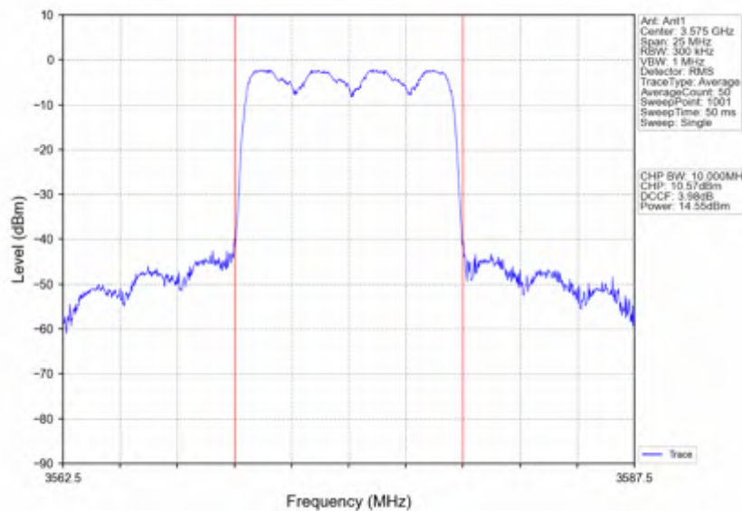
Band42c_10MHz_64QAM_MCH_3575MHz_RB_50_0_NTNV
