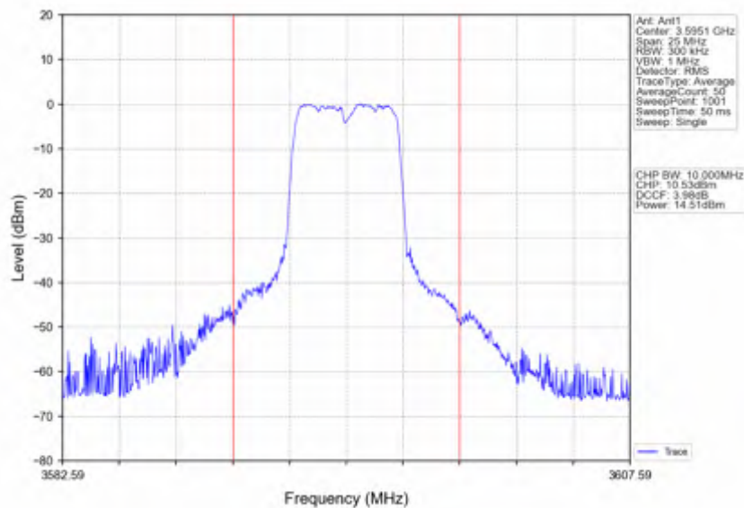
Band42c_10MHz_64QAM_HCH_3595MHz_RB_25_25_NTNV
