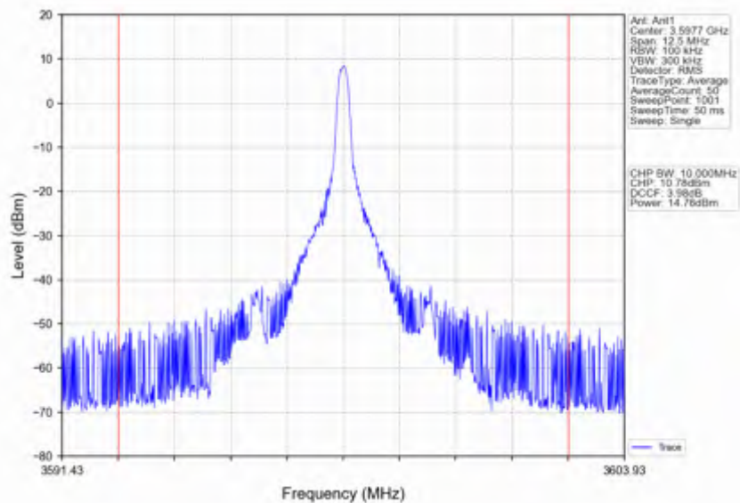
Band42c_5MHz_256QAM_HCH_3597.5MHz_RB_1_24_NTNV
