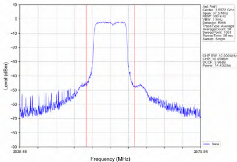
Band42c_15MHz_256QAM_LCH_3557.5MHz_RB_36_18_NTNV
