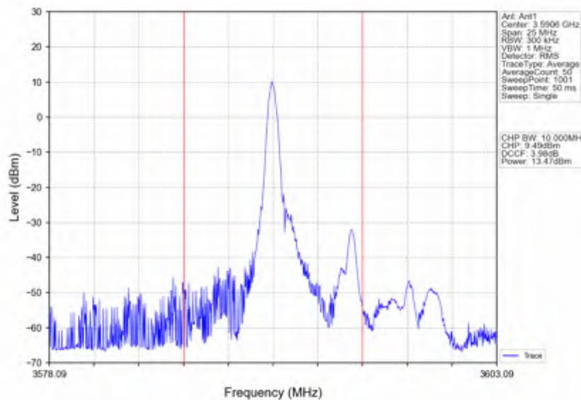
Band42c_10MHz_256QAM_HCH_3595MHz_RB_1_0_NTNV
