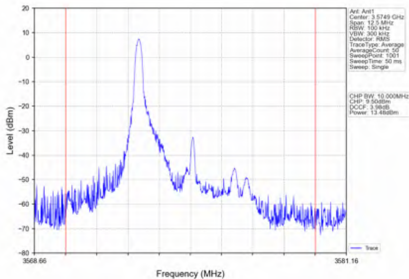
Band42c_5MHz_64QAM_MCH_3575MHz_RB_12_6_NTNV
