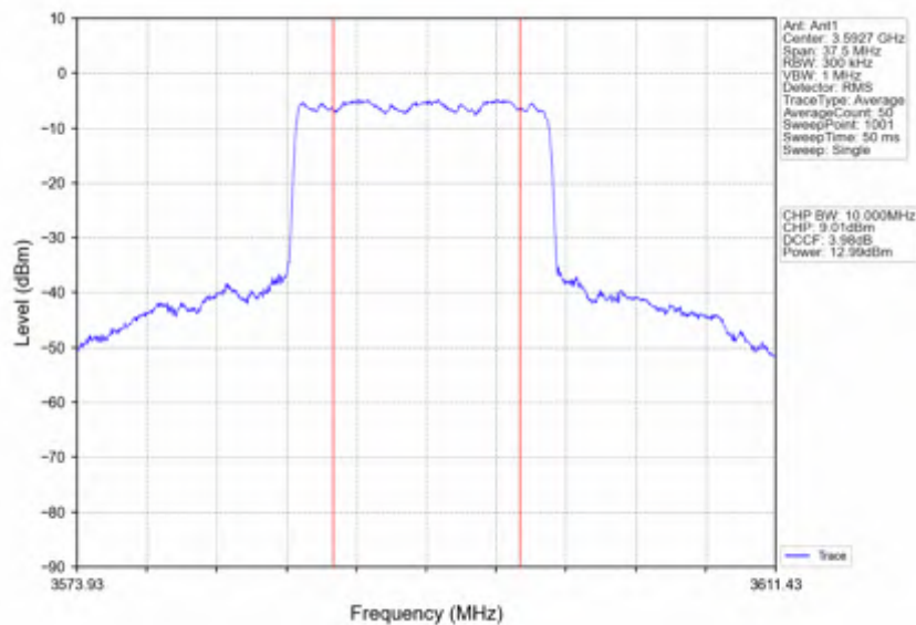
Band42c_15MHz_16QAM_HCH_3592.5MHz_RB_1_74_NTNV
