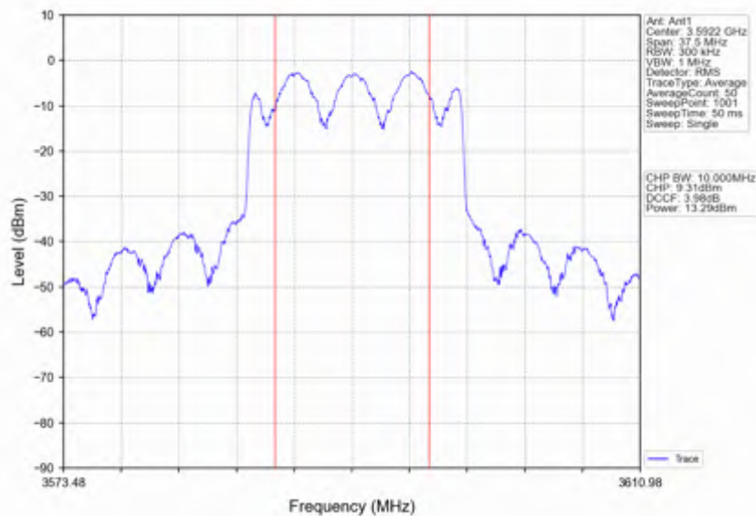
Band42c_15MHz_16QAM_HCH_3592.5MHz_RB_36_18_NTNV
