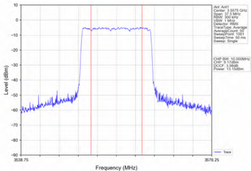
Band42c_15MHz_256QAM_LCH_3557.5MHz_RB_75_0_NTNV
