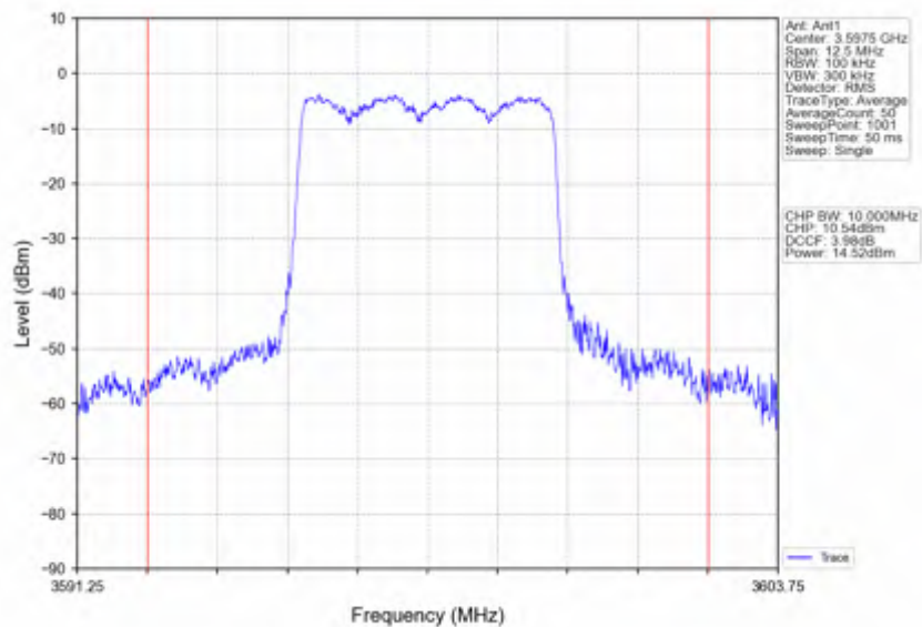
Band42c_5MHz_256QAM_HCH_3597.5MHz_RB_25_0_NTNV
