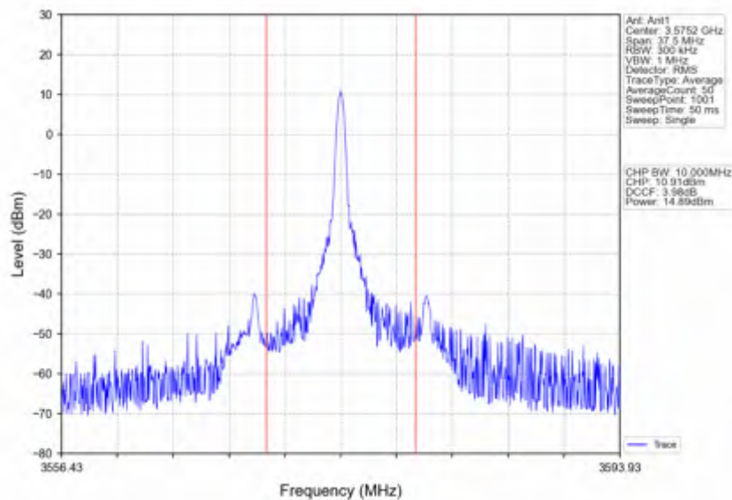
Band42c_15MHz_64QAM_MCH_3575MHz_RB_1_74_NTNV
