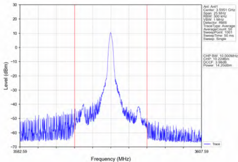
Band42c_10MHz_256QAM_HCH_3595MHz_RB_1_49_NTNV
