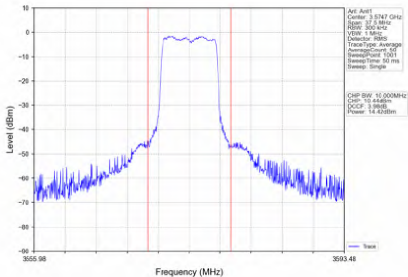
Band42c_15MHz_256QAM_MCH_3575MHz_RB_36_39_NTNV
