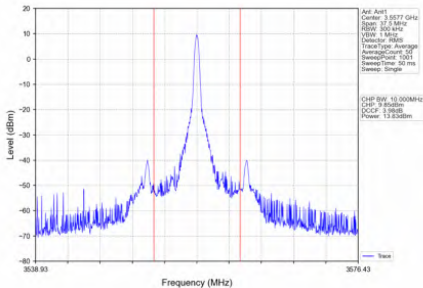
Band42c_15MHz_64QAM_LCH_3557.5MHz_RB_1_38_NTNV
