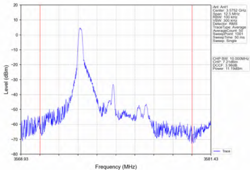
Band42c_5MHz_QPSK_MCH_3575MHz_RB_1_24_NTNV
