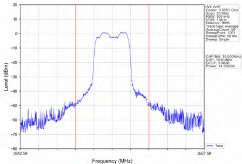
Band42c_10MHz_64QAM_LCH_3555MHz_RB_25_25_NTNV
