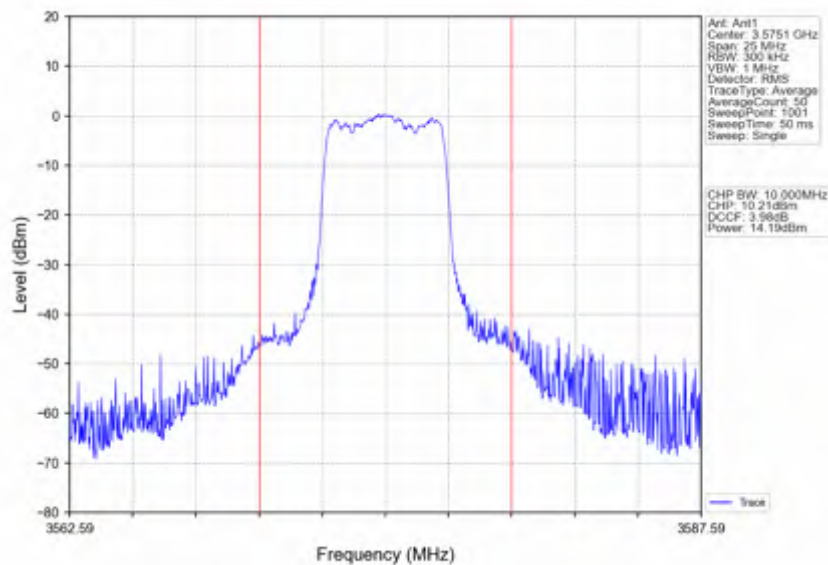
Band42c_10MHz_64QAM_MCH_3575MHz_RB_25_13_NTNV
