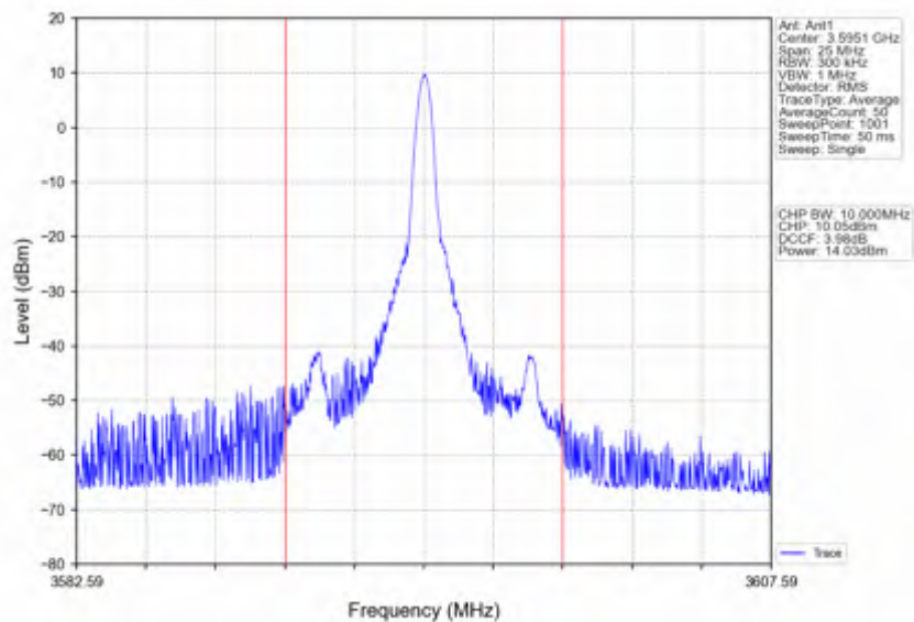
Band42c_10MHz_64QAM_HCH_3595MHz_RB_1_25_NTNV
