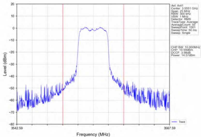
Band42c_10MHz_256QAM_LCH_3555MHz_RB_25_13_NTNV
