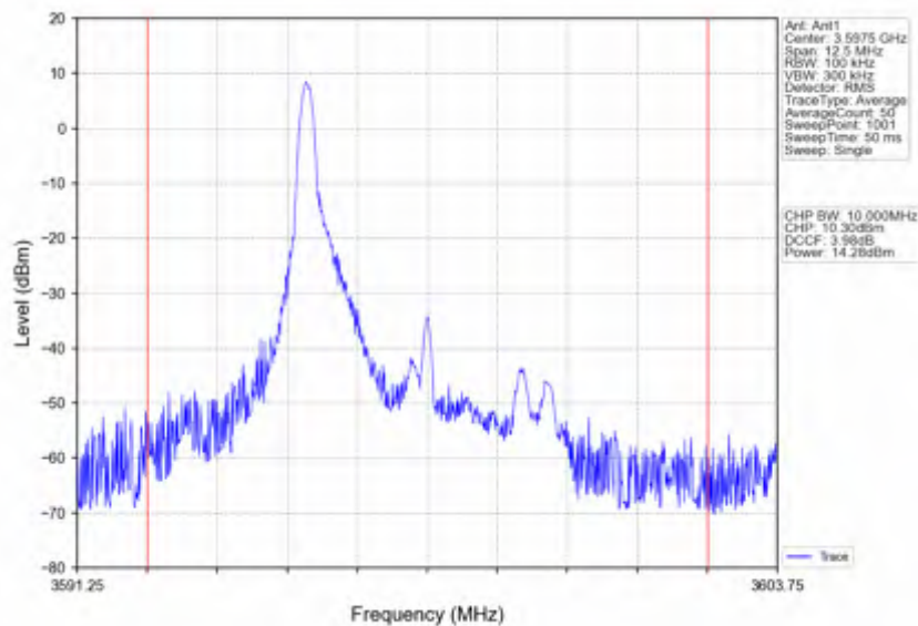
Band42c_5MHz_16QAM_HCH_3597.5MHz_RB_25_0_NTNV
