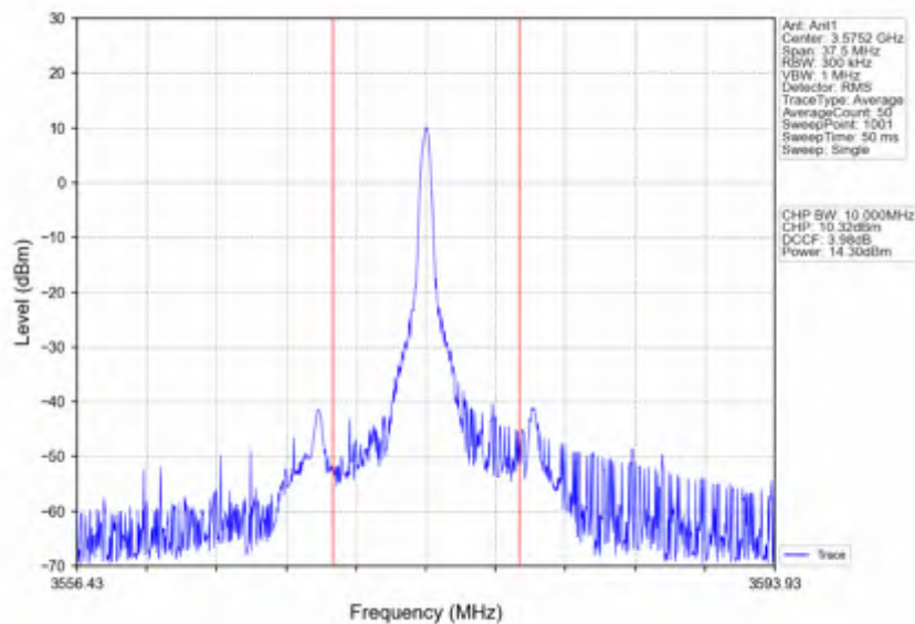
Band42c_15MHz_256QAM_MCH_3575MHz_RB_1_38_NTNV
