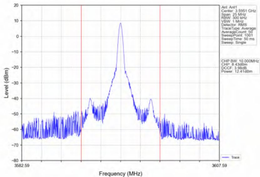
Band42c_10MHz_16QAM_HCH_3595MHz_RB_1_49_NTNV
