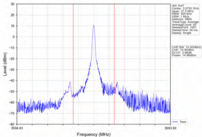
Band42c_15MHz_16QAM_MCH_3575MHz_RB_1_38_NTNV
