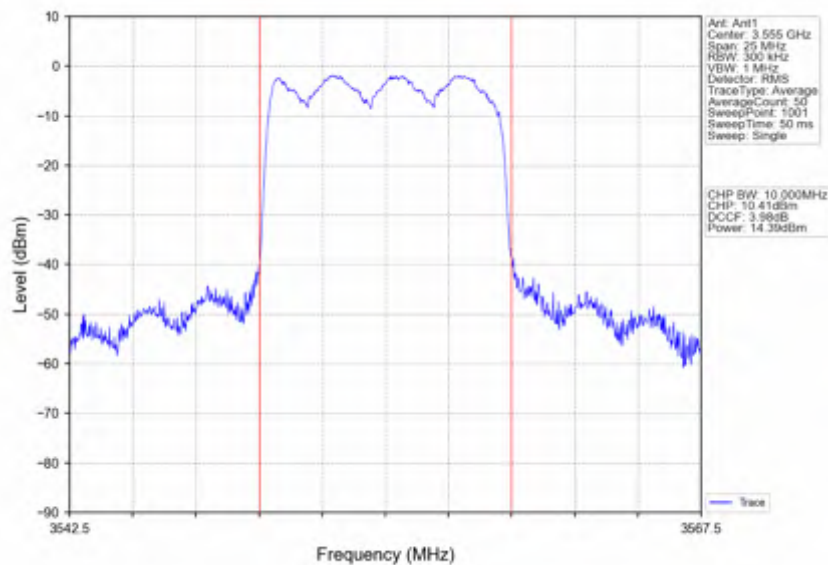
Band42c_10MHz_16QAM_LCH_3555MHz_RB_50_0_NTNV
