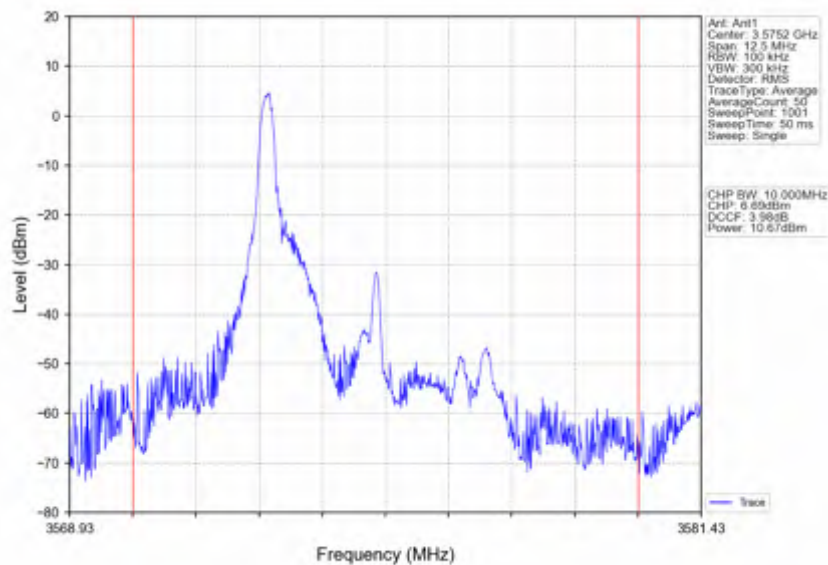
Band42c 5MHz 64QAM MCH 3575MHz RB 1 24 NTN
