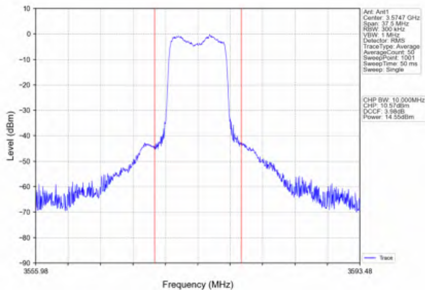
Band42c_15MHz_64QAM_MCH_3575MHz_RB_36_18_NTNV
