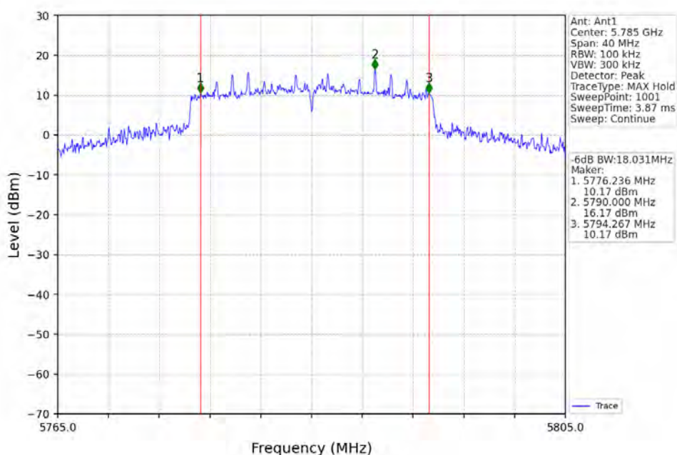
802.11ax(HEW20)_MCH_5785MHz_RU242_Left_Ant1_NTNV
