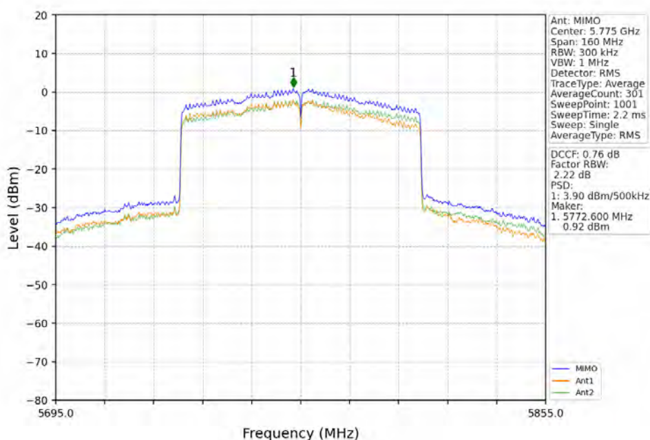
802.11ax(HEW80)_MCH_5775MHz_RU996_Left_MIMO_NTNV
