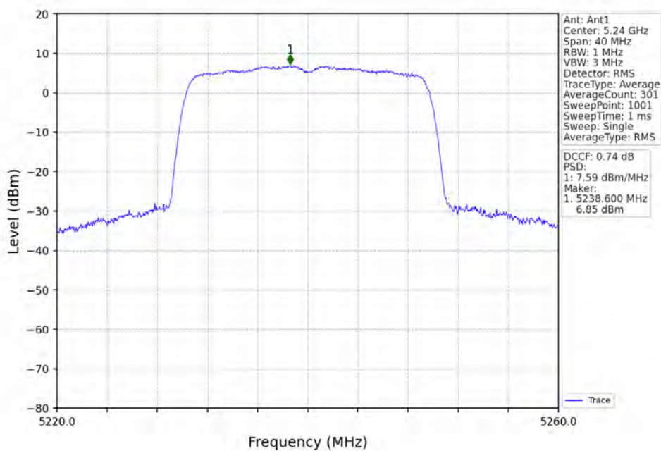
802.11ax(HEW20)_HCH_5240MHz_RU242_Left_Ant1_NTNV
