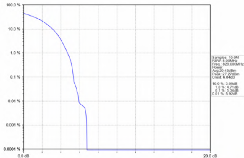
n5_15kHz_SISO_NTNV_10MHz_DFT-s-OFDM QPSK_829MHz_Outer_Full
