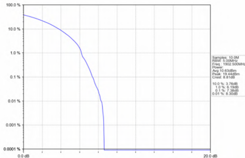
n2_15kHz_SISO_NTNV_15MHz_DFT-s-OFDM 64 QAM_1902.5MHz_Outer_Full
