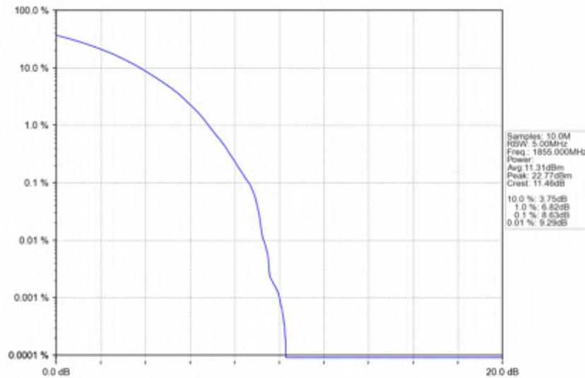
n2_15kHz_SISO_NTNV_10MHz_CP-OFDM 16 QAM_1855MHz_Outer_Full
