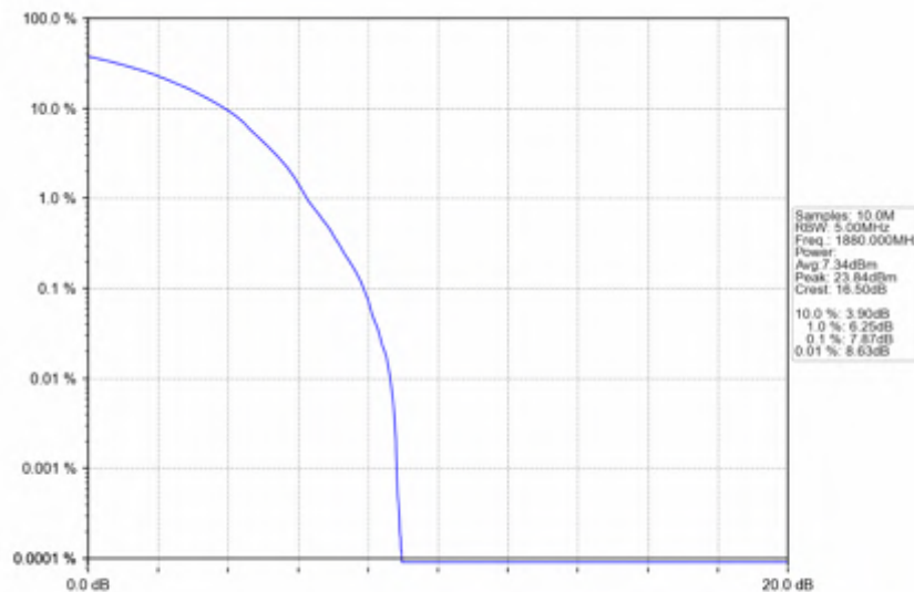
n2_15kHz_SISO_NTNV_20MHz_DFT-s-OFDM_256_QAM_1880MHz_Outer_Full
