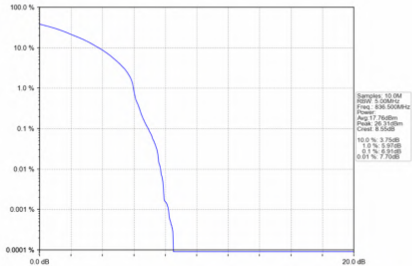
n5_15kHz_SISO_NTV_15MHz_DFT-s-OFDM_16 QAM_836.5MHz_Outer_Full
