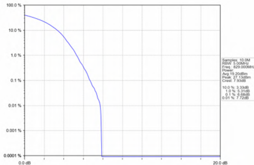
n5_30kHz_SISO_NTNV_10MHz_DFT-s-OFDM 64 QAM_829MHz_Outer_Full
