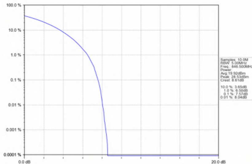
n5_15kHz_SISO_NTV_5MHz_CP-OFDM 64 QAM_846.5MHz_Outer_Full
