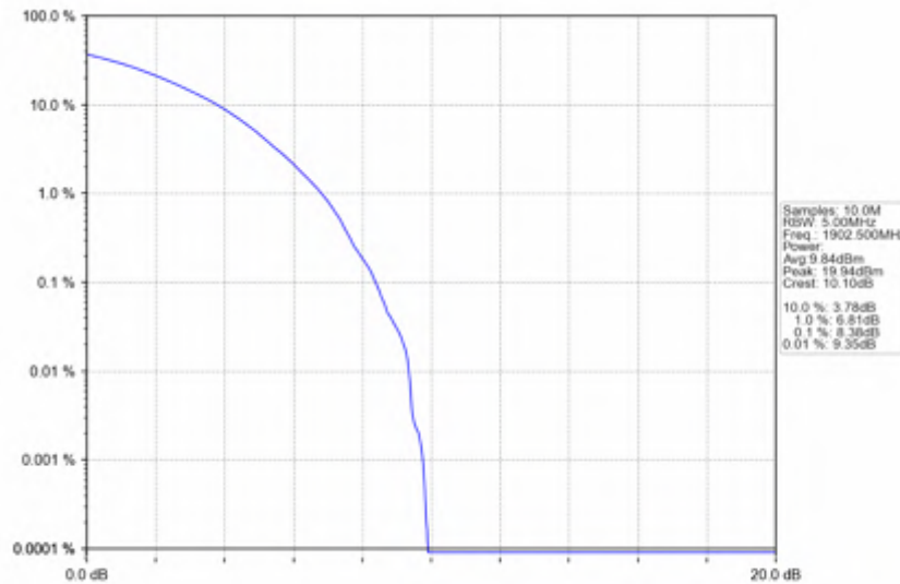
n2_15kHz_SISO_NTV_15MHz_CP-OFDM QPSK_1902.5MHz_Outer_Full
