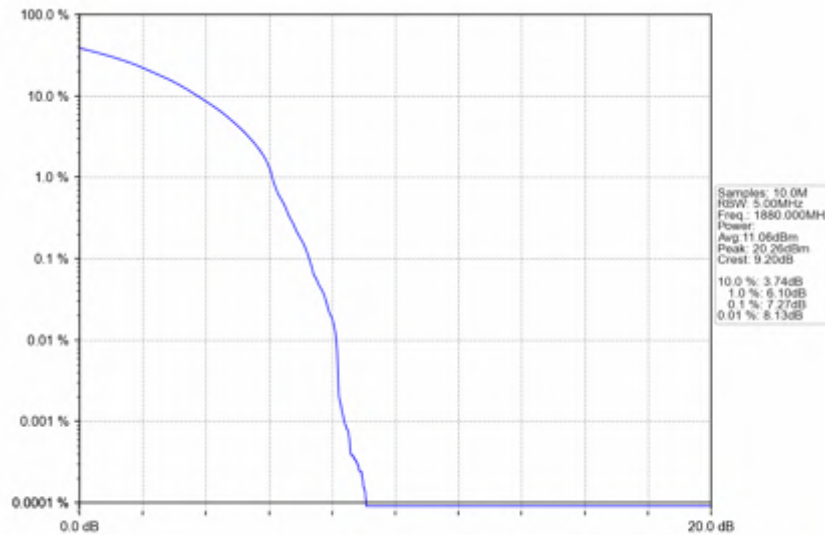
n2_15kHz_SISO_NTNV_15MHz_DFT-s-OFDM 16 QAM_1880MHz_Outer_Full
