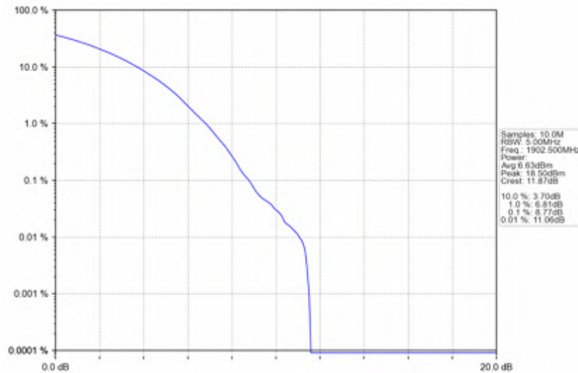
n2_30kHz_SISO_NTNV_15MHz_CP-OFDM 256 QAM_1902.5MHz_Outer_Full
