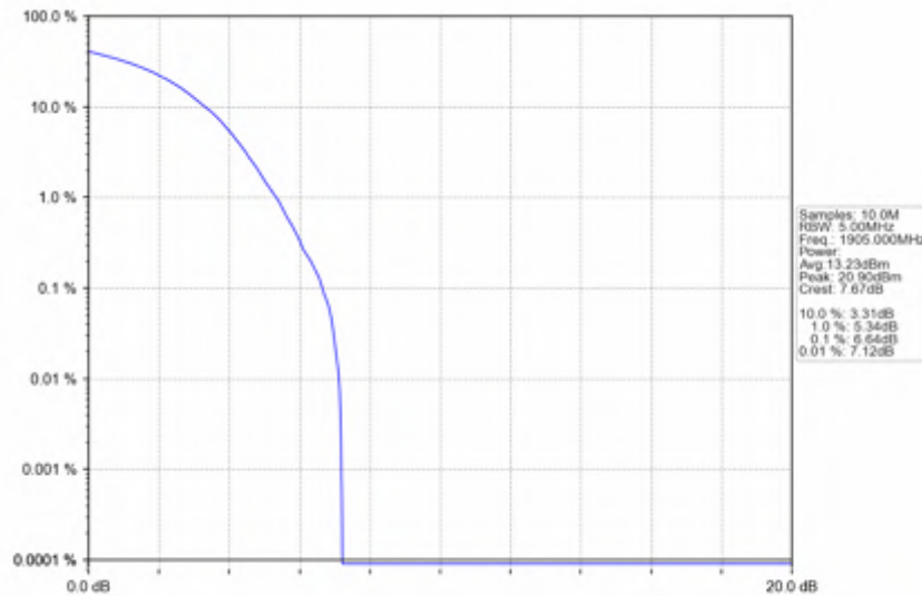
n2_30kHz_SISO_NTNV_10MHz_DFT-s-OFDM 16 QAM_1905MHz_Outer_Full
