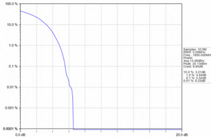
n2_15kHz_SISO_NTNV_10MHz_DFT-s-OFDM QPSK_1855MHz_Outer_Full
