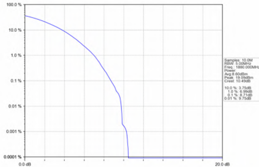
n2_15kHz_SISO_NTNV_20MHz_CP-OFDM QPSK_1880MHz_Outer_Full
