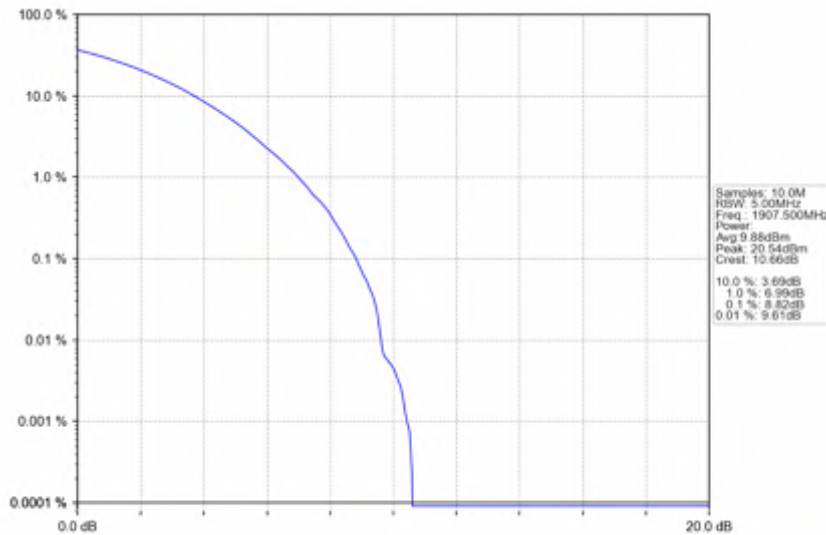
n2_15kHz_SISO_NTNV_5MHz_CP-OFDM 256 QAM_1907.5MHz_Outer_Full
