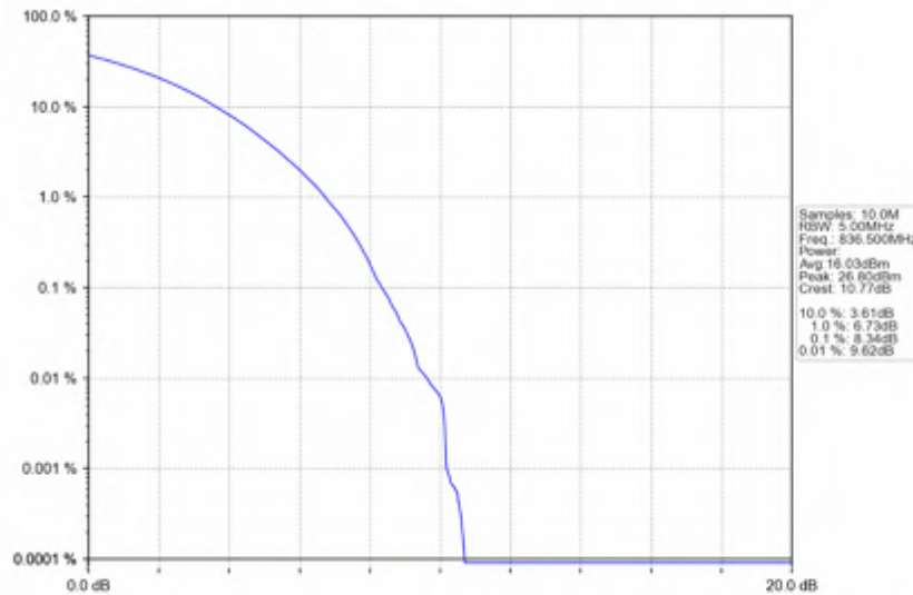
n5_15kHz_SISO_NTV_15MHz_CP-OFDM 64 QAM_836.5MHz_Outer_Full
