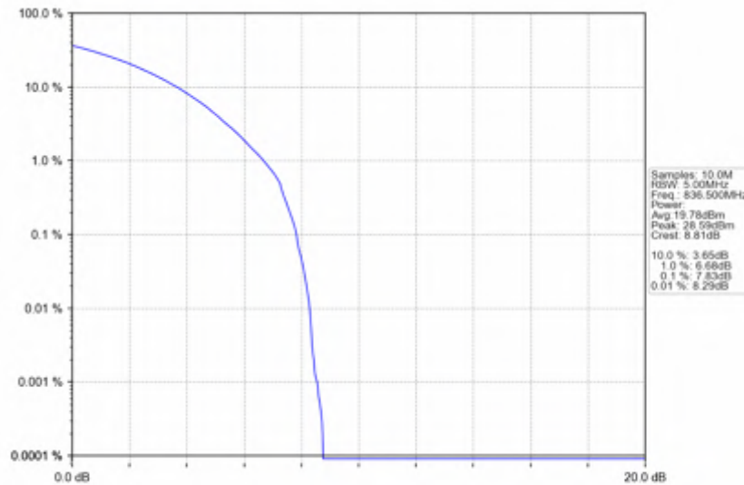
n5_15kHz_SISO_NTV_5MHz_CP-OFDM 64 QAM_836.5MHz_Outer_Full
