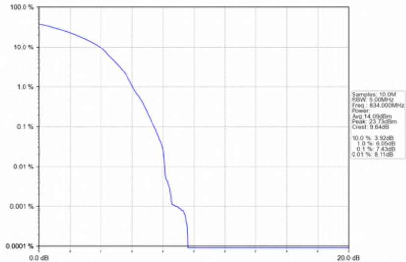
n5_15kHz_SISO_NTNV_20MHz_DFT-s-OFDM 256 QAM_834MHz_Outer_Full
