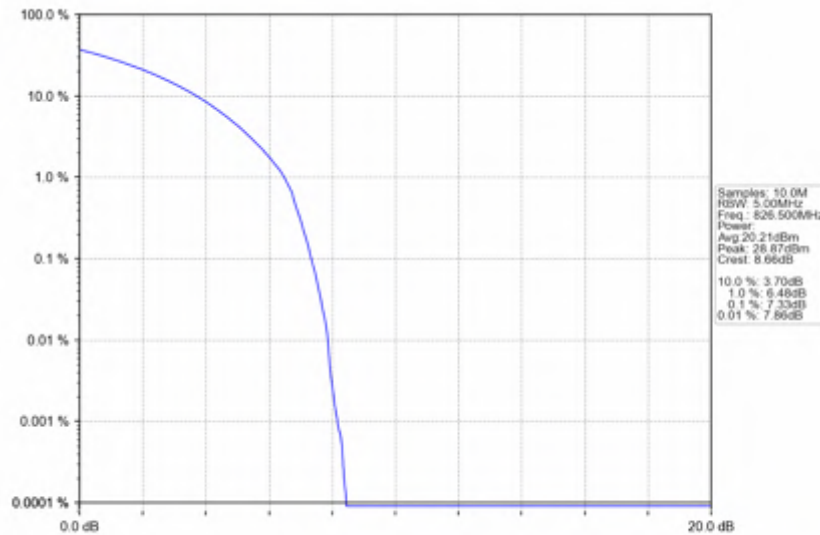
n5_15kHz_SISO_NTNV_5MHz_CP-OFDM_16 QAM_826.5MHz_Outer_Full
