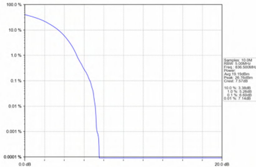
n5_15kHz_SISO_NTNV_10MHz_DFT-s-OFDM 64 QAM_836.5MHz_Outer_Full
