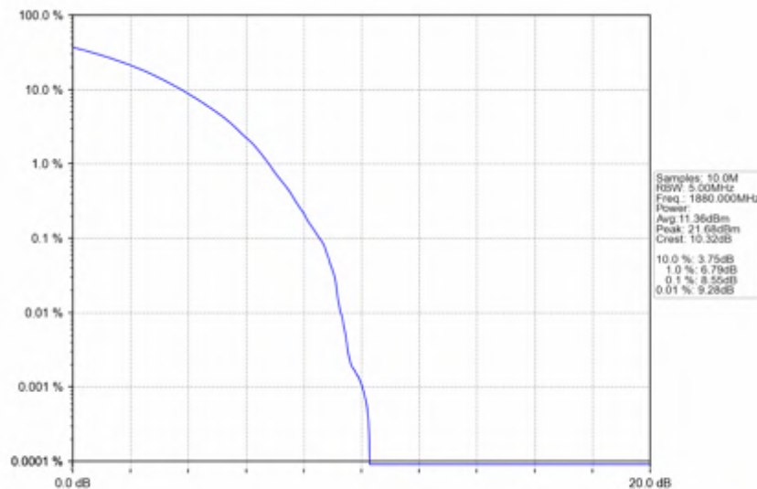
n2_15kHz_SISO_NTNV_10MHz_CP-OFDM 16 QAM_1880MHz_Outer_Full
