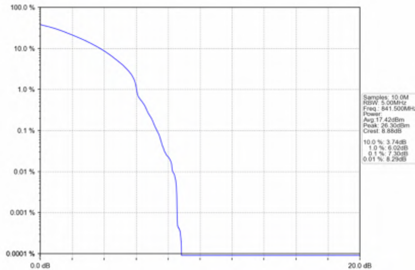
n5_15kHz_SISO_NTV_15MHz_DFT-s-OFDM_64_QAM_841.5MHz_Outer_Full
