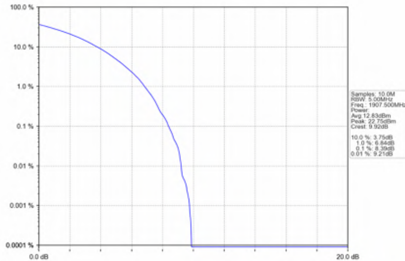
n2_15kHz_SISO_NTV_5MHz_CP-OFDM 64 QAM_1907.5MHz_Outer_Full
