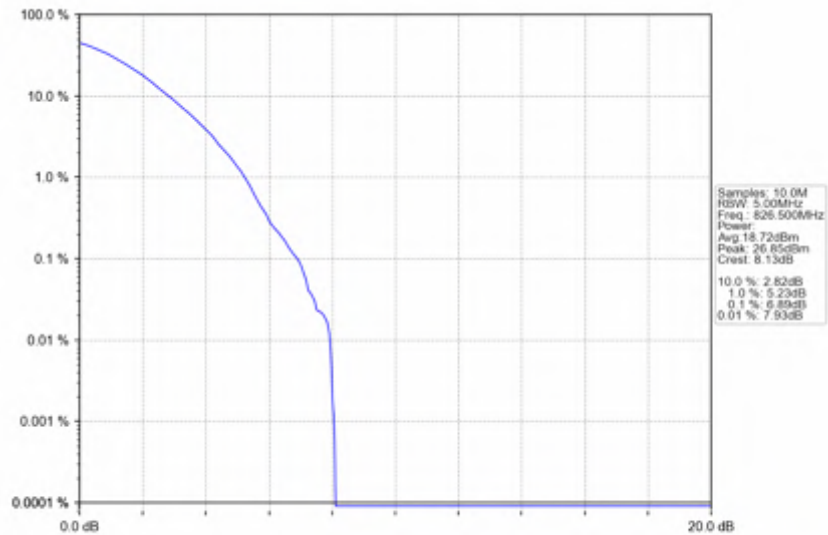
n5_15kHz_SISO_NTV_5MHz_DFT-s-OFDM_256_QAM_826.5MHz_Outer_Full
