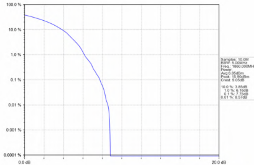
n2_15kHz_SISO_NTNV_20MHz_DFT-s-OFDM_256_QAM_1860MHz_Outer_Full
