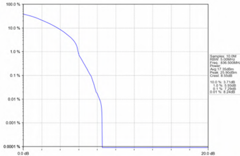
n5_15kHz_SISO_NTV_15MHz_DFT-s-OFDM_64_QAM_836.5MHz_Outer_Full
