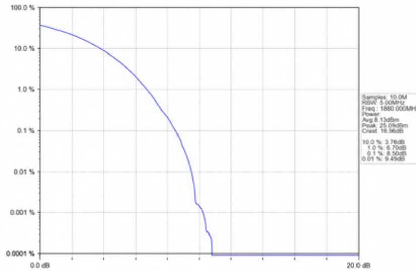
n2_15kHz_SISO_NTNV_20MHz_CP-OFDM 64 QAM_1880MHz_Outer_Full
