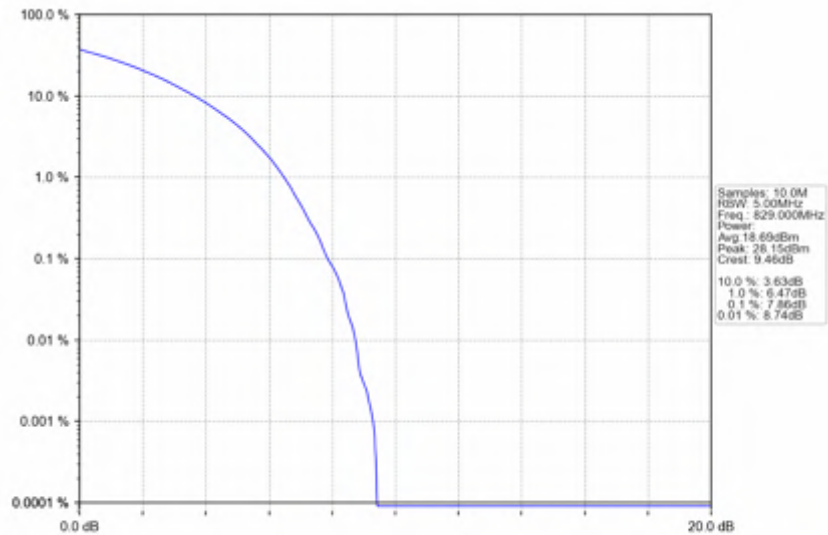
n5_30kHz_SISO_NTNV_10MHz_CP-OFDM 16 QAM_829MHz_Outer_Full
