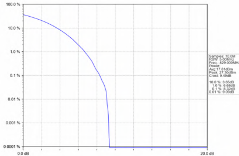
n5_15kHz_SISO_NTNV_10MHz_CP-OFDM 64 QAM_829MHz_Outer_Full
