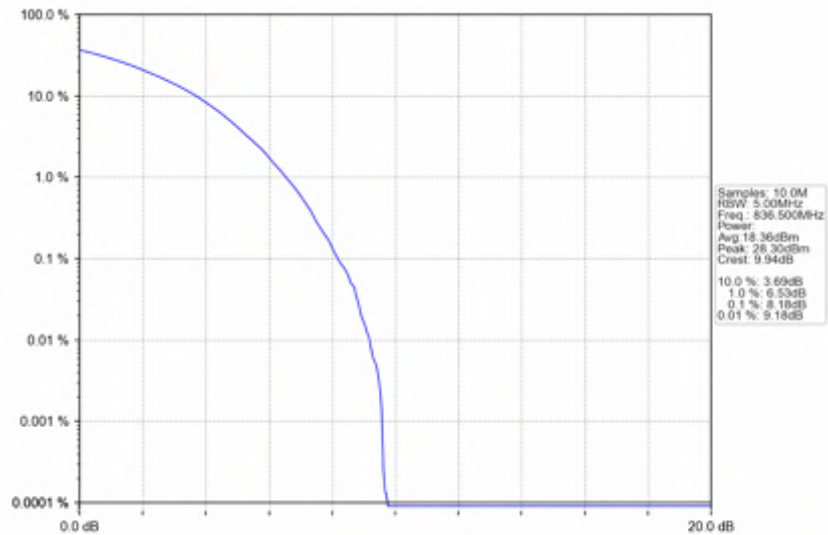
n5_15kHz_SISO_NTV_10MHz_CP-OFDM 16 QAM_836.5MHz_Outer_Full
