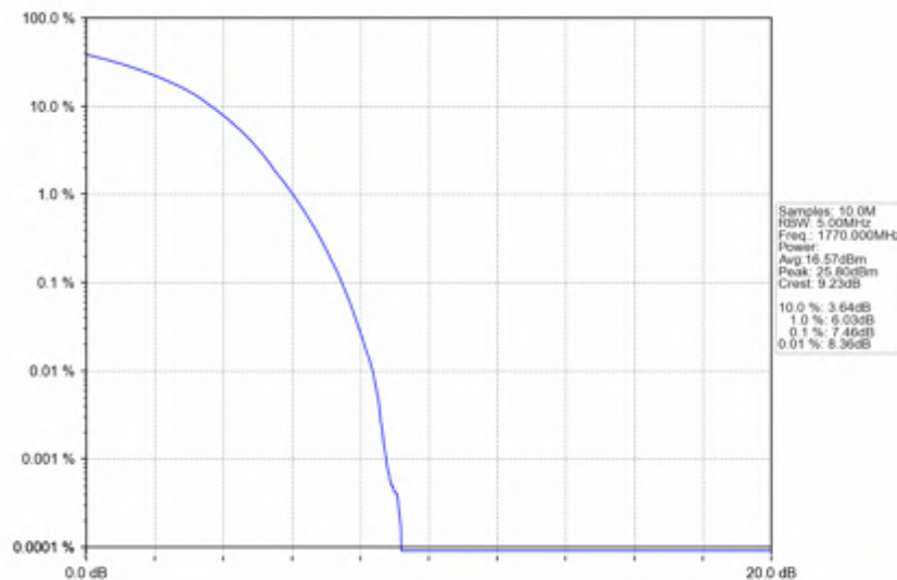
Band66_20MHz_16QAM_HCH_1770MHz_RB_100_0_NTNV
