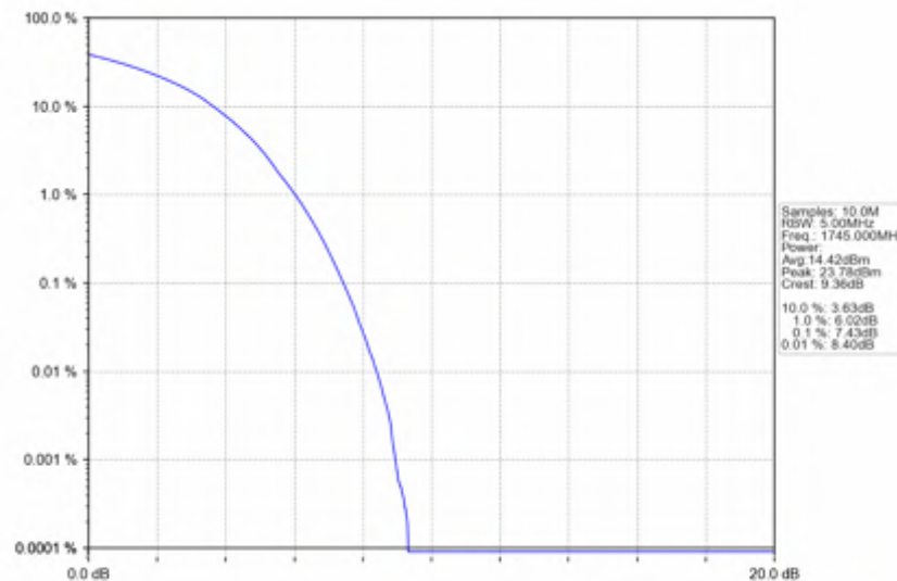
Band66_20MHz_256QAM_MCH_1745MHz_RB_100_0_NTNV
