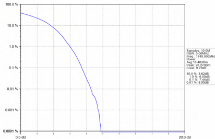
Band66_20MHz_16QAM_MCH_1745MHz_RB_100_0_NTNV
