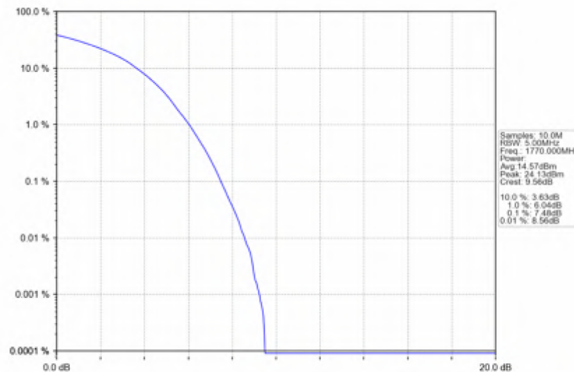
Band66_20MHz_256QAM_HCH_1770MHz_RB_100_0_NTNV
