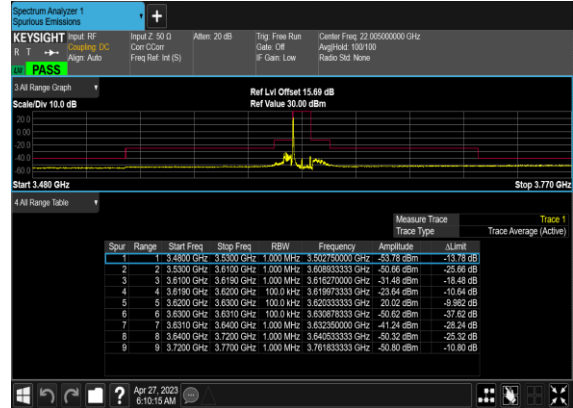
N48(10M)_DFT-s- OFDM_BPSK_Edge_1RB_Left_Mid_CH
