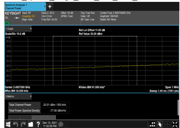
N41(50M)_DFT-s- OFDM_QPSK_Edge_1RB_Left_Low_CH_CHP_PASS
