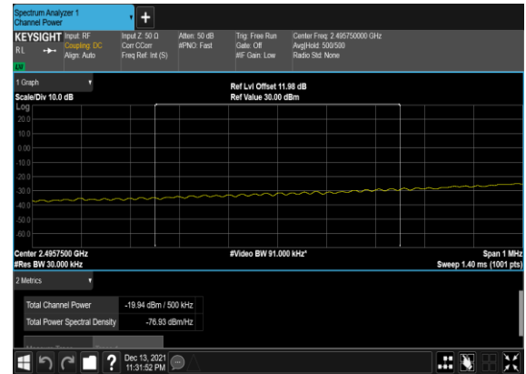
N41(50M)_DFT-s- OFDM_BPSK_Edge_1RB_Left_Low_CH_CHP_PASS
