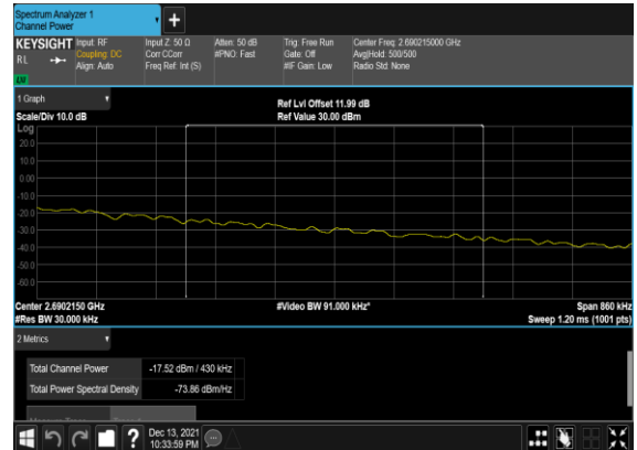
N41(20M)_DFT-s- OFDM_BPSK_Edge_1RB_Right_High_CH_chp_PASS
