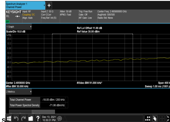
N41(20M)_DFT-s- OFDM_BPSK_Edge_1RB_Left_Low_CH_CHP_PAS
