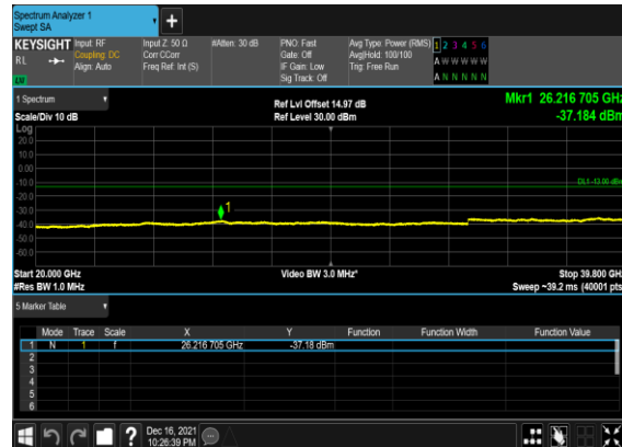
N77(10M)_CP- OFDM_QPSK_Edge_1RB_Left_Low_CH
