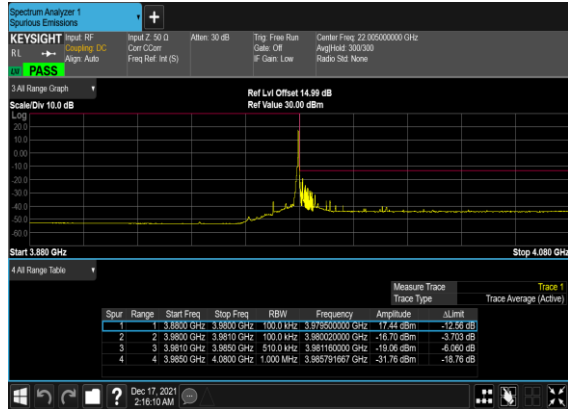
N77(10M)_CP- OFDM_QPSK_Edge_1RB_Right_High_CH
