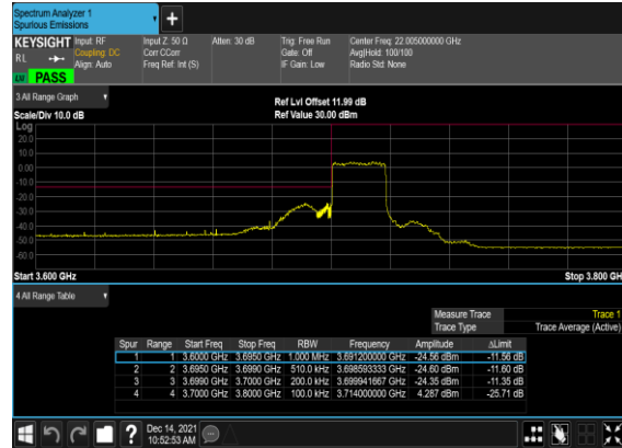
N77(20M)_DFT-s- OFDM_BPSK_Outer_Full_Low_CH
