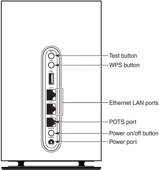
Figure 5 Location of physical interfaces on the side of the Nokia FastMile 4G Gateway
