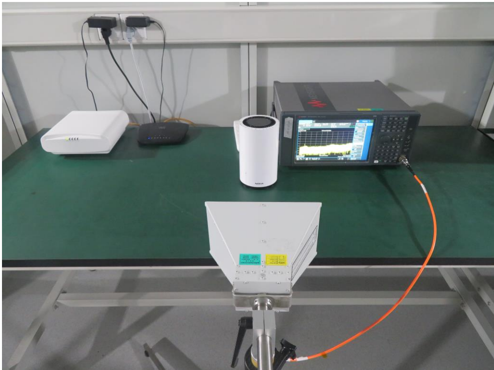
Description: CBRS Test Setup
