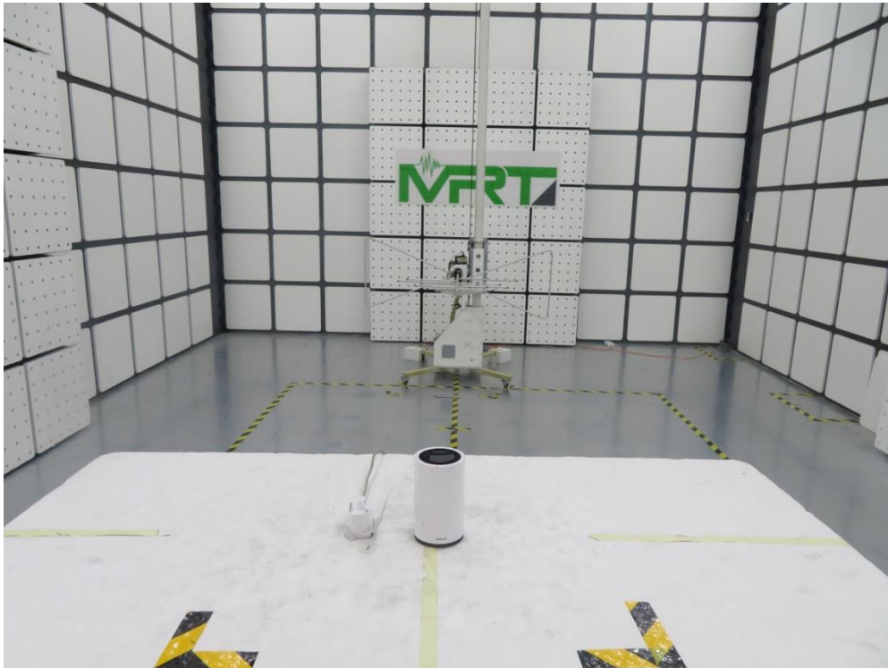
Description: Radiated Spurious Emissions Test Setup for Below 1GHz
