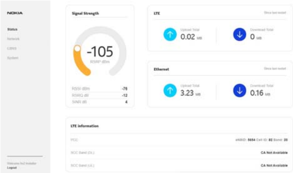
Figure 59 Example of the top part of the Status screen when the FastMile 4G Receiver is connected to a cell
