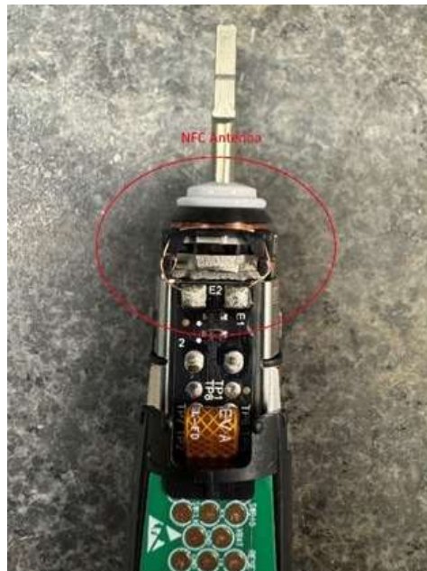
Figure 10: NFC Antenna on PCB2
