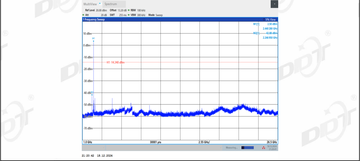
BLE_2M_Left side_2478_0~Reference
