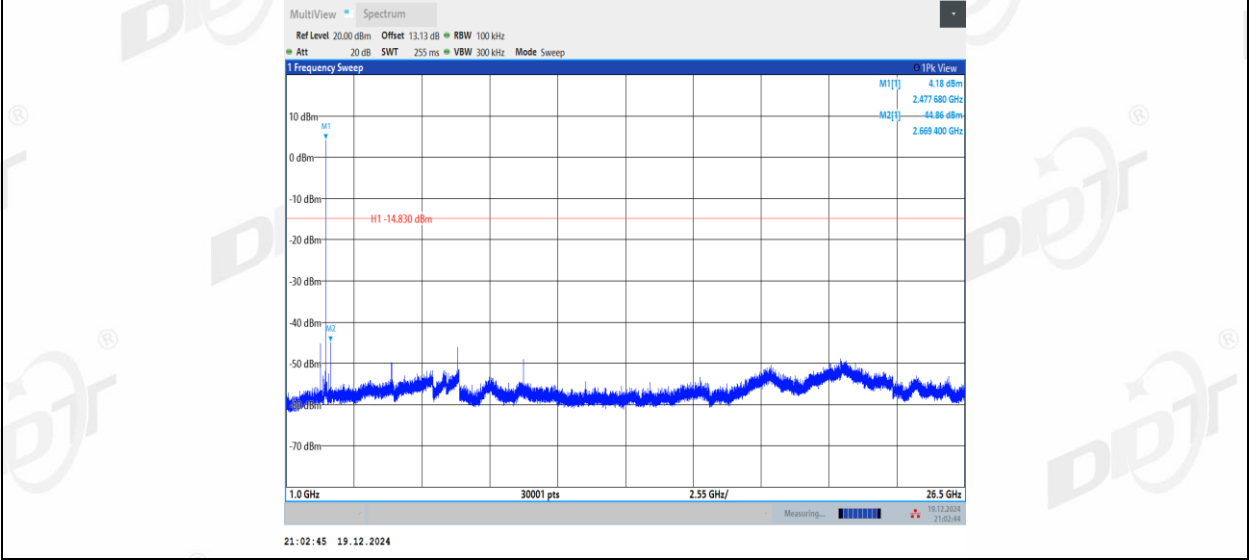
BLE_2M_Right side_2478_0~Reference
