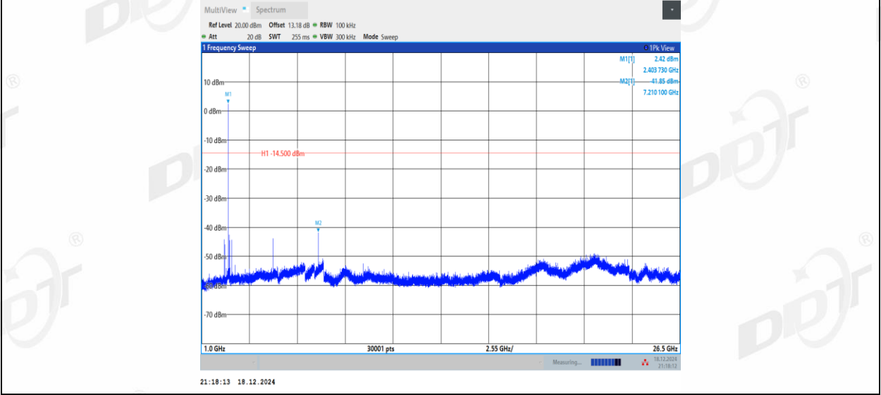
BLE_2M_Left side_2440_0~Reference
