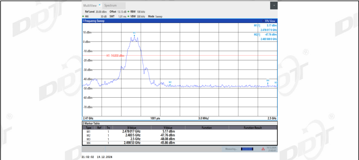
BLE_2M_Right side_High_2478
