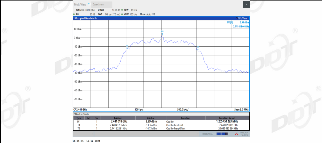
2DH5_Right side_2441
