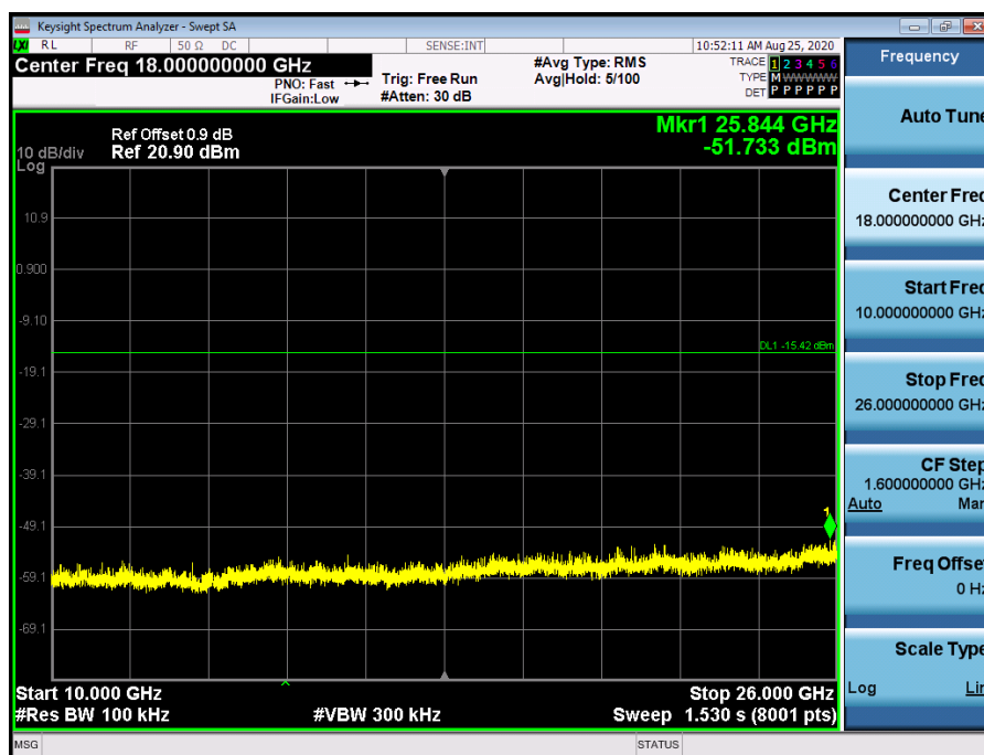
RF Conducted Spurious Emissions_3DH5_2441
