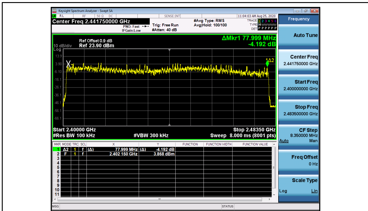
Hopping Channel Number_3DH5_2402
