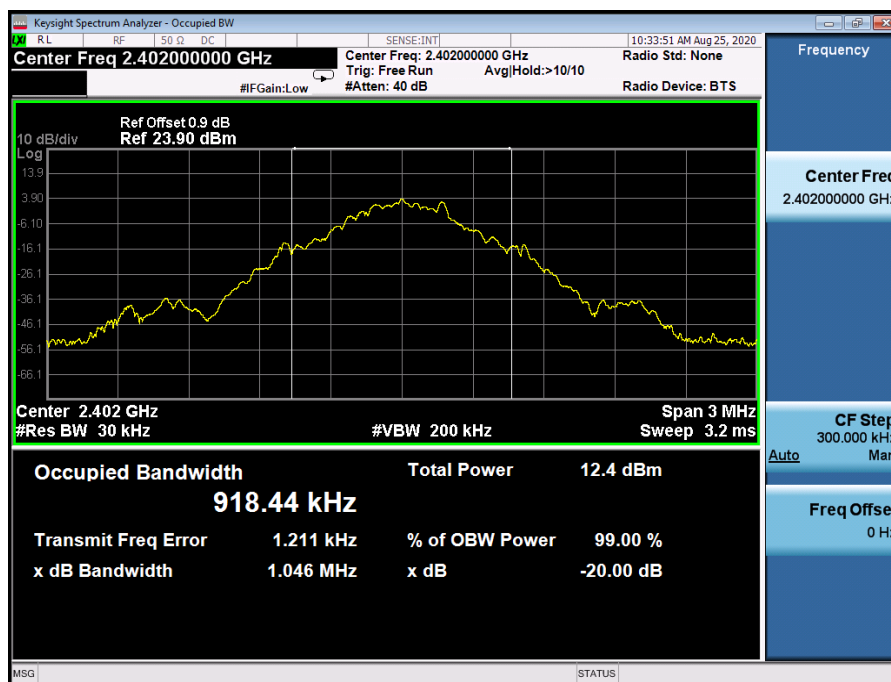
20 dB Bandwidth_DH5_2402
