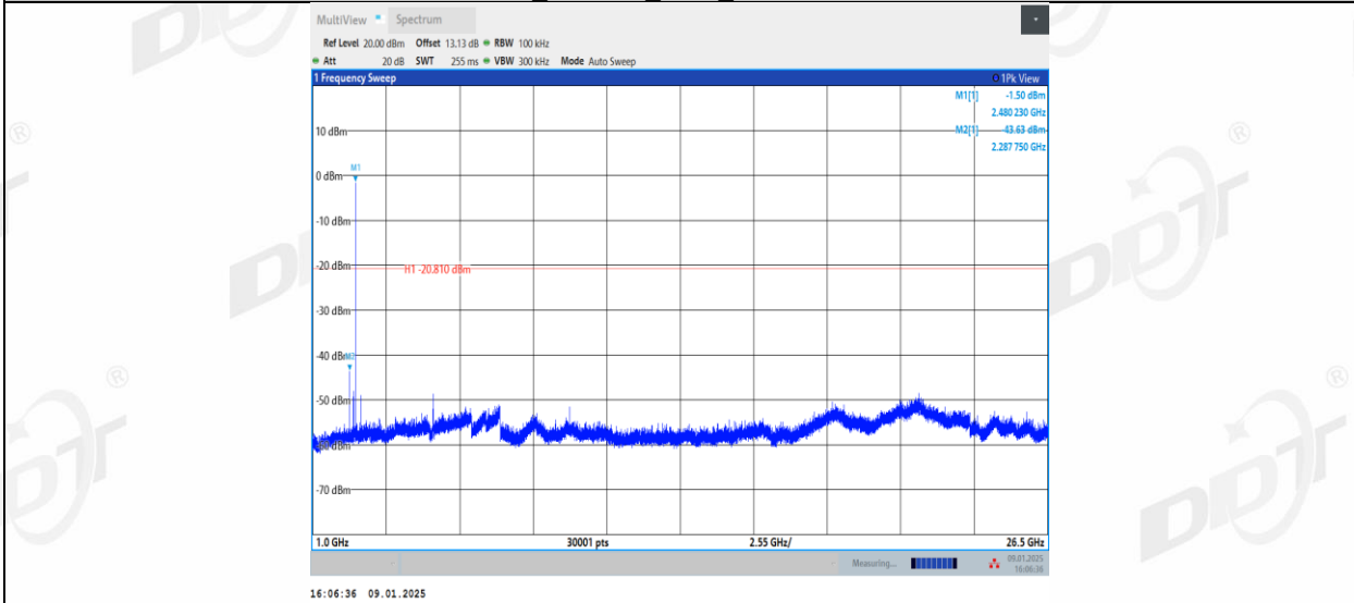
DH5_Right side_2480_0~Reference
