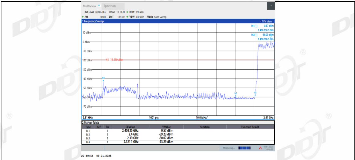
3DH5_Left side_High_Hop_2480
