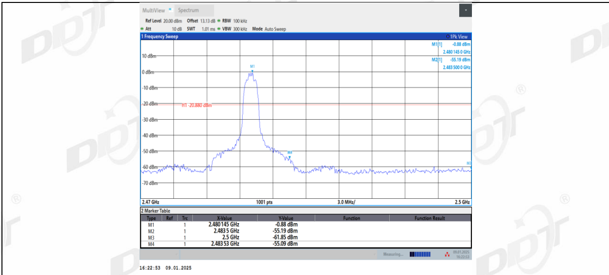
3DH5_Right side_High_2480
