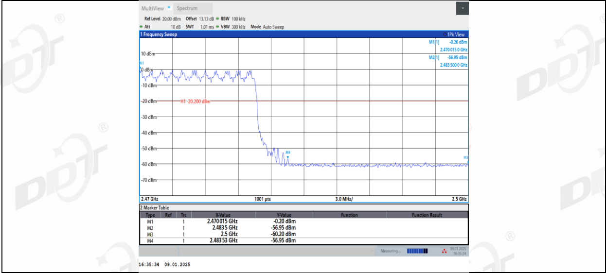
3DH5_Right side_High_Hop_2480
