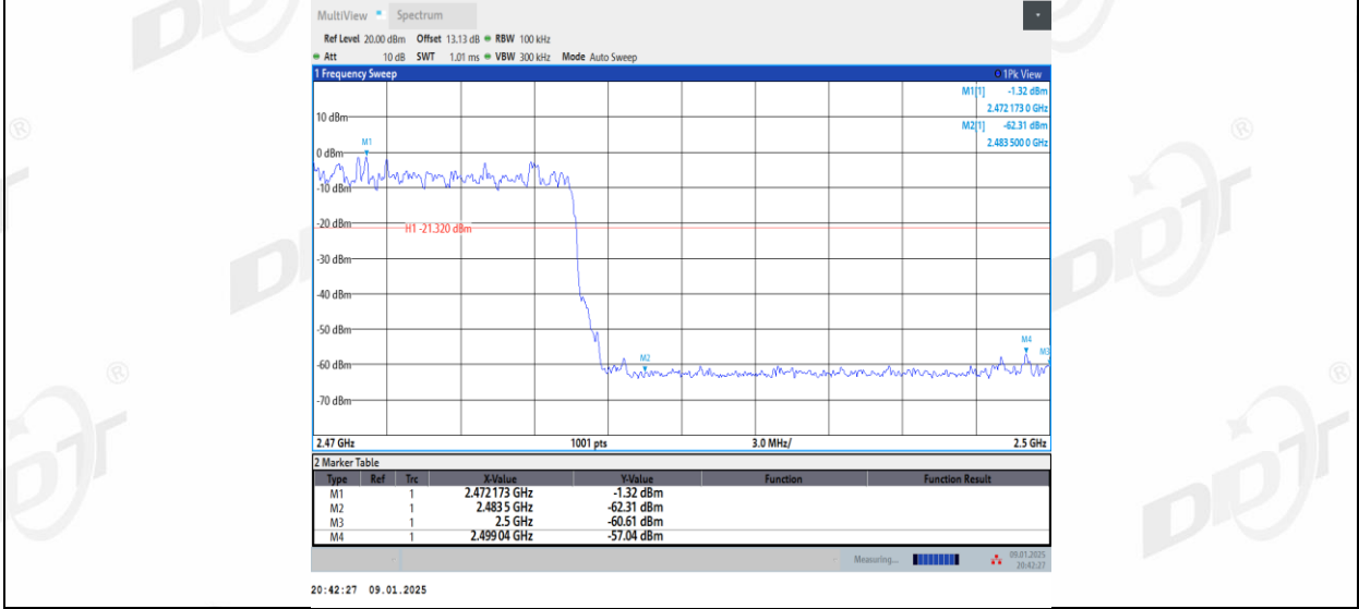
3DH5_Right side_High_Hop_2480
