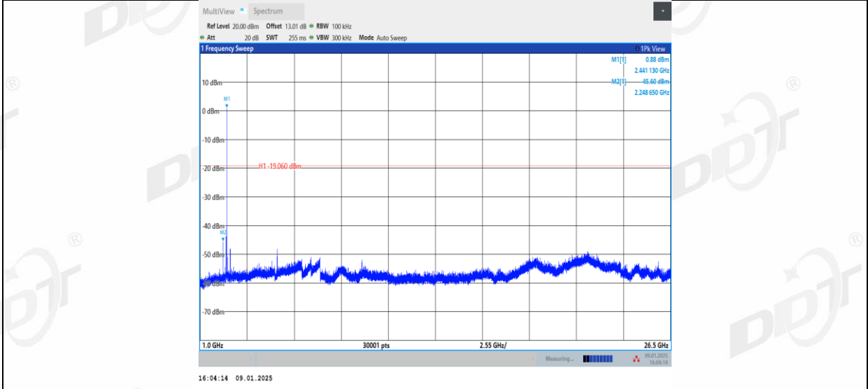
DH5_Right side_2441_0~Reference
