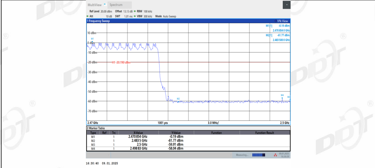
2DH5_Right side_High_Hop_2480
