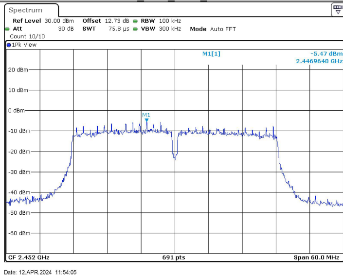
11N40SISO_Ant2_2452_0~Reference
