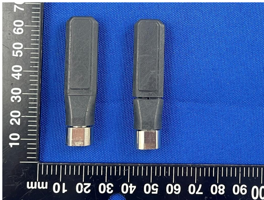
Accessory-Antenna
