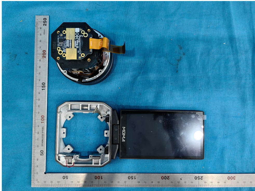
Camera Lens 1
