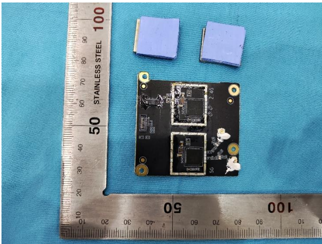
WIFI Module Front 1
