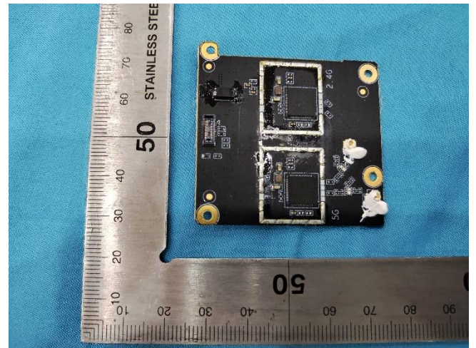
WIFI Module Front 2
