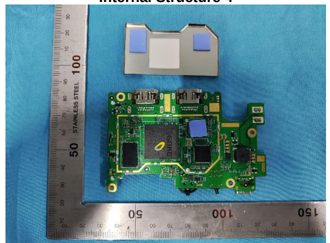
Mainboard Back
