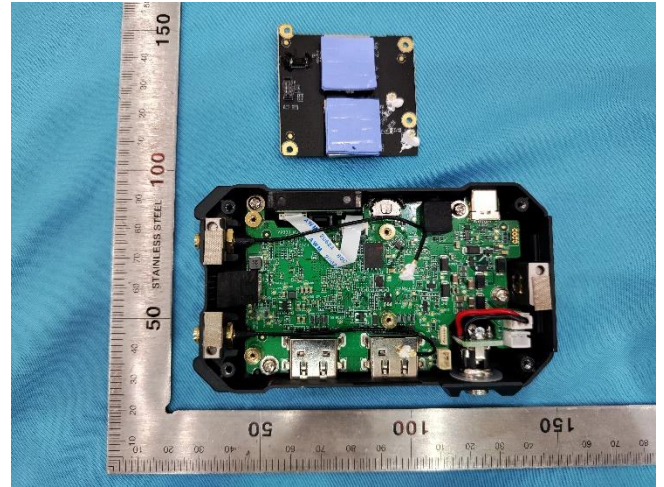
Internal Structure 2
