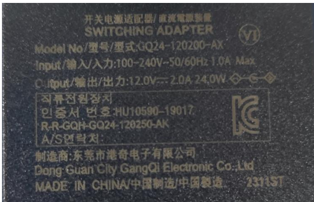
Switching Adapter
