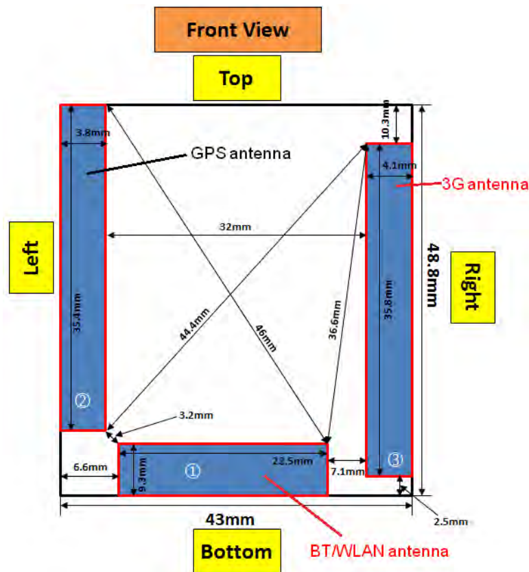
Antenna location
