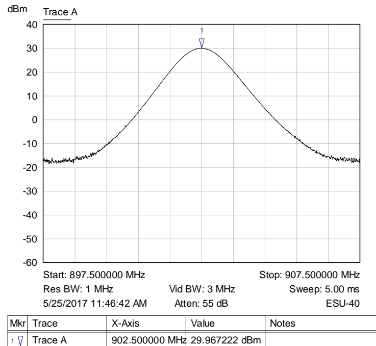
Graph 35: Lowest Channel Output Power – 31.25 kHz LoRa
