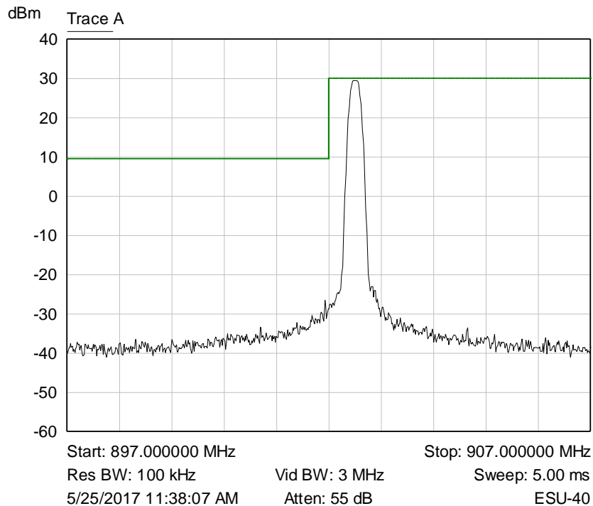
Graph 44: Lower Channel Plot –62.5 kHz LoRa
