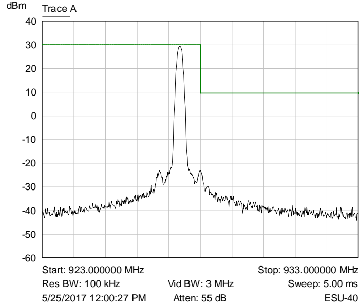
Graph 48: Upper Channel Plot – 31.25 kHz LoRa
