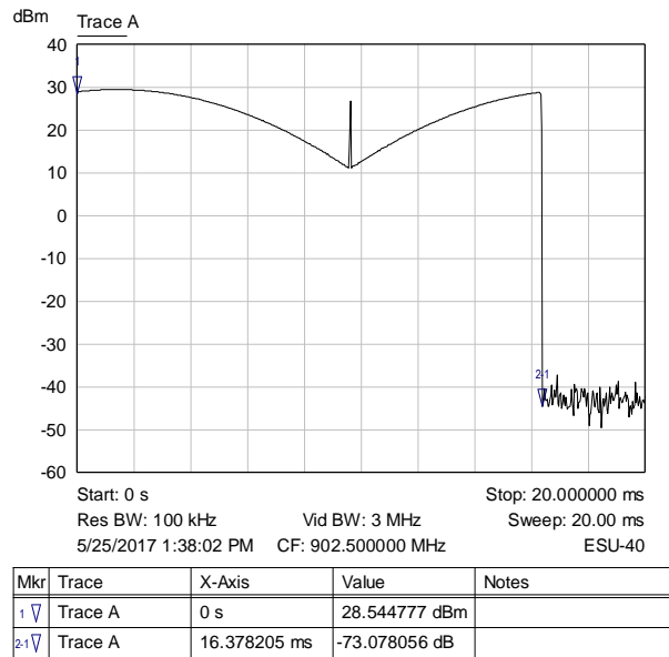
Graph 16: Data On Time
