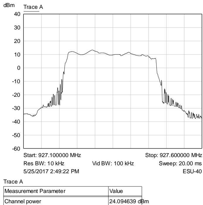
Graph 64: Upper Channel Output Power – 250 kHz LoRa
