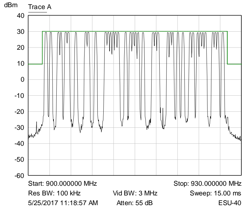
Graph 43: Operating Band While Hopping – 125 kHz LoRa
