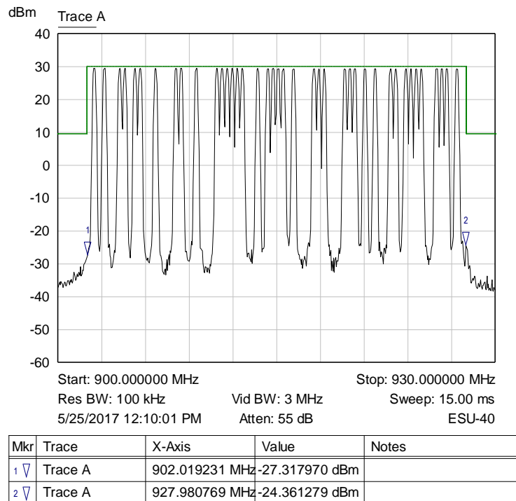
Graph 49: Operating Band While Hopping – 31.25 kHz LoRa
