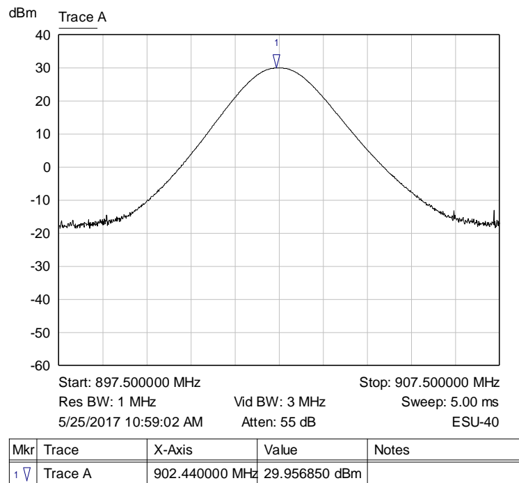
Graph 29: Lowest Channel Output Power – 125 kHz LoRa
