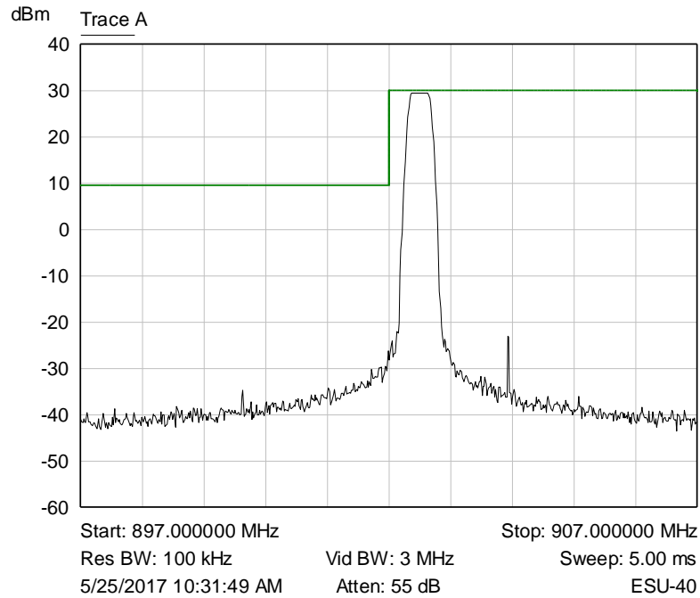
Graph 38: Lower Channel Plot – 250 kHz LoRa
