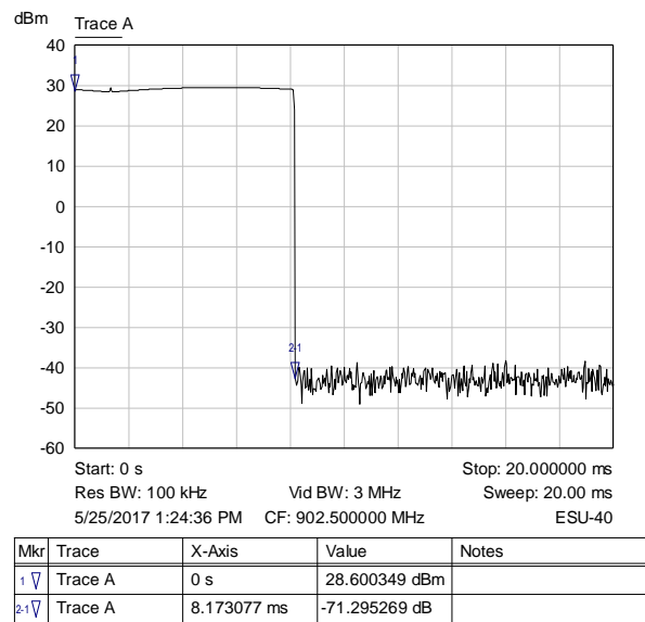
Graph 22: Data On Time
