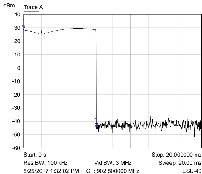
Graph 18: Preamble On Time
