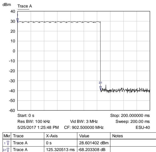
Graph 21: Preamble On Time
