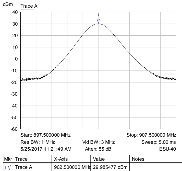
Graph 32: Lowest Channel Output Power – 62.5 kHz LoRa
