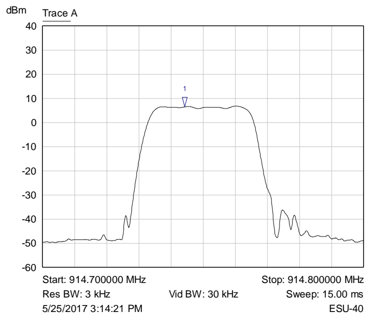
Graph 59: Lower Channel PSD – 31.25 kHz LoRa
