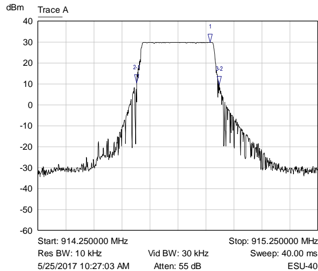
Graph 2: Lowest Channel 20 dB Bandwidth – 250 kHz LoRa
