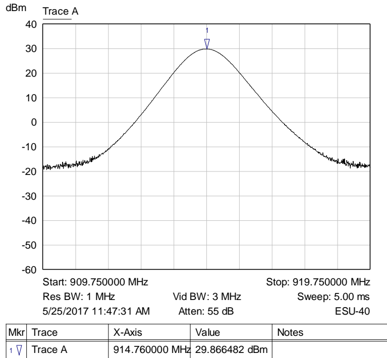
Graph 36: Middle Channel Output Power – 31.25 kHz LoRa
