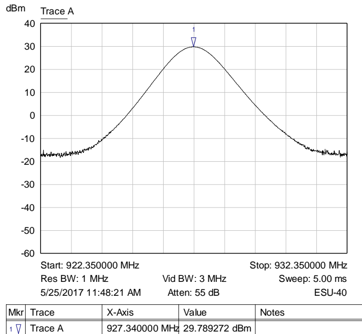
Graph 37: Upper Channel Output Power – 31.25 kHz LoRa
