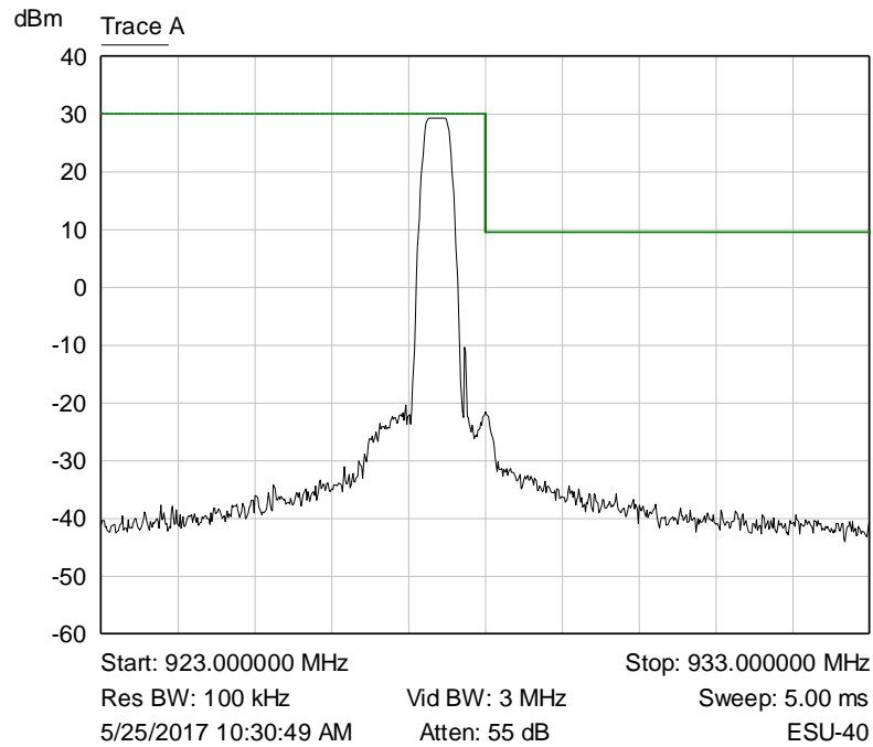
Graph 39: Upper Channel Plot – 250 kHz LoRa
