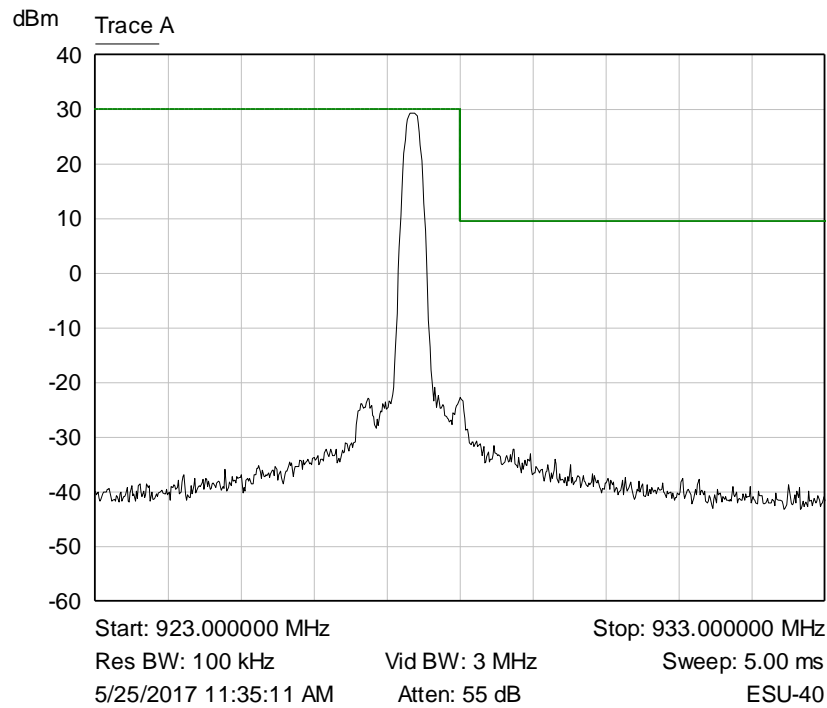
Graph 45: Upper Channel Plot – 62.5 kHz LoRa
