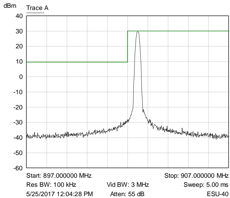
Graph 47: Lower Channel Plot – 31.25 kHz LoRa
