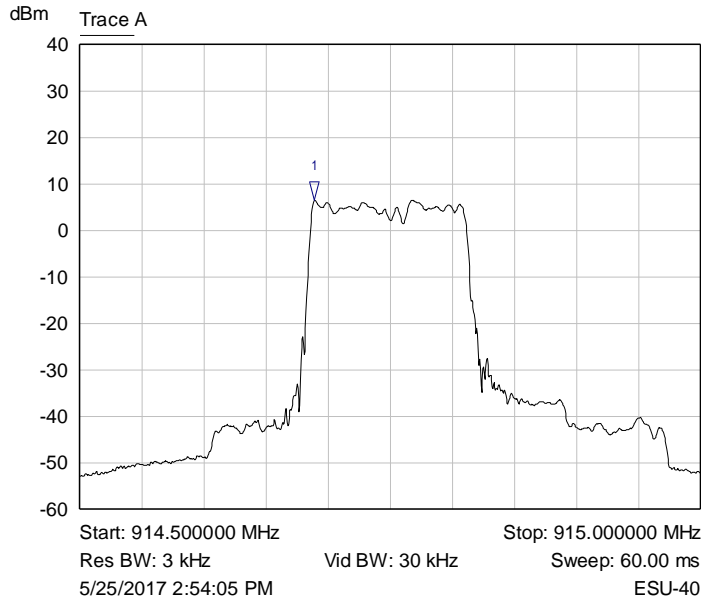
Graph 53: Lower Channel PSD – 125kHz LoRa
