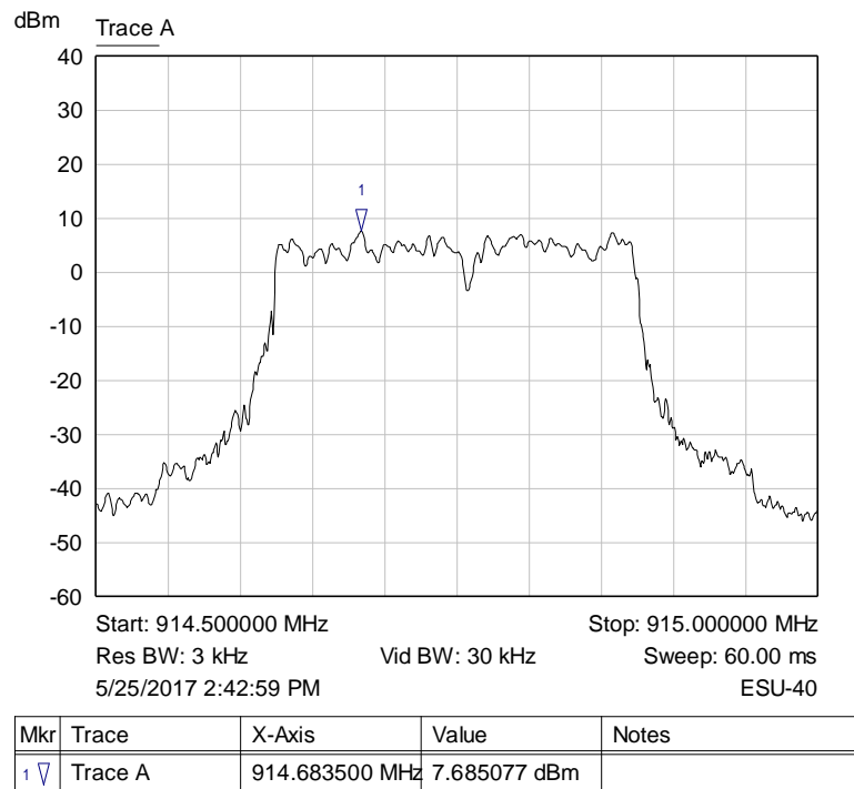
Graph 51: Middle Channel PSD – 250 kHz LoRa
