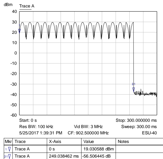
Graph 15: Preamble On Time
