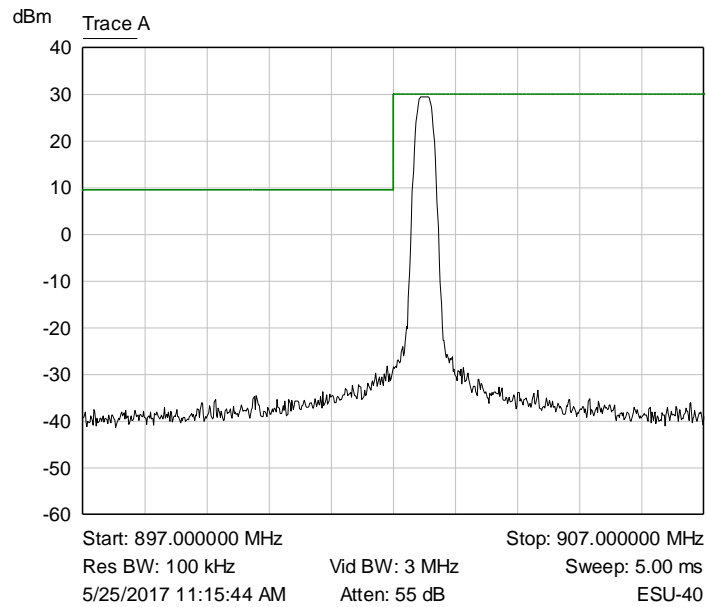
Graph 41: Lower Channel Plot – 125 kHz LoRa
