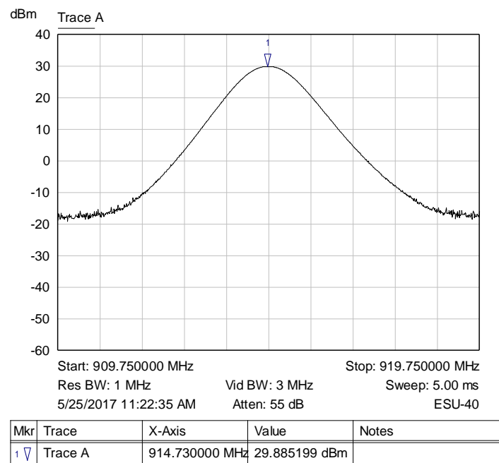
Graph 33: Middle Channel Output Power – 62.5 kHz LoRa
