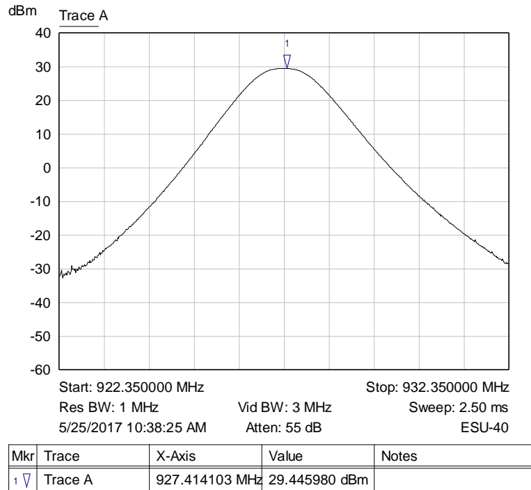
Graph 28: Upper Channel Output Power – 250 kHz LoRa
