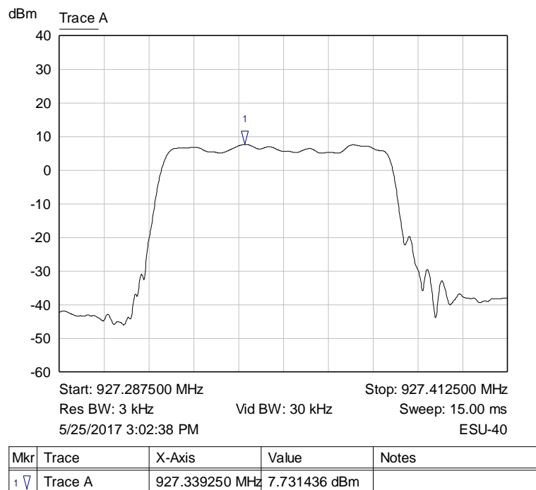
Graph 57: Middle Channel PSD – 62.5 kHz LoRa
