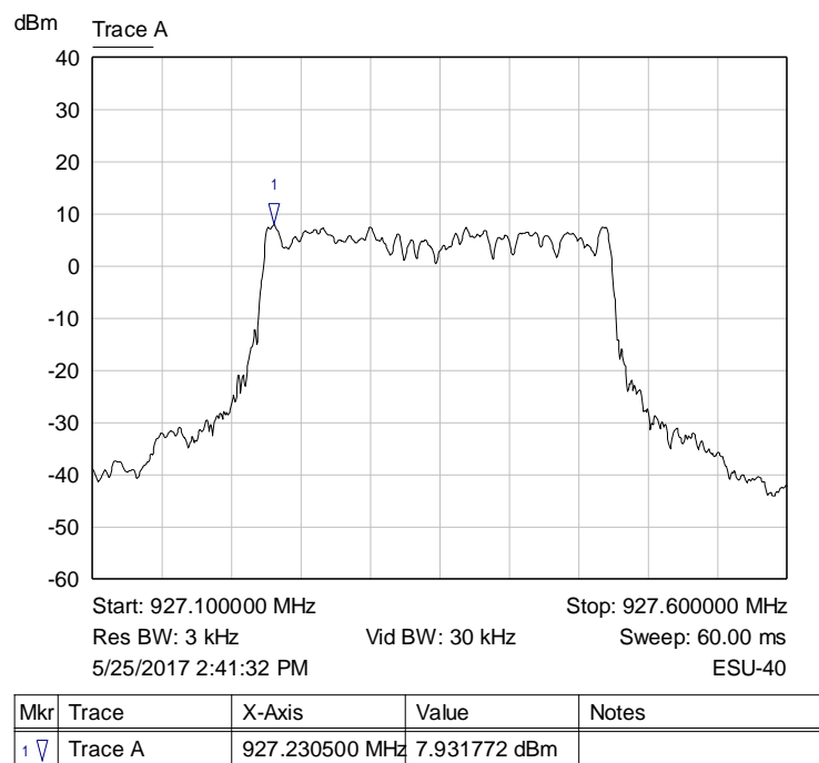
Graph 52: Upper Channel PSD – 250 kHz LoRa
