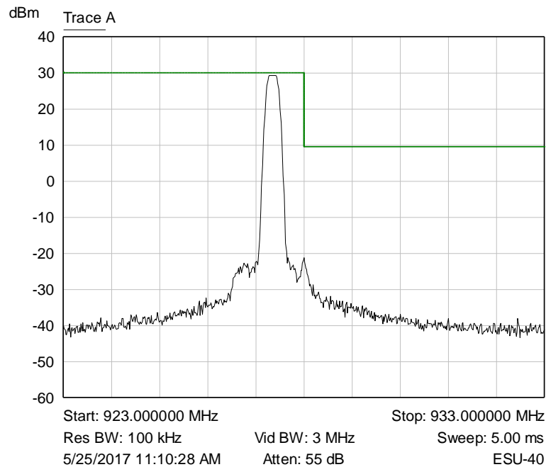
Graph 42: Upper Channel Plot – 125 kHz LoRa
