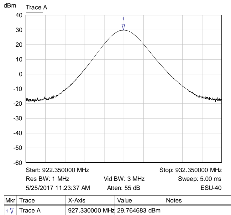
Graph 34: Upper Channel Output Power – 62.5 kHz LoRa
