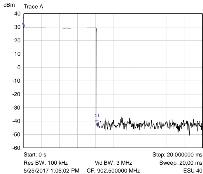
Graph 24: Preamble On Time
