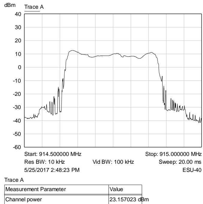
Graph 63: Middle Channel Output Power – 250 kHz LoRa
