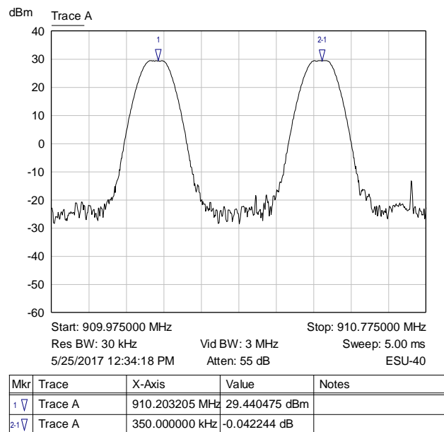
Graph 1: Channel Separation Plot
