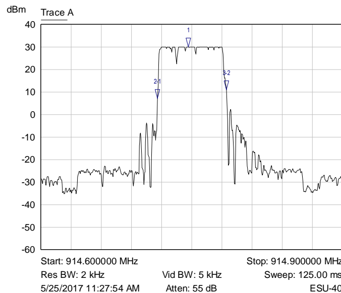
Graph 8: Lowest Channel 20 dB Bandwidth – 62.5 kHz LoRa
