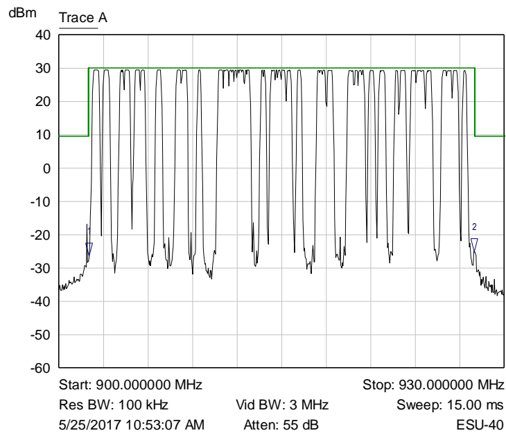
Graph 39: Upper Channel Plot – 250 kHz LoRa
