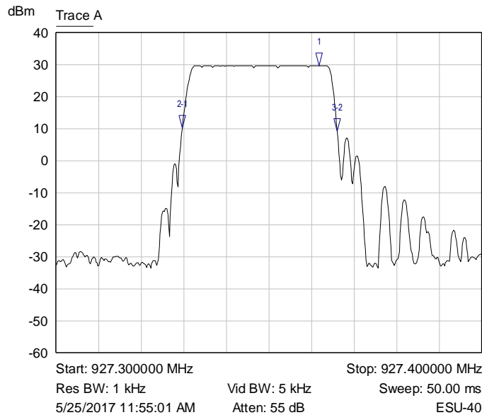
Graph 12: Middle Channel 20 dB Bandwidth – 31.25 kHz LoRa
