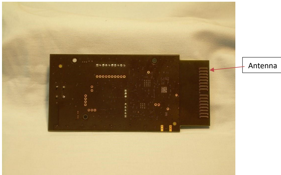
Photograph 2 – Back View of the EUT
