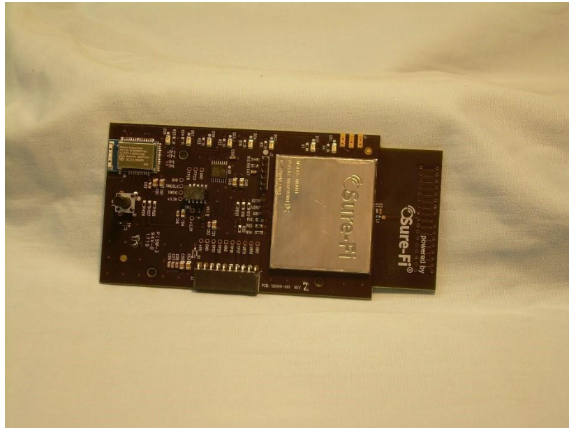
Photograph 1 – Front View of Component Side of the EUT
