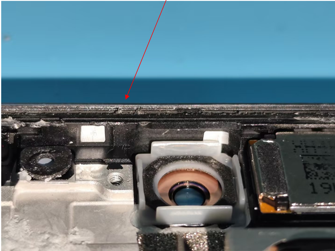
ANT12 GPS L1 + BT + 2.4G Wi-Fi Chain 0
