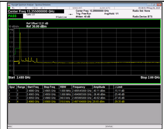
41-41-20MHz-5MHz-16QAM@16QAM-16QAM@16QAM-3 9750-39867-1RB#0@100RB#0-0RB#0@25RB#0-PASS
