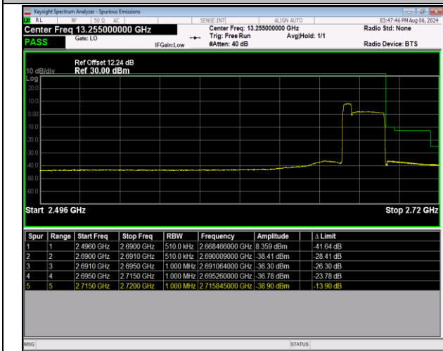
41-41-5MHz-20MHz-QPSK@QPSK-QPSK@QPSK-41373 -41490-25RB#0@25RB#0-100RB#0@100RB#0-PASS
