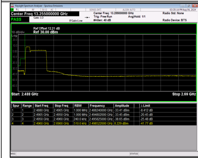
41-41-5MHz-20MHz-QPSK@QPSK-QPSK@QPSK-39683 -39800-25RB#0@25RB#0-100RB#0@100RB#0-PASS
