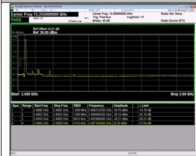
41-41-20MHz-10MHz-QPSK@QPSK-QPSK@QPSK-3975 0-39894-1RB#0@100RB#0-0RB#0@50RB#0-PASS
