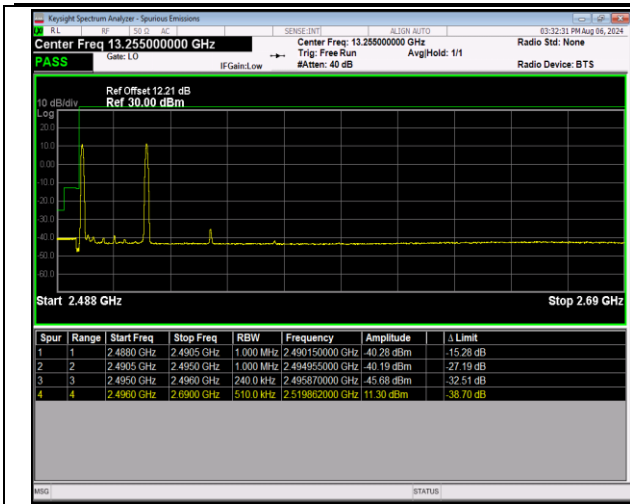
41-41-5MHz-20MHz-QPSK@QPSK-QPSK@QPSK-39683 -39800-1RB#0@25RB#0-1RB#99@100RB#0-PASS
