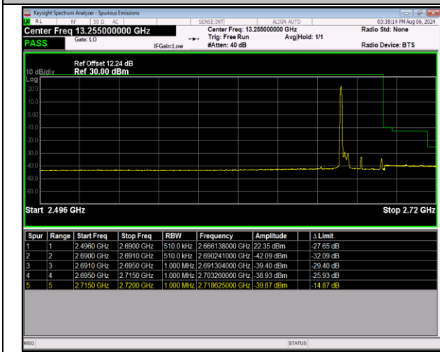
41-41-5MHz-20MHz-QPSK@QPSK-QPSK@QPSK-41373 -41490-1RB#0@25RB#0-ORB#0@100RB#0-PASS
