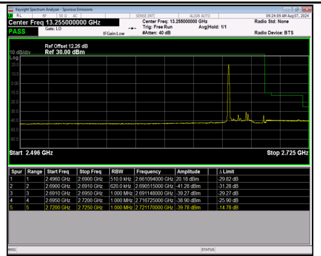
41-41-20MHz-10MHz-16QAM@16QAM-16QAM@16QAM- 41391-41535-1RB#0@100RB#0-0RB#0@50RB#0-PASS
