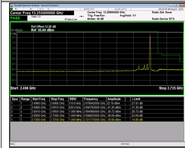
41-41-20MHz-10MHz-QPSK@QPSK-QPSK@QPSK-4139 1-41535-1RB#99@100RB#0-0RB#0@50RB#0-PASS
