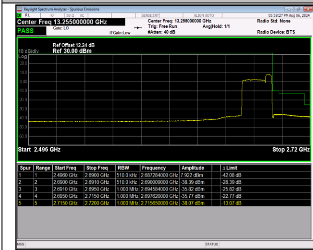
41-41-20MHz-5MHz-QPSK@QPSK-QPSK@QPSK-41440 -41557-100RB#0@100RB#0-25RB#0@25RB#0-PASS
