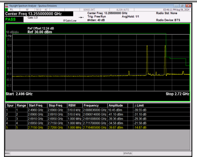
41-41-5MHz-20MHz-16QAM@16QAM-16QAM@16QAM-4 1373-41490-1RB#0@25RB#0-1RB#99@100RB#0-PASS
