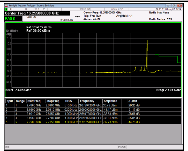
41-41-20MHz-10MHz-16QAM@16QAM-16QAM@16QAM- 41391-41535-1RB#99@100RB#0-0RB#0@50RB#0-PASS
