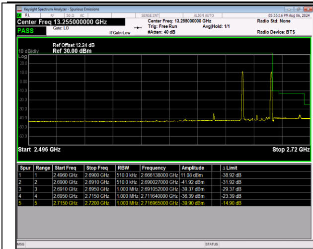
41-41-20MHz-5MHz-QPSK@QPSK-QPSK@QPSK-41440 -41557-1RB#0@100RB#0-1RB#24@25RB#0-PASS
