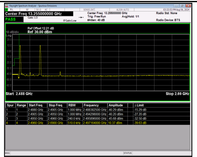
41-41-5MHz-20MHz-16QAM@16QAM-16QAM@16QAM-3 9683-39800-1RB#0@25RB#0-1RB#99@100RB#0-PASS
