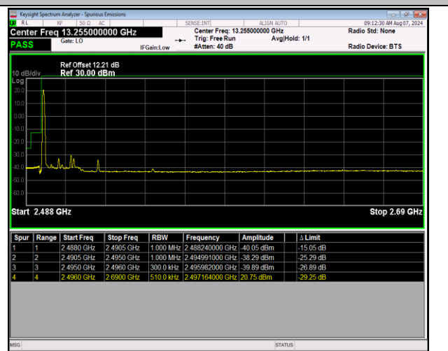
41-41-20MHz-10MHz-16QAM@16QAM-16QAM@16QAM- 39750-39894-1RB#0@100RB#0-0RB#0@50RB#0-PASS
