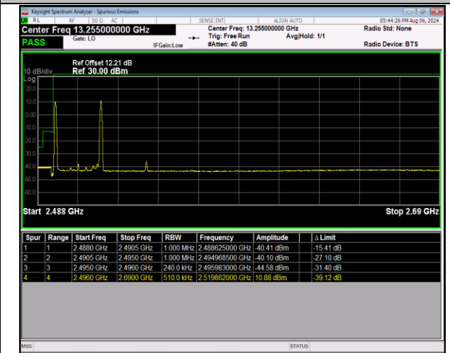
41-41-20MHz-5MHz-16QAM@16QAM-16QAM@16QAM-3 9750-39867-1RB#0@100RB#0-1RB#24@25RB#0-PASS
