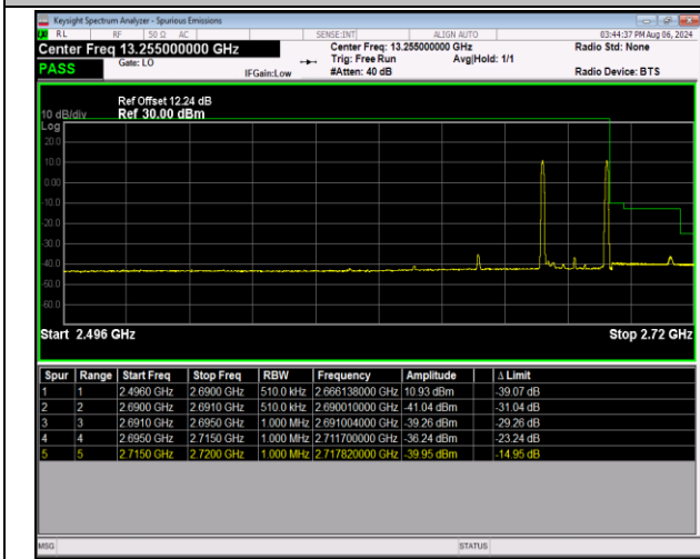
41-41-5MHz-20MHz-QPSK@QPSK-QPSK@QPSK-41373 -41490-1RB#0@25RB#0-1RB#99@100RB#0-PASS
