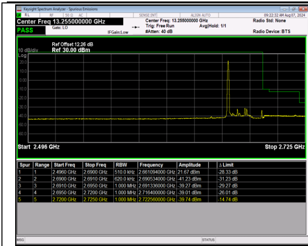
41-41-20MHz-10MHz-QPSK@QPSK-QPSK@QPSK-4139 1-41535-1RB#0@100RB#0-0RB#0@50RB#0-PASS
