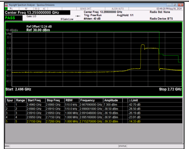
41-41-5MHz-20MHz-16QAM@16QAM-16QAM@16QAM-4 1373-41490-25RB#0@25RB#0-100RB#0@100RB#0-PAS
