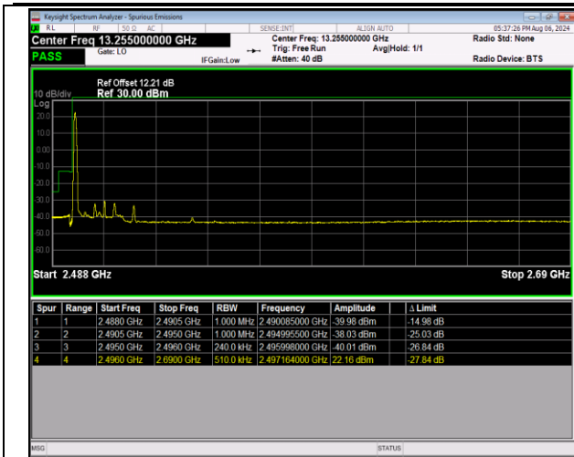
41-41-20MHz-5MHz-QPSK@QPSK-QPSK@QPSK-39750 -39867-1RB#0@100RB#0-0RB#0@25RB#0-PASS
