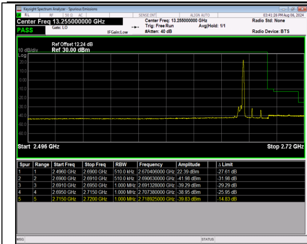
41-41-5MHz-20MHz-QPSK@QPSK-QPSK@QPSK-41373 -41490-1RB#24@25RB#0-0RB#0@100RB#0-PASS
