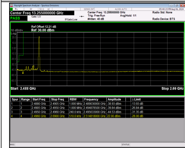
41-41-20MHz-5MHz-QPSK@QPSK-QPSK@QPSK-39750 -39867-1RB#99@100RB#0-0RB#0@25RB#0-PASS
