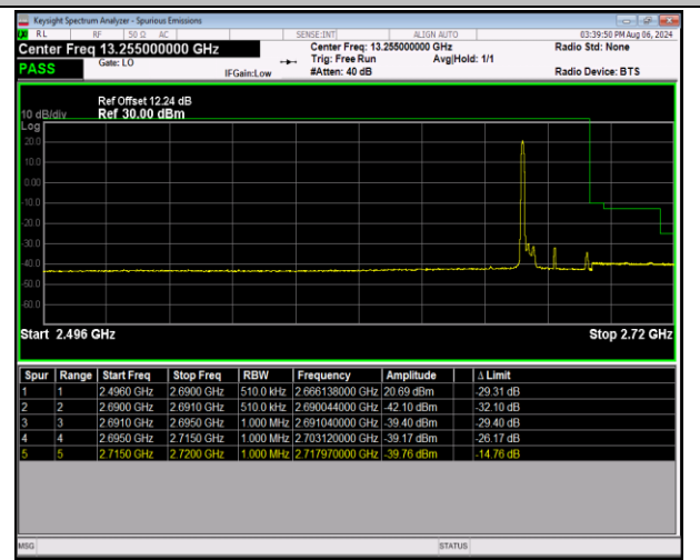
41-41-5MHz-20MHz-16QAM@16QAM-16QAM@16QAM-4 1373-41490-1RB#0@25RB#0-ORB#0@100RB#0-PASS
