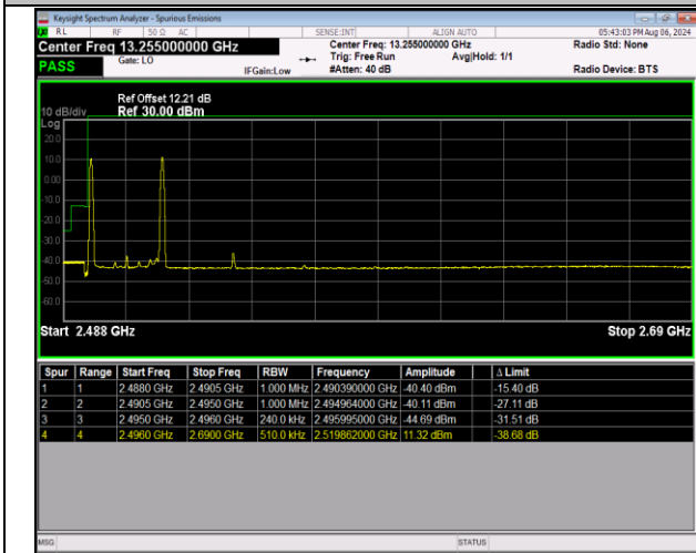
41-41-20MHz-5MHz-QPSK@QPSK-QPSK@QPSK-39750 -39867-1RB#0@100RB#0-1RB#24@25RB#0-PASS
