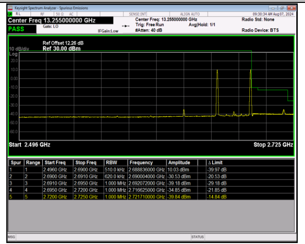
41-41-20MHz-10MHz-16QAM@16QAM-16QAM@16QAM- 41391-41535-1RB#0@100RB#0-1RB#49@50RB#0-PASS
