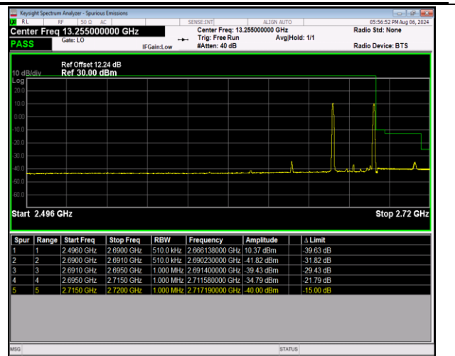
41-41-20MHz-5MHz-16QAM@16QAM-16QAM@16QAM-4 1440-41557-1RB#0@100RB#0-1RB#24@25RB#0-PASS
