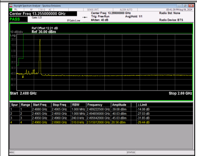
41-41-20MHz-5MHz-16QAM@16QAM-16QAM@16QAM-3 9750-39867-1RB#99@100RB#0-0RB#0@25RB#0-PASS
