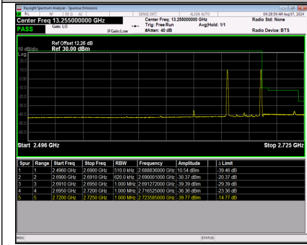
41-41-20MHz-10MHz-QPSK@QPSK-QPSK@QPSK-4139 1-41535-1RB#0@100RB#0-1RB#49@50RB#0-PASS
