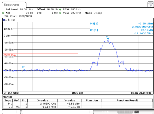
BLE_2M_Low_Channel
