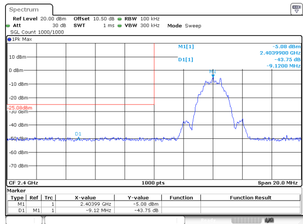
BLE_2M_Low_Channel
