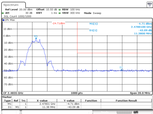
BLE_2M_High_Channel
