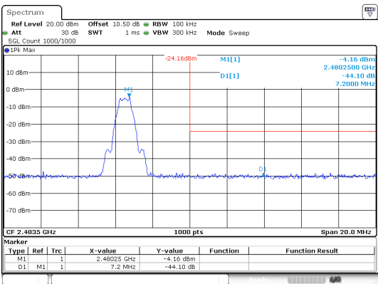
BLE_1M_High_Channel
