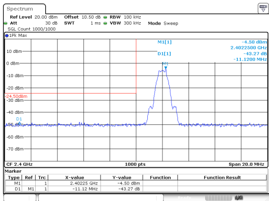
BLE_1M_Low_Channel
