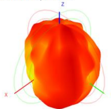
5850.0MHz H+V, Eff: 35.26%
