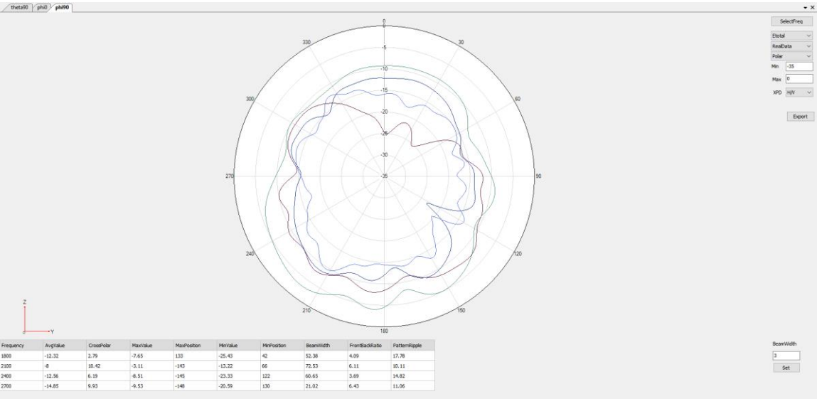
WCDMA B1/B4/LTE B1/B4/B7/B38/B41NR n1/n7/n38/n41 Phi=90deg
