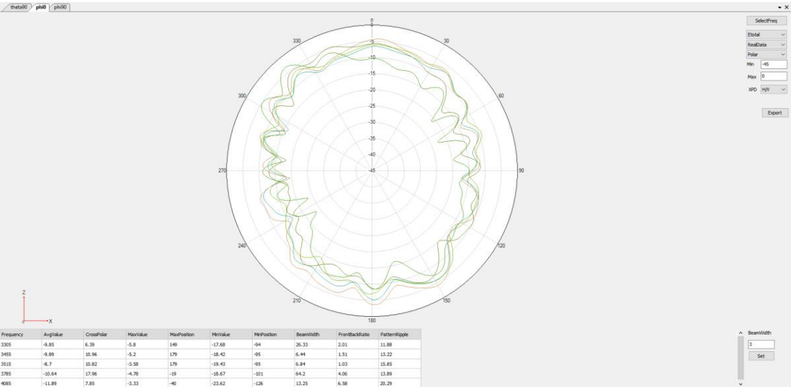
LTEB42NRn77/78Phi=0deg
