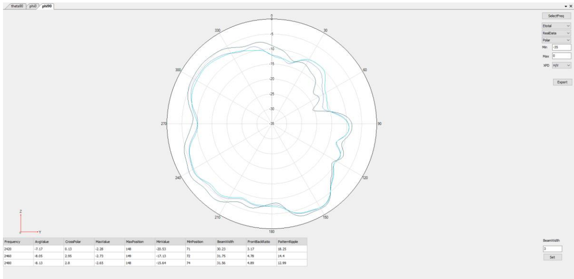
WIFI2.4 Phi=90deg
